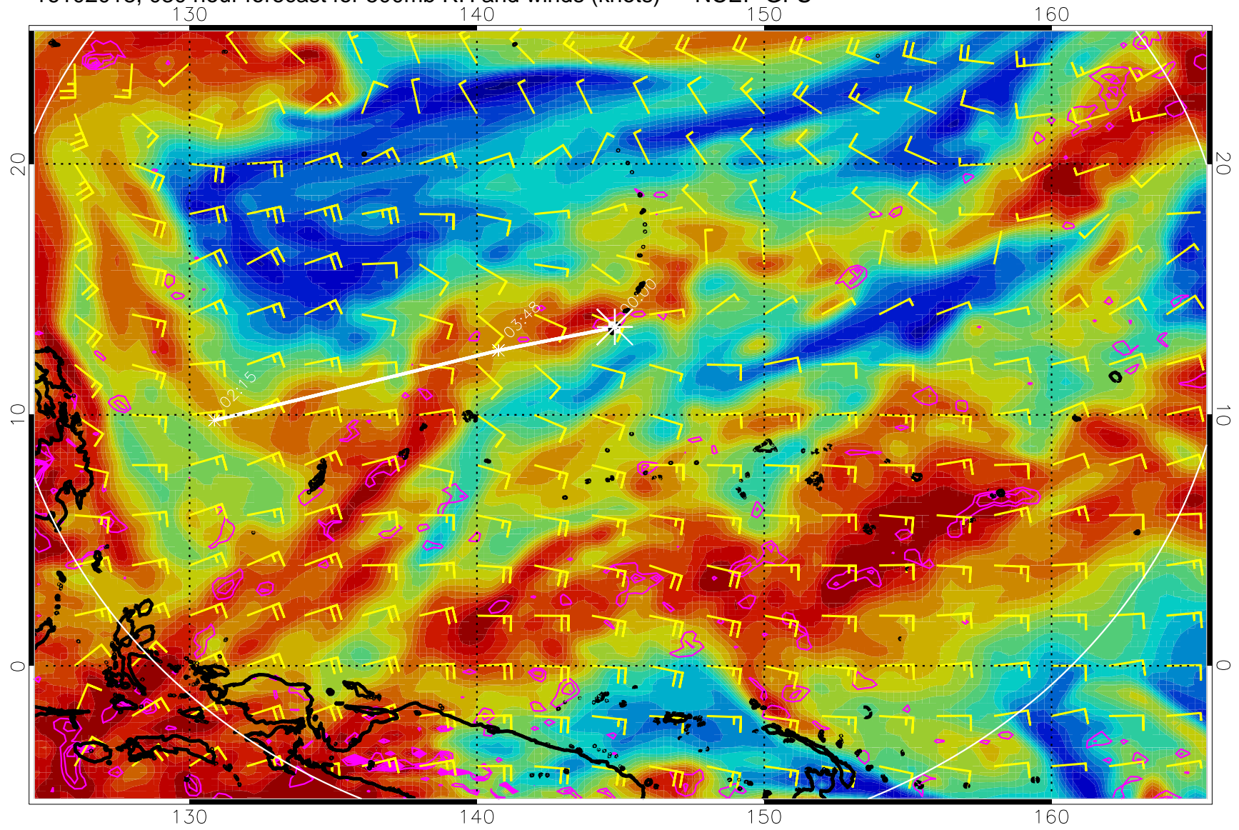
16102018, 030 hour forecast for 500mb RH and winds (knots) -- NCEP GFS
