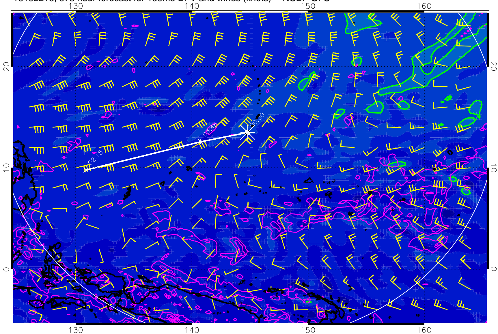
16102218, 078 hour forecast for 150mb EPV and winds (knots) -- NCEP GFS
