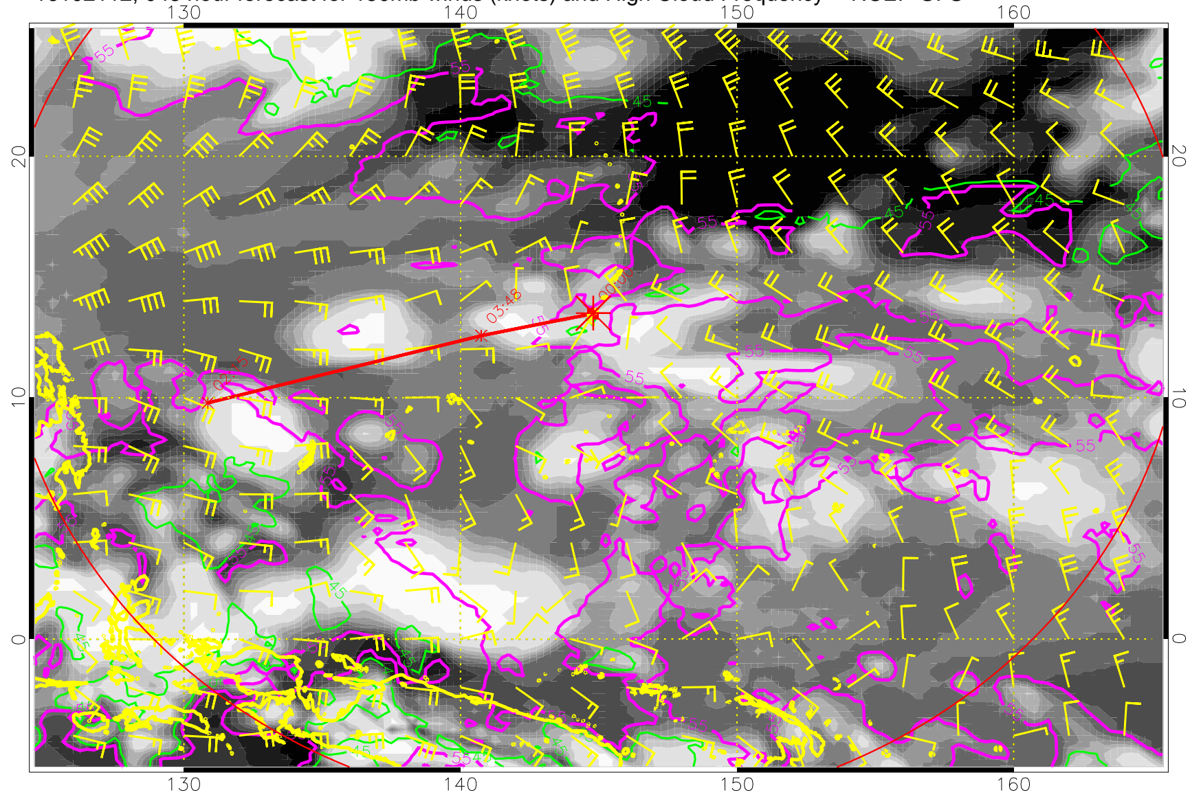
16102112, 048 hour forecast for 150mb winds (knots) and High Cloud Frequency -- NCEP GFS
