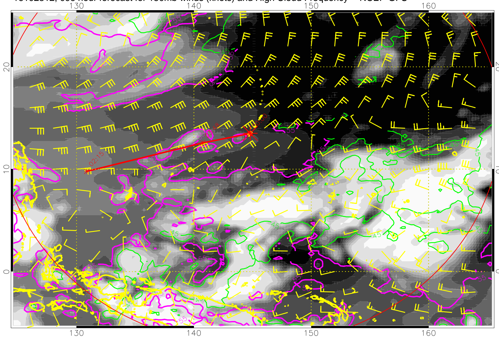
16102312, 096 hour forecast for 150mb winds (knots) and High Cloud Frequency -- NCEP GFS
