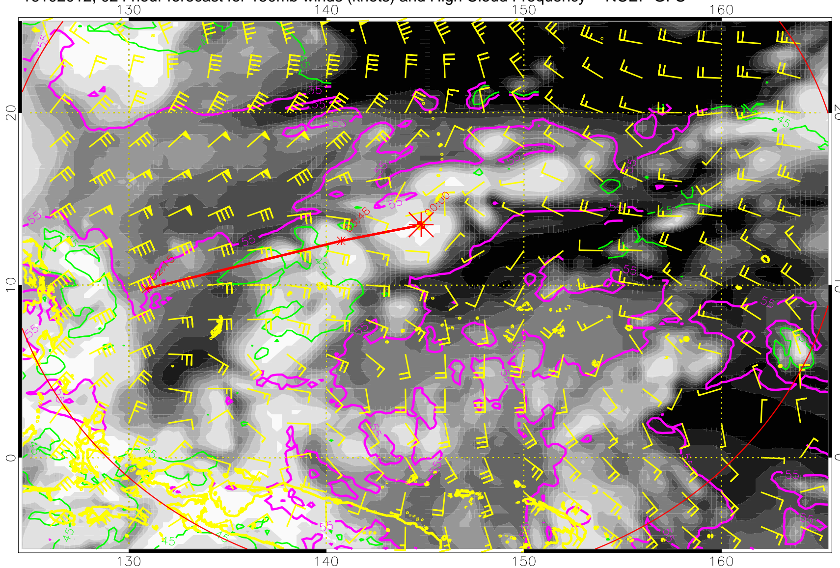
16102012, 024 hour forecast for 150mb winds (knots) and High Cloud Frequency -- NCEP GFS
