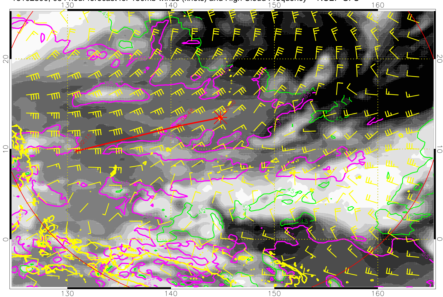
16102300, 084 hour forecast for 150mb winds (knots) and High Cloud Frequency -- NCEP GFS
