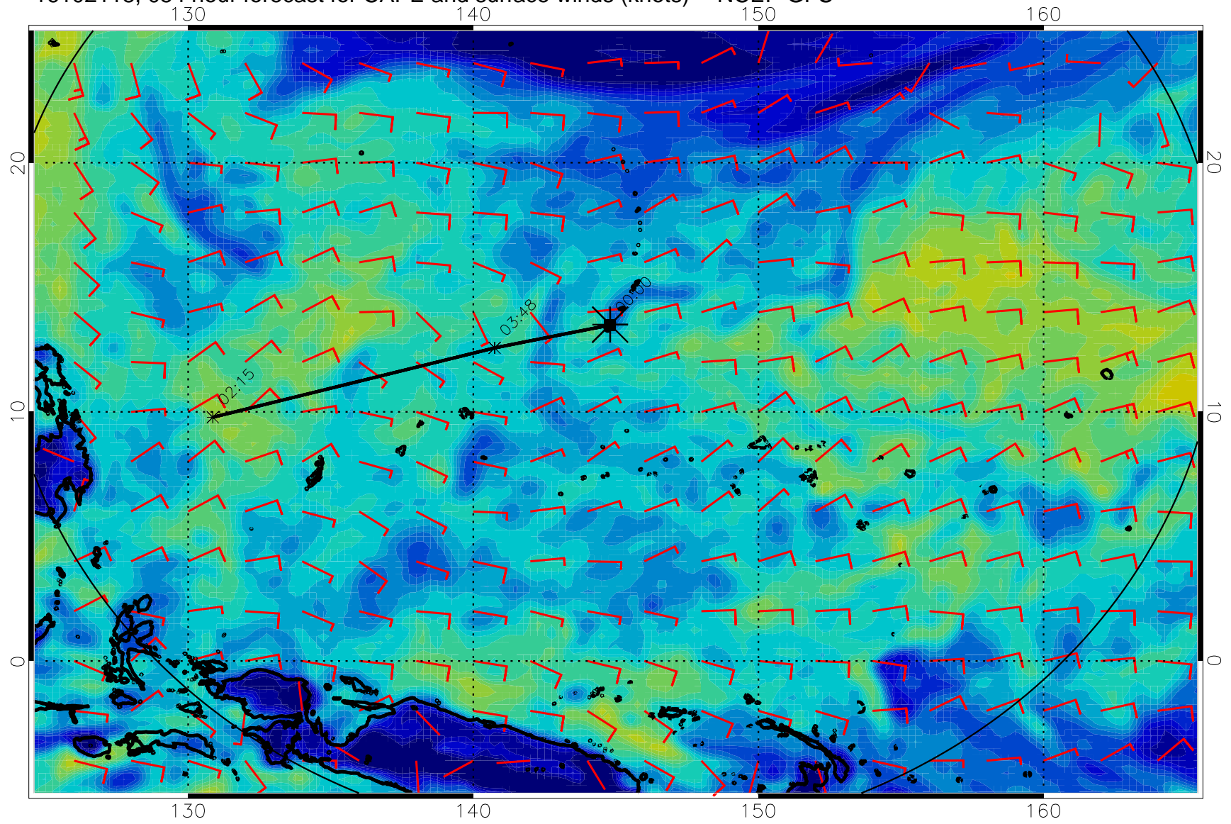
16102118, 054 hour forecast for CAPE and surface winds (knots) -- NCEP GFS
