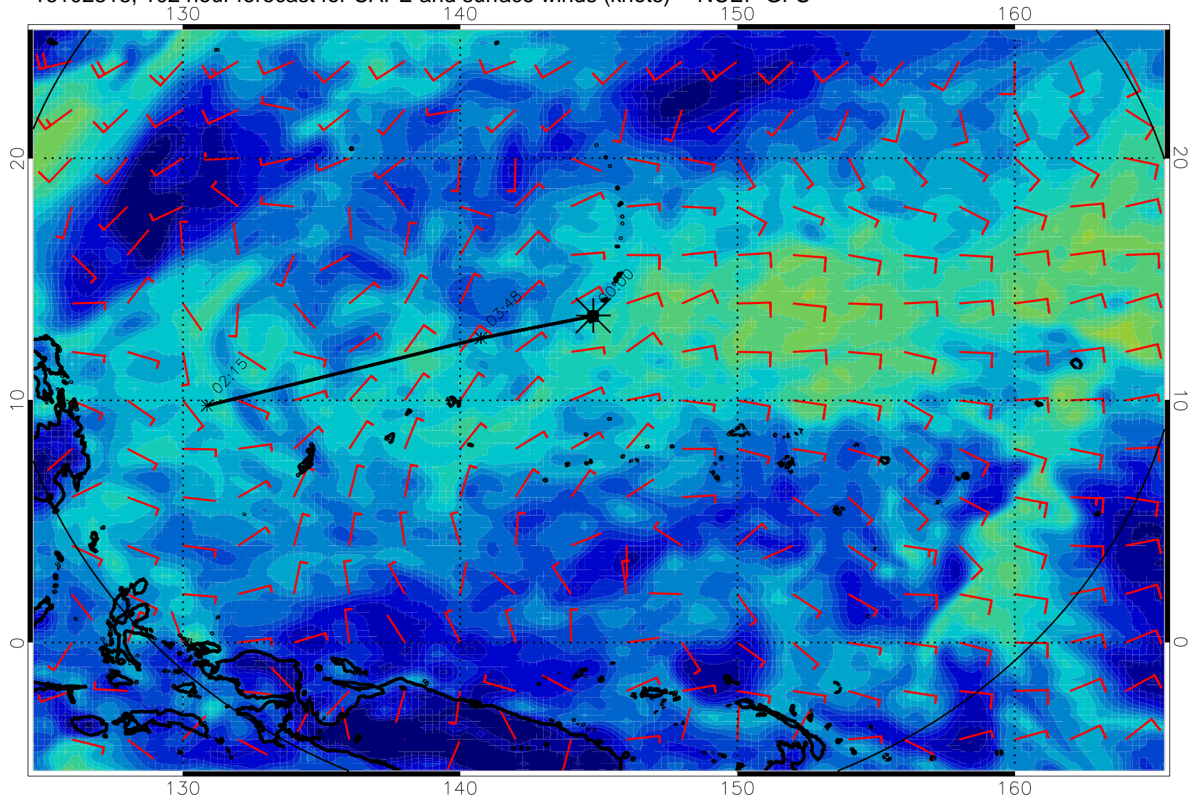
16102318, 102 hour forecast for CAPE and surface winds (knots) -- NCEP GFS
