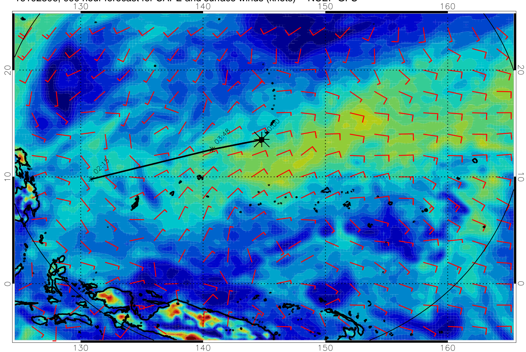
16102306, 090 hour forecast for CAPE and surface winds (knots) -- NCEP GFS
