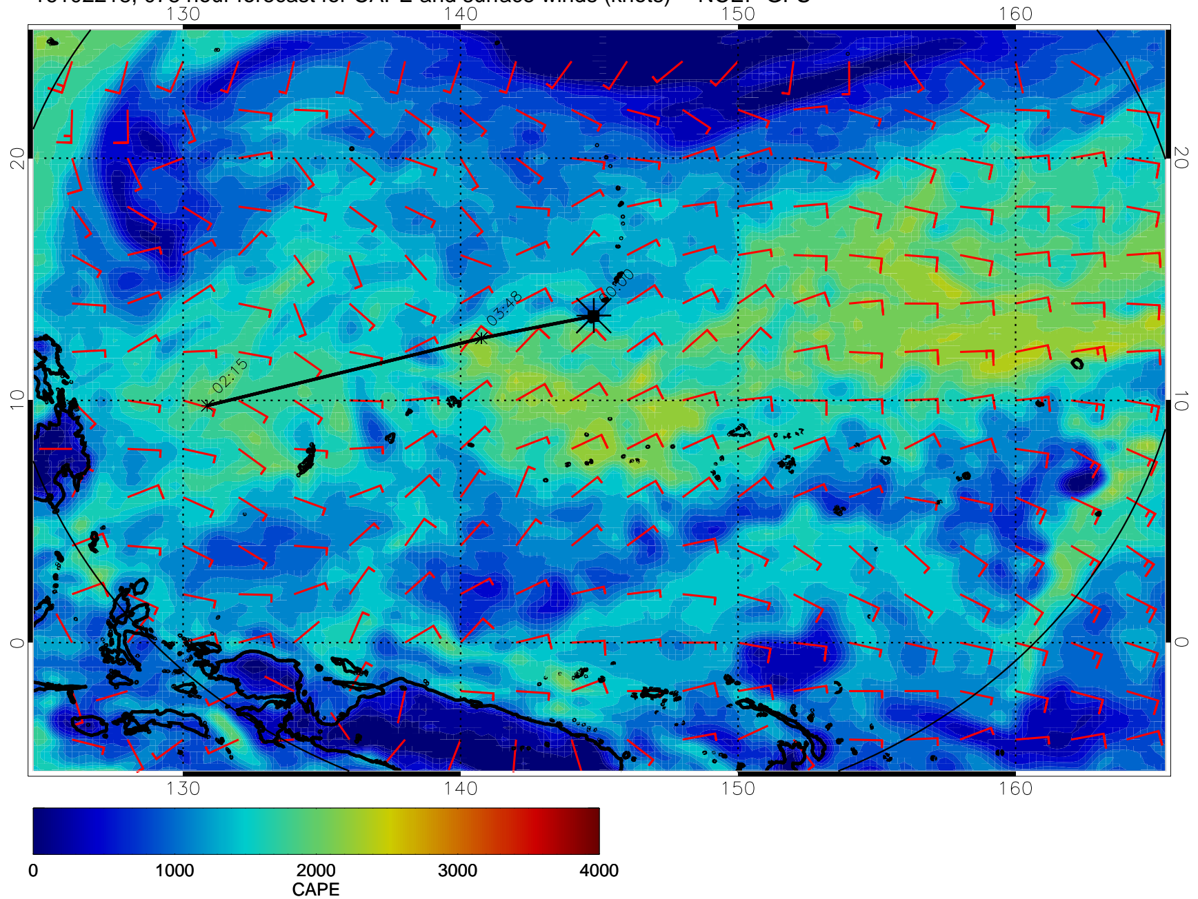
16102218, 078 hour forecast for CAPE and surface winds (knots) -- NCEP GFS
