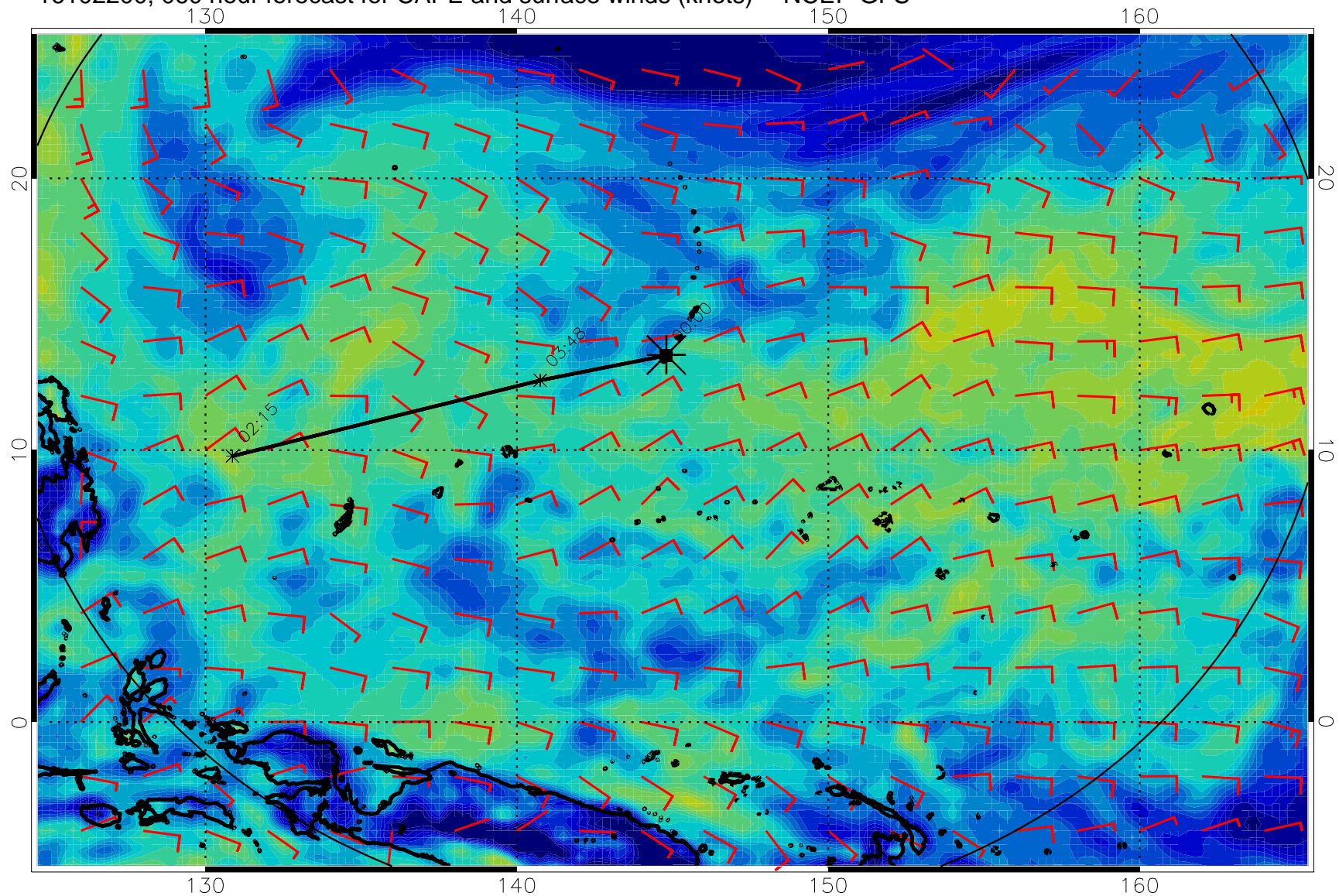
16102200, 060 hour forecast for CAPE and surface winds (knots) -- NCEP GFS
