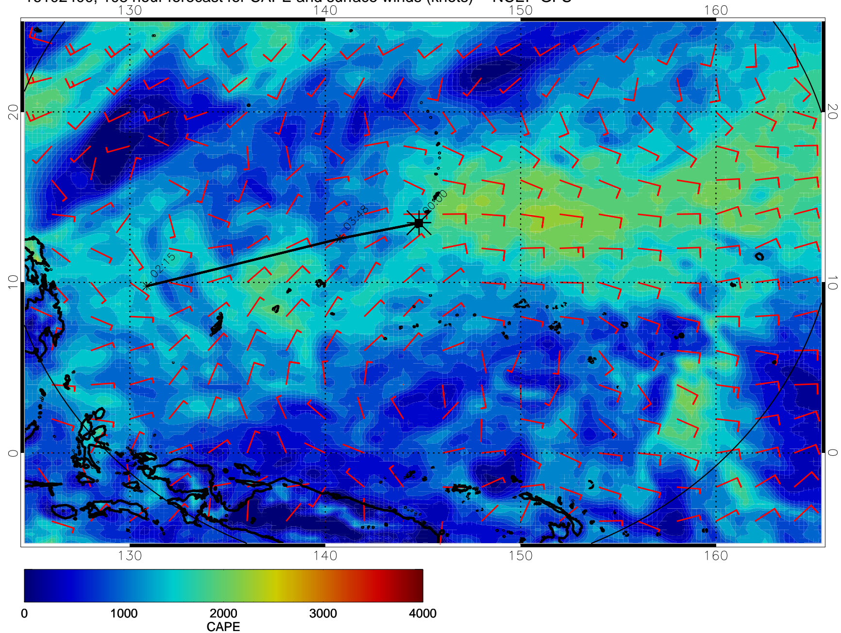
16102400, 108 hour forecast for CAPE and surface winds (knots) -- NCEP GFS
