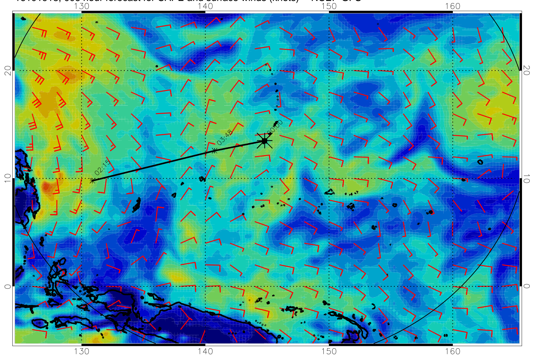
16101918, 006 hour forecast for CAPE and surface winds (knots) -- NCEP GFS
