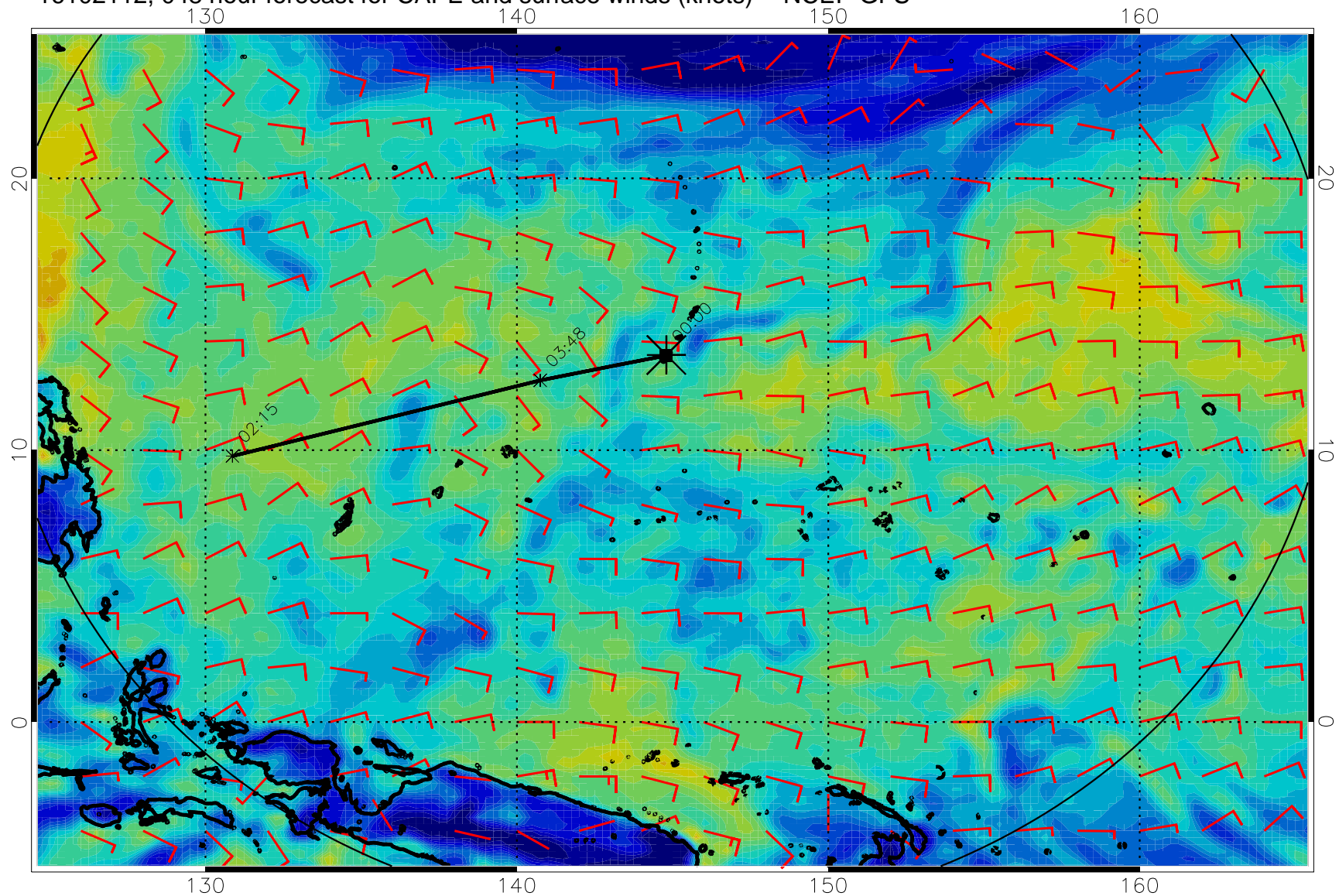
16102112, 048 hour forecast for CAPE and surface winds (knots) -- NCEP GFS
