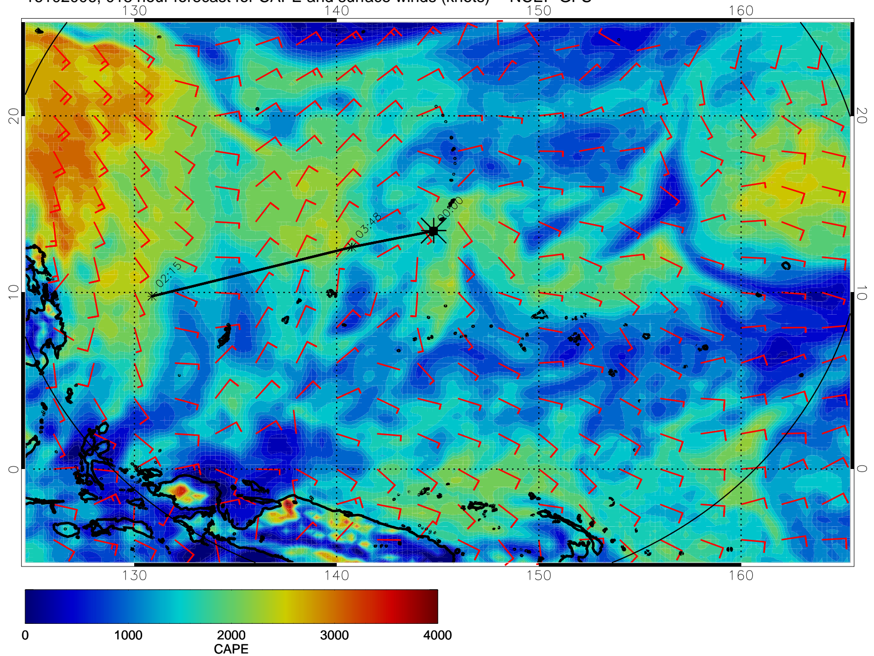
16102006, 018 hour forecast for CAPE and surface winds (knots) -- NCEP GFS
