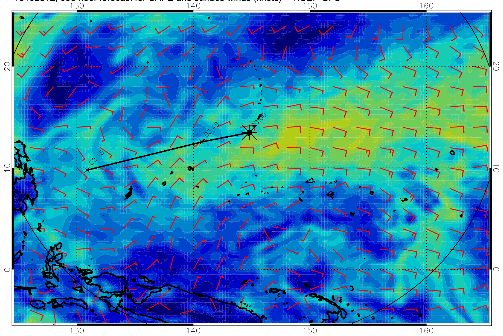
16102312, 096 hour forecast for CAPE and surface winds (knots) -- NCEP GFS
