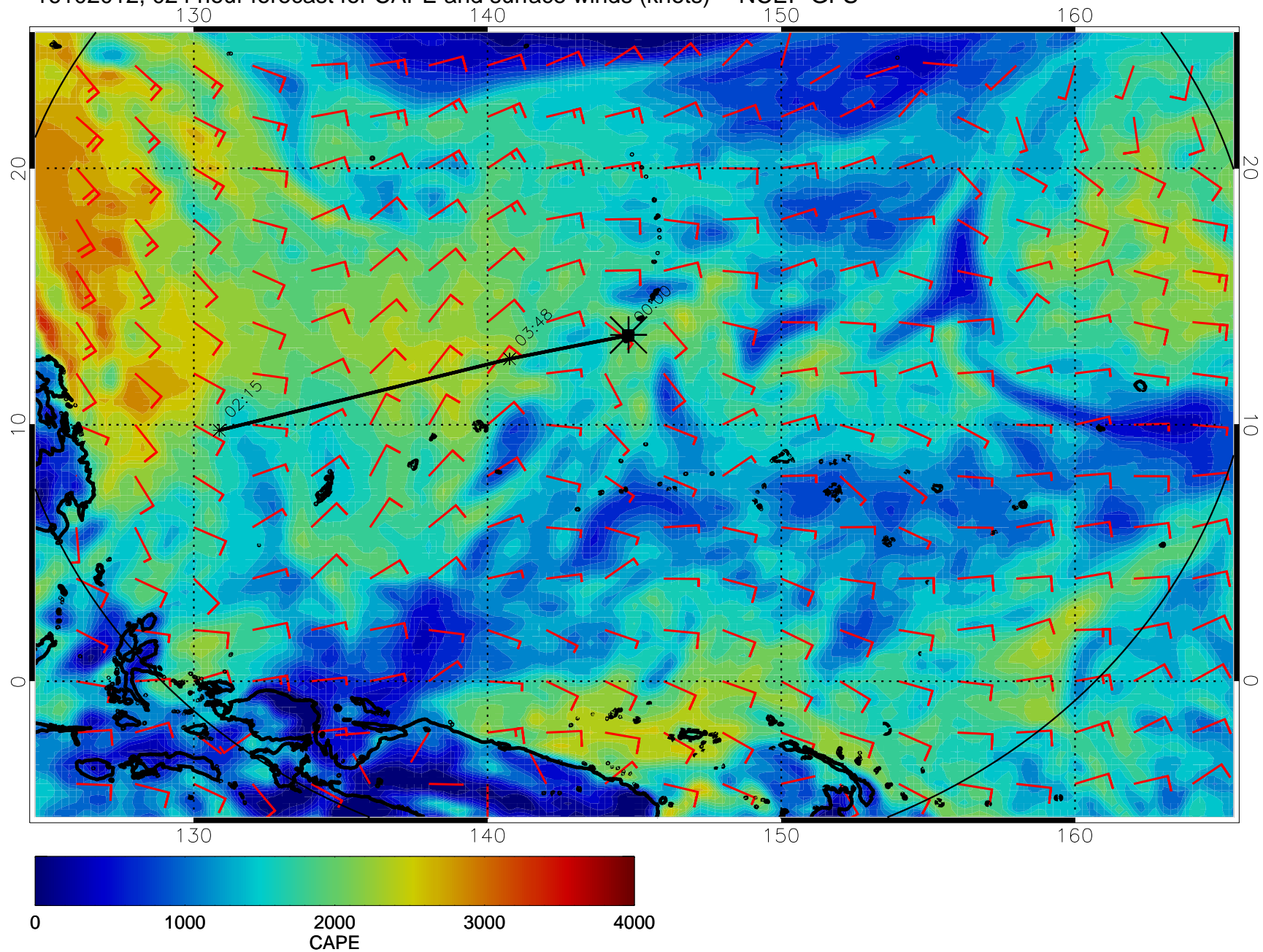
16102012, 024 hour forecast for CAPE and surface winds (knots) -- NCEP GFS
