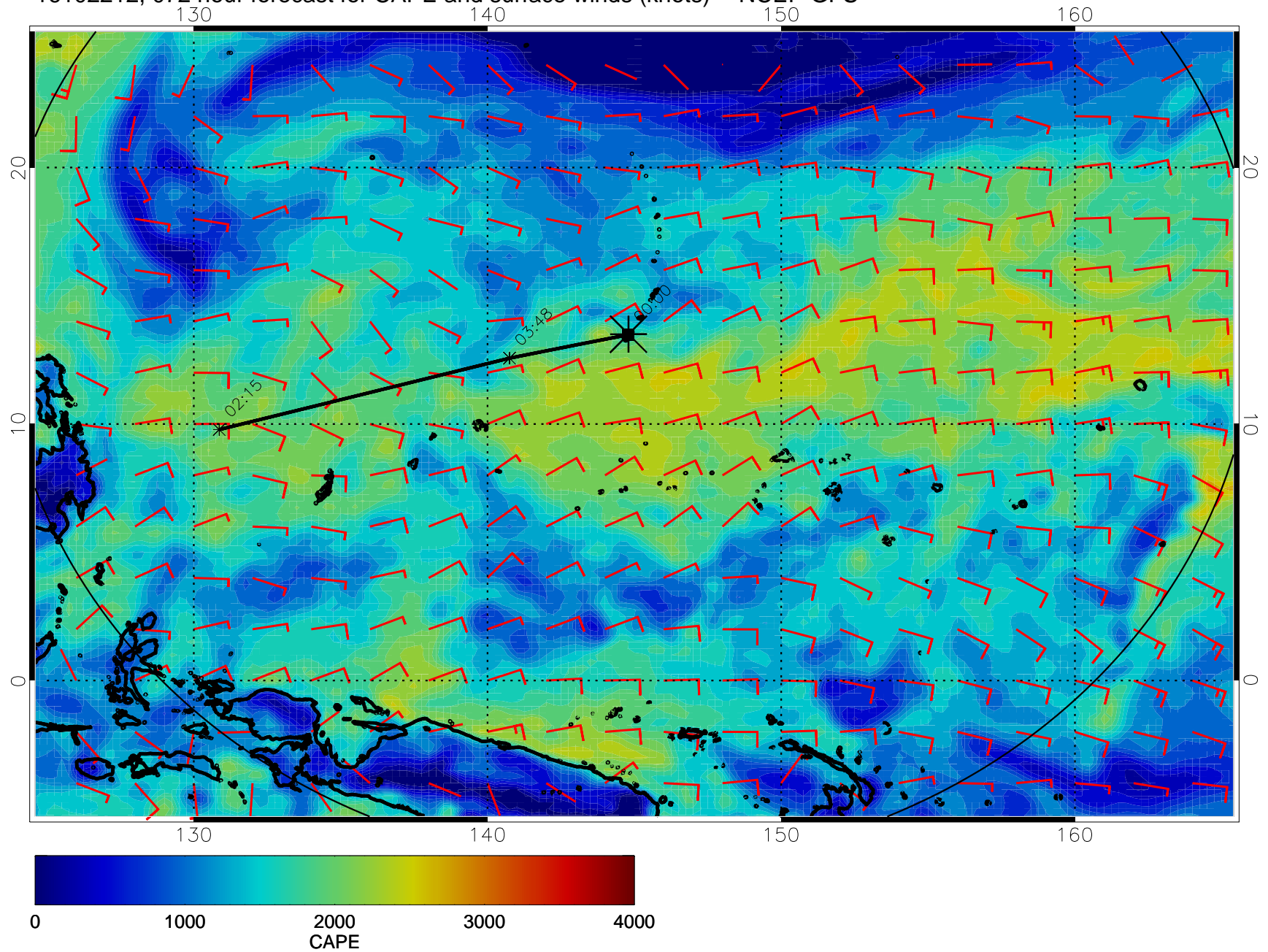
16102212, 072 hour forecast for CAPE and surface winds (knots) -- NCEP GFS
