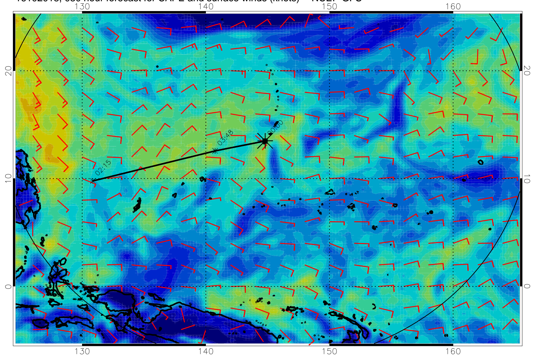
16102018, 030 hour forecast for CAPE and surface winds (knots) -- NCEP GFS
