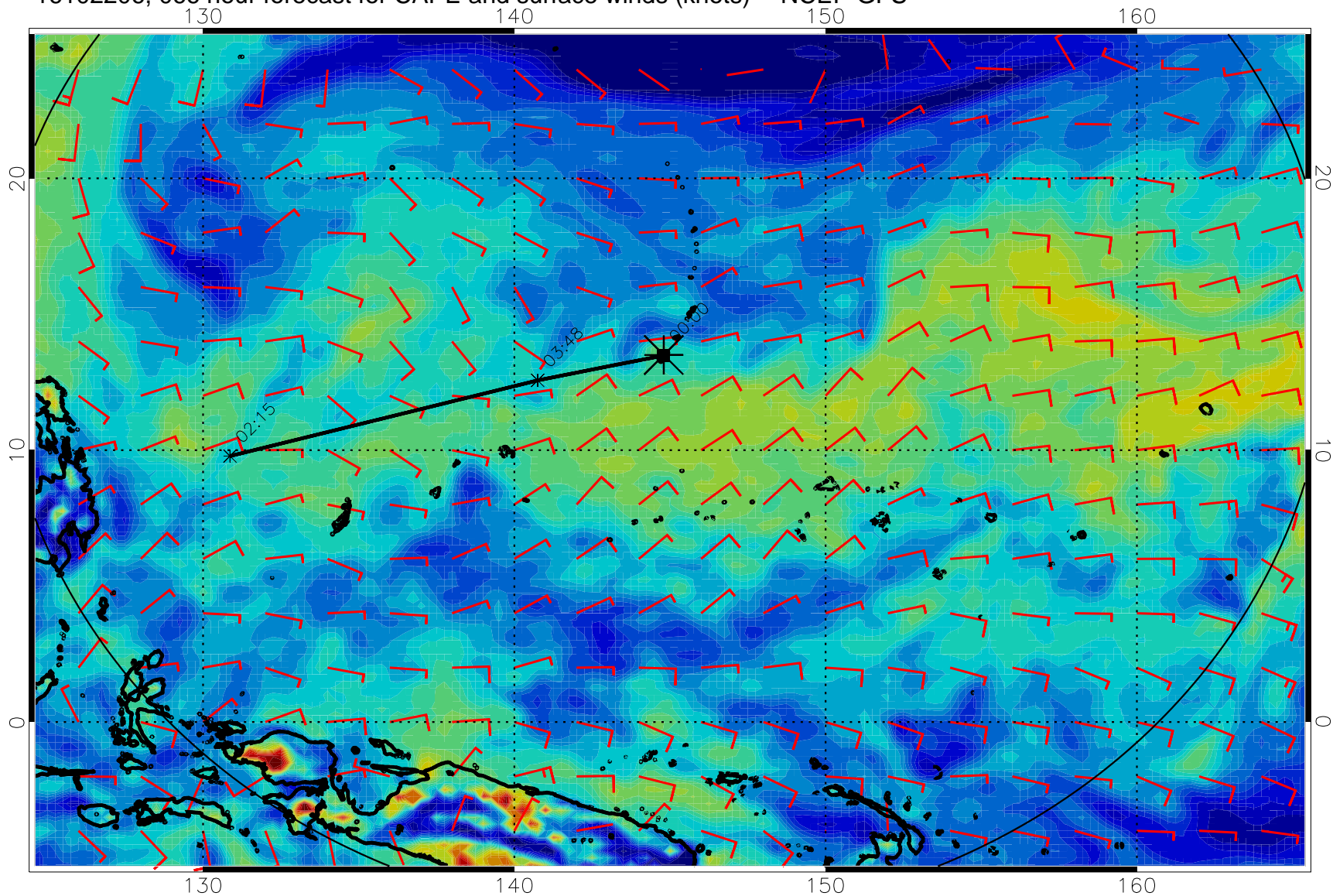
16102206, 066 hour forecast for CAPE and surface winds (knots) -- NCEP GFS
