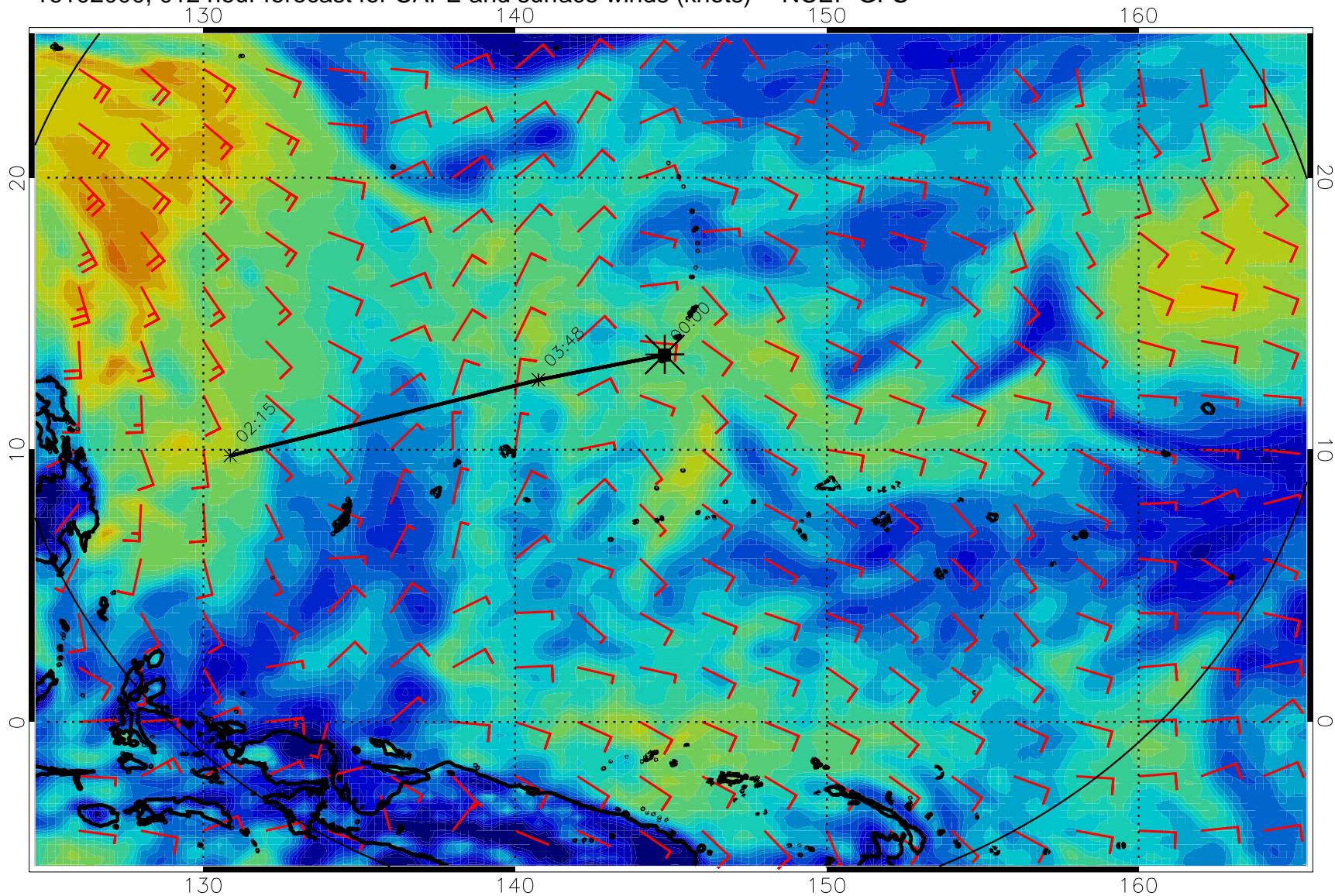
16102000, 012 hour forecast for CAPE and surface winds (knots) -- NCEP GFS
