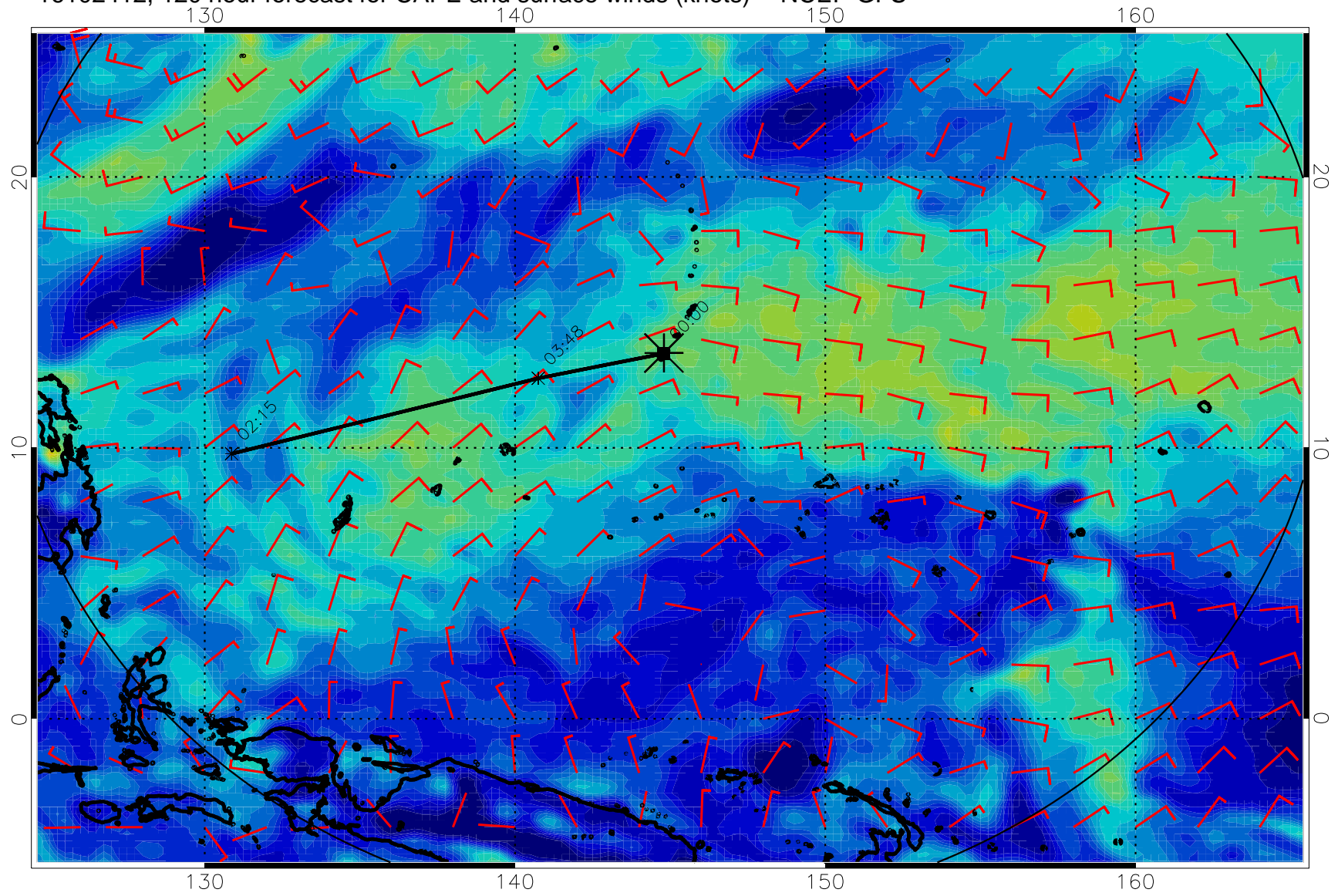
16102412, 120 hour forecast for CAPE and surface winds (knots) -- NCEP GFS
