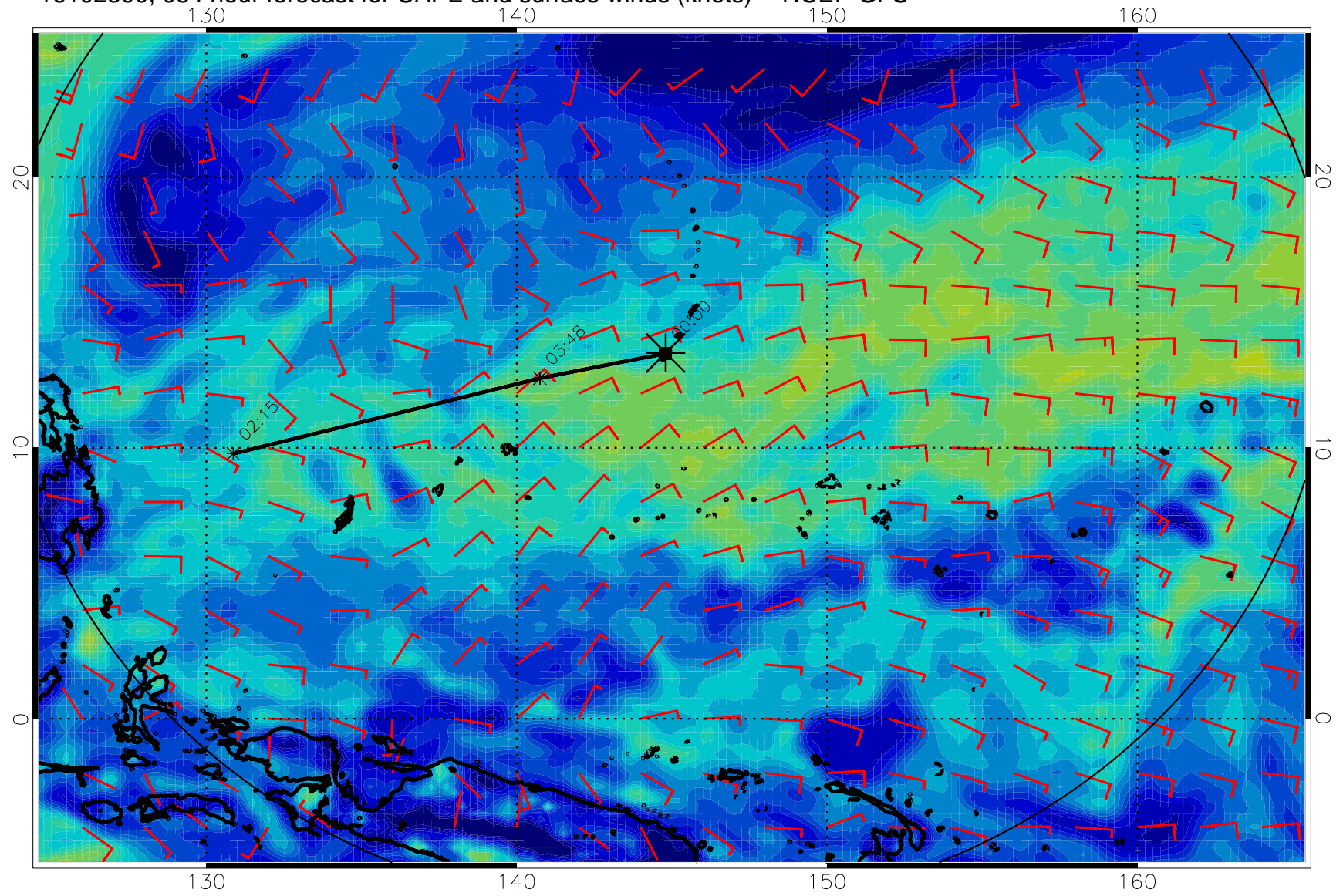
16102300, 084 hour forecast for CAPE and surface winds (knots) -- NCEP GFS
