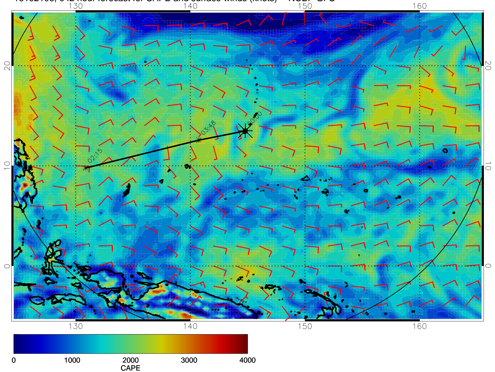
16102106, 042 hour forecast for CAPE and surface winds -- NCEP GFS
