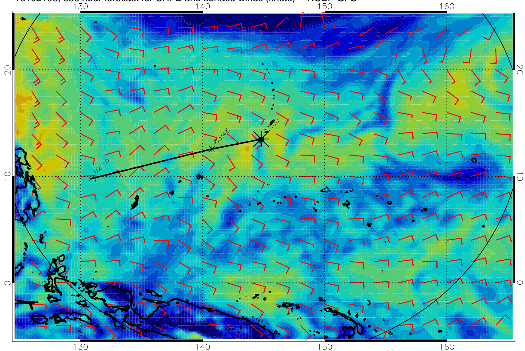
16102100, 036 hour forecast for CAPE and surface winds (knots) -- NCEP GFS
