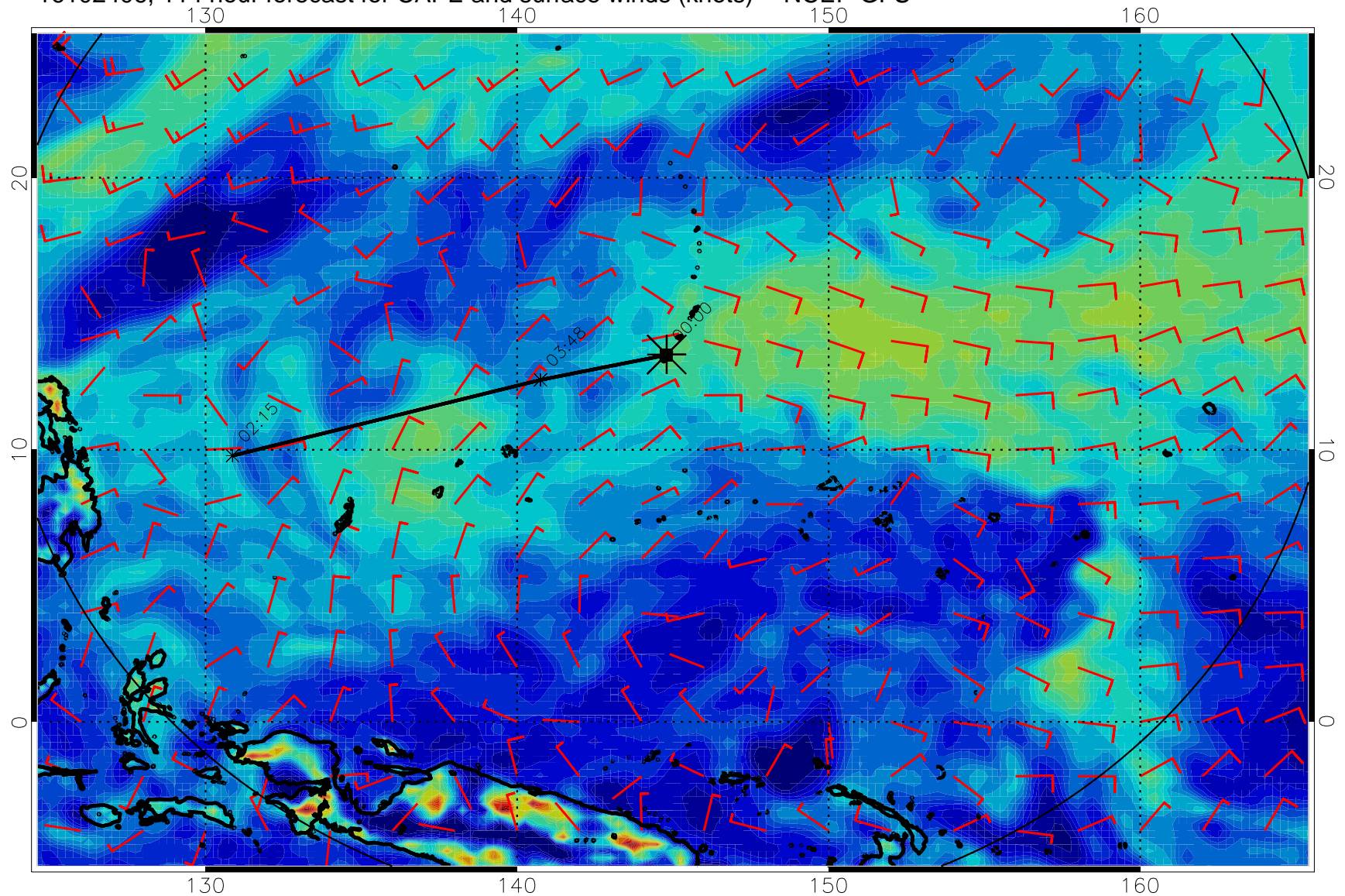
16102406, 114 hour forecast for CAPE and surface winds (knots) -- NCEP GFS
