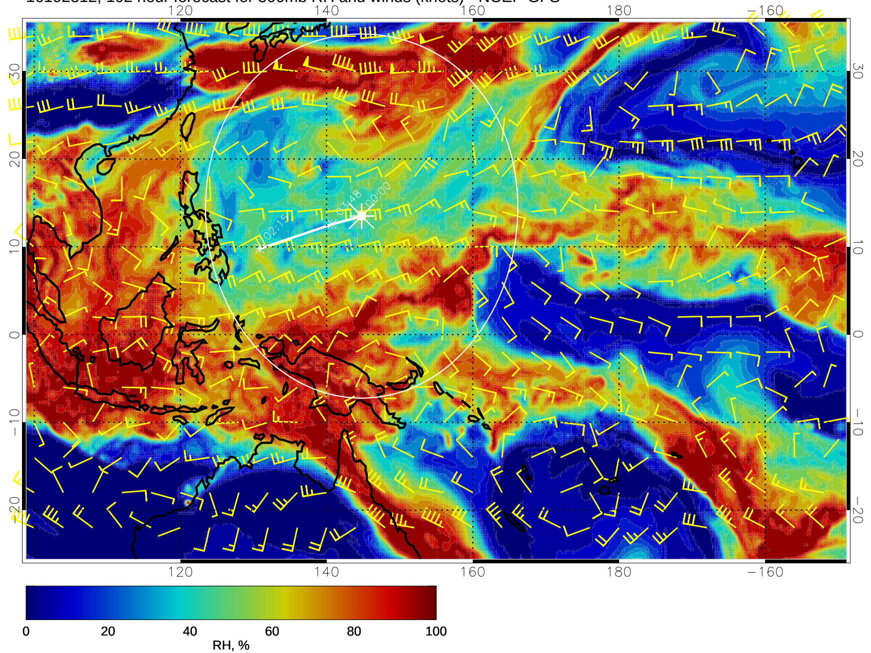
16102312, 102 hour forecast for 500mb RH and winds (knots) - NCEP GFS
