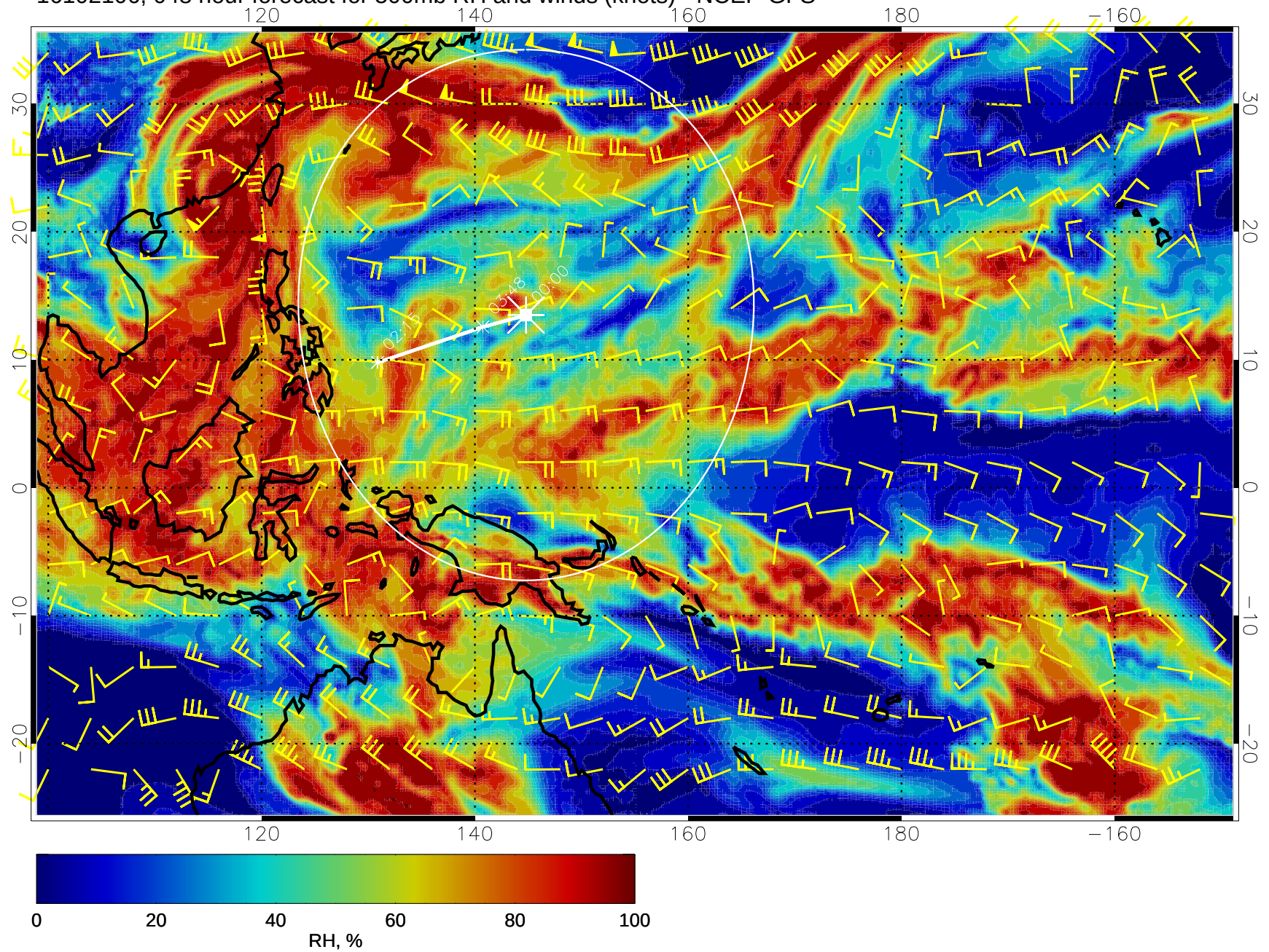
16102106, 048 hour forecast for 500mb RH and winds (knots) - NCEP GFS
