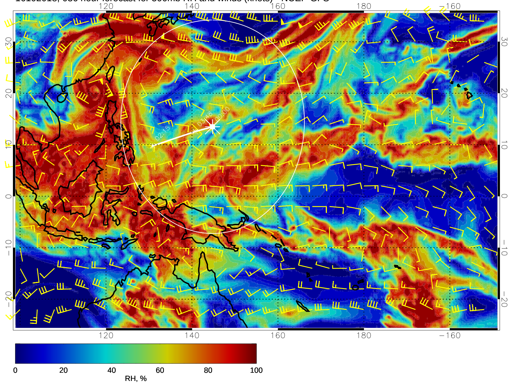
16102018, 036 hour forecast for 500mb RH and winds (knots) - NCEP GFS
