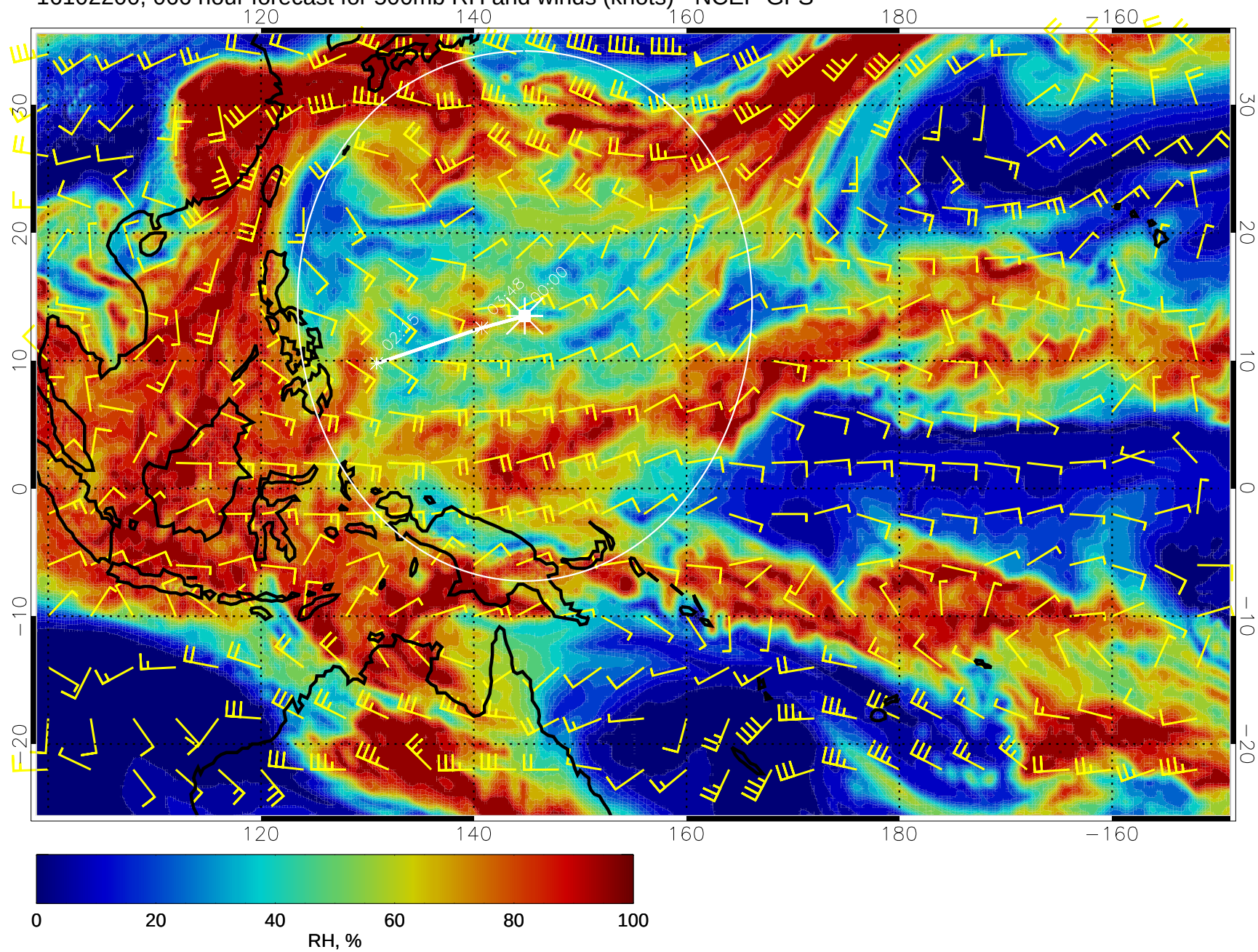
16102200, 066 hour forecast for 500mb RH and winds (knots) - NCEP GFS
