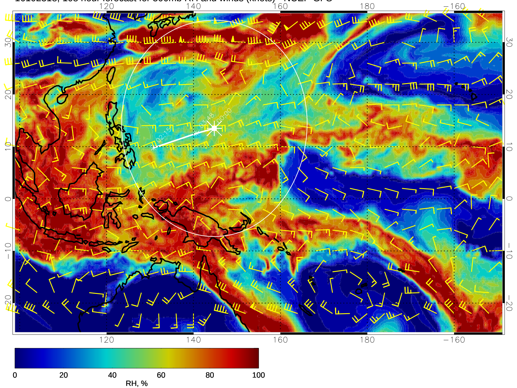
16102318, 108 hour forecast for 500mb RH and winds (knots) - NCEP GFS
