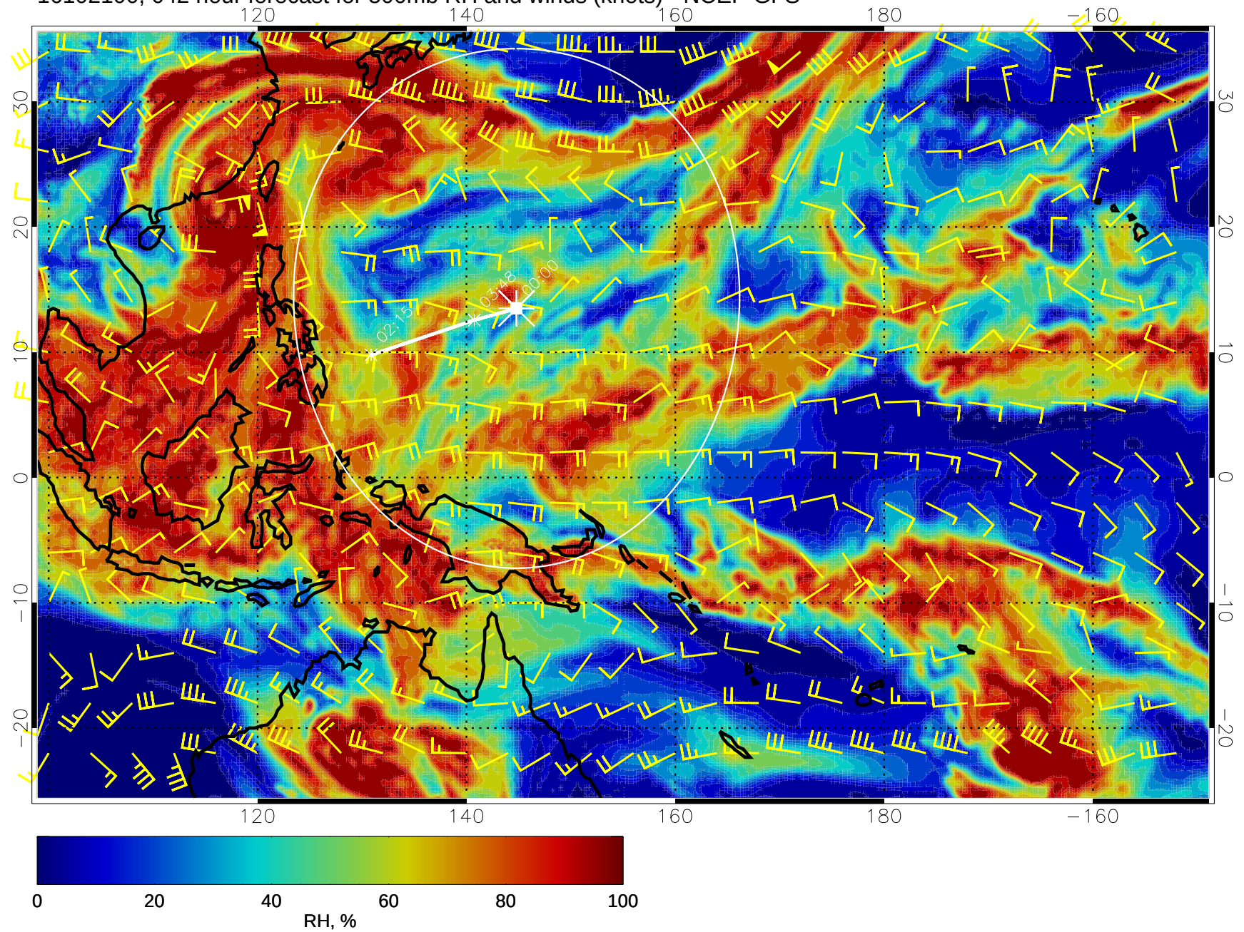
16102100, 042 hour forecast for 500mb RH and winds (knots) - NCEP GFS
