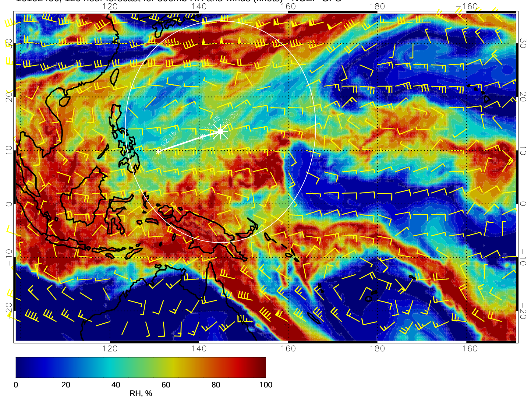
16102406, 120 hour forecast for 500mb RH and winds (knots) - NCEP GFS
