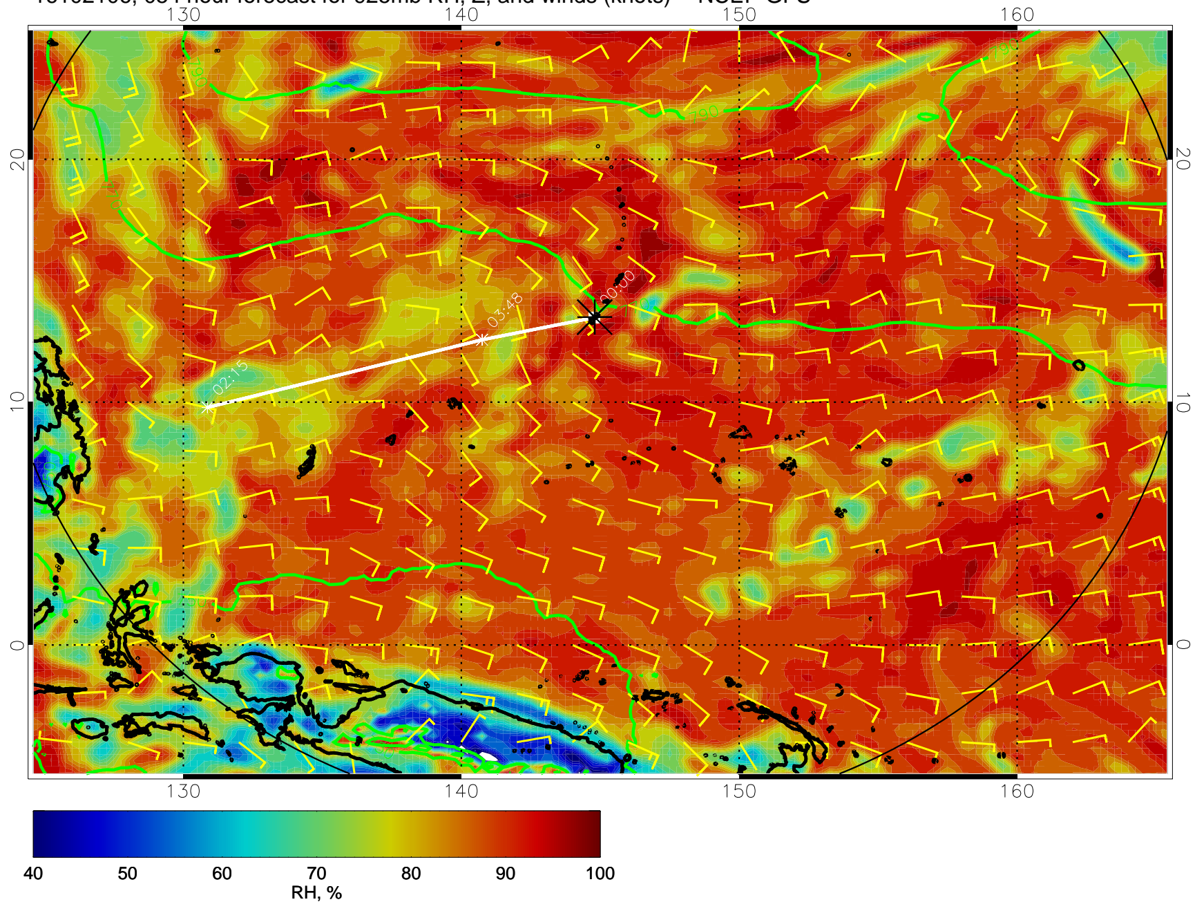
16102106, 054 hour forecast for 925mb RH, Z, and winds (knots) -- NCEP GFS
