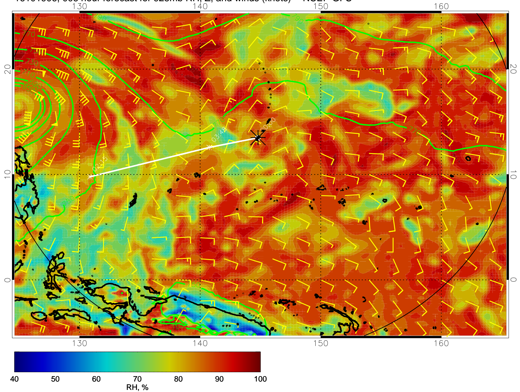
16101906, 006 hour forecast for 925mb RH, Z, and winds (knots) -- NCEP GFS
