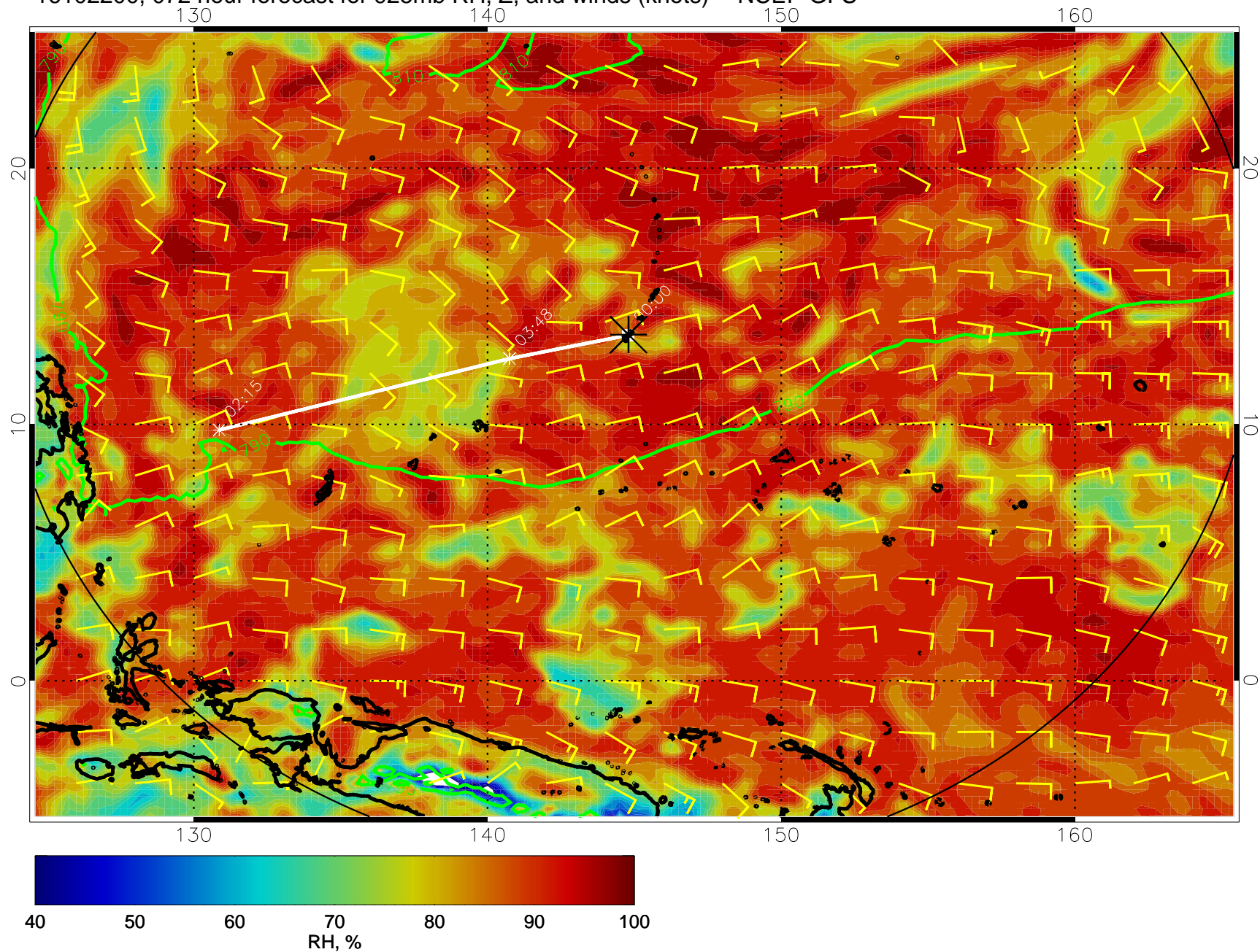
16102200, 072 hour forecast for 925mb RH, Z, and winds (knots) -- NCEP GFS
