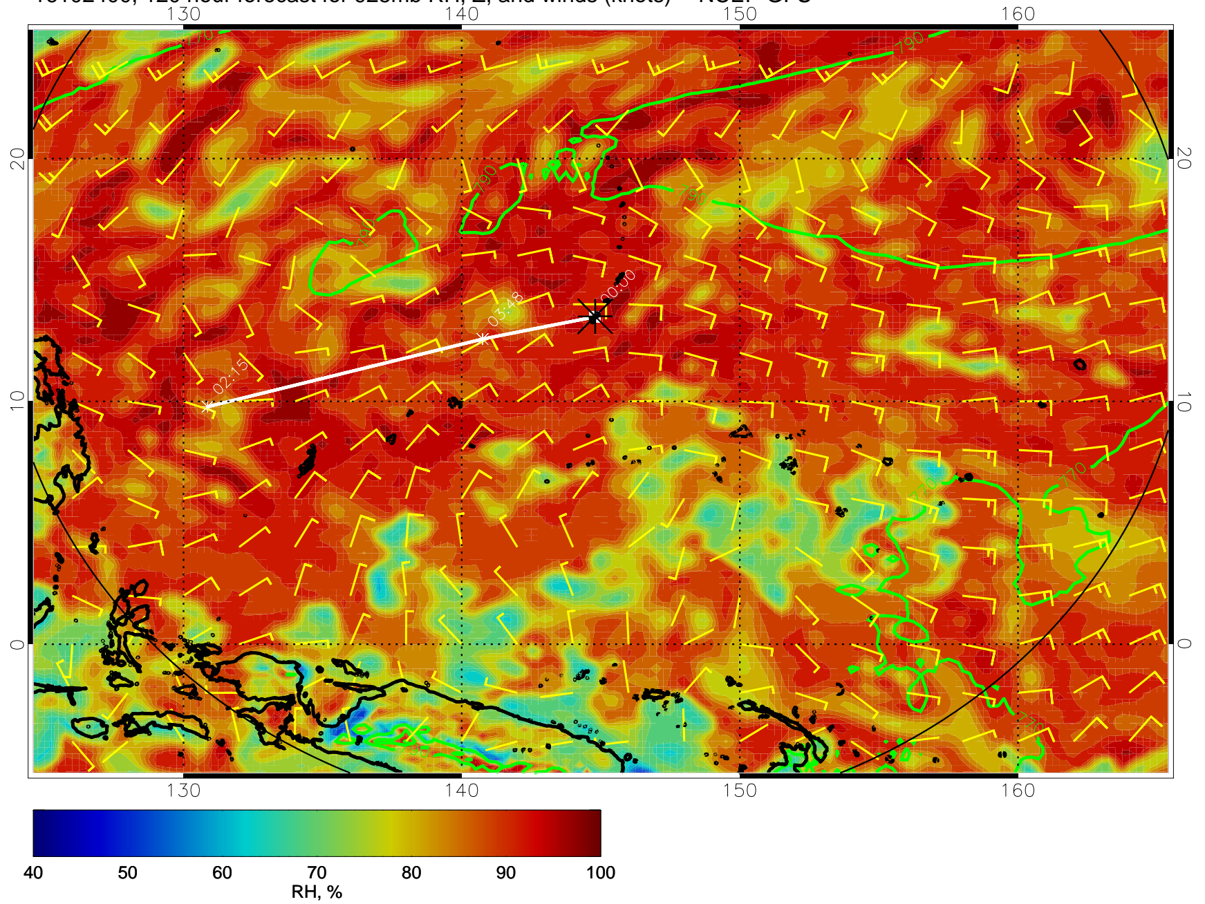
16102400, 120 hour forecast for 925mb RH, Z, and winds (knots) -- NCEP GFS
