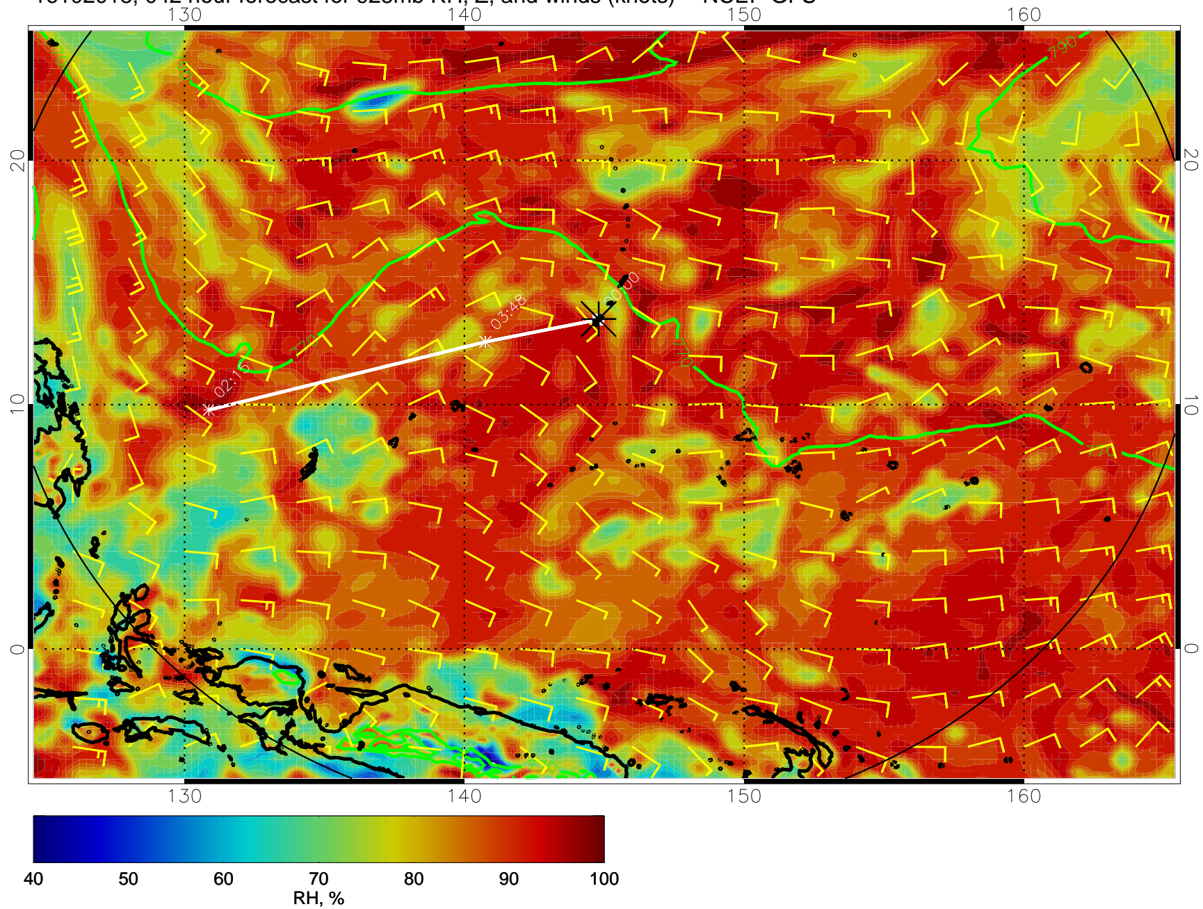
16102018, 042 hour forecast for 925mb RH, Z, and winds (knots) -- NCEP GFS
