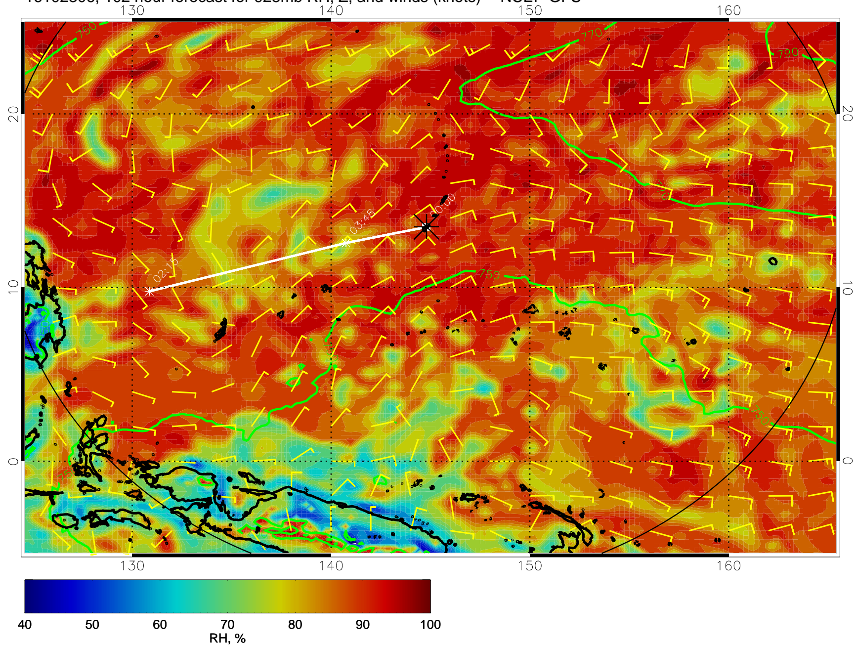
16102306, 102 hour forecast for 925mb RH, Z, and winds (knots) -- NCEP GFS
