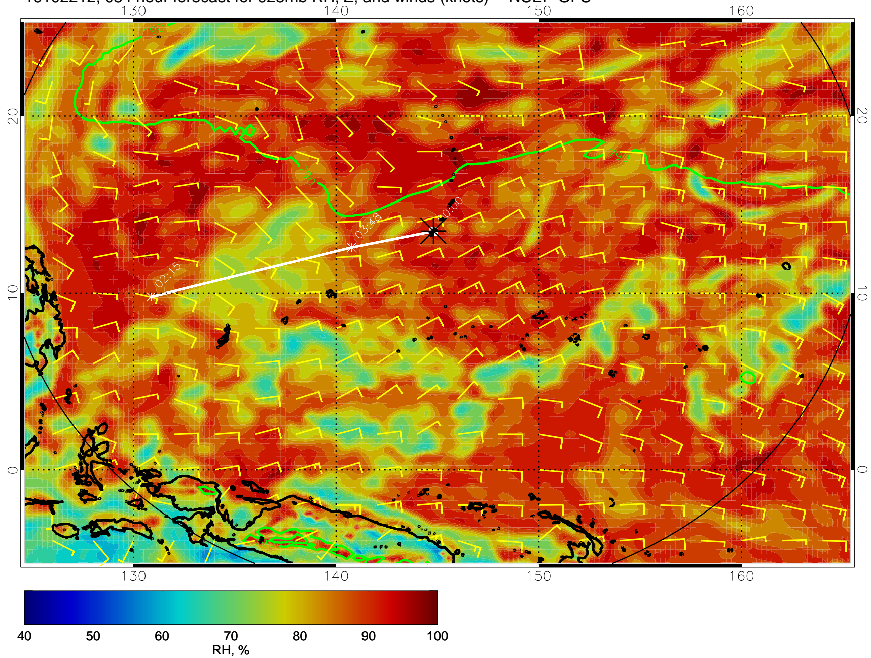
16102212, 084 hour forecast for 925mb RH, Z, and winds (knots) -- NCEP GFS
