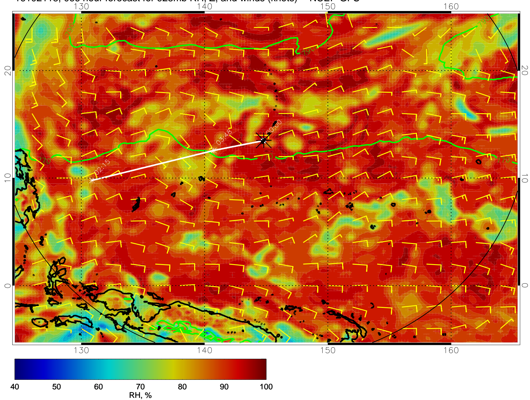
16102118, 066 hour forecast for 925mb RH, Z, and winds (knots) -- NCEP GFS
