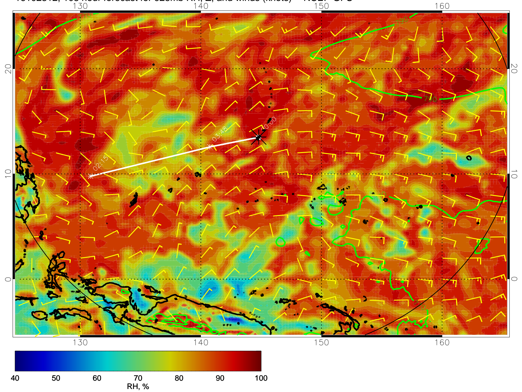
16102312, 108 hour forecast for 925mb RH, Z, and winds (knots) -- NCEP GFS
