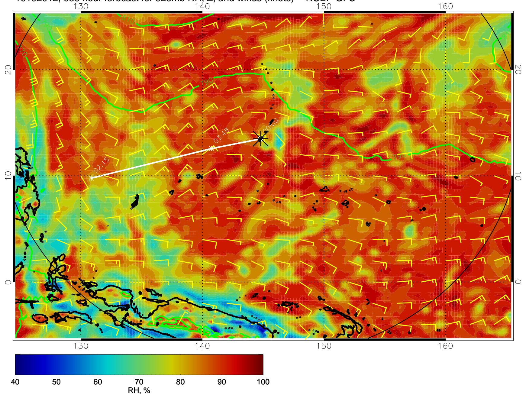
16102012, 036 hour forecast for 925mb RH, Z, and winds (knots) -- NCEP GFS
