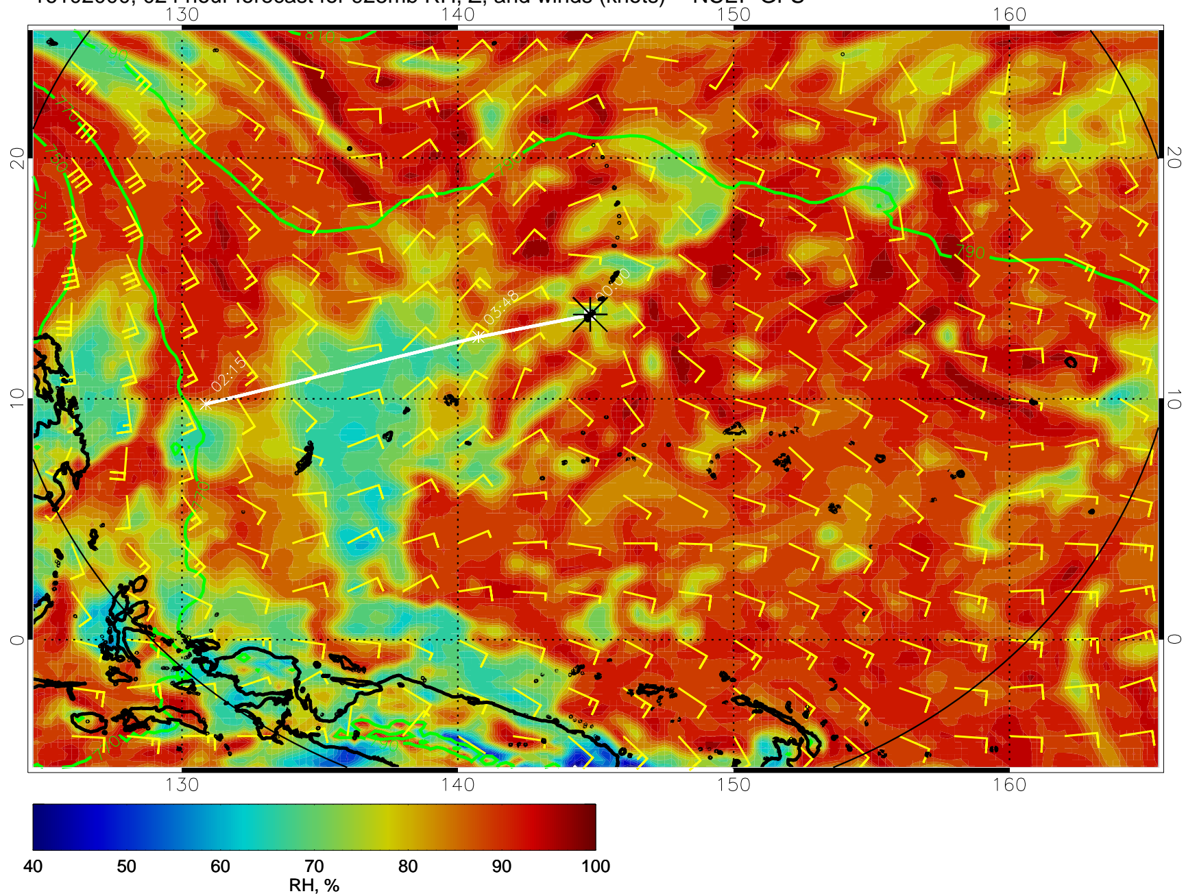
16102000, 024 hour forecast for 925mb RH, Z, and winds (knots) -- NCEP GFS
