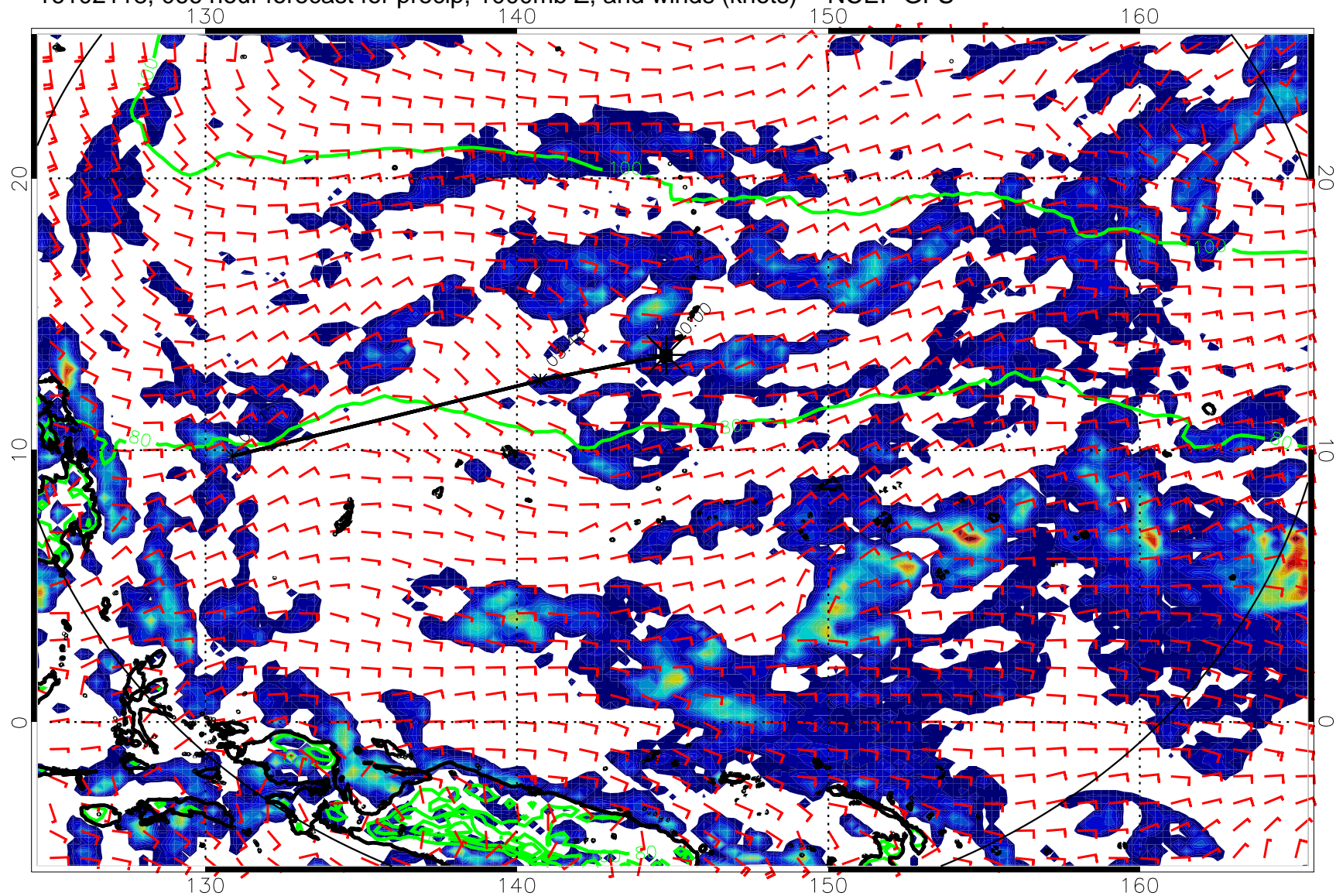
16102118, 066 hour forecast for precip, 1000mb Z, and winds (knots) -- NCEP GFS
