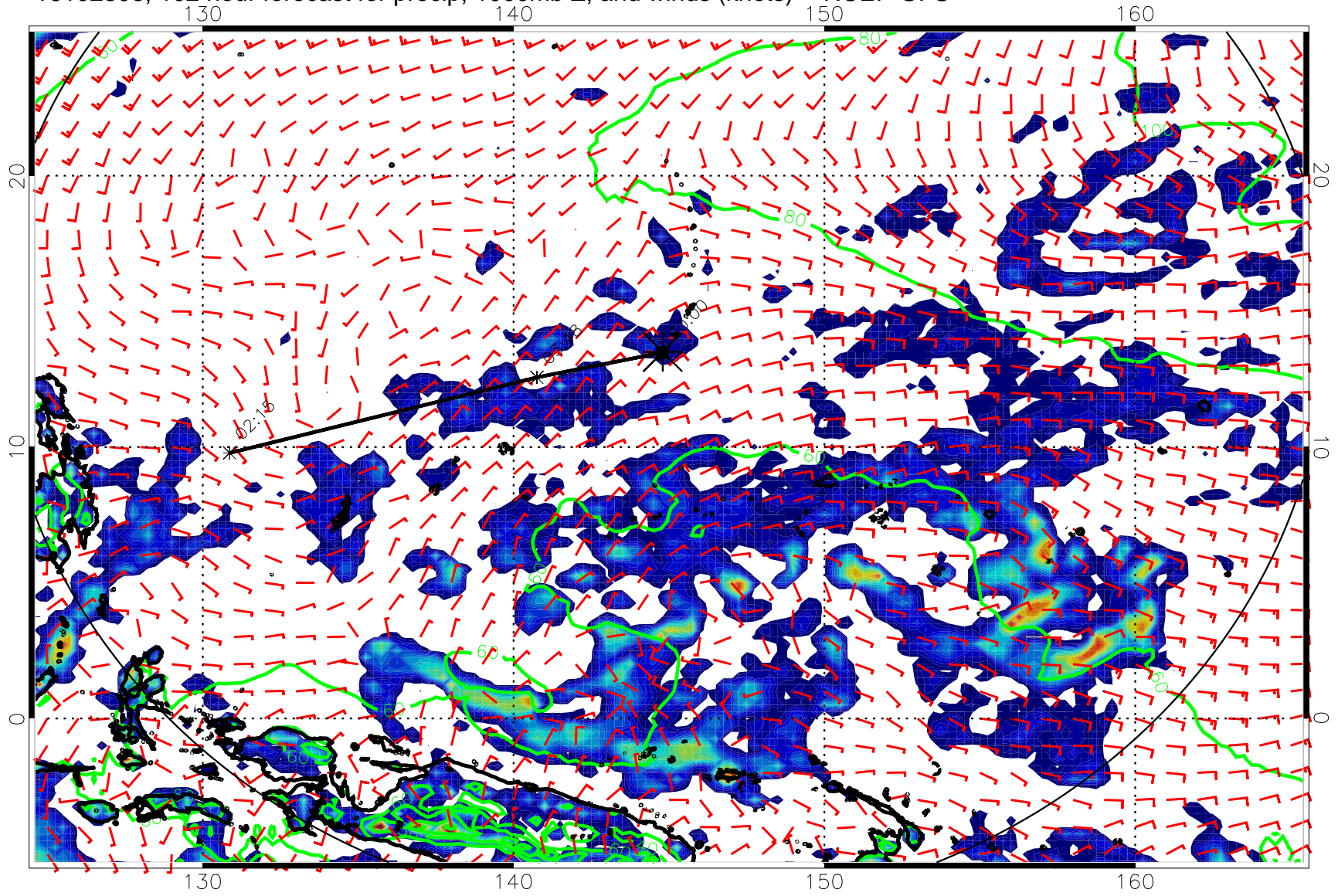
16102306, 102 hour forecast for precip, 1000mb Z, and winds (knots) -- NCEP GFS
