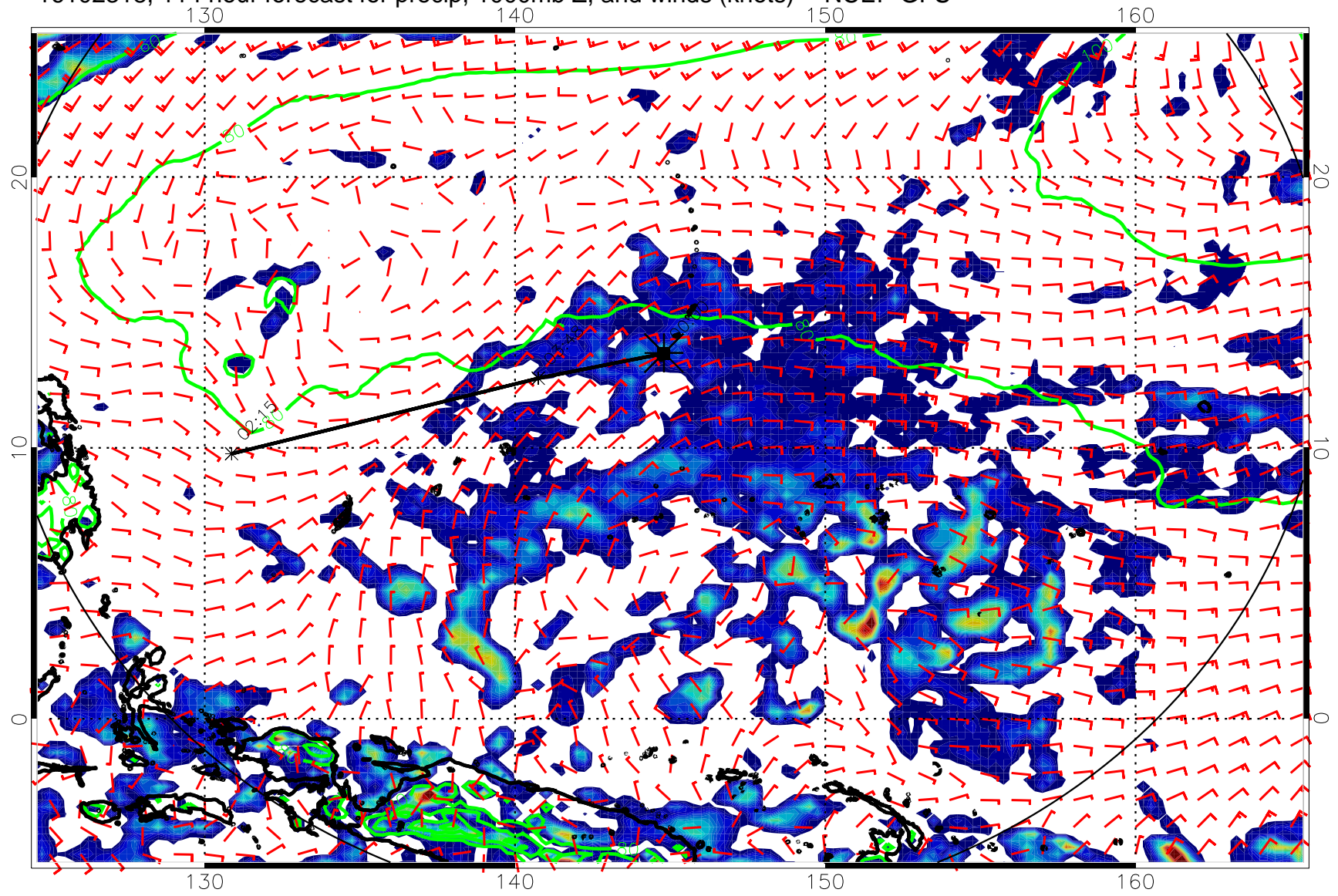
16102318, 114 hour forecast for precip, 1000mb Z, and winds (knots) -- NCEP GFS
