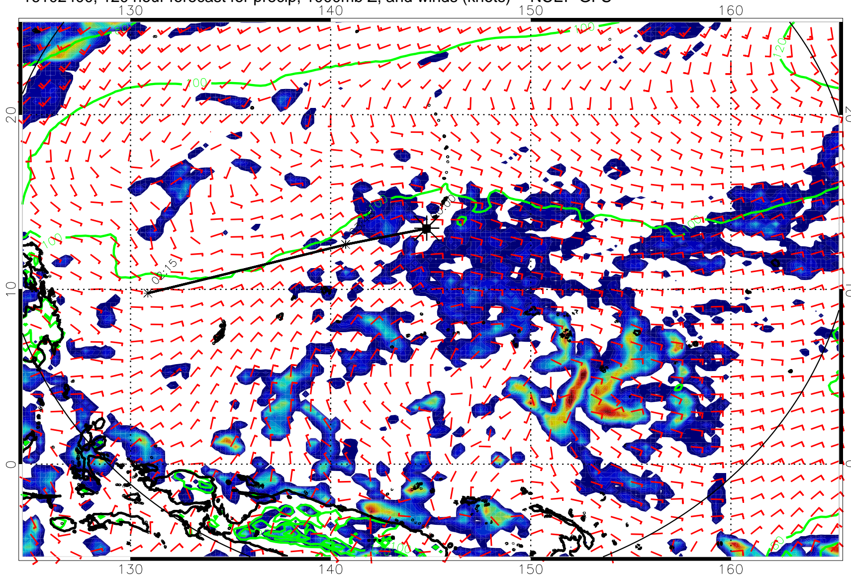
16102400, 120 hour forecast for precip, 1000mb Z, and winds (knots) -- NCEP GFS
