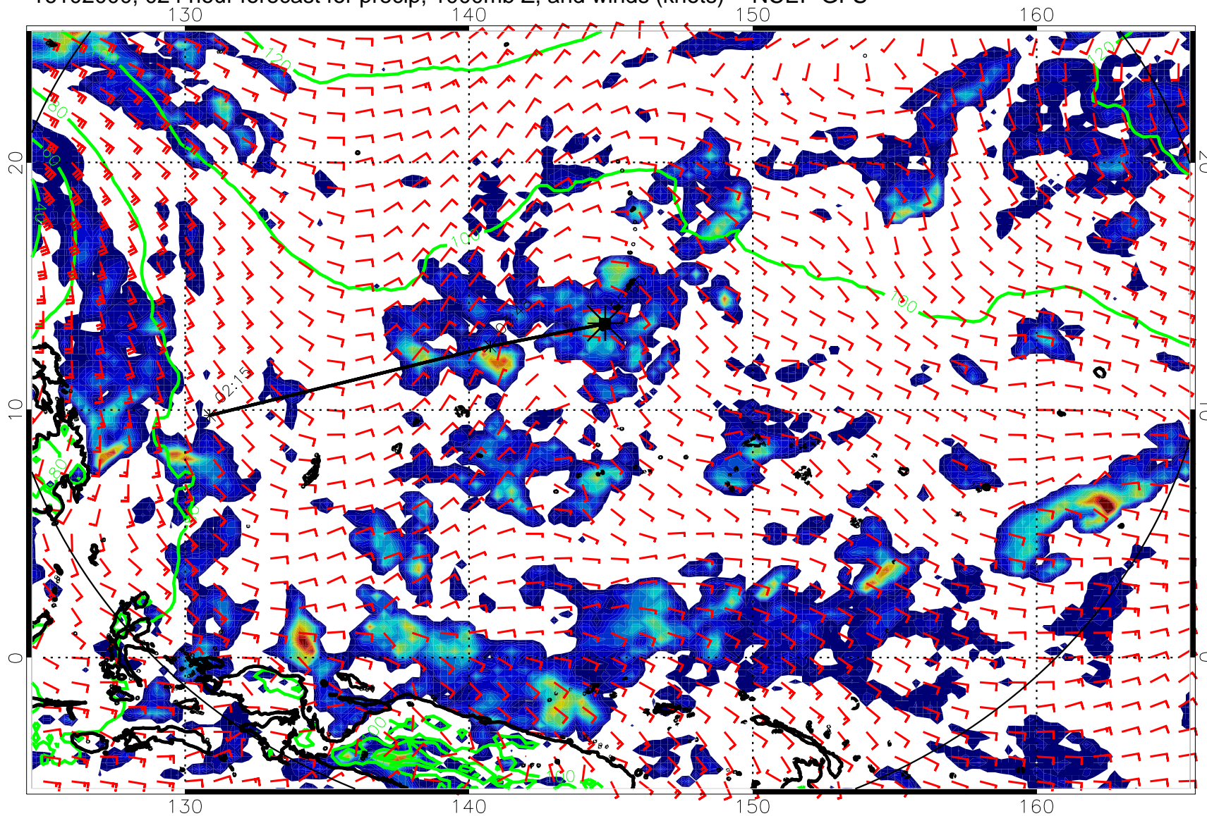
16102000, 024 hour forecast for precip, 1000mb Z, and winds (knots) -- NCEP GFS
