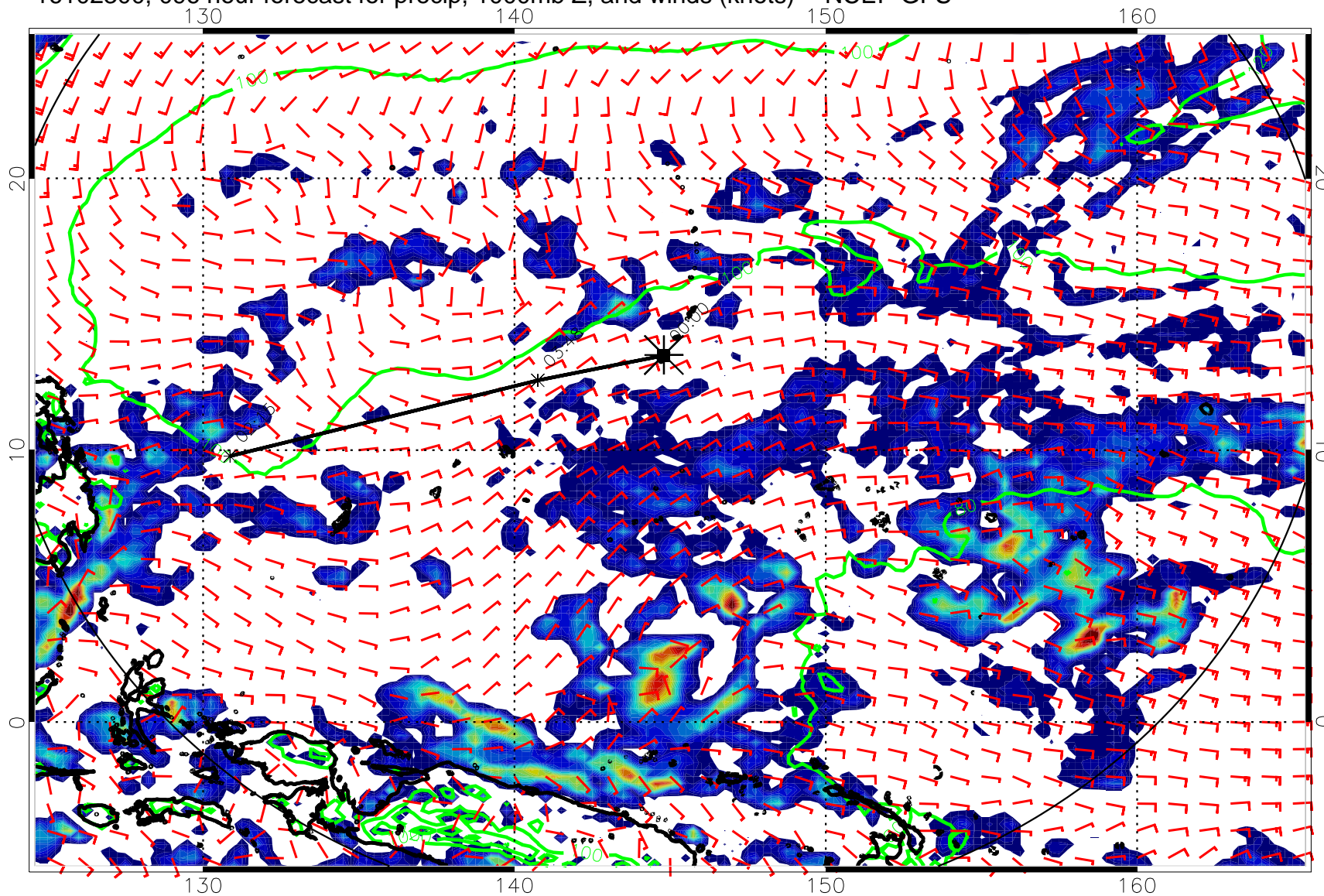
16102300, 096 hour forecast for precip, 1000mb Z, and winds (knots) -- NCEP GFS
