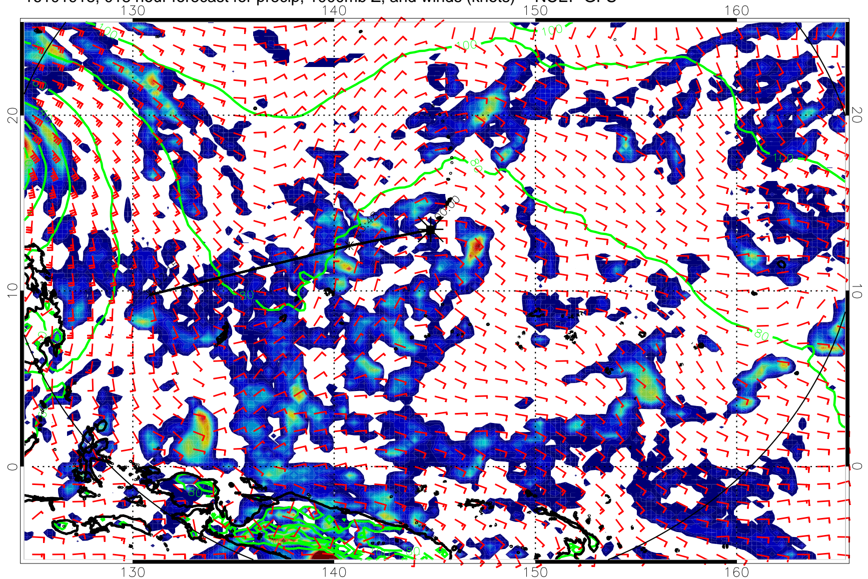
16101918, 018 hour forecast for precip, 1000mb Z, and winds (knots) -- NCEP GFS
