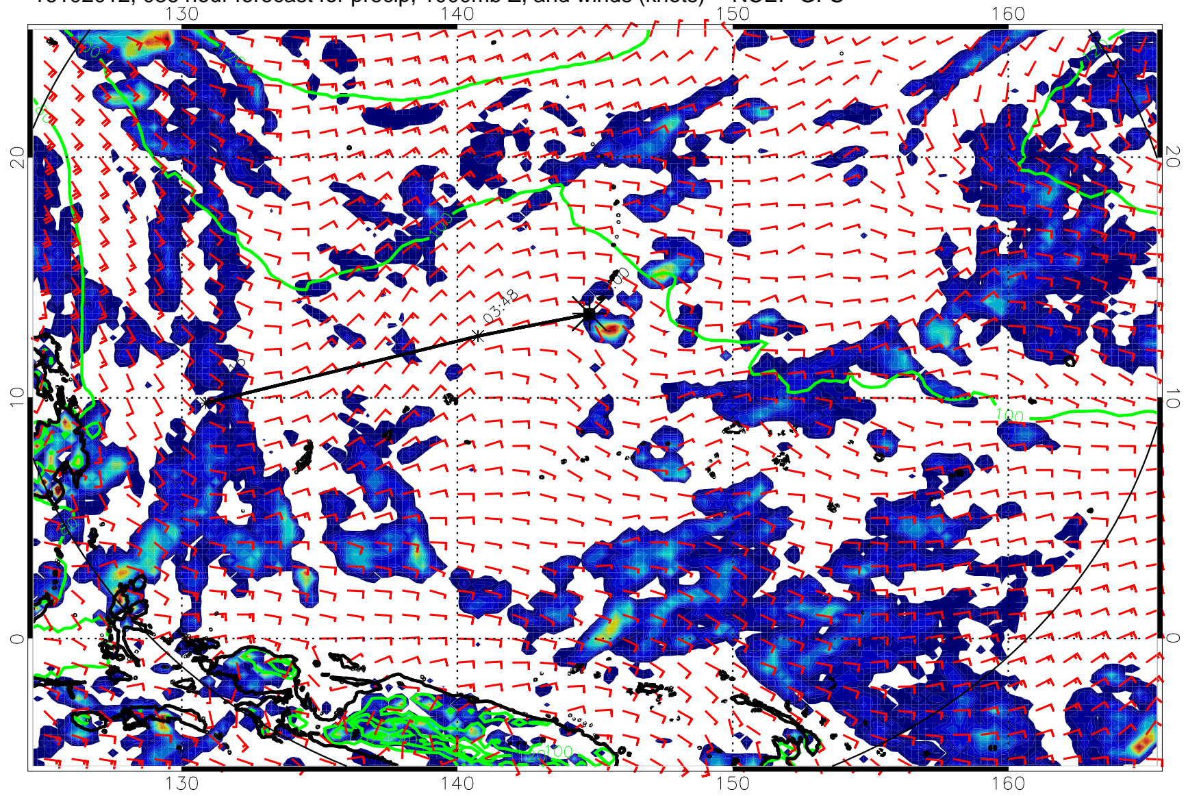
16102012, 036 hour forecast for precip, 1000mb Z, and winds (knots) -- NCEP GFS
