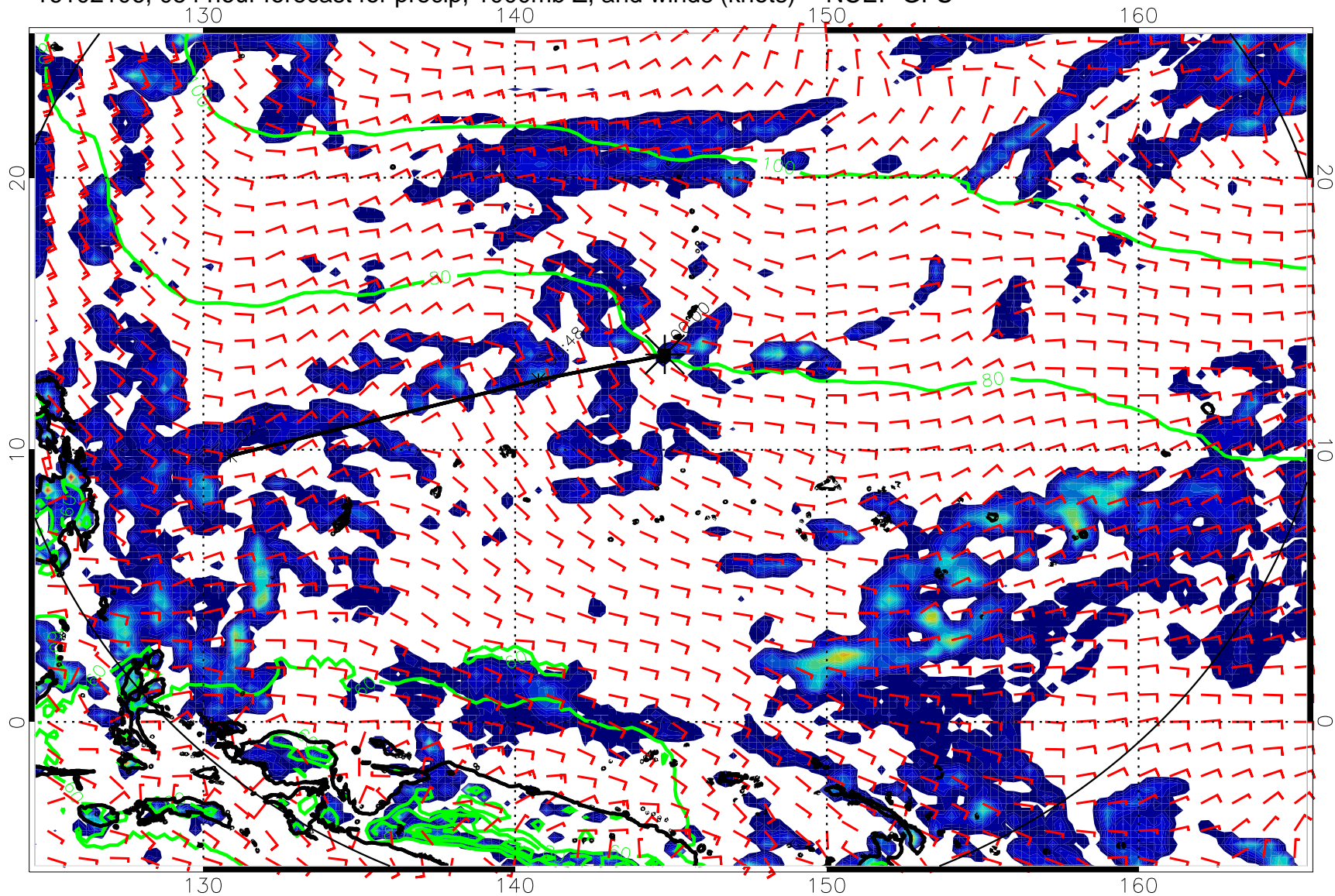
16102106, 054 hour forecast for precip, 1000mb Z, and winds (knots) -- NCEP GFS
