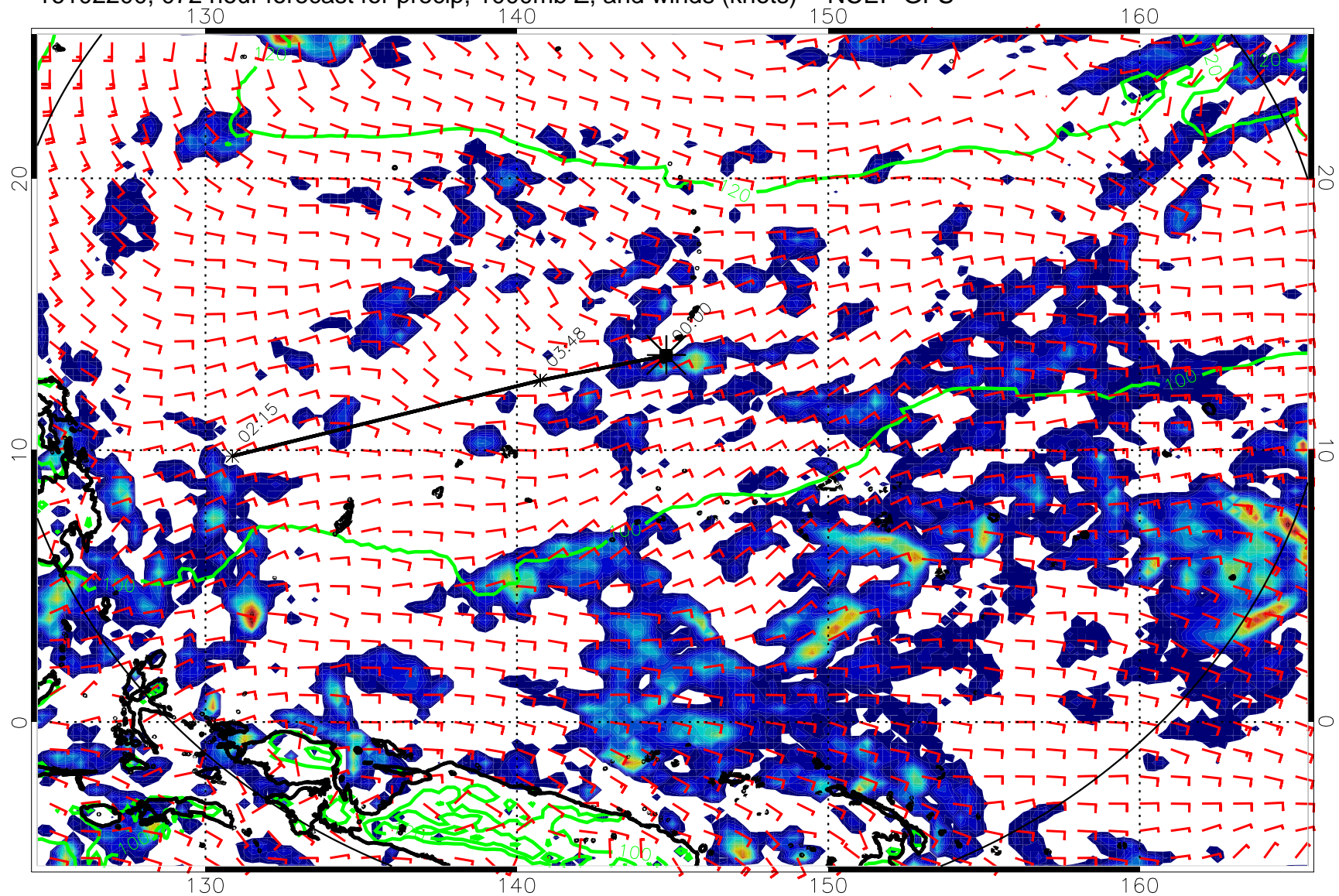
16102200, 072 hour forecast for precip, 1000mb Z, and winds (knots) -- NCEP GFS
