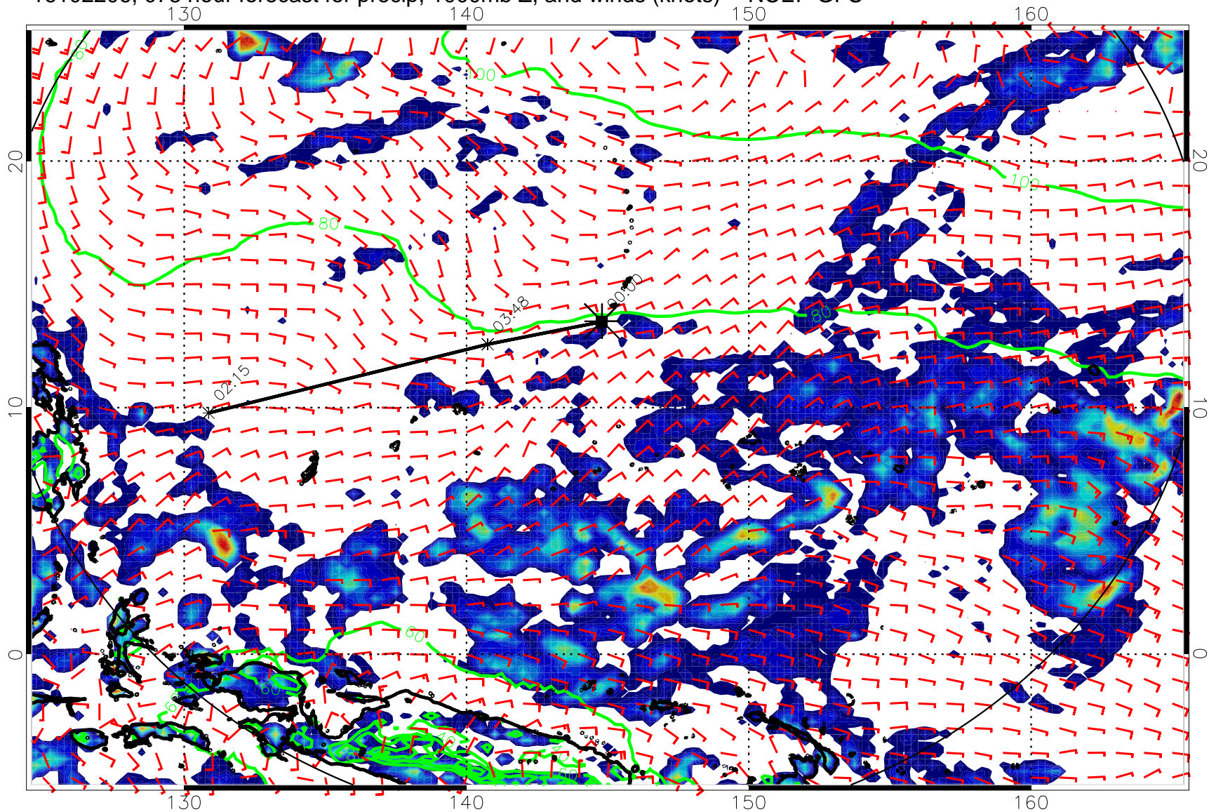
16102206, 078 hour forecast for precip, 1000mb Z, and winds (knots) -- NCEP GFS
