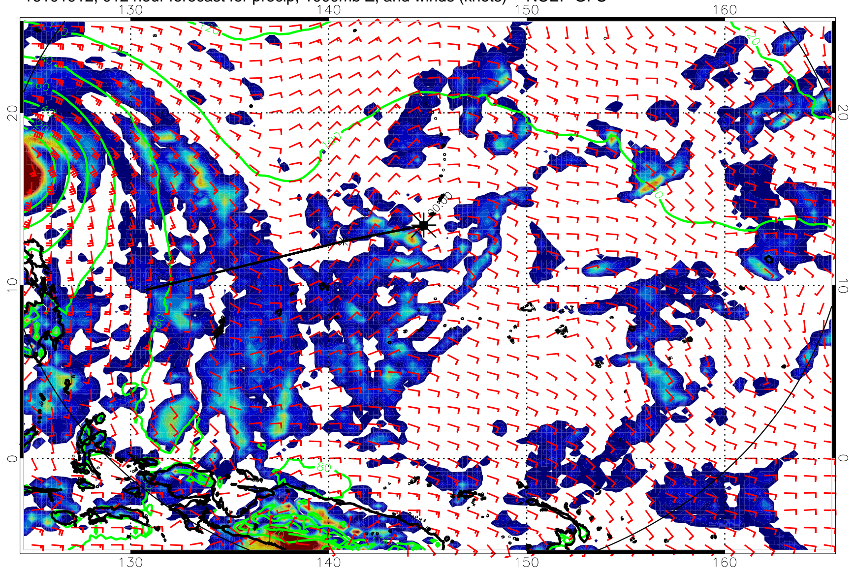
16101912, 012 hour forecast for precip, 1000mb Z, and winds (knots) -- NCEP GFS
