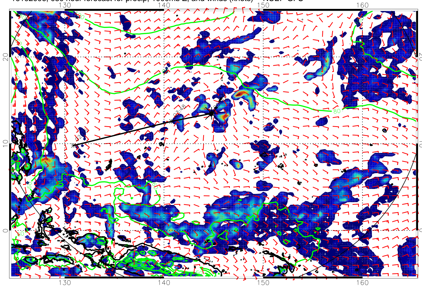
16102006, 030 hour forecast for precip, 1000mb Z, and winds (knots) -- NCEP GFS
