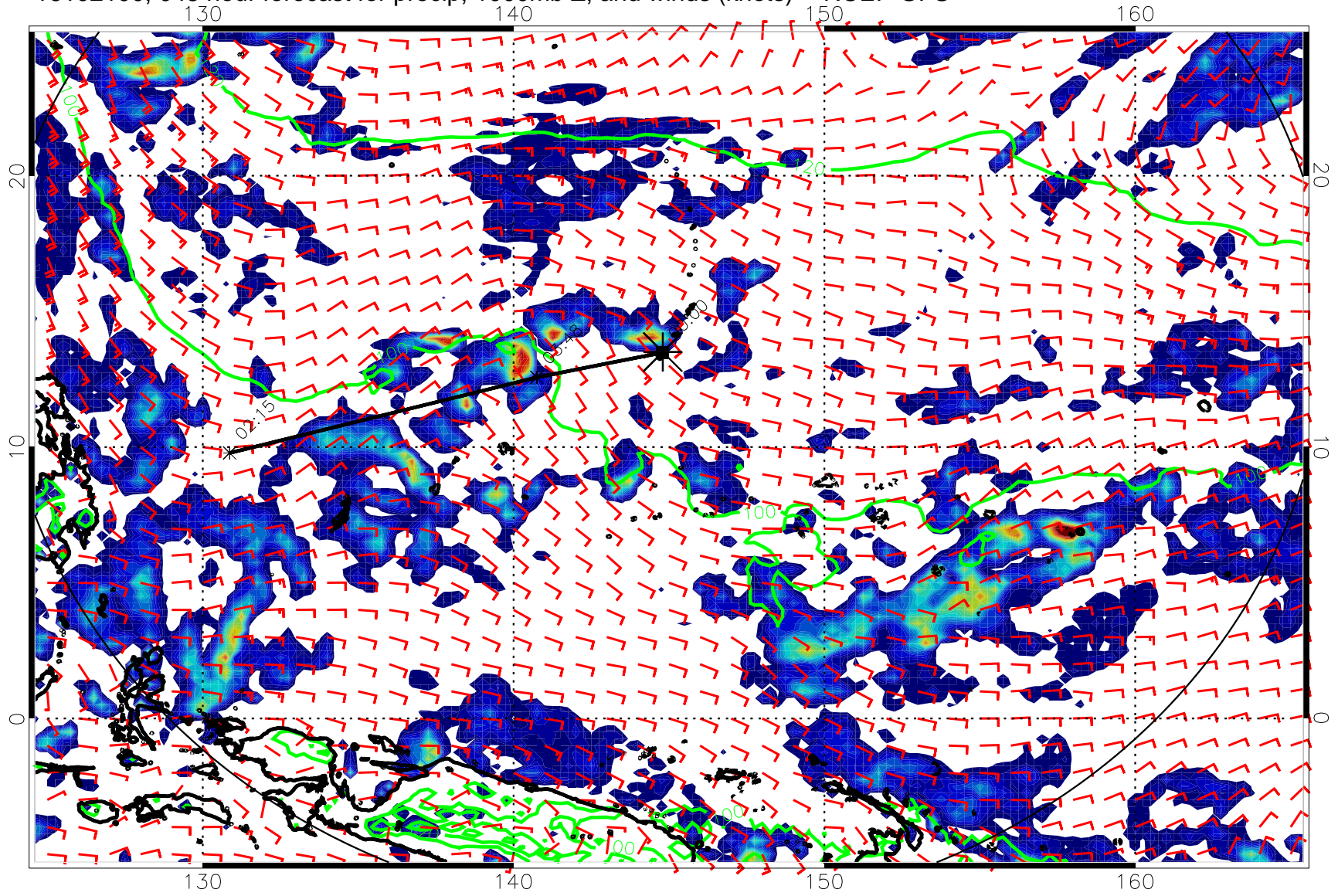
16102100, 048 hour forecast for precip, 1000mb Z, and winds (knots) -- NCEP GFS
