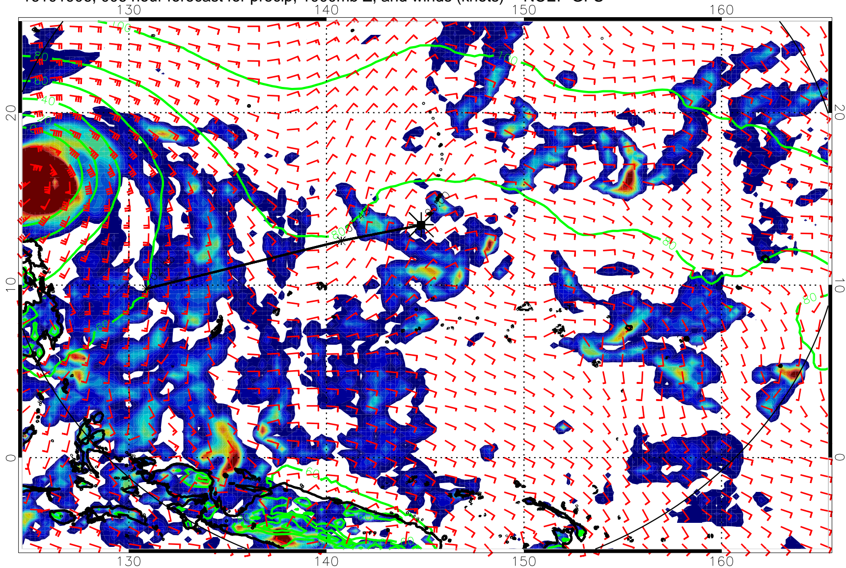
16101906, 006 hour forecast for precip, 1000mb Z, and winds (knots) -- NCEP GFS
