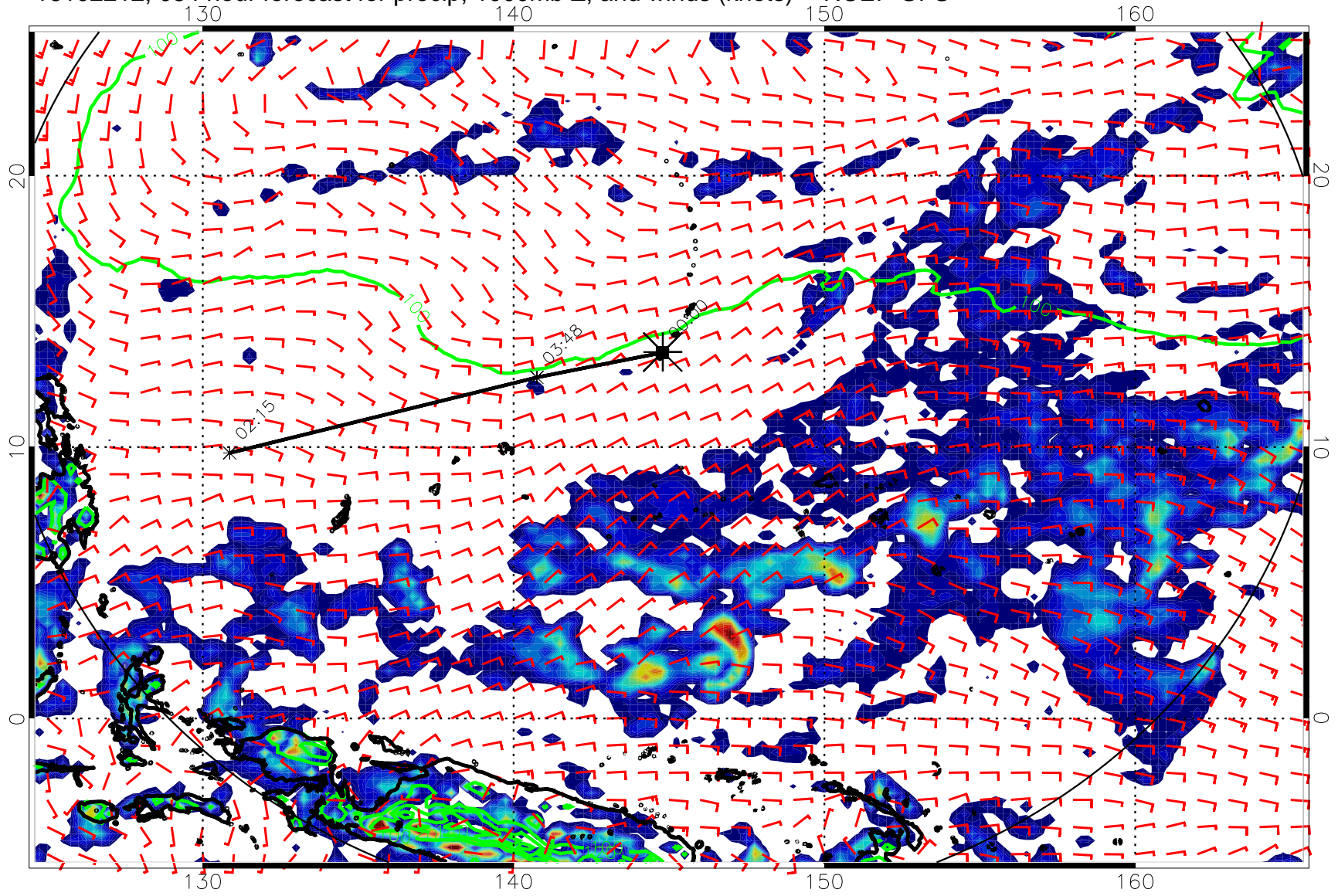
16102212, 084 hour forecast for precip, 1000mb Z, and winds (knots) -- NCEP GFS
