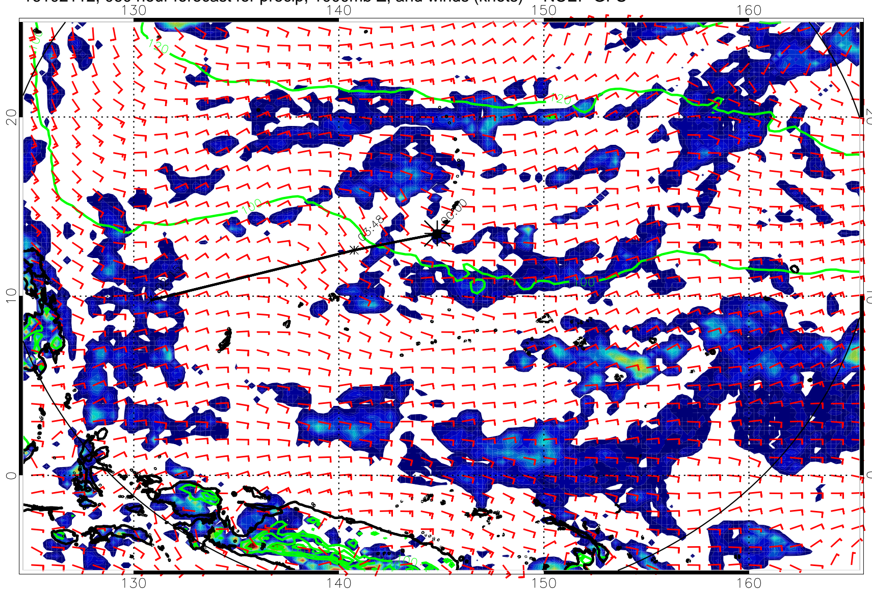
16102112, 060 hour forecast for precip, 1000mb Z, and winds (knots) -- NCEP GFS
