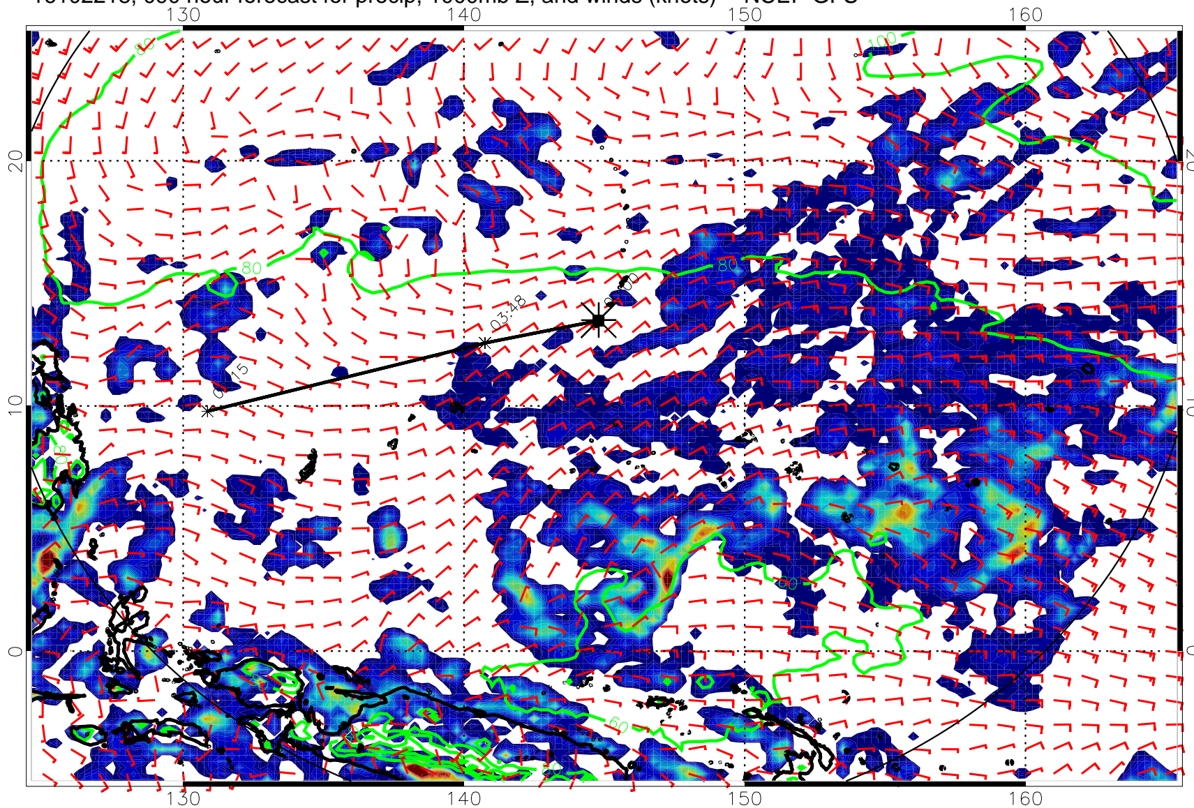
16102218, 090 hour forecast for precip, 1000mb Z, and winds (knots) -- NCEP GFS
