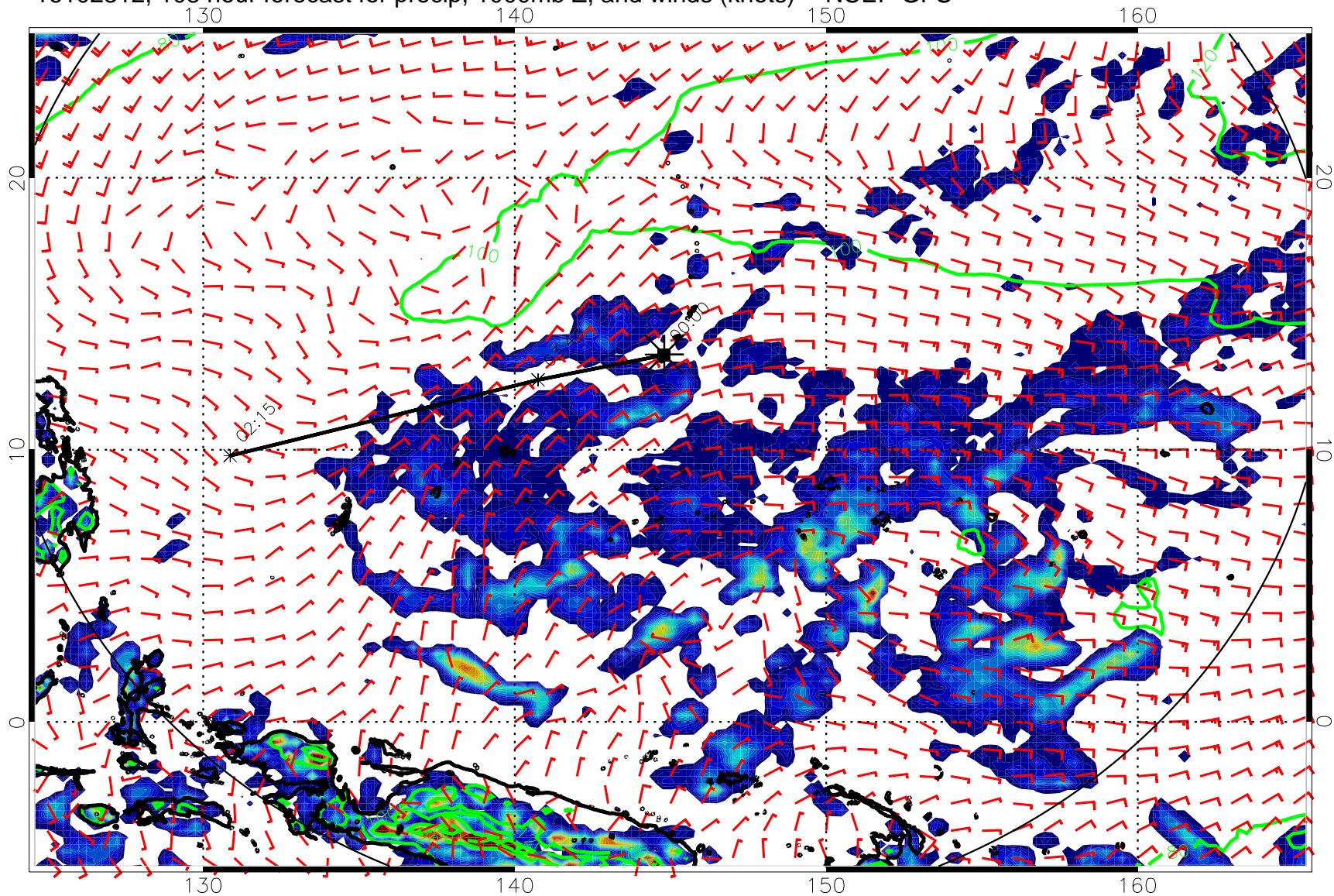
16102312, 108 hour forecast for precip, 1000mb Z, and winds (knots) -- NCEP GFS
