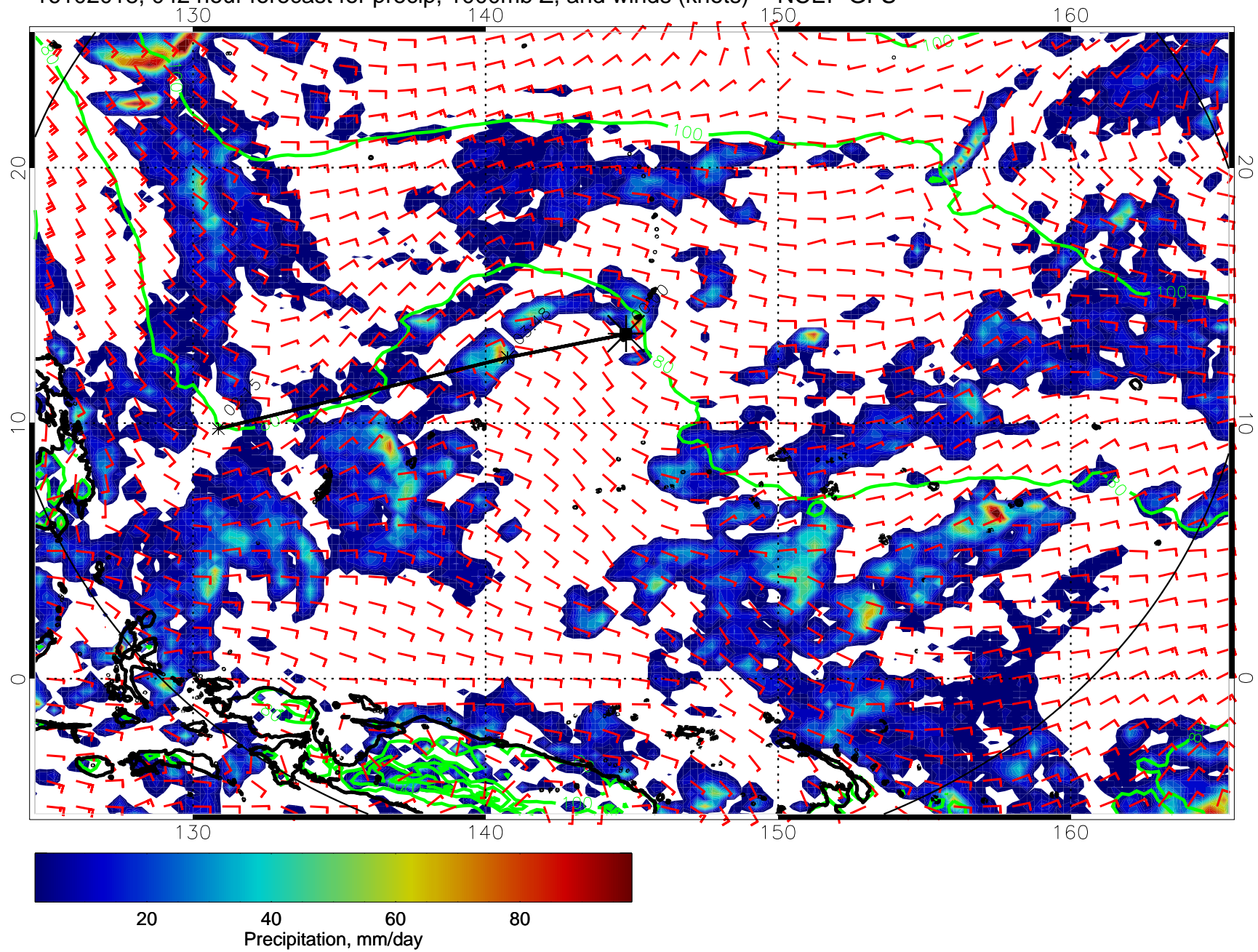
16102018, 04Z hour forecast for precip, 1000mb Z, and winds (knots) -- NCEP GFS
