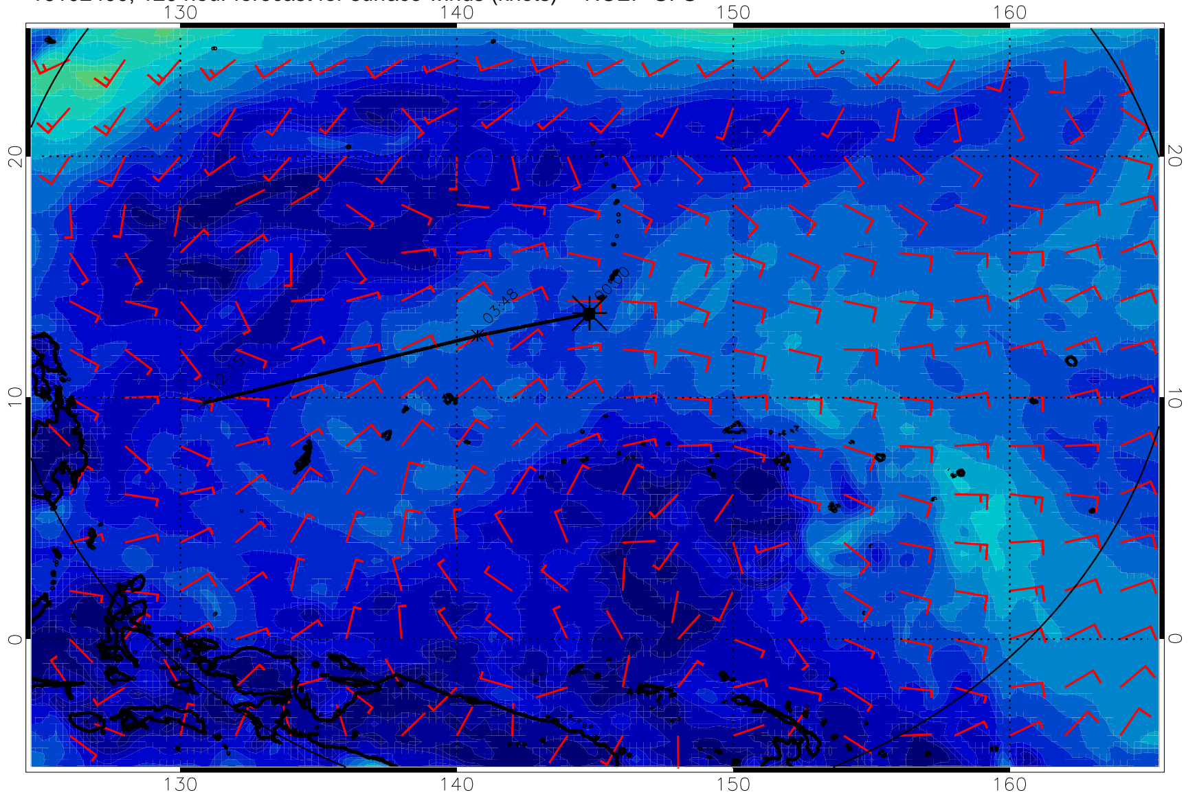
16102400, 120 hour forecast for surface winds (knots) -- NCEP GFS
