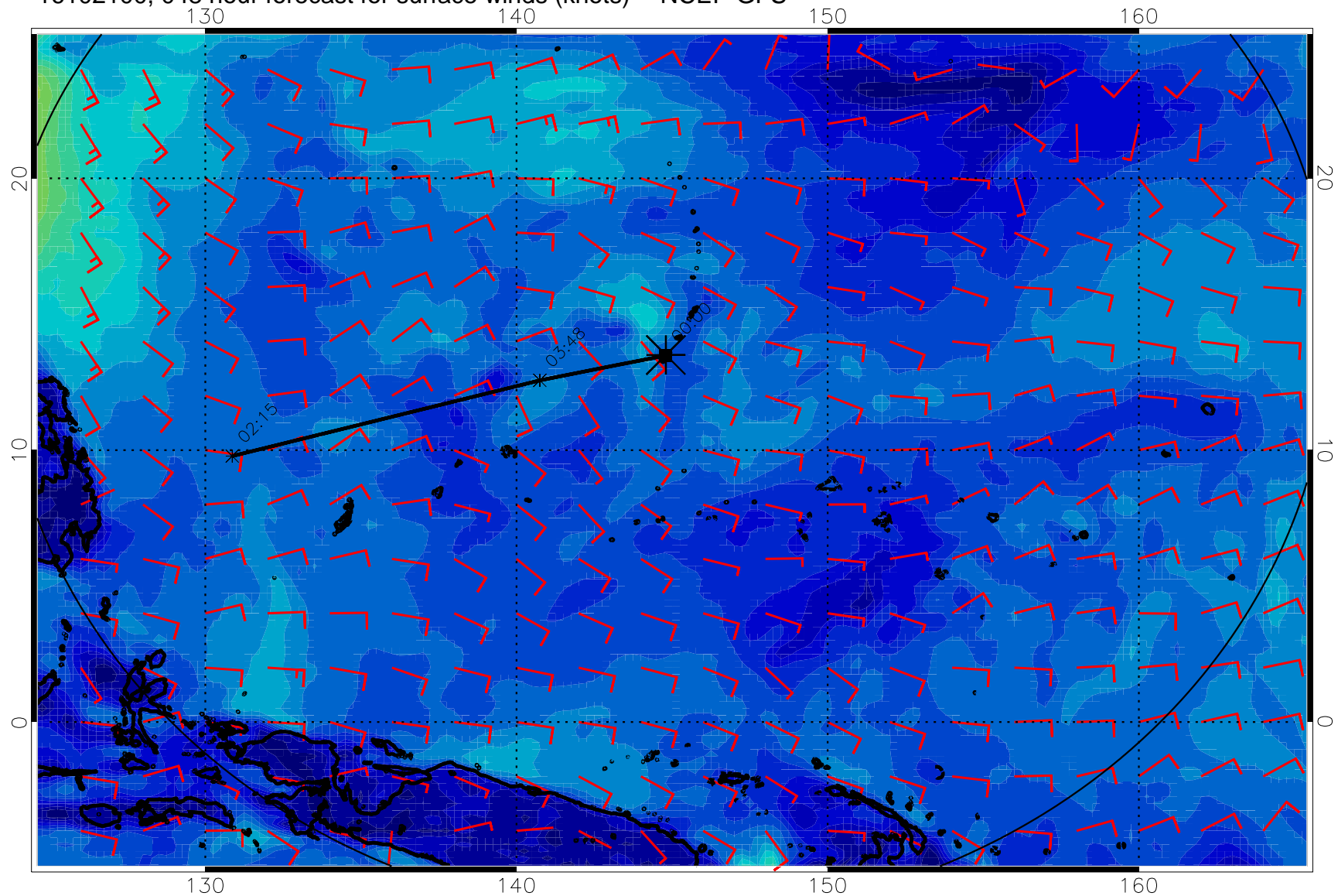
16102100, 048 hour forecast for surface winds (knots) -- NCEP GFS
