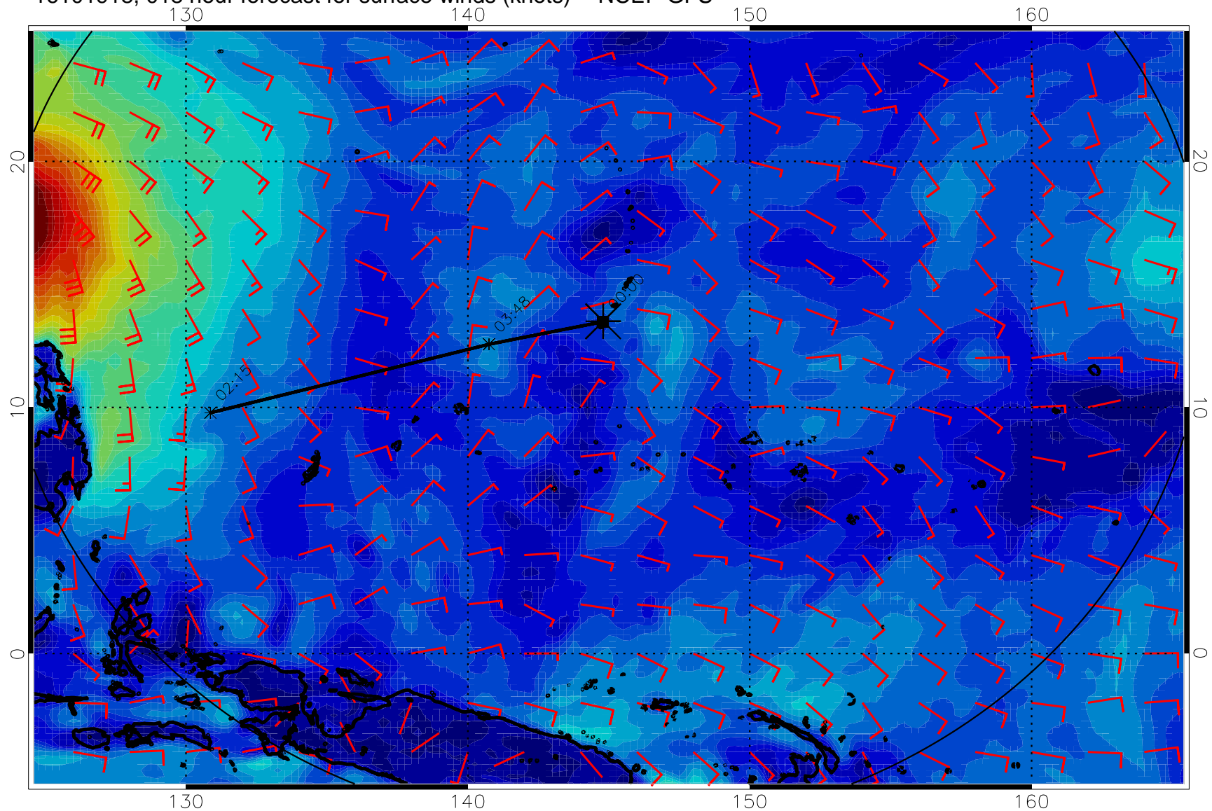
16101918, 018 hour forecast for surface winds (knots) -- NCEP GFS
