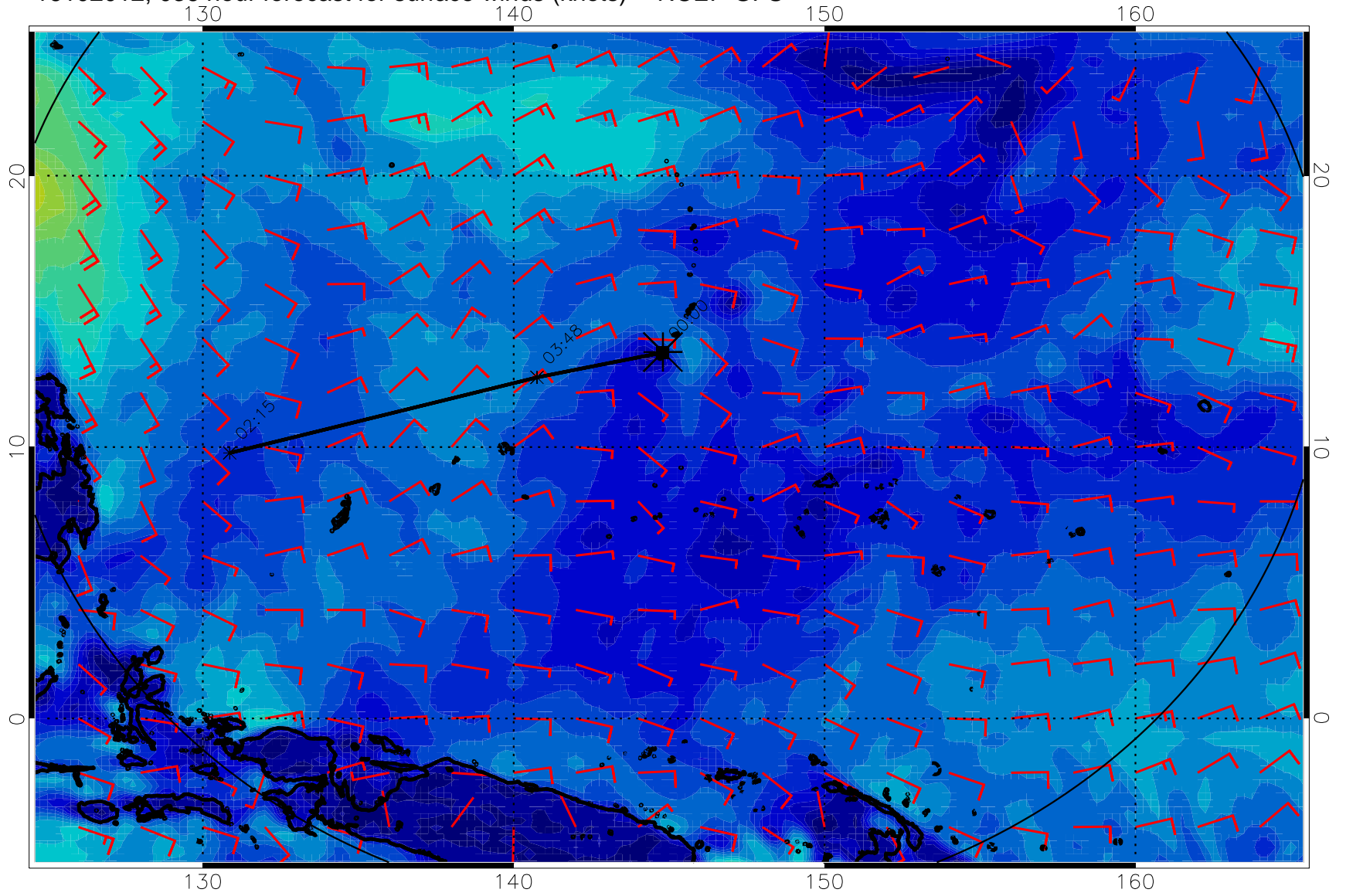
16102012, 036 hour forecast for surface winds (knots) -- NCEP GFS
