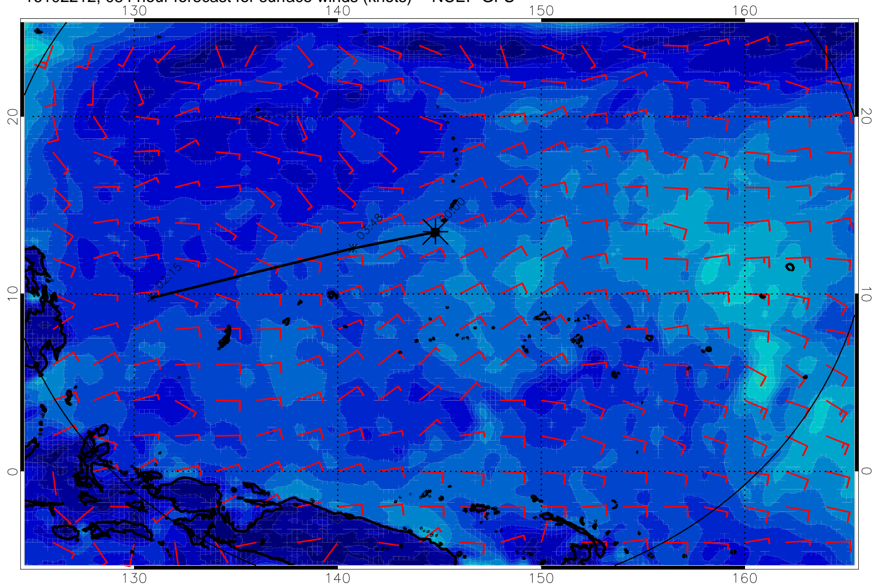
16102212, 084 hour forecast for surface winds (knots) -- NCEP GFS
