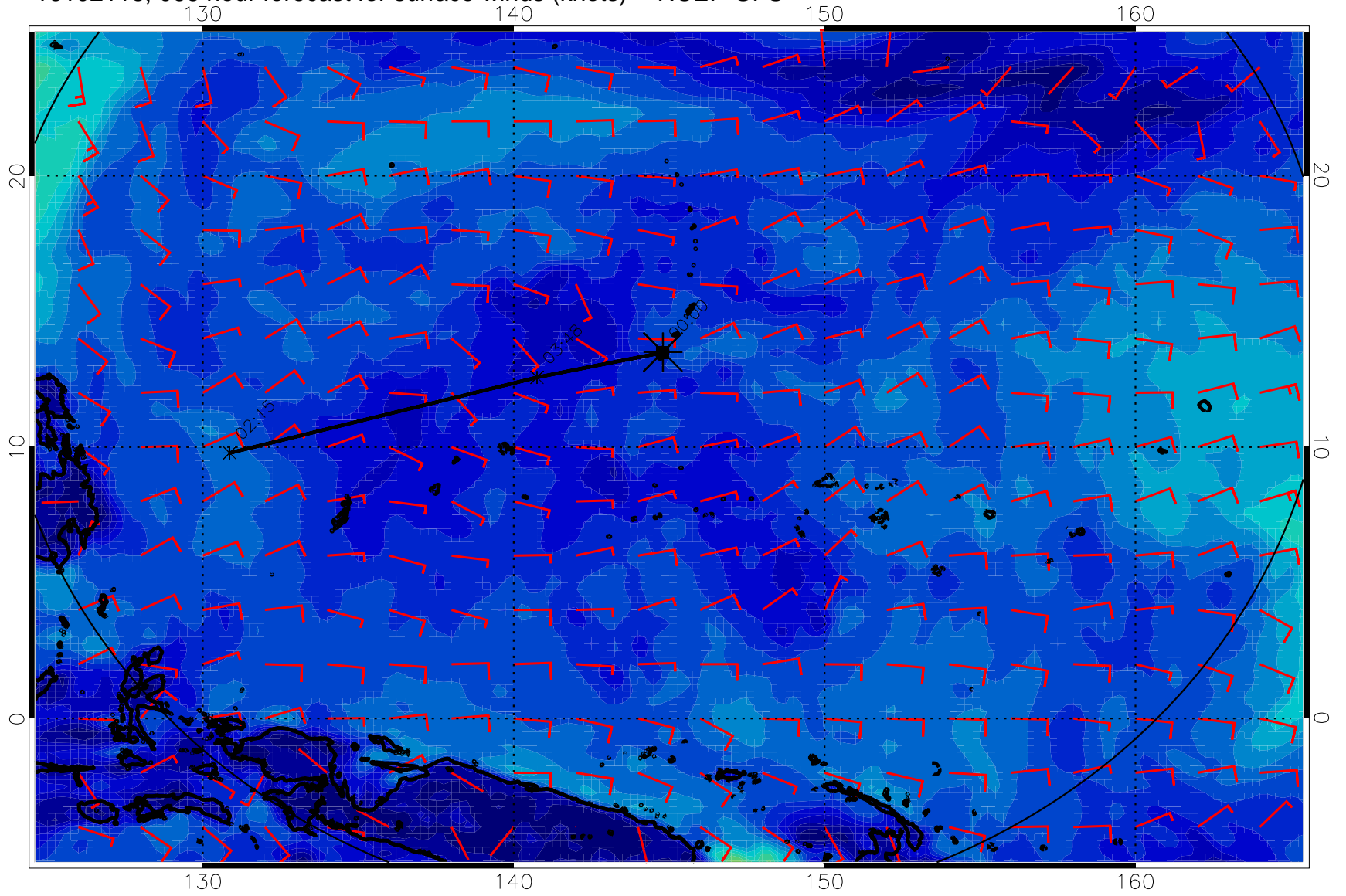
16102118, 066 hour forecast for surface winds (knots) -- NCEP GFS
