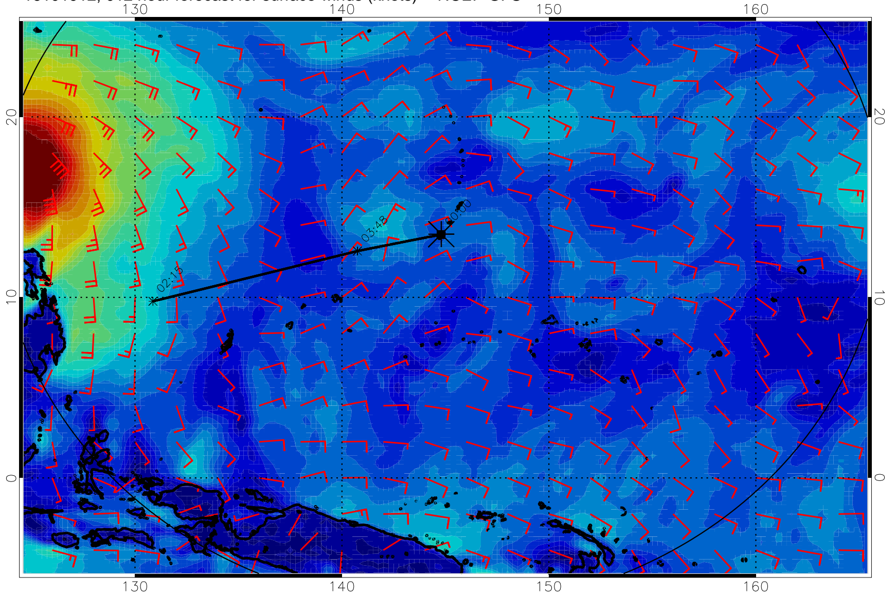
16101912, 012 hour forecast for surface winds (knots) -- NCEP GFS
