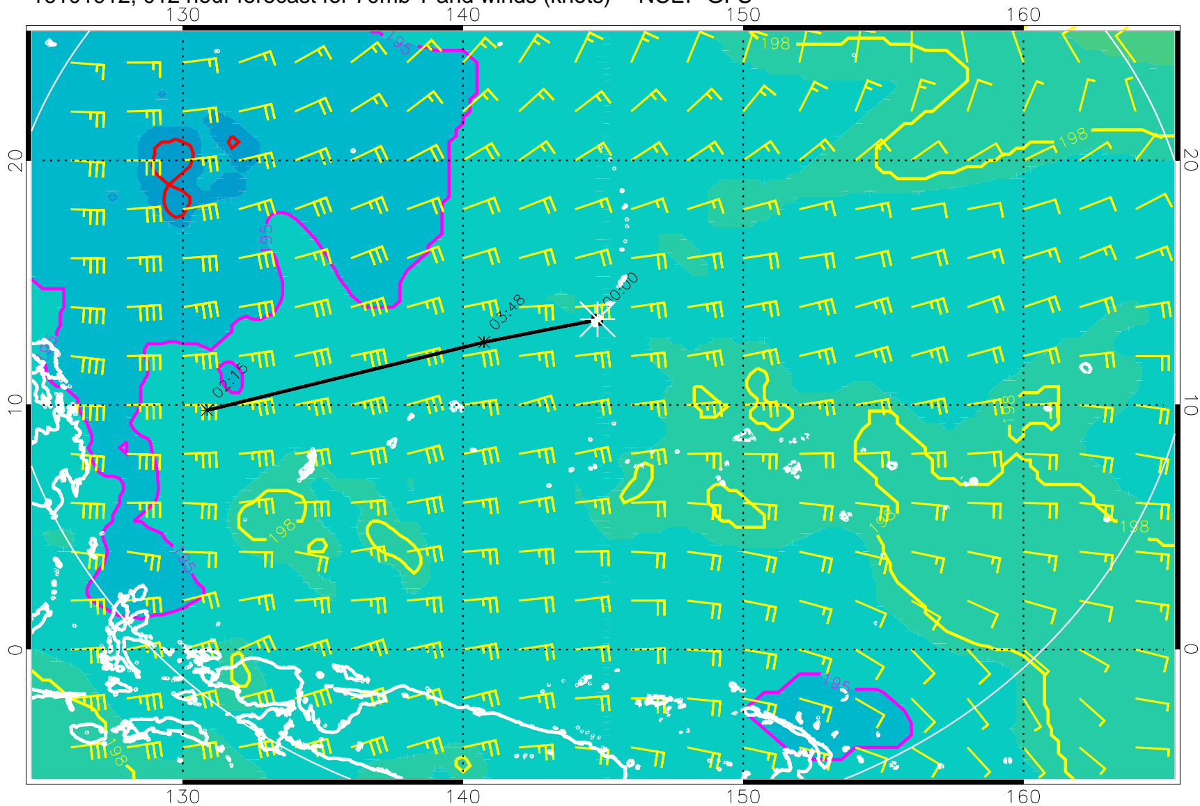
16101912, 012 hour forecast for 70mb T and winds (knots) -- NCEP GFS
