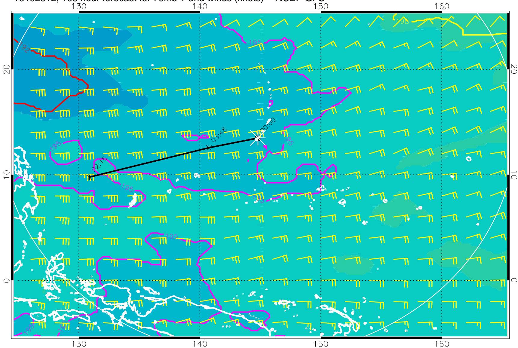
16102312, 108 hour forecast for 70mb T and winds (knots) -- NCEP GFS
