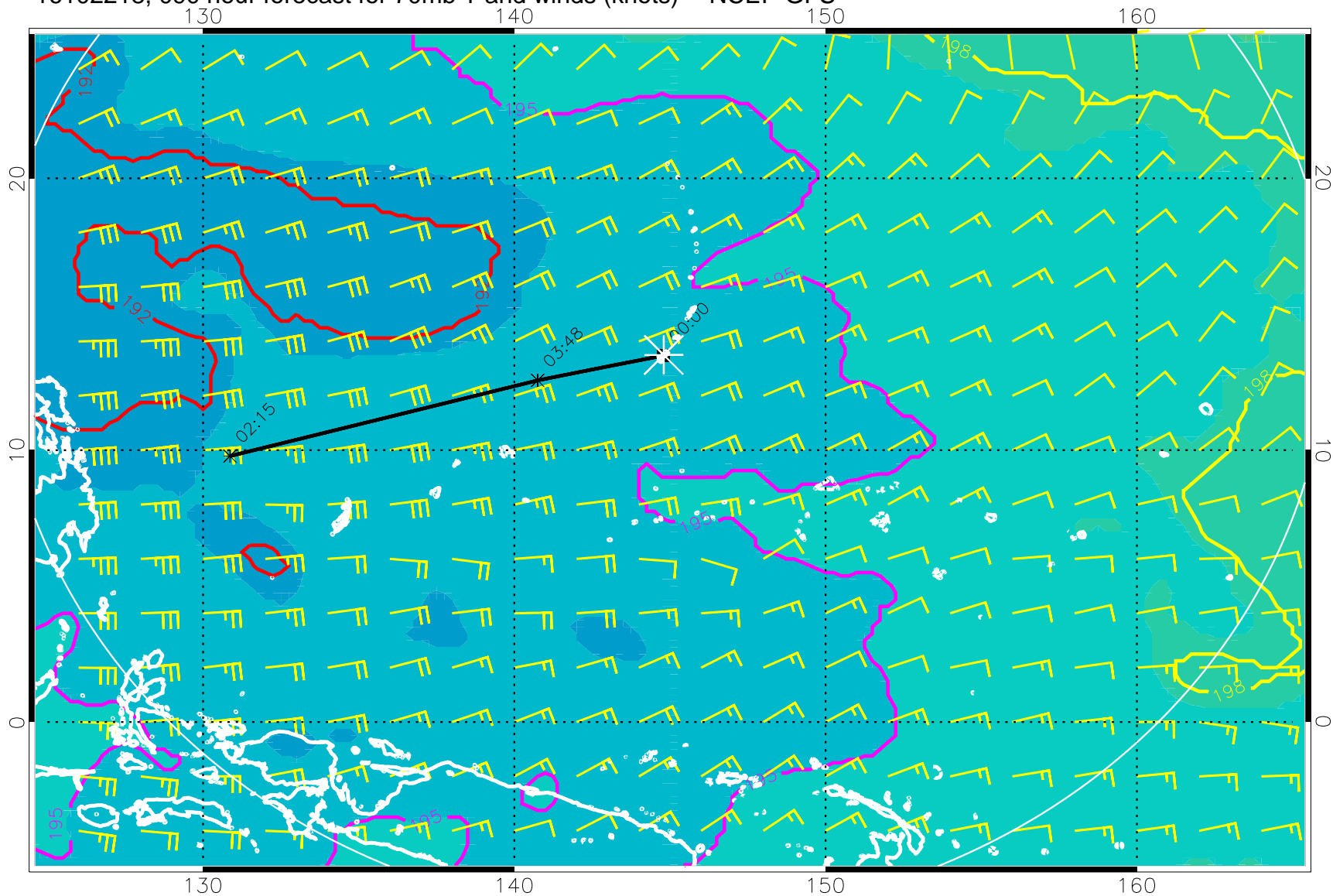
16102218, 090 hour forecast for 70mb T and winds (knots) -- NCEP GFS
