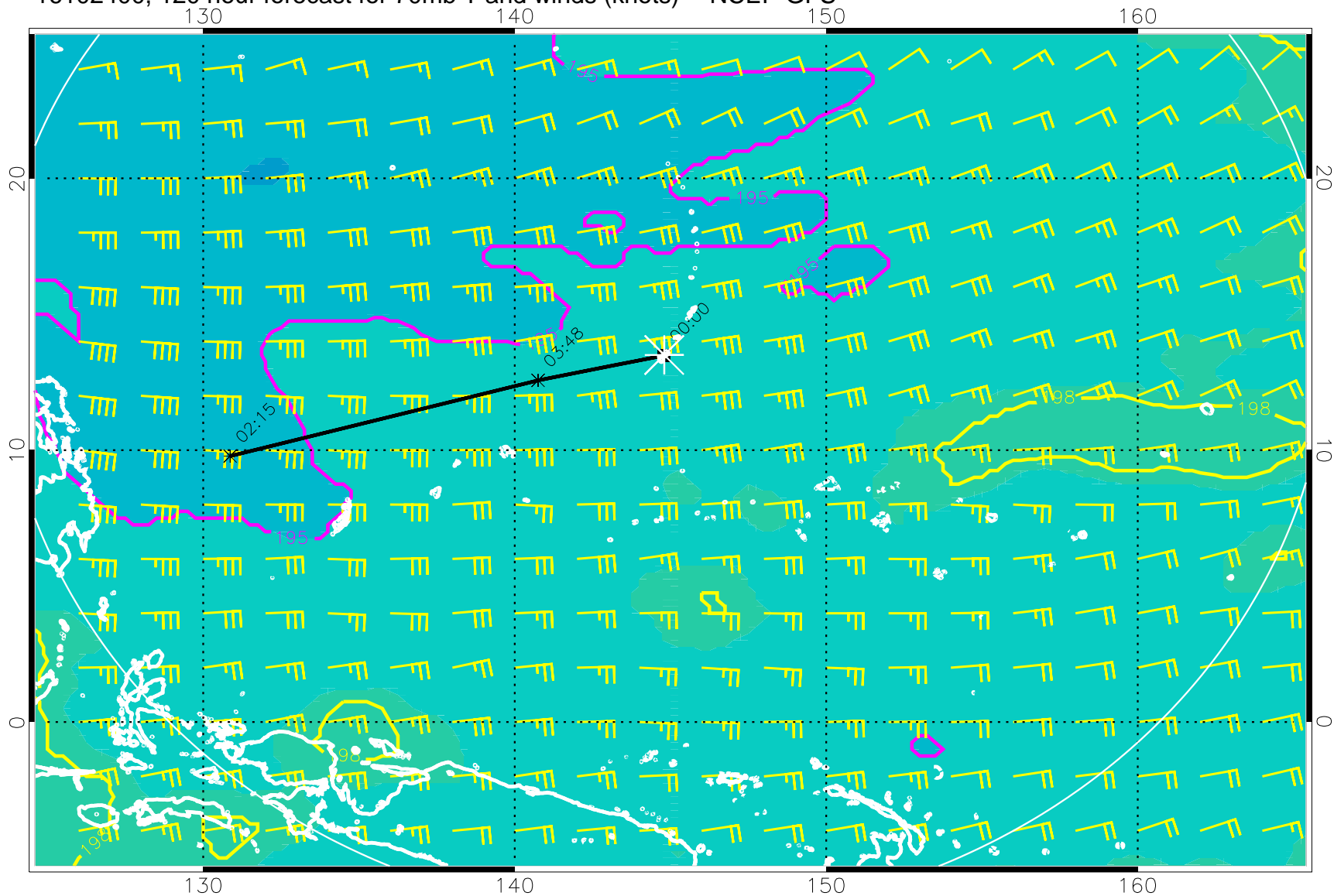
16102400, 120 hour forecast for 70mb T and winds (knots) -- NCEP GFS
