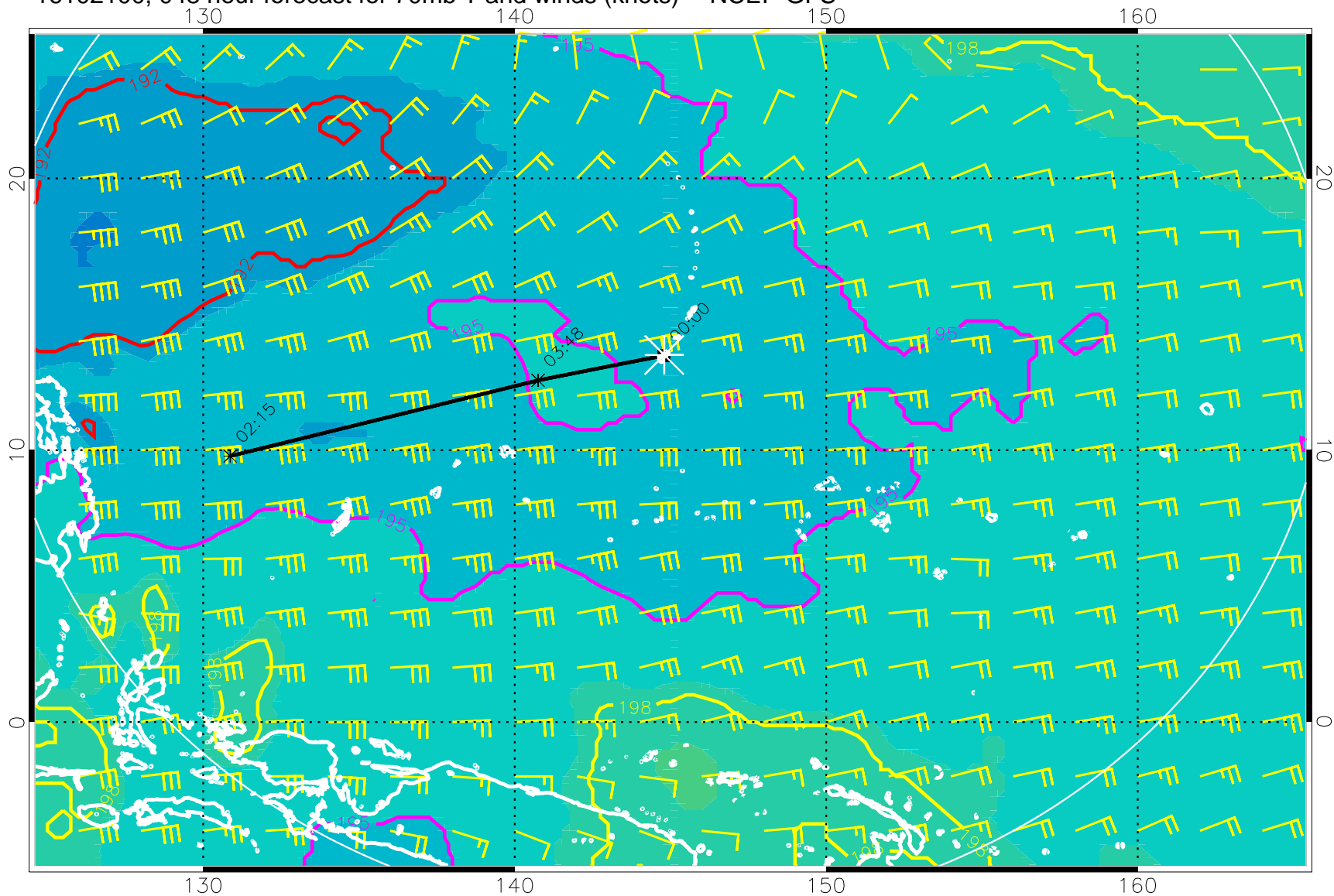
16102100, 048 hour forecast for 70mb T and winds (knots) -- NCEP GFS
