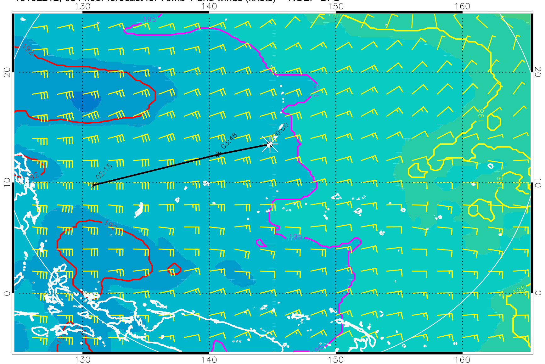
16102212, 084 hour forecast for 70mb T and winds (knots) -- NCEP GFS
