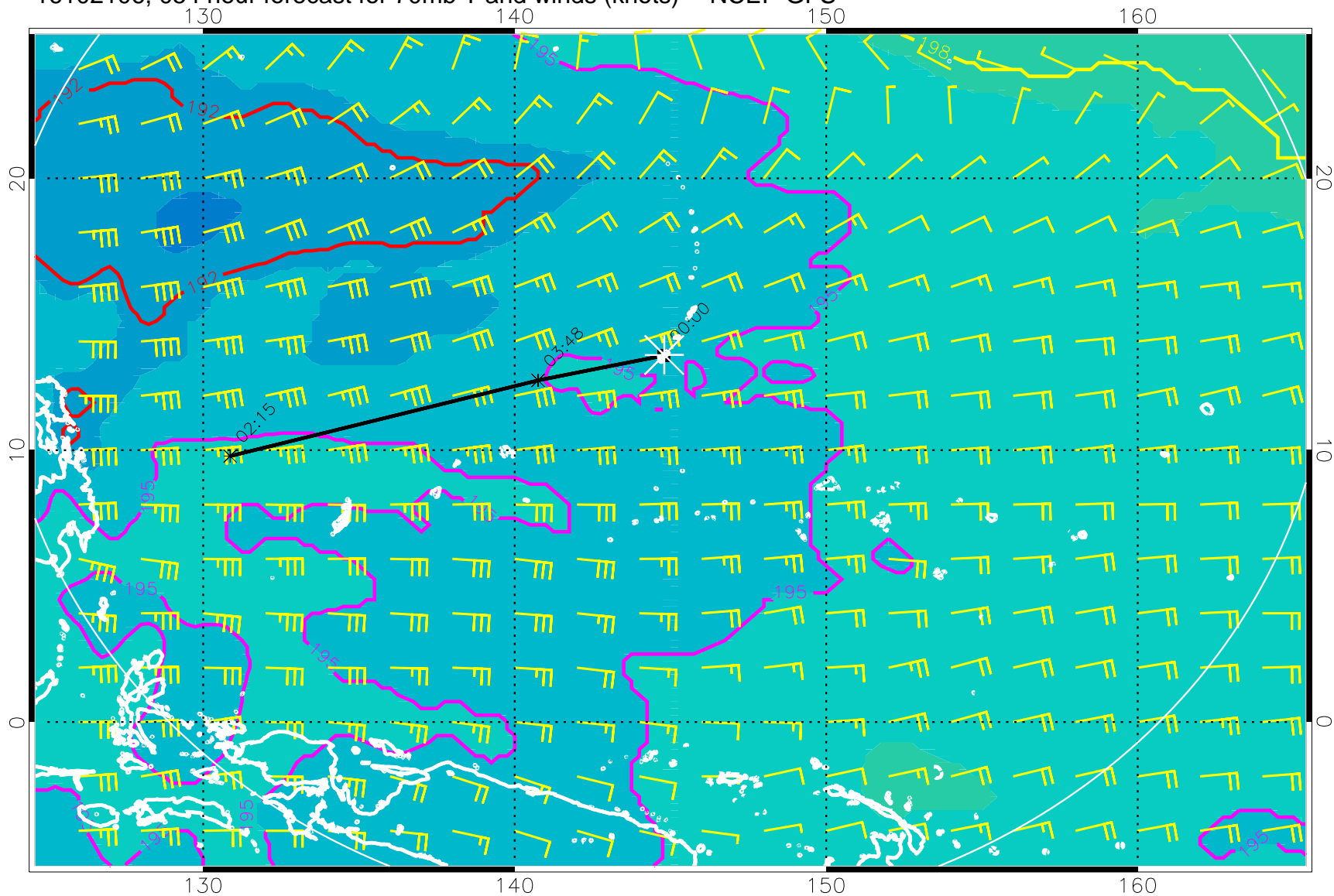
16102106, 054 hour forecast for 70mb T and winds (knots) -- NCEP GFS
