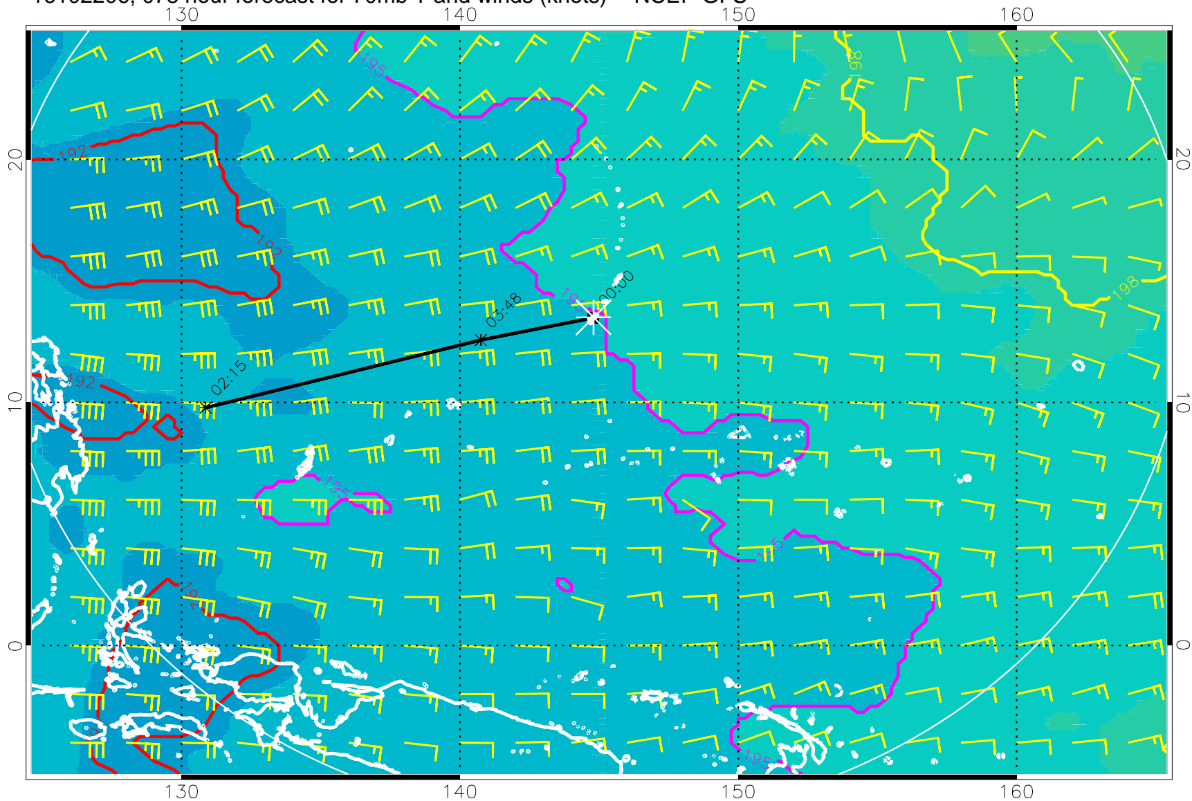
16102206, 078 hour forecast for 70mb T and winds (knots) -- NCEP GFS
