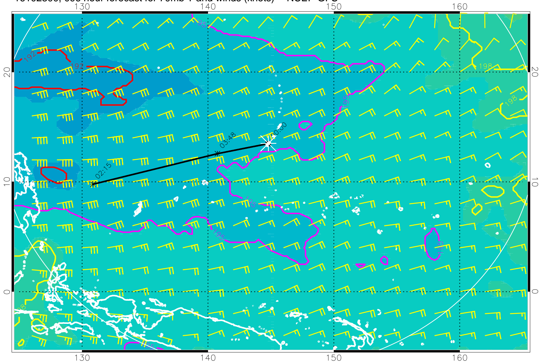
16102300, 096 hour forecast for 70mb T and winds (knots) -- NCEP GFS
