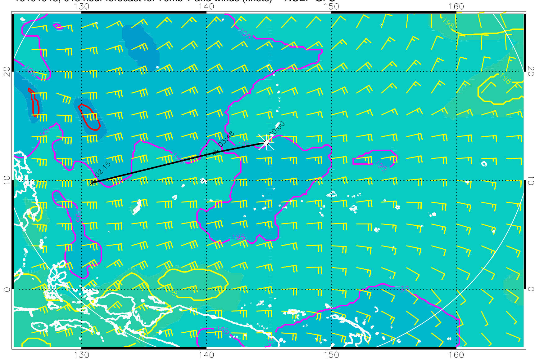
16101918, 018 hour forecast for 70mb T and winds (knots) -- NCEP GFS
