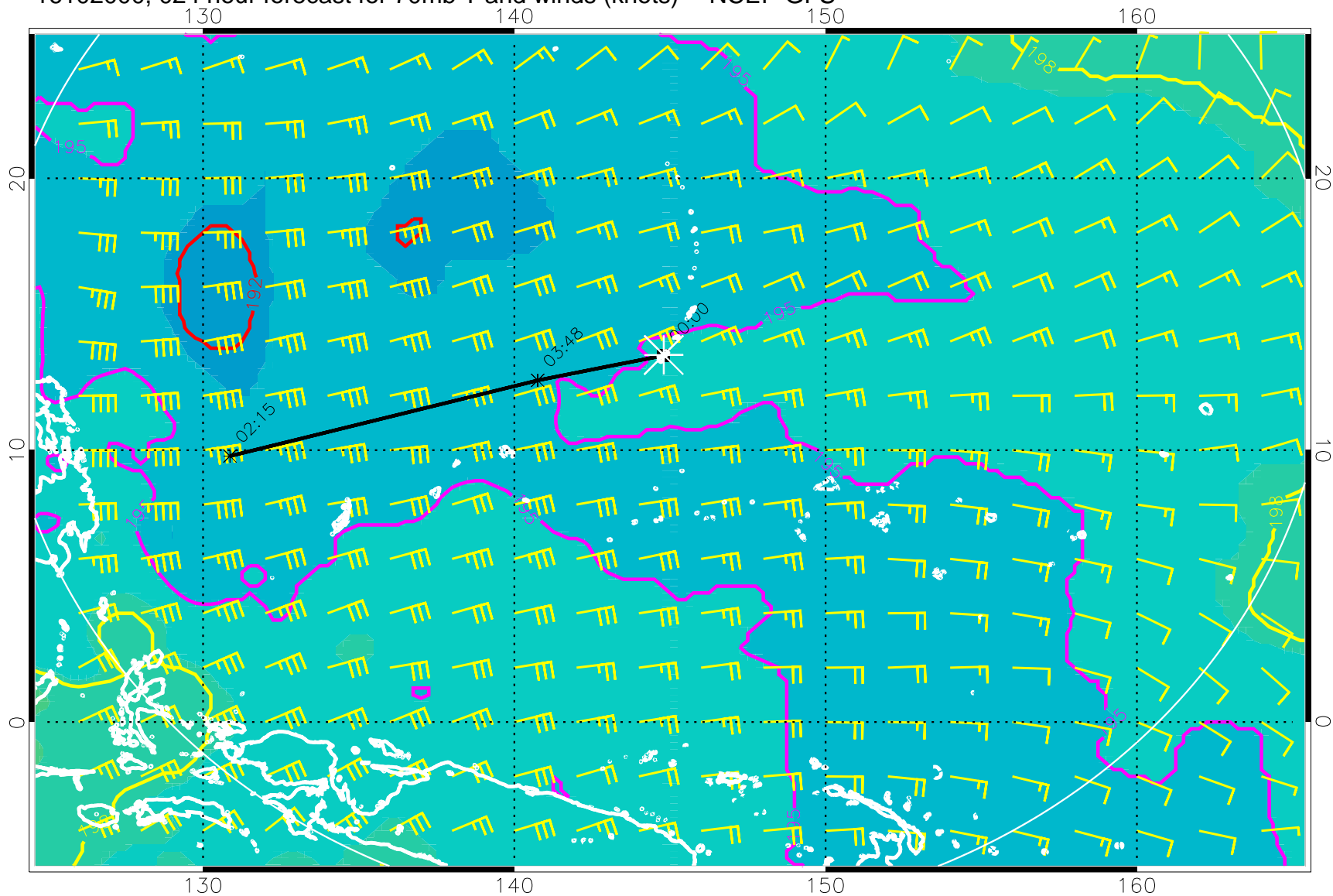
16102000, 024 hour forecast for 70mb T and winds (knots) -- NCEP GFS
