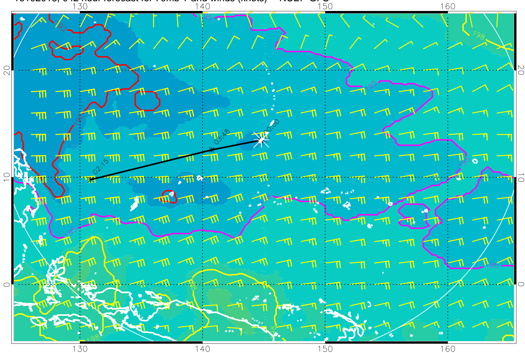
16102018, 042 hour forecast for 70mb T and winds (knots) -- NCEP GFS
