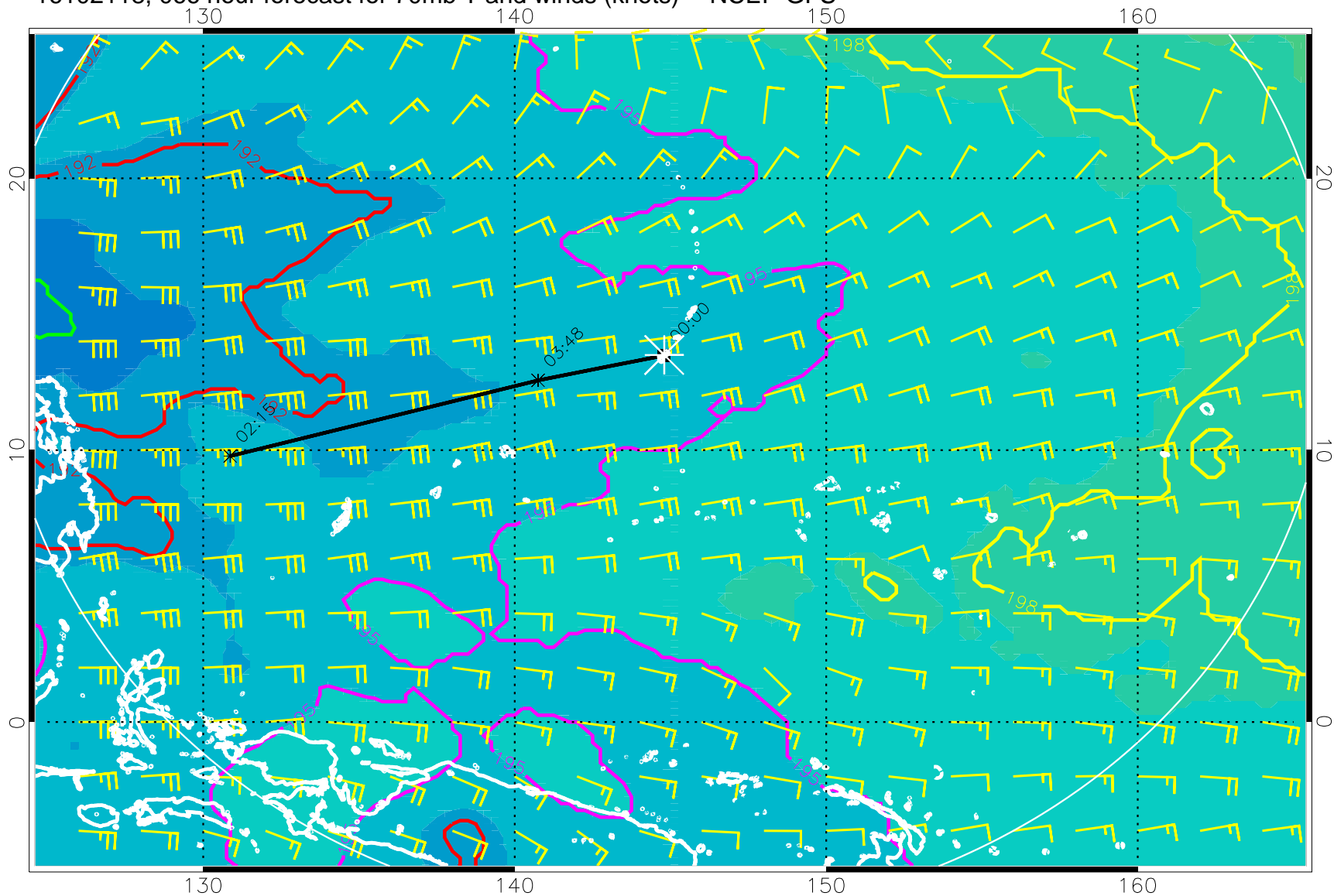
16102118, 066 hour forecast for 70mb T and winds (knots) -- NCEP GFS
