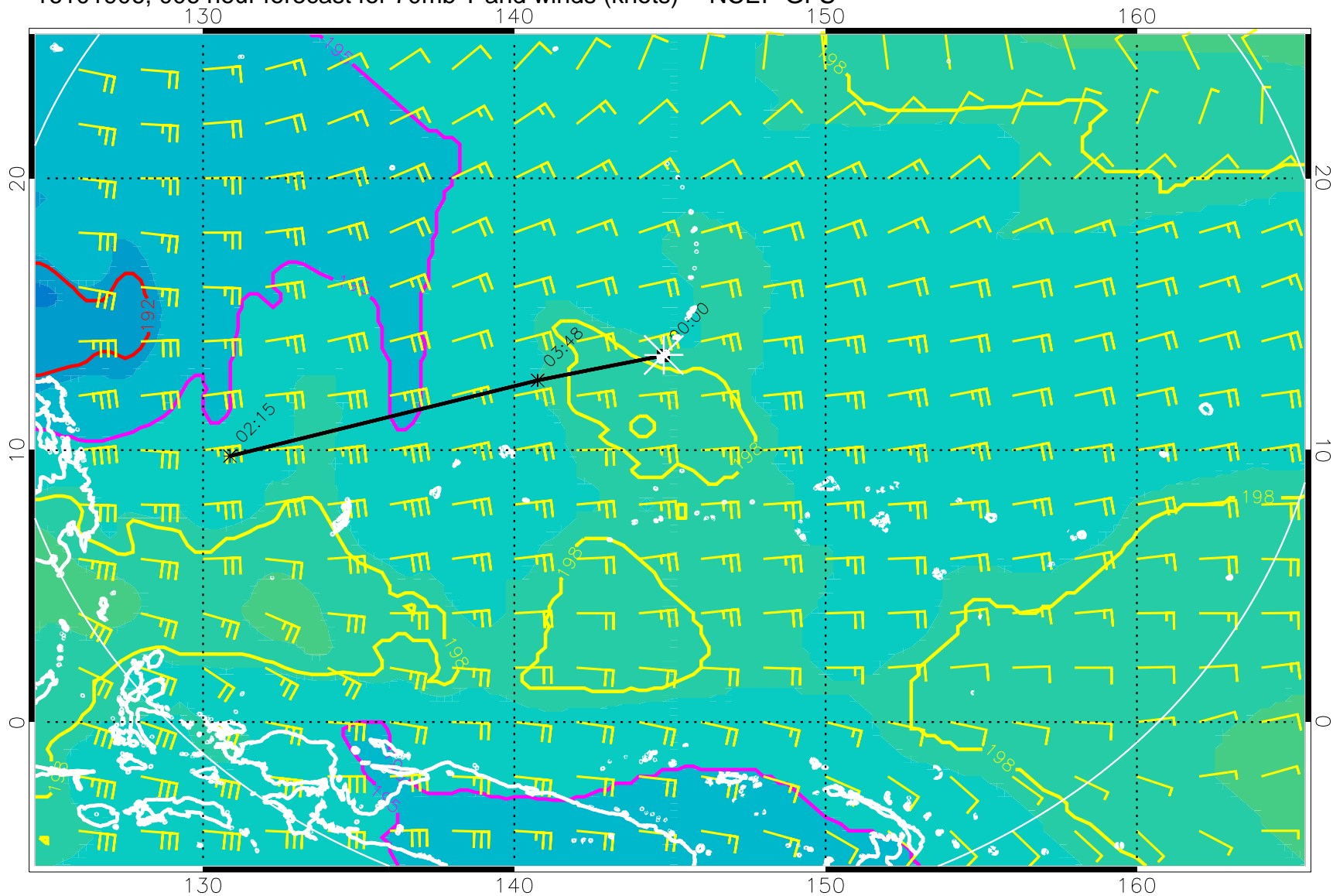
16101906, 006 hour forecast for 70mb T and winds (knots) -- NCEP GFS
