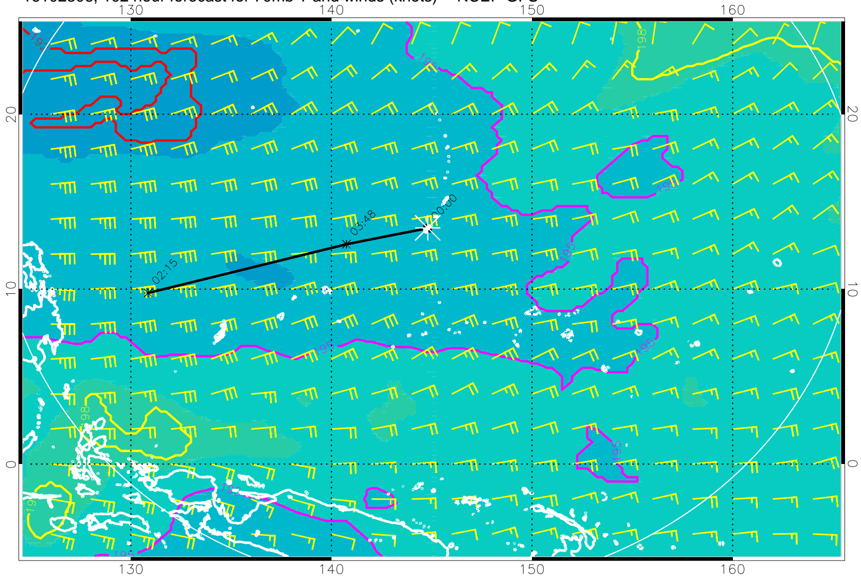
16102306, 102 hour forecast for 70mb T and winds (knots) -- NCEP GFS
