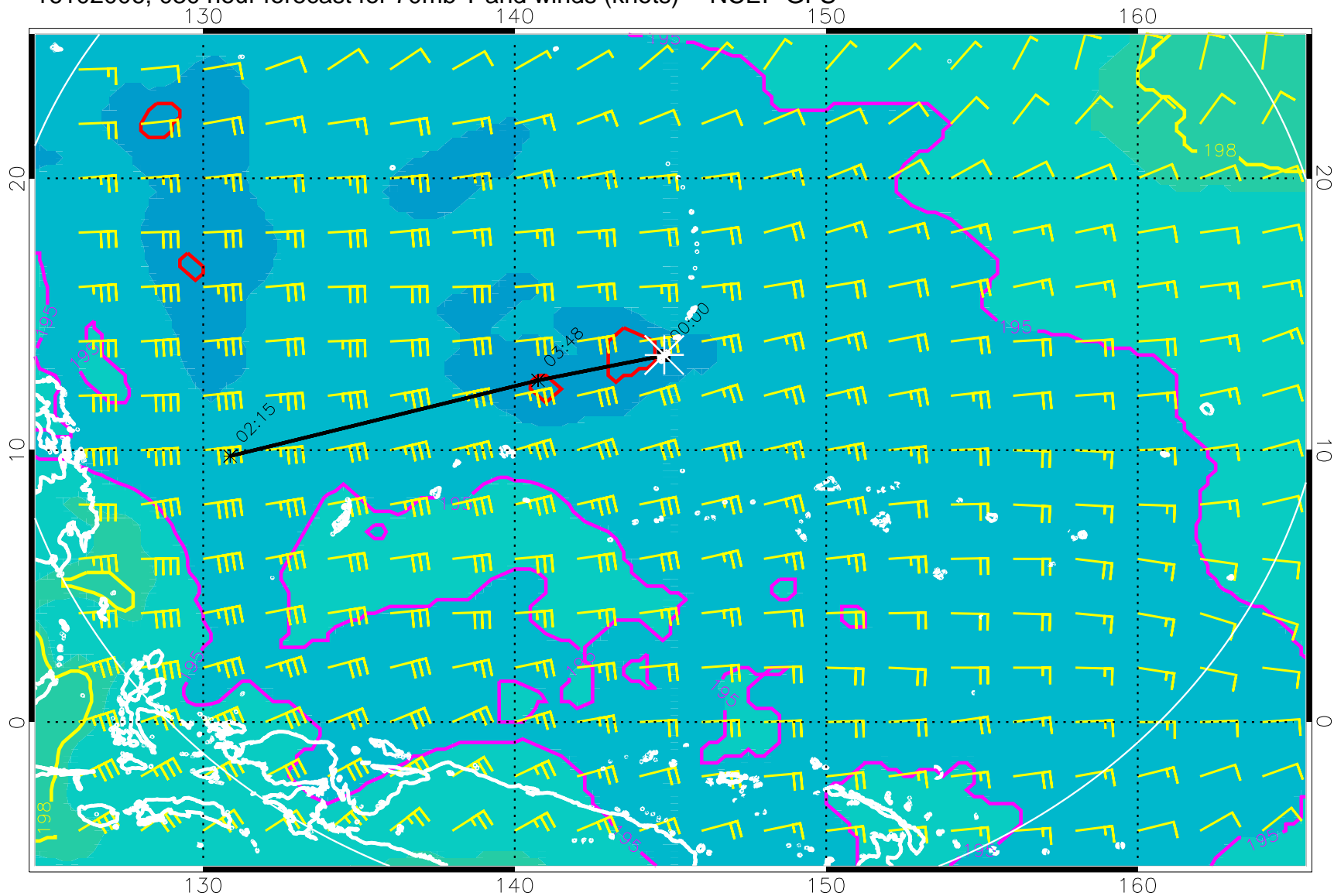
16102006, 030 hour forecast for 70mb T and winds (knots) -- NCEP GFS
