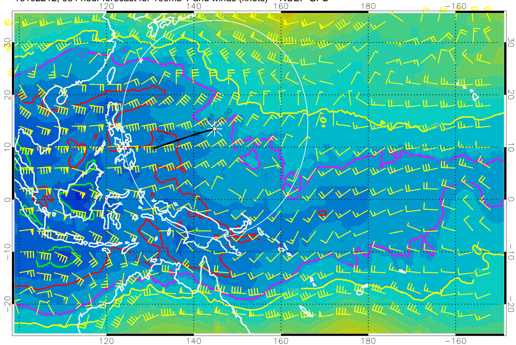
16102212, 084 hour forecast for 100mb T and winds (knots) -- NCEP GFS
