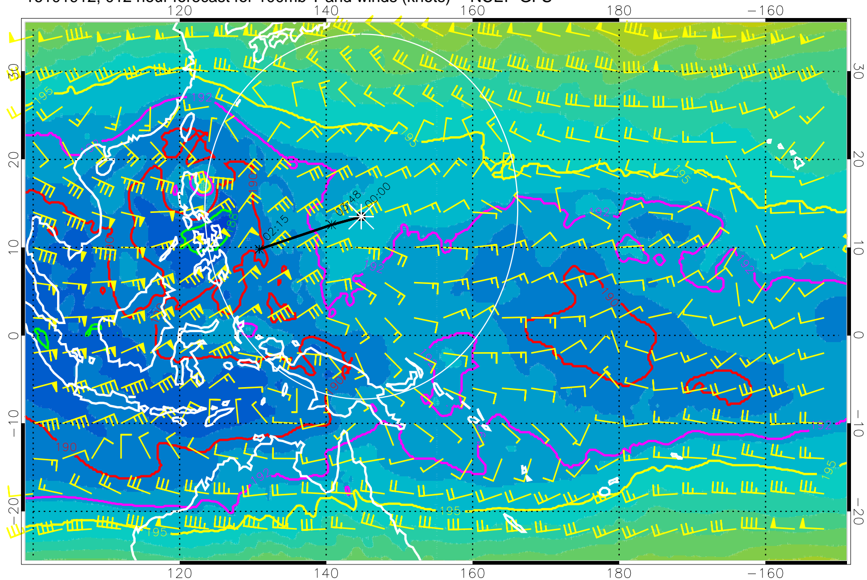
16101912, 012 hour forecast for 100mb T and winds (knots) -- NCEP GFS
