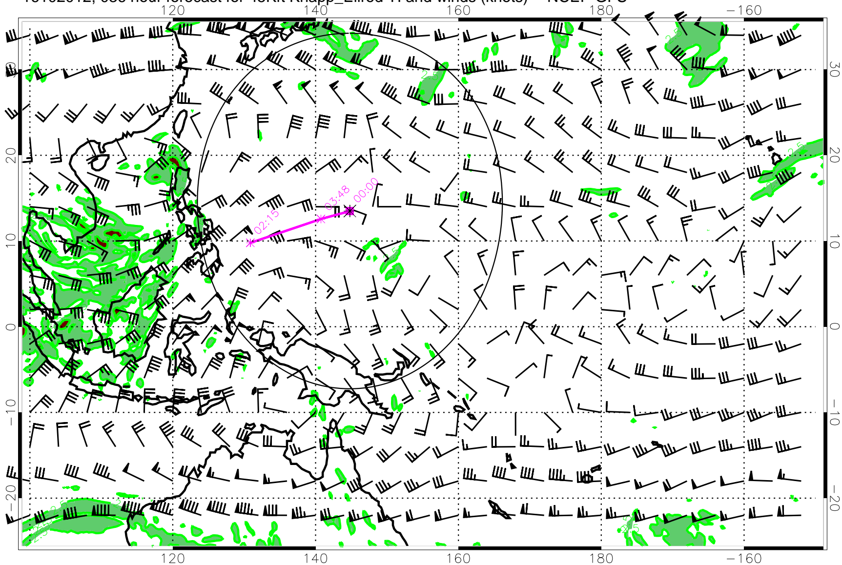
16102012, 036 hour forecast for 45Kft Knapp_Ellrod TI and winds (knots) -- NCEP GFS
