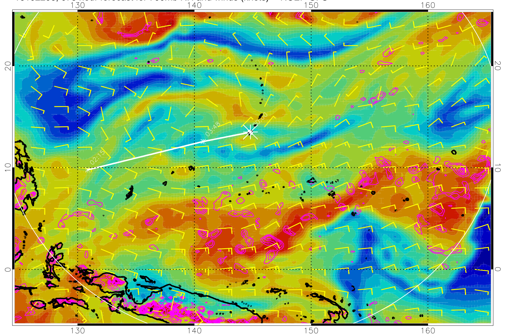
16102206, 078 hour forecast for 700mb RH and winds (knots) -- NCEP GFS
