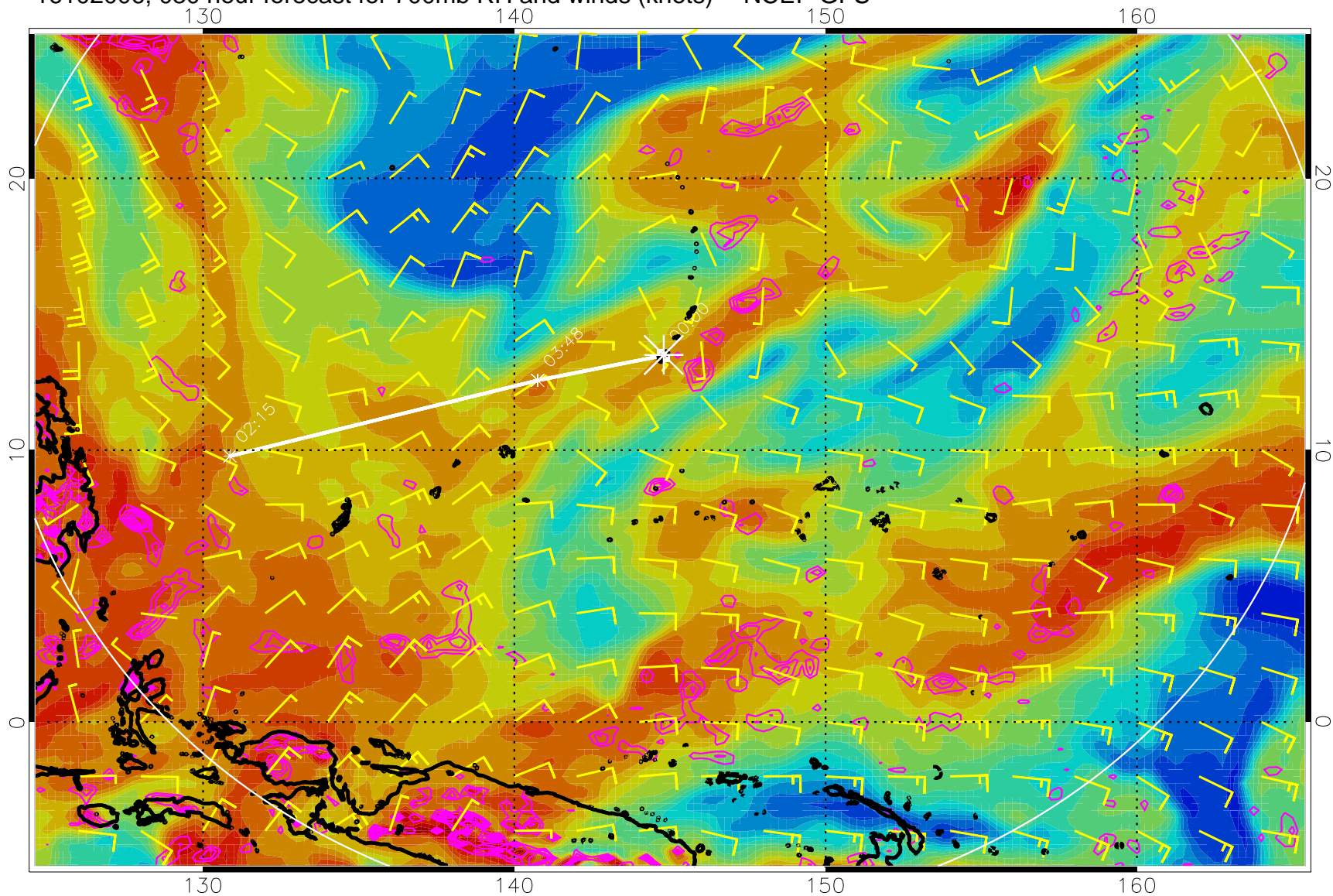
16102006, 030 hour forecast for 700mb RH and winds (knots) -- NCEP GFS
