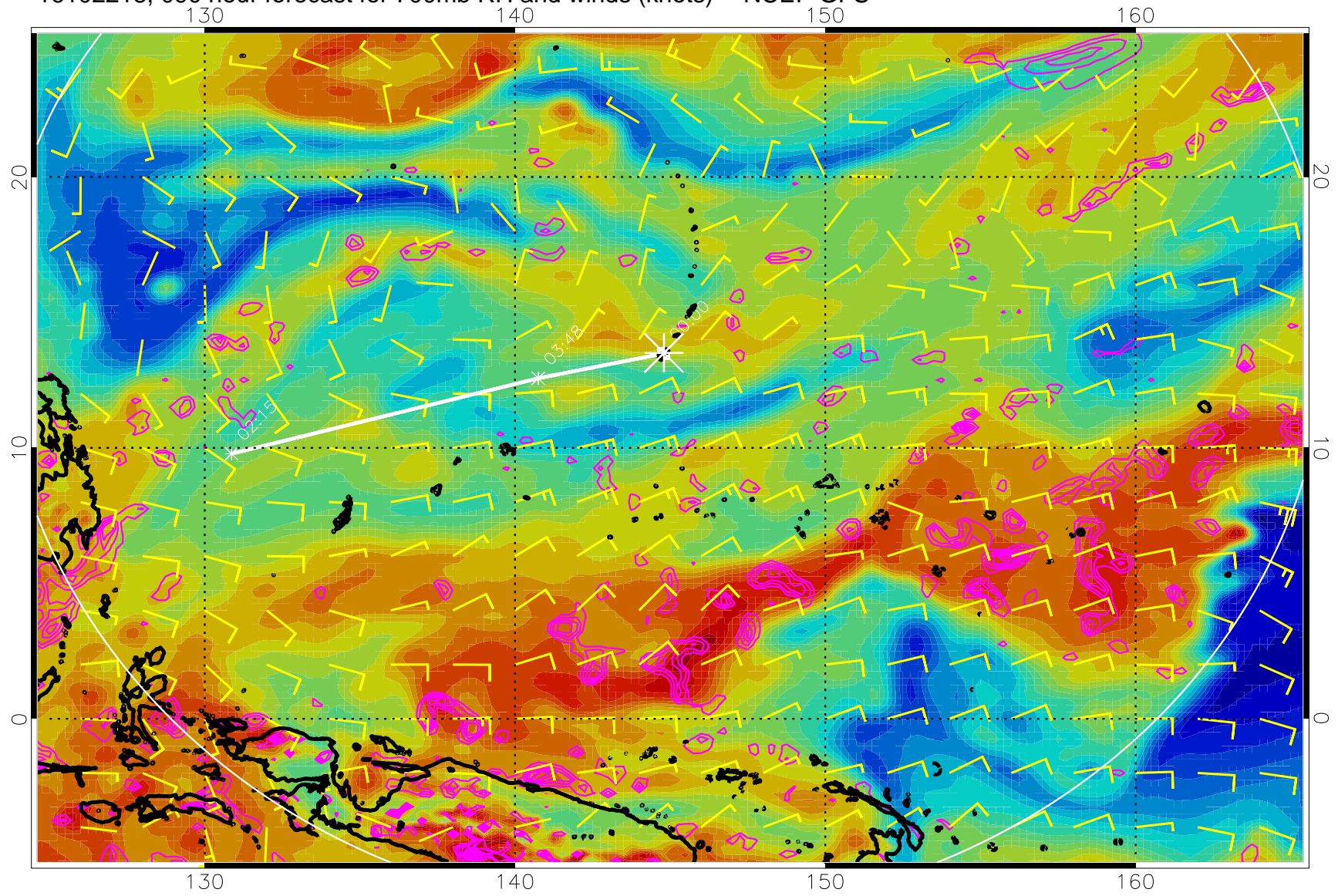
16102218, 090 hour forecast for 700mb RH and winds (knots) -- NCEP GFS
