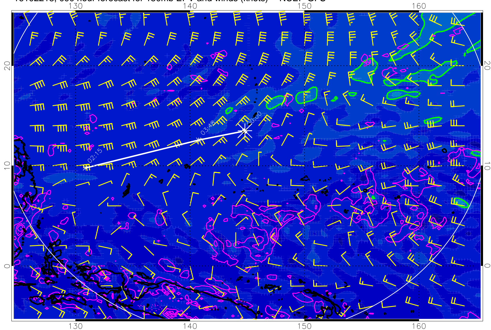
16102218, 090 hour forecast for 150mb EPV and winds (knots) -- NCEP GFS
