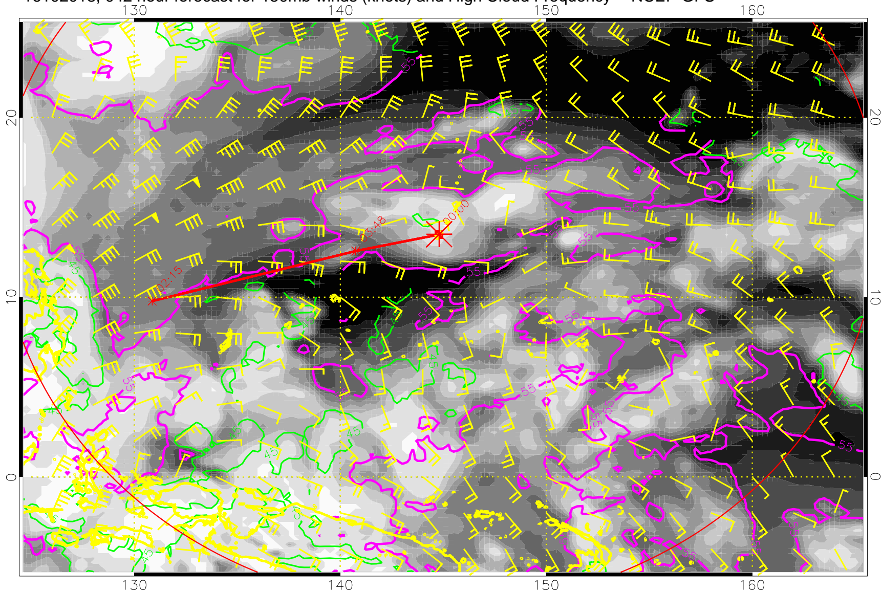
16102018, 042 hour forecast for 150mb winds (knots) and High Cloud Frequency -- NCEP GFS
