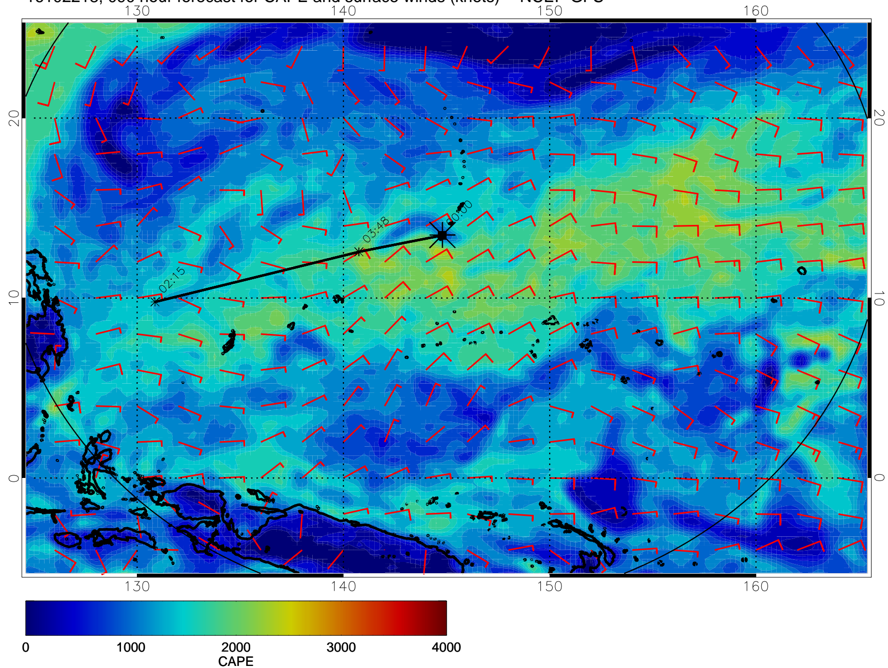
16102218, 090 hour forecast for CAPE and surface winds (knots) -- NCEP GFS
