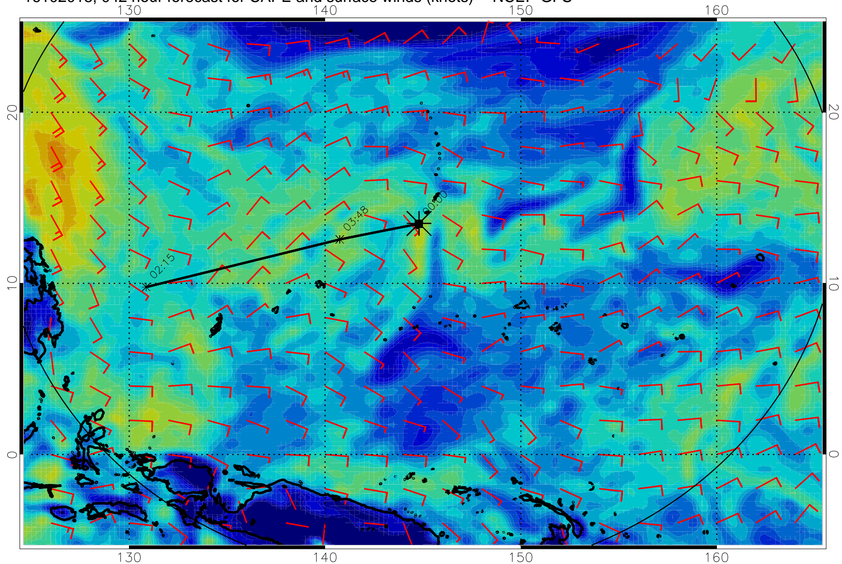
16102018, 042 hour forecast for CAPE and surface winds (knots) -- NCEP GFS
