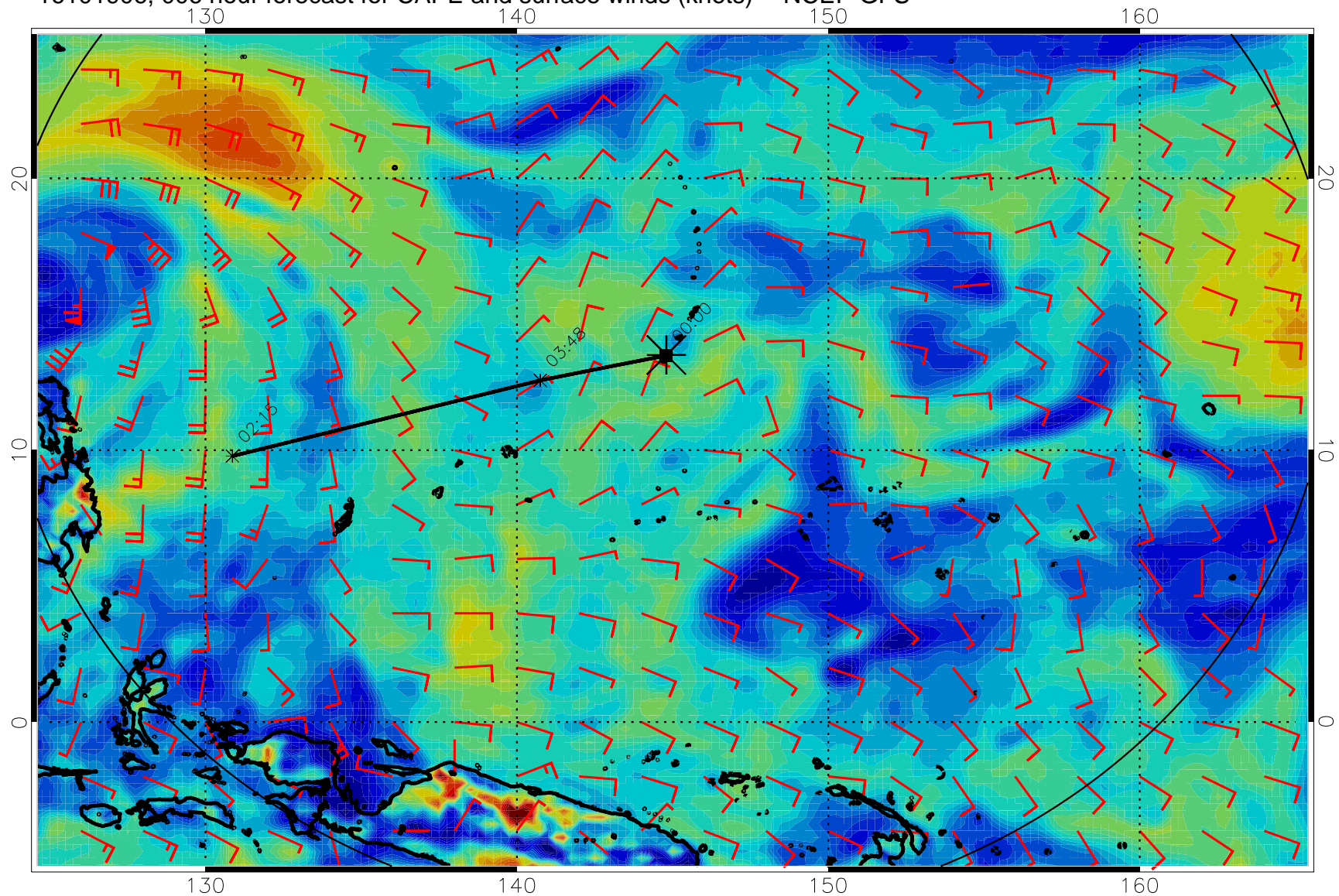
16101906, 006 hour forecast for CAPE and surface winds (knots) -- NCEP GFS
