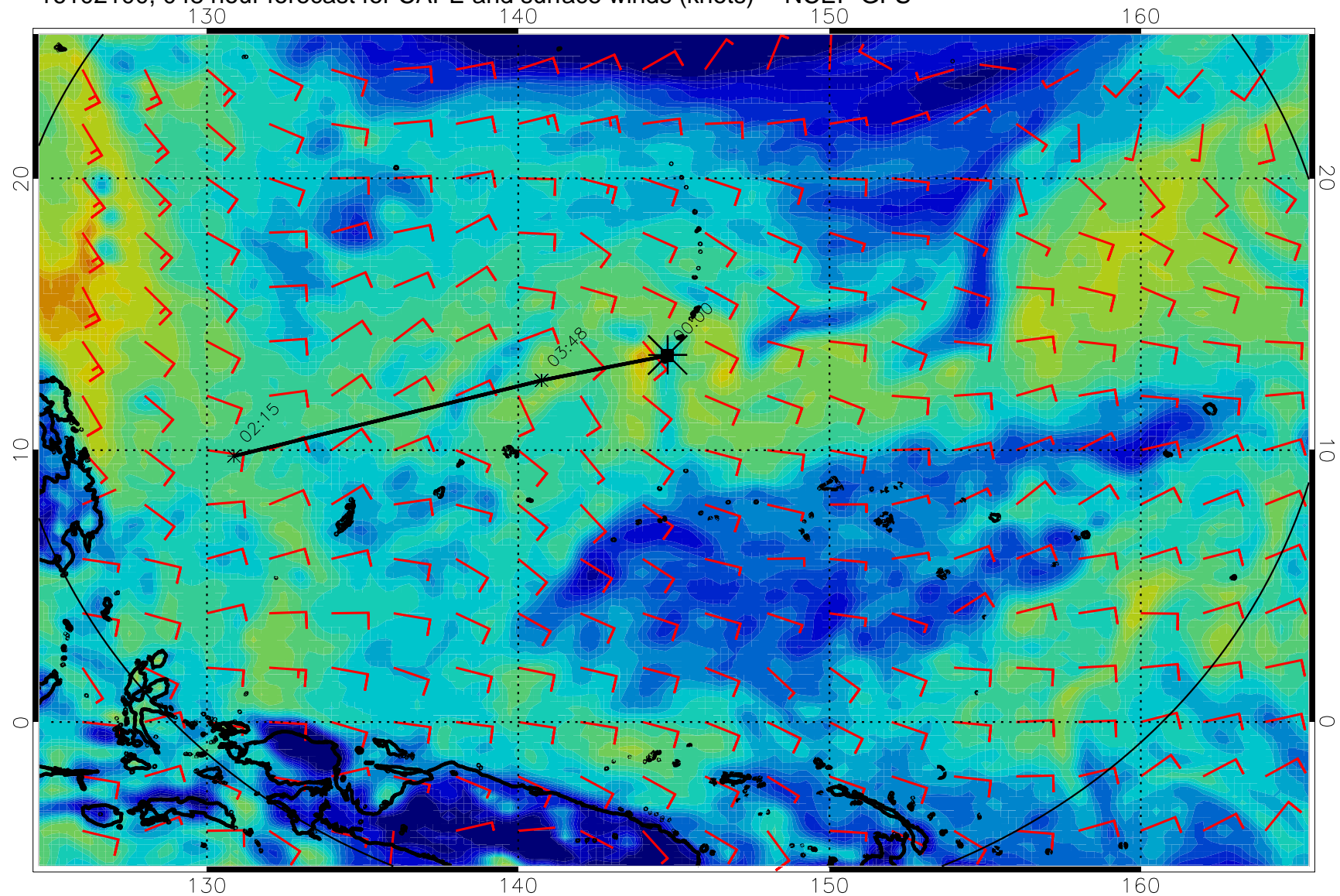
16102100, 048 hour forecast for CAPE and surface winds (knots) -- NCEP GFS
