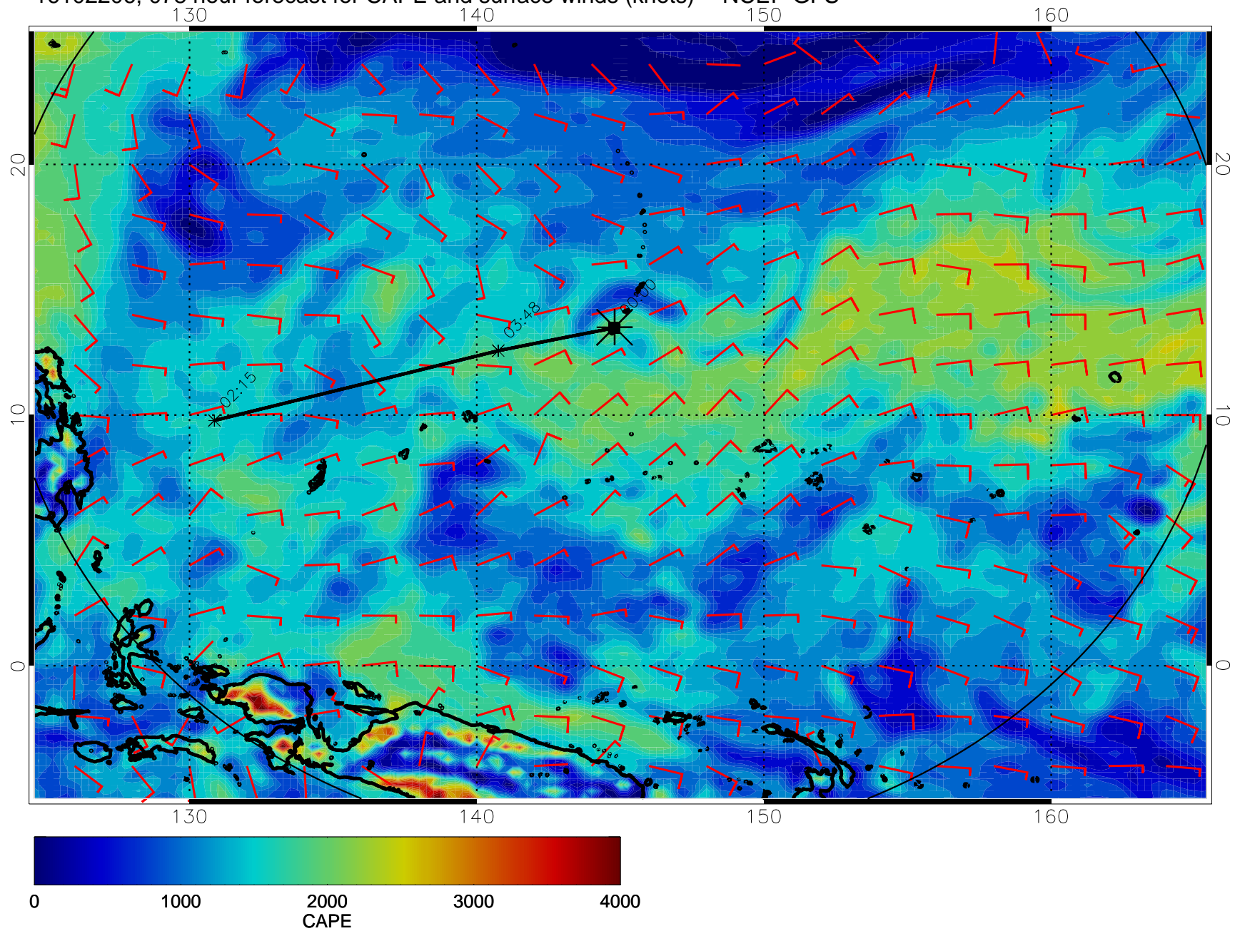
16102206, 078 hour forecast for CAPE and surface winds (knots) -- NCEP GFS
