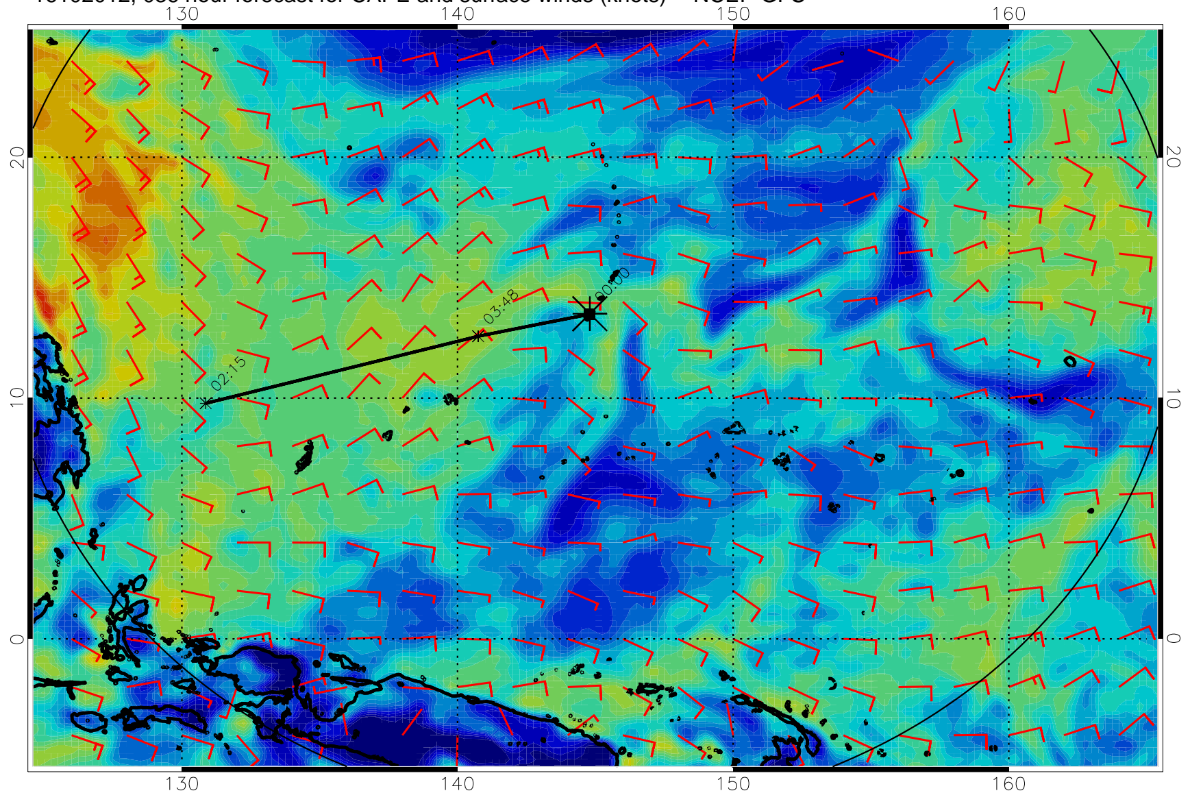
16102012, 036 hour forecast for CAPE and surface winds (knots) -- NCEP GFS
