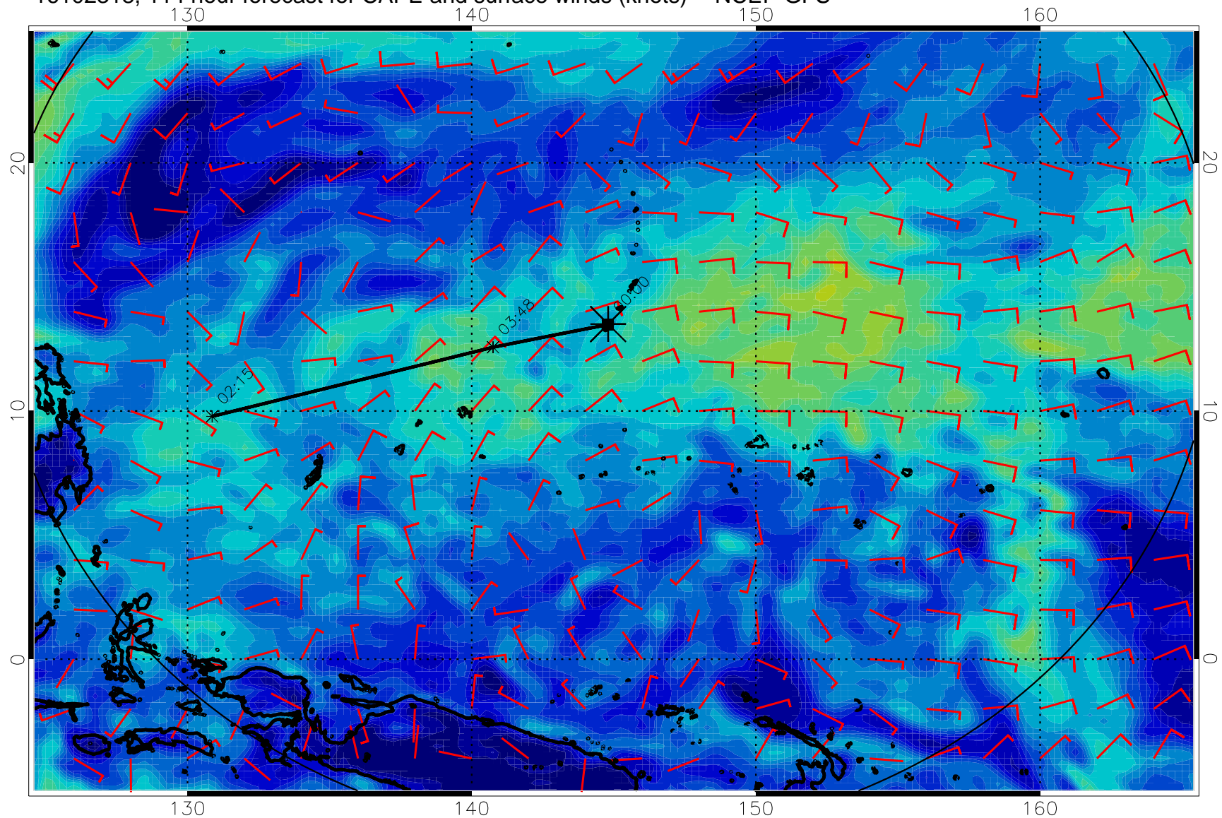
16102318, 114 hour forecast for CAPE and surface winds (knots) -- NCEP GFS
