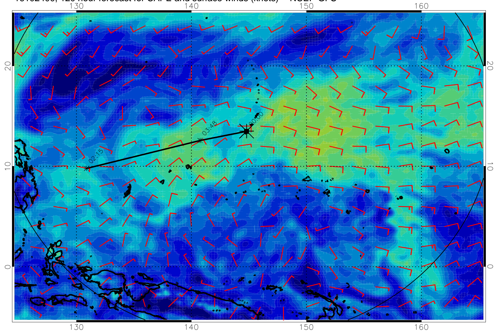
16102400, 120 hour forecast for CAPE and surface winds (knots) -- NCEP GFS
