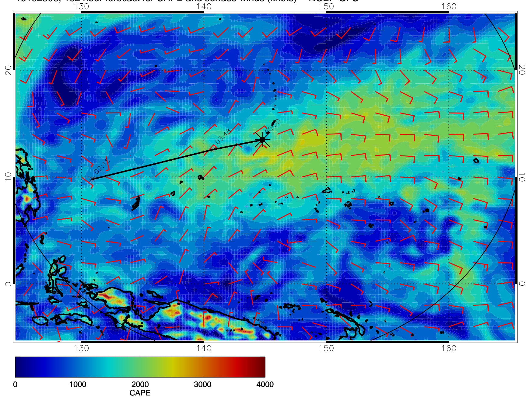
16102306, 102 hour forecast for CAPE and surface winds (knots) -- NCEP GFS
