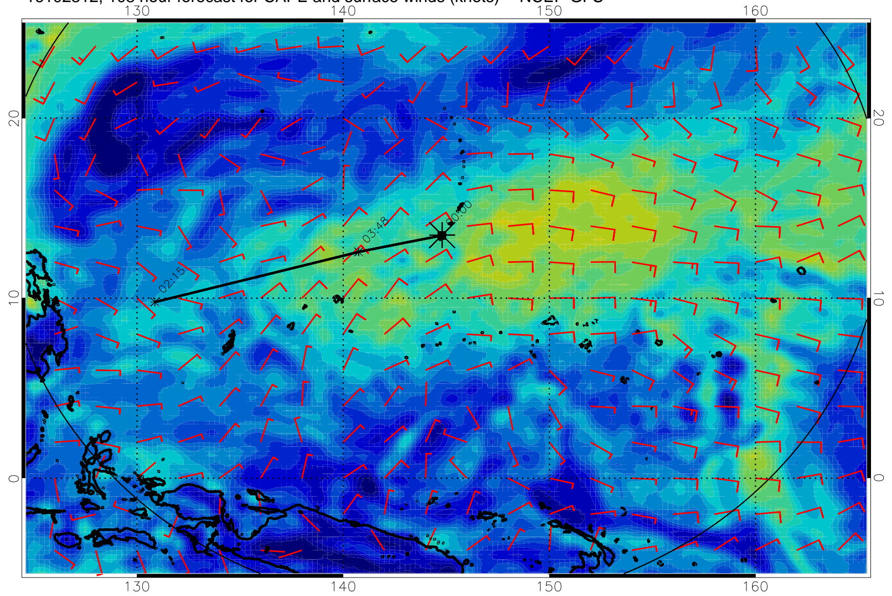
16102312, 108 hour forecast for CAPE and surface winds (knots) -- NCEP GFS
