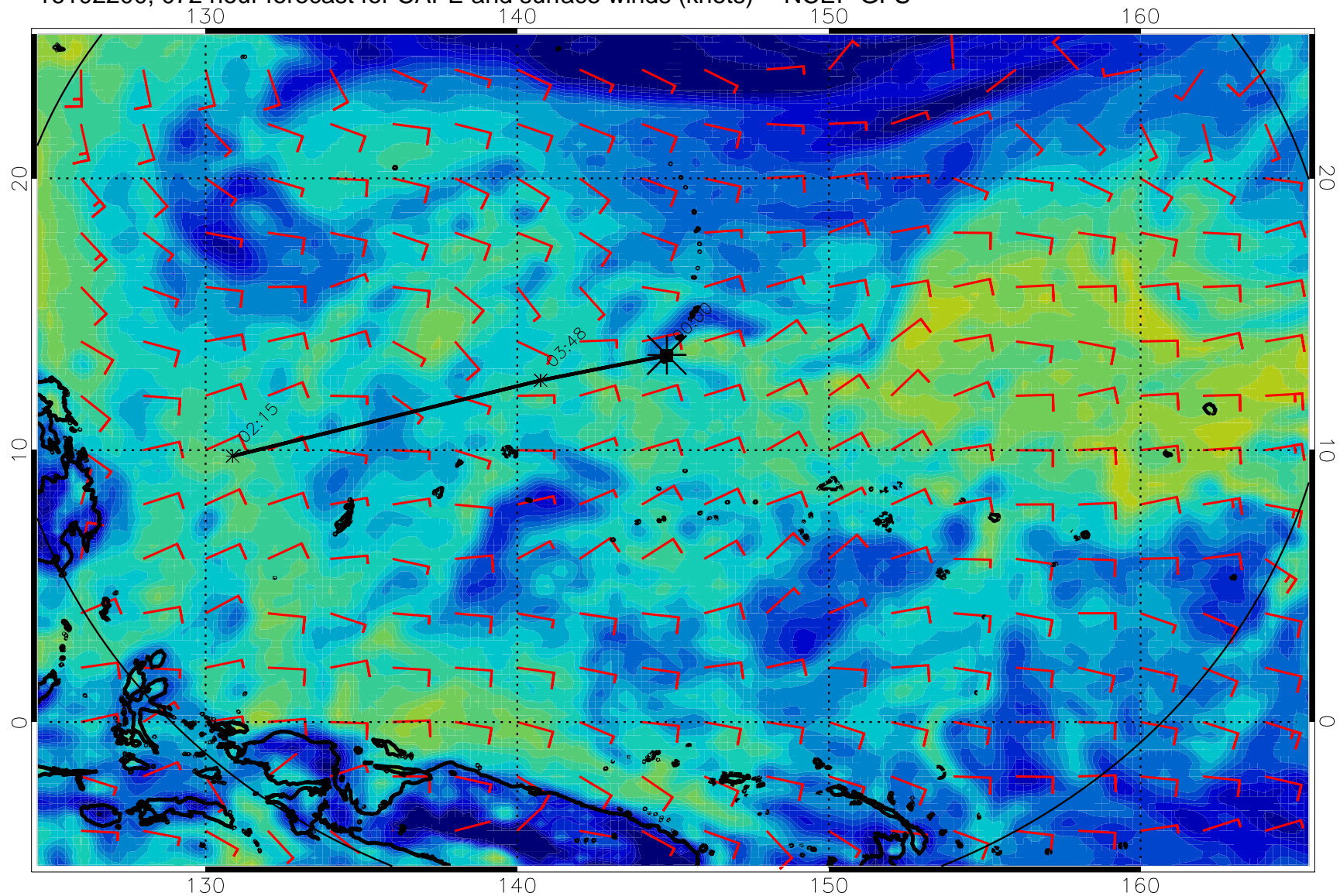
16102200, 072 hour forecast for CAPE and surface winds (knots) -- NCEP GFS
