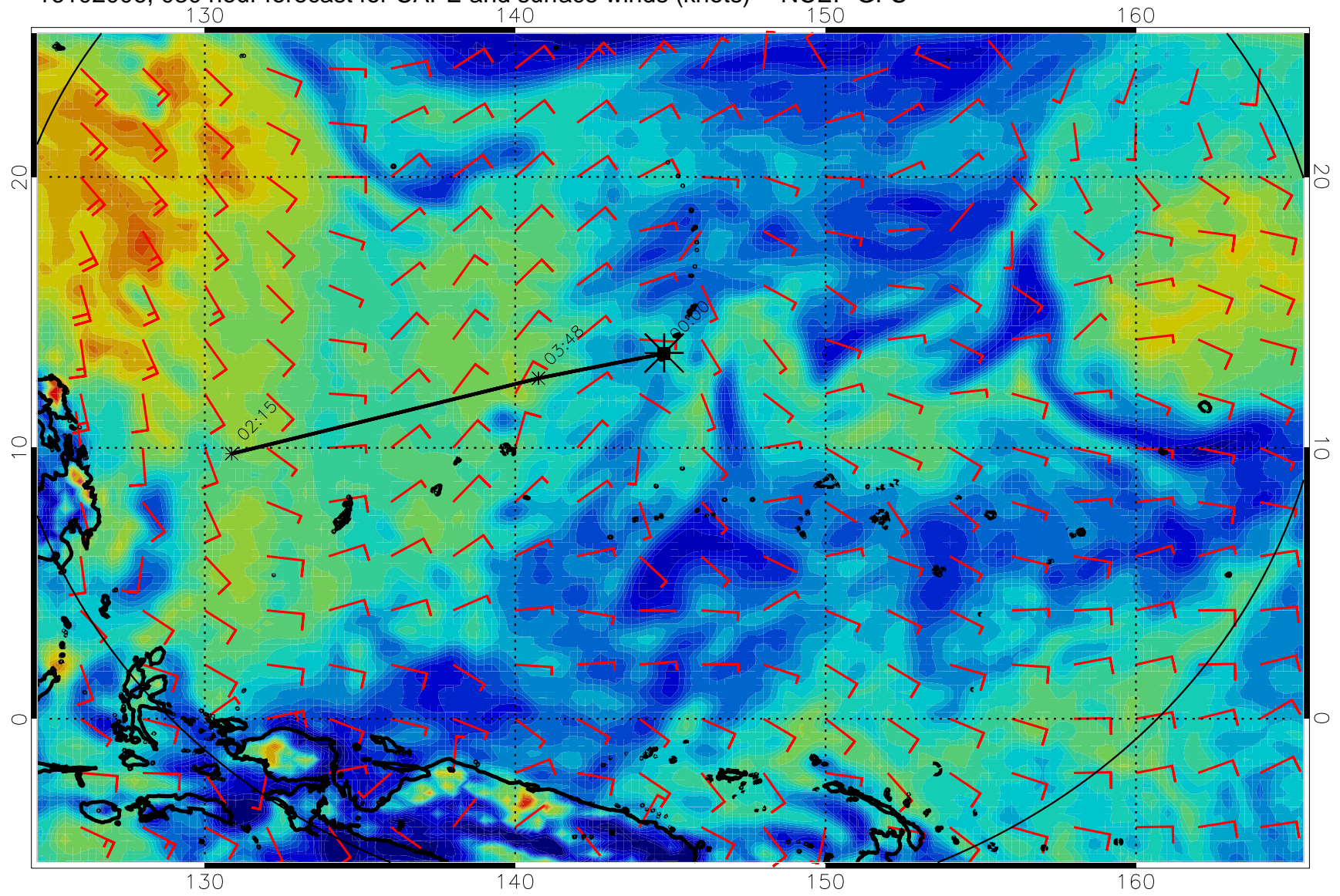
16102006, 030 hour forecast for CAPE and surface winds (knots) -- NCEP GFS
