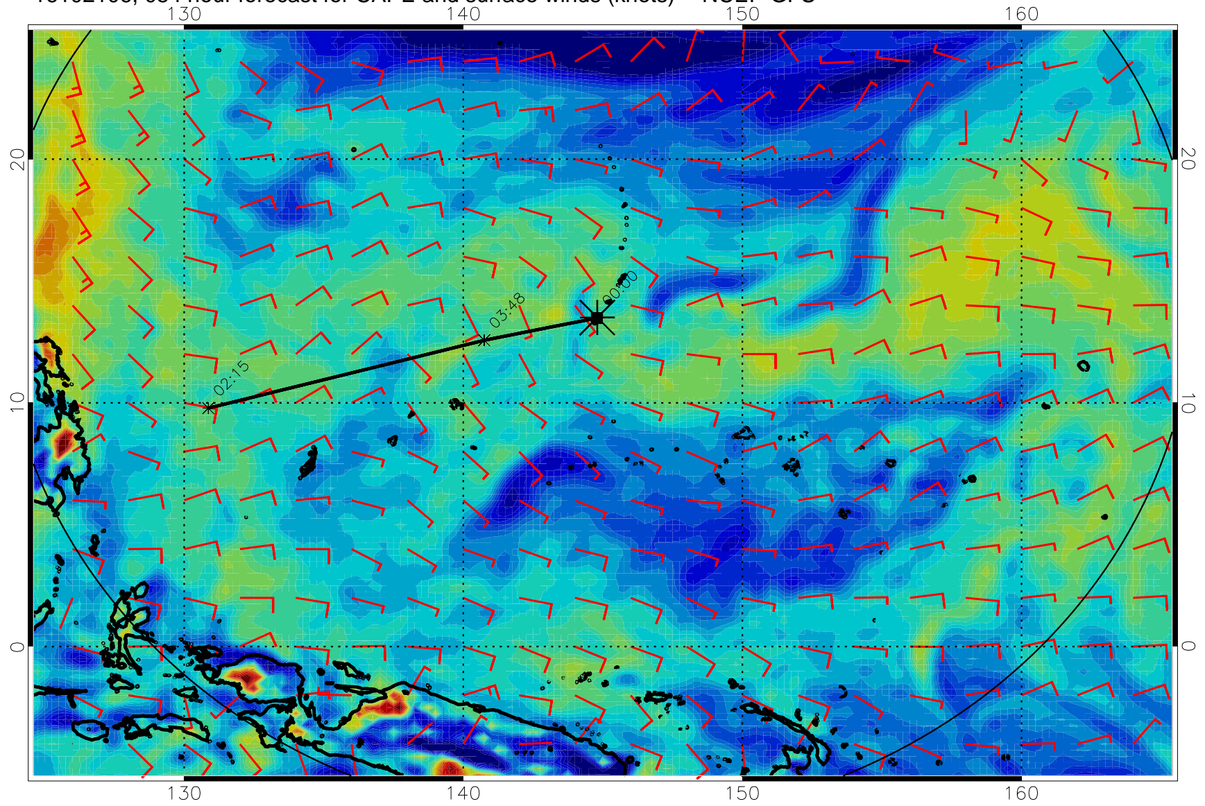
16102106, 054 hour forecast for CAPE and surface winds (knots) -- NCEP GFS
