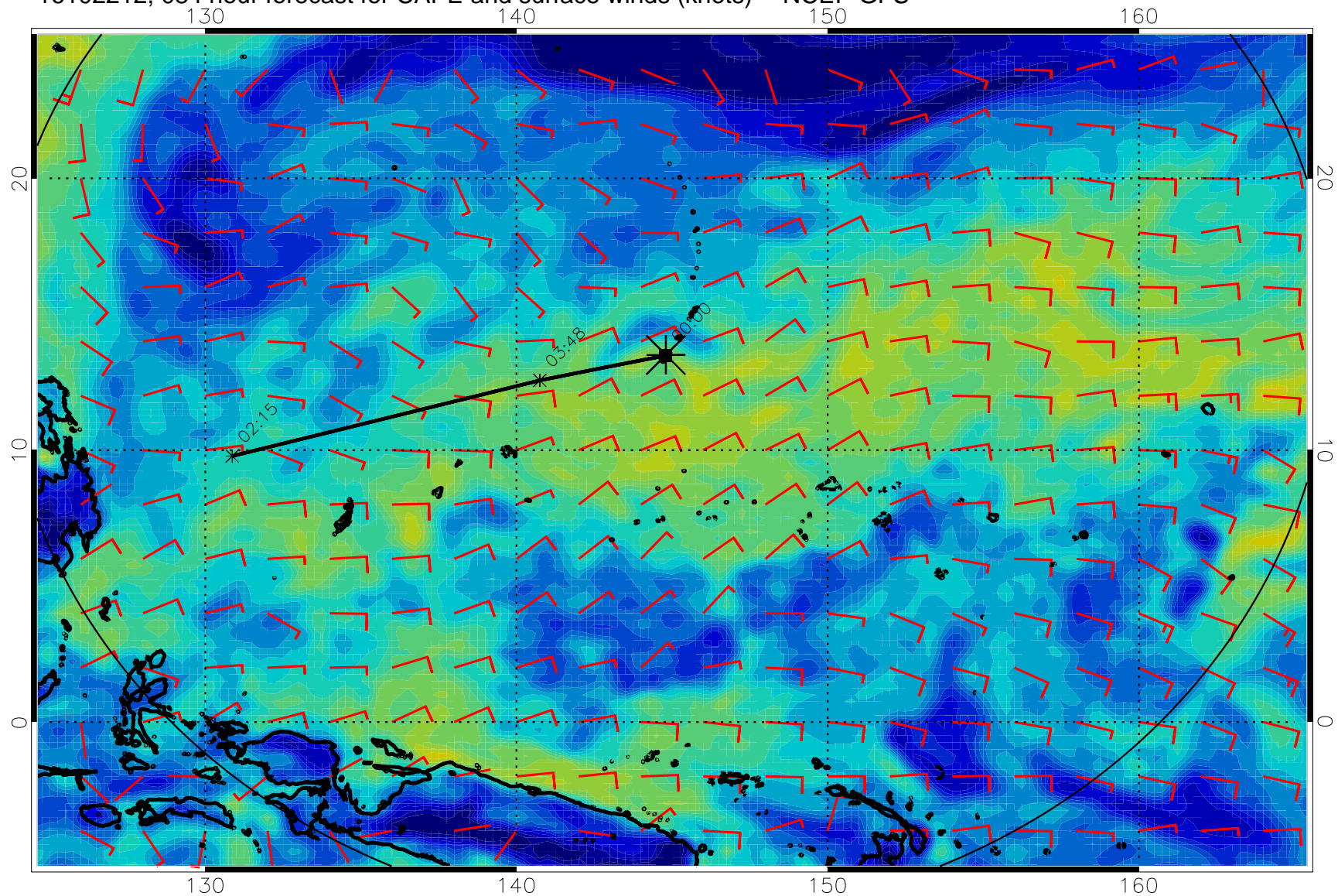
16102212, 084 hour forecast for CAPE and surface winds (knots) -- NCEP GFS
