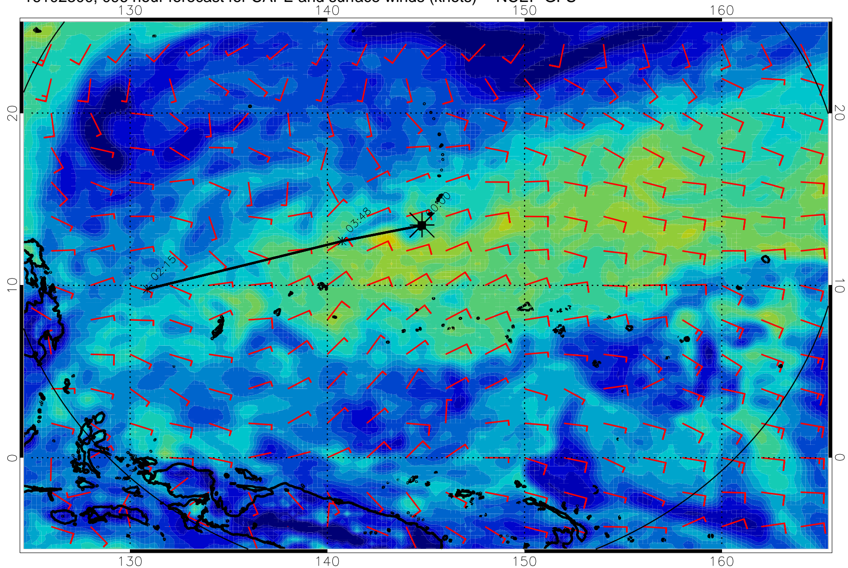
16102300, 096 hour forecast for CAPE and surface winds (knots) -- NCEP GFS
