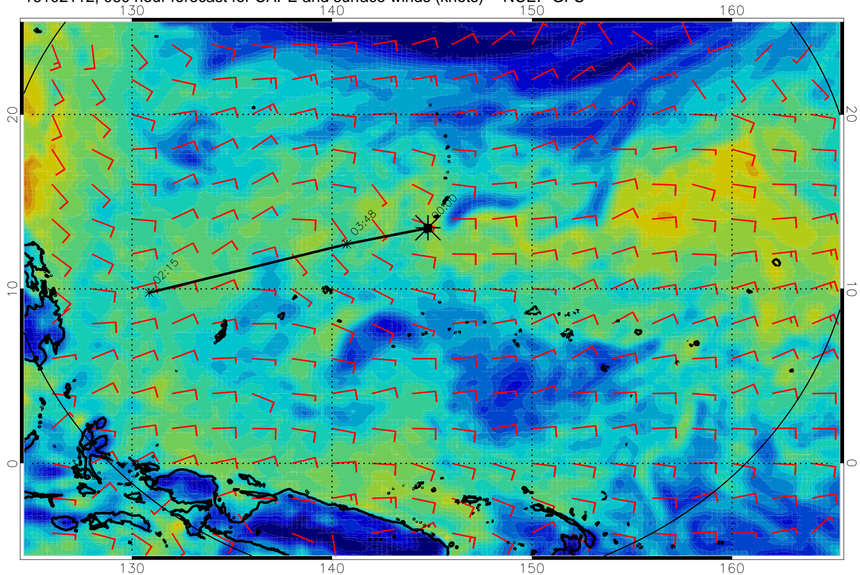
16102112, 060 hour forecast for CAPE and surface winds (knots) -- NCEP GFS
