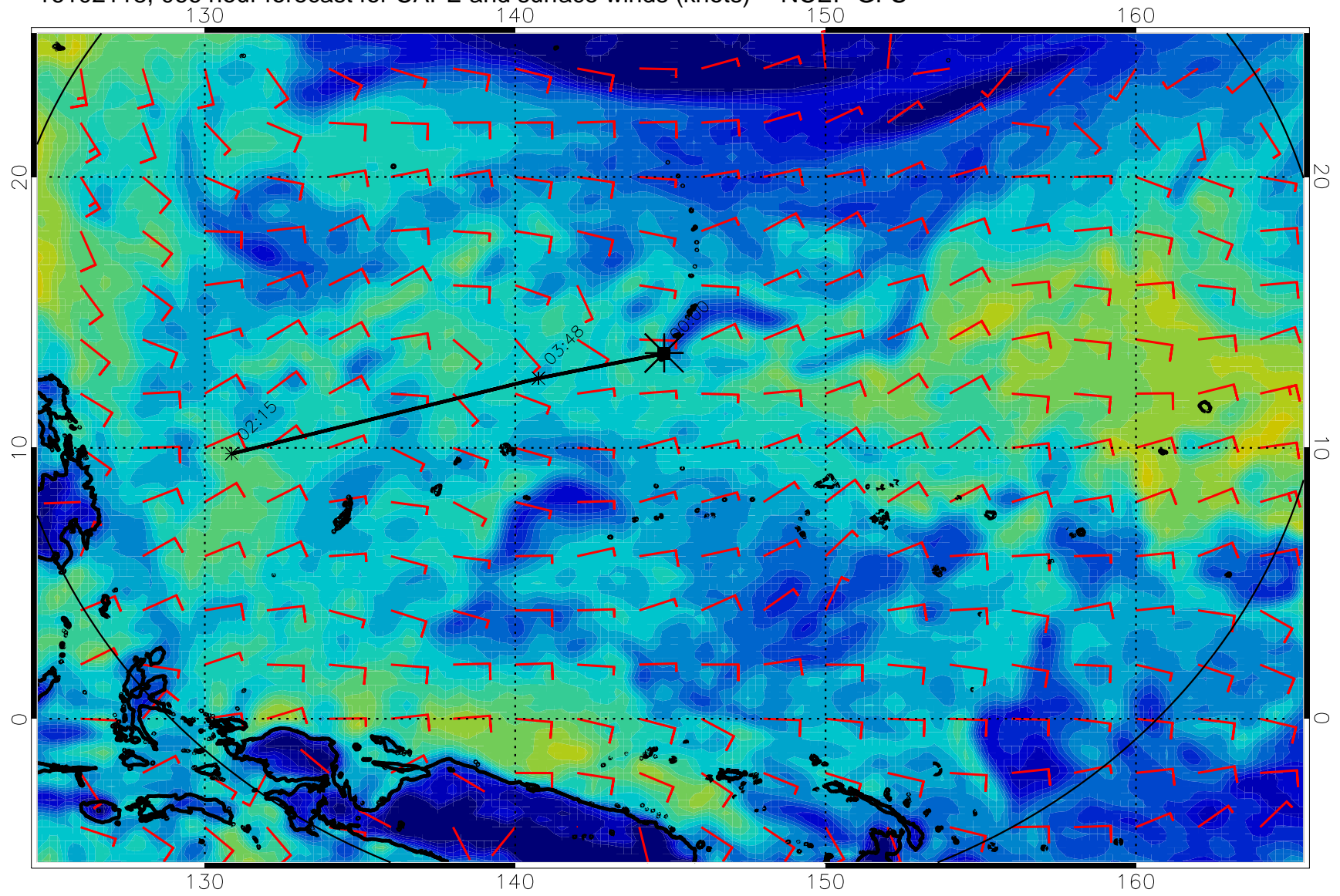
16102118, 066 hour forecast for CAPE and surface winds (knots) -- NCEP GFS
