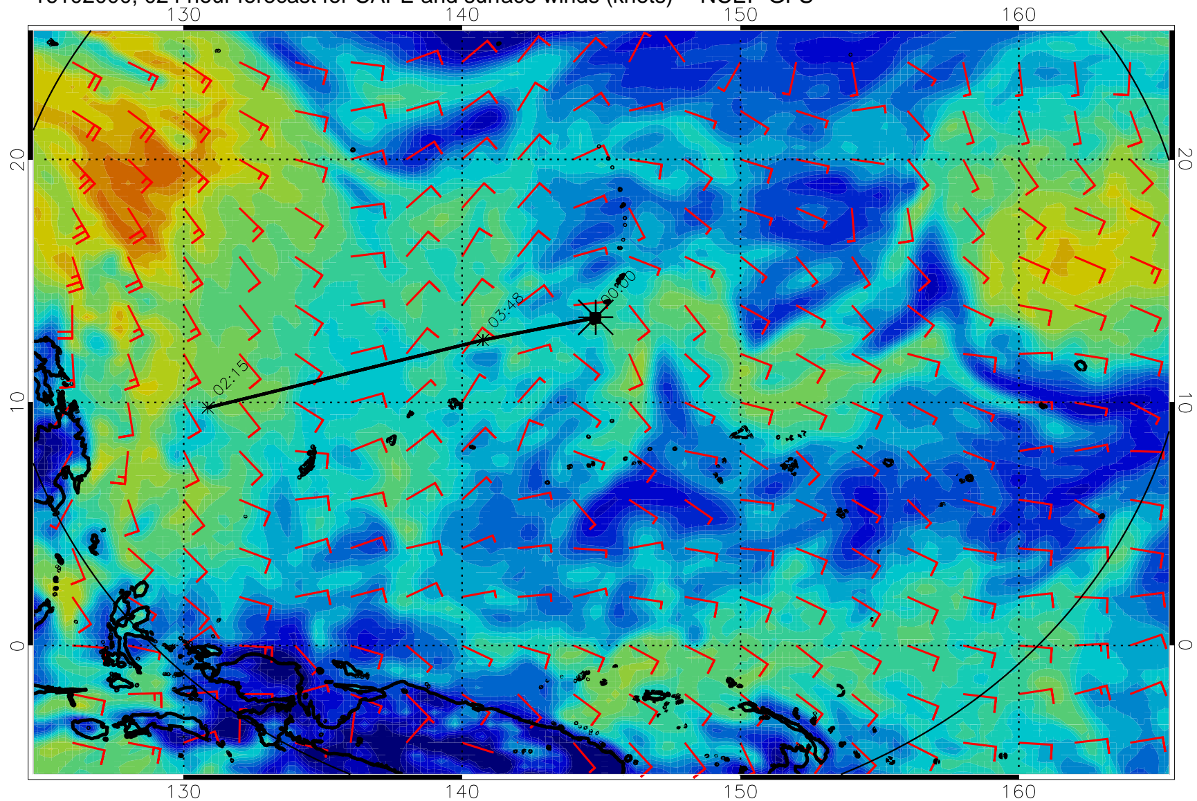
16102000, 024 hour forecast for CAPE and surface winds (knots) -- NCEP GFS
