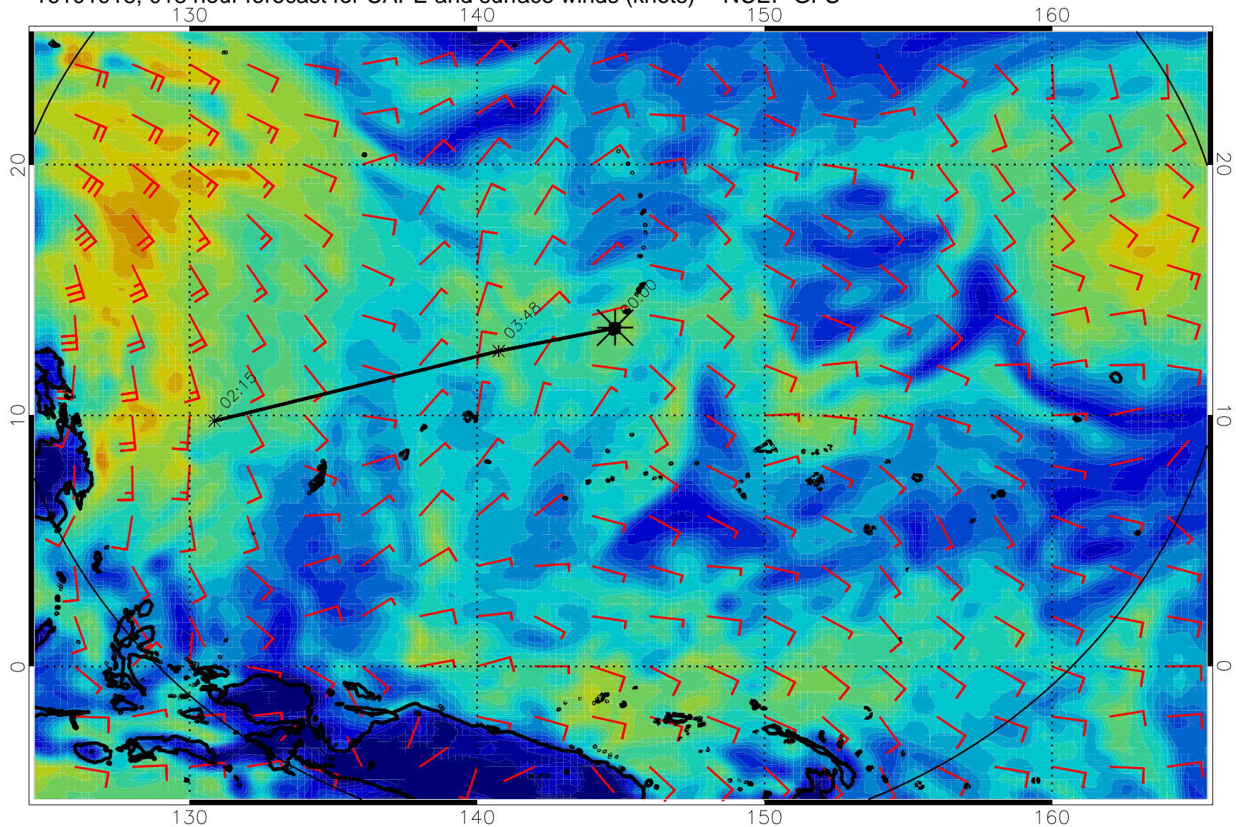
16101918, 018 hour forecast for CAPE and surface winds (knots) -- NCEP GFS
