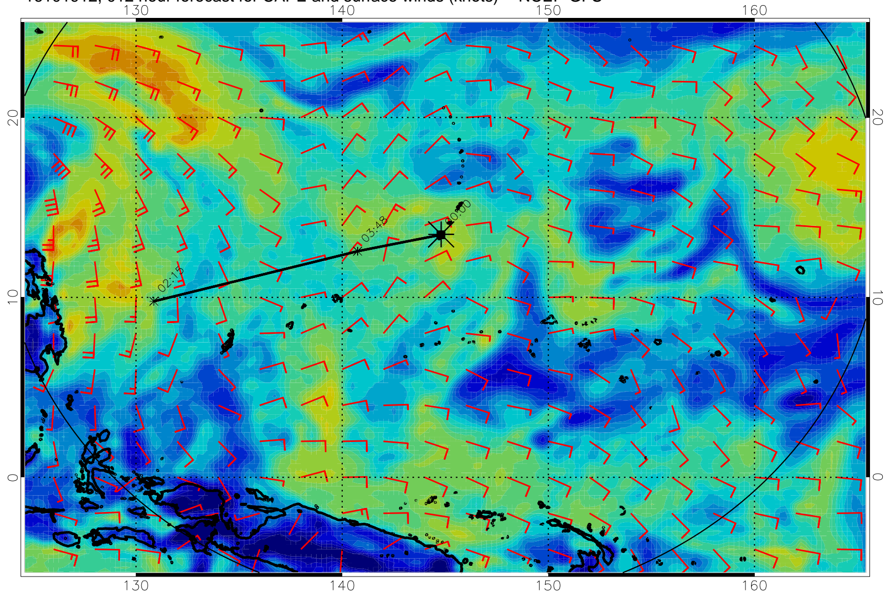
16101912, 012 hour forecast for CAPE and surface winds (knots) -- NCEP GFS
