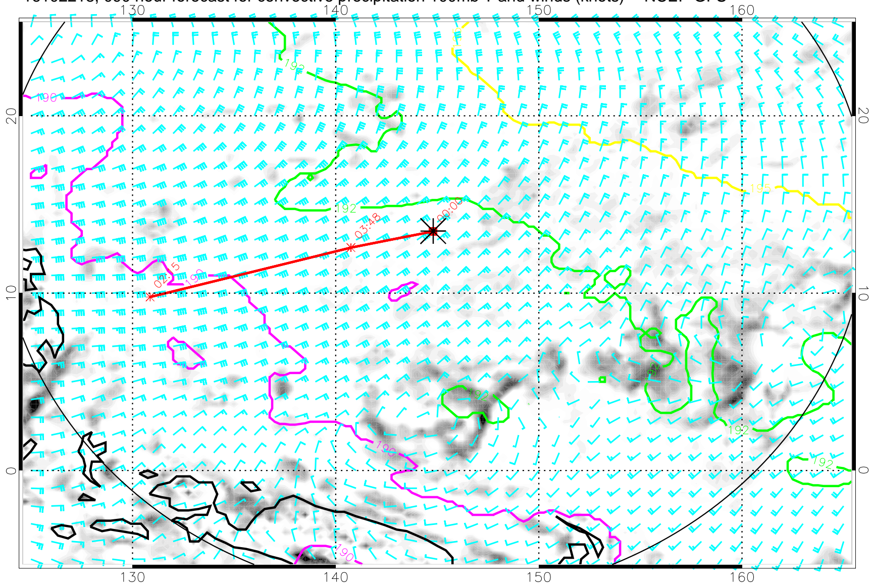
16102218, 090 hour forecast for convective precipitation 100mb T and winds (knots) -- NCEP GFS
