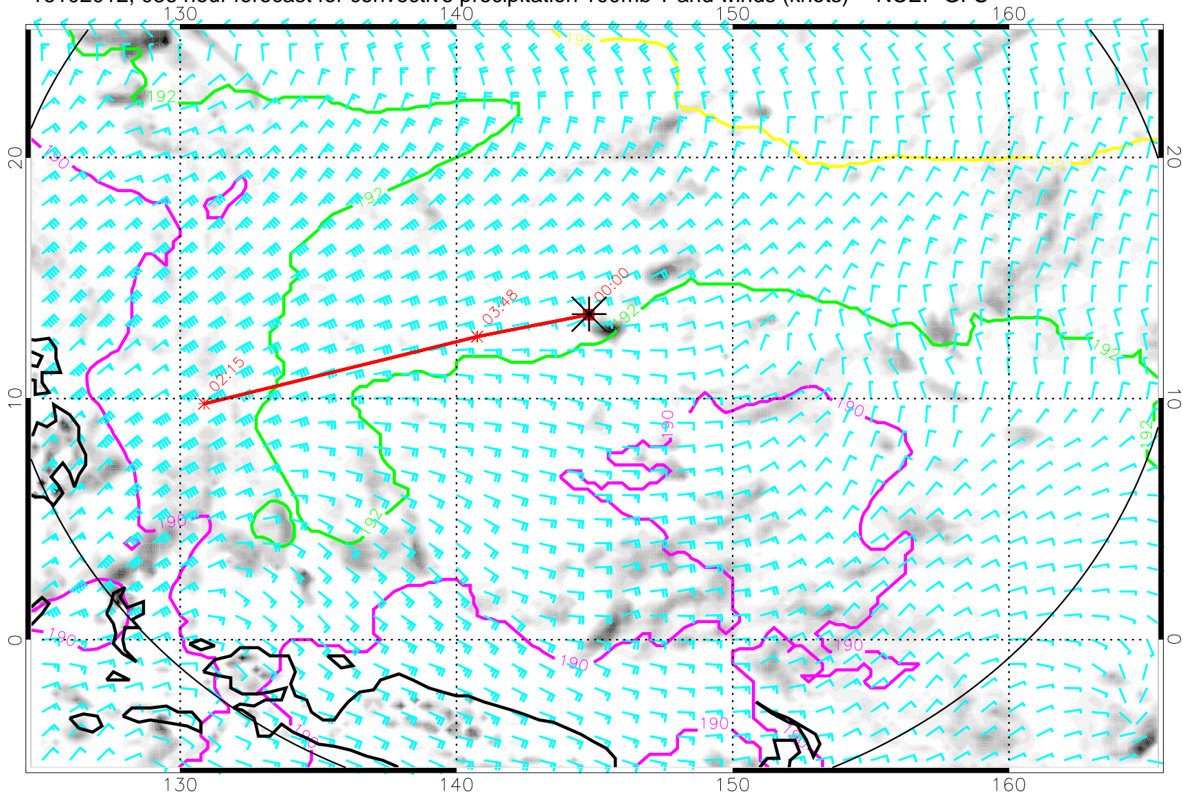
16102012, 036 hour forecast for convective precipitation 100mb T and winds (knots) -- NCEP GFS
