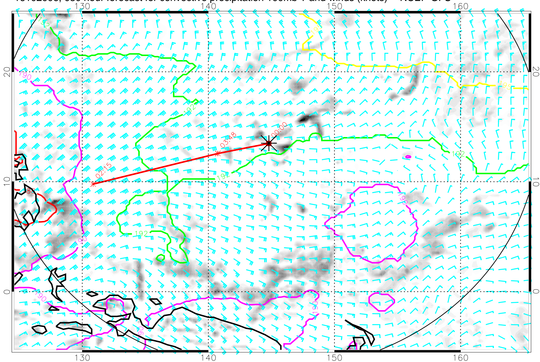
16102006, 030 hour forecast for convective precipitation 100mb T and winds (knots) -- NCEP GFS
