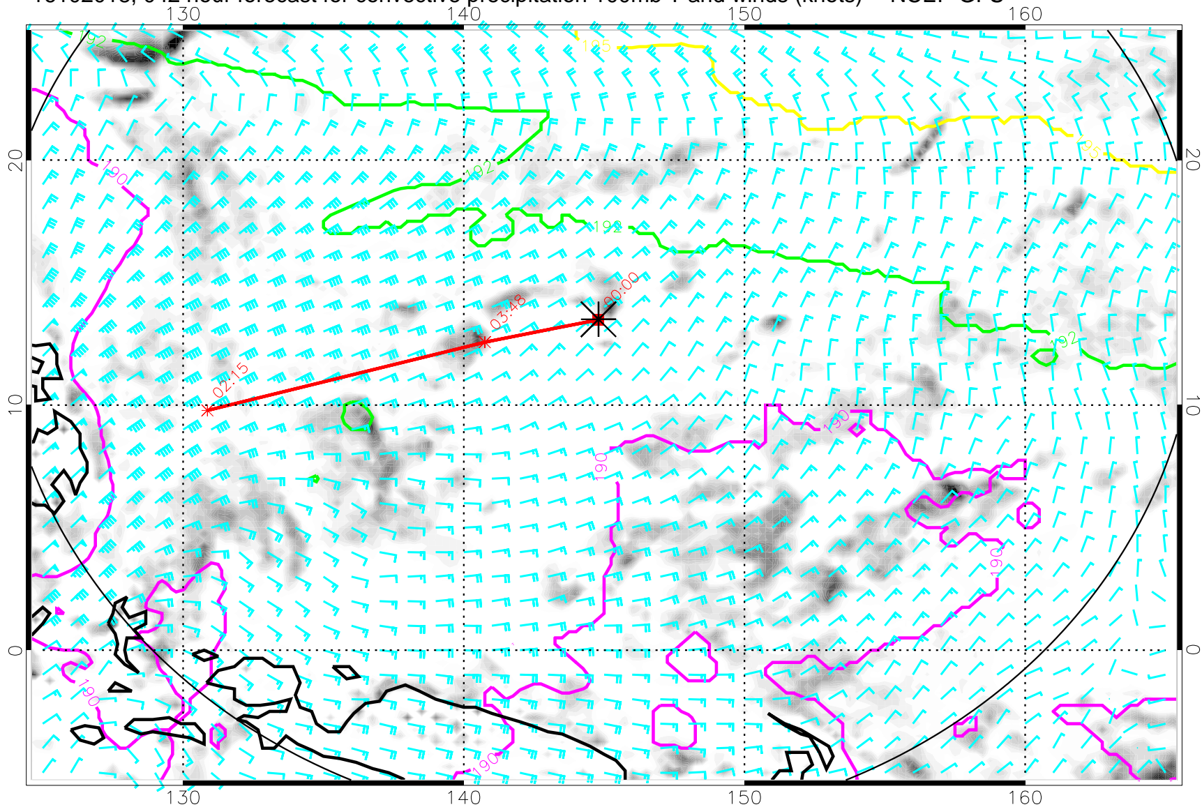
16102018, 042 hour forecast for convective precipitation 100mb T and winds (knots) -- NCEP GFS
