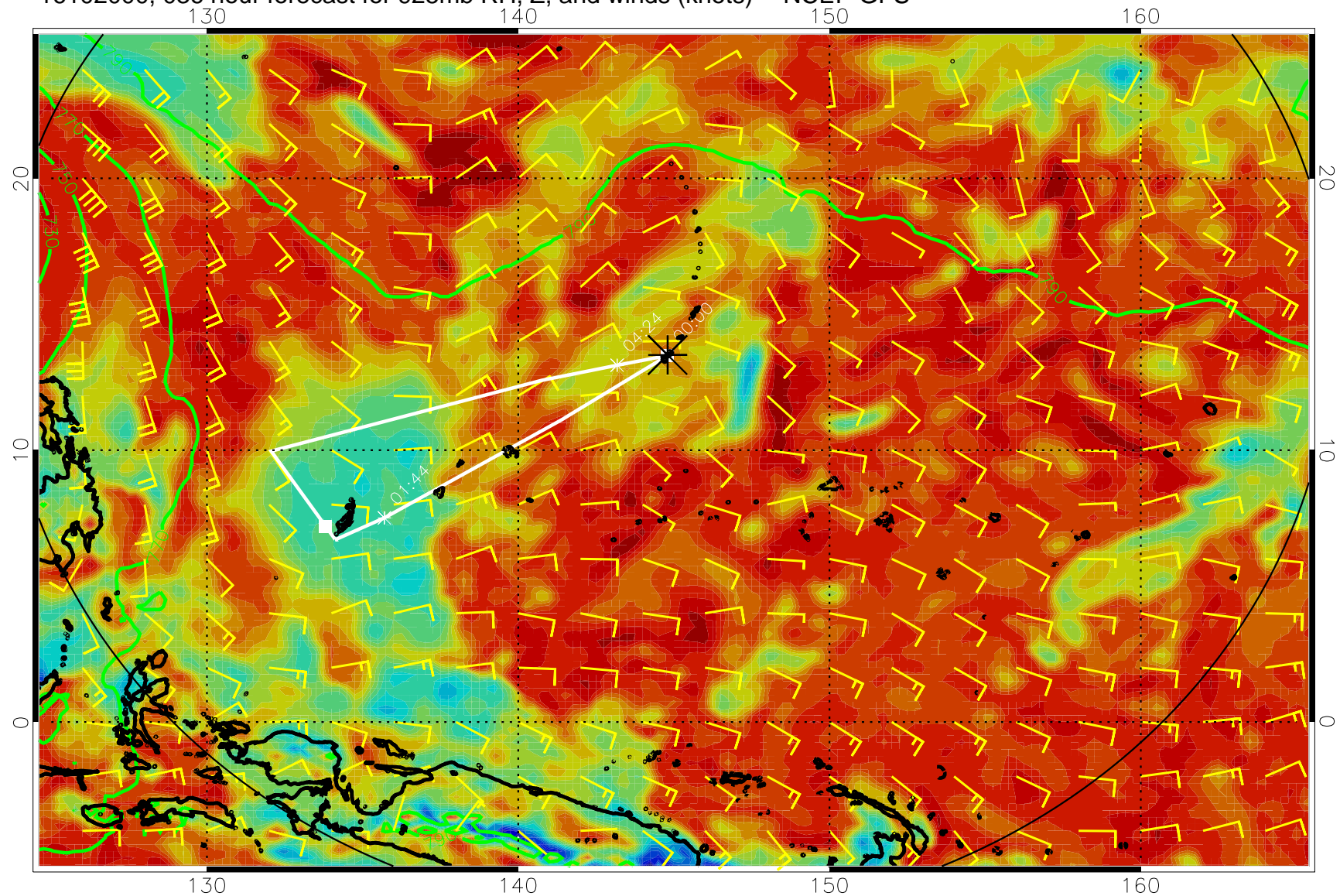
16102000, 036 hour forecast for 925mb RH, Z, and winds (knots) -- NCEP GFS
