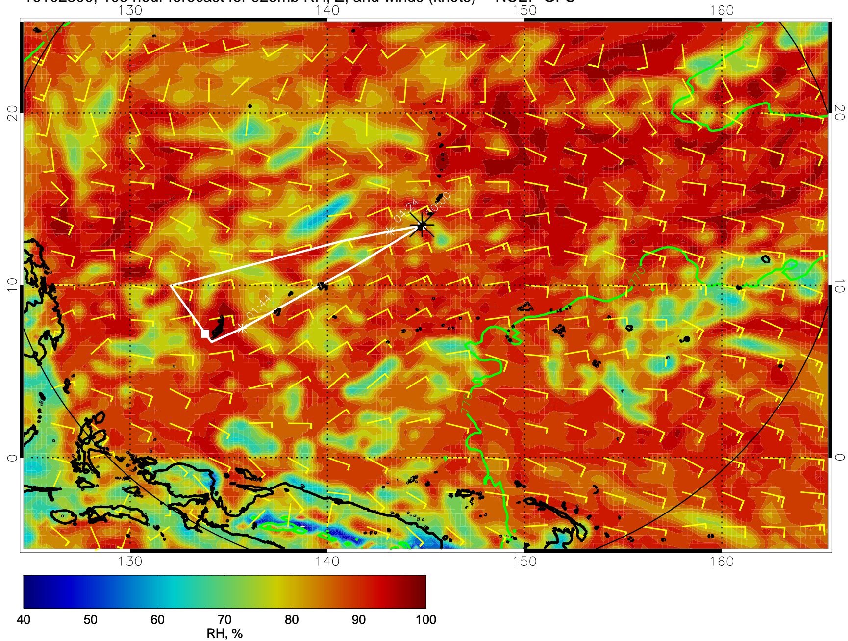
16102300, 108 hour forecast for 925mb RH, Z, and winds (knots) -- NCEP GFS
