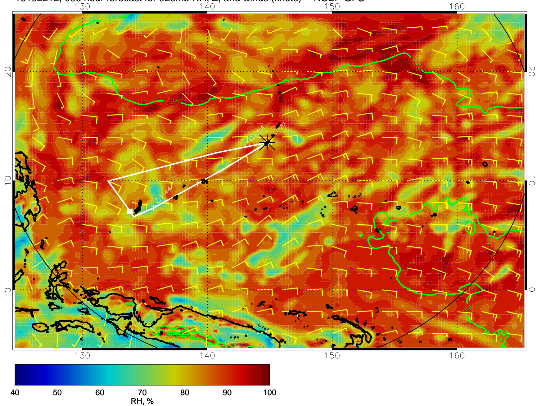
16102212, 096 hour forecast for 925mb RH, Z, and winds (knots) -- NCEP GFS
