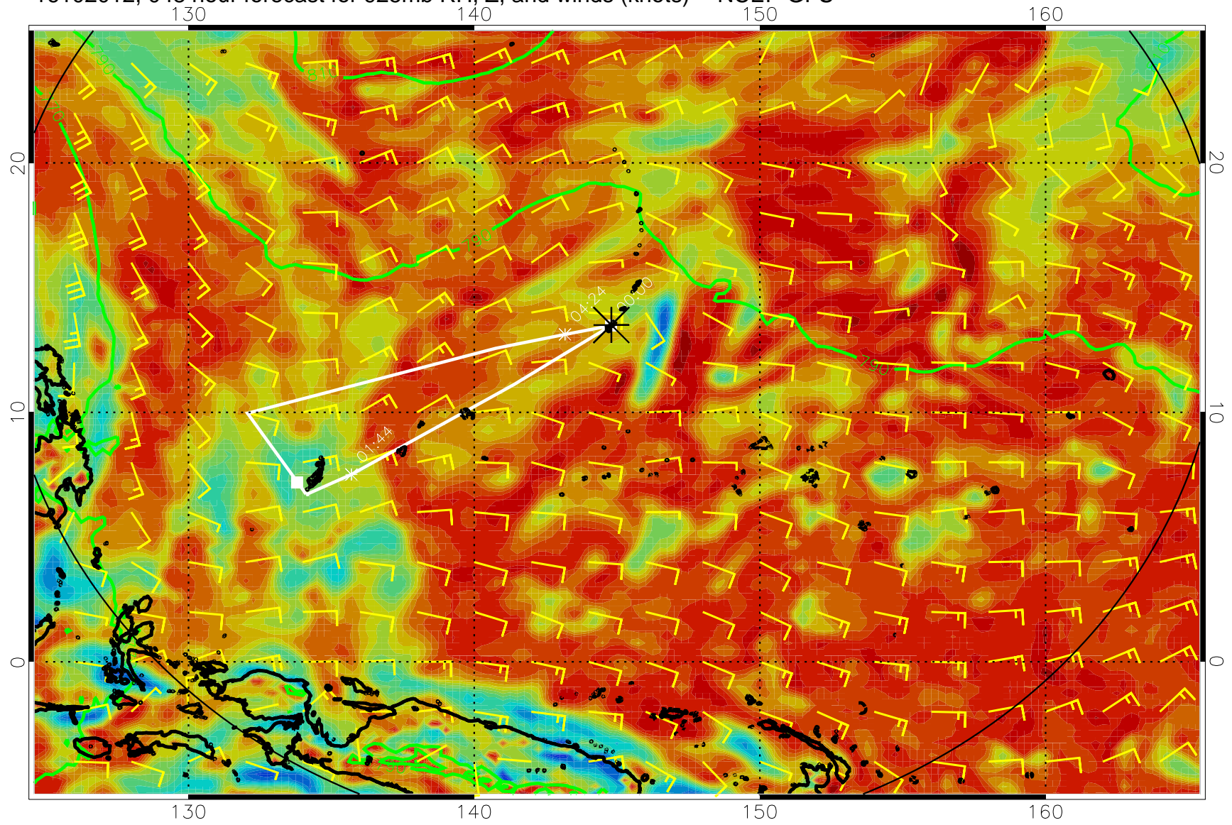
16102012, 048 hour forecast for 925mb RH, Z, and winds (knots) -- NCEP GFS
