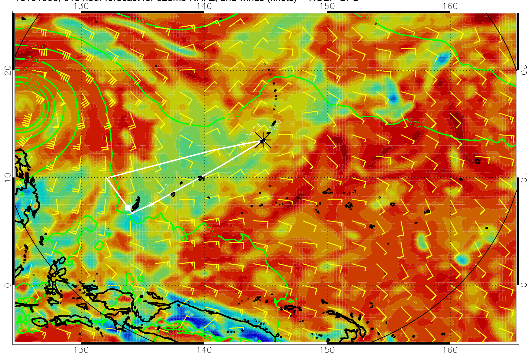
16101906, 018 hour forecast for 925mb RH, Z, and winds (knots) -- NCEP GFS
