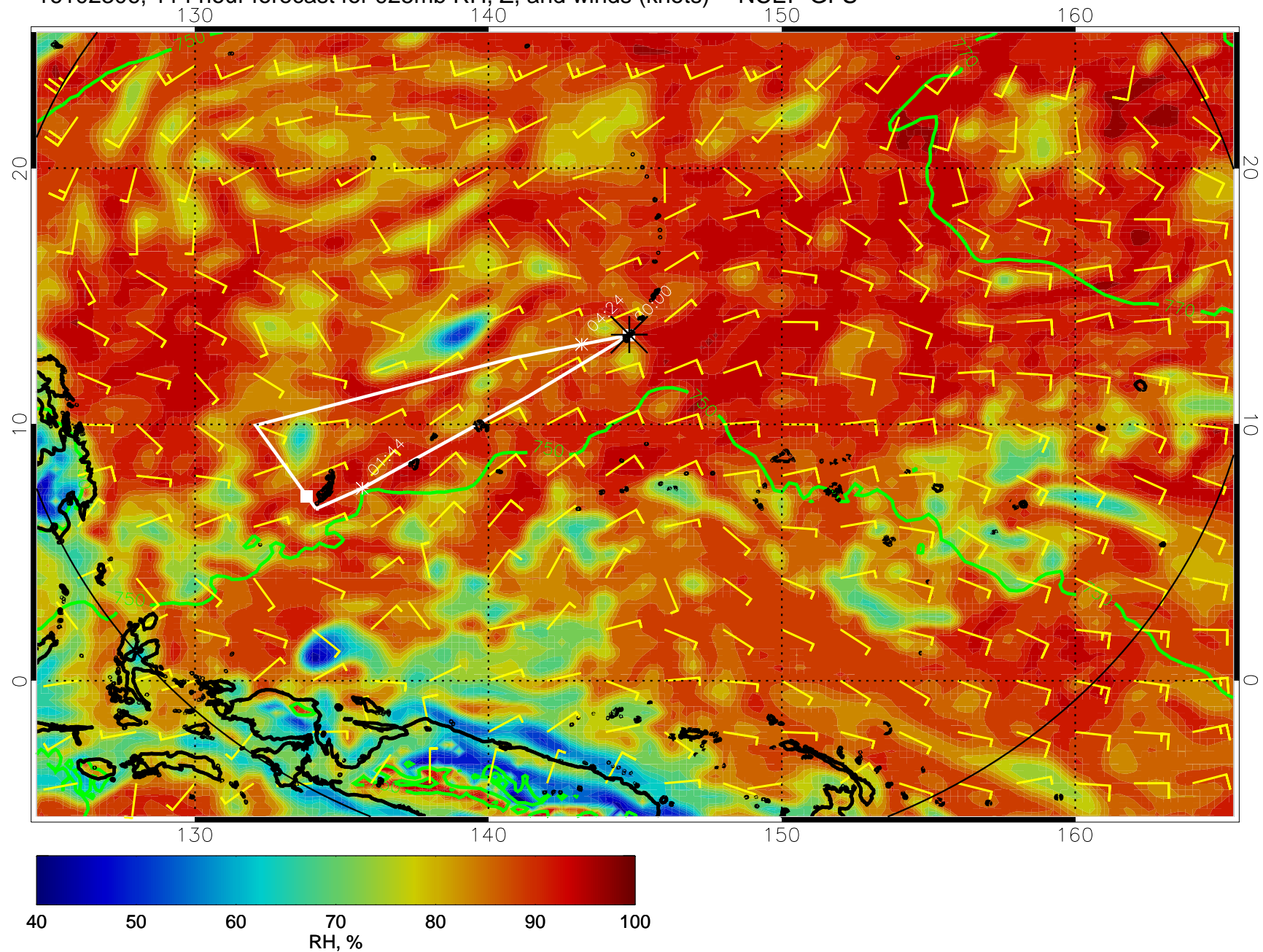
16102306, 114 hour forecast for 925mb RH, Z, and winds (knots) -- NCEP GFS
