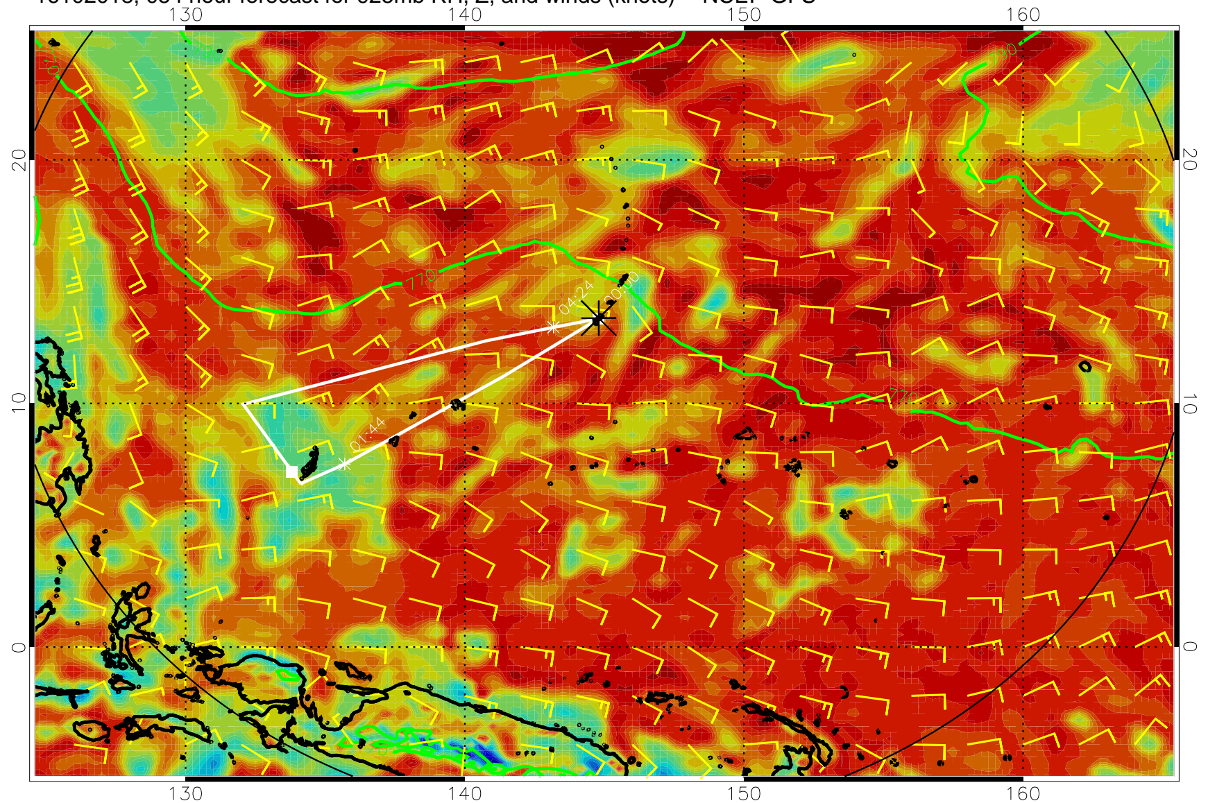
16102018, 054 hour forecast for 925mb RH, Z, and winds (knots) -- NCEP GFS
