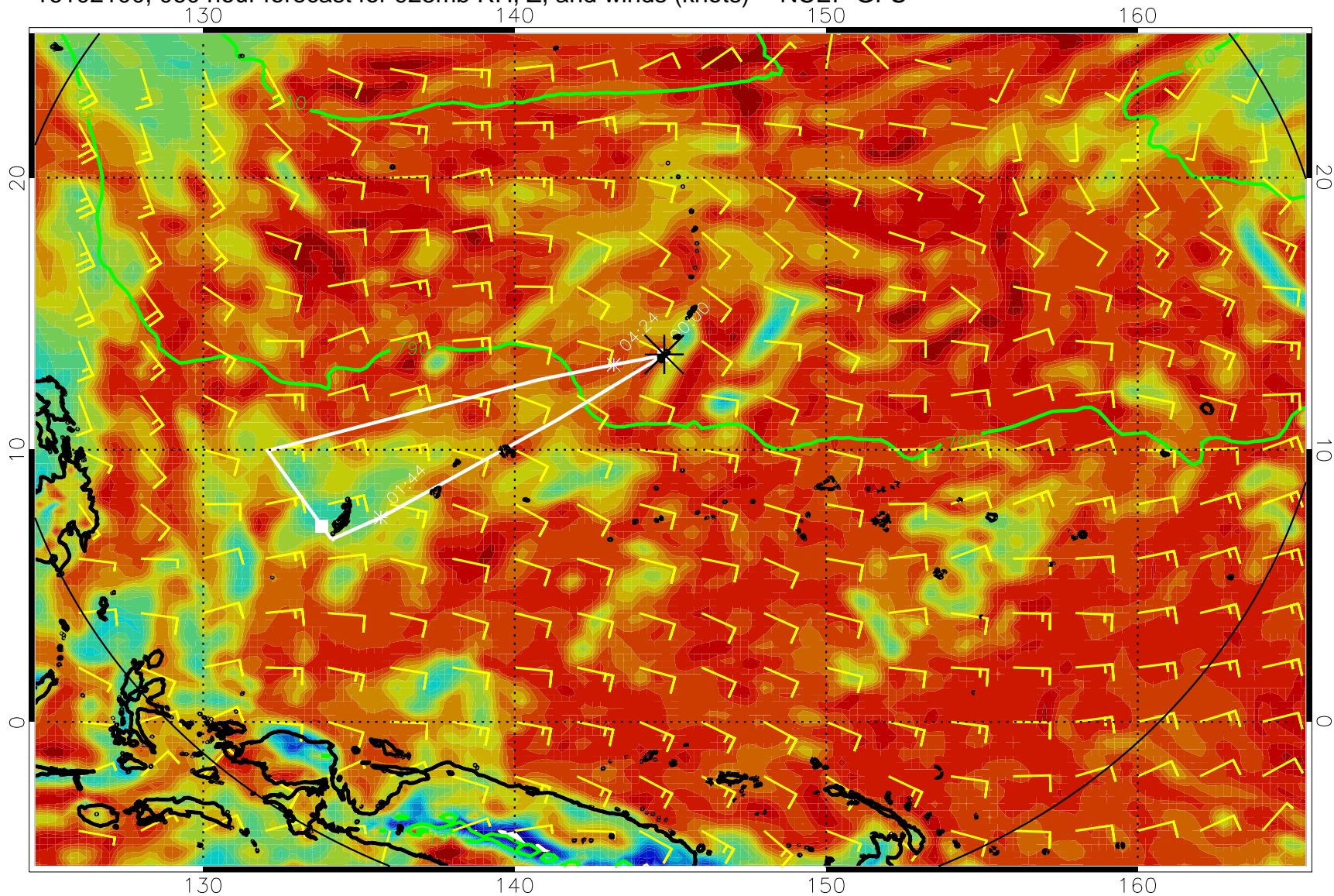
16102100, 060 hour forecast for 925mb RH, Z, and winds (knots) -- NCEP GFS
