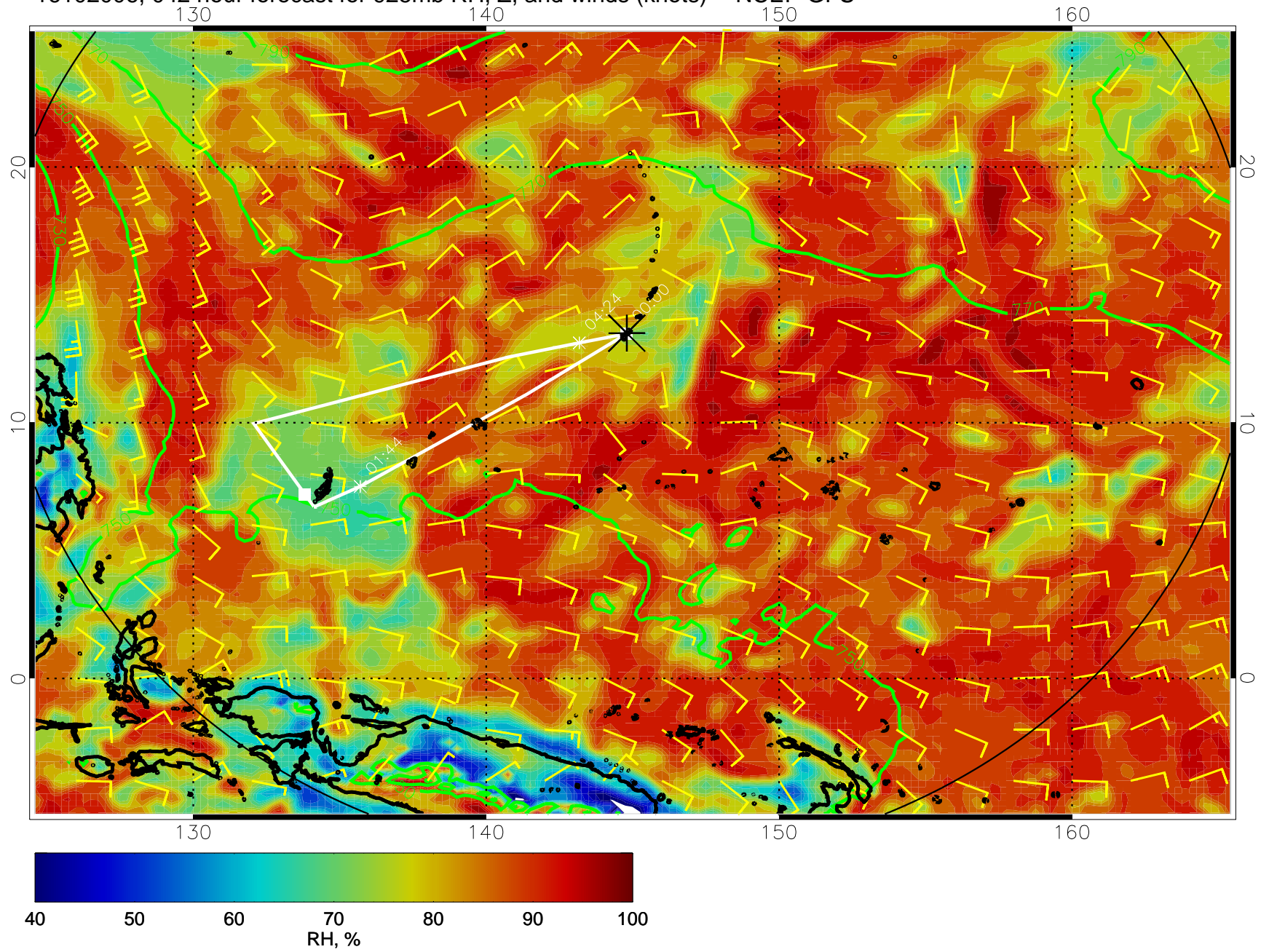
16102006, 042 hour forecast for 925mb RH, Z, and winds (knots) -- NCEP GFS
