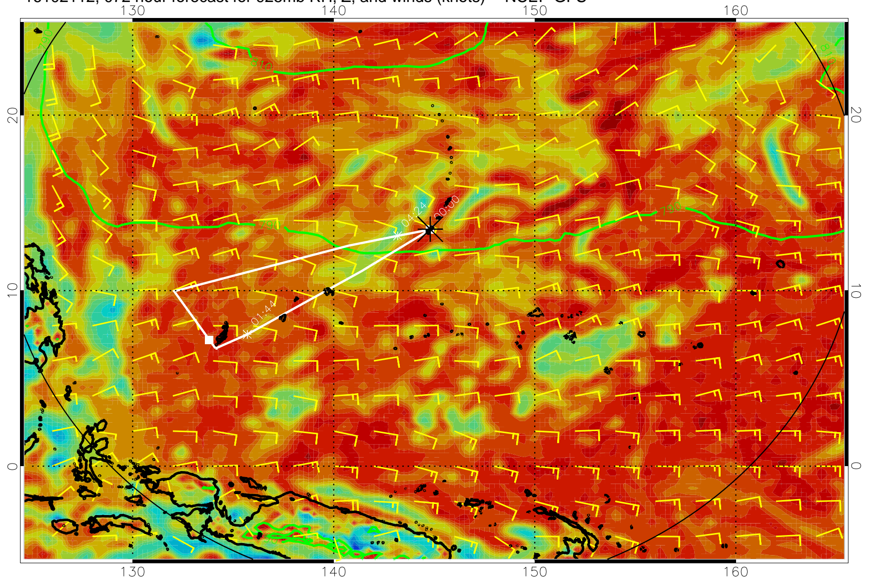
16102112, 072 hour forecast for 925mb RH, Z, and winds (knots) -- NCEP GFS
