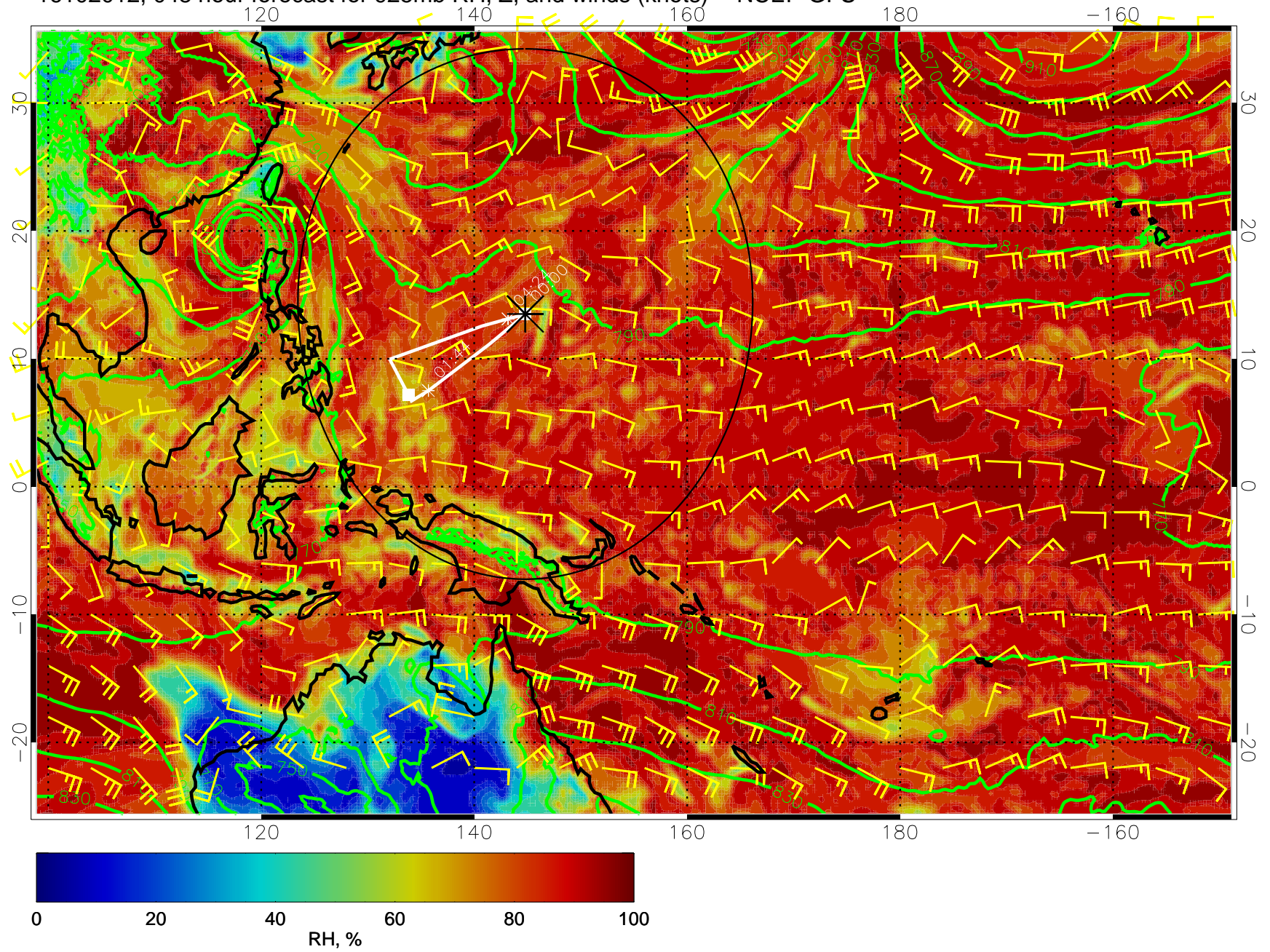
16102012, 048 hour forecast for 925mb RH, Z, and winds (knots) -- NCEP GFS
