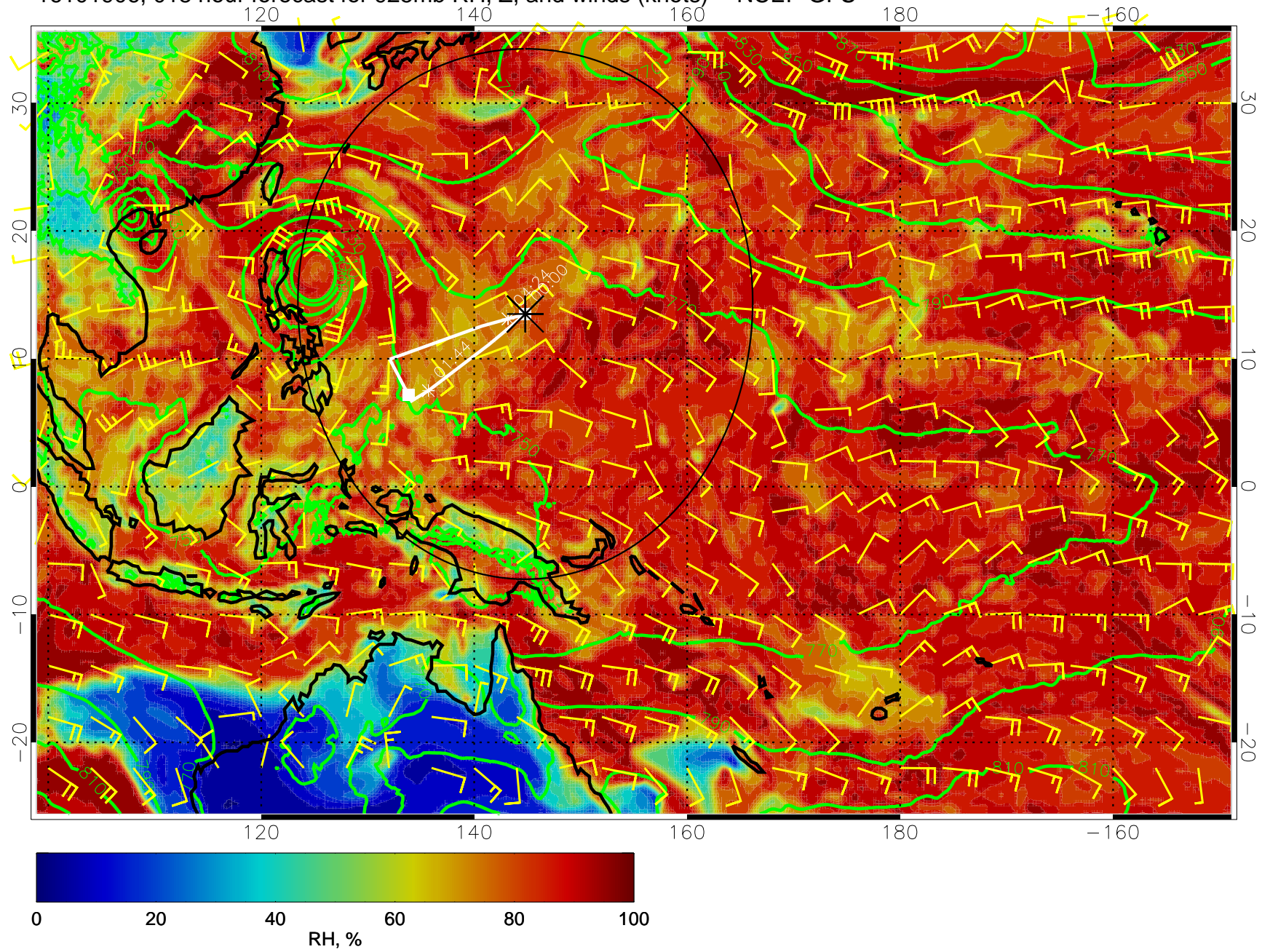
16101906, 018 hour forecast for 925mb RH, Z, and winds (knots) -- NCEP GFS
