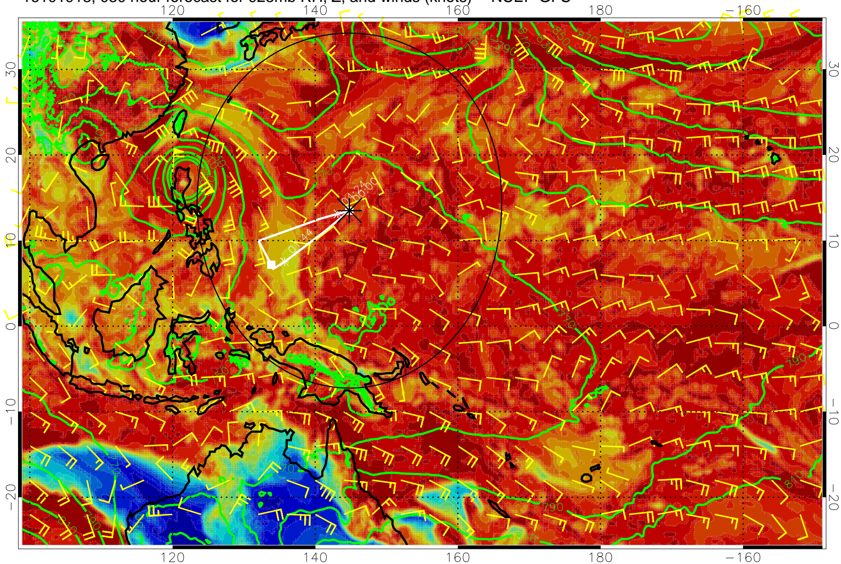
16101918, 030 hour forecast for 925mb RH, Z, and winds (knots) -- NCEP GFS
