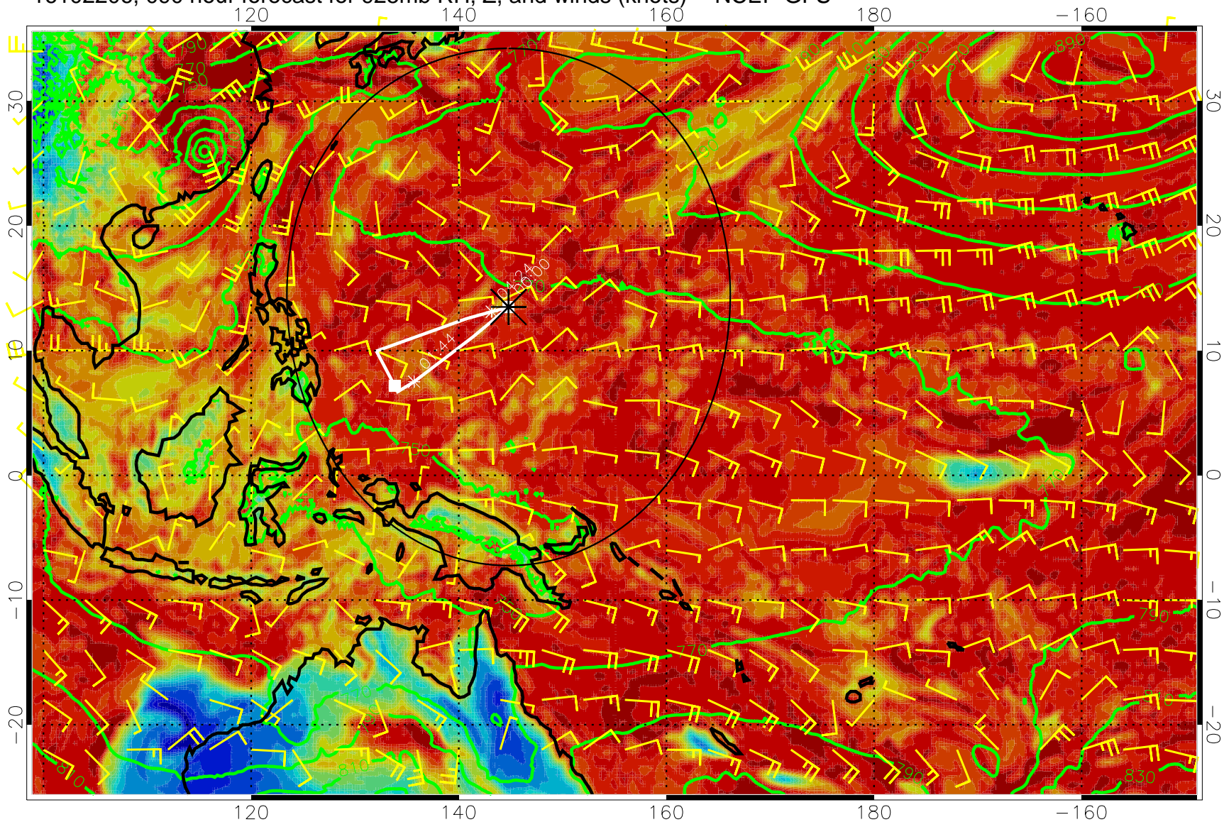
16102206, 090 hour forecast for 925mb RH, Z, and winds (knots) -- NCEP GFS
