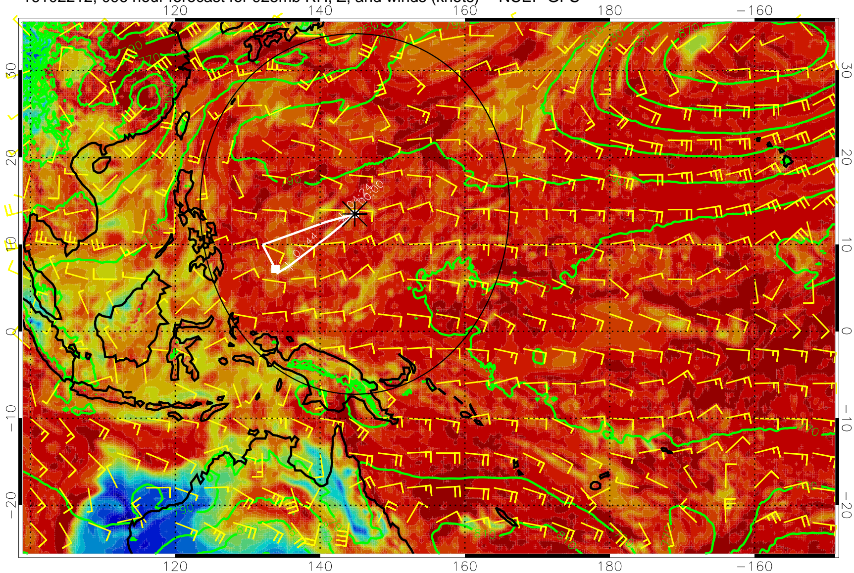
16102212, 096 hour forecast for 925mb RH, Z, and winds (knots) -- NCEP GFS
