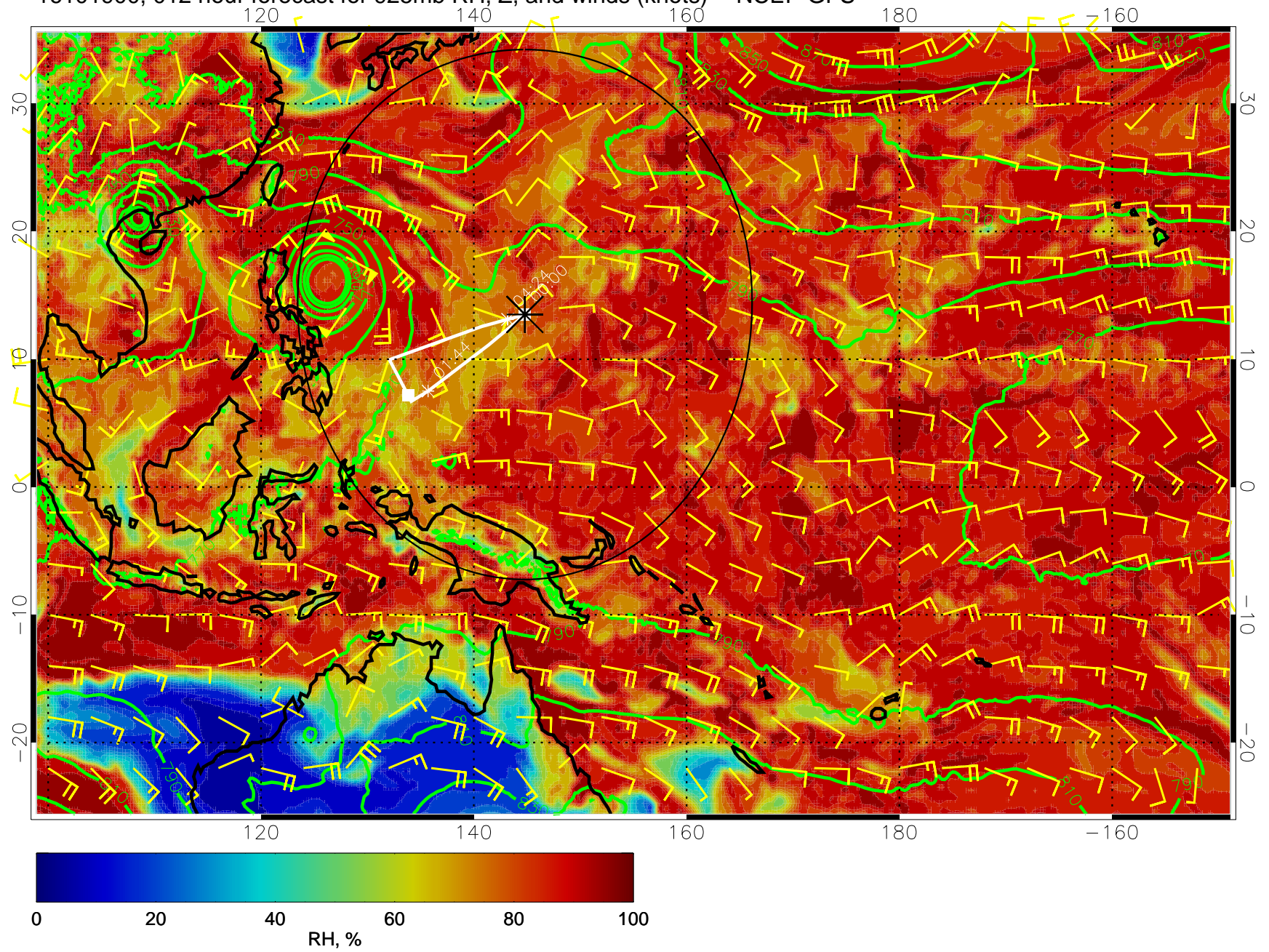
16101900, 012 hour forecast for 925mb RH, Z, and winds (knots) -- NCEP GFS
