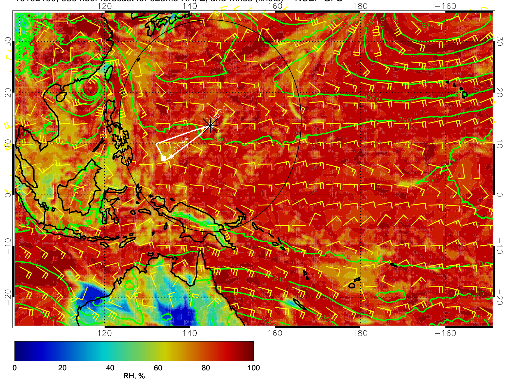
16102100, 060 hour forecast for 925mb RH, Z, and winds (knots) -- NCEP GFS
