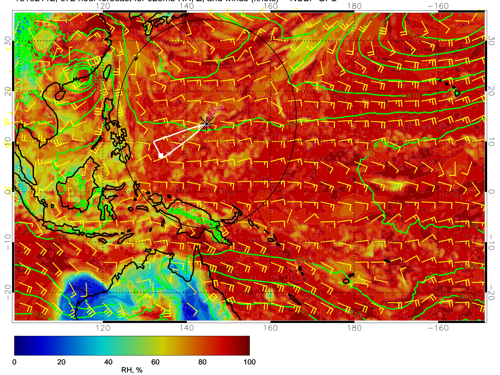
16102112, 072 hour forecast for 925mb RH, Z, and winds (knots) -- NCEP GFS
