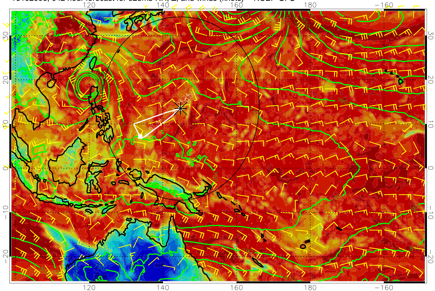
16102006, 042 hour forecast for 925mb RH, Z, and winds (knots) -- NCEP GFS
