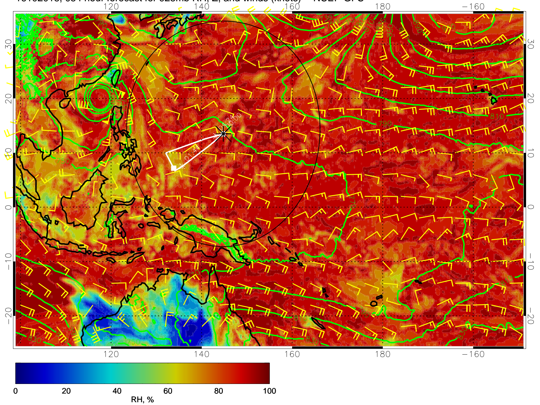
16102018, 054 hour forecast for 925mb RH, Z, and winds (knots) -- NCEP GFS
