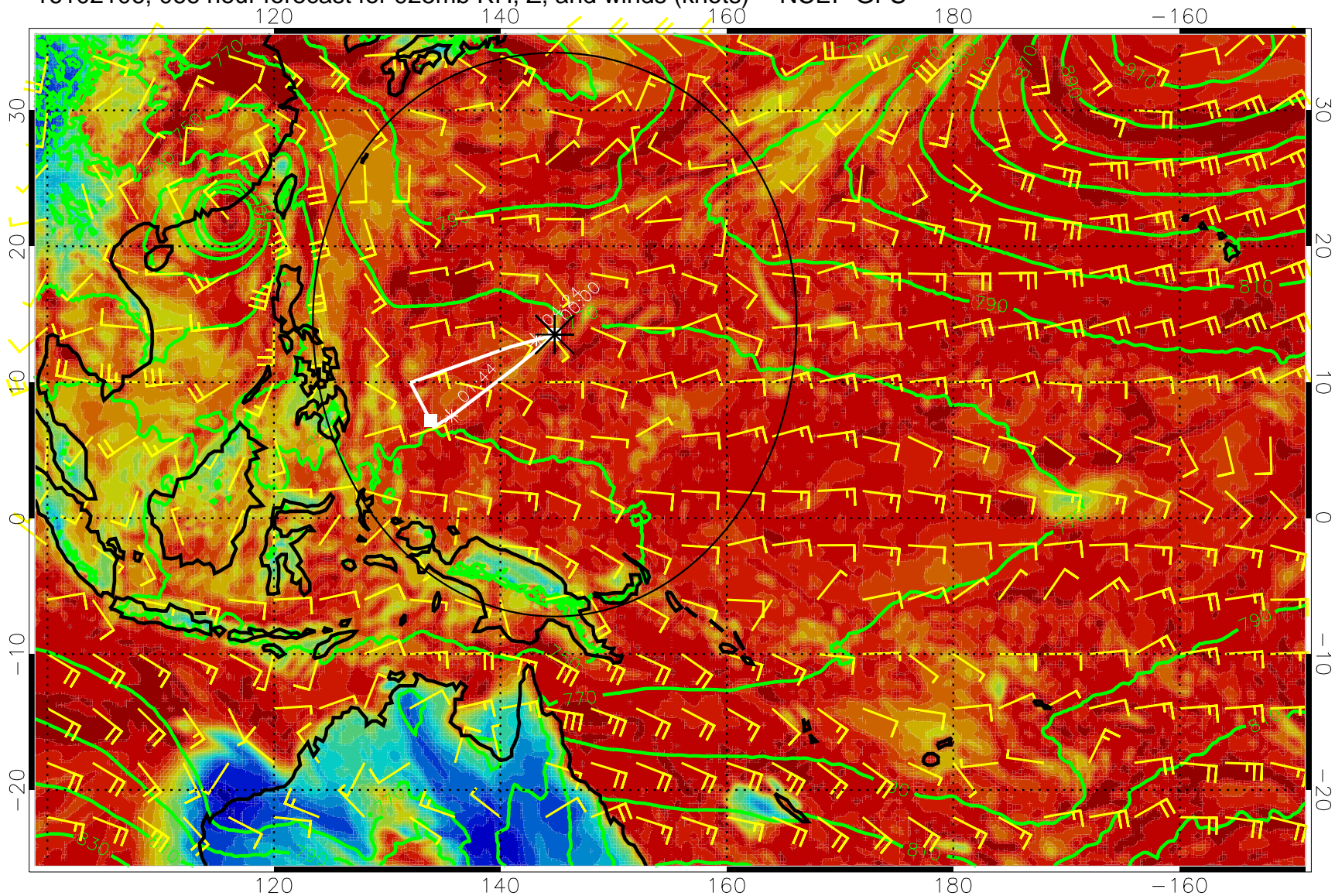
16102106, 066 hour forecast for 925mb RH, Z, and winds (knots) -- NCEP GFS
