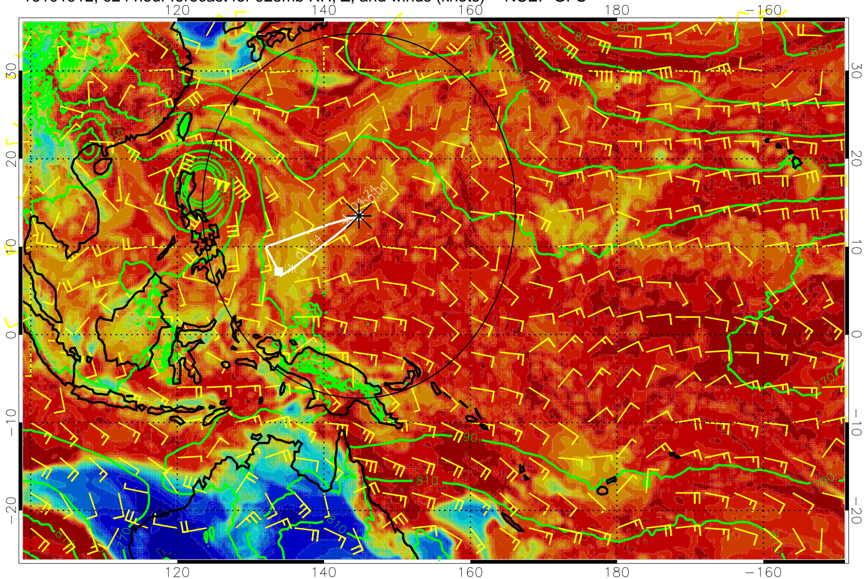
16101912, 024 hour forecast for 925mb RH, Z, and winds (knots) -- NCEP GFS
