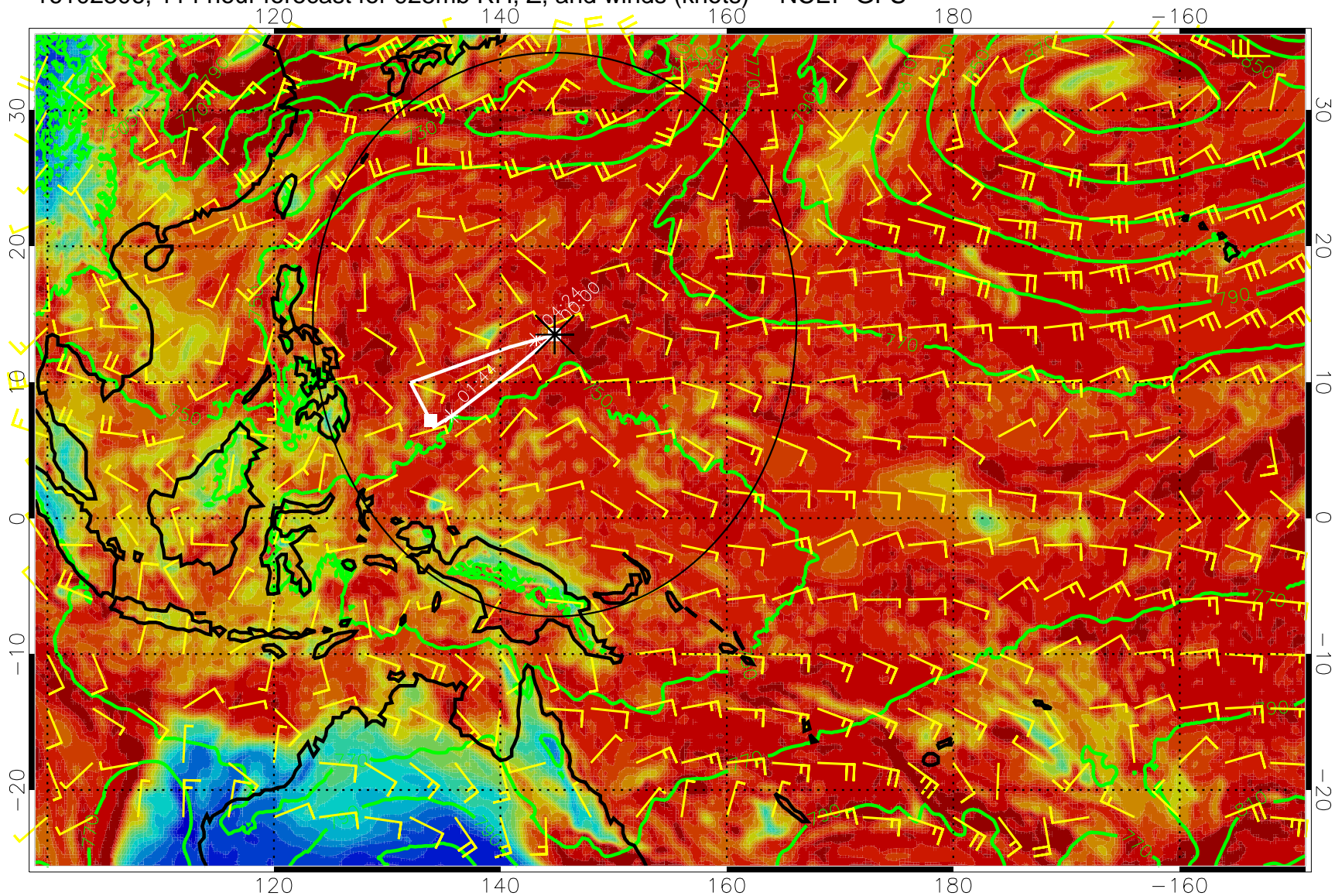
16102306, 114 hour forecast for 925mb RH, Z, and winds (knots) -- NCEP GFS
