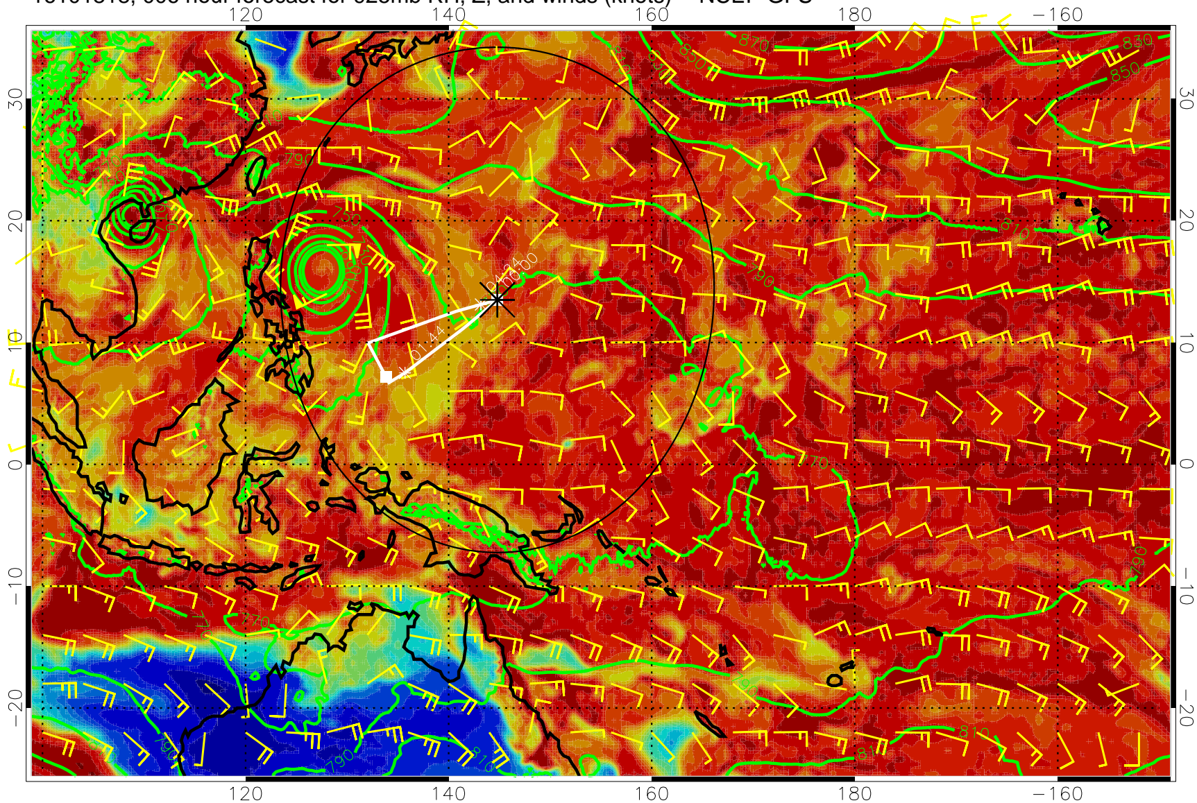
16101818, 006 hour forecast for 925mb RH, Z, and winds (knots) -- NCEP GFS
