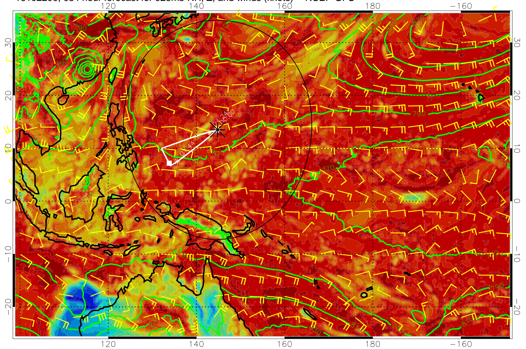
16102200, 084 hour forecast for 925mb RH, Z, and winds (knots) -- NCEP GFS
