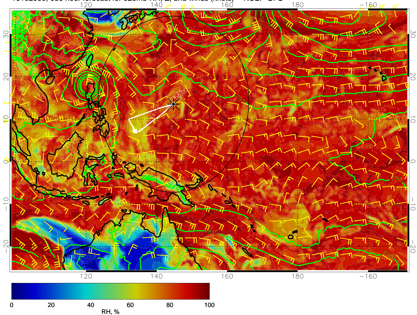
16102000, 036 hour forecast for 925mb RH, Z, and winds (knots) -- NCEP GFS
