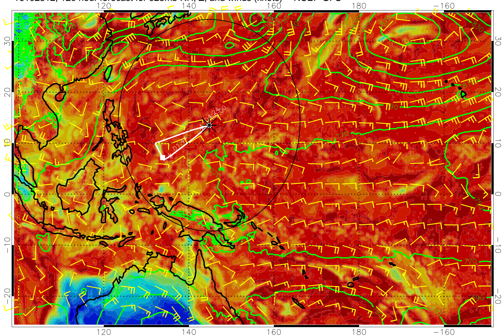
16102312, 120 hour forecast for 925mb RH, Z, and winds (knots) -- NCEP GFS
