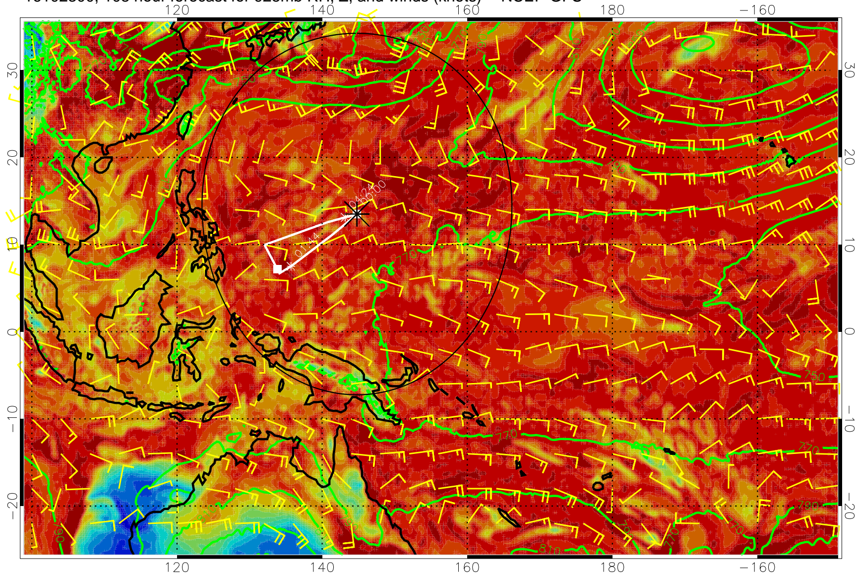
16102300, 108 hour forecast for 925mb RH, Z, and winds (knots) -- NCEP GFS
