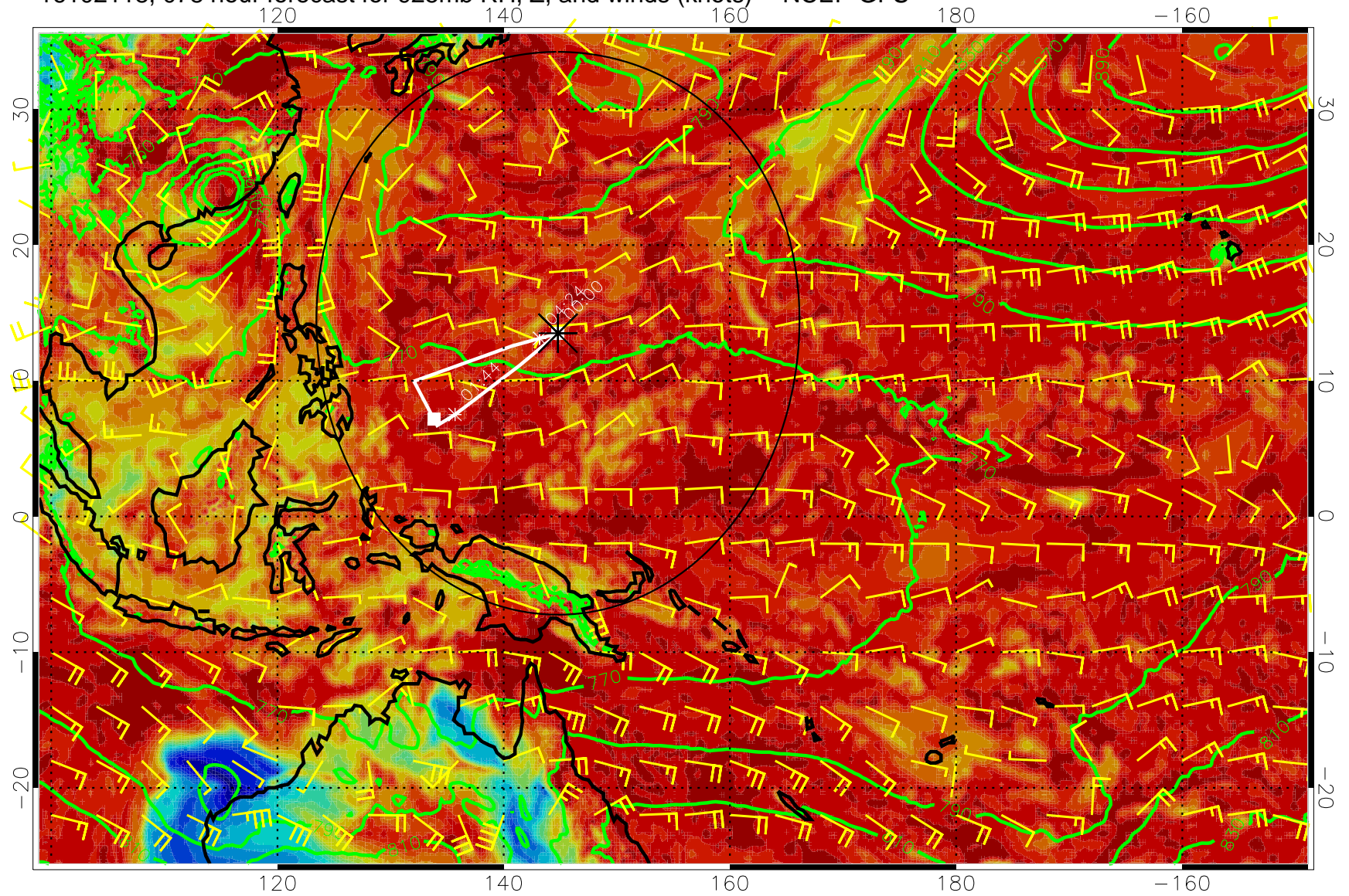
16102118, 078 hour forecast for 925mb RH, Z, and winds (knots) -- NCEP GFS
