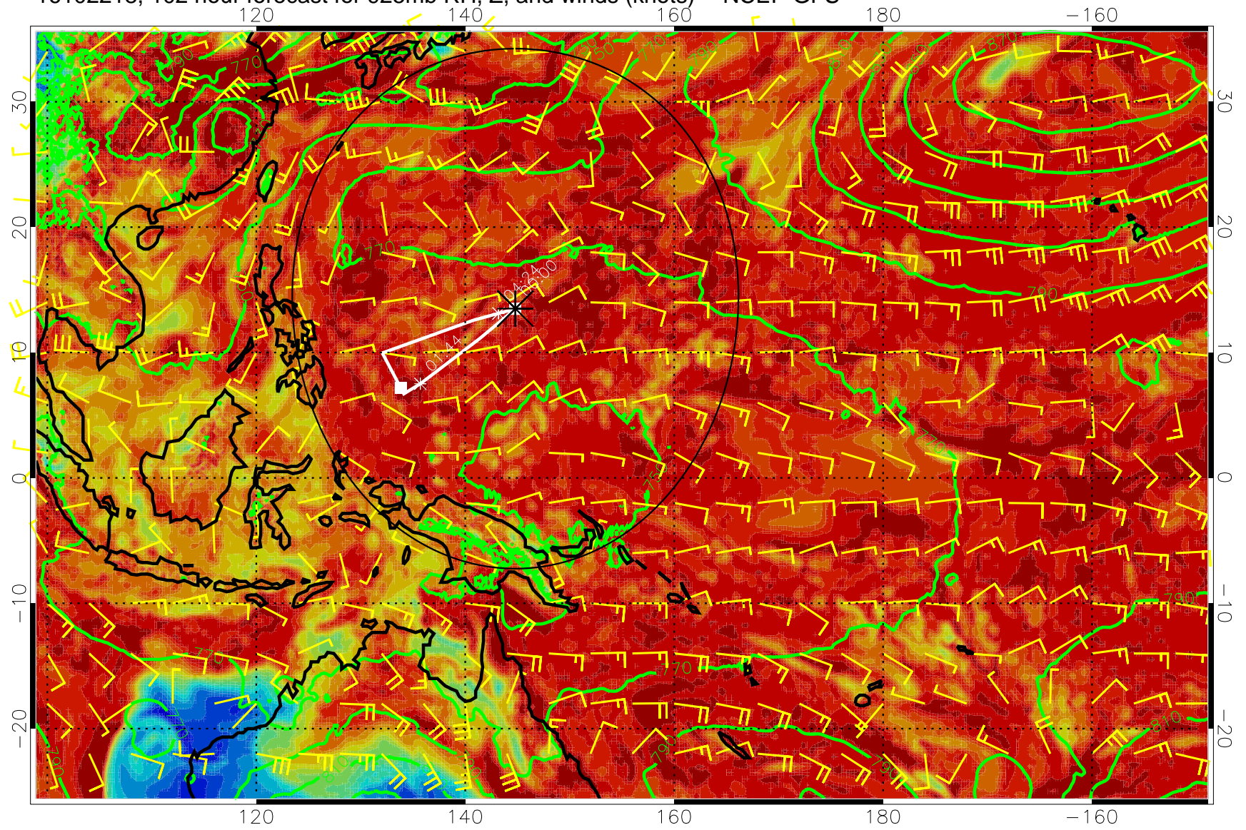
16102218, 102 hour forecast for 925mb RH, Z, and winds (knots) -- NCEP GFS
