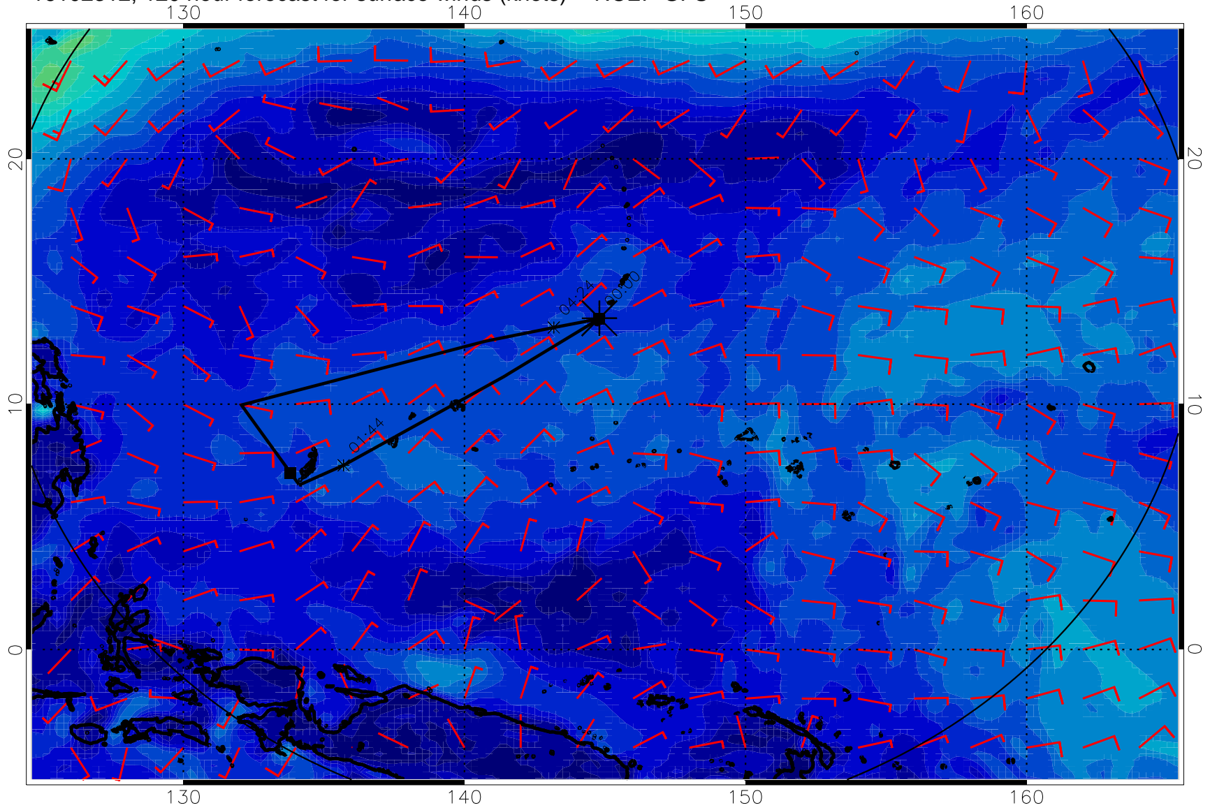
16102312, 120 hour forecast for surface winds (knots) -- NCEP GFS
