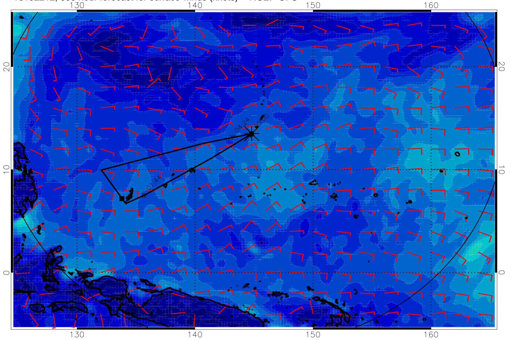
16102212, 096 hour forecast for surface winds (knots) -- NCEP GFS
