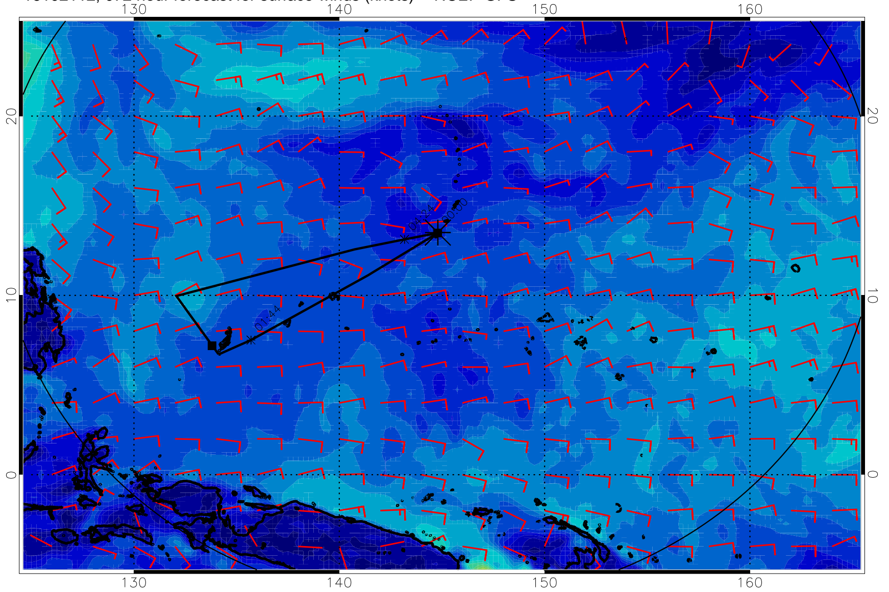
16102112, 072 hour forecast for surface winds (knots) -- NCEP GFS
