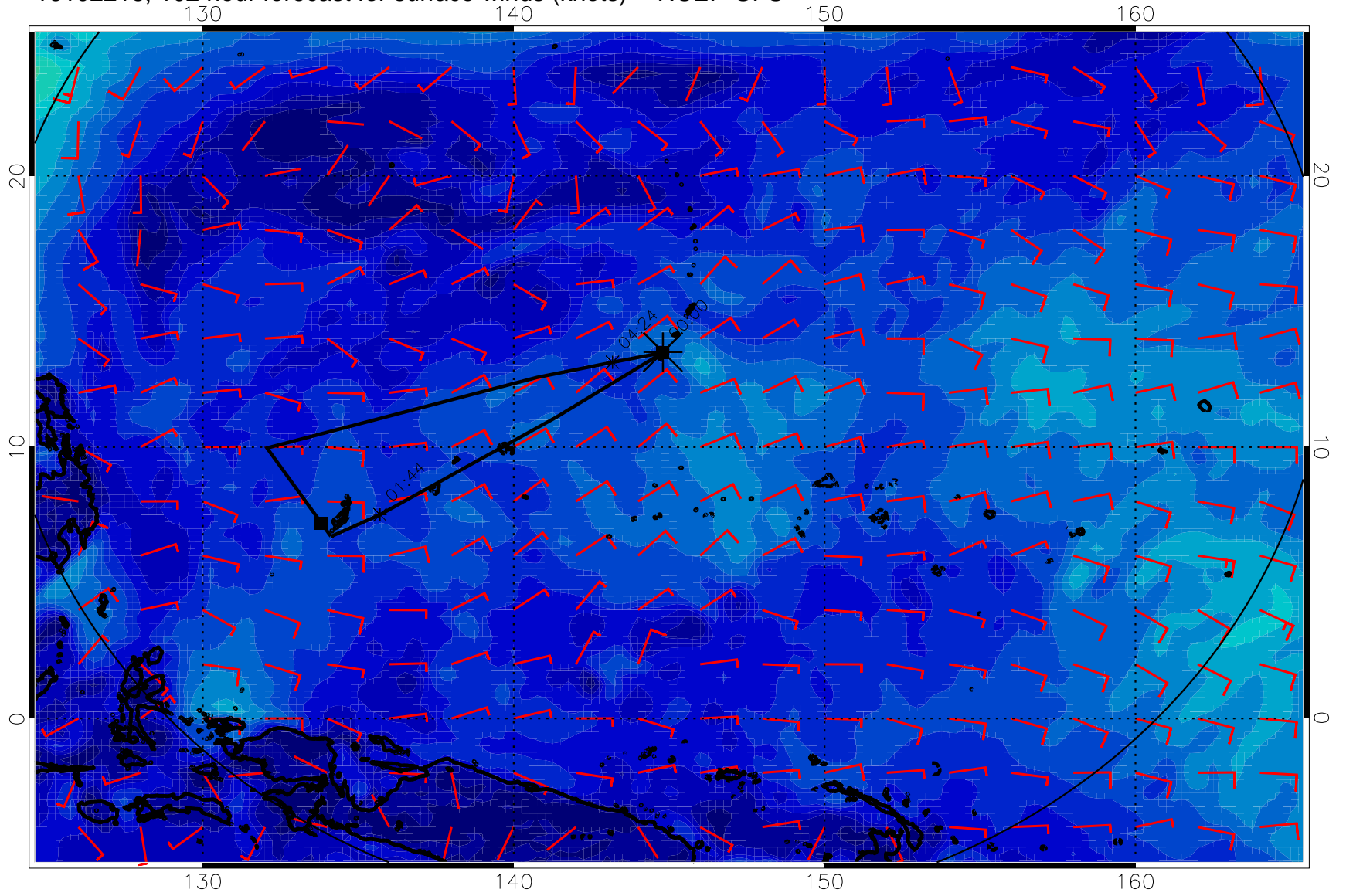
16102218, 102 hour forecast for surface winds (knots) -- NCEP GFS
