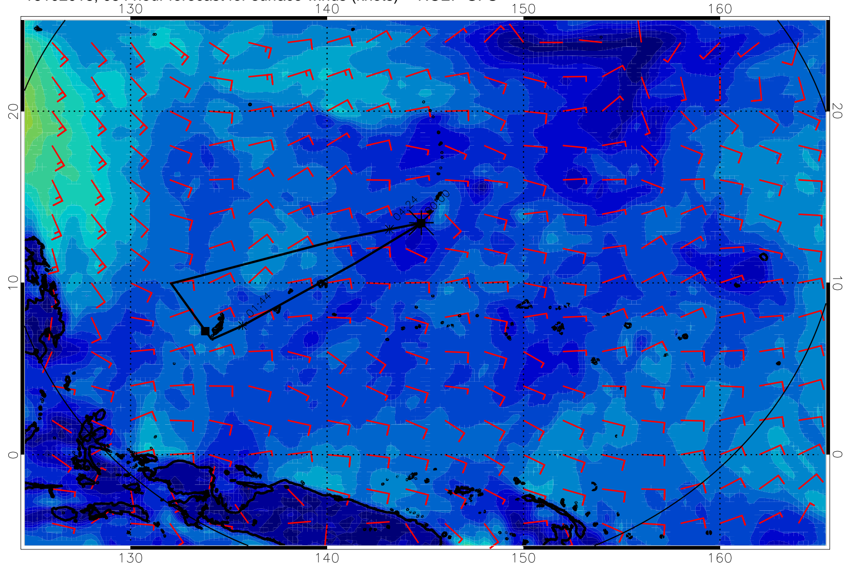
16102018, 054 hour forecast for surface winds (knots) -- NCEP GFS
