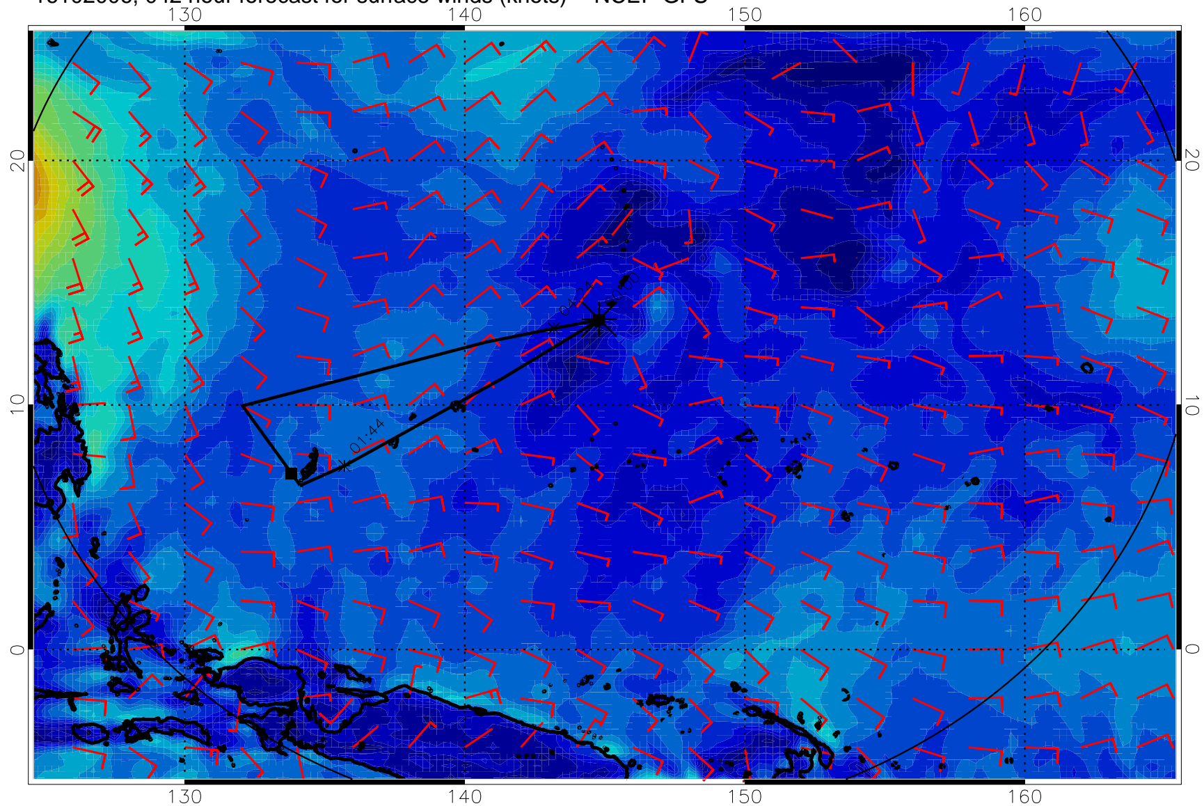
16102006, 042 hour forecast for surface winds (knots) -- NCEP GFS
