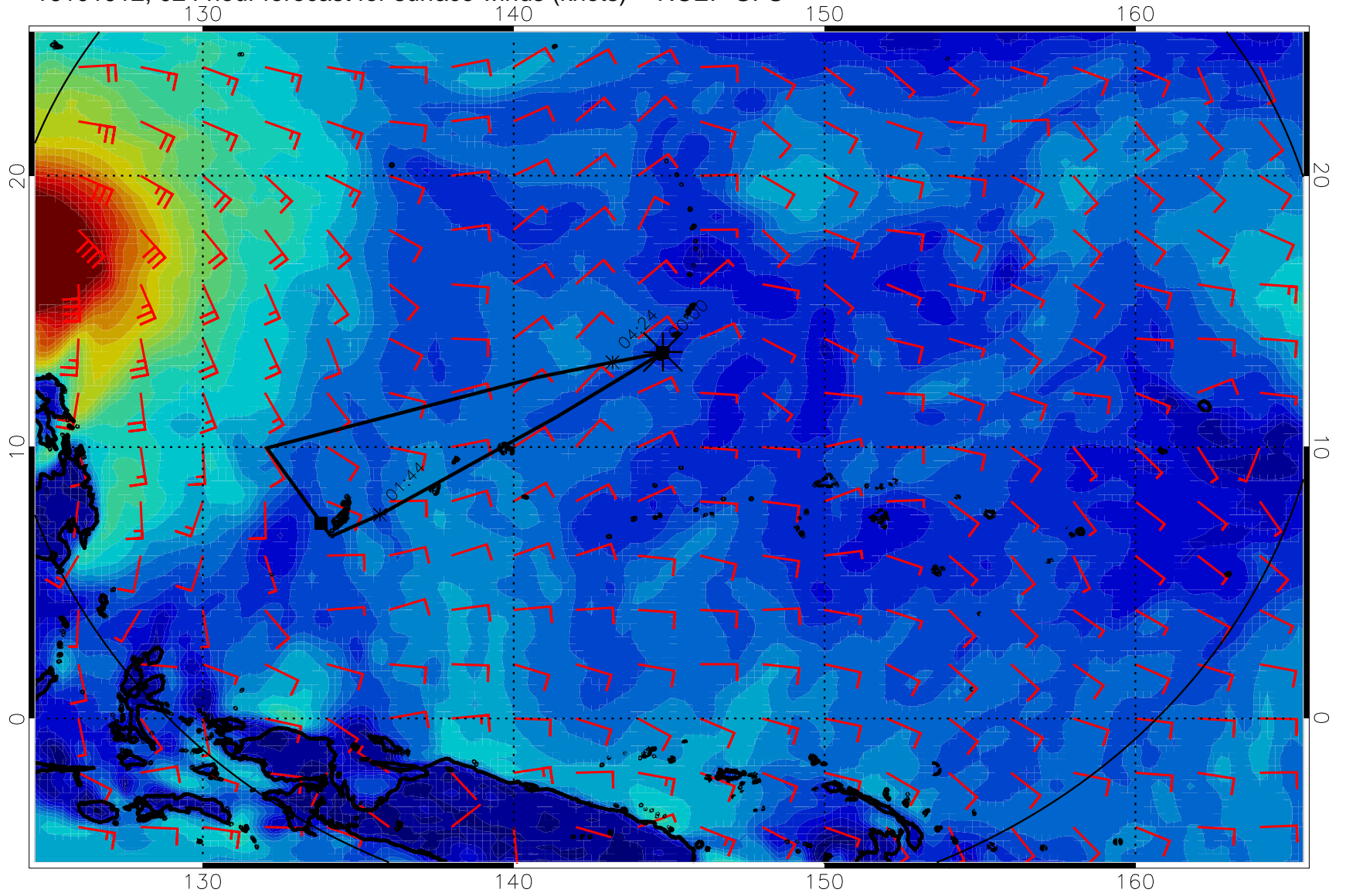
16101912, 024 hour forecast for surface winds (knots) -- NCEP GFS
