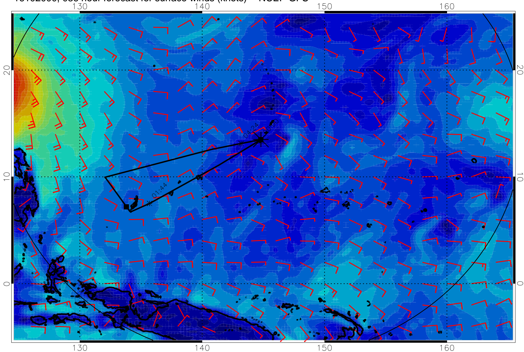
16102000, 036 hour forecast for surface winds (knots) -- NCEP GFS
