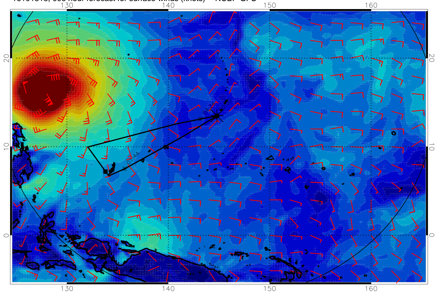
16101818, 006 hour forecast for surface winds (knots) -- NCEP GFS
