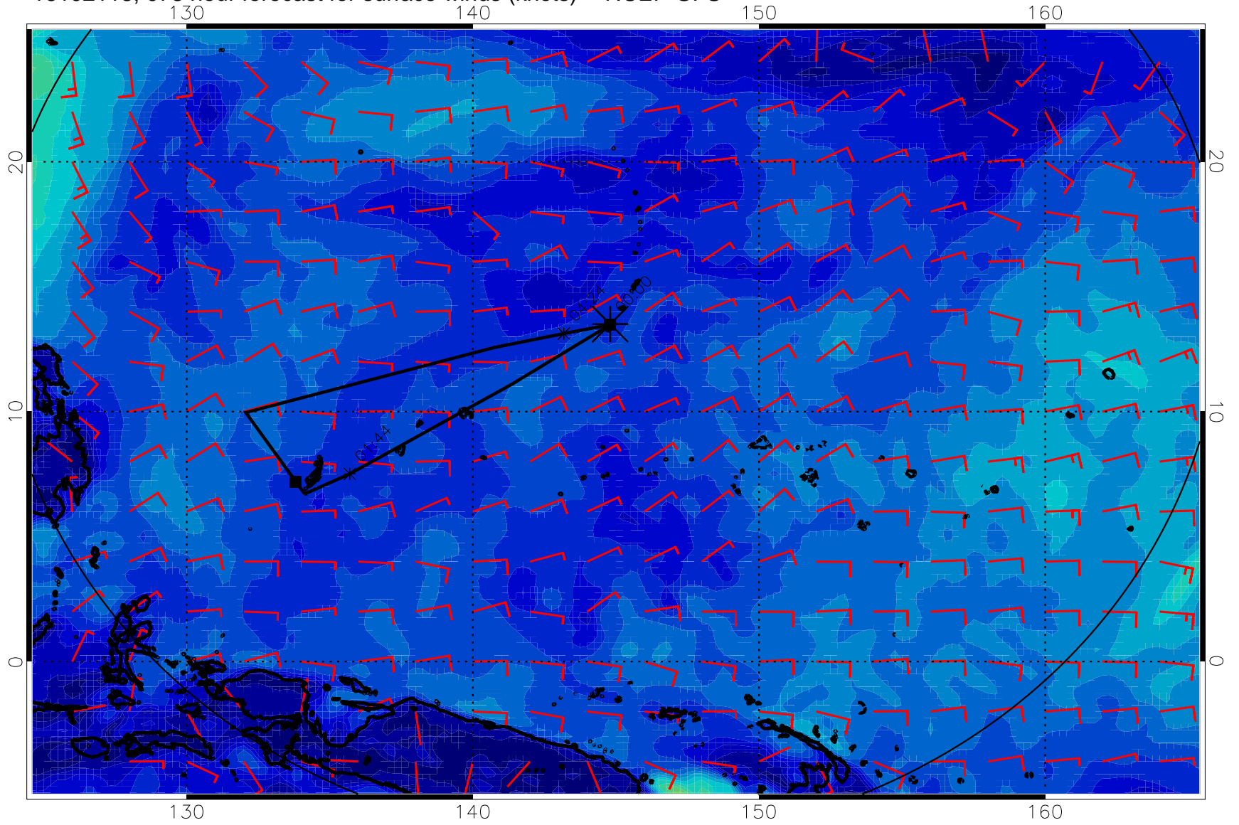
16102118, 078 hour forecast for surface winds (knots) -- NCEP GFS
