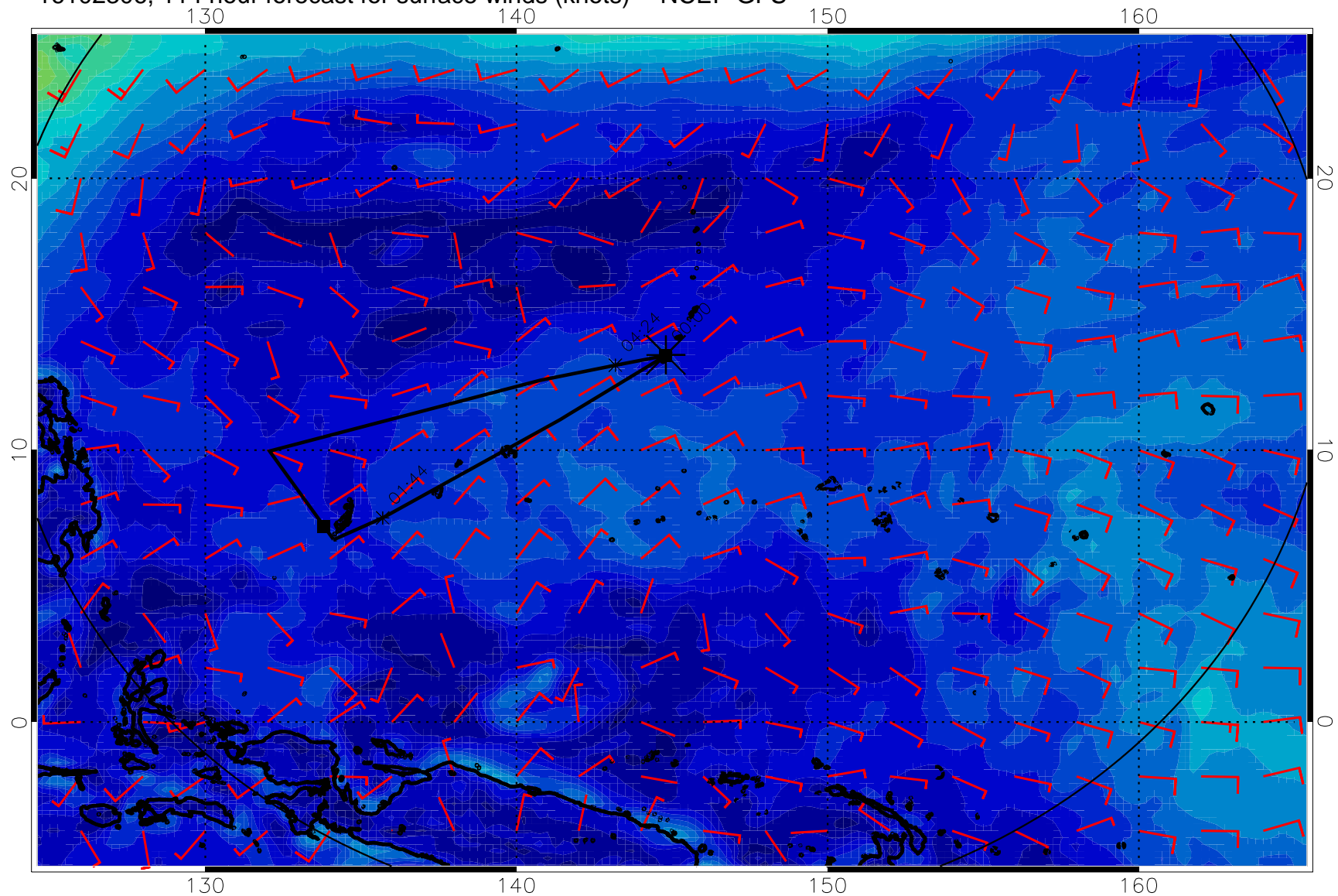
16102306, 114 hour forecast for surface winds (knots) -- NCEP GFS
