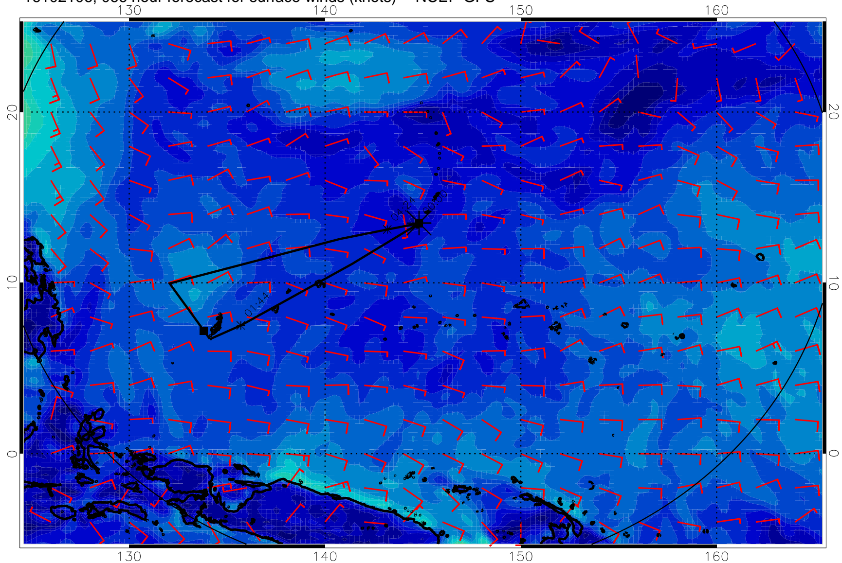
16102106, 066 hour forecast for surface winds (knots) -- NCEP GFS
