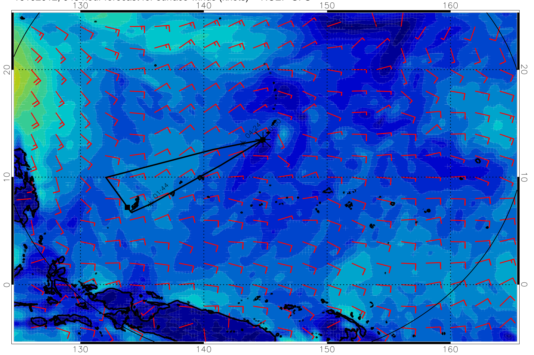
16102012, 048 hour forecast for surface winds (knots) -- NCEP GFS
