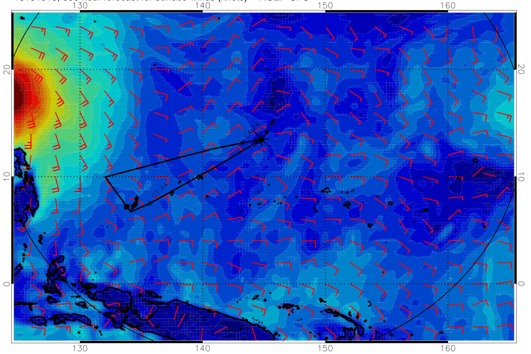
16101918, 030 hour forecast for surface winds (knots) -- NCEP GFS
