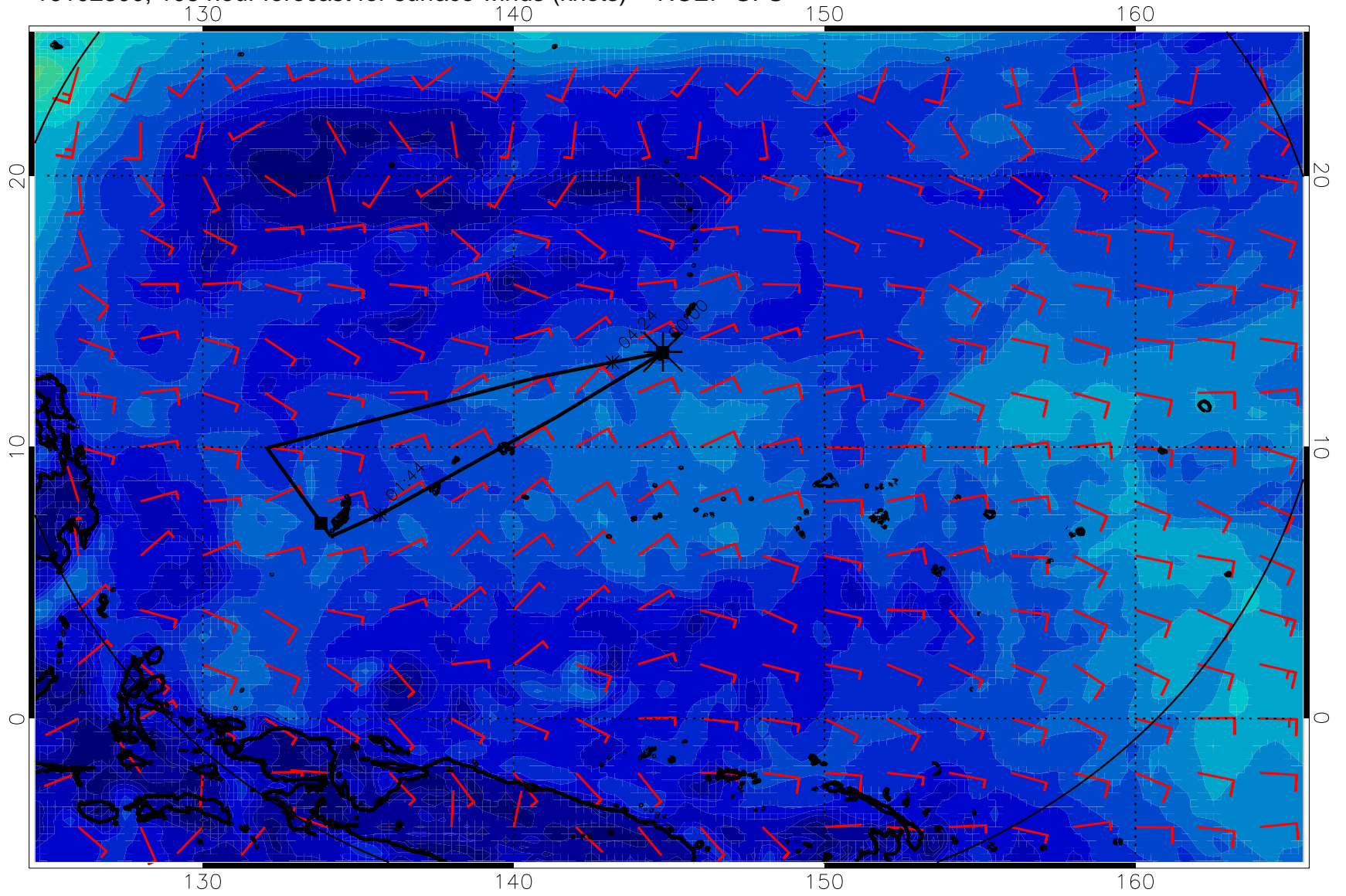
16102300, 108 hour forecast for surface winds (knots) -- NCEP GFS
