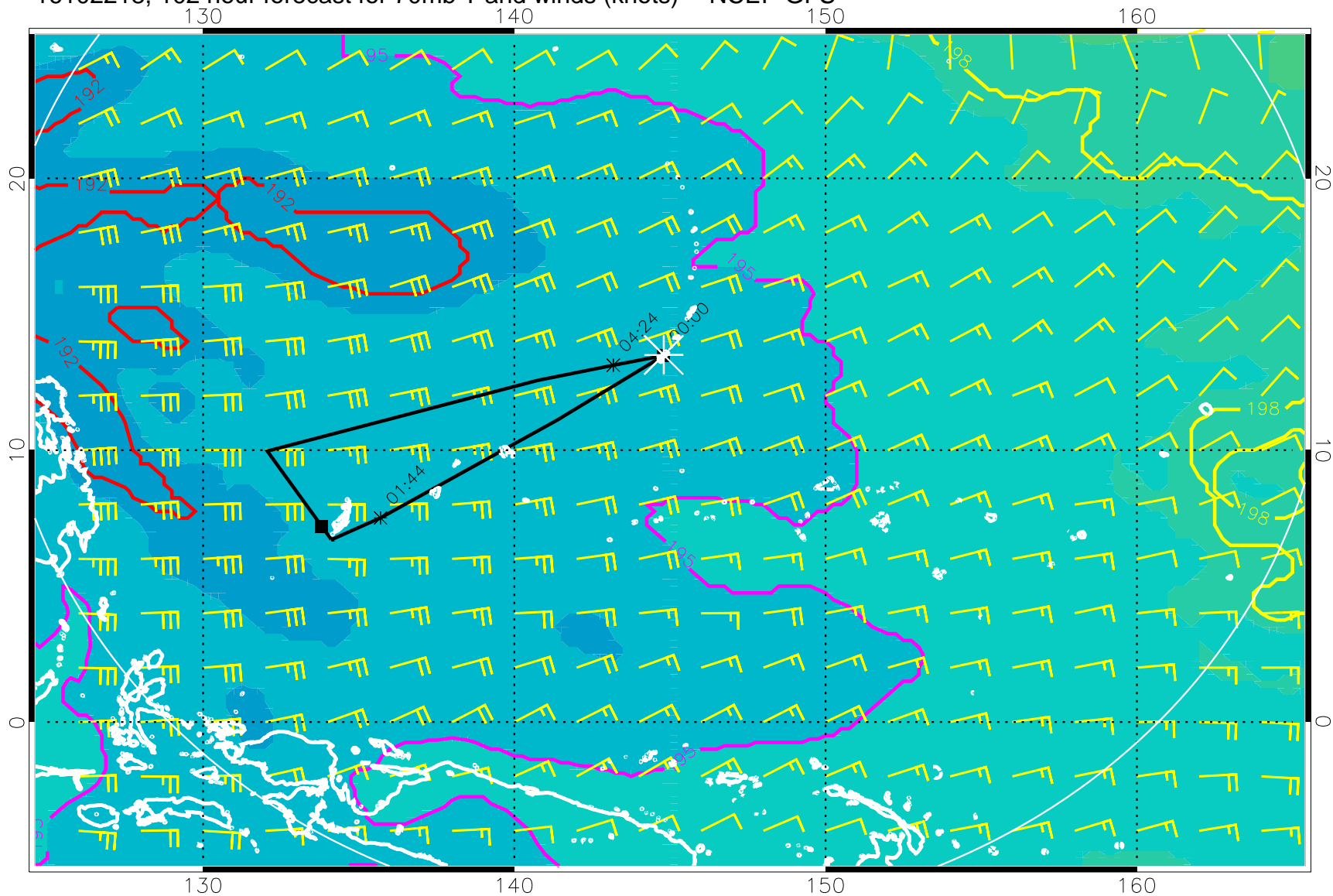
16102218, 102 hour forecast for 70mb T and winds (knots) -- NCEP GFS
