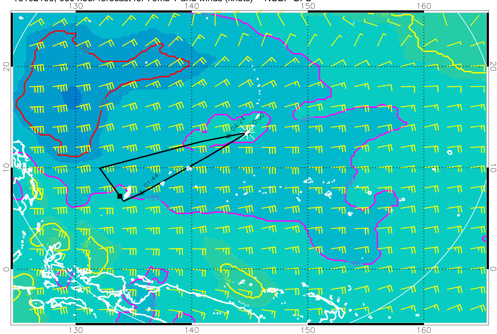
16102100, 060 hour forecast for 70mb T and winds (knots) -- NCEP GFS
