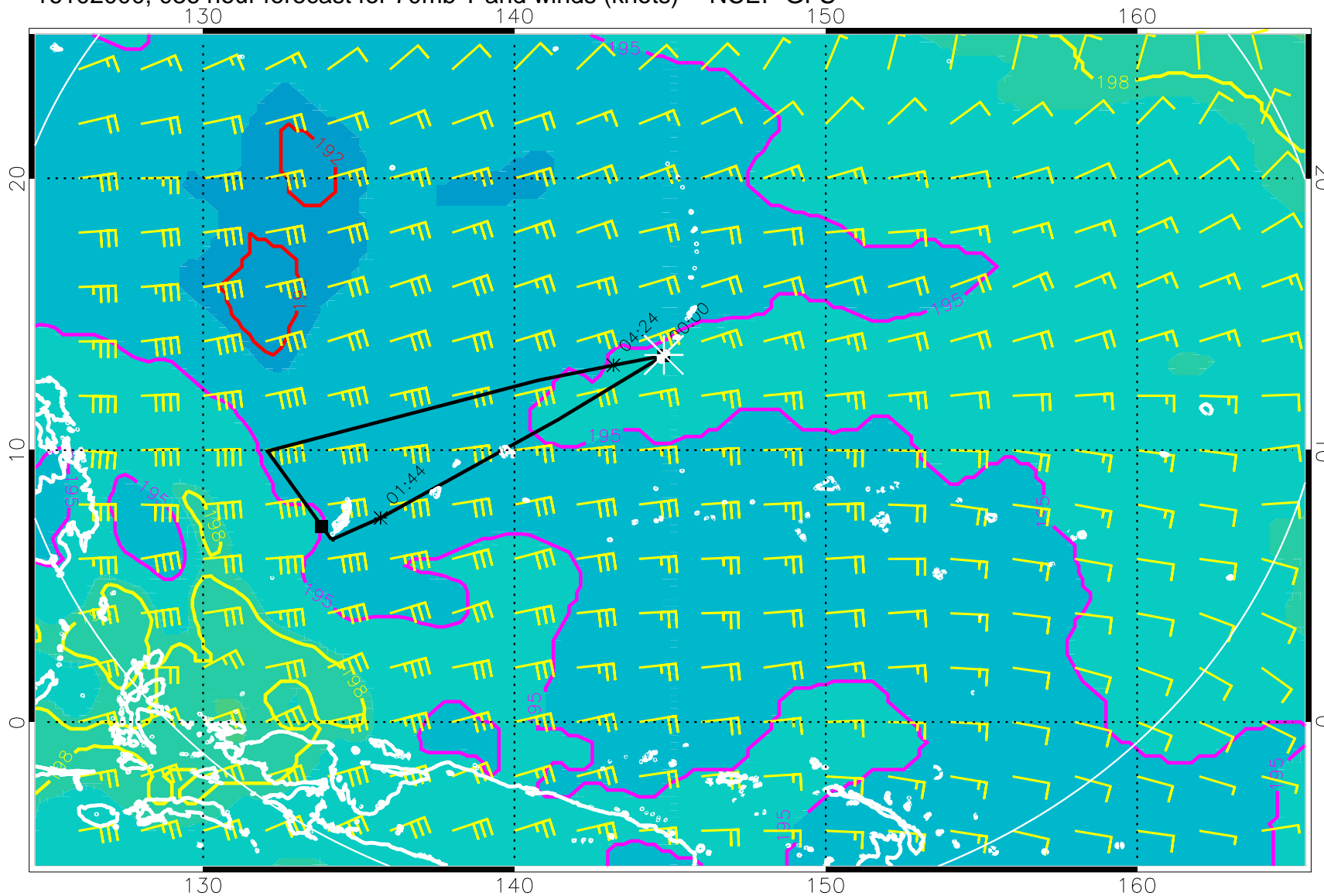
16102000, 036 hour forecast for 70mb T and winds (knots) -- NCEP GFS
