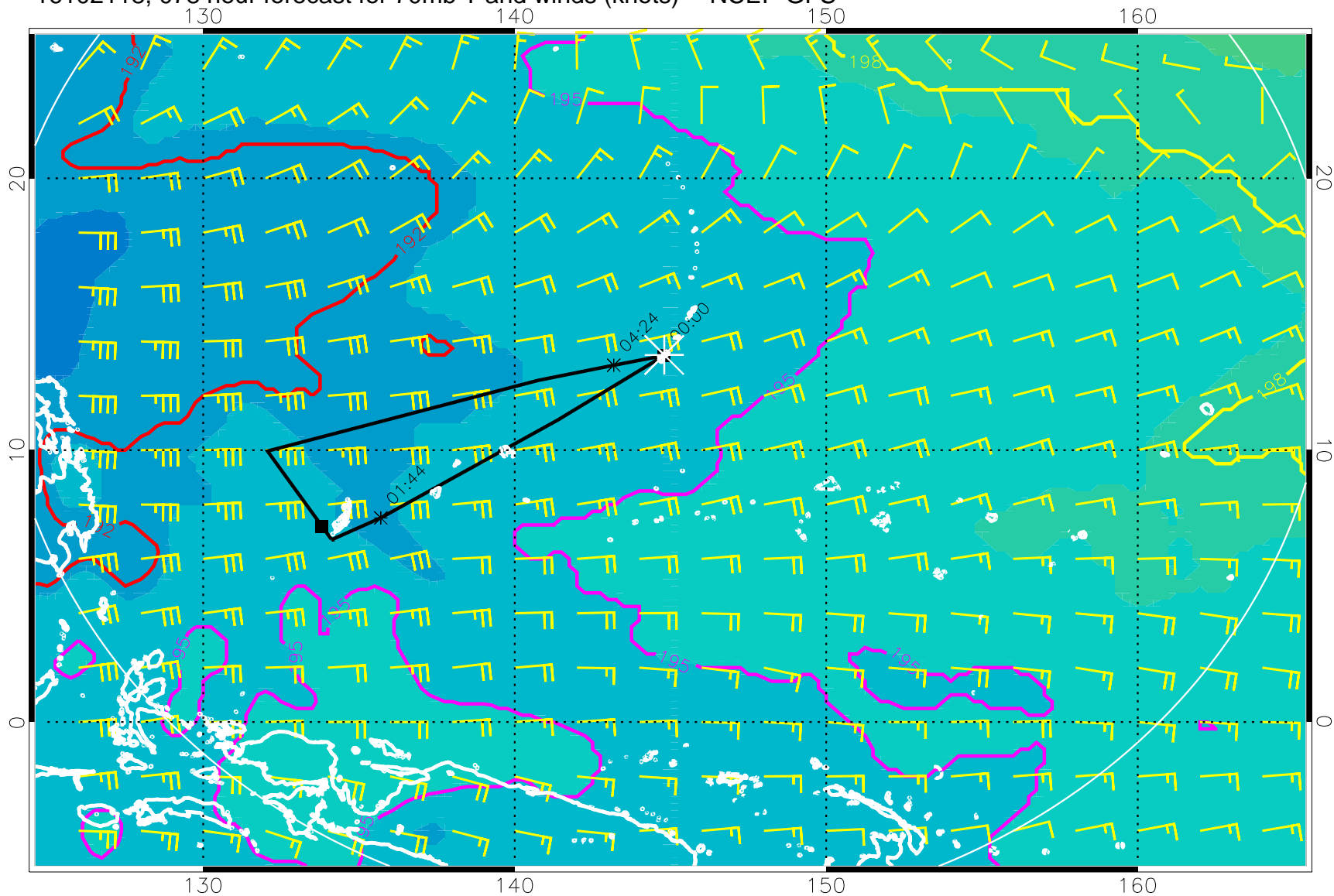
16102118, 078 hour forecast for 70mb T and winds (knots) -- NCEP GFS
