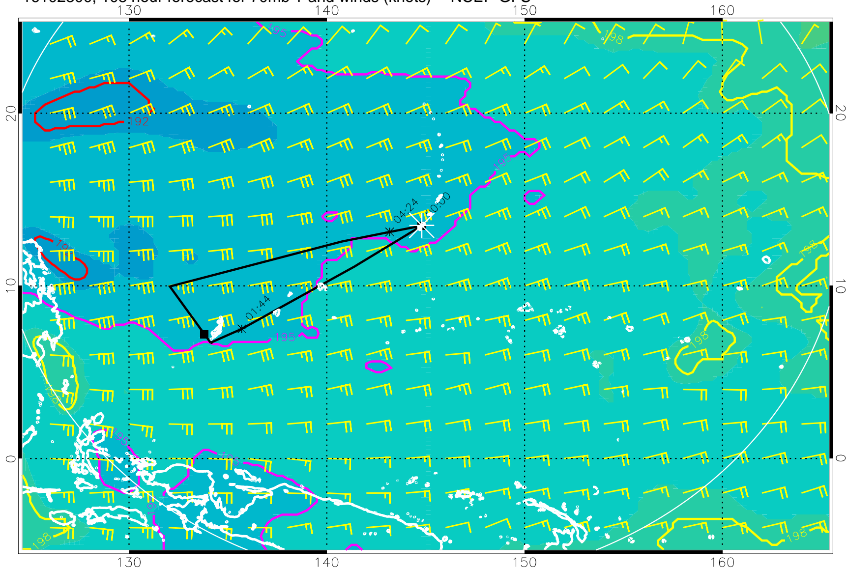
16102300, 108 hour forecast for 70mb T and winds (knots) -- NCEP GFS
