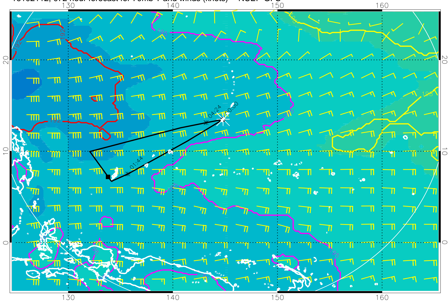
16102112, 072 hour forecast for 70mb T and winds (knots) -- NCEP GFS
