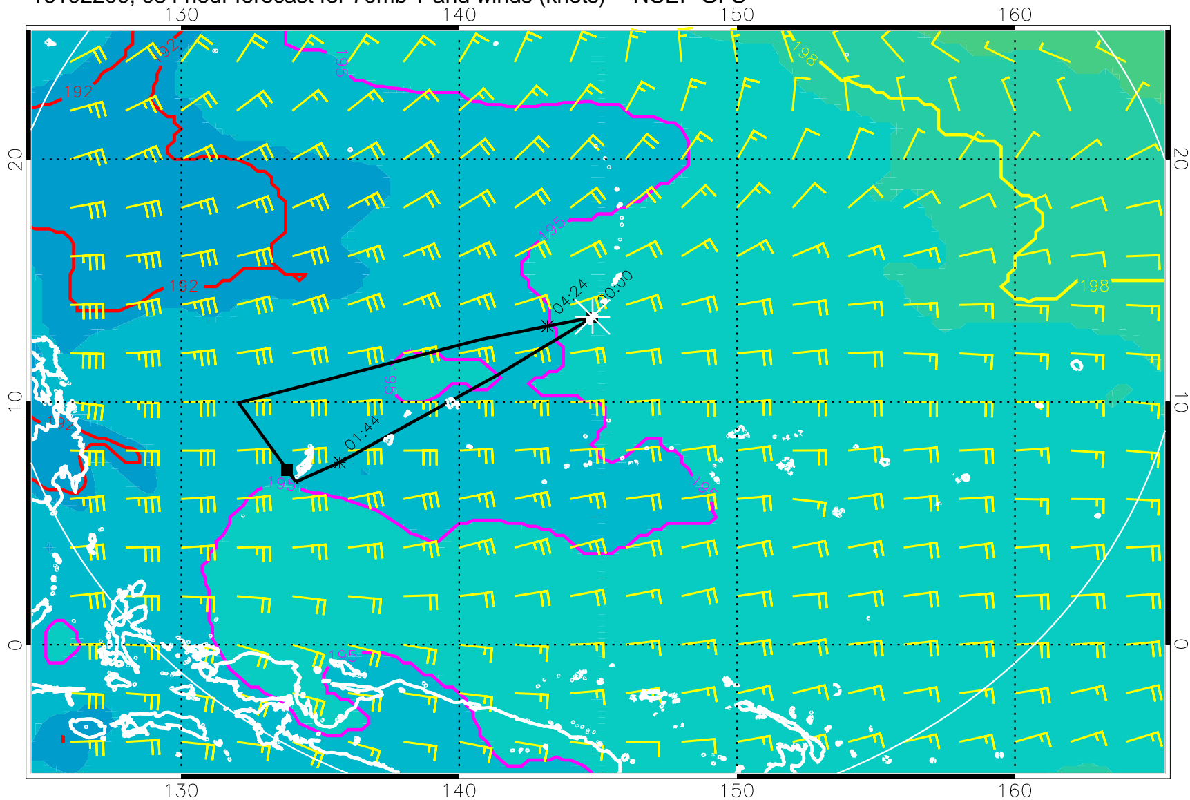
16102200, 084 hour forecast for 70mb T and winds (knots) -- NCEP GFS
