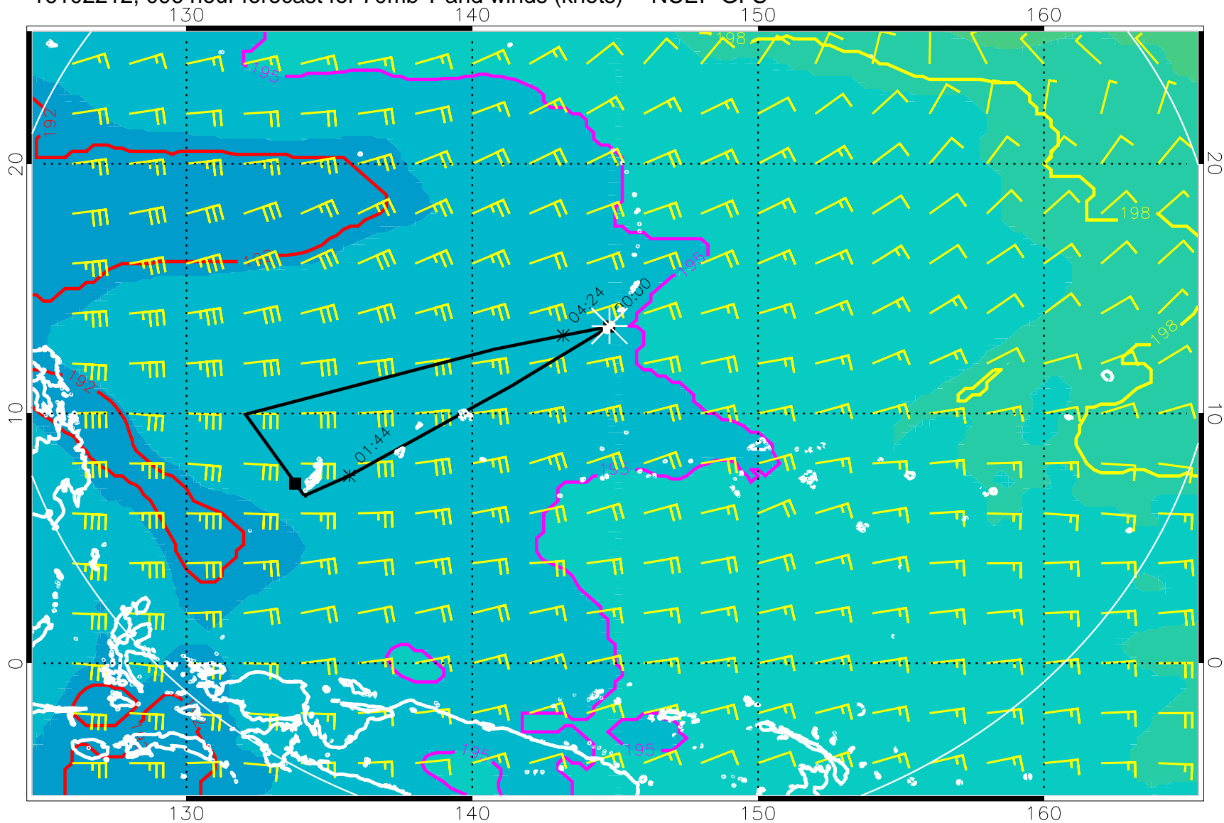
16102212, 096 hour forecast for 70mb T and winds (knots) -- NCEP GFS
