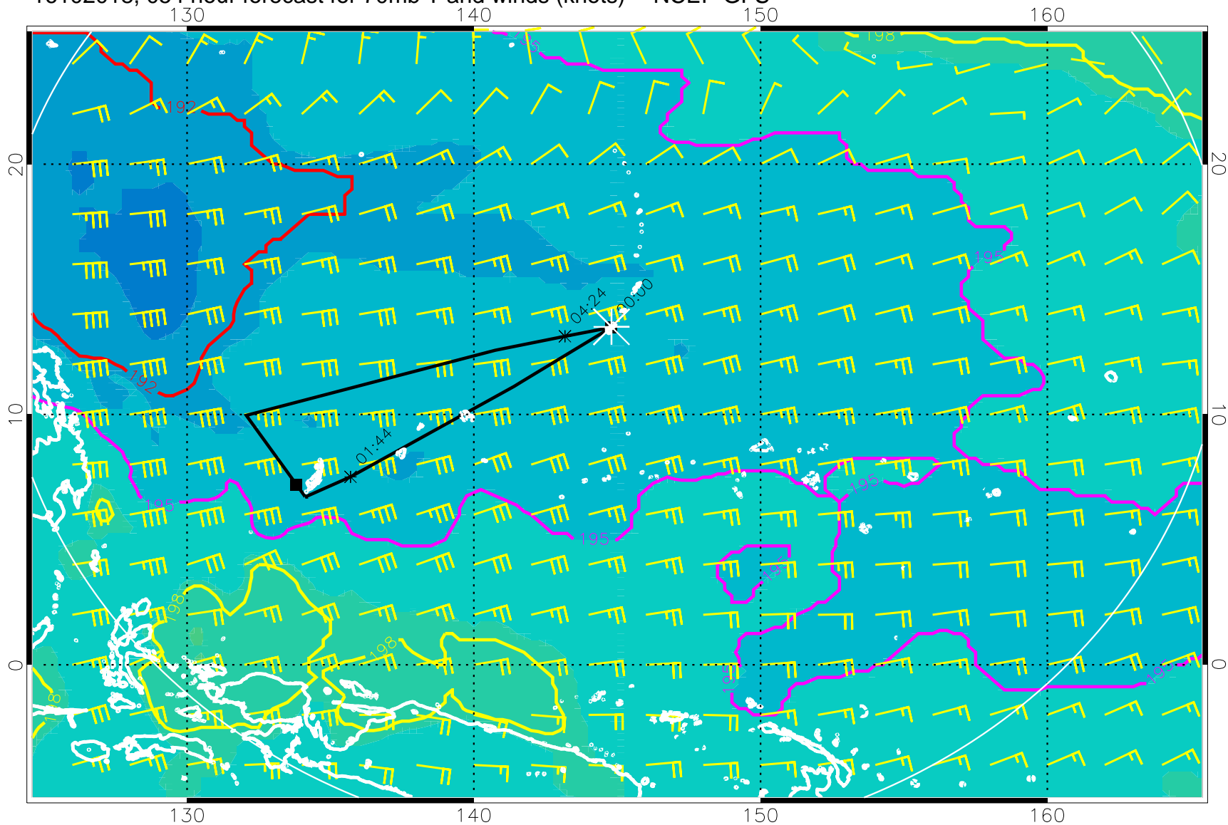
16102018, 054 hour forecast for 70mb T and winds (knots) -- NCEP GFS
