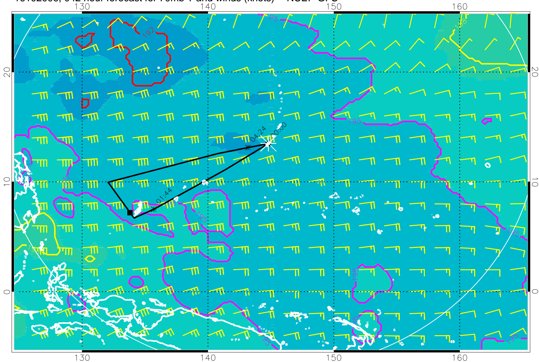
16102006, 042 hour forecast for 70mb T and winds (knots) -- NCEP GFS
