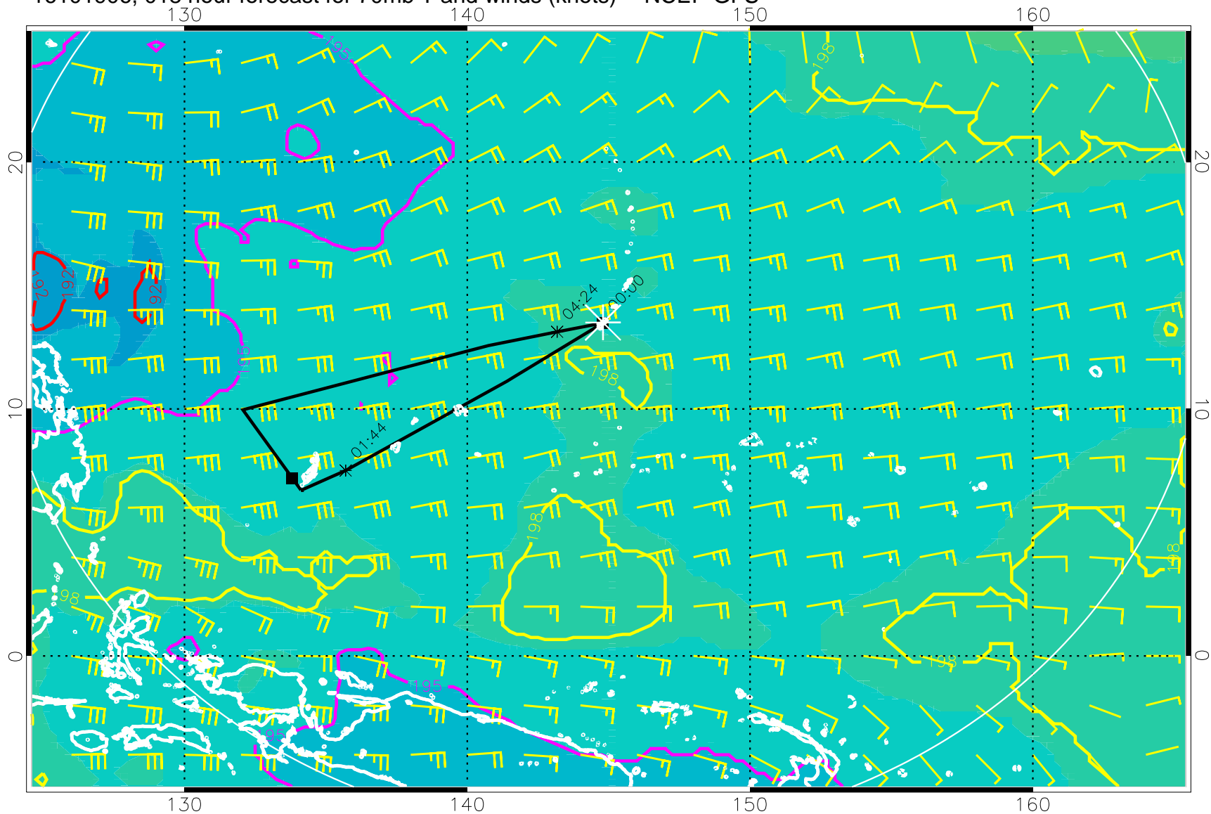
16101906, 018 hour forecast for 70mb T and winds (knots) -- NCEP GFS
