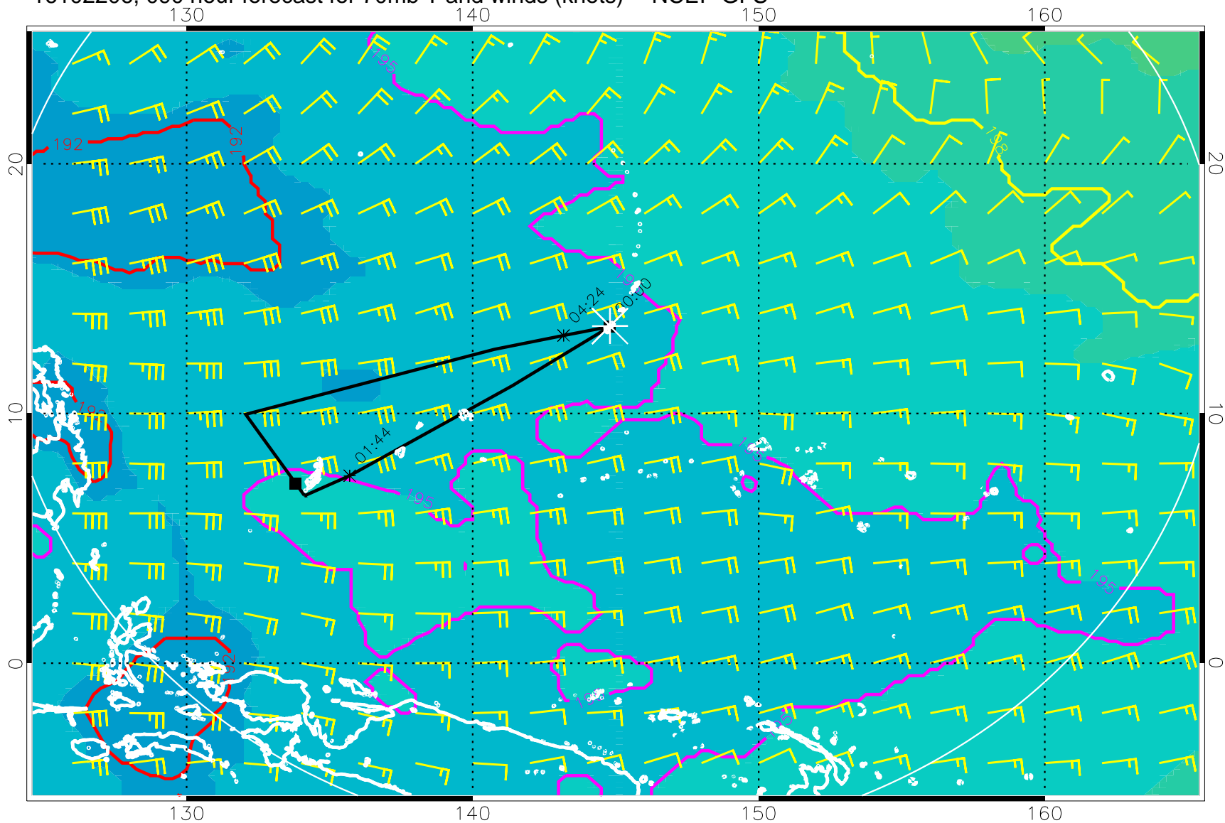
16102206, 090 hour forecast for 70mb T and winds (knots) -- NCEP GFS
