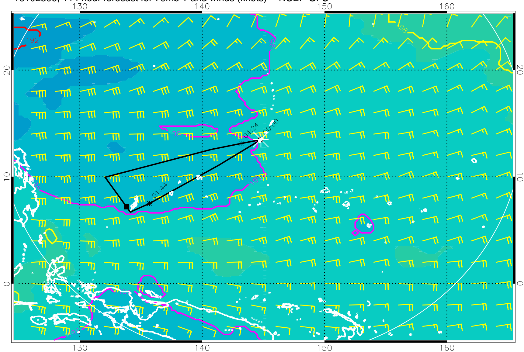
16102306, 114 hour forecast for 70mb T and winds (knots) -- NCEP GFS
