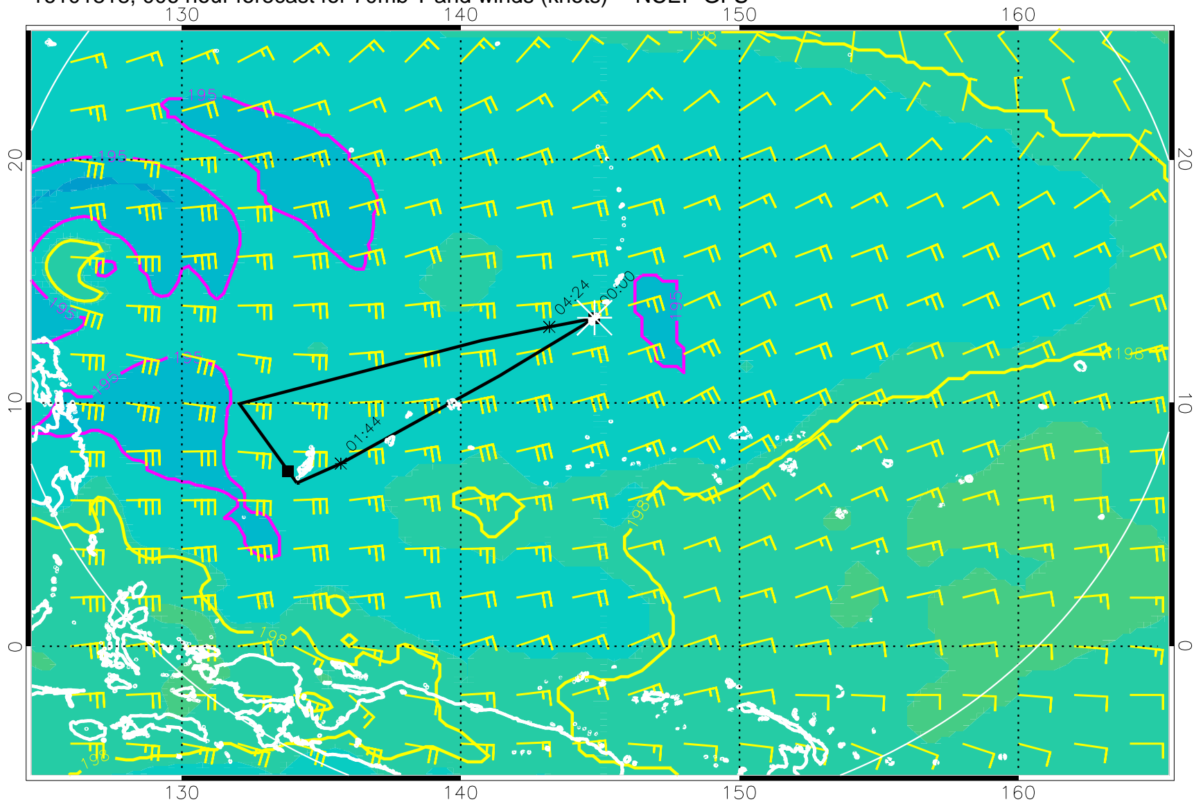
16101818, 006 hour forecast for 70mb T and winds (knots) -- NCEP GFS
