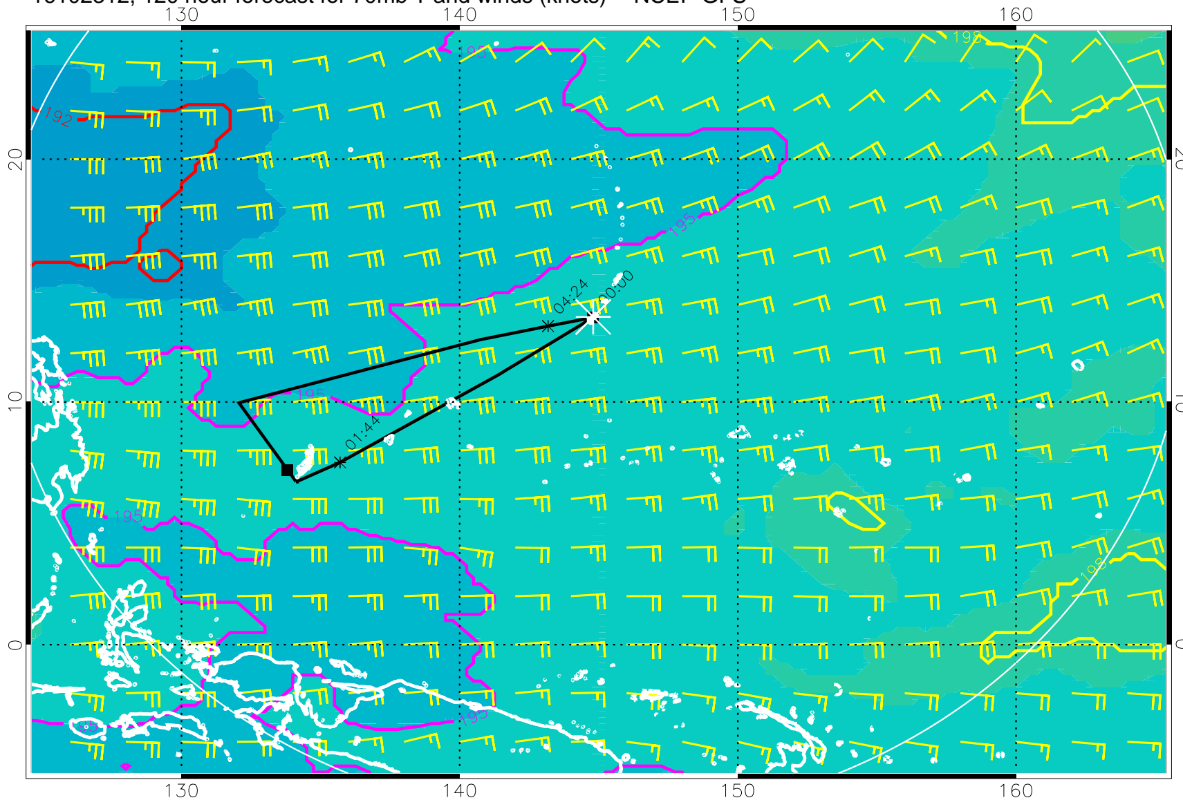
16102312, 120 hour forecast for 70mb T and winds (knots) -- NCEP GFS
