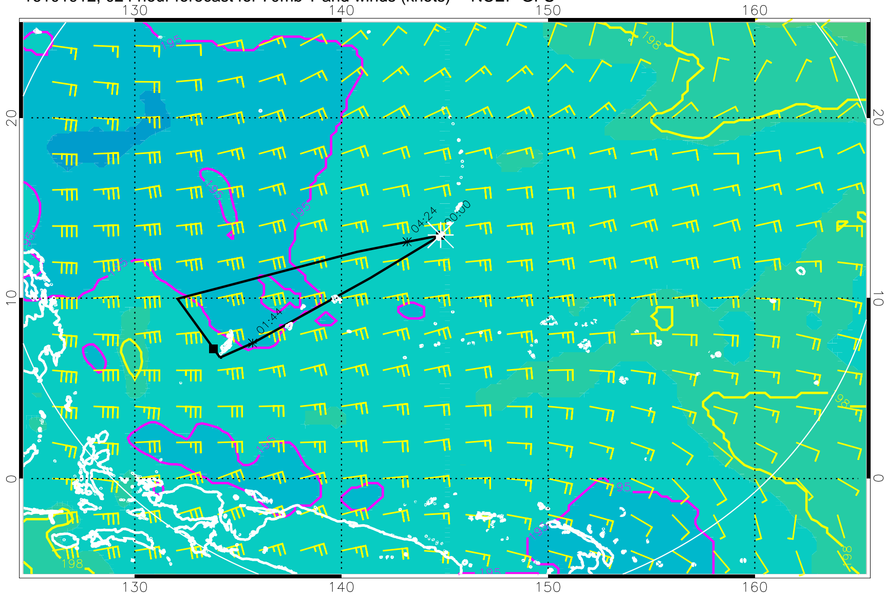
16101912, 024 hour forecast for 70mb T and winds (knots) -- NCEP GFS
