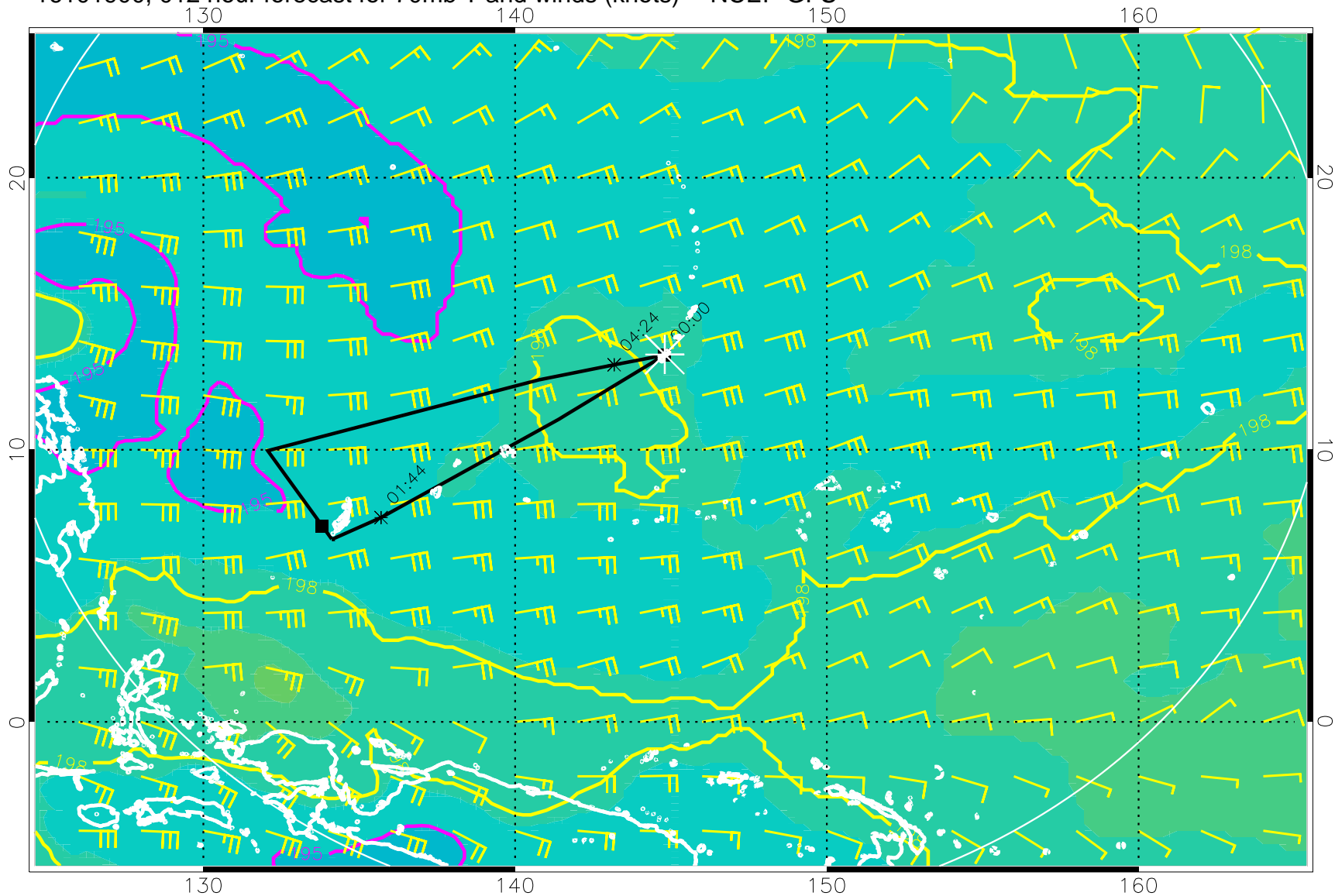
16101900, 012 hour forecast for 70mb T and winds (knots) -- NCEP GFS
