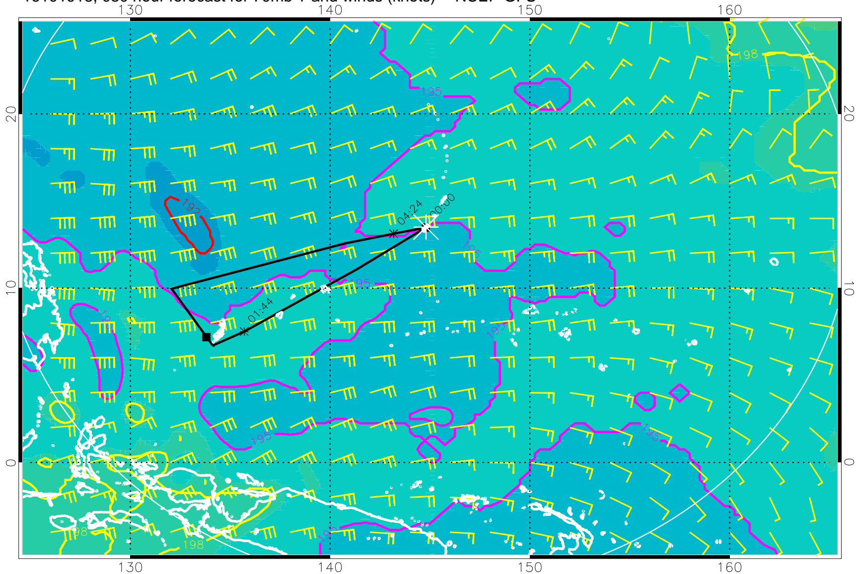
16101918, 030 hour forecast for 70mb T and winds (knots) -- NCEP GFS
