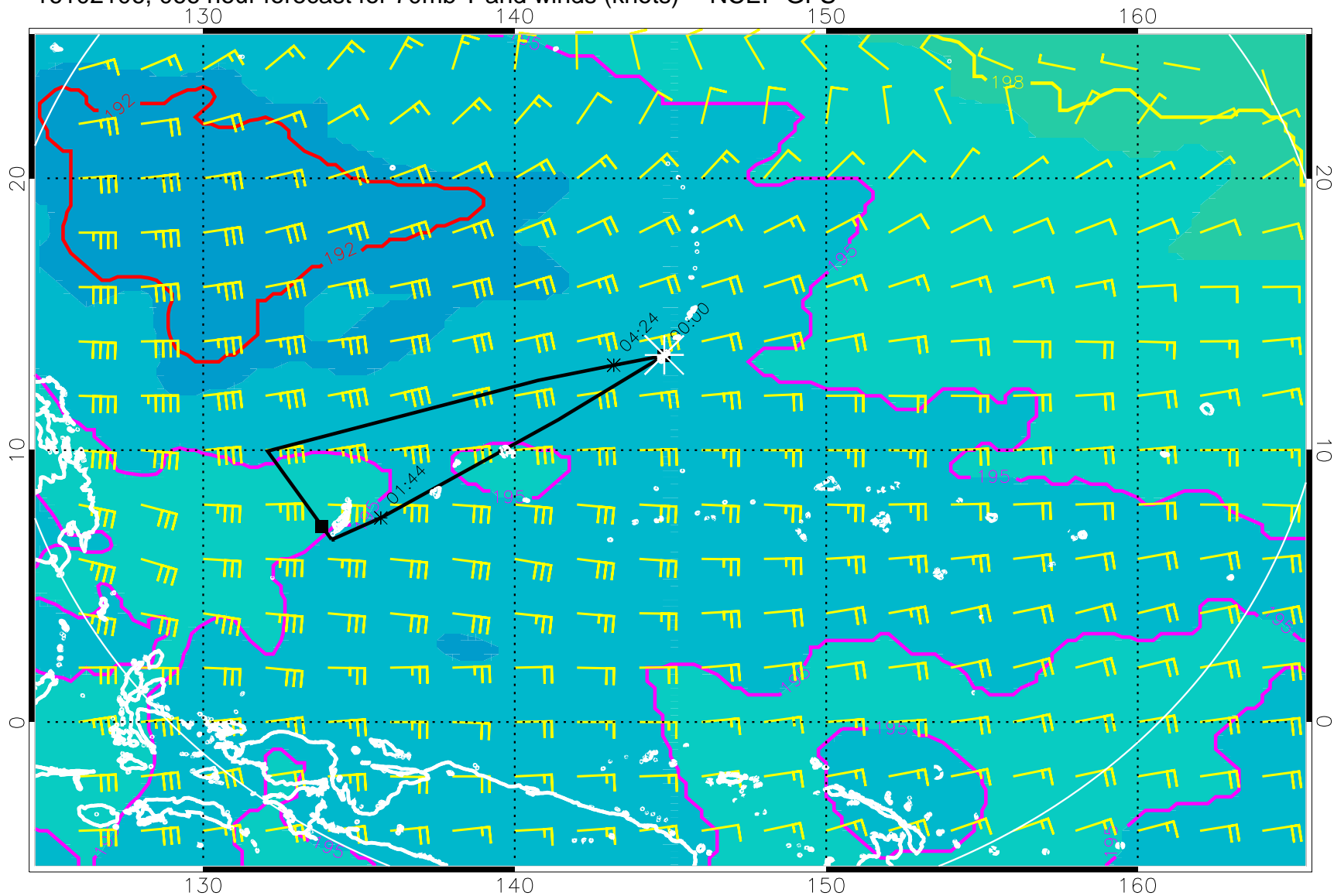
16102106, 066 hour forecast for 70mb T and winds (knots) -- NCEP GFS
