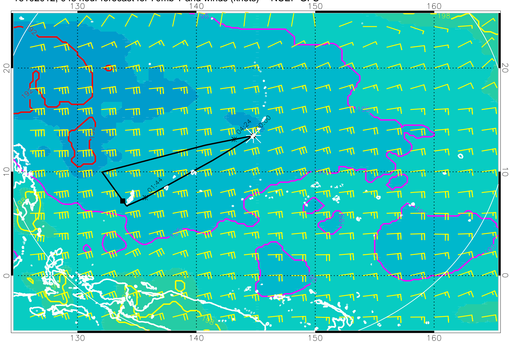
16102012, 048 hour forecast for 70mb T and winds (knots) -- NCEP GFS
