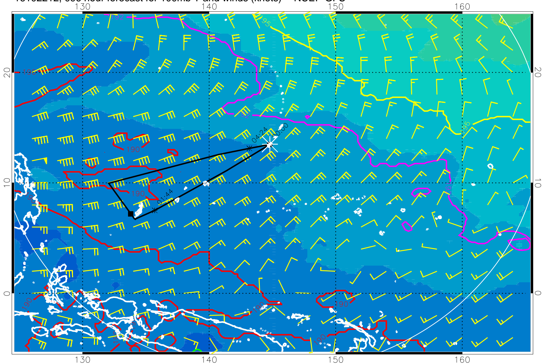
16102212, 096 hour forecast for 100mb T and winds (knots) -- NCEP GFS
