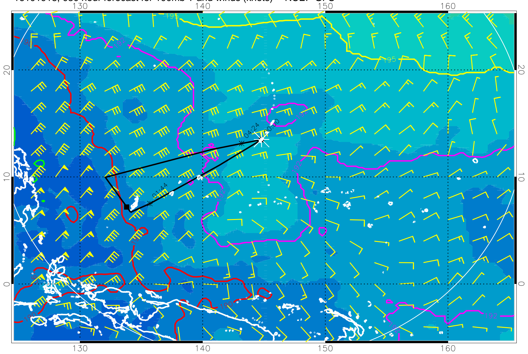
16101918, 030 hour forecast for 100mb T and winds (knots) -- NCEP GFS
