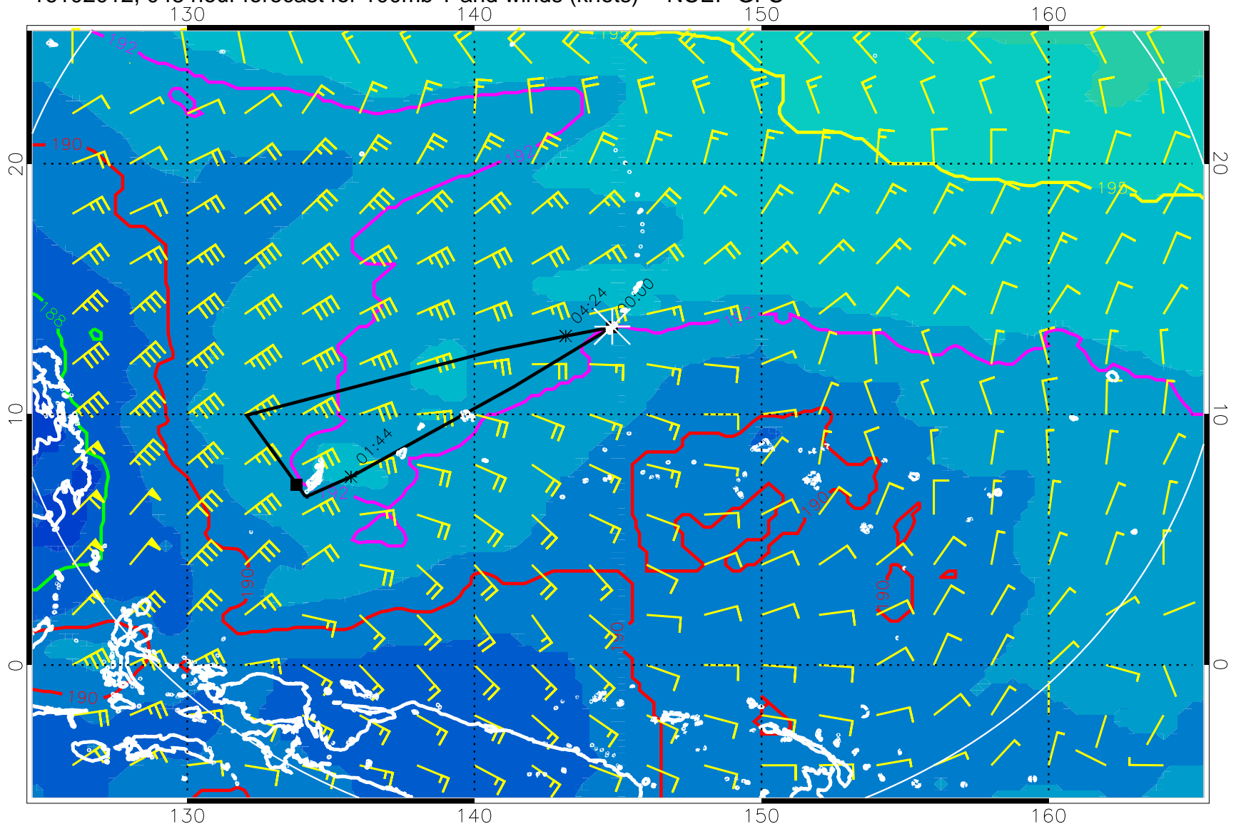
16102012, 048 hour forecast for 100mb T and winds (knots) -- NCEP GFS
