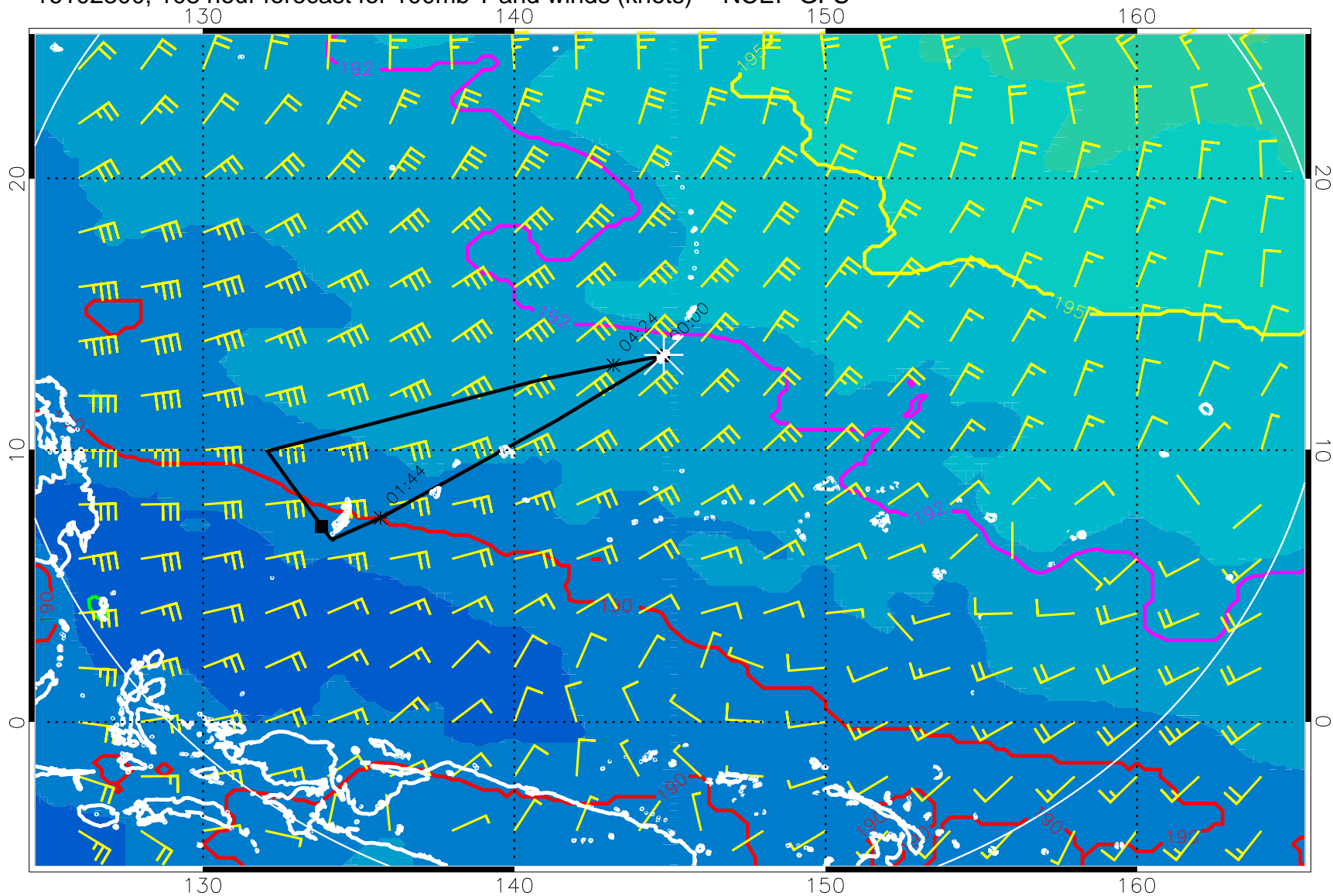
16102300, 108 hour forecast for 100mb T and winds (knots) -- NCEP GFS
