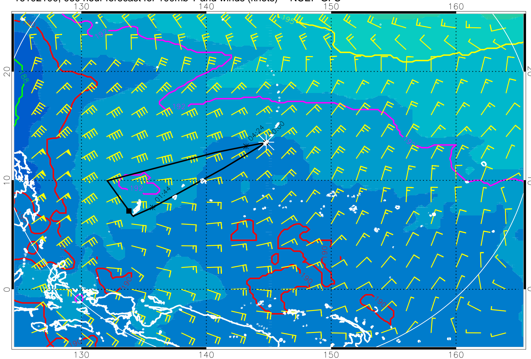
16102100, 060 hour forecast for 100mb T and winds (knots) -- NCEP GFS
