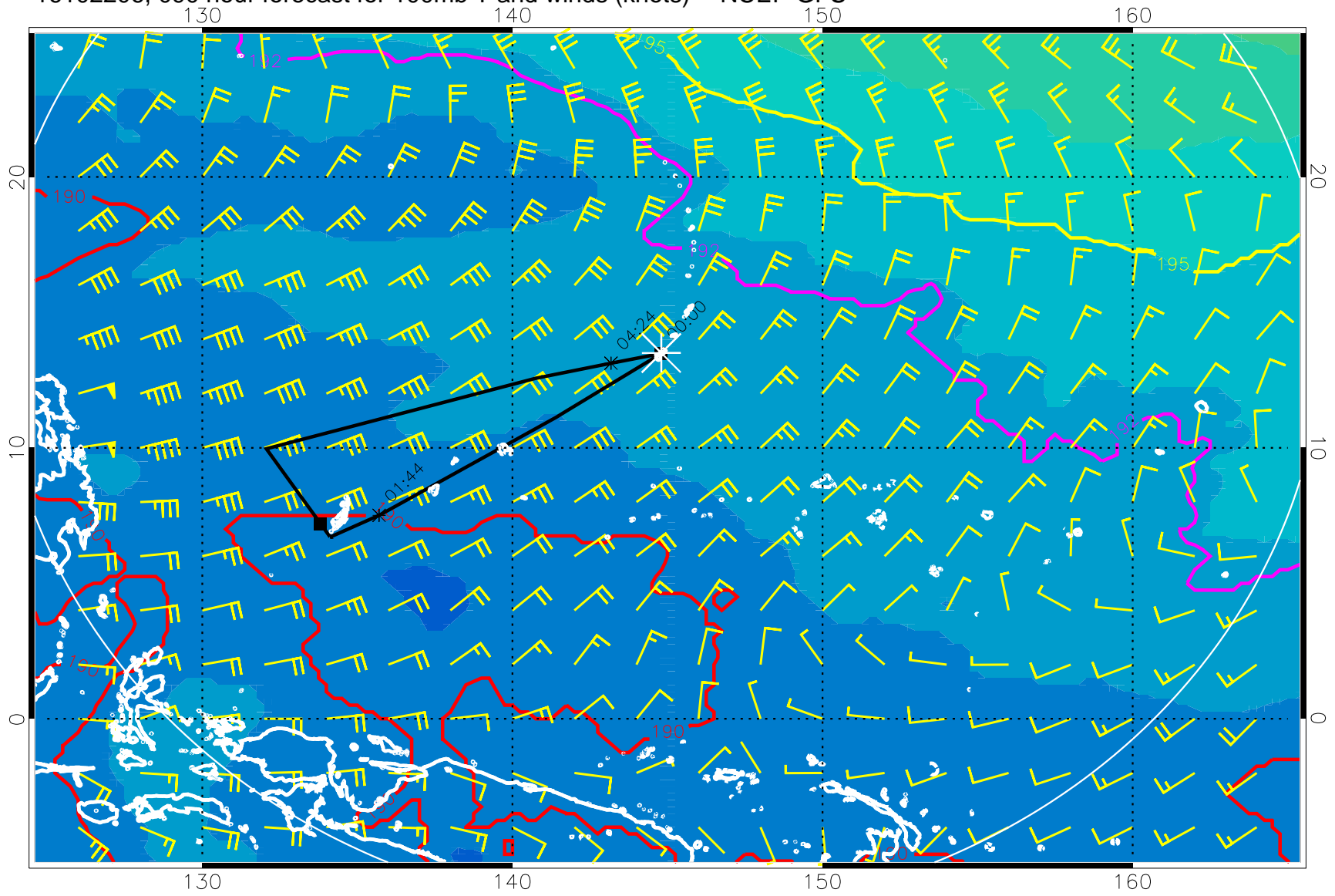
16102206, 090 hour forecast for 100mb T and winds (knots) -- NCEP GFS
