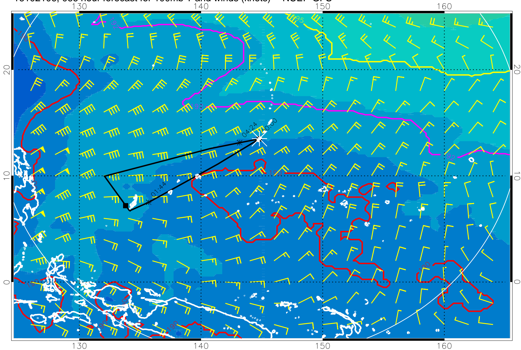
16102106, 066 hour forecast for 100mb T and winds (knots) -- NCEP GFS
