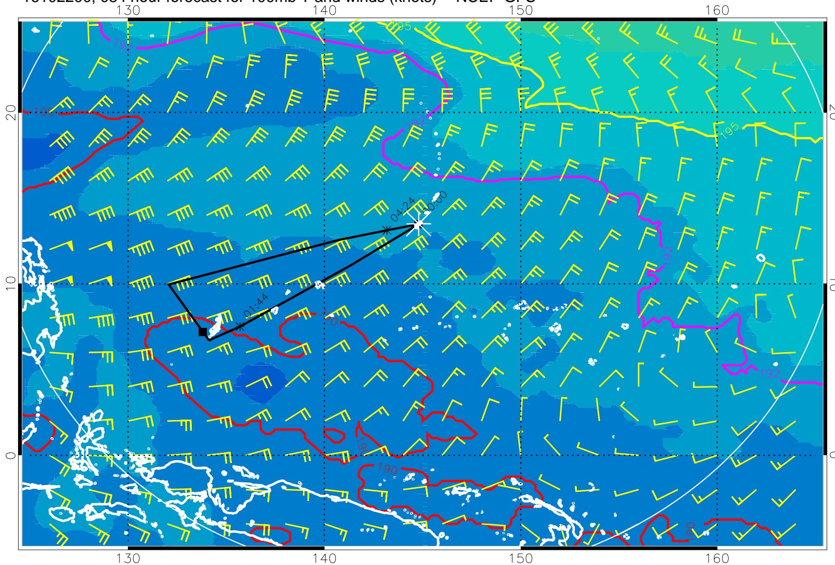
16102200, 084 hour forecast for 100mb T and winds (knots) -- NCEP GFS
