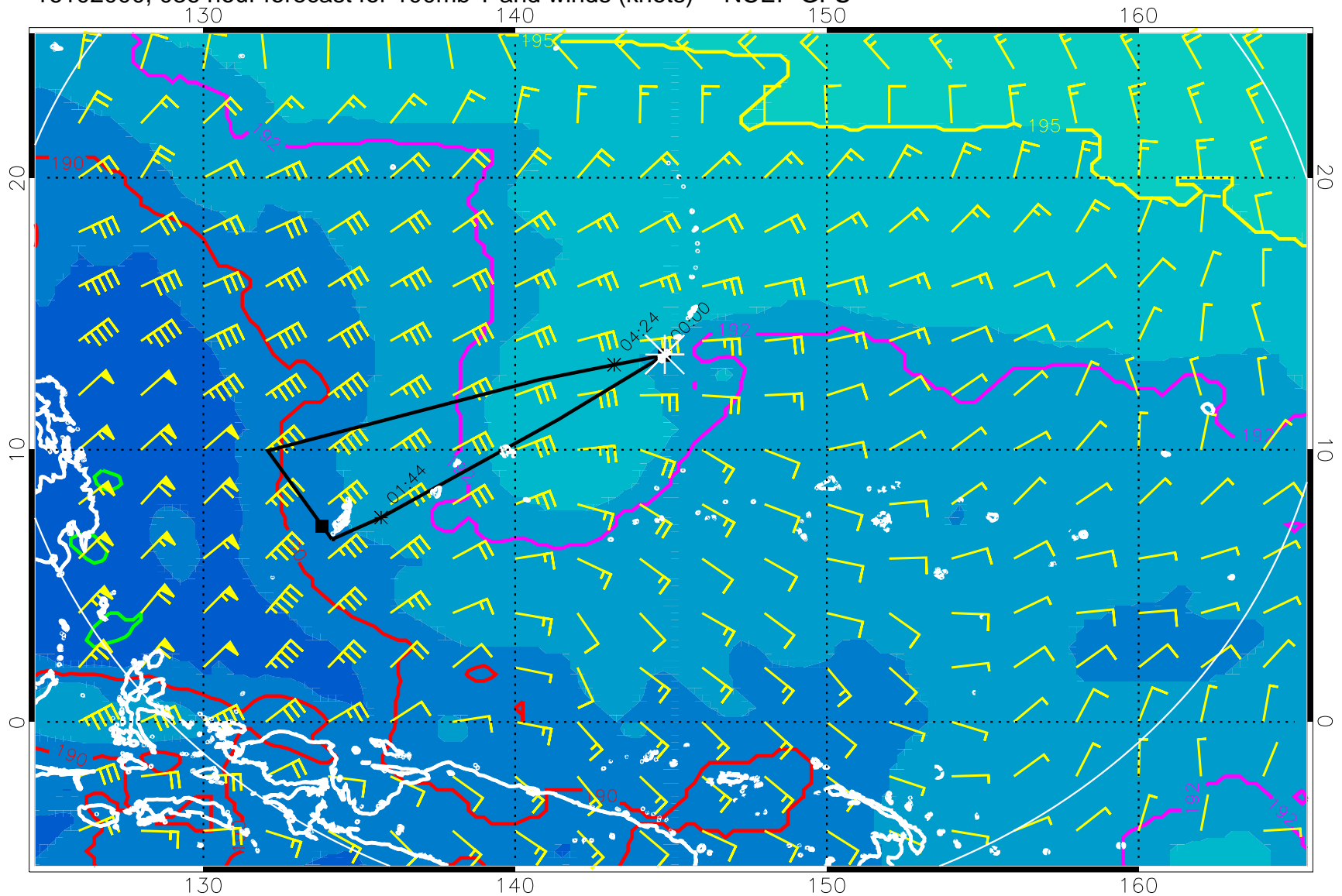
16102000, 036 hour forecast for 100mb T and winds (knots) -- NCEP GFS
