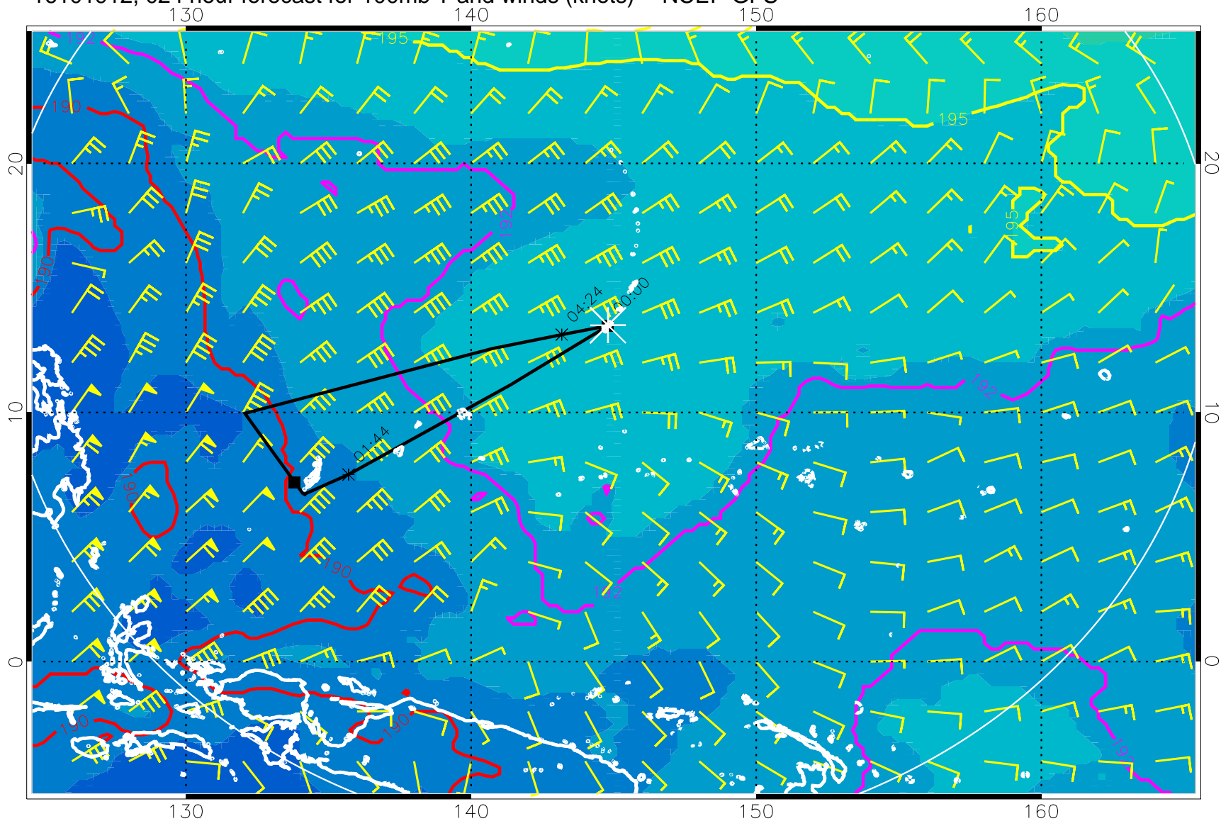
16101912, 024 hour forecast for 100mb T and winds (knots) -- NCEP GFS
