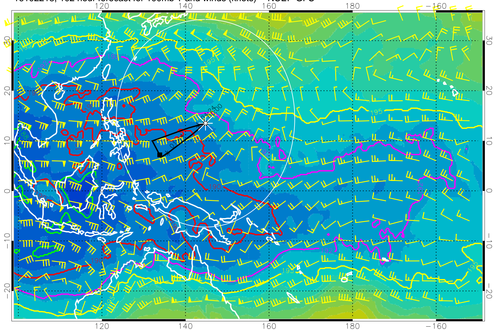
16102218, 102 hour forecast for 100mb T and winds (knots) -- NCEP GFS
