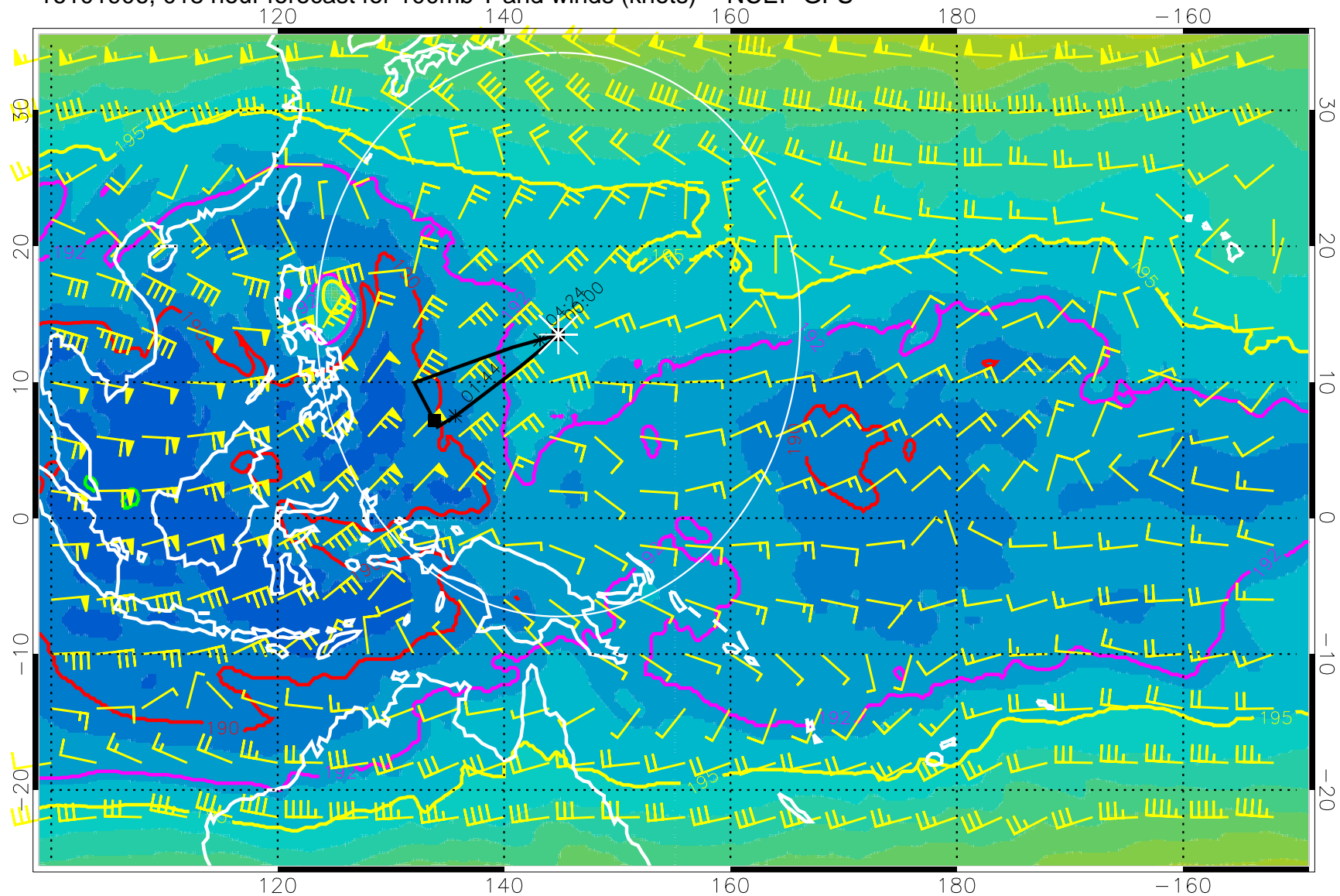
16101906, 018 hour forecast for 100mb T and winds (knots) -- NCEP GFS
