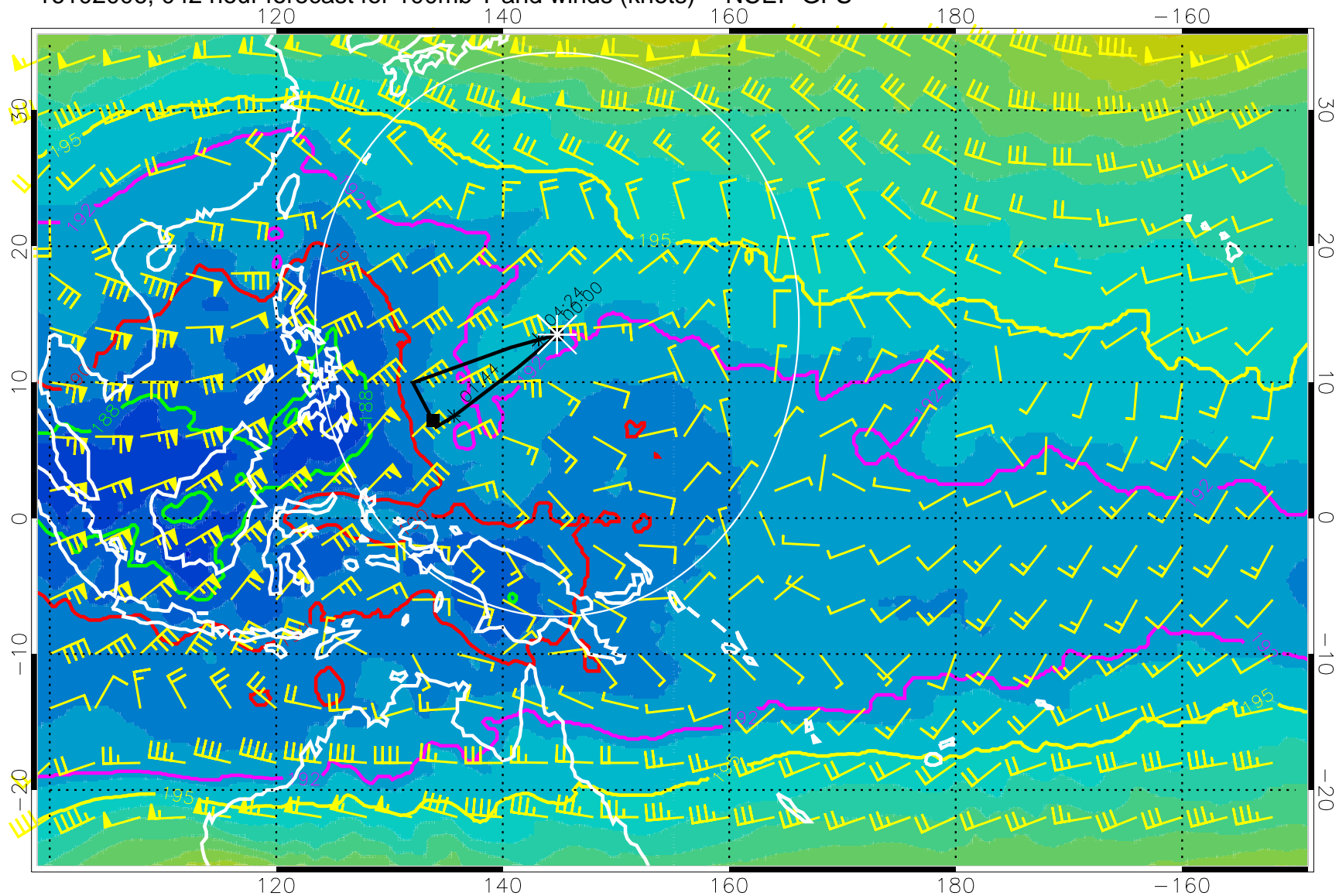
16102006, 042 hour forecast for 100mb T and winds (knots) -- NCEP GFS
