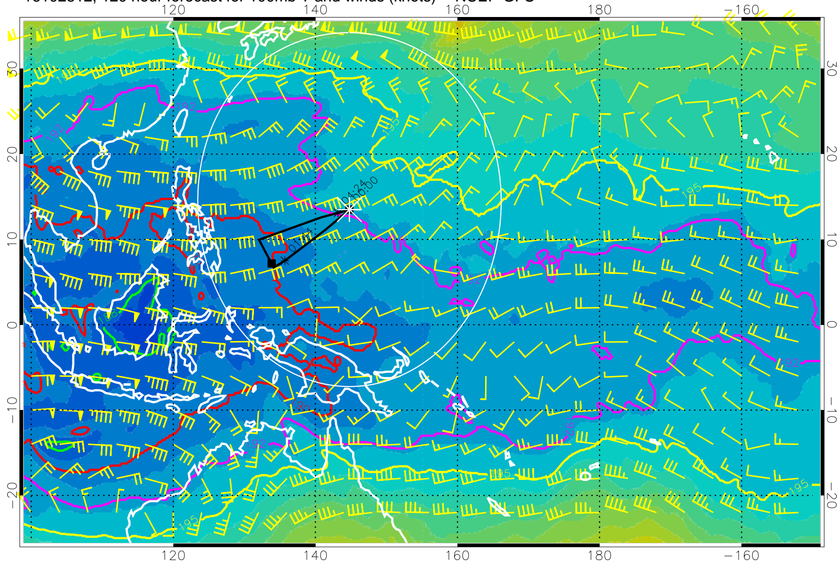
16102312, 120 hour forecast for 100mb T and winds (knots) -- NCEP GFS
