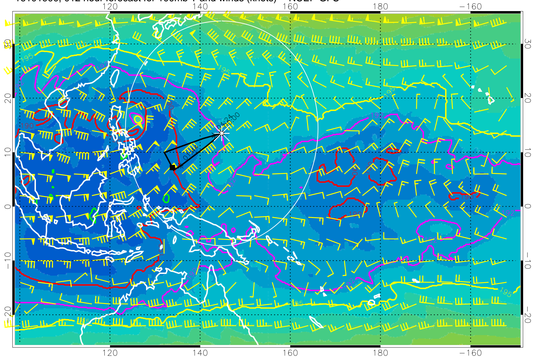
16101900, 012 hour forecast for 100mb T and winds (knots) -- NCEP GFS
