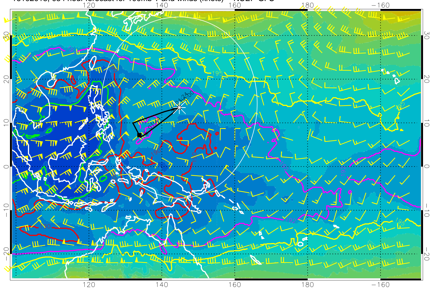
16102018, 054 hour forecast for 100mb T and winds (knots) -- NCEP GFS
