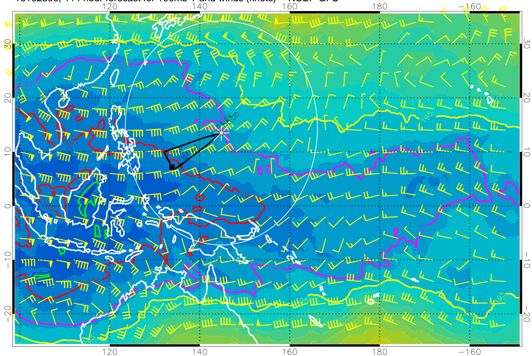
16102306, 114 hour forecast for 100mb T and winds (knots) -- NCEP GFS
