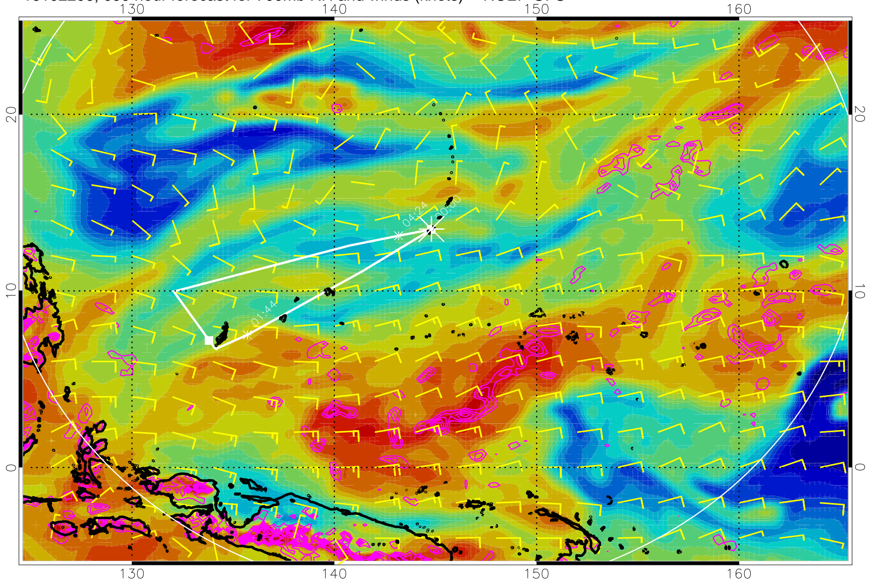
16102206, 090 hour forecast for 700mb RH and winds (knots) -- NCEP GFS
