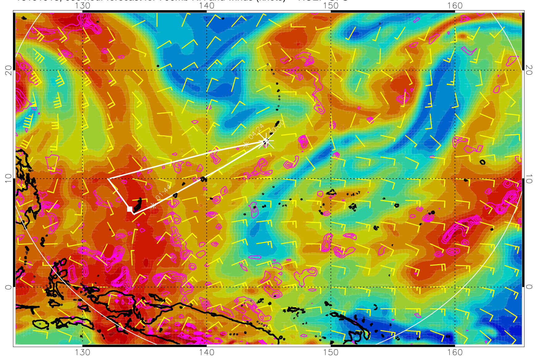
16101918, 030 hour forecast for 700mb RH and winds (knots) -- NCEP GFS
