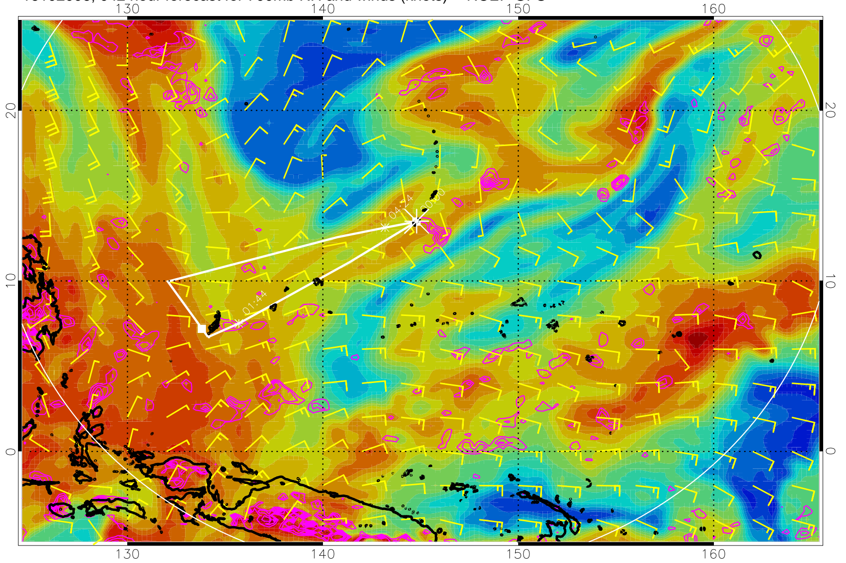
16102006, 042 hour forecast for 700mb RH and winds (knots) -- NCEP GFS
