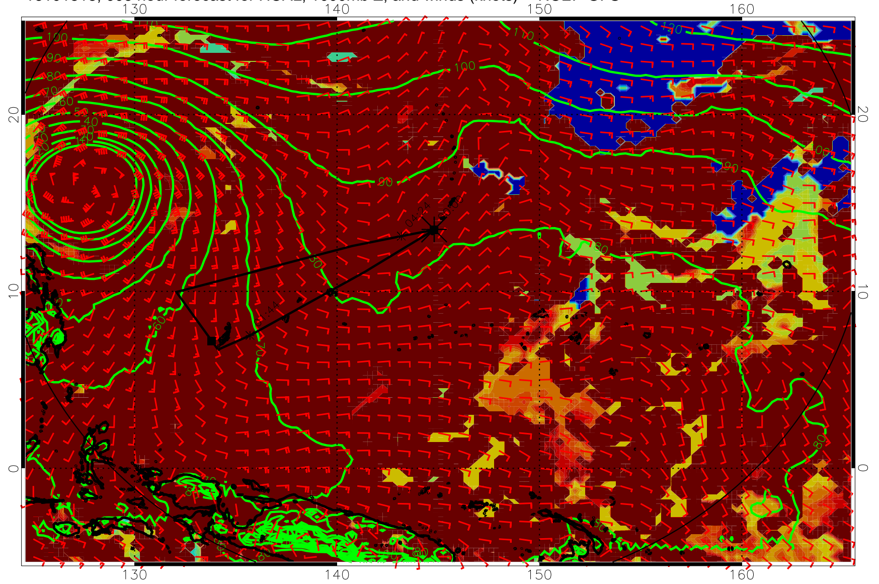
16101818, 006 hour forecast for HCAL, 1000mb Z, and winds (knots) -- NCEP GFS
