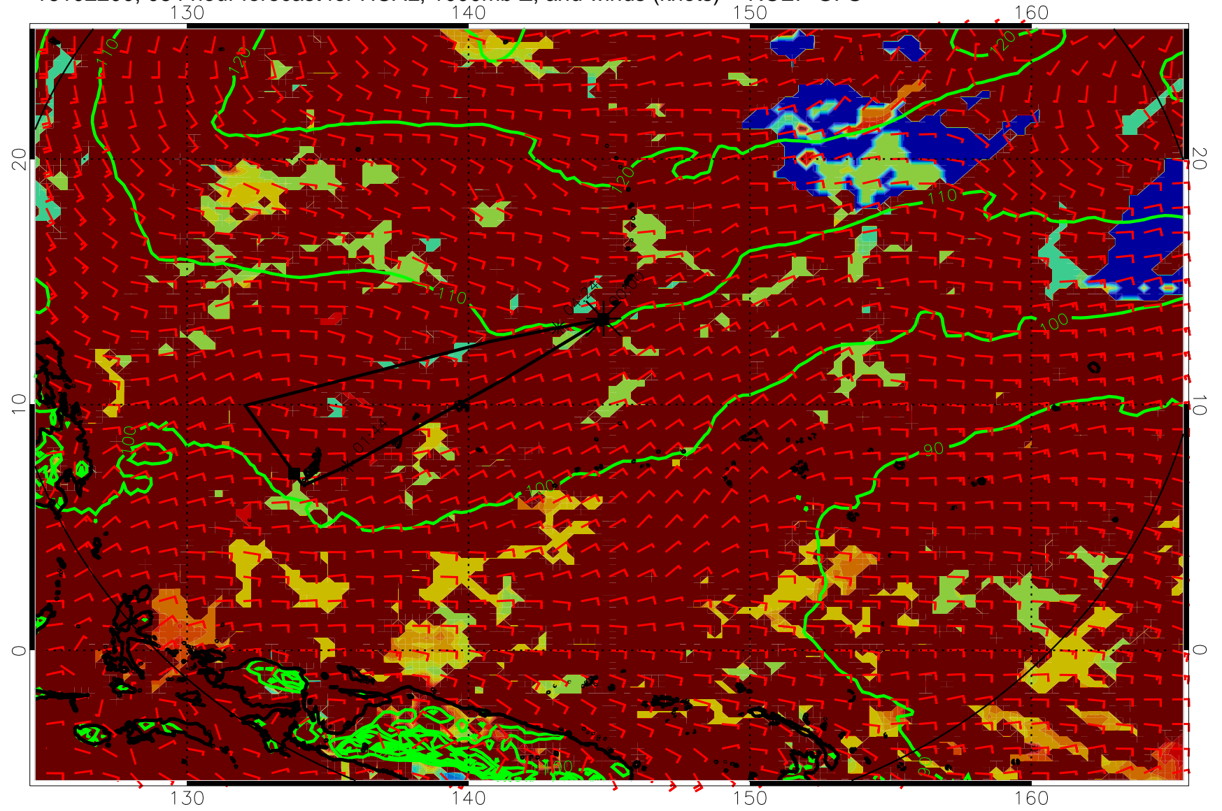
16102200, 084 hour forecast for HCAL, 1000mb Z, and winds (knots) -- NCEP GFS
