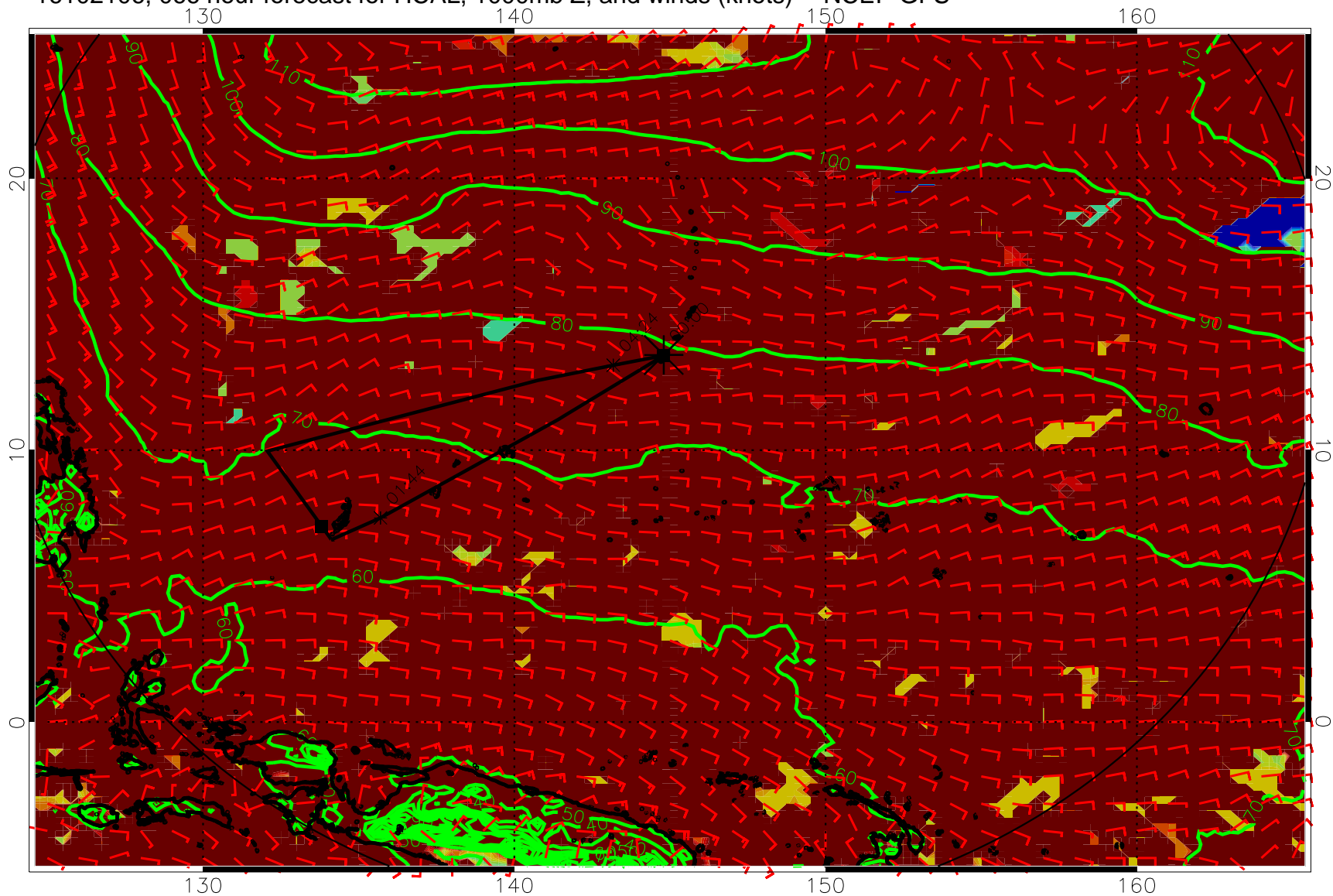
16102106, 066 hour forecast for HCAL, 1000mb Z, and winds (knots) -- NCEP GFS
