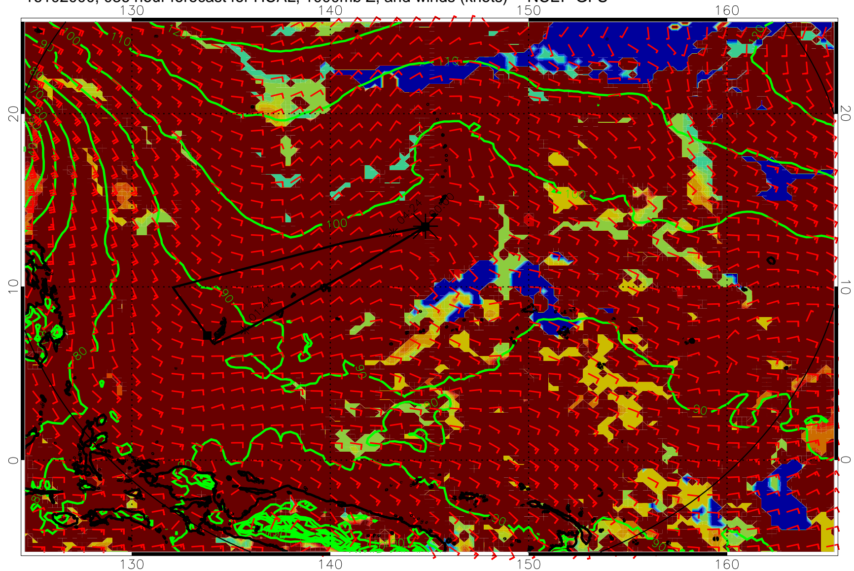
16102000, 036 hour forecast for HCAL, 1000mb Z, and winds (knots) -- NCEP GFS
