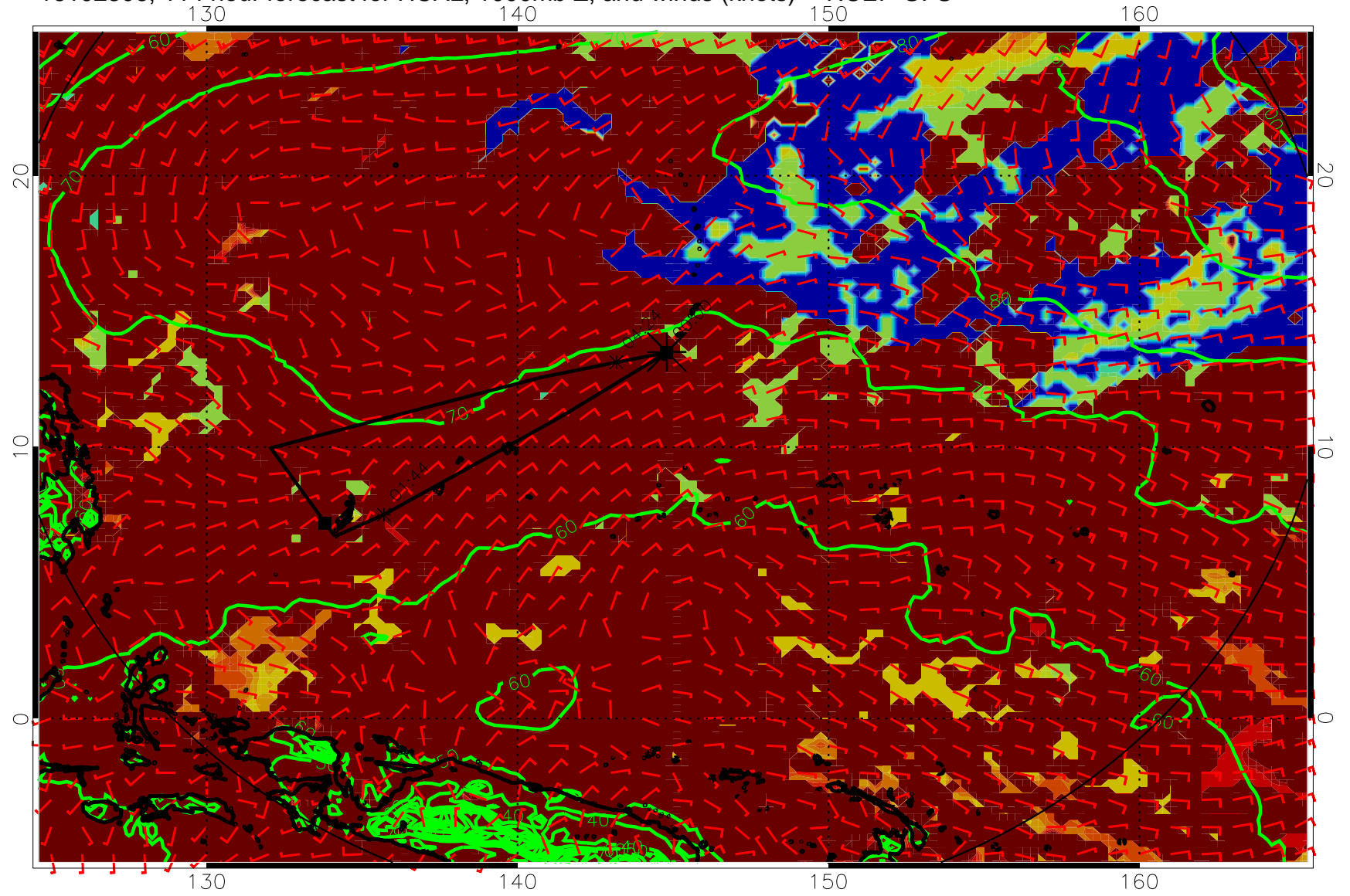
16102306, 114 hour forecast for HCAL, 1000mb Z, and winds (knots) -- NCEP GFS
