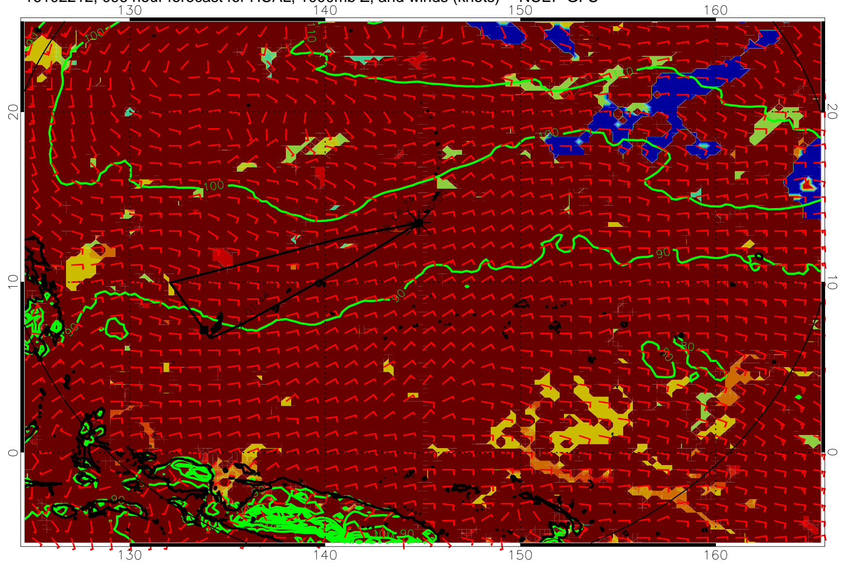
16102212, 096 hour forecast for HCAL, 1000mb Z, and winds (knots) -- NCEP GFS
