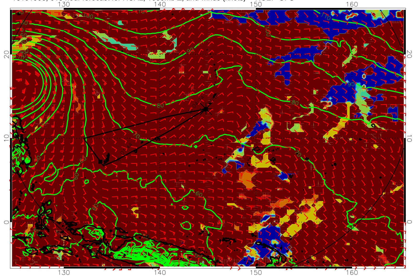
16101906, 018 hour forecast for HCAL, 1000mb Z, and winds (knots) -- NCEP GFS
