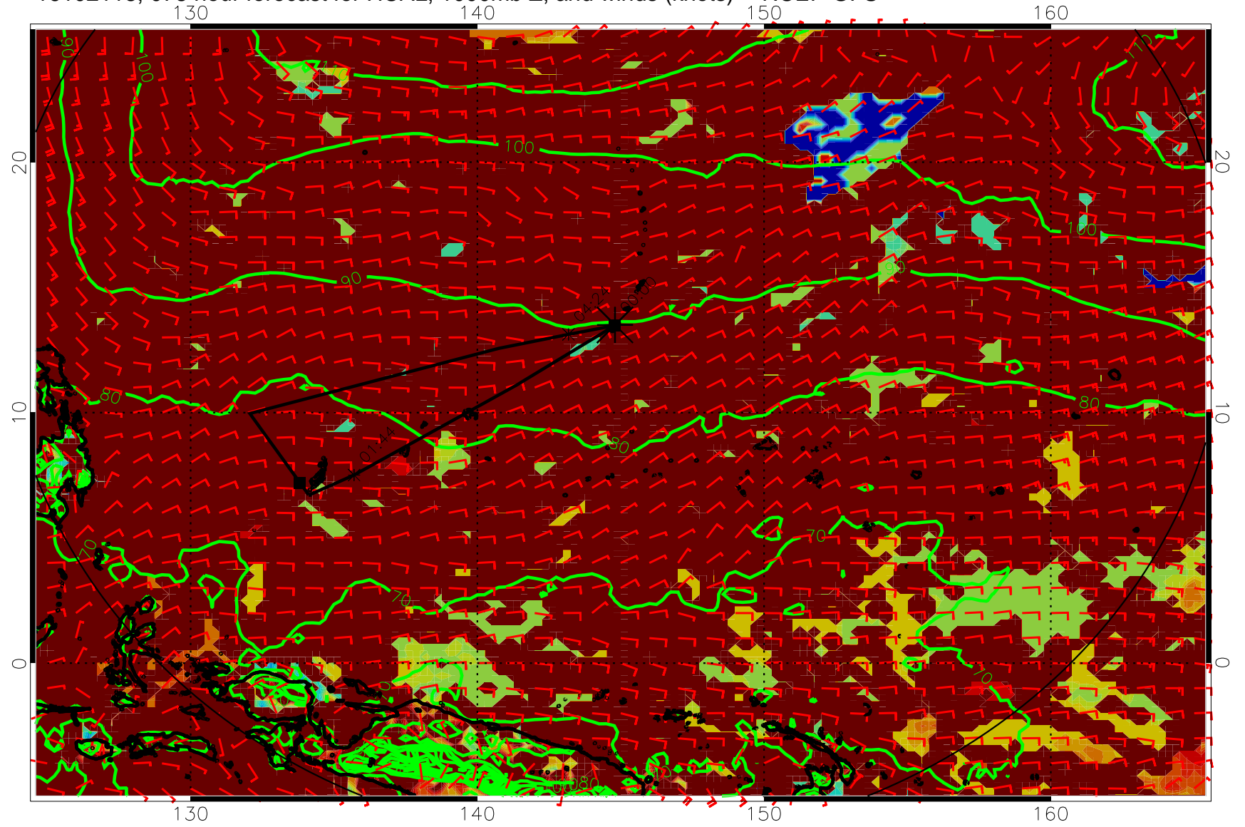
16102118, 078 hour forecast for HCAL, 1000mb Z, and winds (knots) -- NCEP GFS
