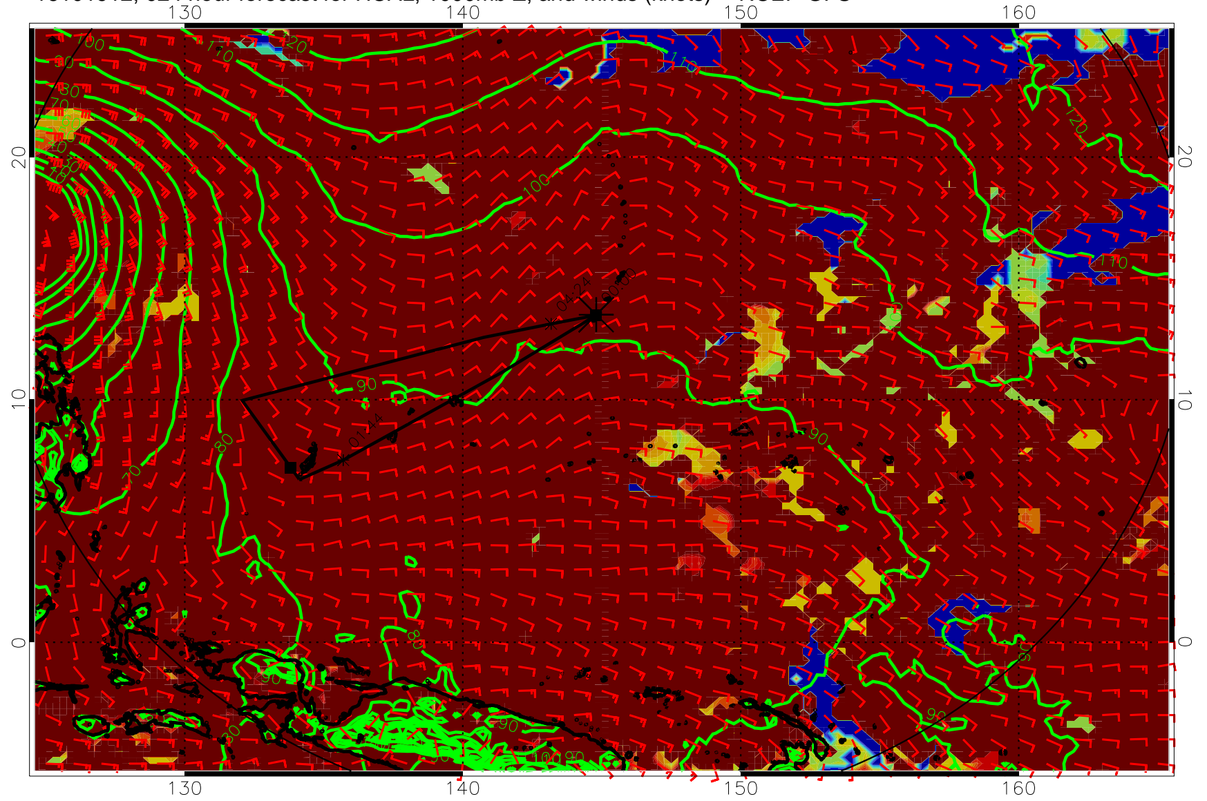
16101912, 024 hour forecast for HCAL, 1000mb Z, and winds (knots) -- NCEP GFS
