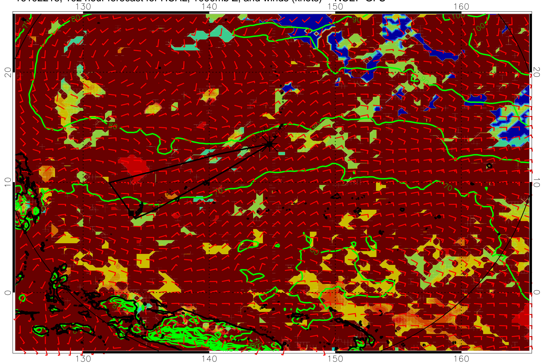
16102218, 102 hour forecast for HCAL, 1000mb Z, and winds (knots) -- NCEP GFS
