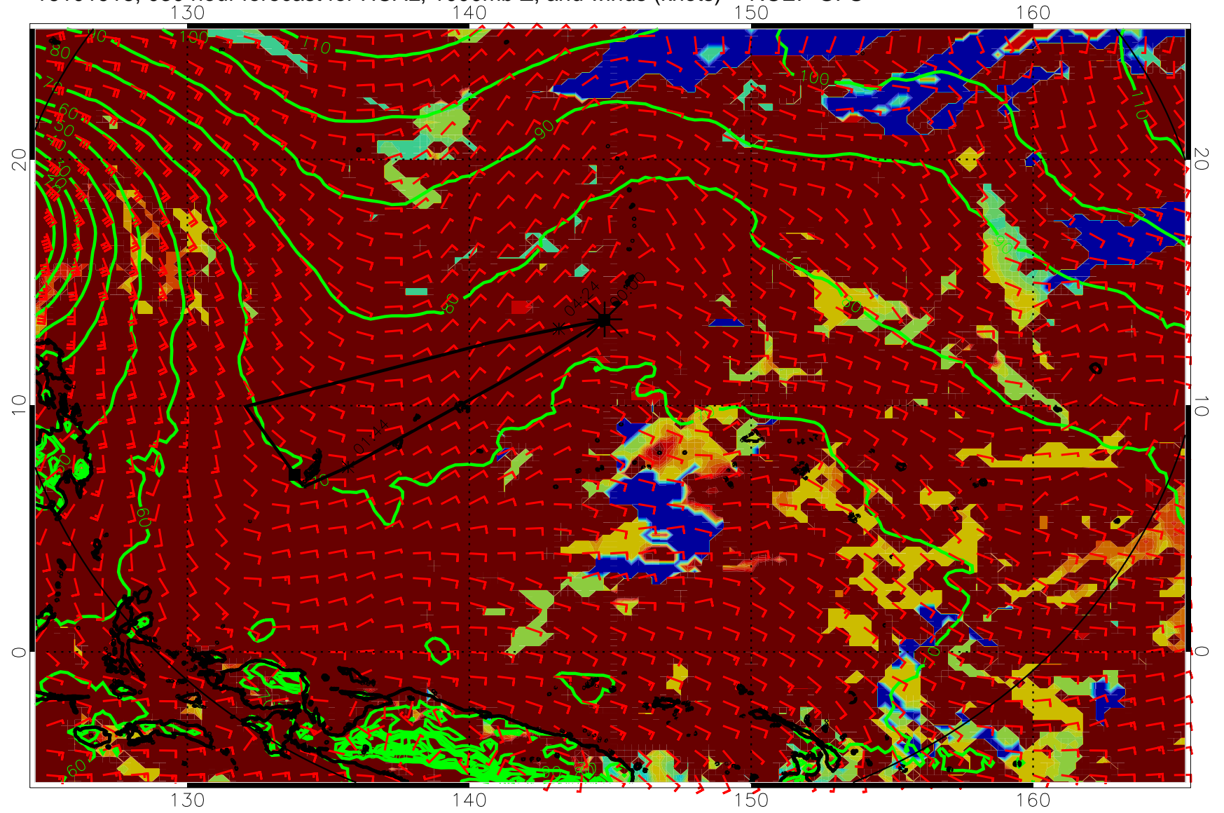
16101918, 030 hour forecast for HCAL, 1000mb Z, and winds (knots) -- NCEP GFS
