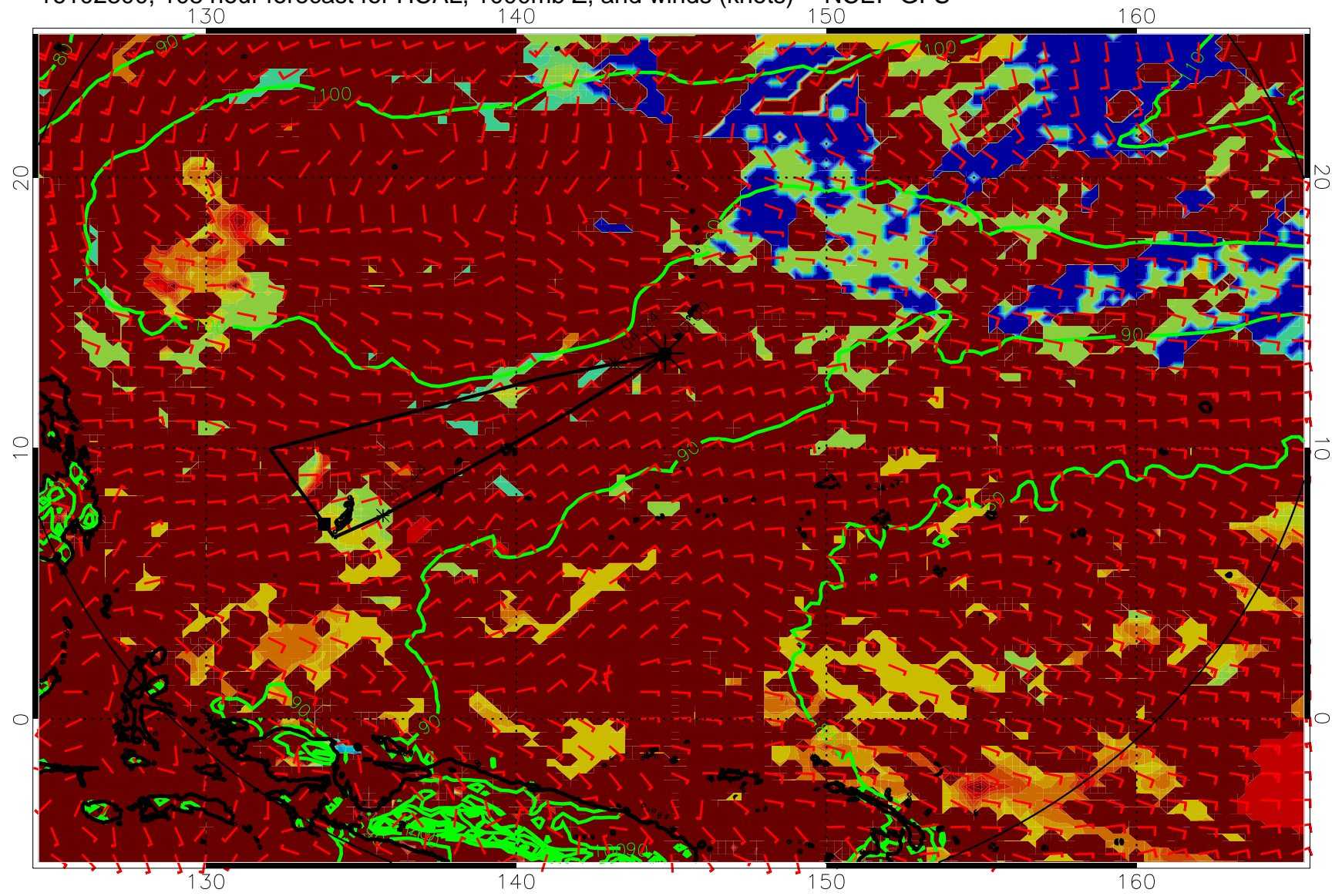
16102300, 108 hour forecast for HCAL, 1000mb Z, and winds (knots) -- NCEP GFS
