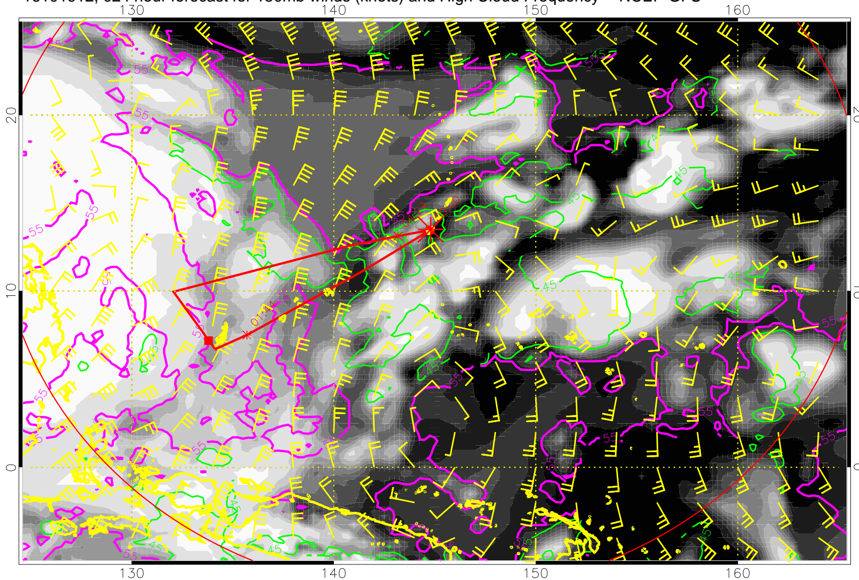
16101912, 024 hour forecast for 150mb winds (knots) and High Cloud Frequency -- NCEP GFS
