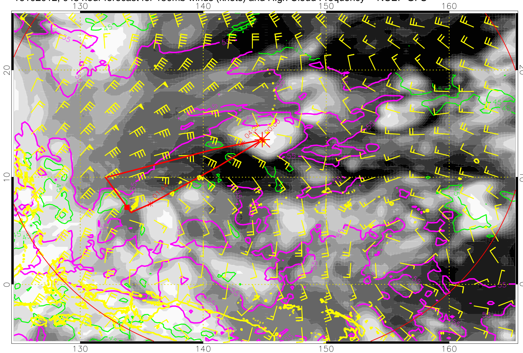
16102012, 048 hour forecast for 150mb winds (knots) and High Cloud Frequency -- NCEP GFS
