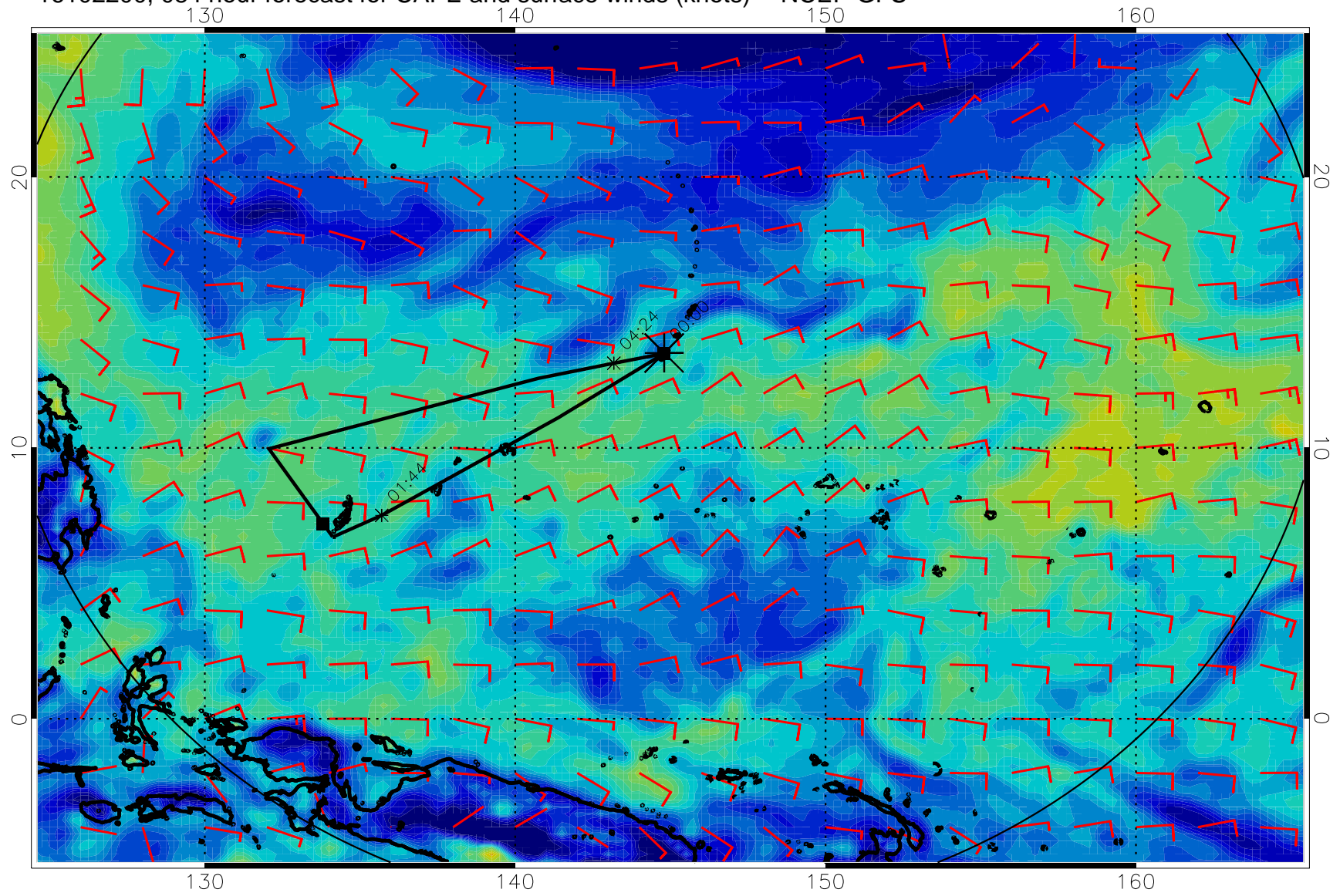
16102200, 084 hour forecast for CAPE and surface winds (knots) -- NCEP GFS
