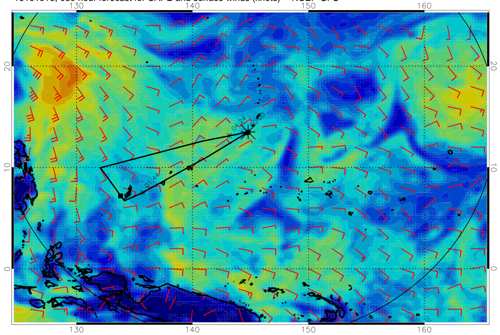
16101918, 030 hour forecast for CAPE and surface winds (knots) -- NCEP GFS
