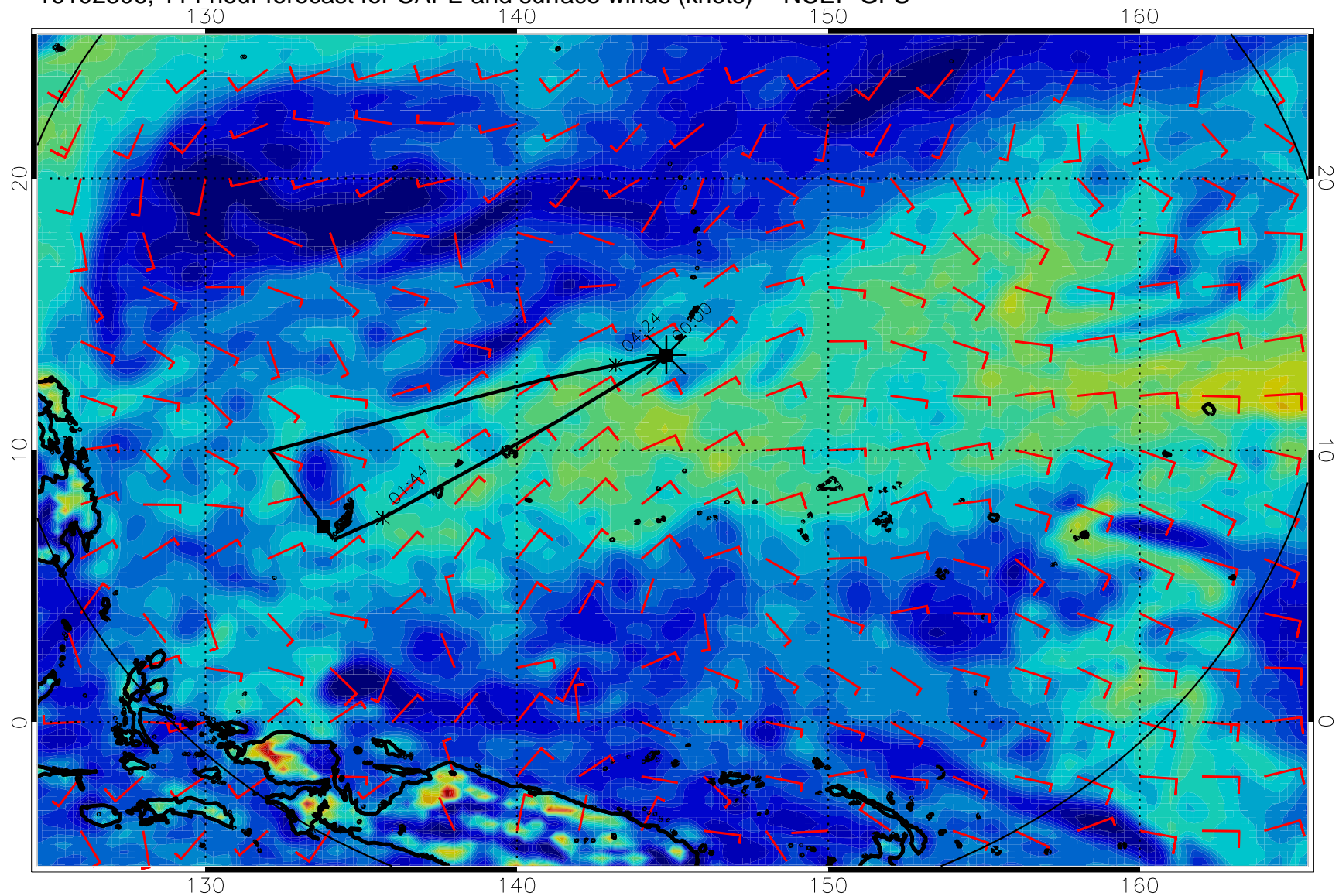
16102306, 114 hour forecast for CAPE and surface winds (knots) -- NCEP GFS
