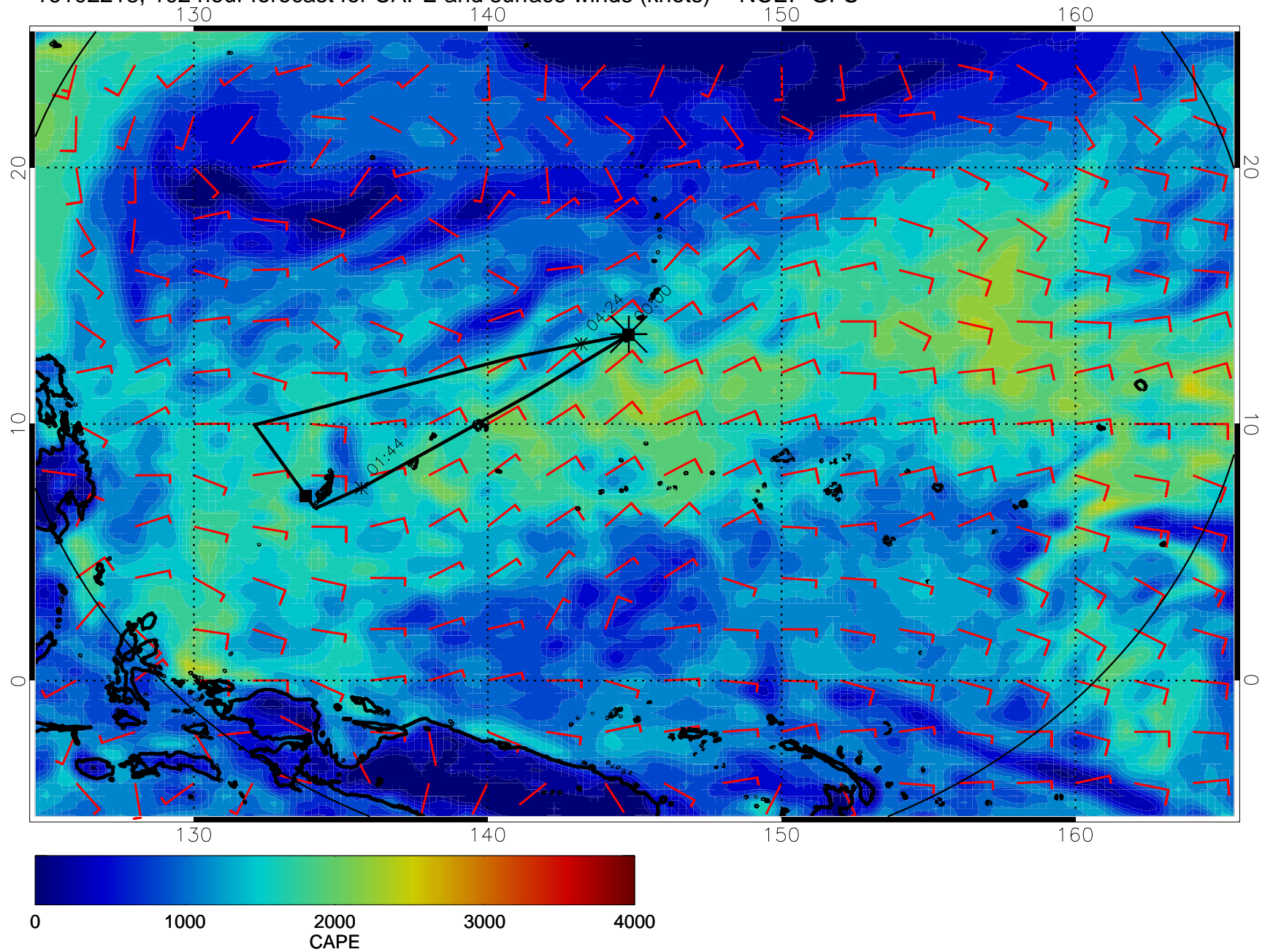
16102218, 102 hour forecast for CAPE and surface winds (knots) -- NCEP GFS
