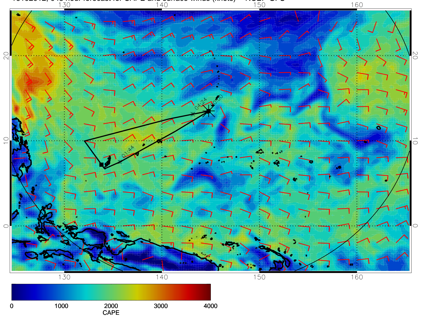
16102012, 048 hour forecast for CAPE and surface winds (knots) -- NCEP GFS
