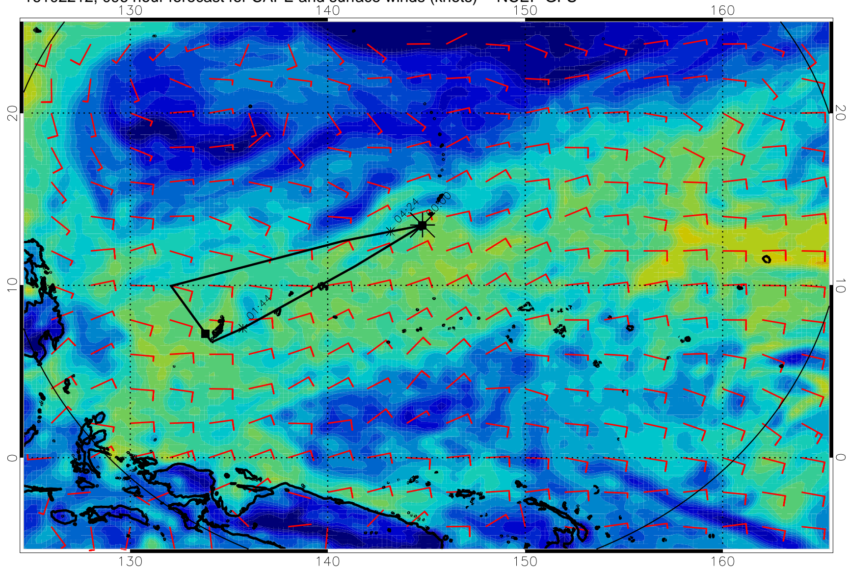
16102212, 096 hour forecast for CAPE and surface winds (knots) -- NCEP GFS
