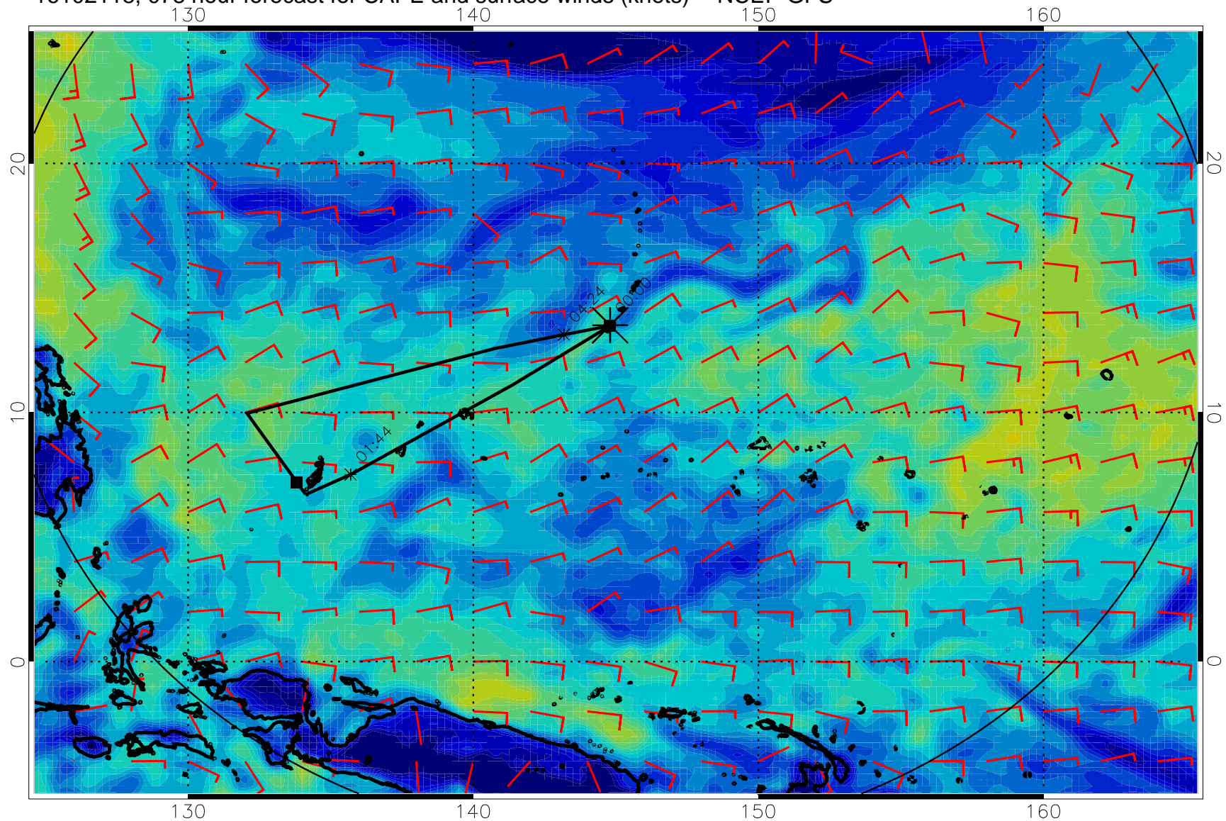
16102118, 078 hour forecast for CAPE and surface winds (knots) -- NCEP GFS
