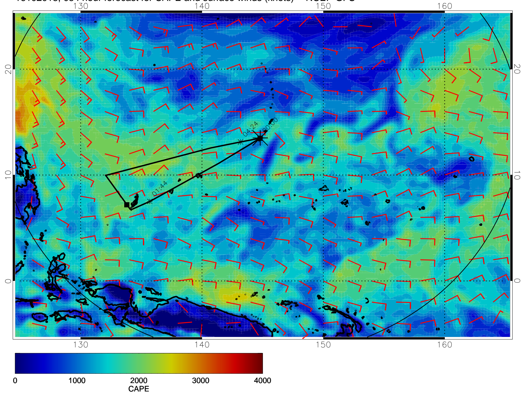
16102018, 054 hour forecast for CAPE and surface winds (knots) -- NCEP GFS
