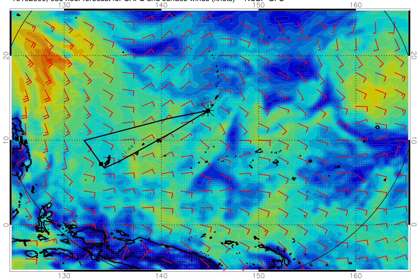
16102000, 036 hour forecast for CAPE and surface winds (knots) -- NCEP GFS
