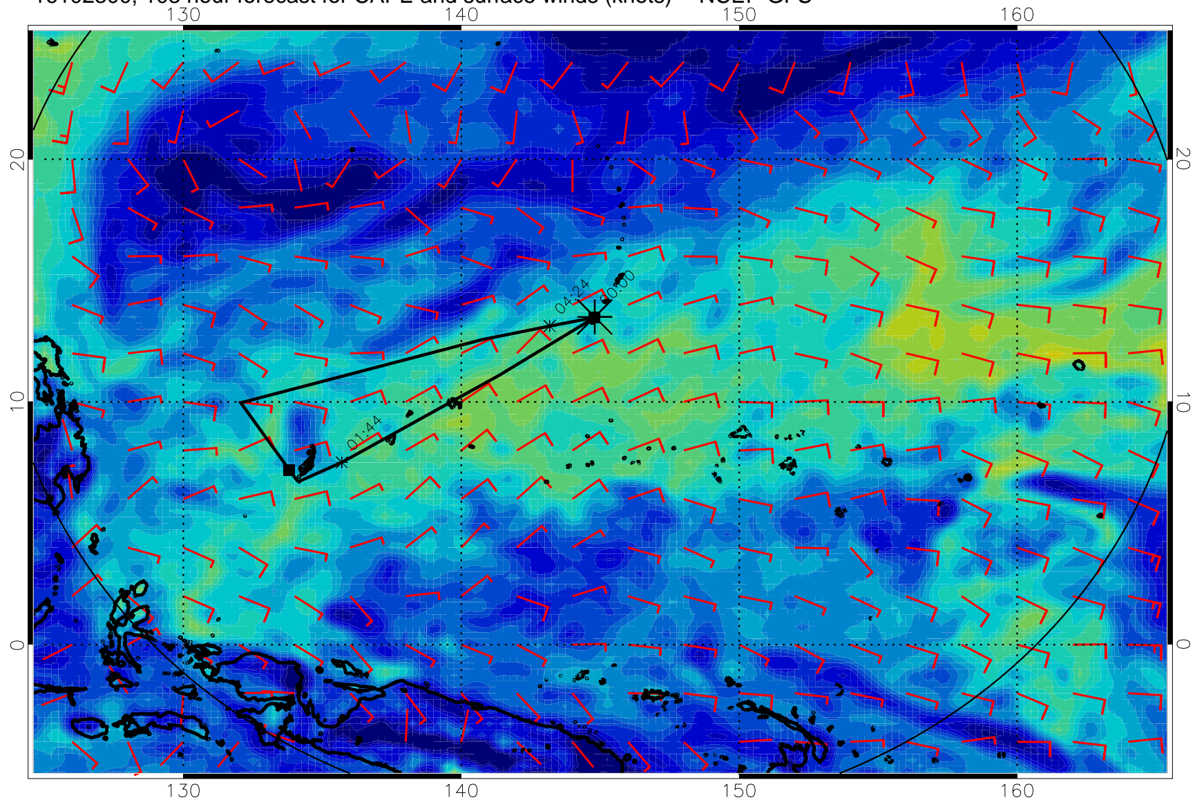
16102300, 108 hour forecast for CAPE and surface winds (knots) -- NCEP GFS
