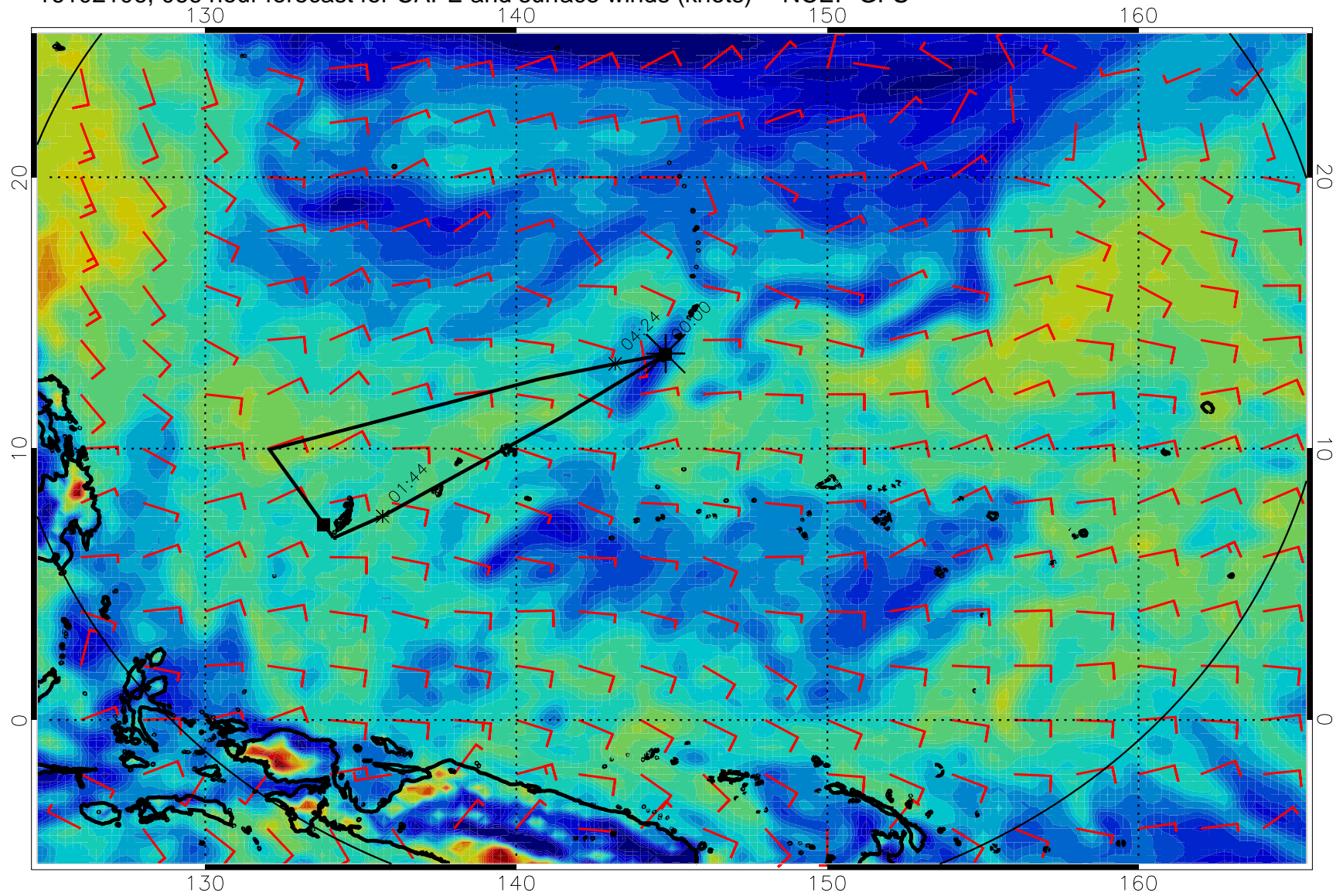
16102106, 066 hour forecast for CAPE and surface winds (knots) -- NCEP GFS
