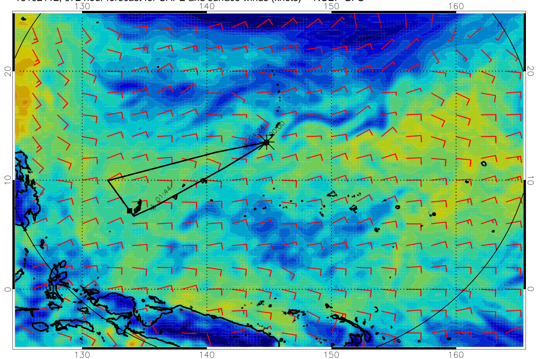
16102112, 072 hour forecast for CAPE and surface winds (knots) -- NCEP GFS
