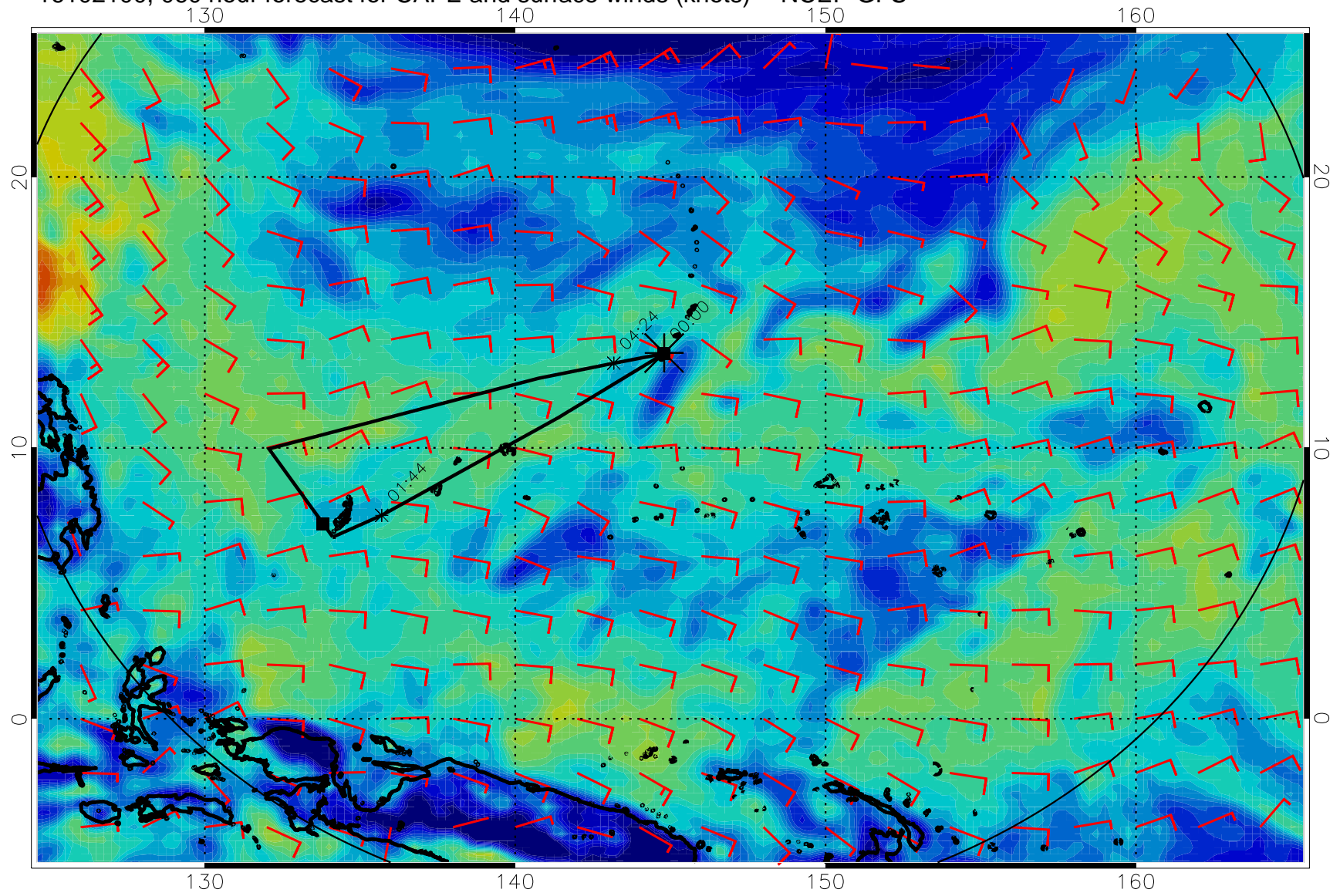
16102100, 060 hour forecast for CAPE and surface winds (knots) -- NCEP GFS
