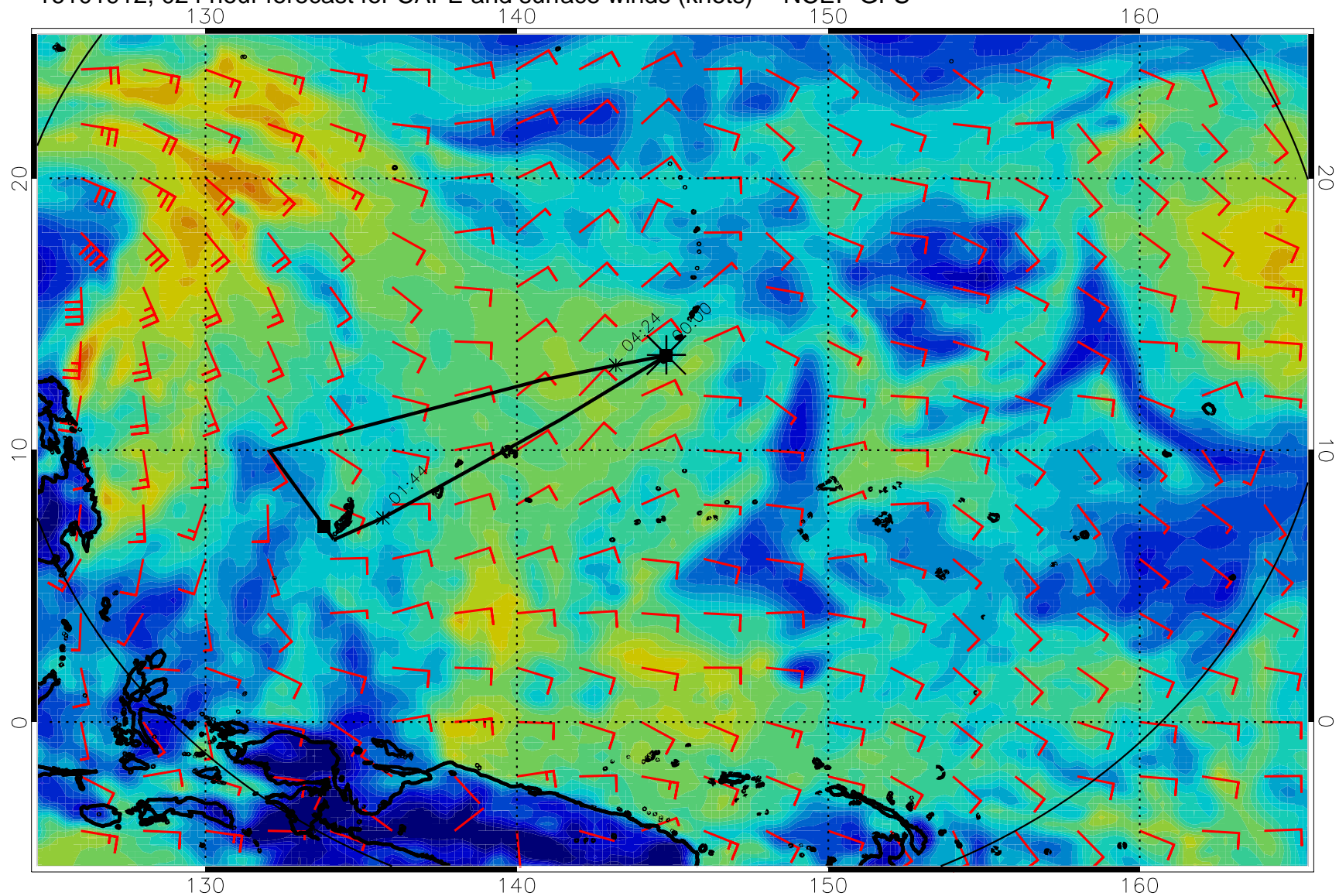
16101912, 024 hour forecast for CAPE and surface winds (knots) -- NCEP GFS
