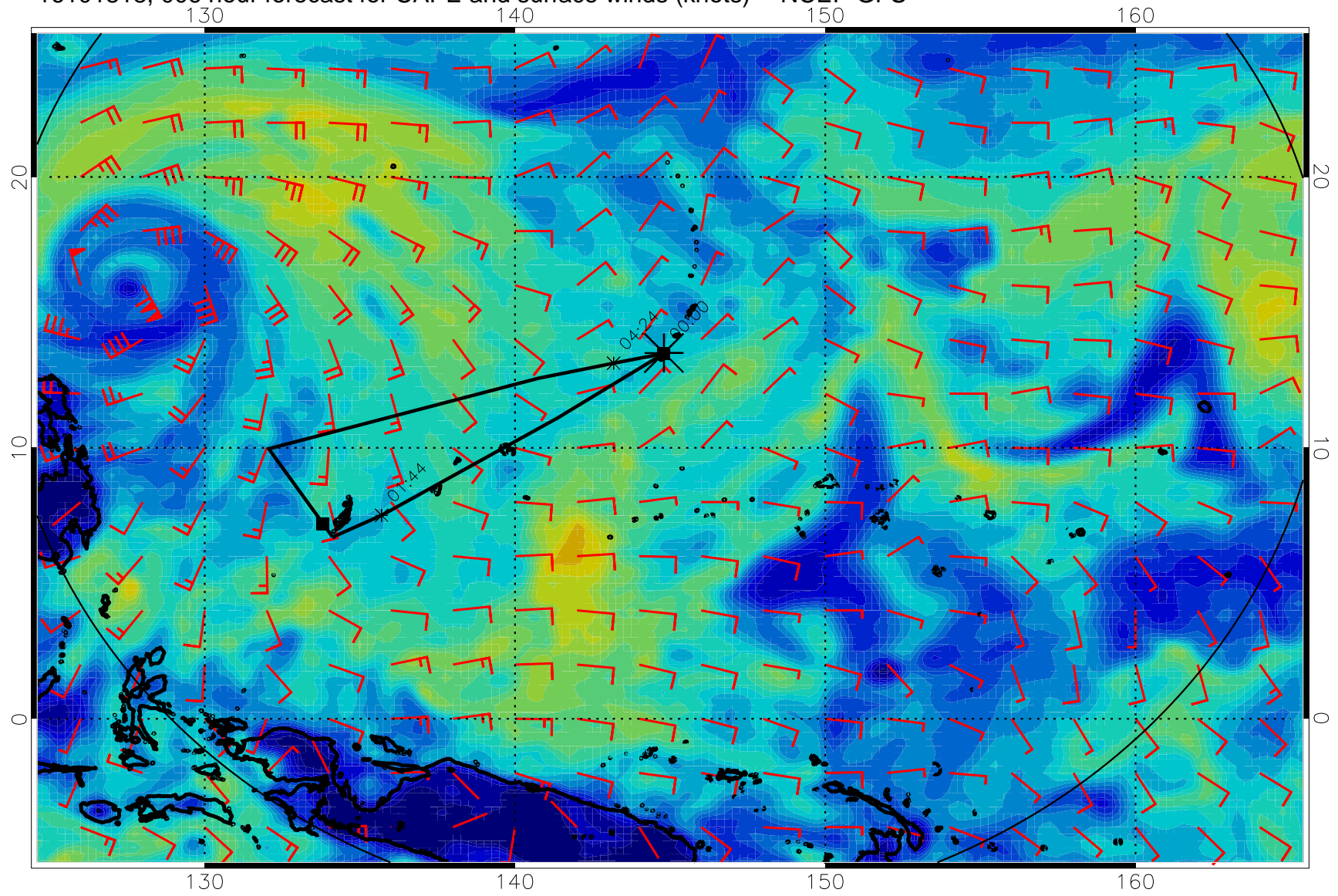
16101818, 006 hour forecast for CAPE and surface winds (knots) -- NCEP GFS
