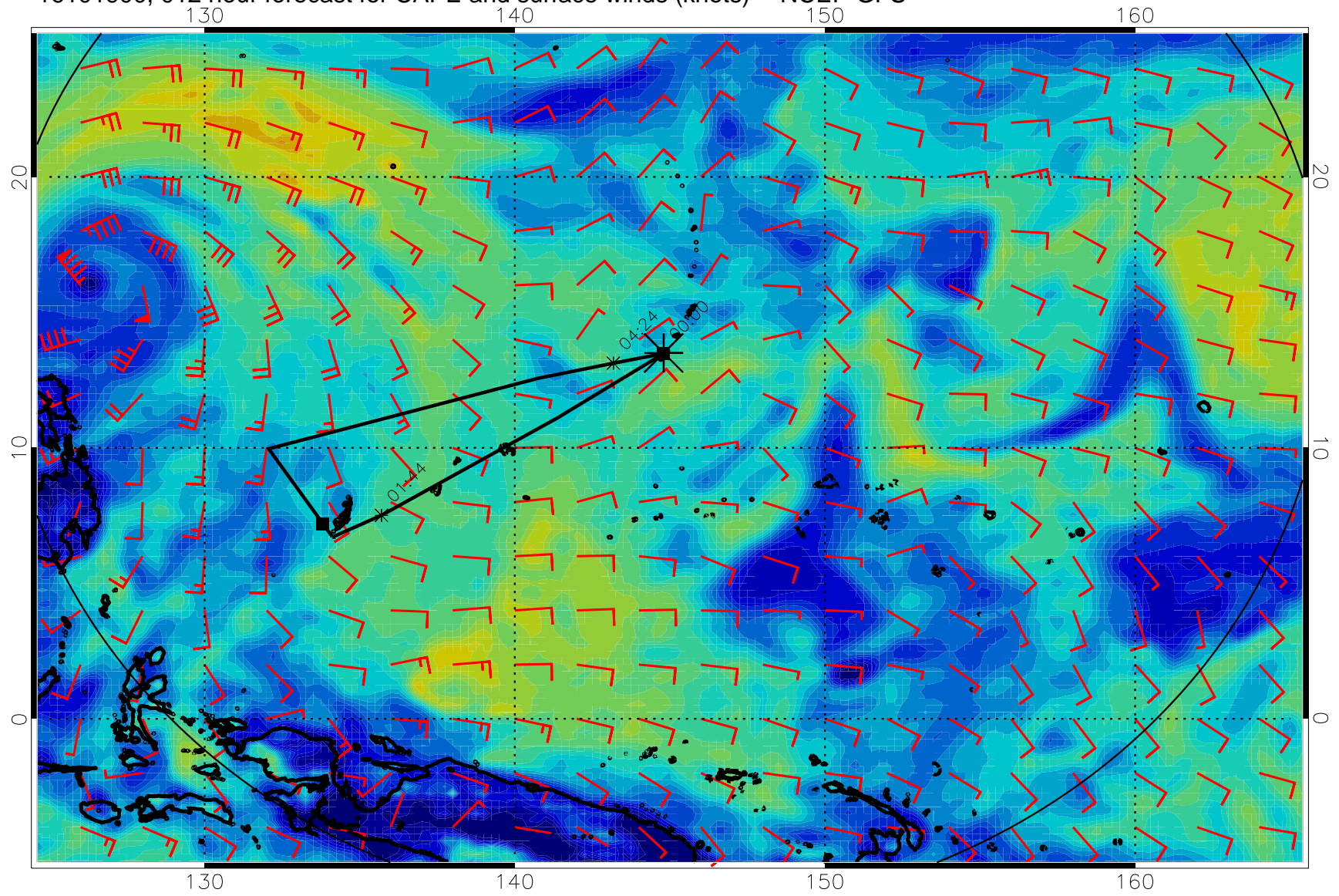
16101900, 012 hour forecast for CAPE and surface winds (knots) -- NCEP GFS
