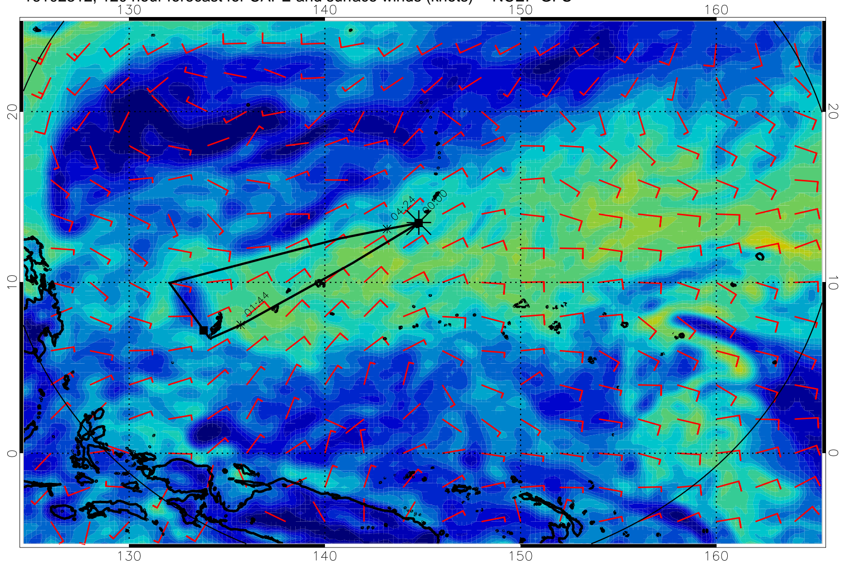
16102312, 120 hour forecast for CAPE and surface winds (knots) -- NCEP GFS
