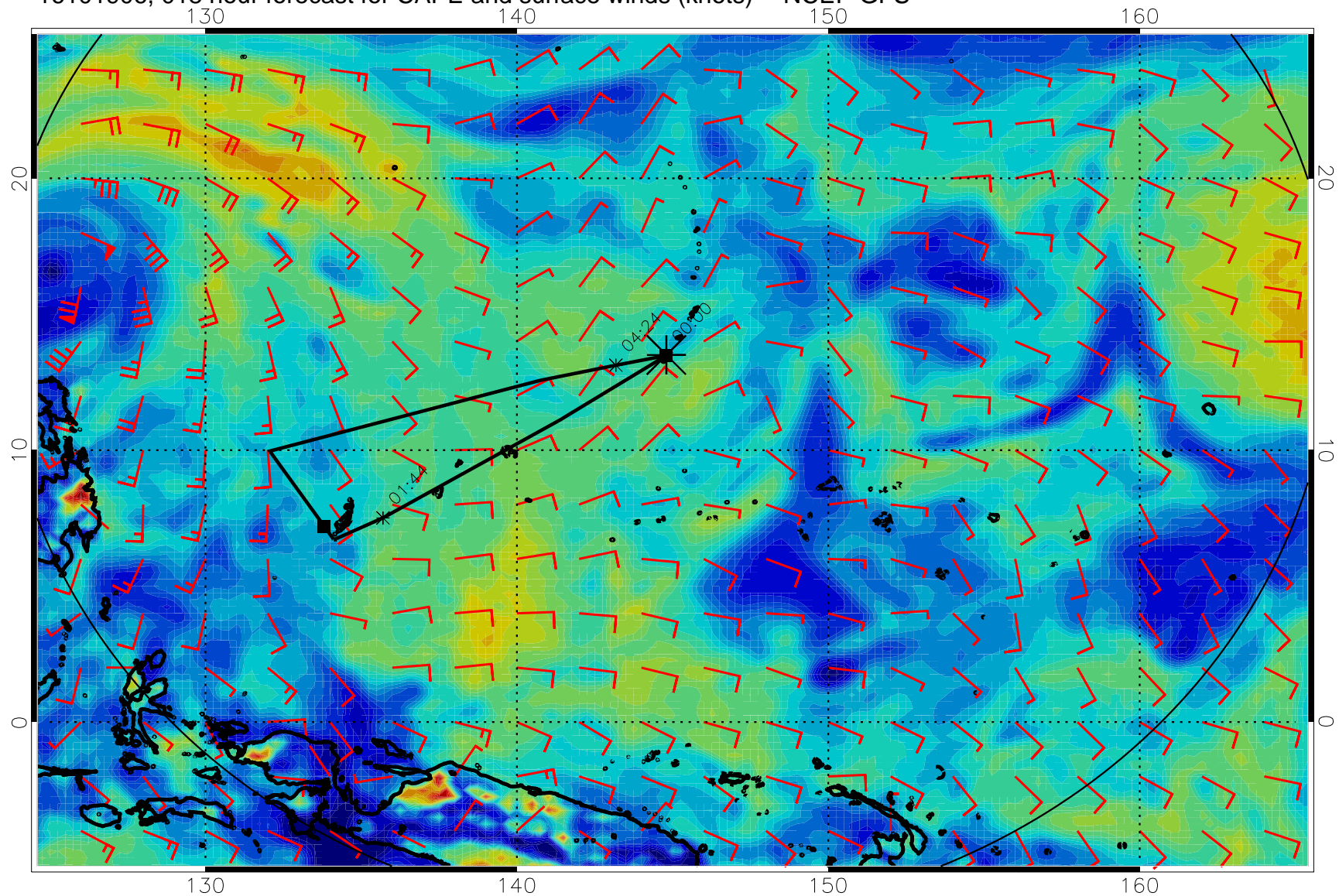
16101906, 018 hour forecast for CAPE and surface winds (knots) -- NCEP GFS
