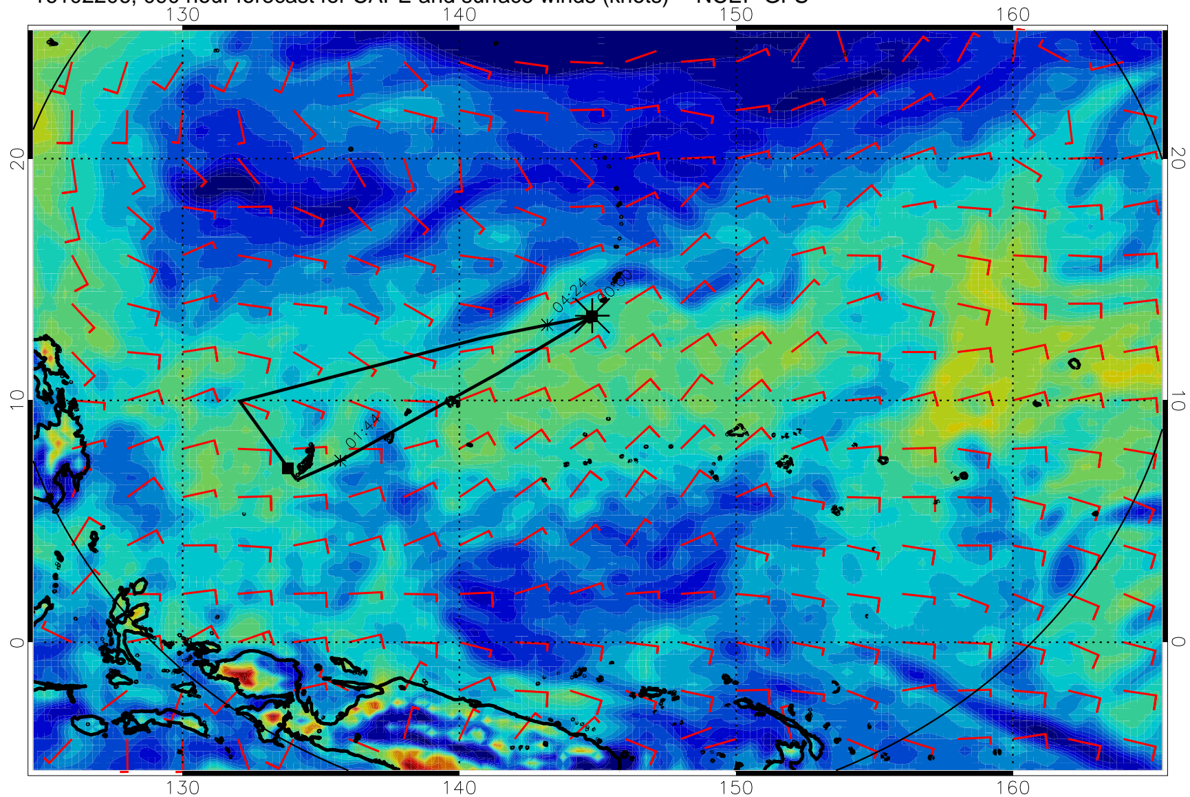
16102206, 090 hour forecast for CAPE and surface winds (knots) -- NCEP GFS
