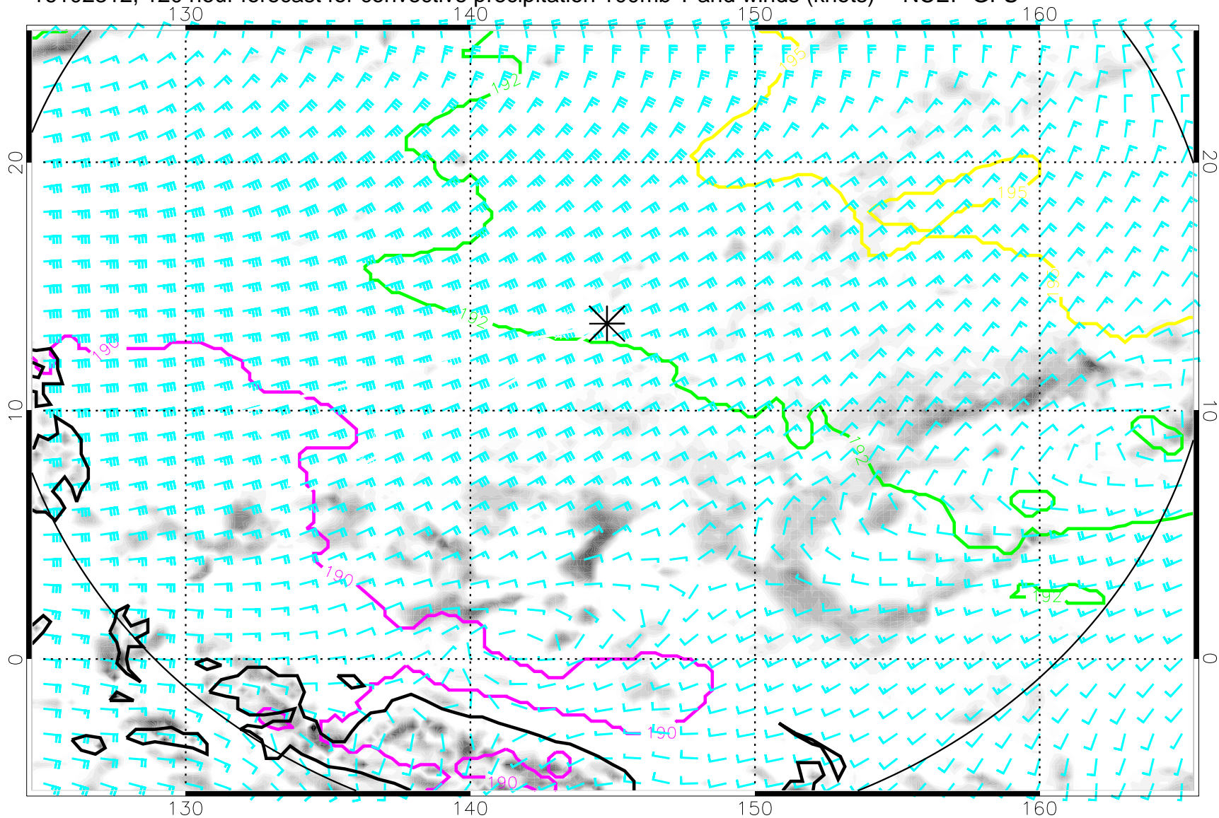
16102312, 120 hour forecast for convective precipitation 100mb T and winds (knots) -- NCEP GFS
