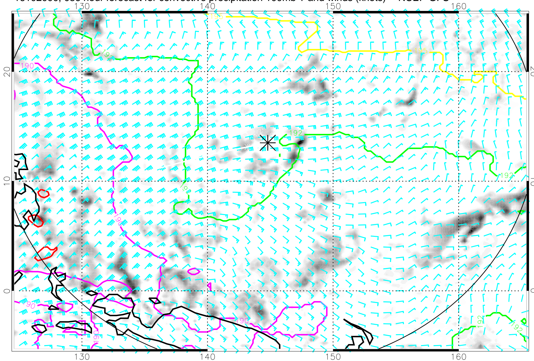
16102000, 036 hour forecast for convective precipitation 100mb T and winds (knots) -- NCEP GFS
