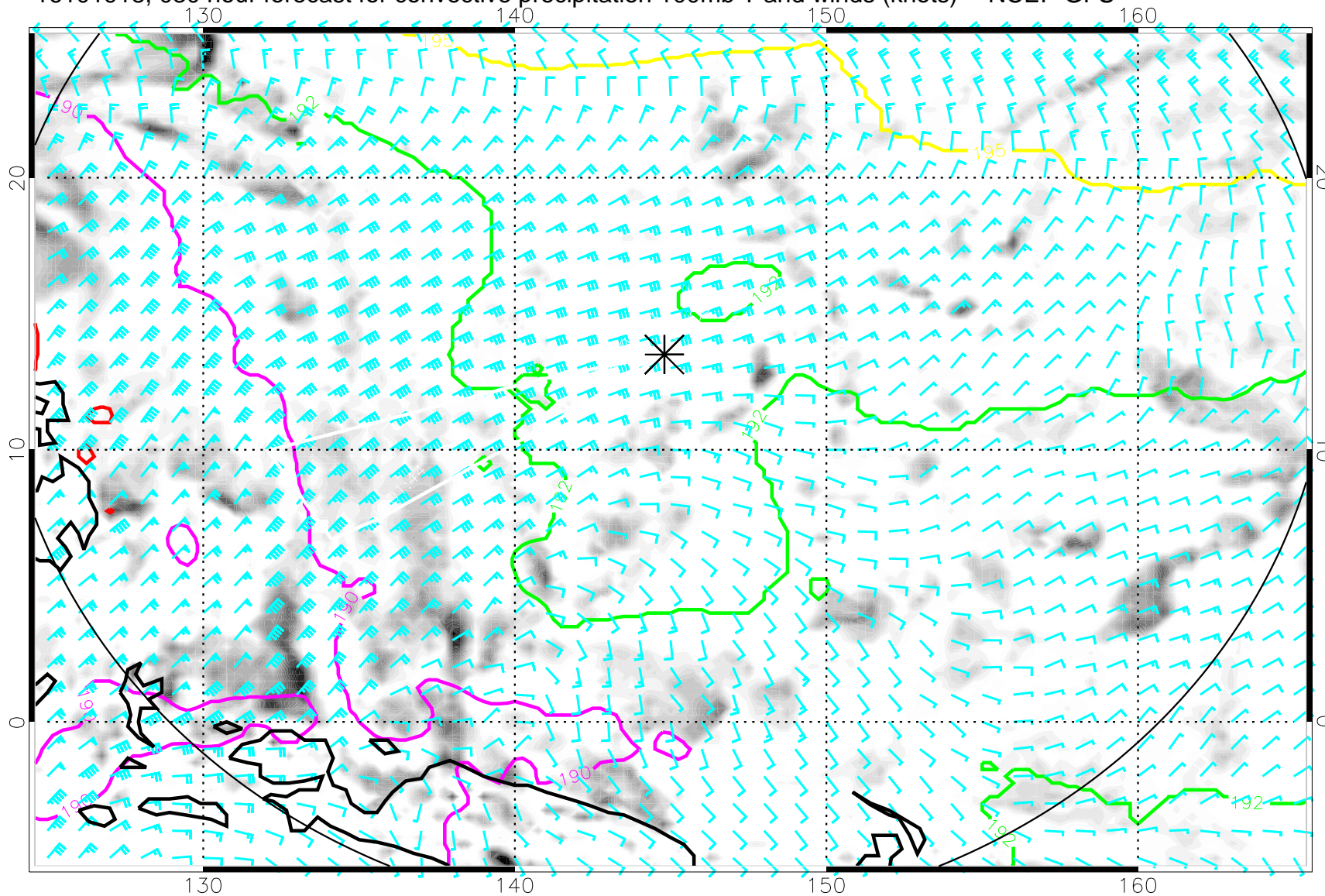
16101918, 030 hour forecast for convective precipitation 100mb T and winds (knots) -- NCEP GFS
