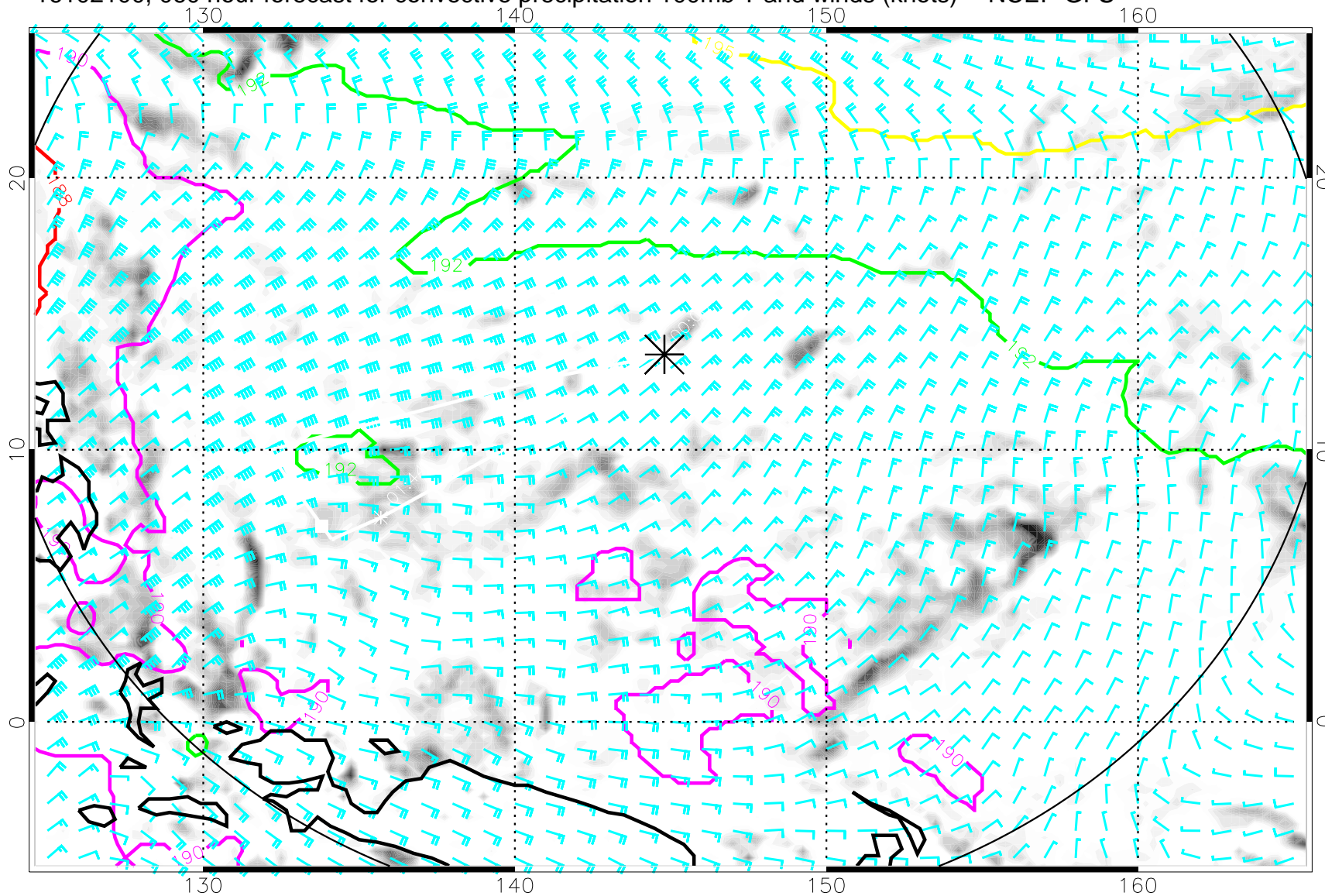
16102100, 060 hour forecast for convective precipitation 100mb T and winds (knots) -- NCEP GFS
