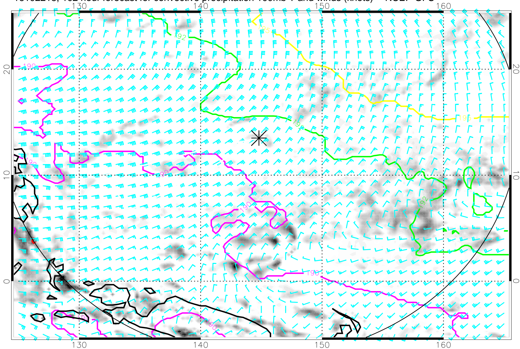
16102218, 102 hour forecast for convective precipitation 100mb T and winds (knots) -- NCEP GFS
