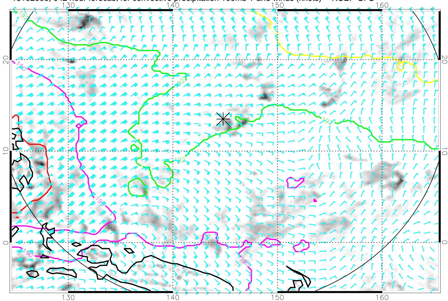
16102006, 04Z hour forecast for convective precipitation 100mb T and winds (knots) -- NCEP GFS
