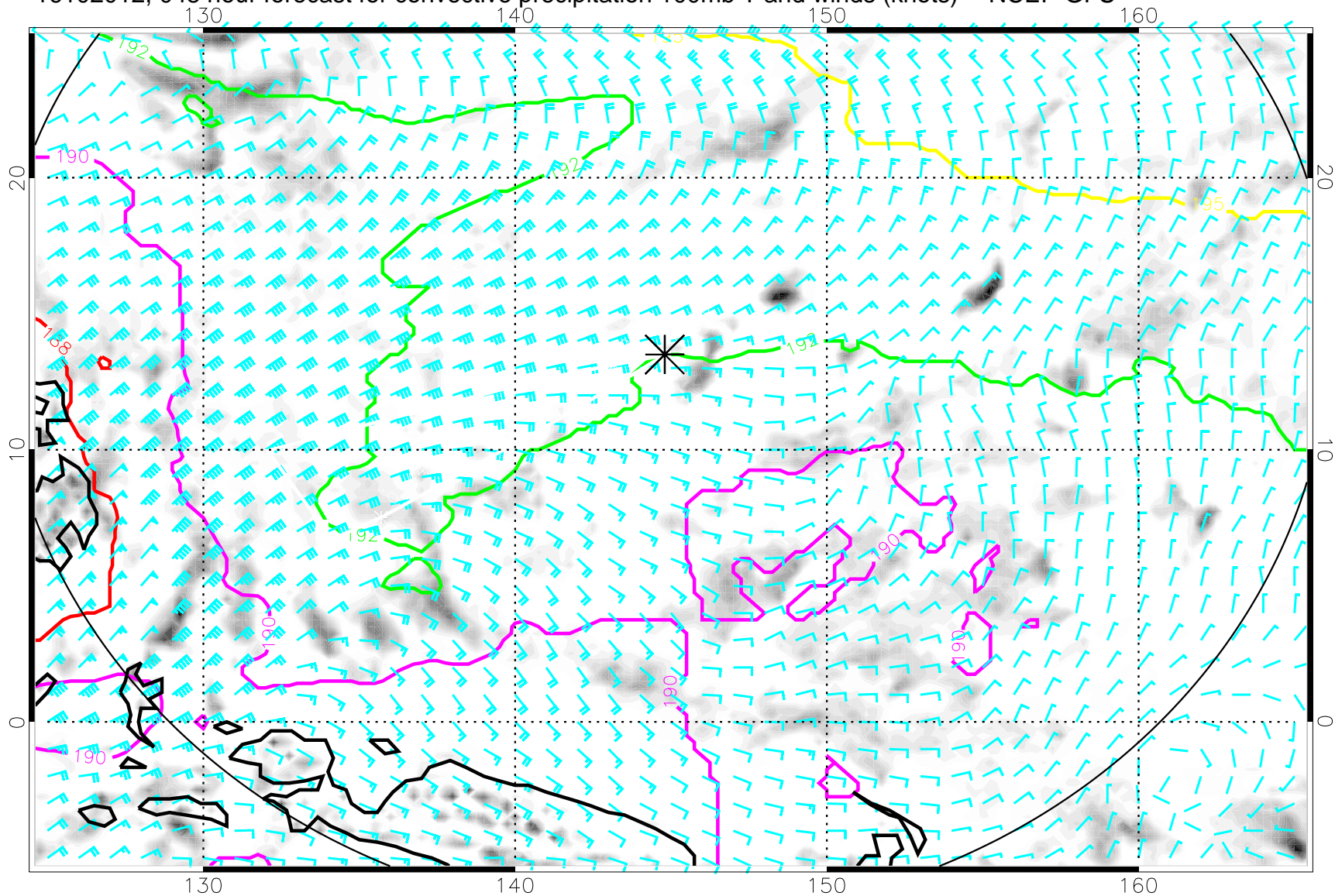
16102012, 048 hour forecast for convective precipitation 100mb T and winds (knots) -- NCEP GFS
