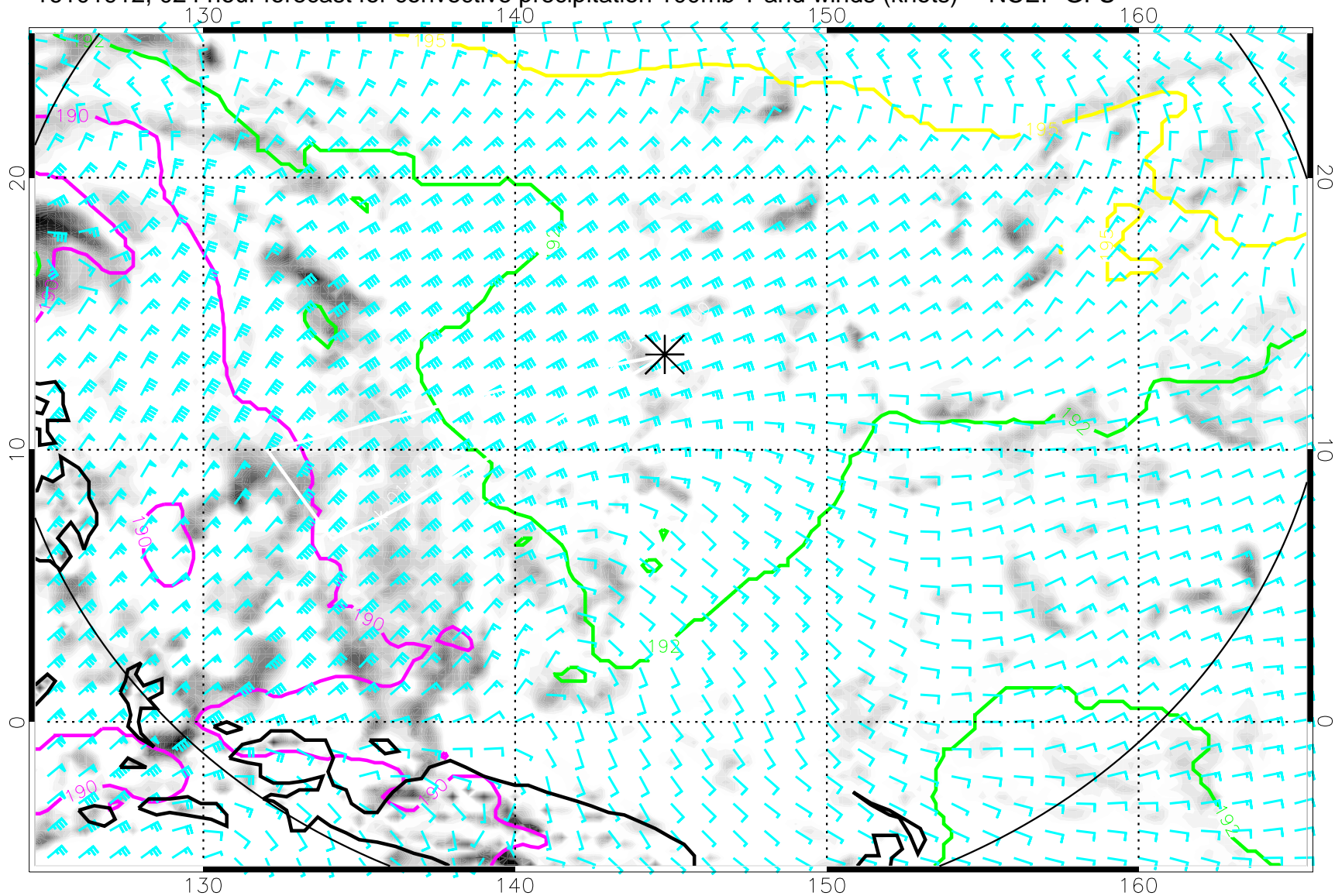
16101912, 024 hour forecast for convective precipitation 100mb T and winds (knots) -- NCEP GFS
