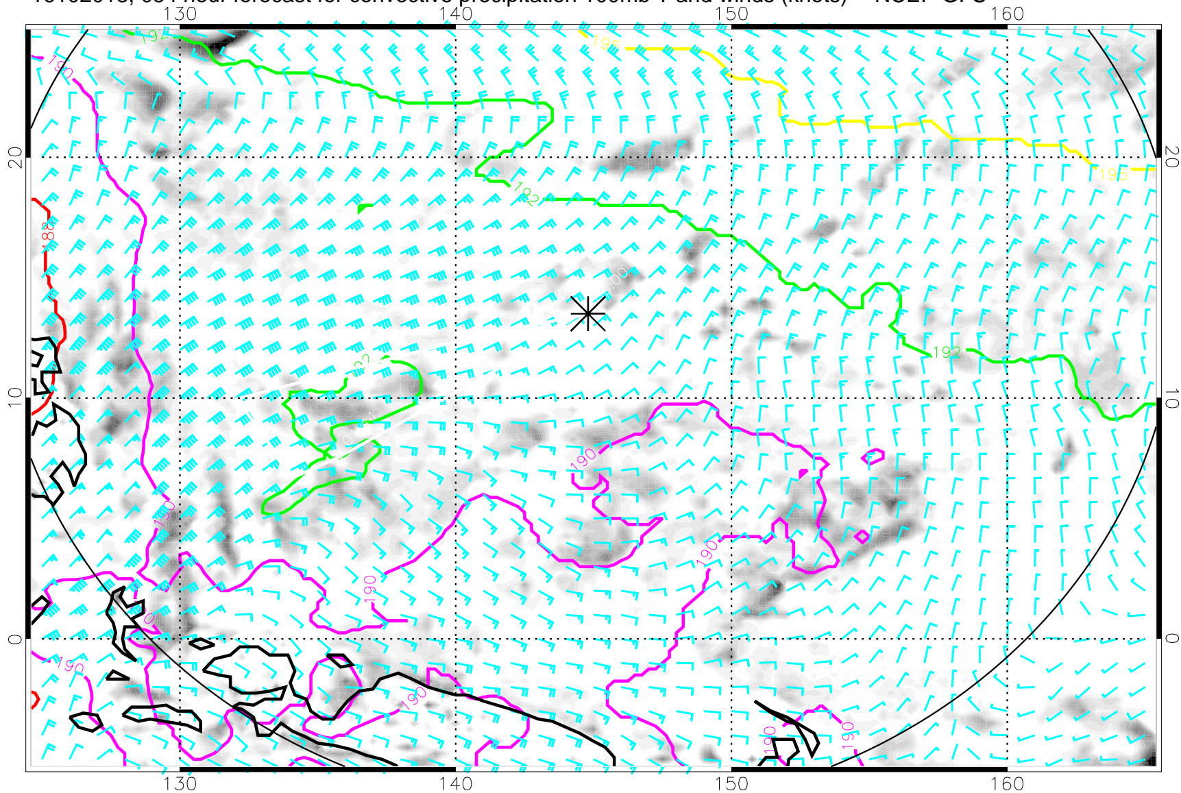
16102018, 054 hour forecast for convective precipitation 100mb T and winds (knots) -- NCEP GFS
