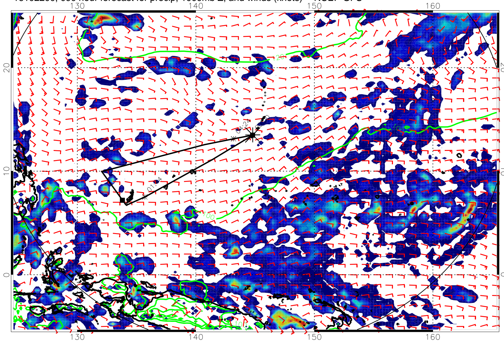
16102200, 090 hour forecast for precip, 1000mb Z, and winds (knots) -- NCEP GFS
