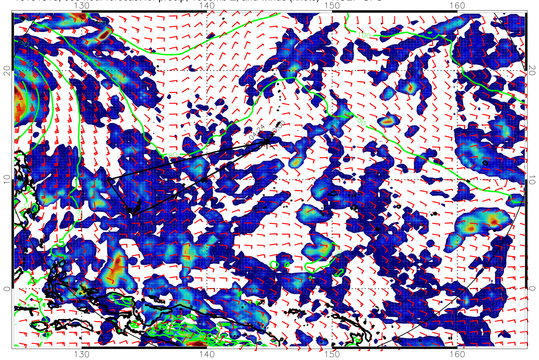
16101918, 036 hour forecast for precip, 1000mb Z, and winds (knots) -- NCEP GFS
