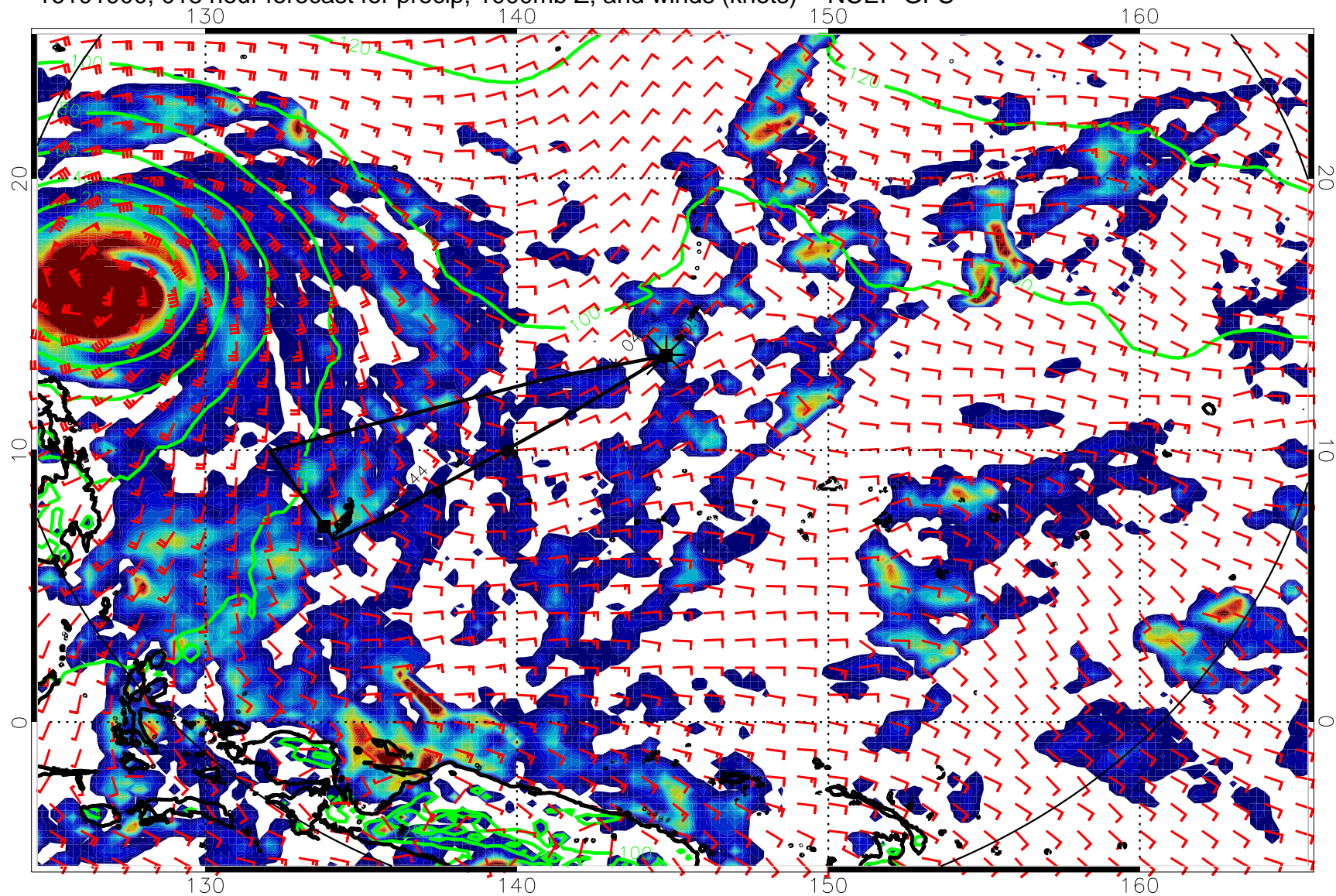
16101900, 018 hour forecast for precip, 1000mb Z, and winds (knots) -- NCEP GFS
