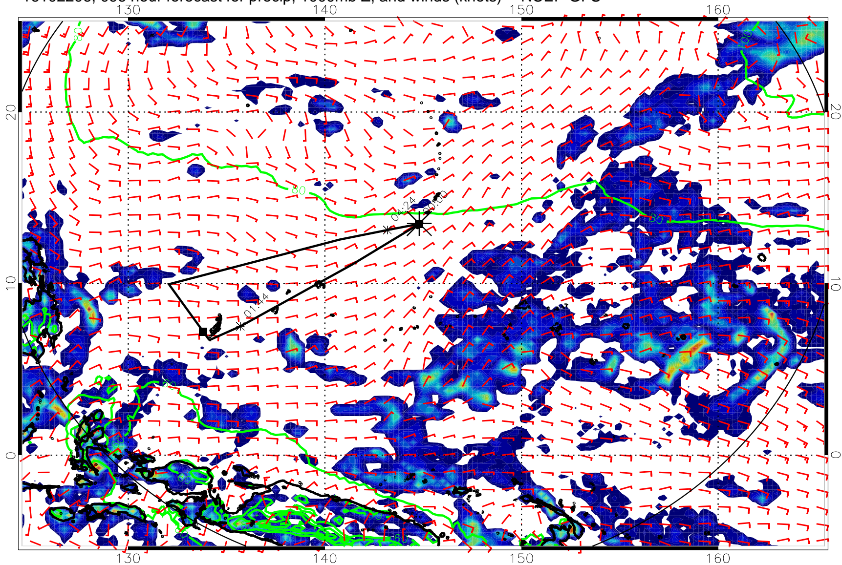
16102206, 096 hour forecast for precip, 1000mb Z, and winds (knots) -- NCEP GFS
