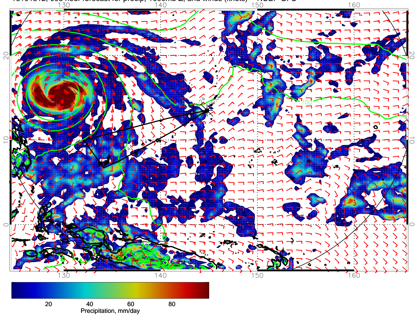
16101812, 006 hour forecast for precip, 1000mb Z, and winds (knots) -- NCEP GFS
