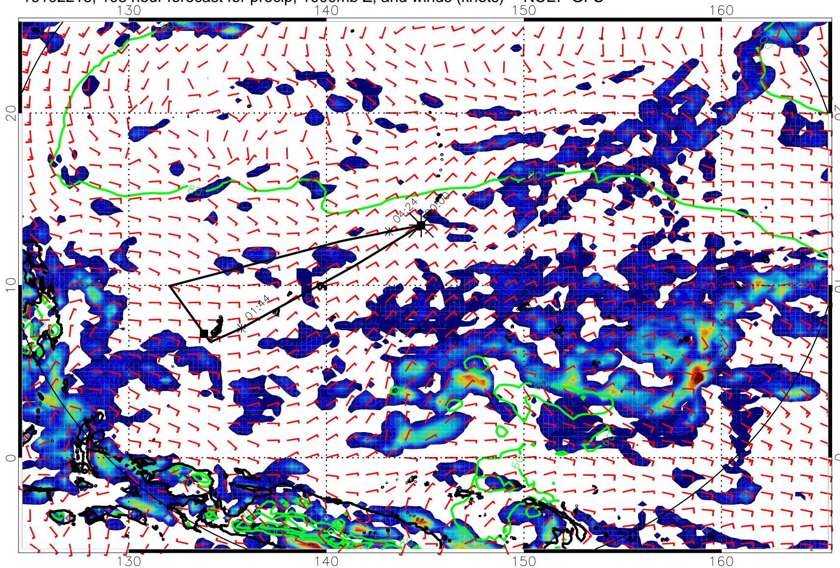
16102218, 108 hour forecast for precip, 1000mb Z, and winds (knots) -- NCEP GFS
