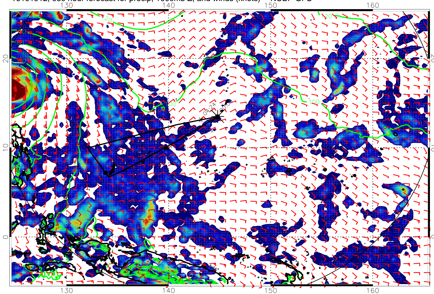
16101912, 030 hour forecast for precip, 1000mb Z, and winds (knots) -- NCEP GFS
