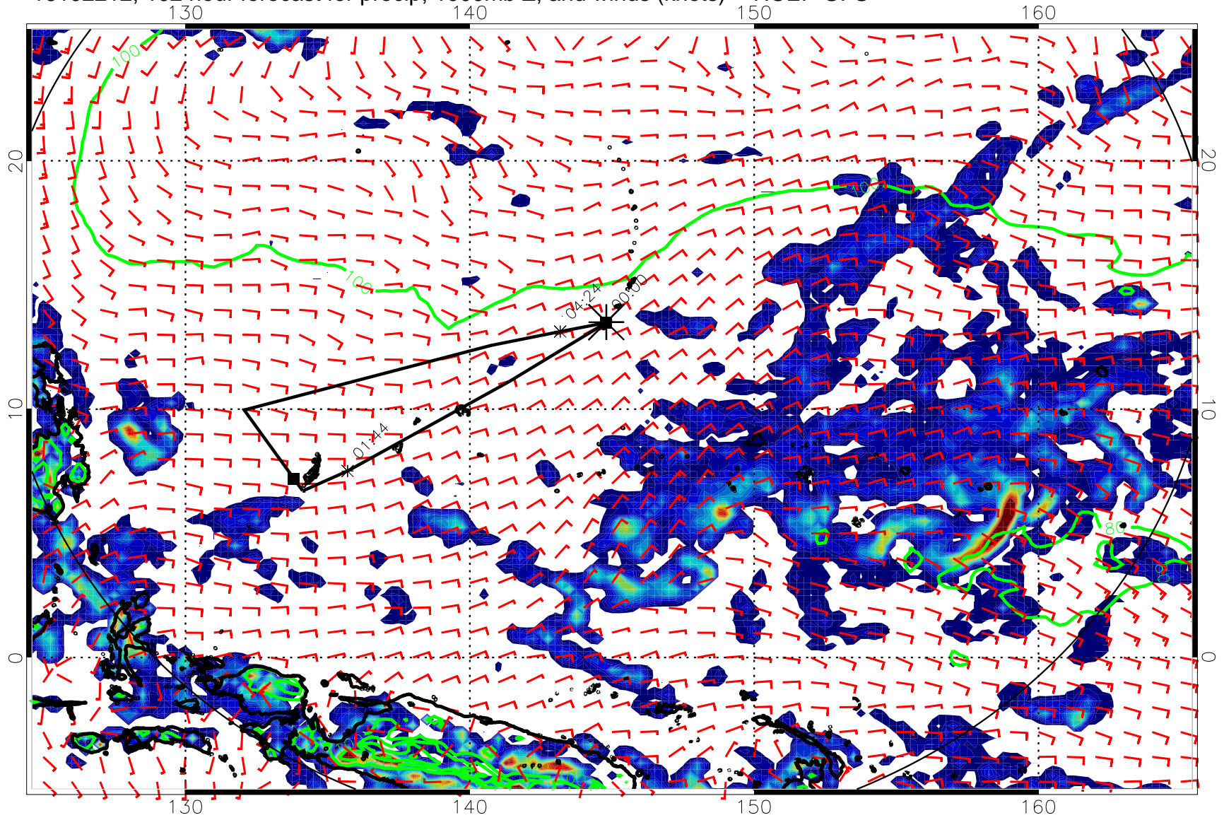
16102212, 102 hour forecast for precip, 1000mb Z, and winds (knots) -- NCEP GFS
