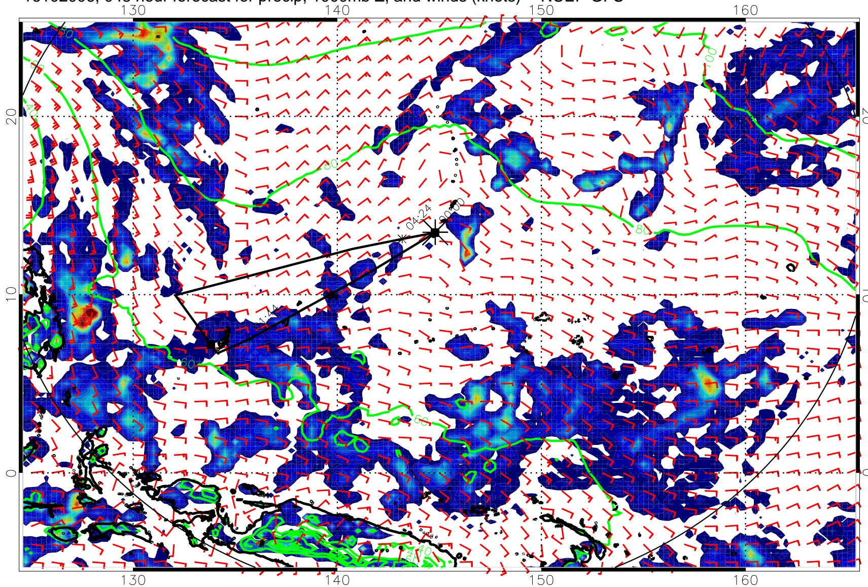
16102006, 048 hour forecast for precip, 1000mb Z, and winds (knots) -- NCEP GFS
