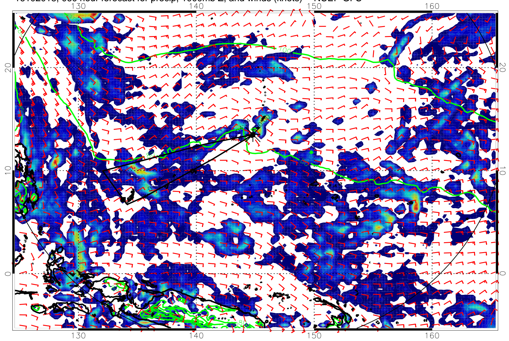
16102018, 060 hour forecast for precip, 1000mb Z, and winds (knots) -- NCEP GFS
