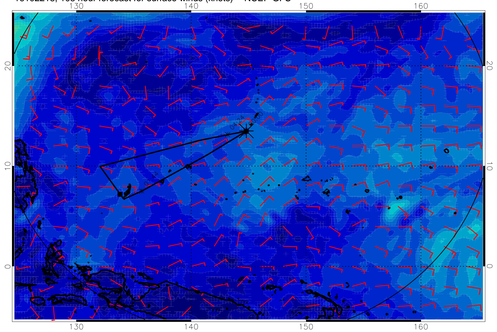
16102218, 108 hour forecast for surface winds (knots) -- NCEP GFS
