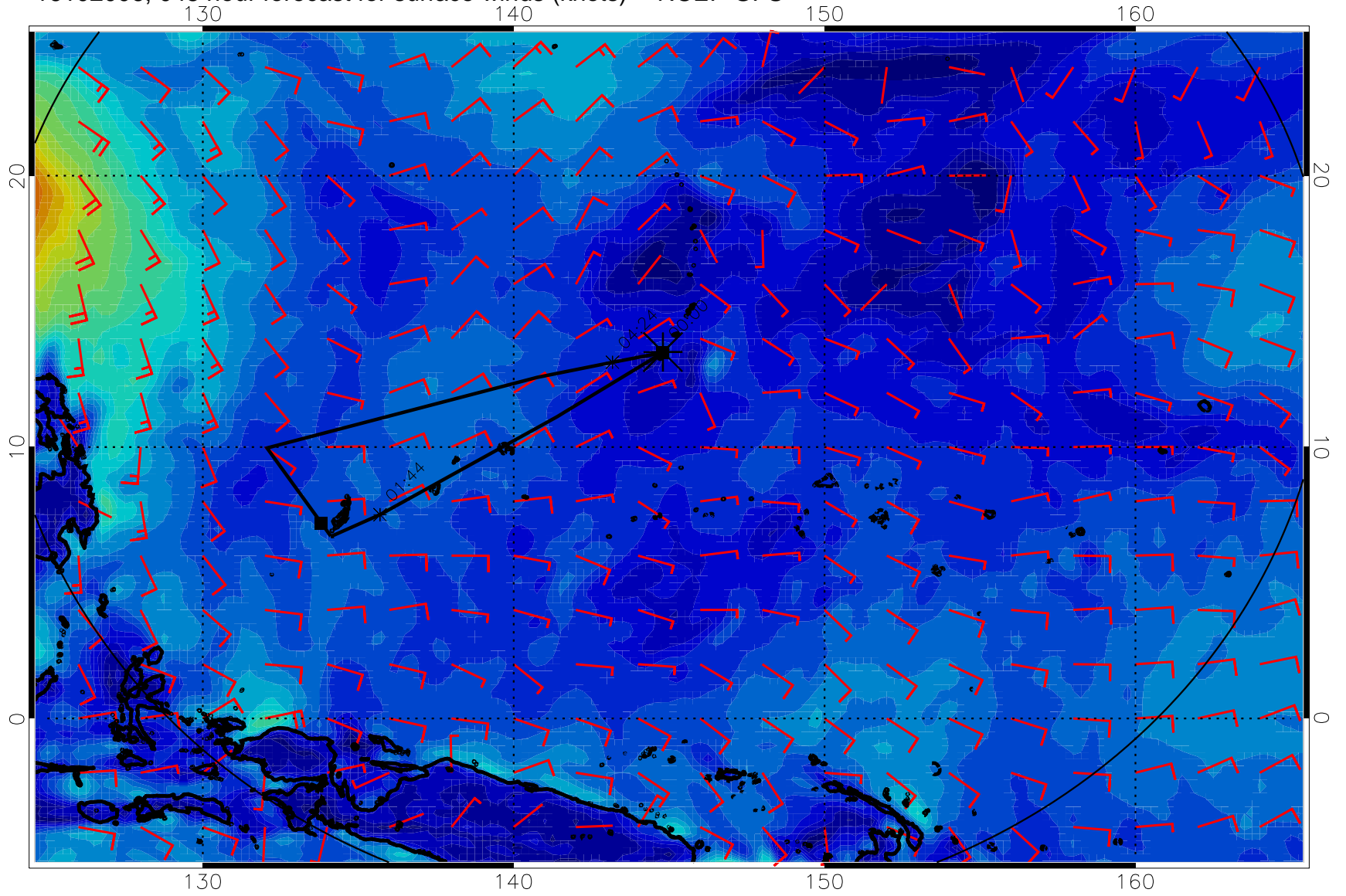
16102006, 048 hour forecast for surface winds (knots) -- NCEP GFS
