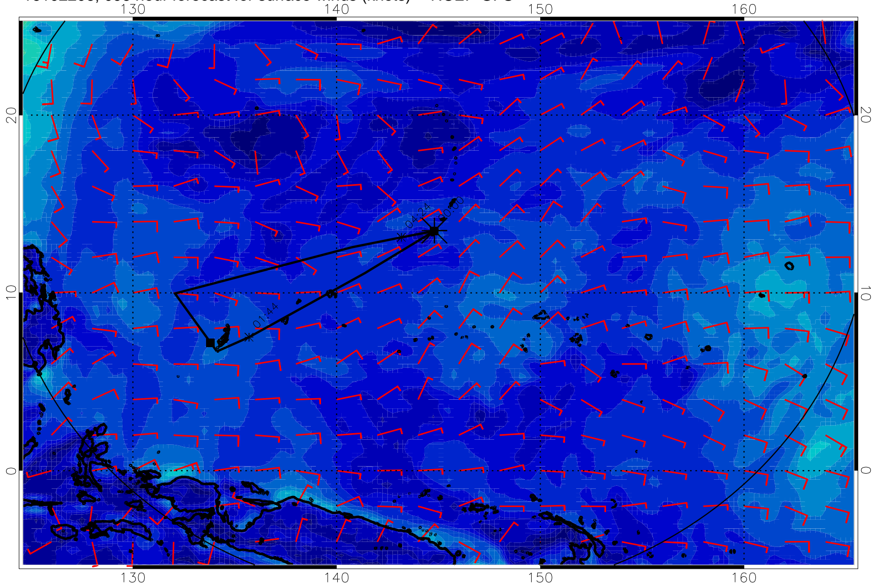
16102206, 096 hour forecast for surface winds (knots) -- NCEP GFS
