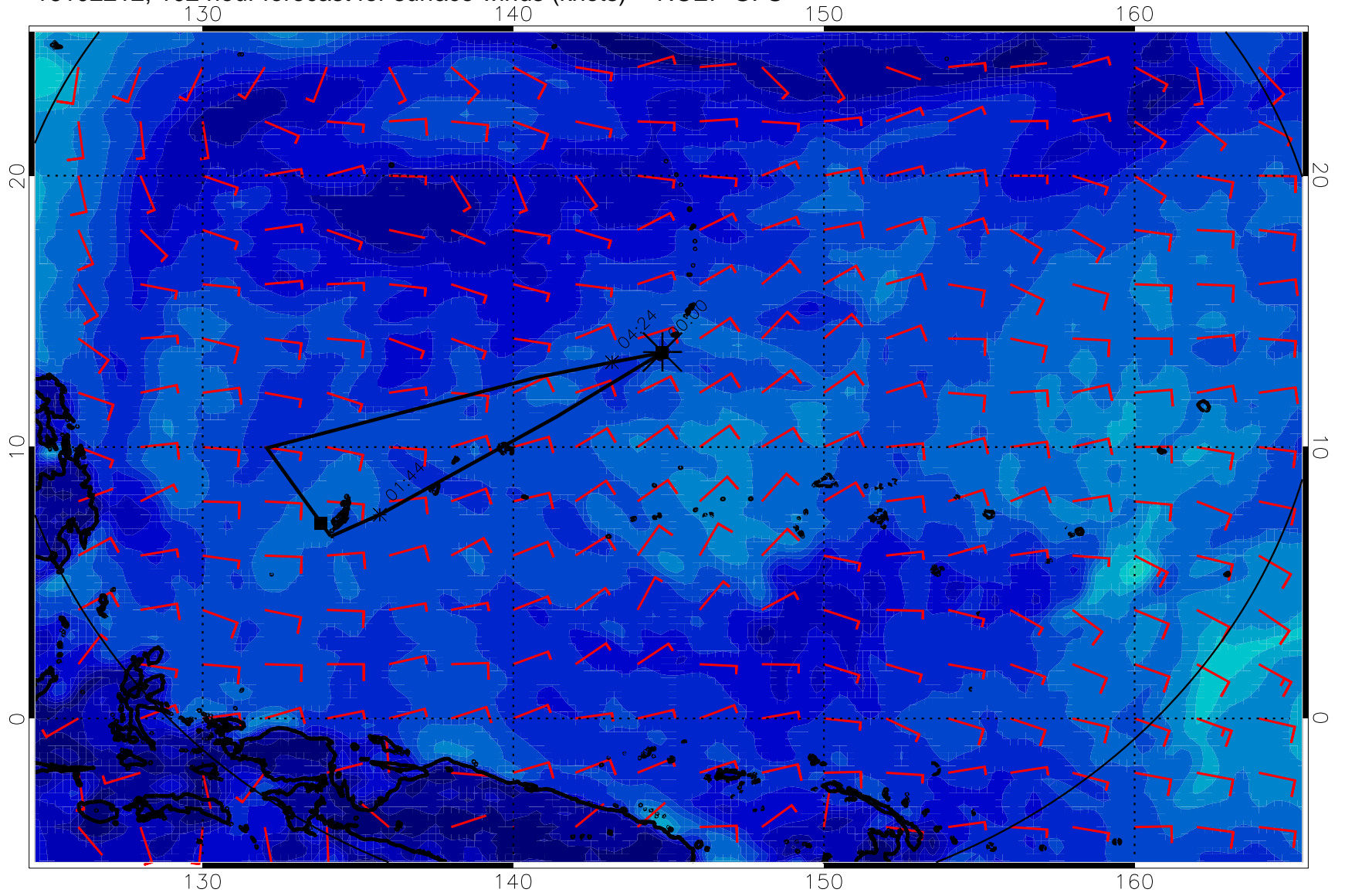
16102212, 102 hour forecast for surface winds (knots) -- NCEP GFS
