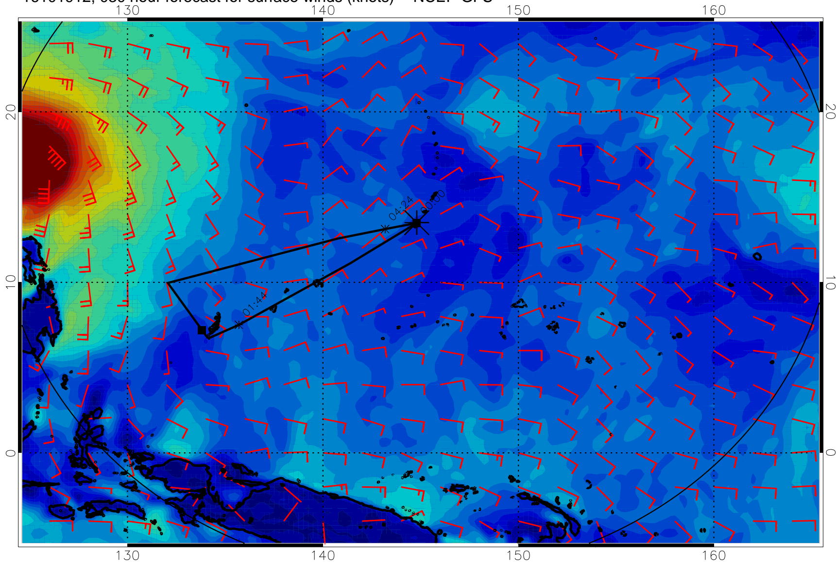
16101912, 030 hour forecast for surface winds (knots) -- NCEP GFS
