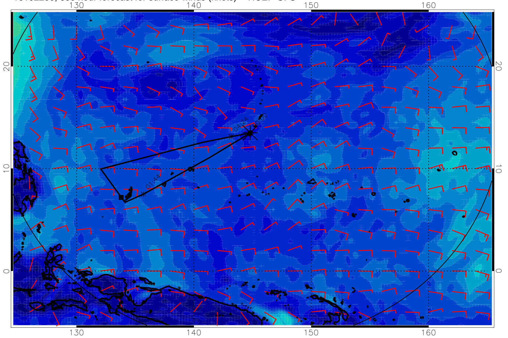
16102200, 090 hour forecast for surface winds (knots) -- NCEP GFS
