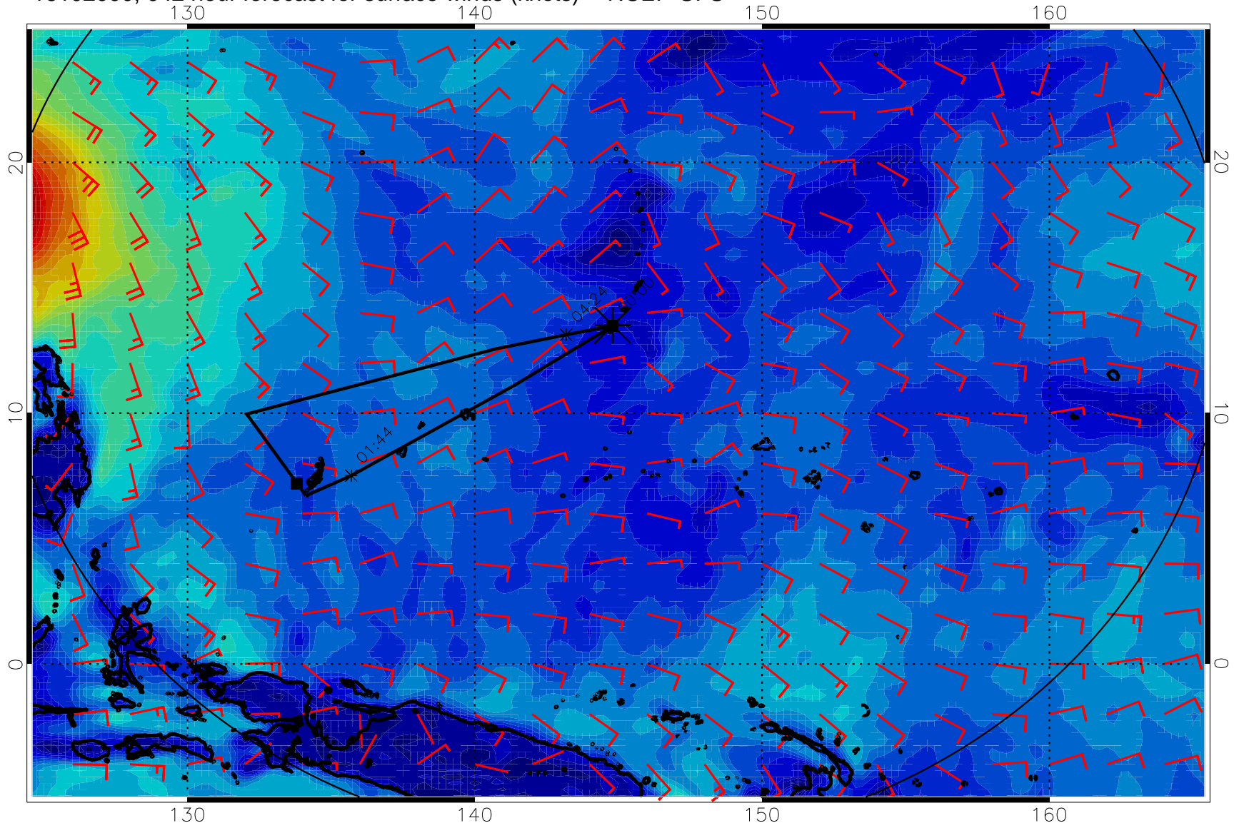
16102000, 042 hour forecast for surface winds (knots) -- NCEP GFS
