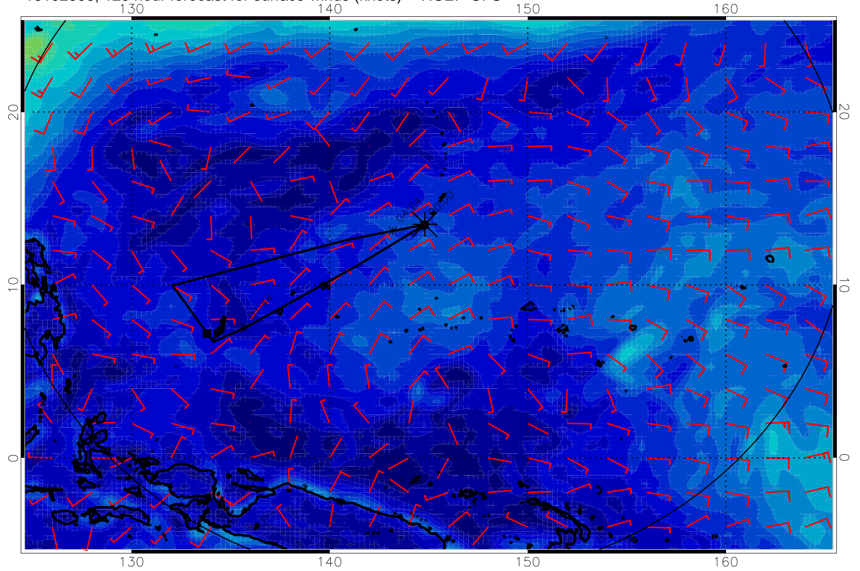
16102306, 120 hour forecast for surface winds (knots) -- NCEP GFS
