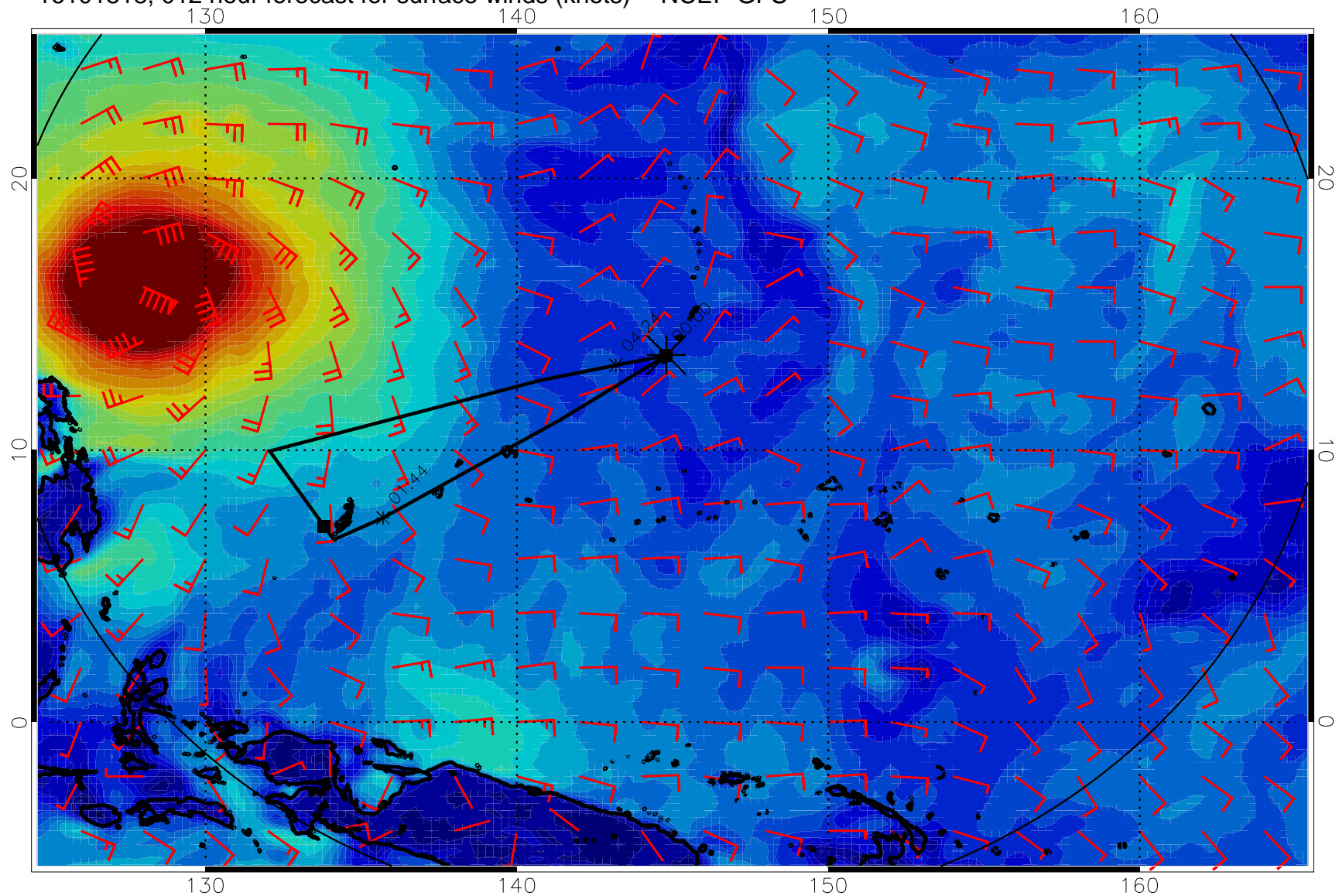
16101818, 012 hour forecast for surface winds (knots) -- NCEP GFS
