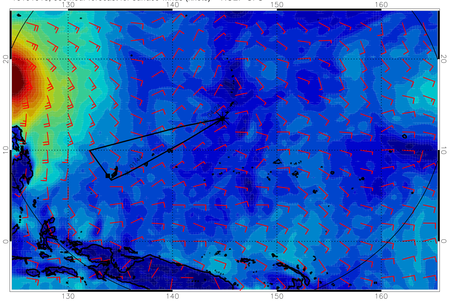
16101918, 036 hour forecast for surface winds (knots) -- NCEP GFS
