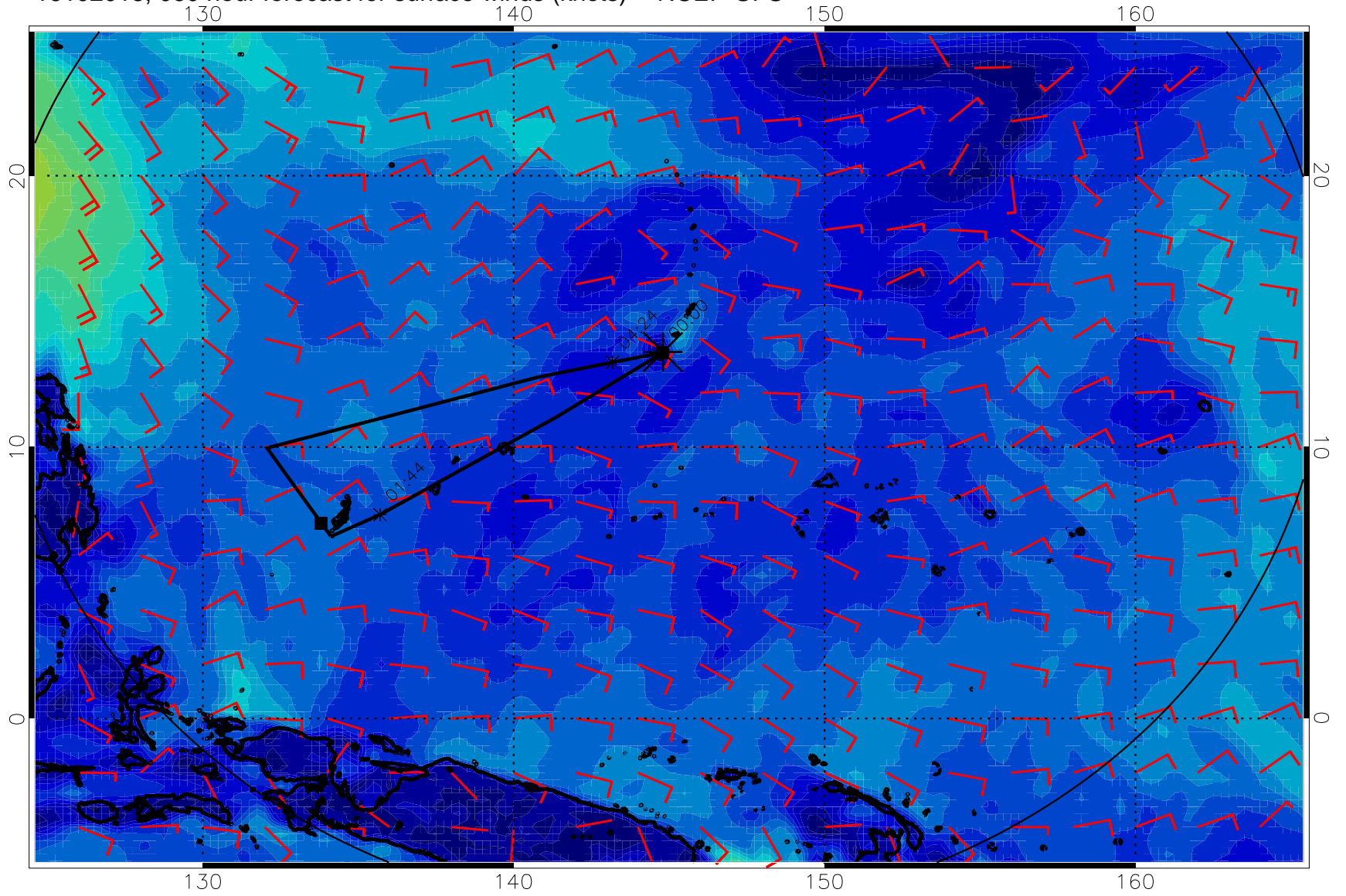
16102018, 060 hour forecast for surface winds (knots) -- NCEP GFS
