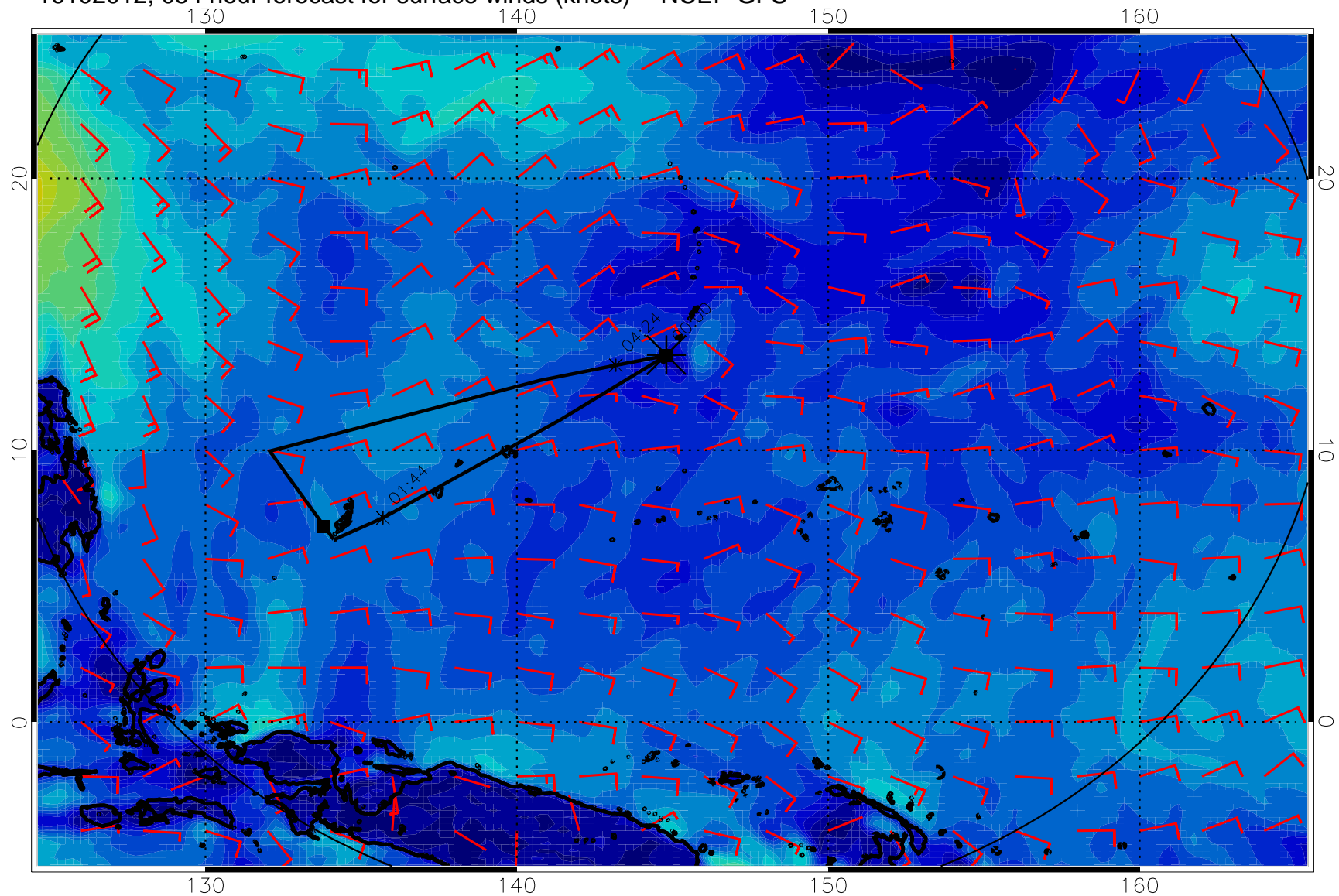
16102012, 054 hour forecast for surface winds (knots) -- NCEP GFS
