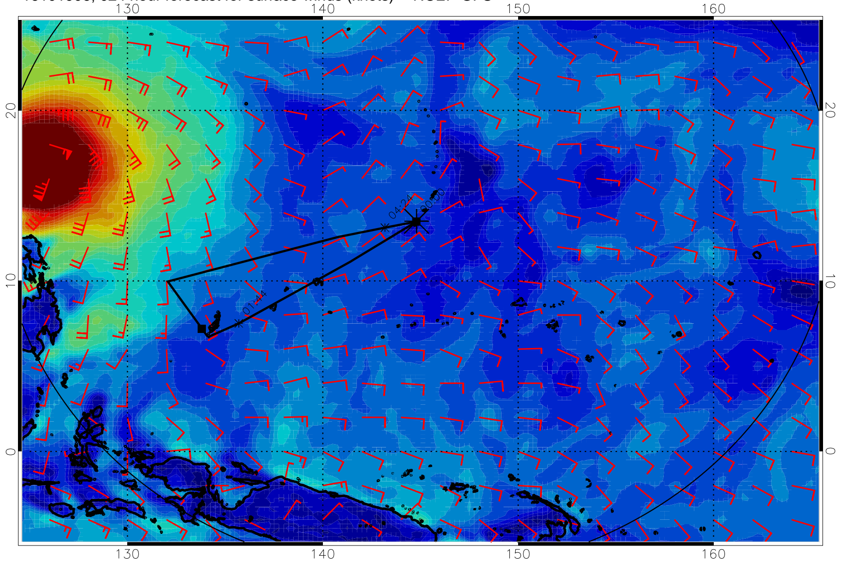
16101906, 024 hour forecast for surface winds (knots) -- NCEP GFS
