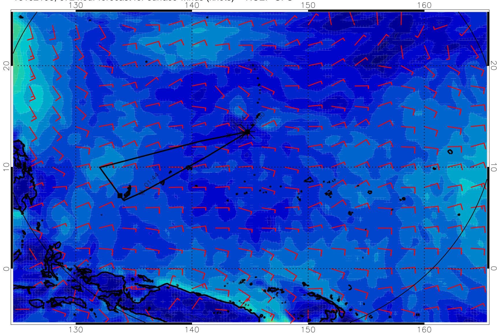
16102106, 072 hour forecast for surface winds (knots) -- NCEP GFS
