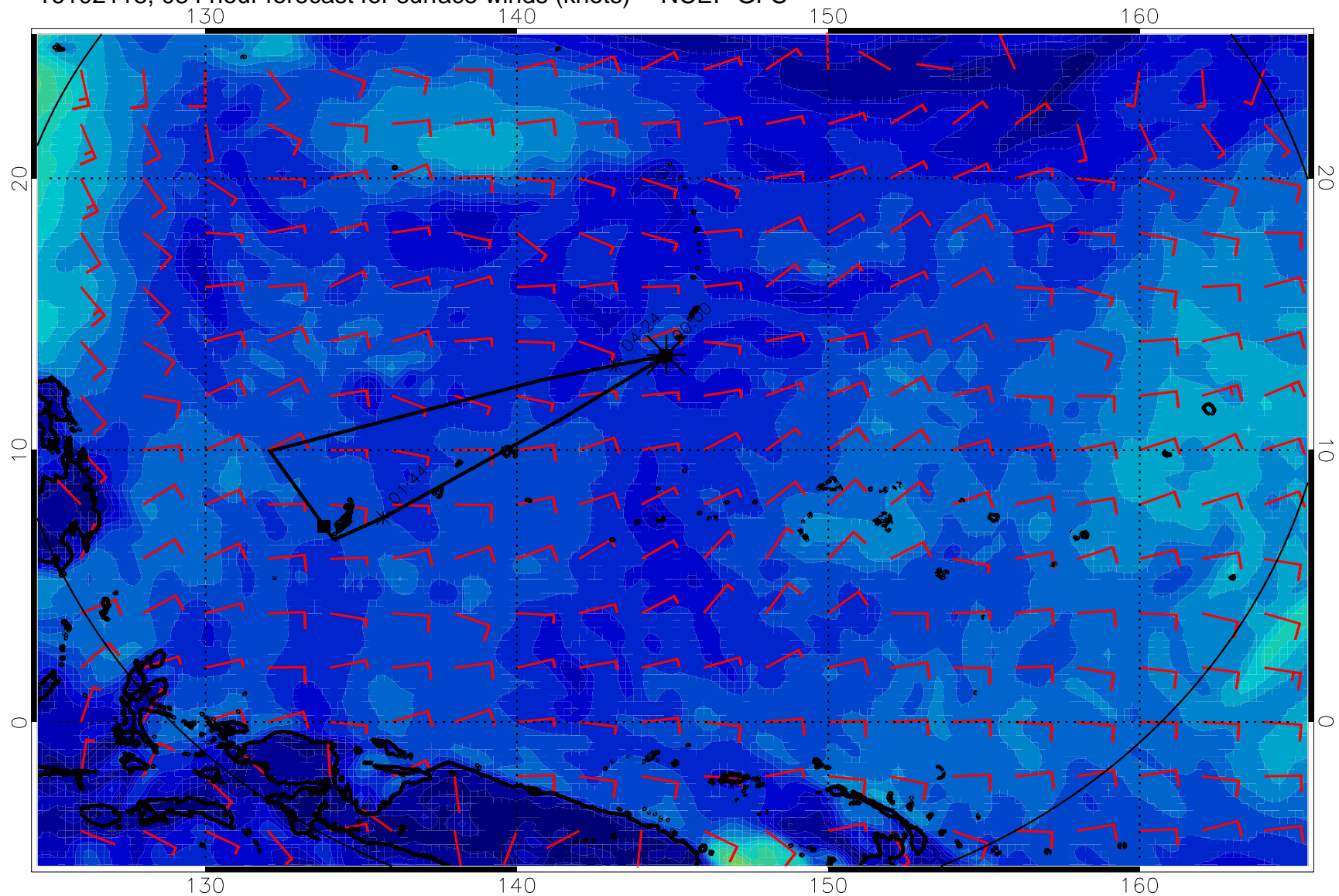
16102118, 084 hour forecast for surface winds (knots) -- NCEP GFS
