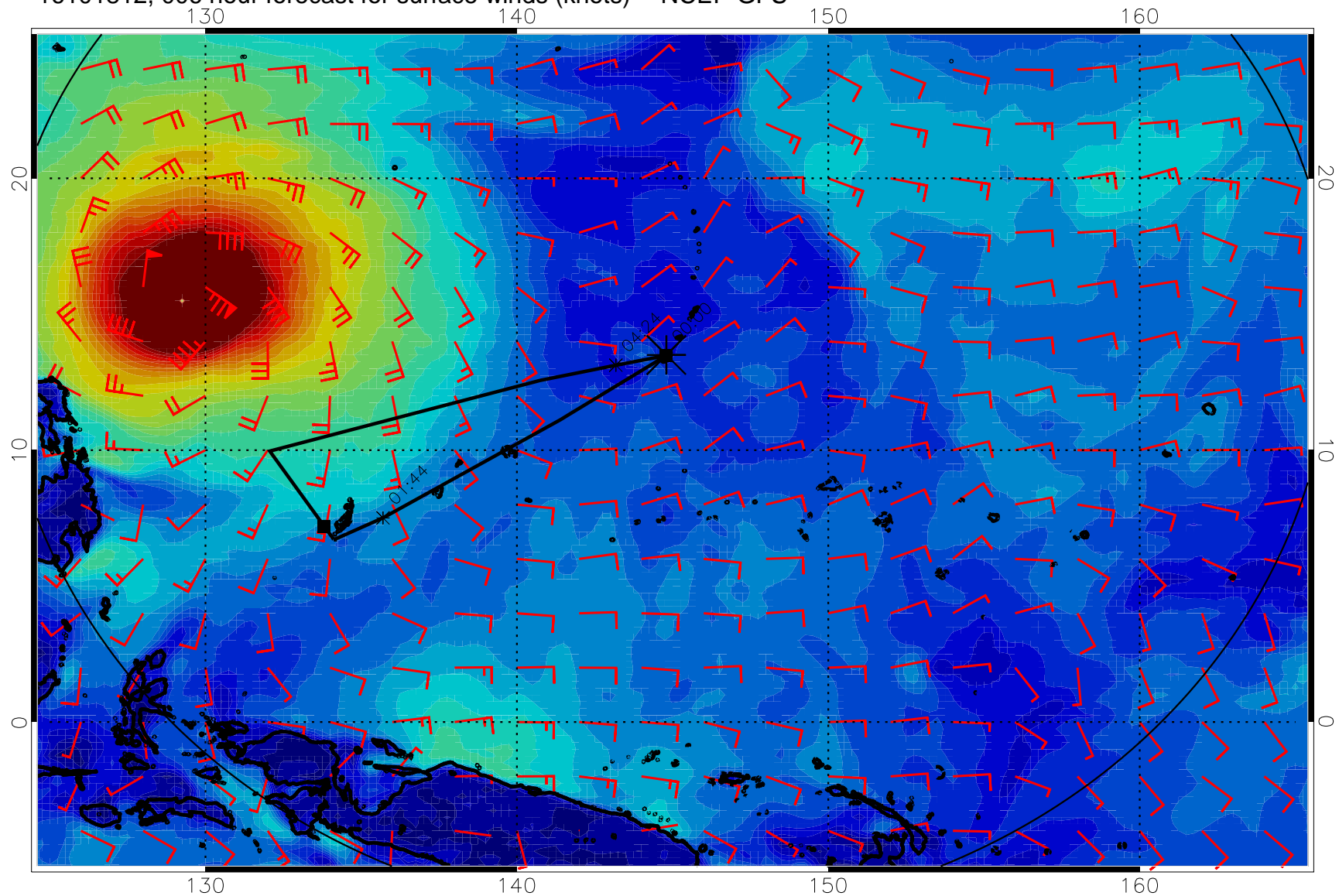
16101812, 006 hour forecast for surface winds (knots) -- NCEP GFS
