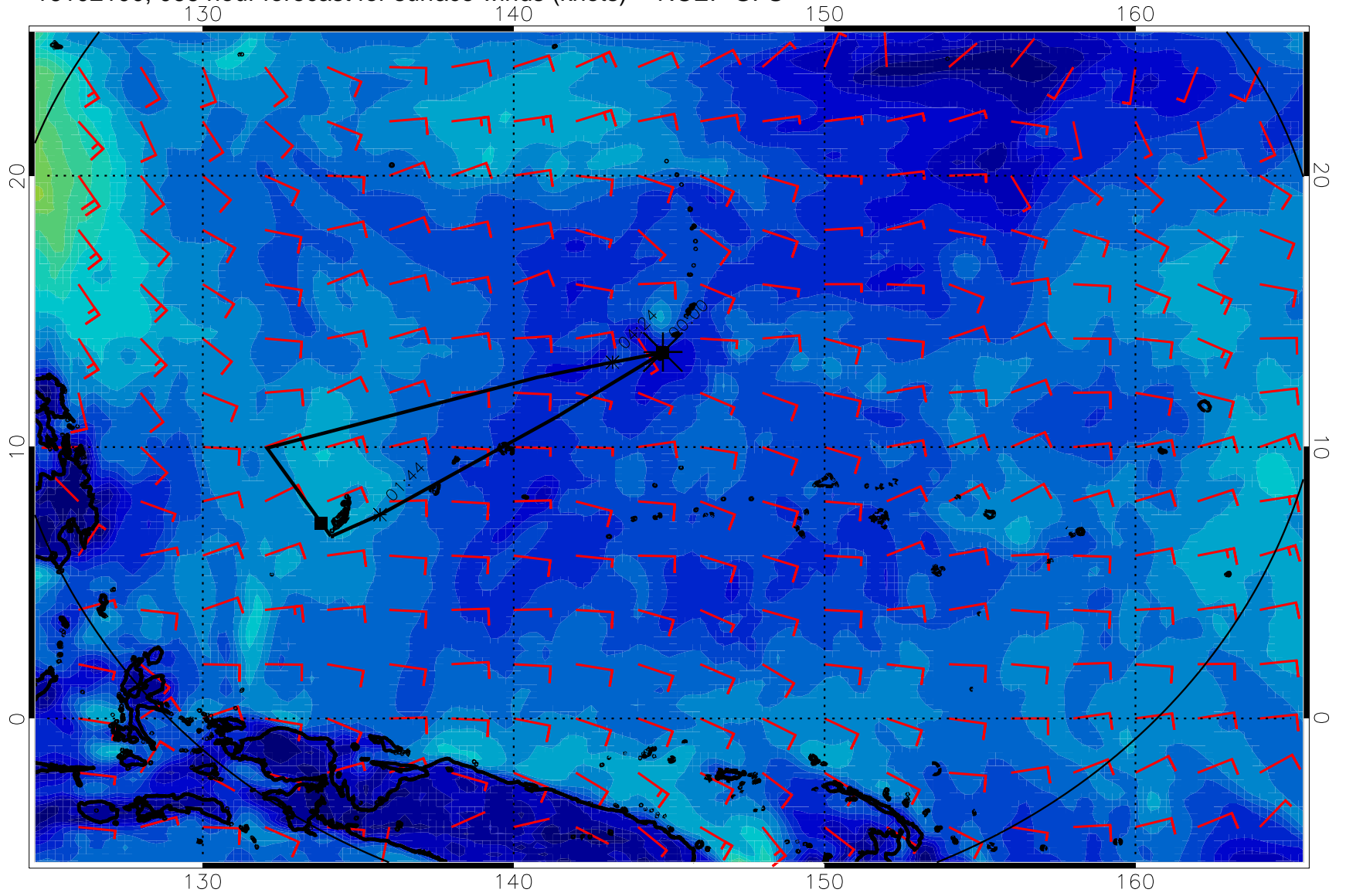
16102100, 066 hour forecast for surface winds (knots) -- NCEP GFS
