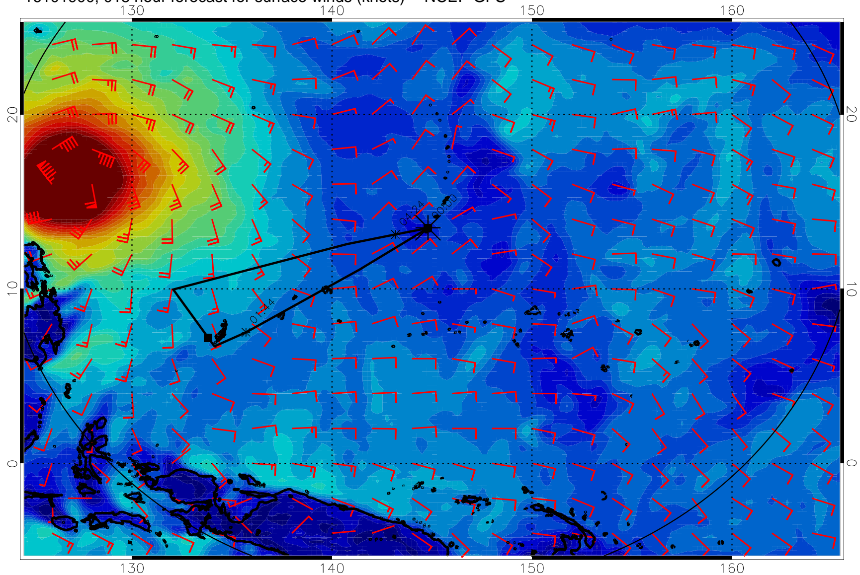
16101900, 018 hour forecast for surface winds (knots) -- NCEP GFS
