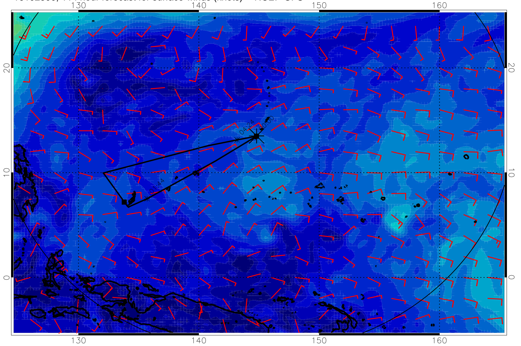
16102300, 114 hour forecast for surface winds (knots) -- NCEP GFS
