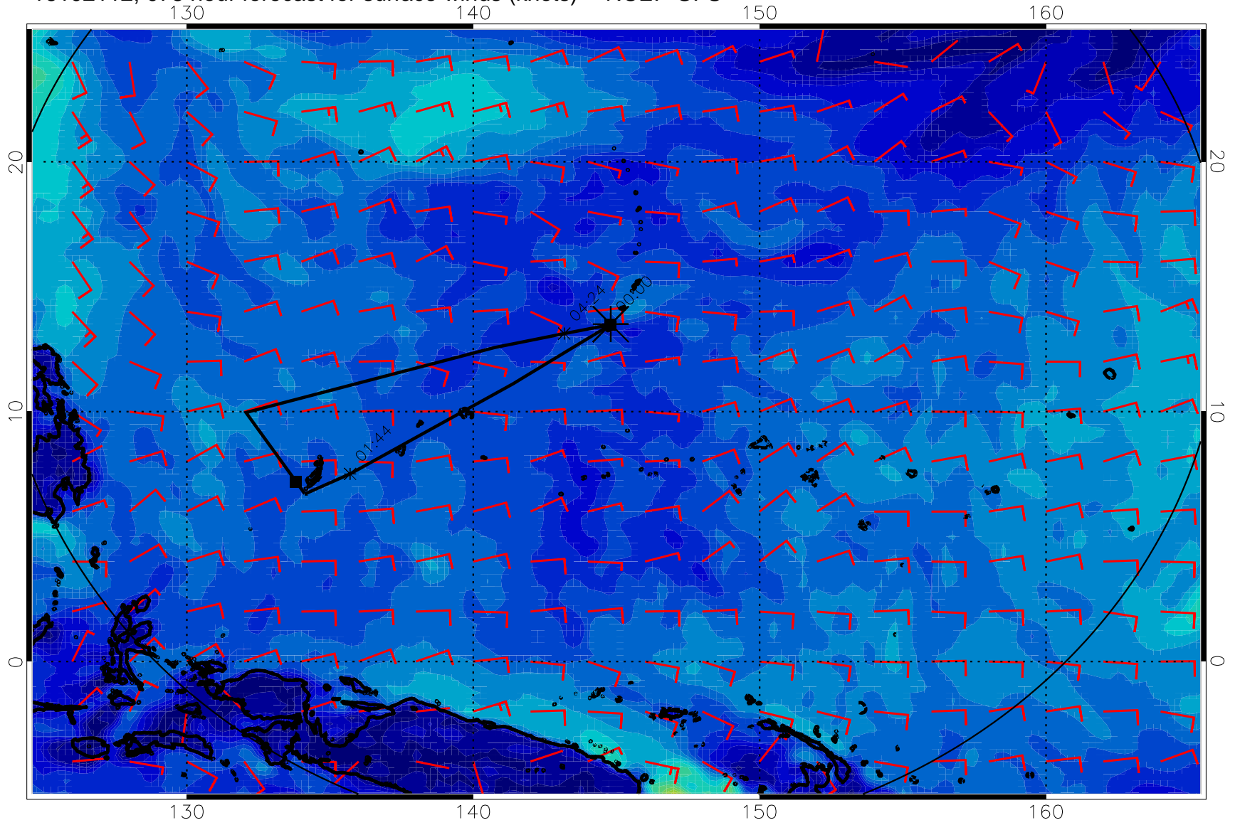
16102112, 078 hour forecast for surface winds (knots) -- NCEP GFS
