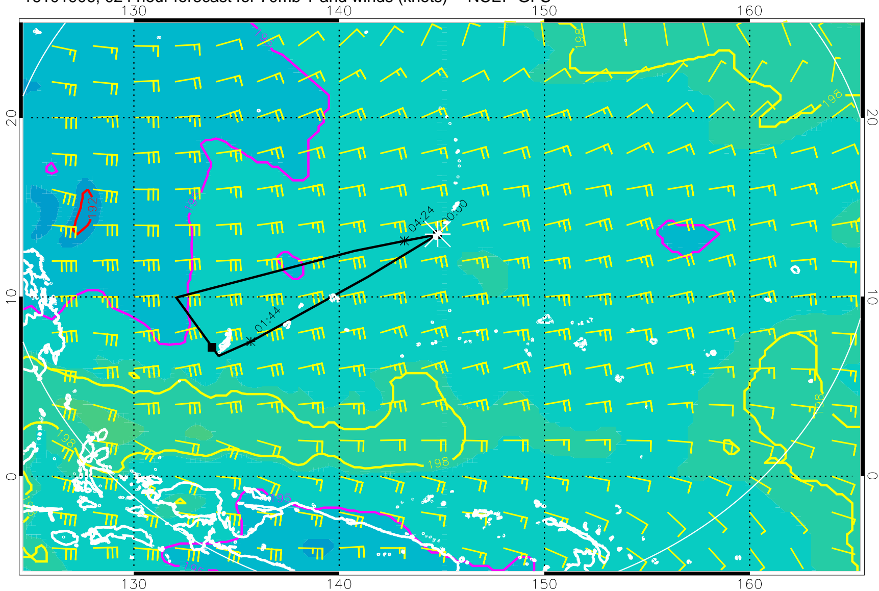
16101906, 024 hour forecast for 70mb T and winds (knots) -- NCEP GFS
