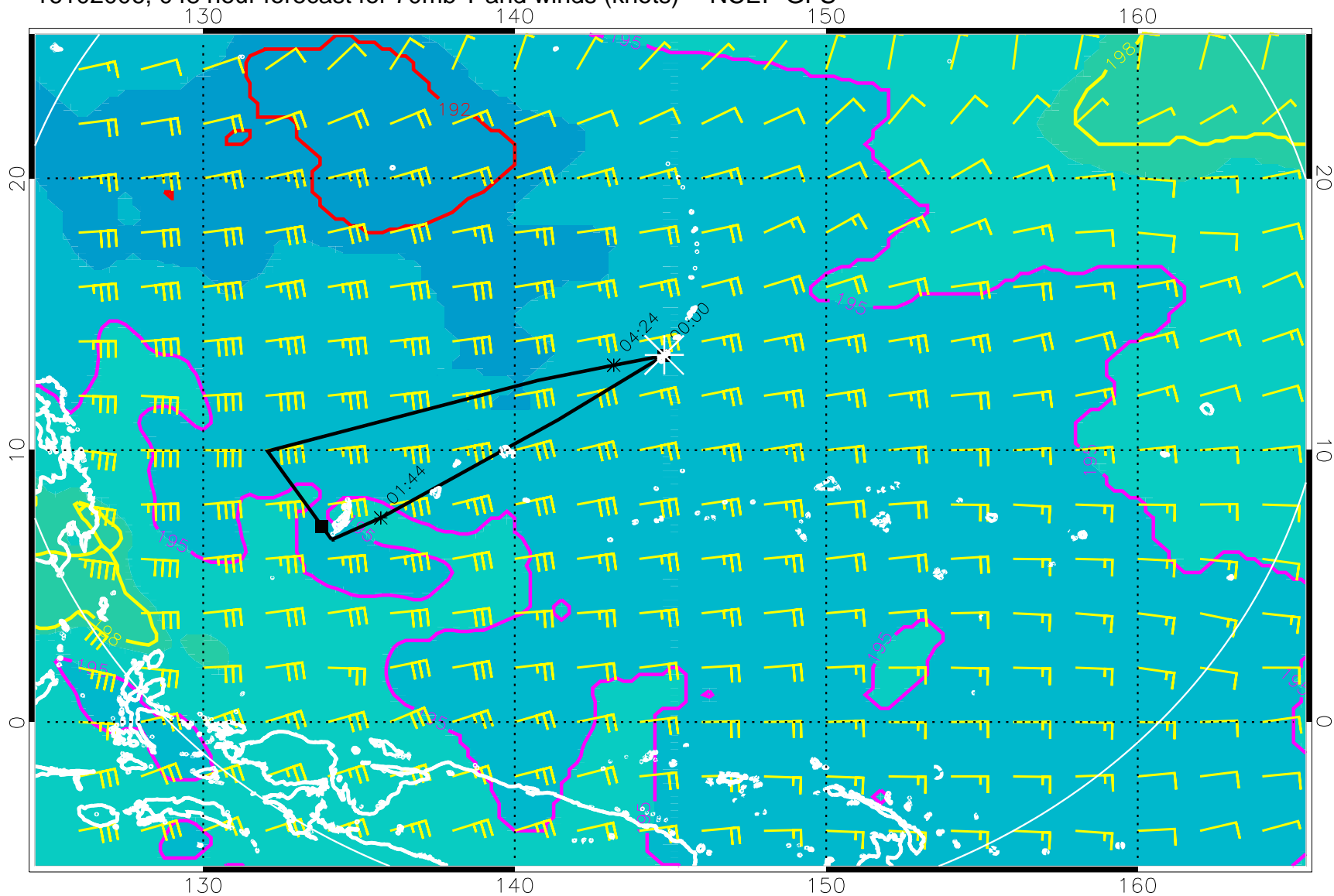
16102006, 048 hour forecast for 70mb T and winds (knots) -- NCEP GFS
