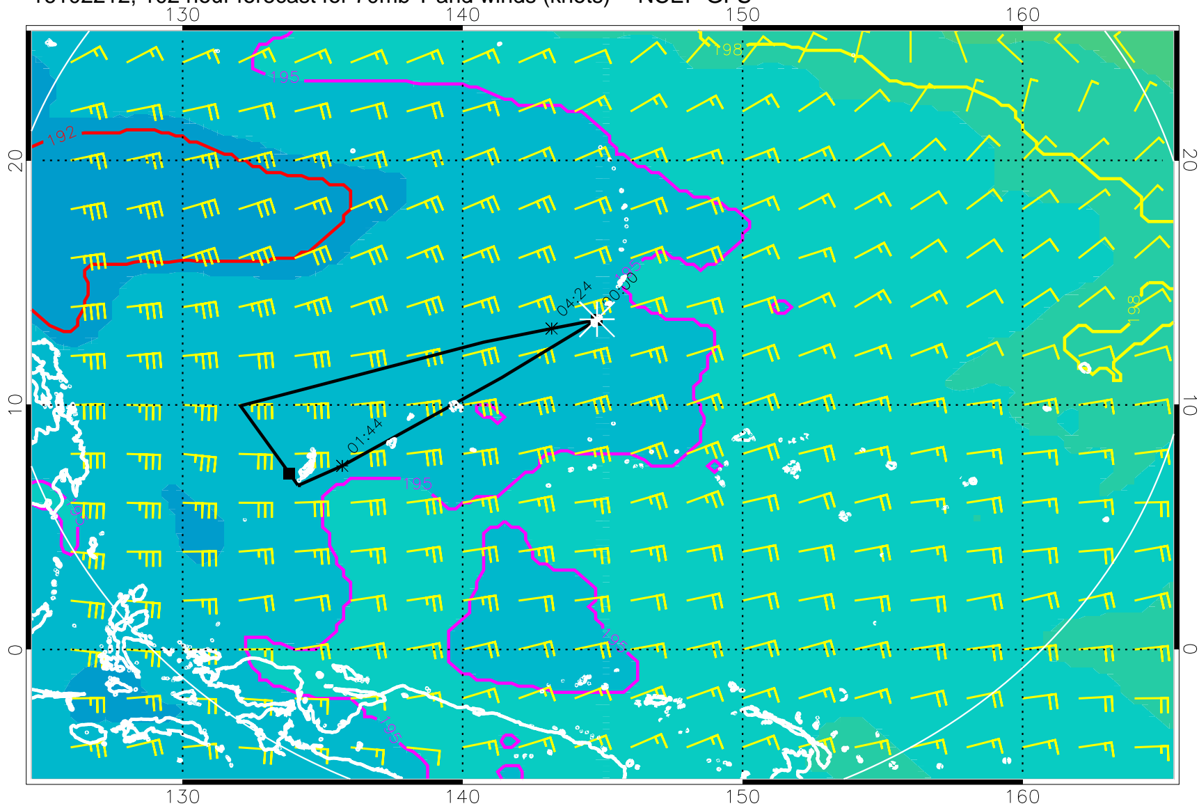
16102212, 102 hour forecast for 70mb T and winds (knots) -- NCEP GFS
