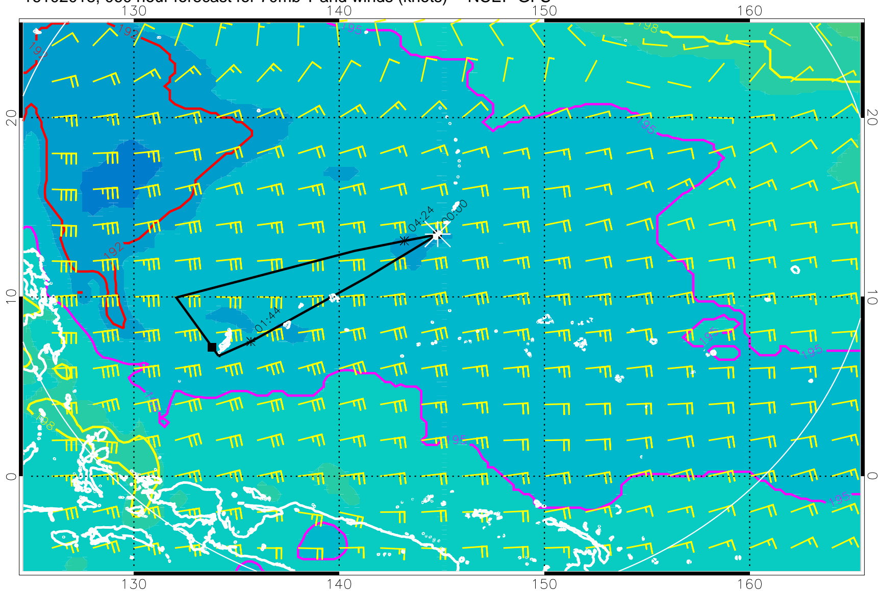
16102018, 060 hour forecast for 70mb T and winds (knots) -- NCEP GFS
