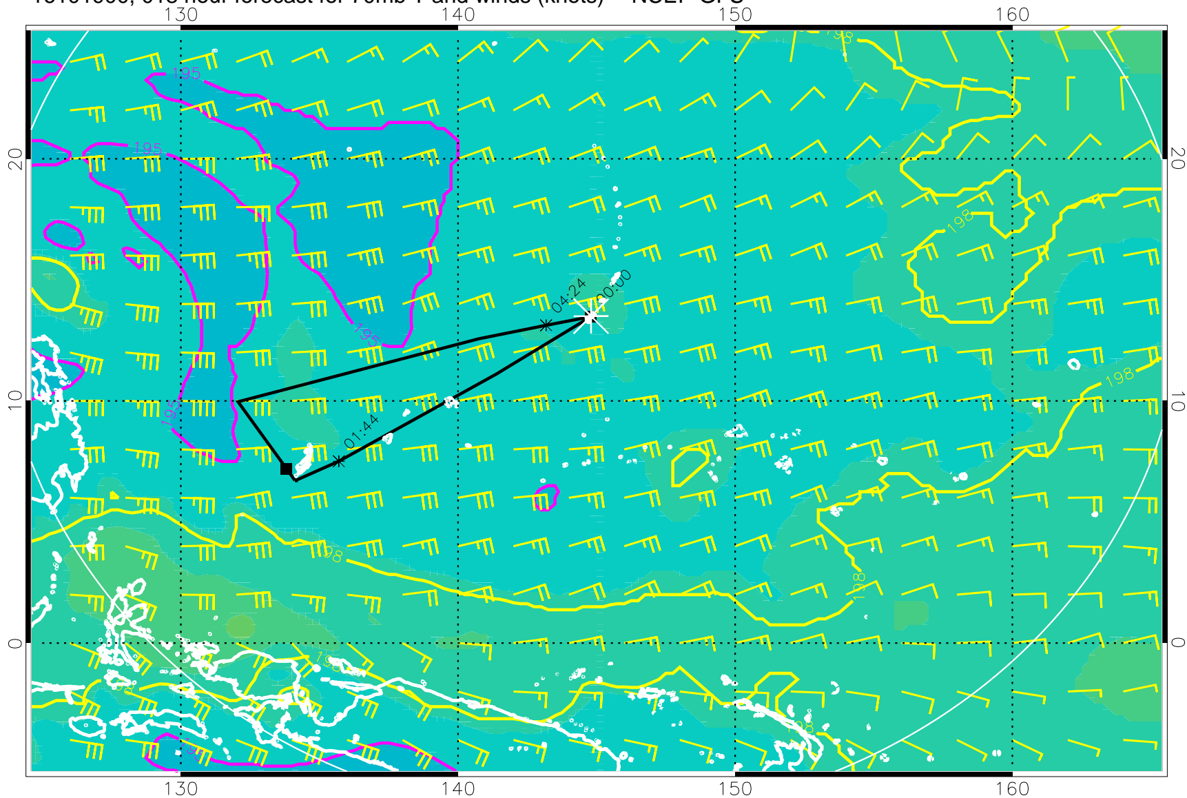
16101900, 018 hour forecast for 70mb T and winds (knots) -- NCEP GFS
