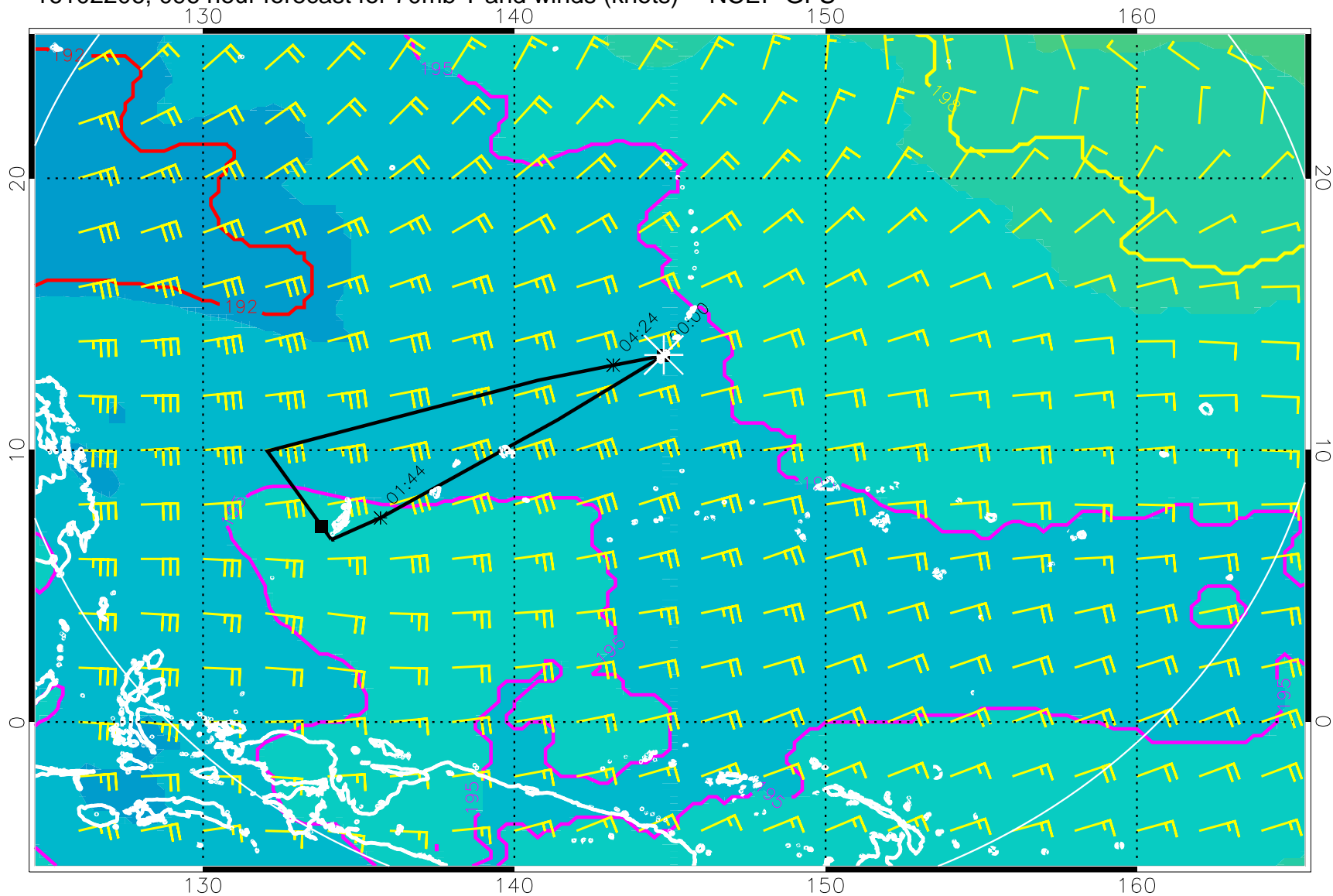
16102206, 096 hour forecast for 70mb T and winds (knots) -- NCEP GFS
