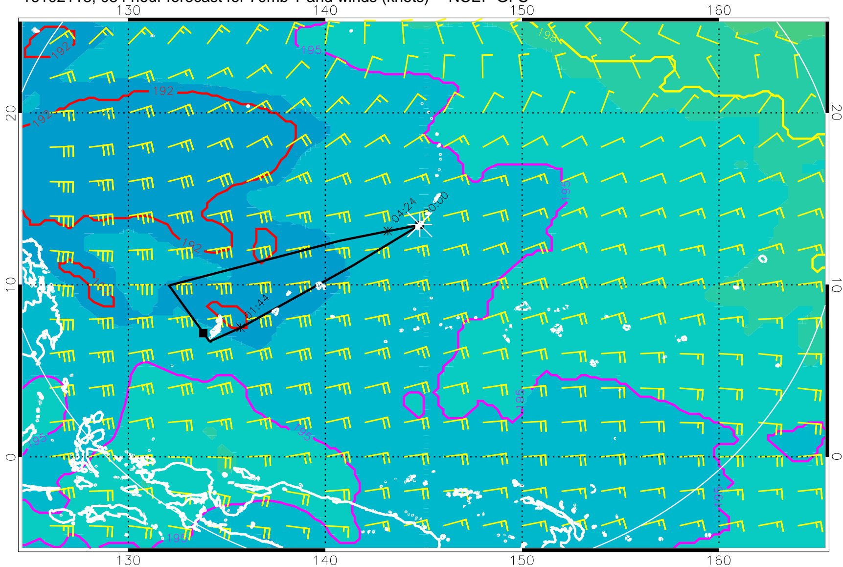
16102118, 084 hour forecast for 70mb T and winds (knots) -- NCEP GFS
