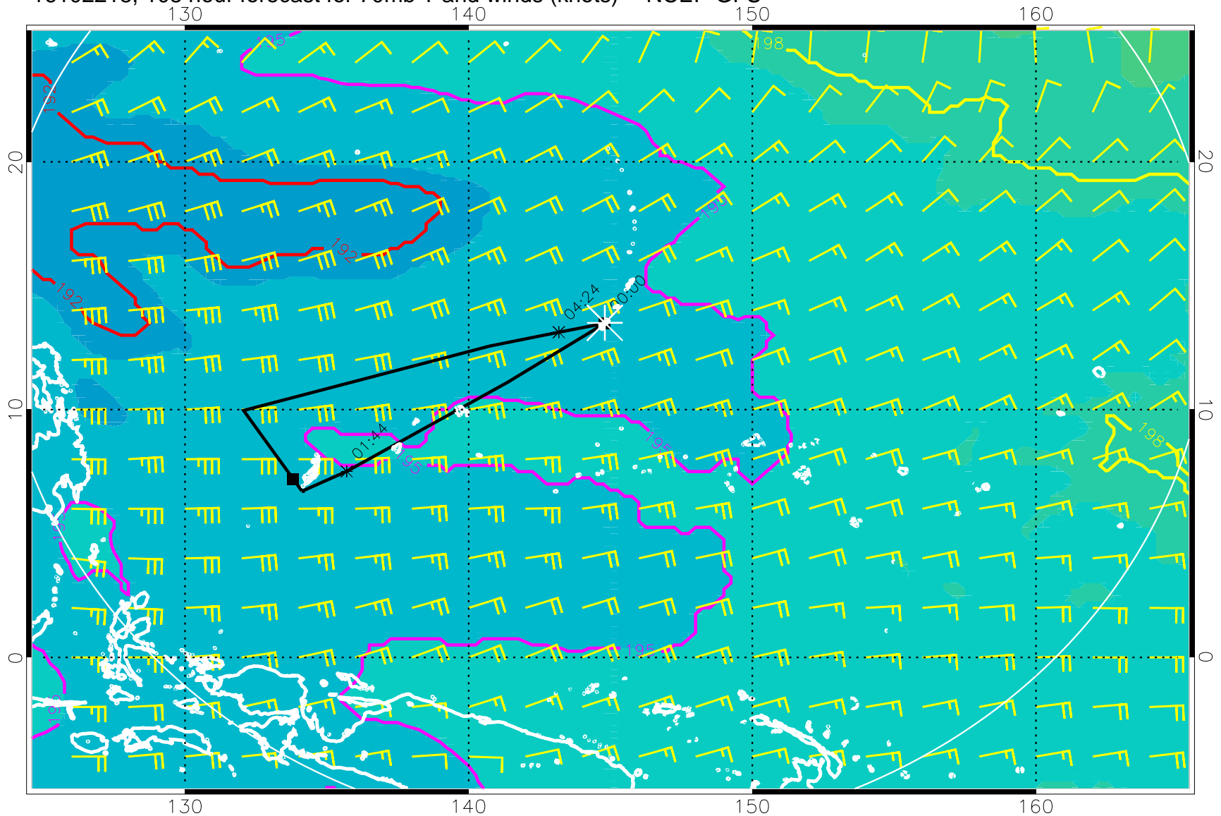
16102218, 108 hour forecast for 70mb T and winds (knots) -- NCEP GFS
