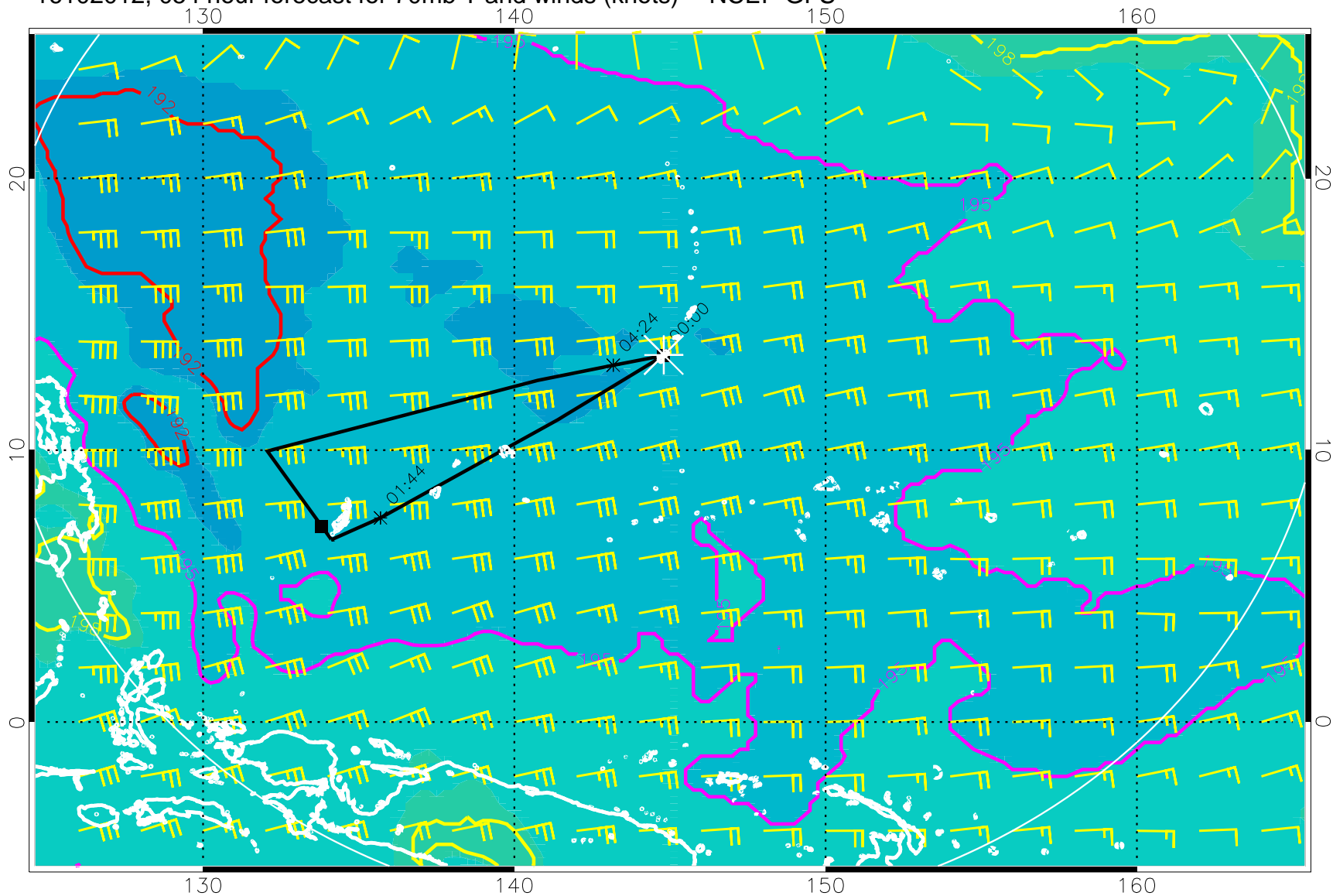
16102012, 054 hour forecast for 70mb T and winds (knots) -- NCEP GFS
