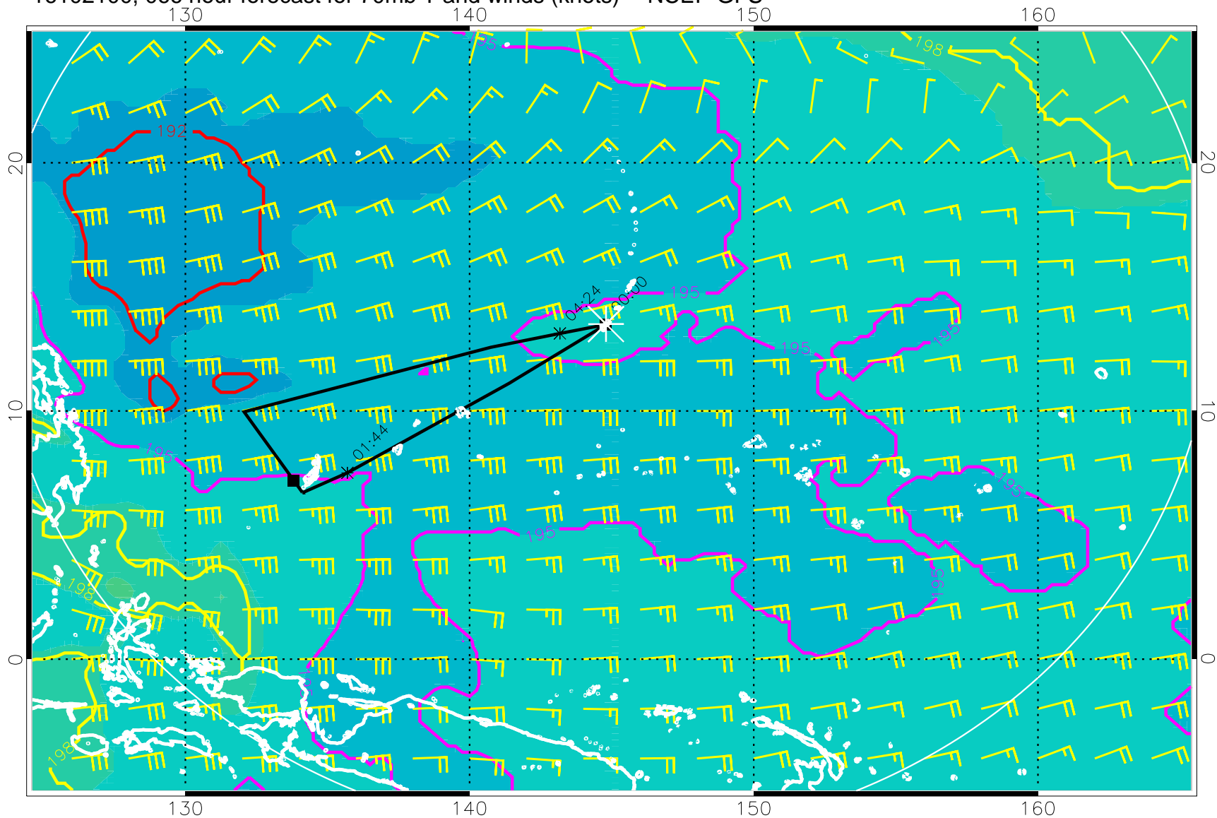
16102100, 066 hour forecast for 70mb T and winds (knots) -- NCEP GFS
