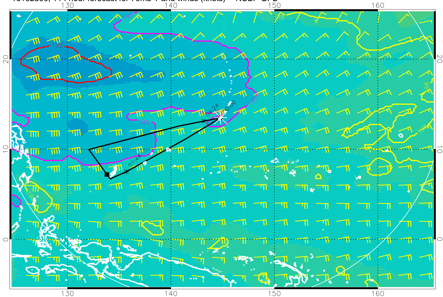
16102300, 114 hour forecast for 70mb T and winds (knots) -- NCEP GFS
