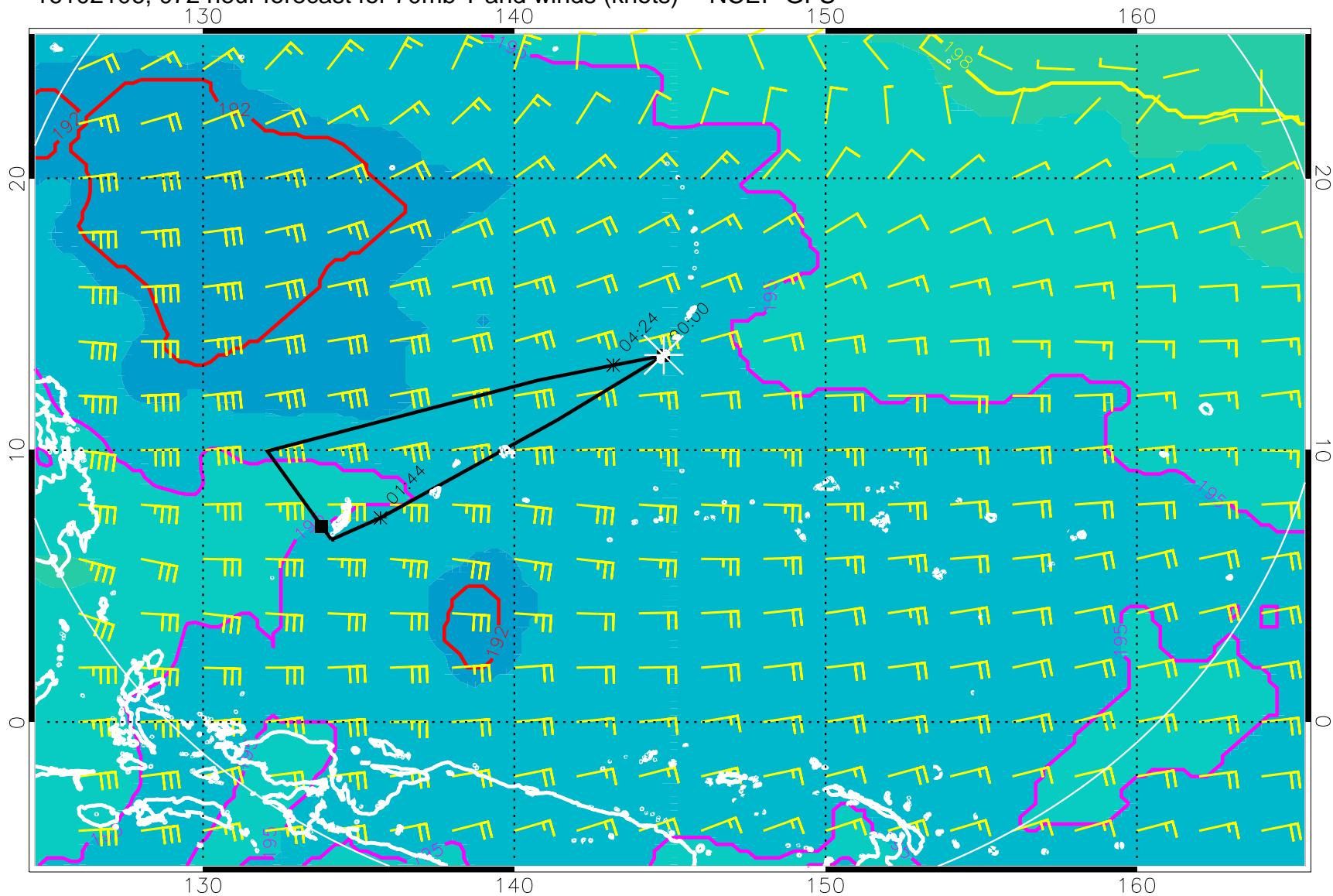
16102106, 072 hour forecast for 70mb T and winds (knots) -- NCEP GFS
