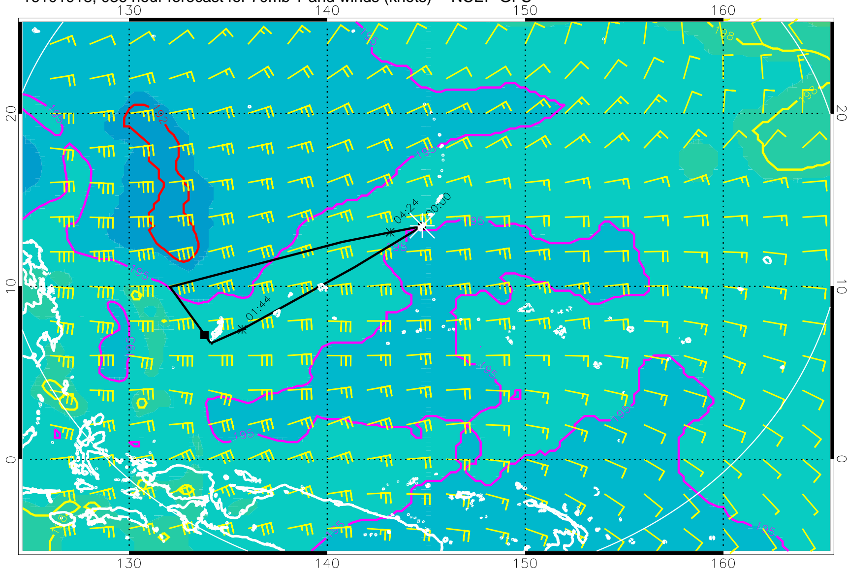
16101918, 036 hour forecast for 70mb T and winds (knots) -- NCEP GFS
