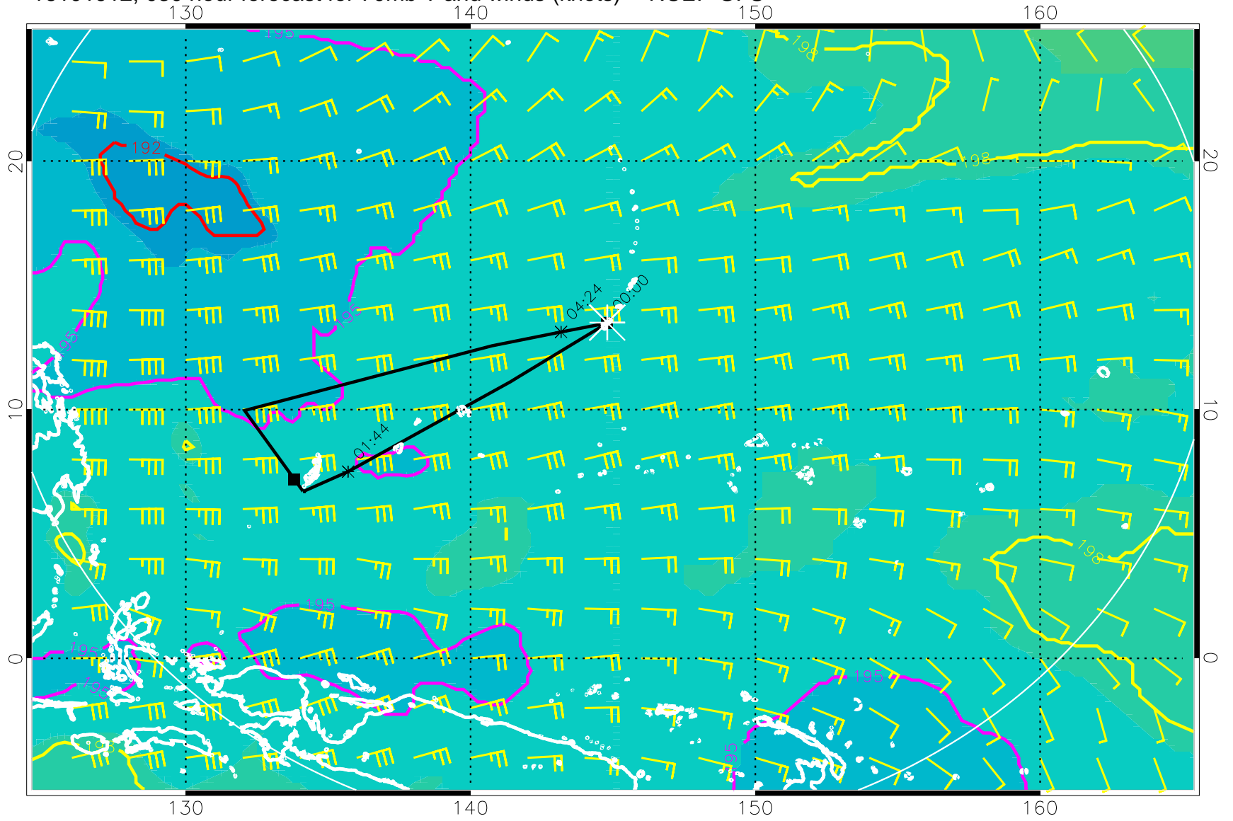
16101912, 030 hour forecast for 70mb T and winds (knots) -- NCEP GFS
