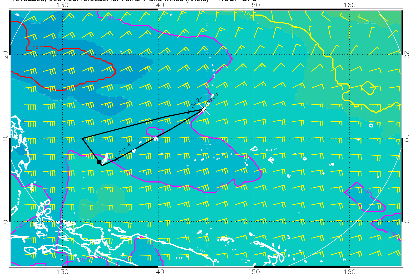
16102200, 090 hour forecast for 70mb T and winds (knots) -- NCEP GFS
