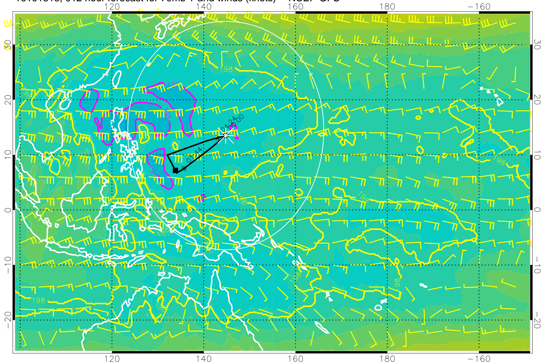
16101818, 012 hour forecast for 70mb T and winds (knots) -- NCEP GFS
