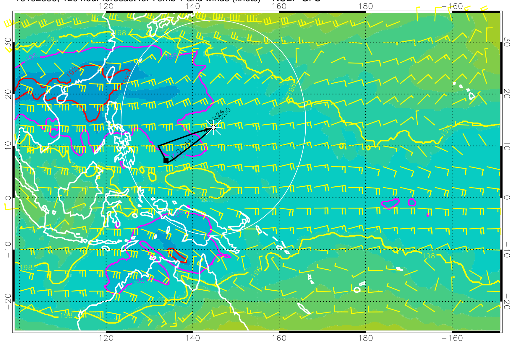
16102306, 120 hour forecast for 70mb T and winds (knots) -- NCEP GFS
