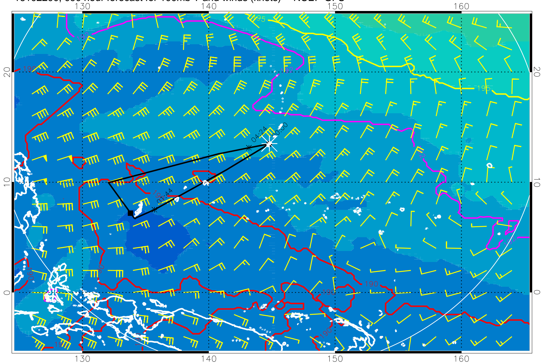
16102200, 090 hour forecast for 100mb T and winds (knots) -- NCEP GFS
