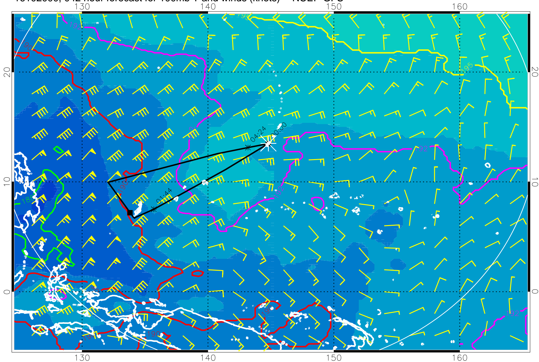
16102000, 042 hour forecast for 100mb T and winds (knots) -- NCEP GFS
