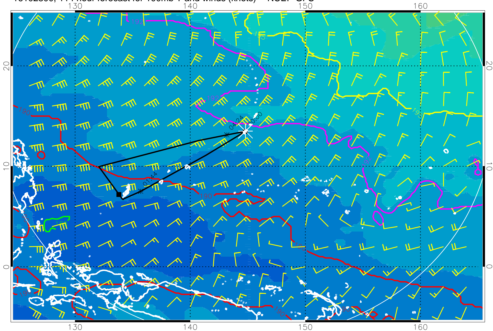
16102300, 114 hour forecast for 100mb T and winds (knots) -- NCEP GFS
