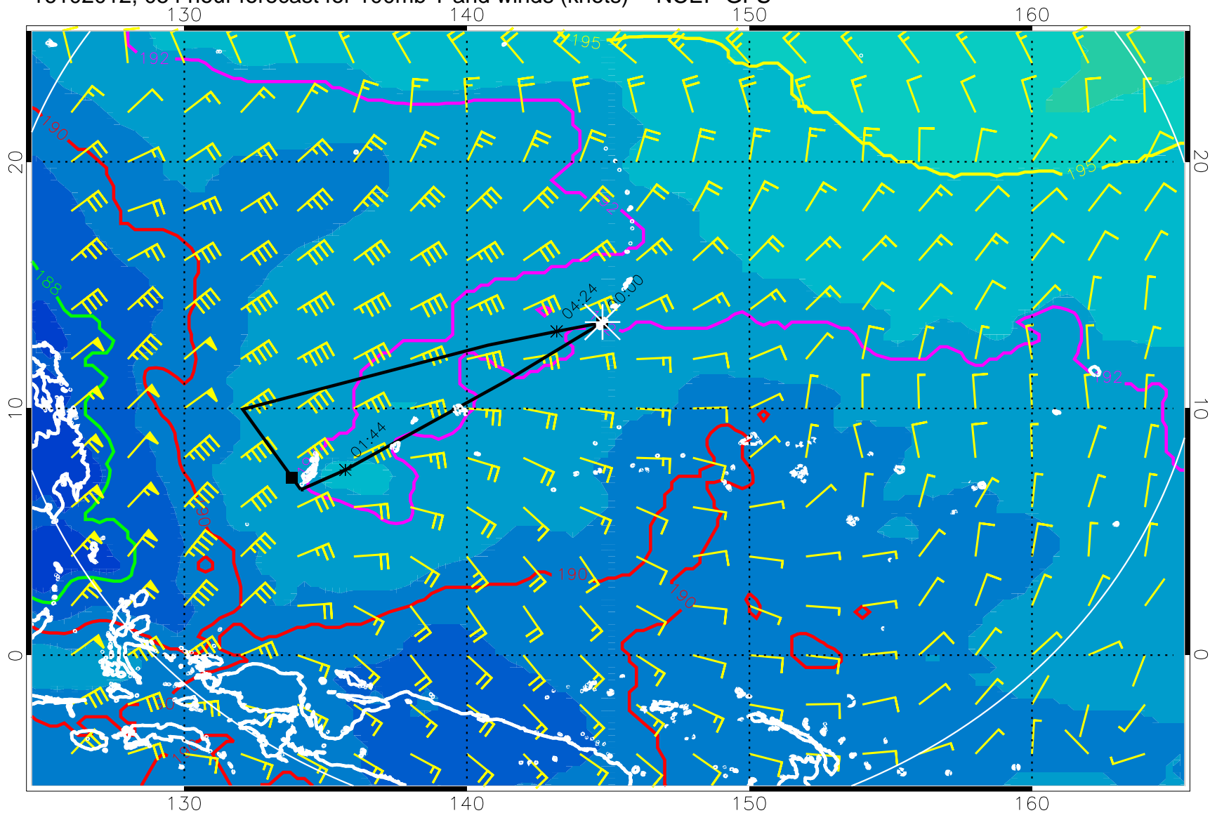
16102012, 054 hour forecast for 100mb T and winds (knots) -- NCEP GFS
