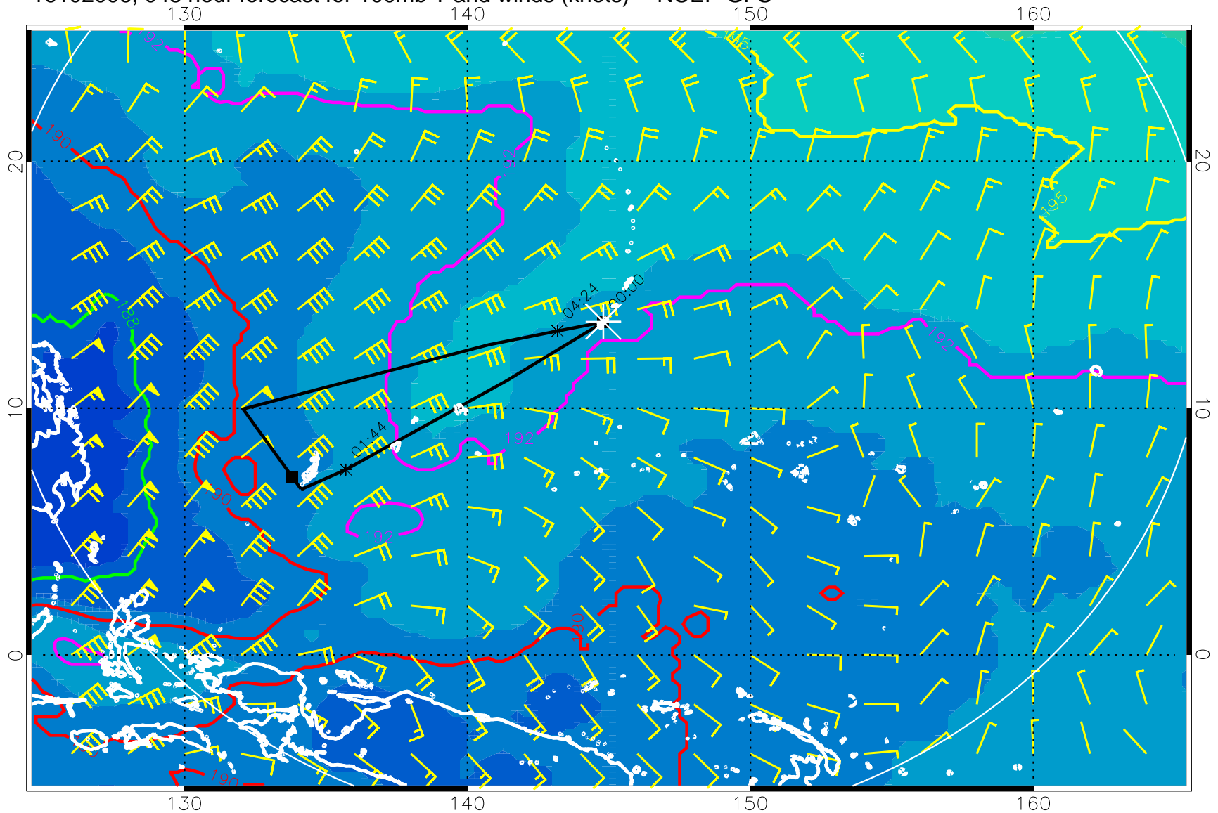
16102006, 048 hour forecast for 100mb T and winds (knots) -- NCEP GFS
