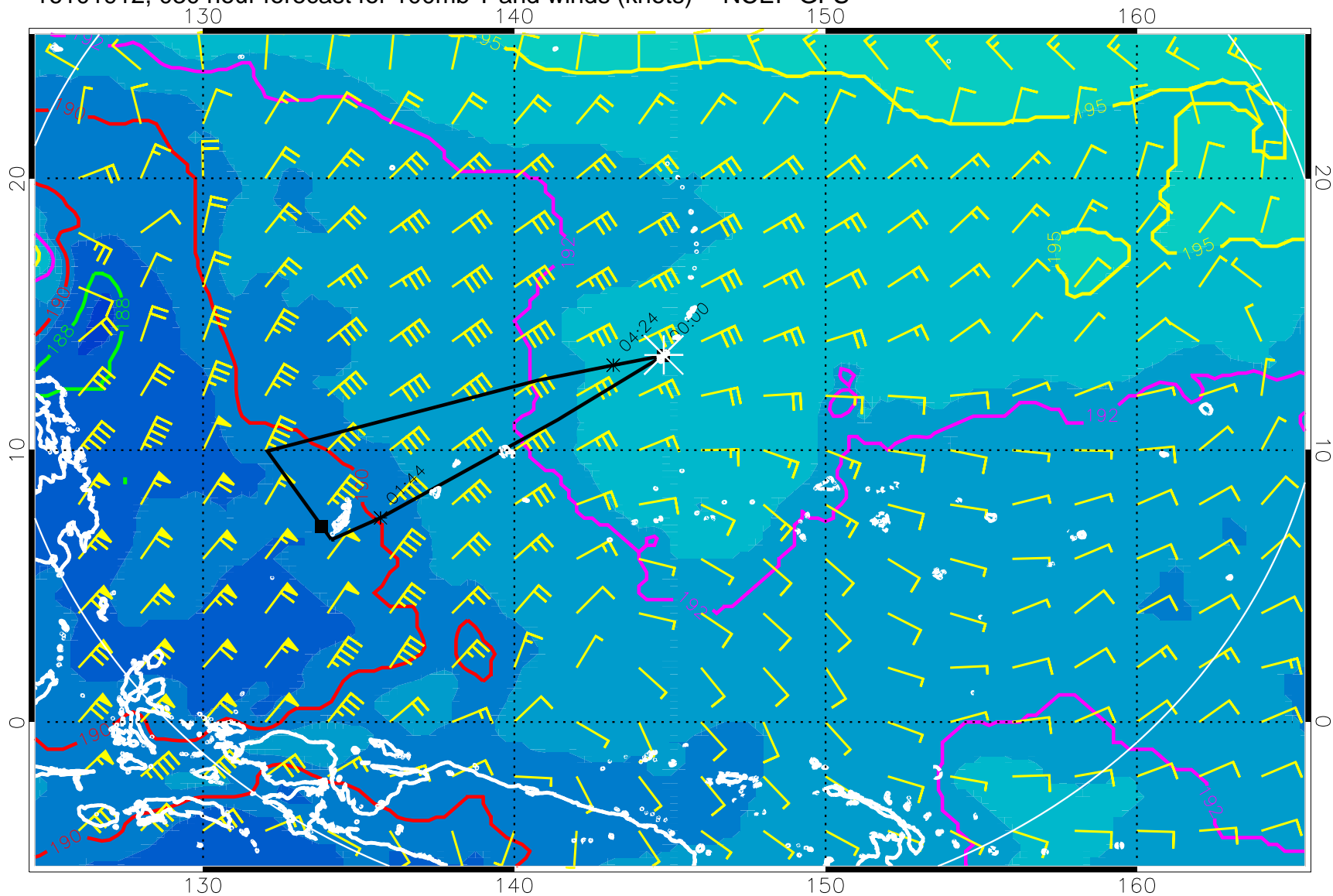
16101912, 030 hour forecast for 100mb T and winds (knots) -- NCEP GFS
