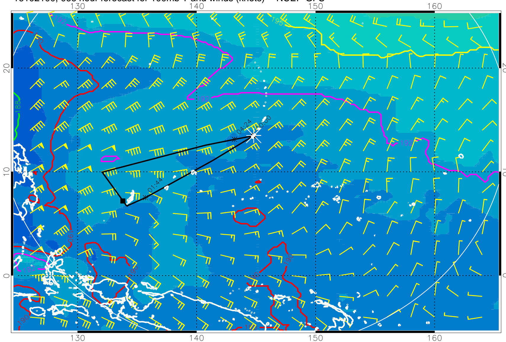
16102100, 066 hour forecast for 100mb T and winds (knots) -- NCEP GFS
