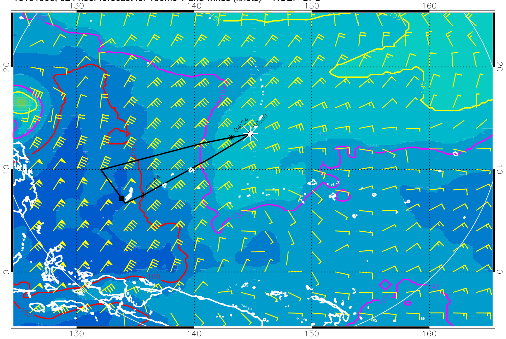
16101906, 024 hour forecast for 100mb T and winds (knots) -- NCEP GFS
