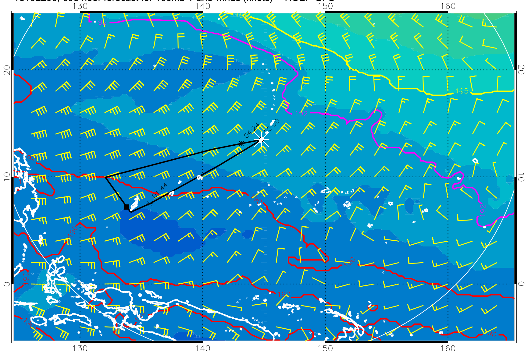
16102206, 096 hour forecast for 100mb T and winds (knots) -- NCEP GFS
