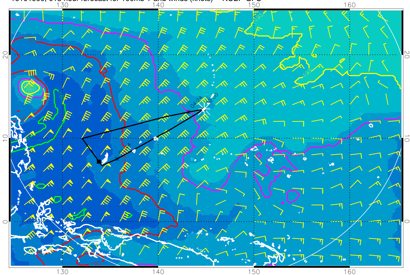
16101900, 018 hour forecast for 100mb T and winds (knots) -- NCEP GFS
