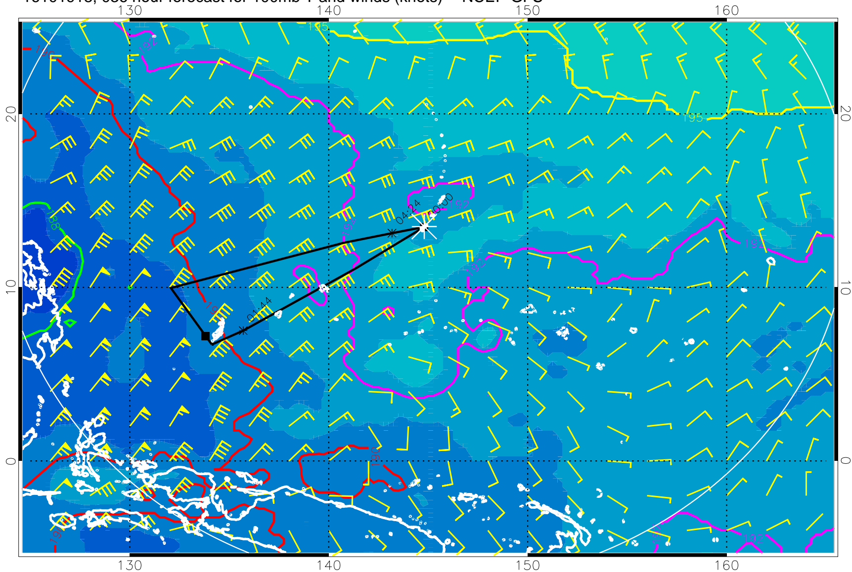
16101918, 036 hour forecast for 100mb T and winds (knots) -- NCEP GFS
