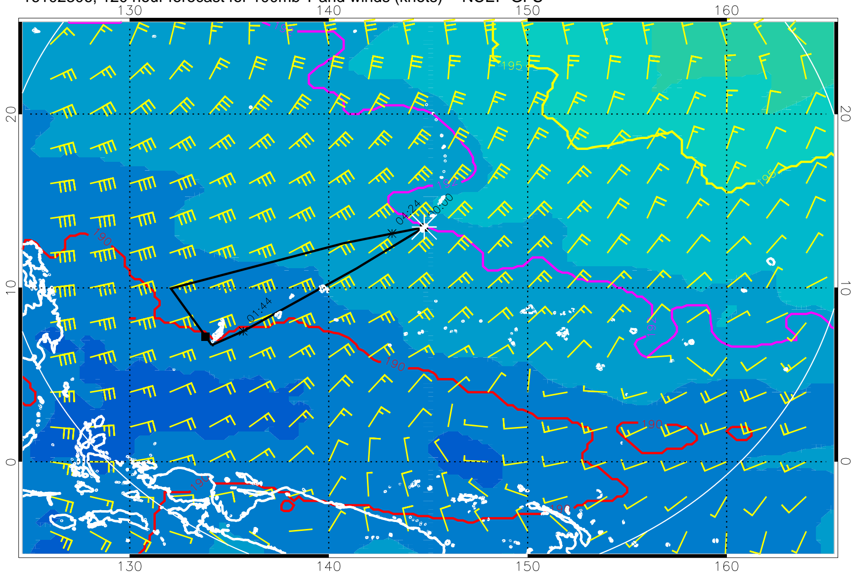
16102306, 120 hour forecast for 100mb T and winds (knots) -- NCEP GFS
