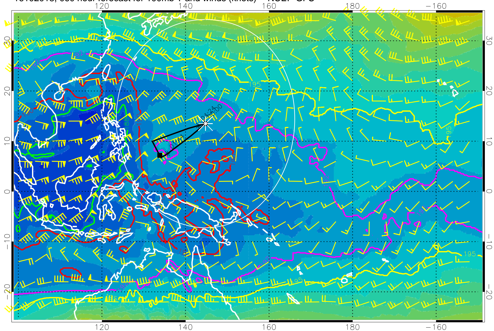
16102018, 060 hour forecast for 100mb T and winds (knots) -- NCEP GFS
