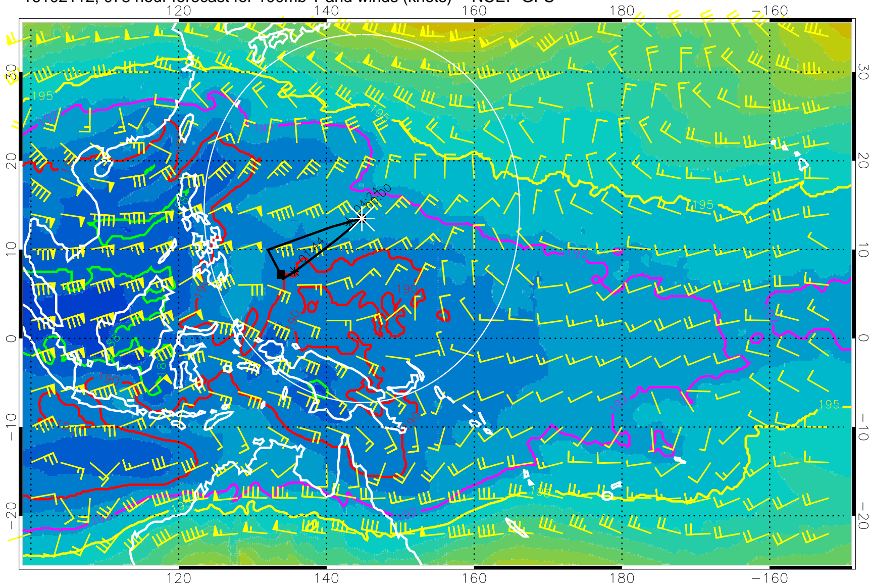
16102112, 078 hour forecast for 100mb T and winds (knots) -- NCEP GFS
