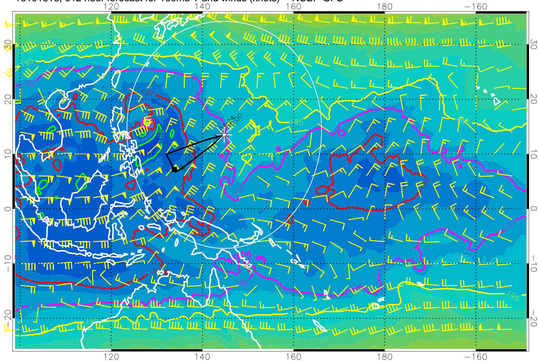
16101818, 012 hour forecast for 100mb T and winds (knots) -- NCEP GFS
