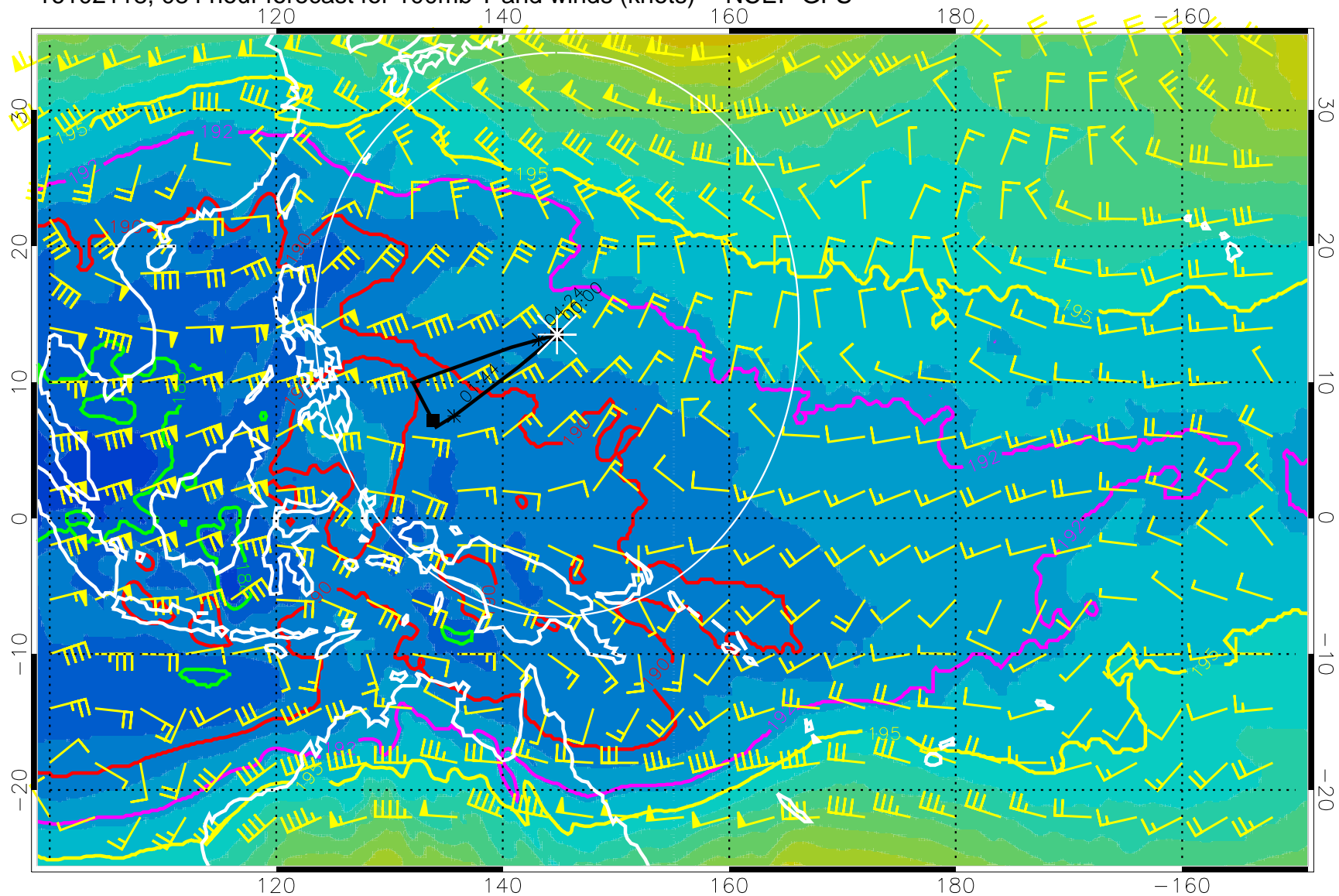
16102118, 084 hour forecast for 100mb T and winds (knots) -- NCEP GFS
