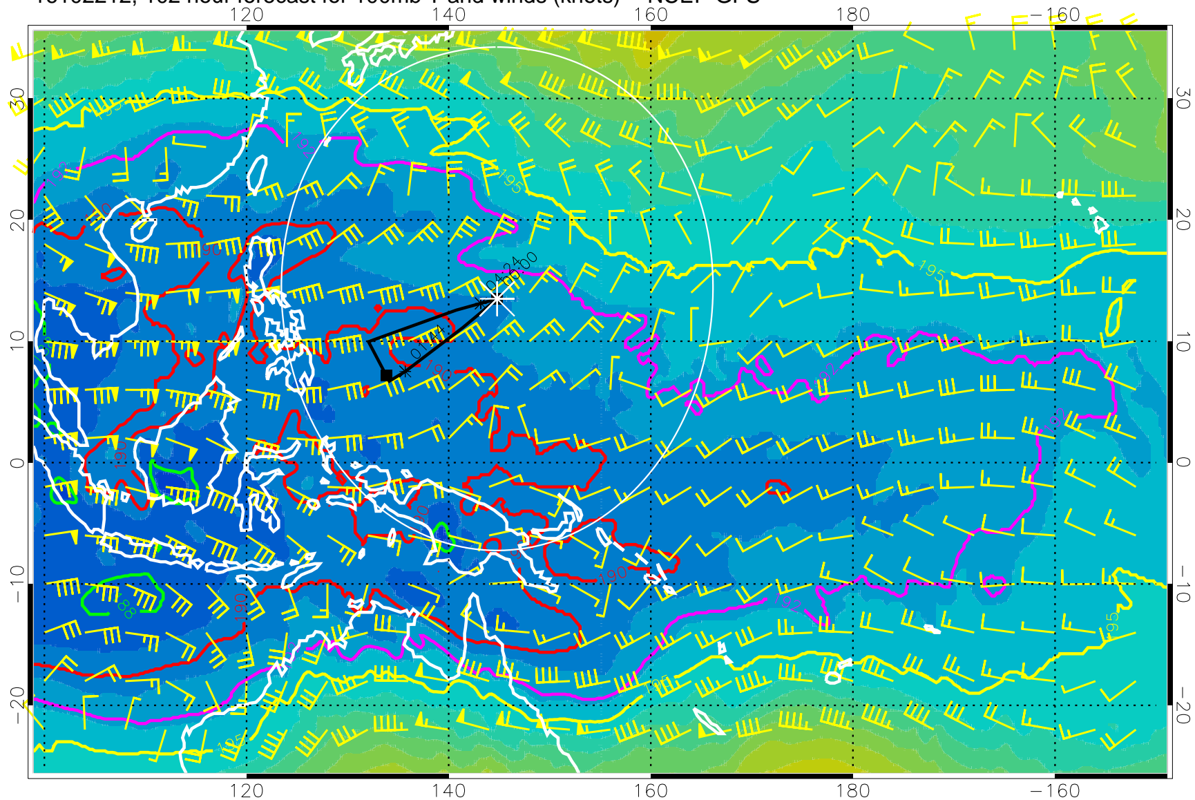
16102212, 102 hour forecast for 100mb T and winds (knots) -- NCEP GFS
