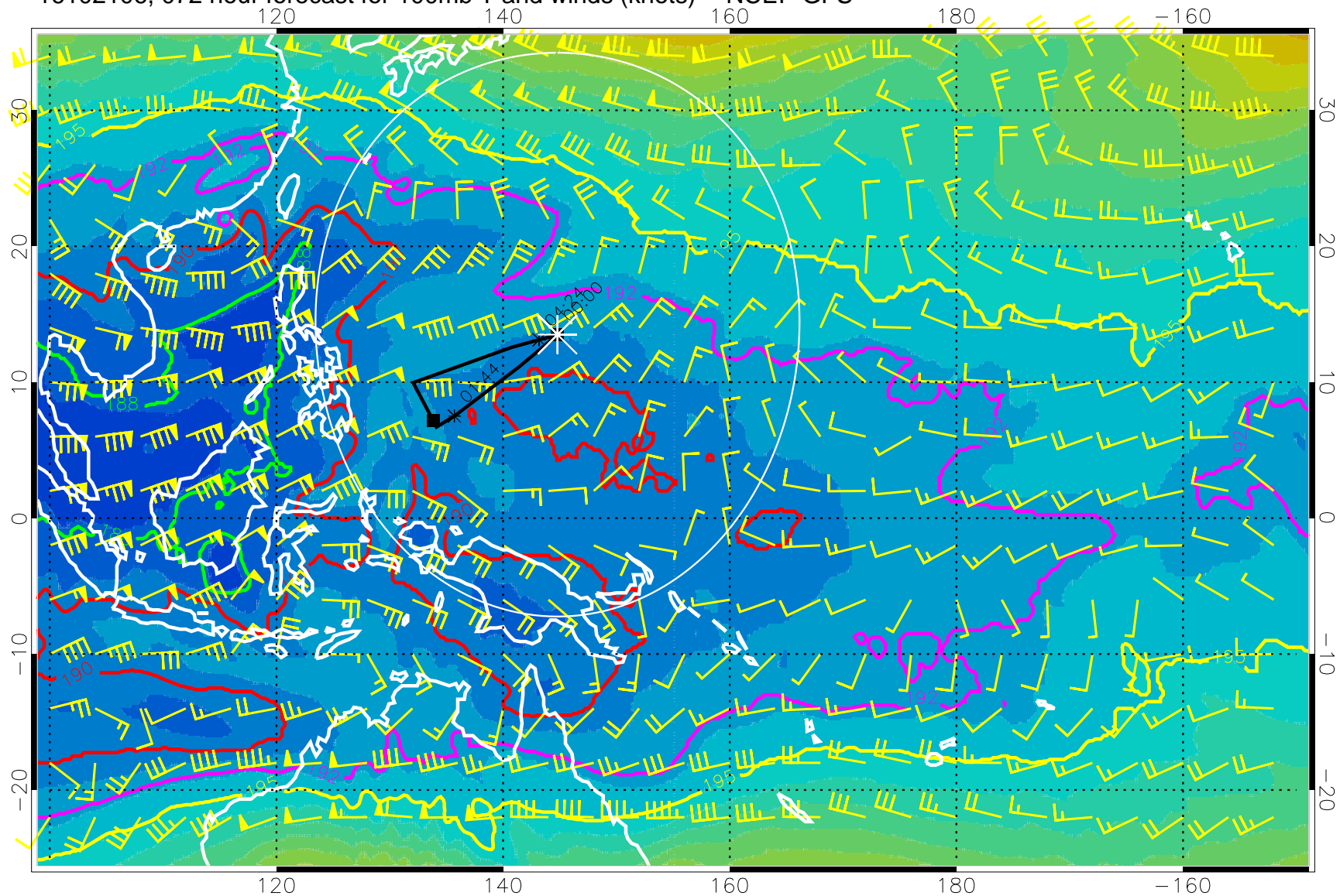
16102106, 072 hour forecast for 100mb T and winds (knots) -- NCEP GFS
