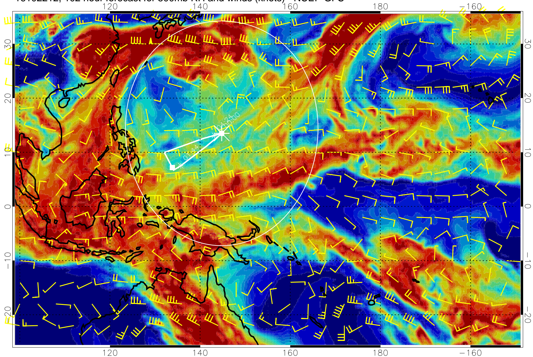
16102212, 102 hour forecast for 500mb RH and winds (knots) - NCEP GFS
