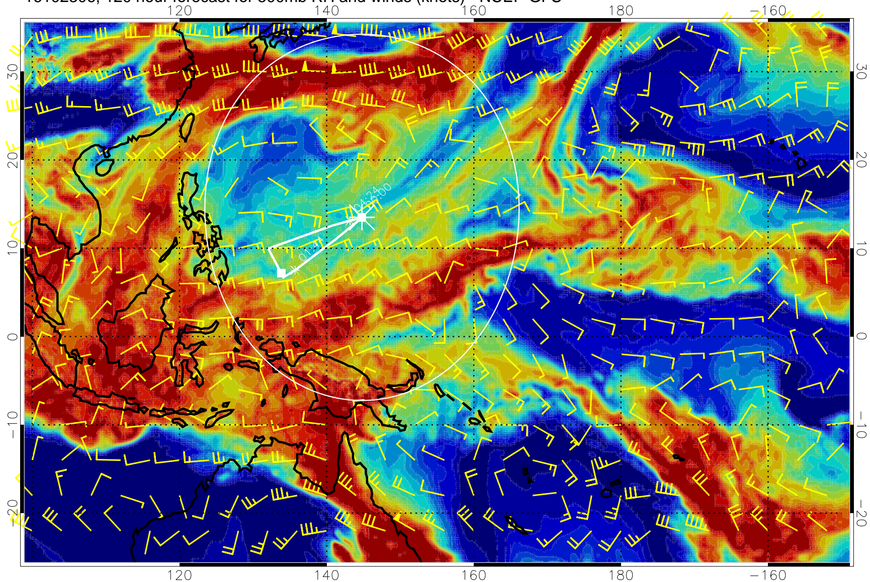
16102306, 120 hour forecast for 500mb RH and winds (knots) - NCEP GFS
