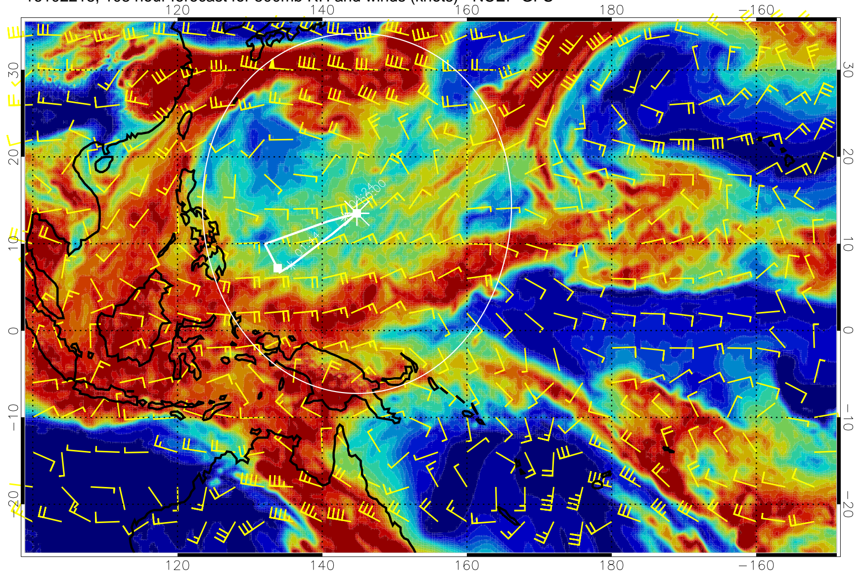
16102218, 108 hour forecast for 500mb RH and winds (knots) - NCEP GFS
