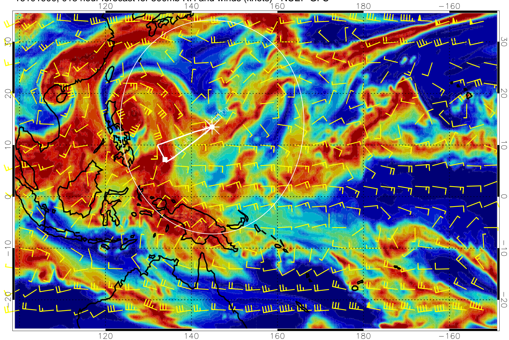
16101900, 018 hour forecast for 500mb RH and winds (knots) - NCEP GFS
