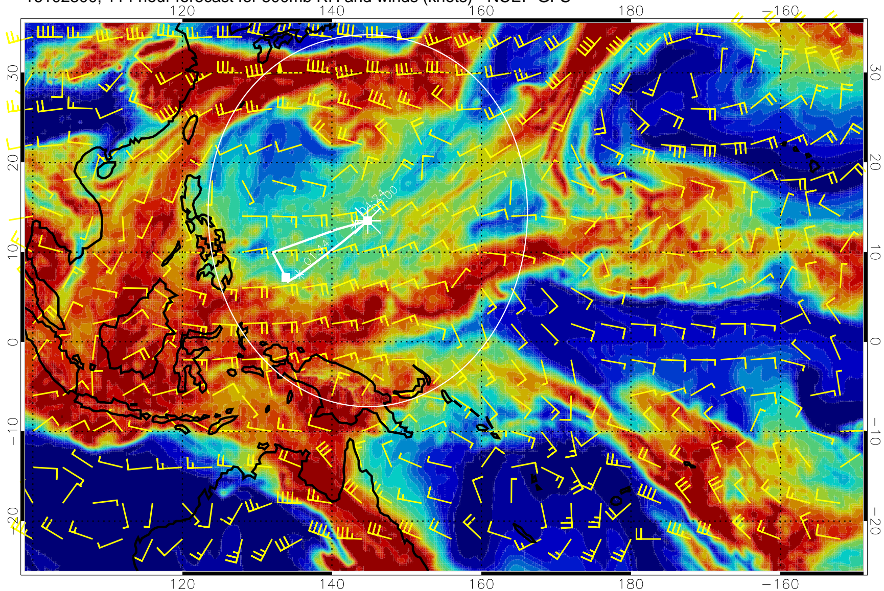
16102300, 114 hour forecast for 500mb RH and winds (knots) - NCEP GFS
