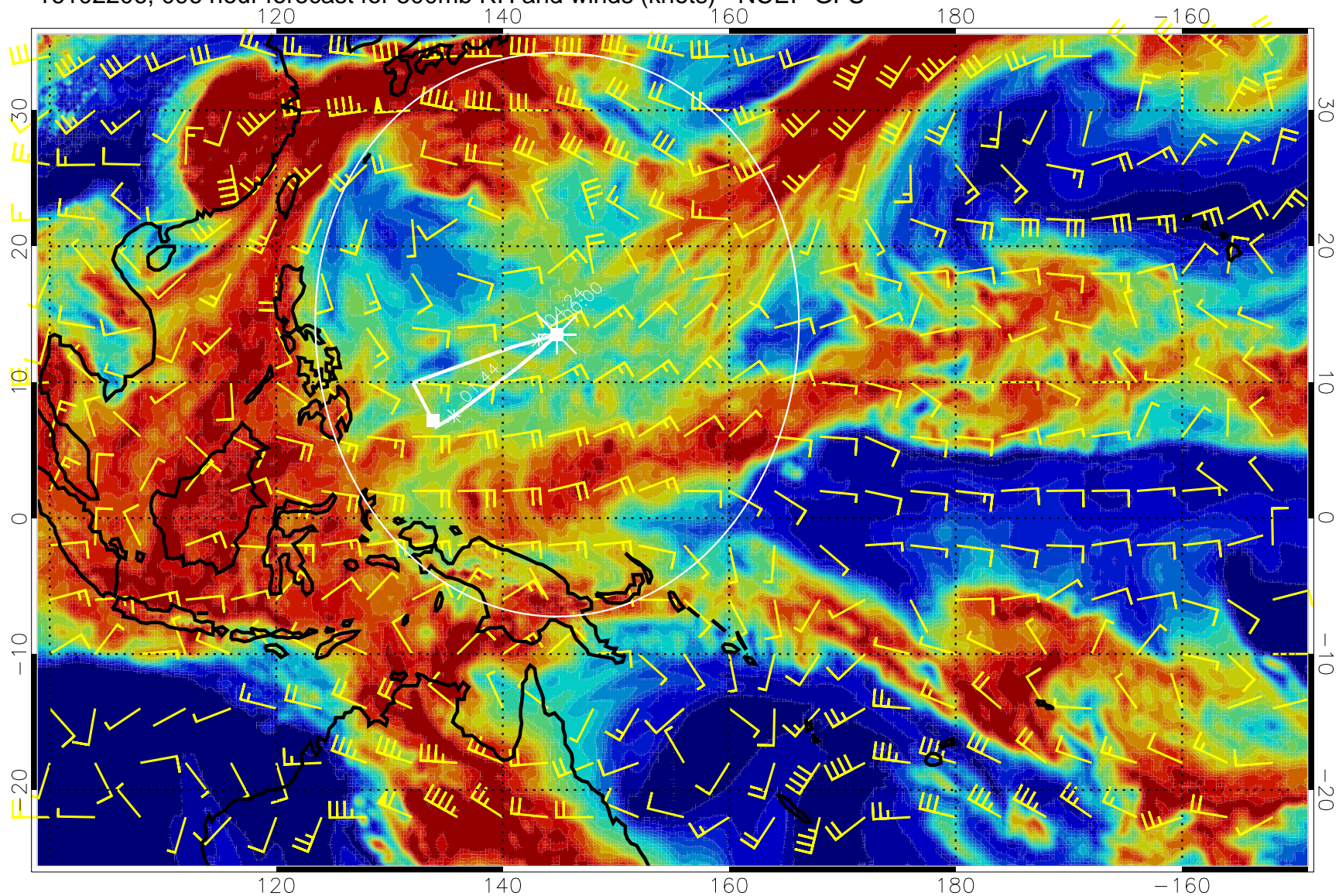
16102206, 096 hour forecast for 500mb RH and winds (knots) - NCEP GFS
