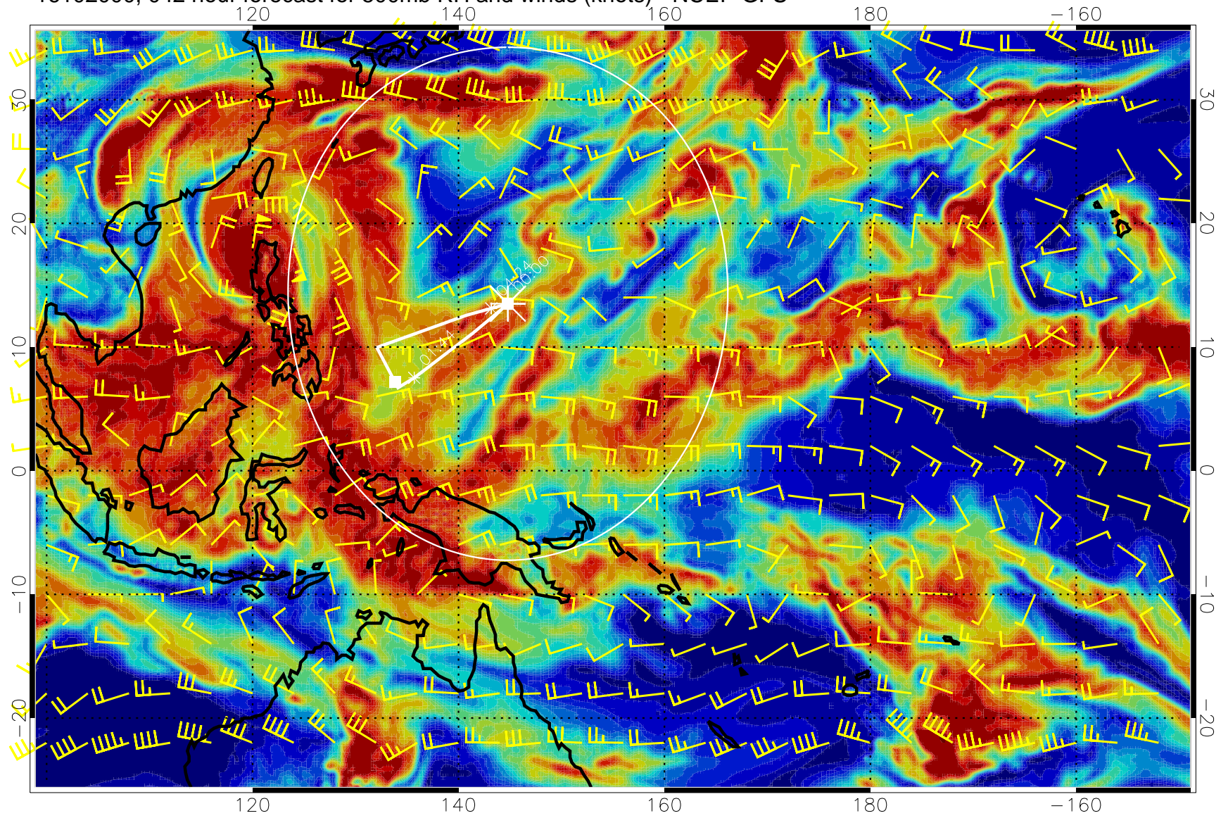
16102000, 042 hour forecast for 500mb RH and winds (knots) - NCEP GFS
