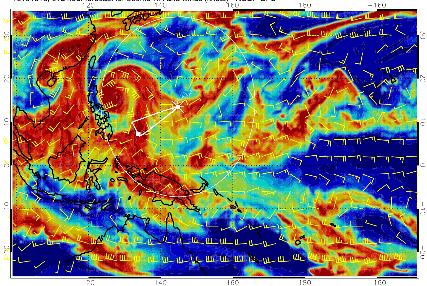
16101818, 012 hour forecast for 500mb RH and winds (knots) - NCEP GFS
