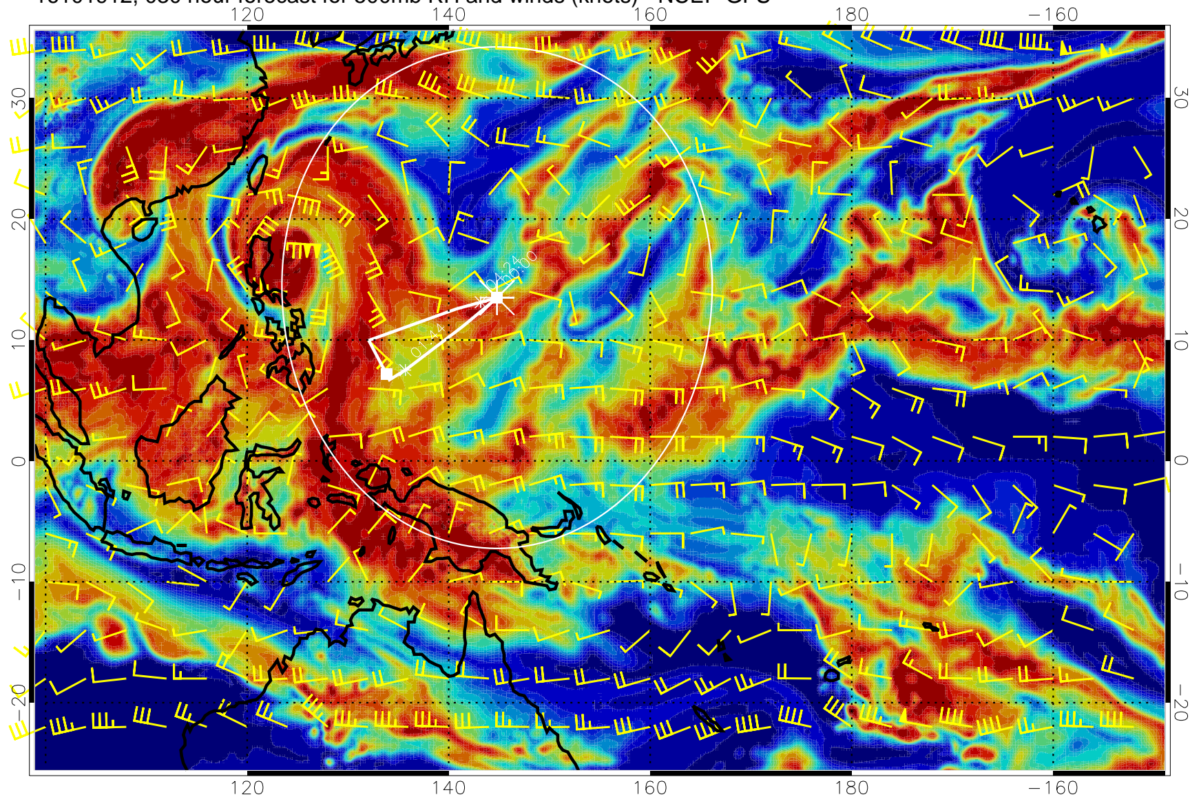
16101912, 030 hour forecast for 500mb RH and winds (knots) - NCEP GFS
