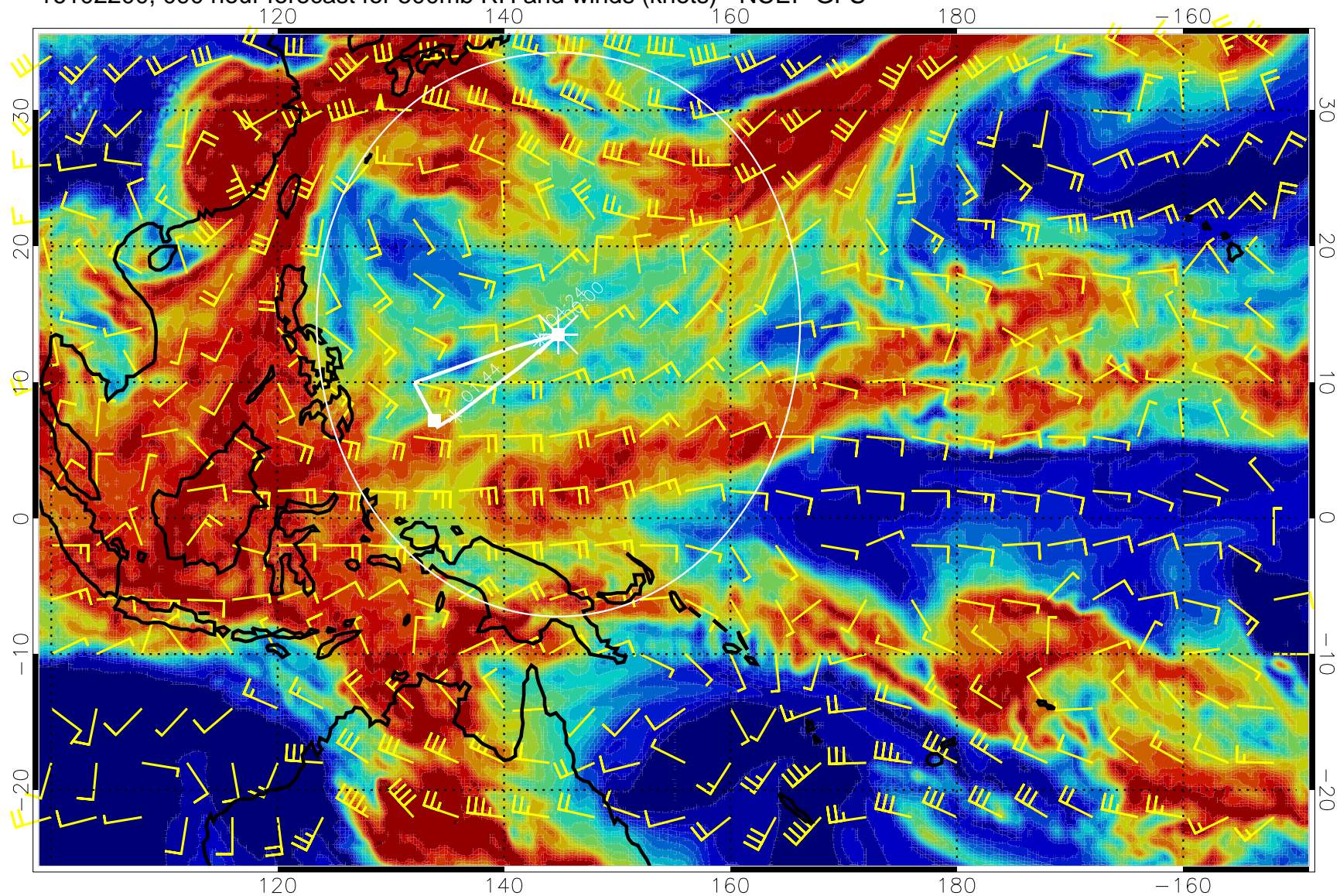
16102200, 090 hour forecast for 500mb RH and winds (knots) - NCEP GFS
