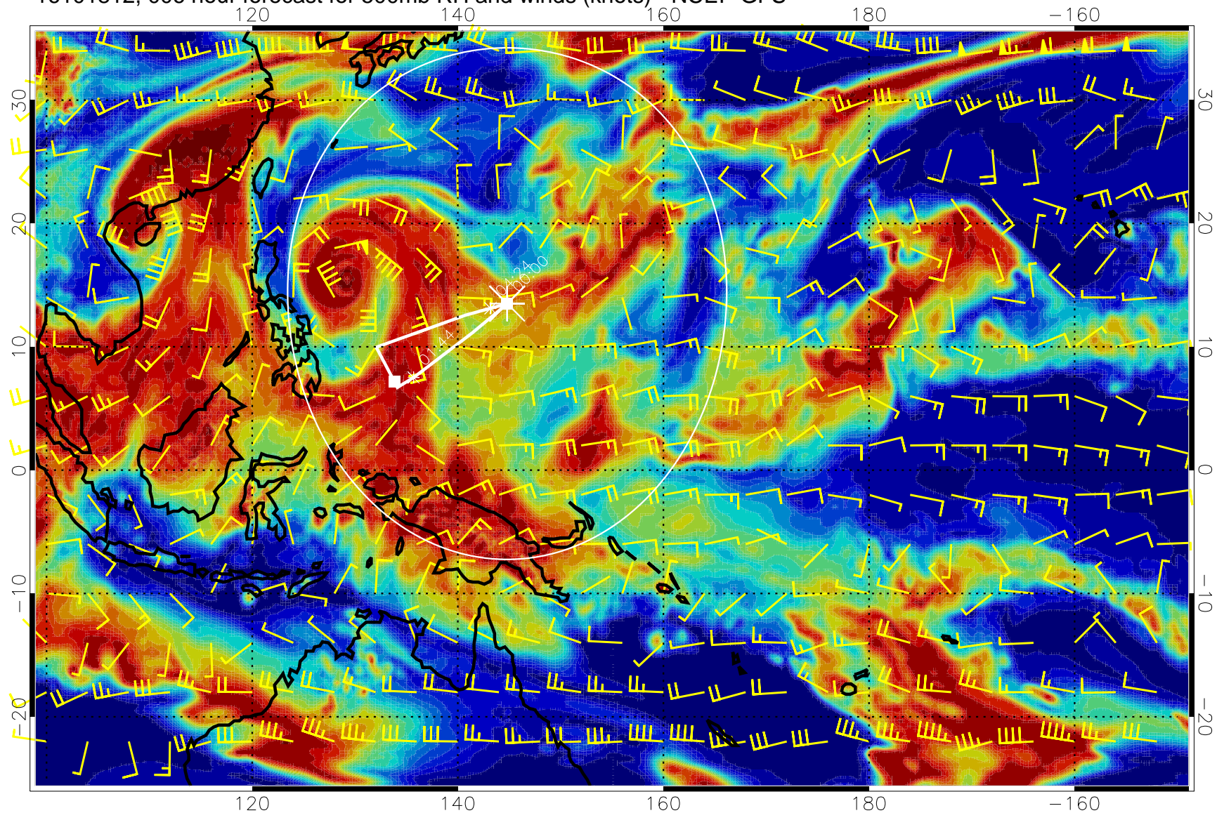
16101812, 006 hour forecast for 500mb RH and winds (knots) - NCEP GFS
