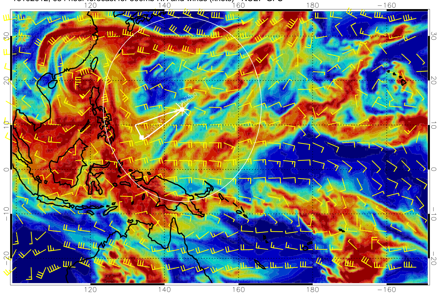
16102012, 054 hour forecast for 500mb RH and winds (knots) - NCEP GFS
