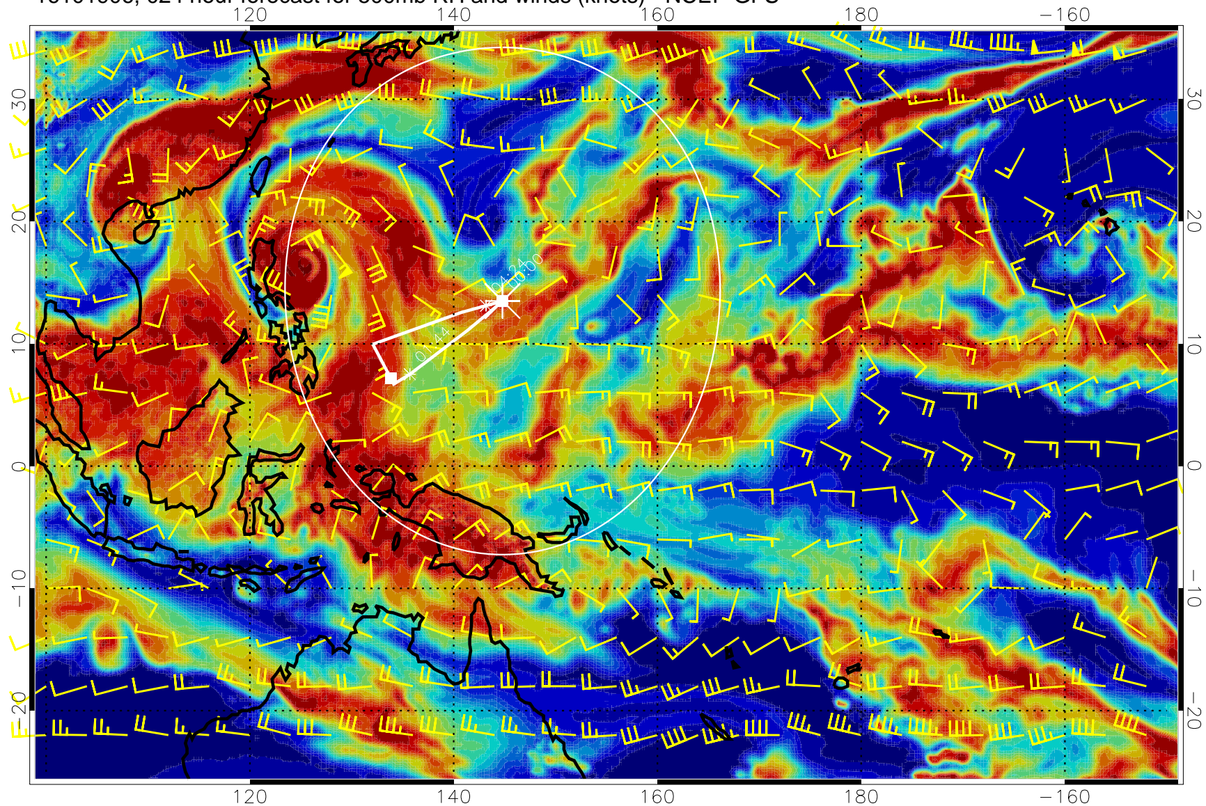
16101906, 024 hour forecast for 500mb RH and winds (knots) - NCEP GFS
