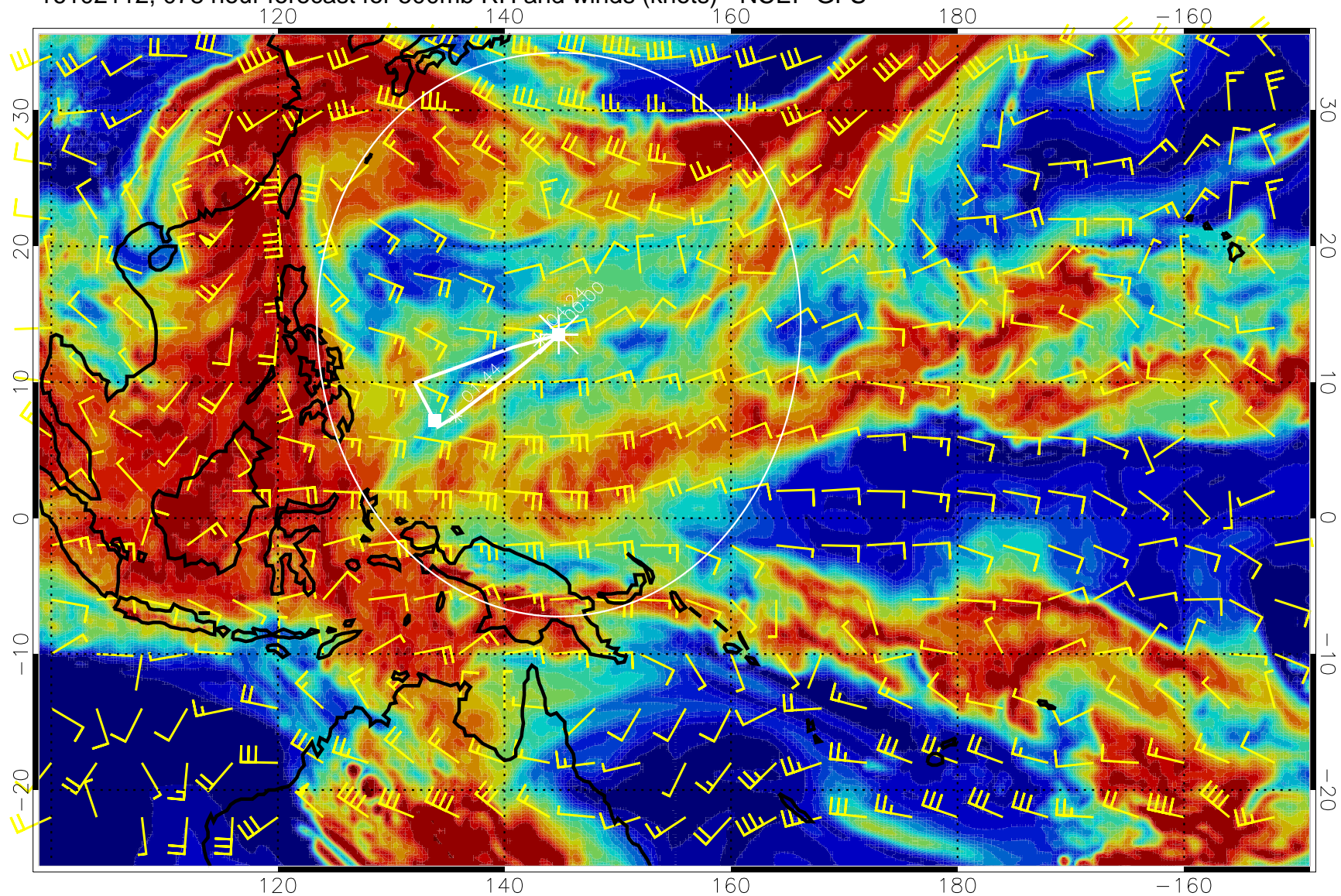
16102112, 078 hour forecast for 500mb RH and winds (knots) - NCEP GFS
