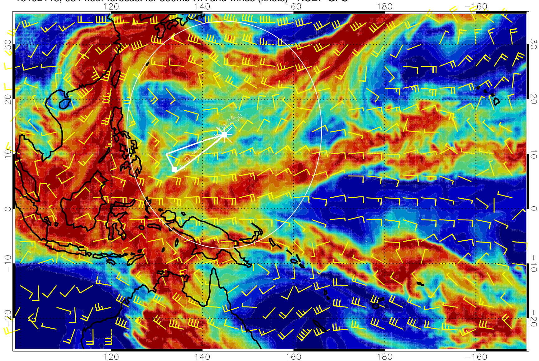
16102118, 084 hour forecast for 500mb RH and winds (knots) - NCEP GFS
