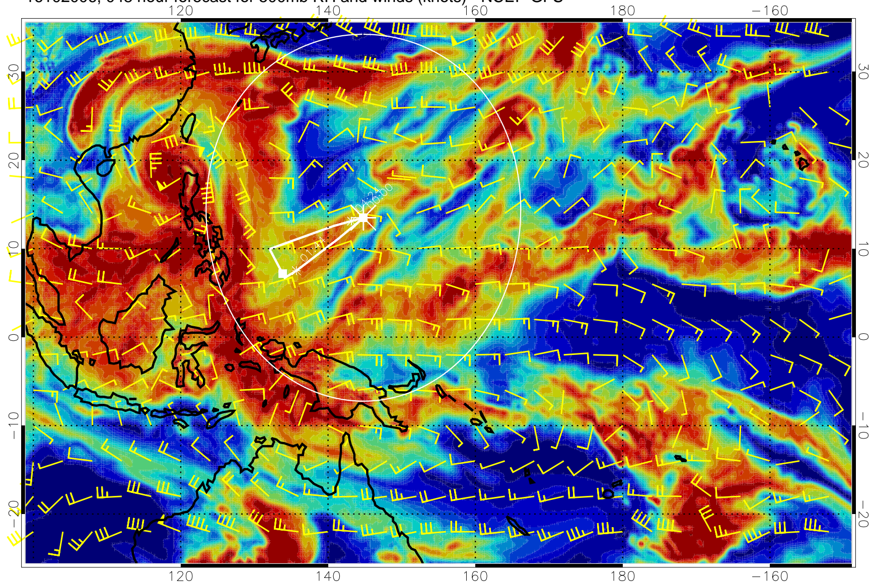
16102006, 048 hour forecast for 500mb RH and winds (knots) - NCEP GFS
