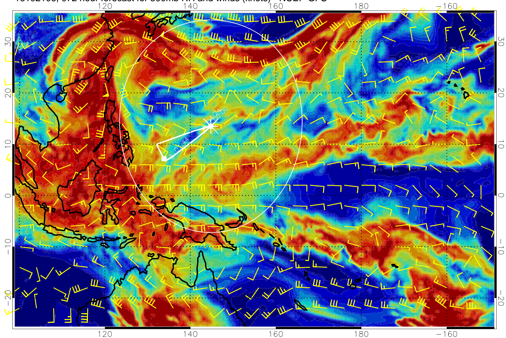
16102106, 072 hour forecast for 500mb RH and winds (knots) - NCEP GFS
