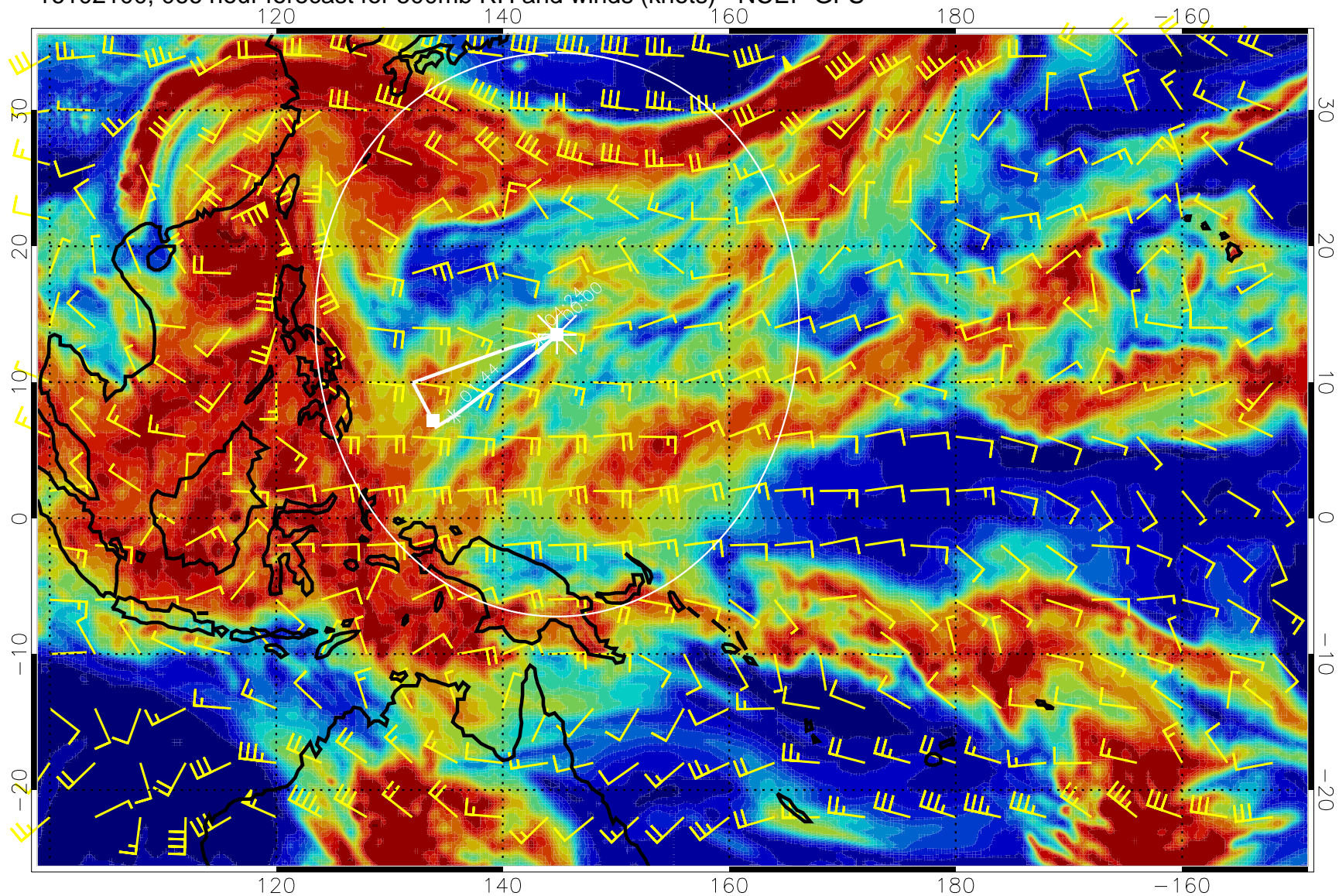
16102100, 066 hour forecast for 500mb RH and winds (knots) - NCEP GFS
