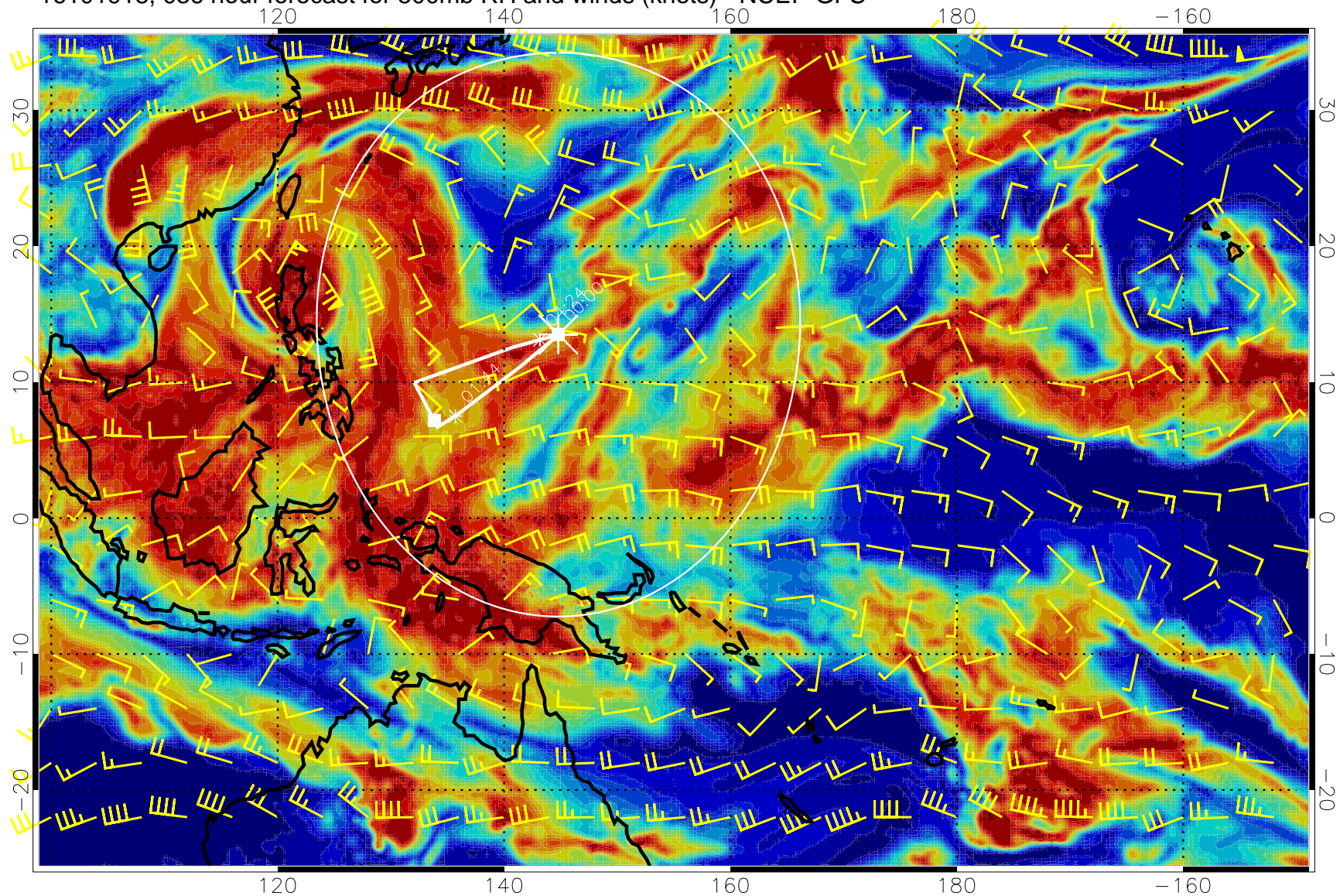
16101918, 036 hour forecast for 500mb RH and winds (knots) - NCEP GFS
