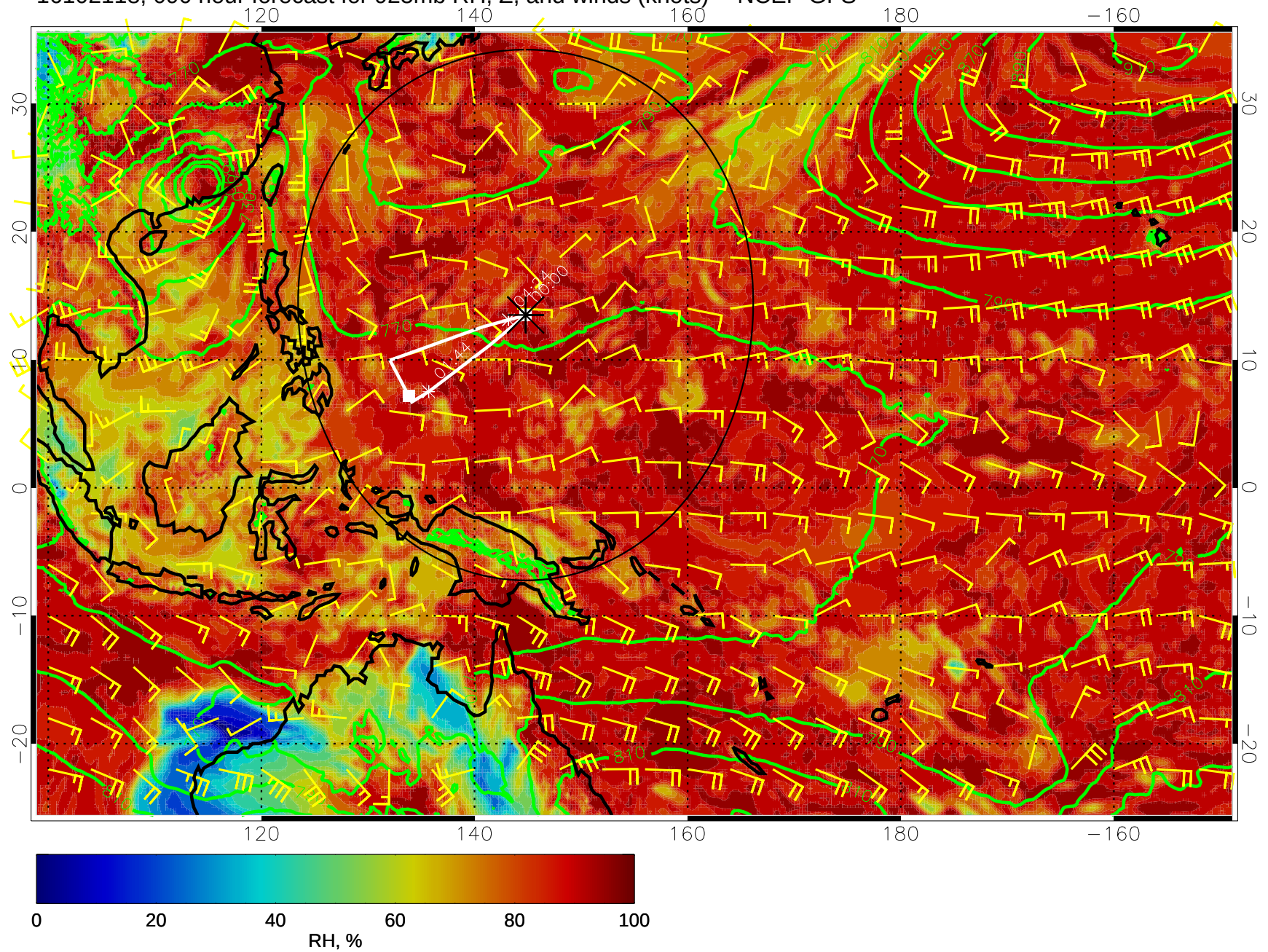
16102118, 090 hour forecast for 925mb RH, Z, and winds (knots) -- NCEP GFS
