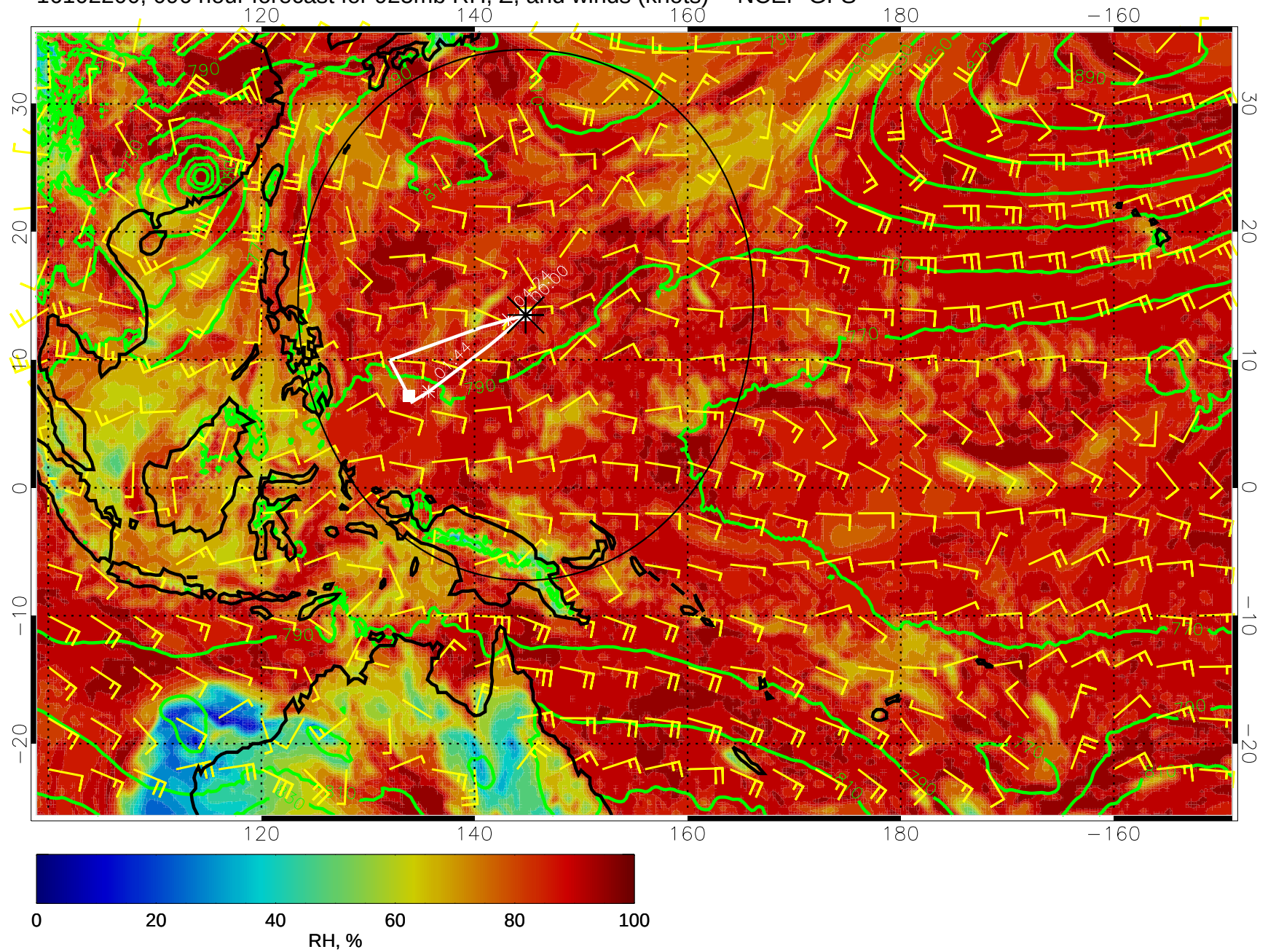
16102200, 096 hour forecast for 925mb RH, Z, and winds (knots) -- NCEP GFS
