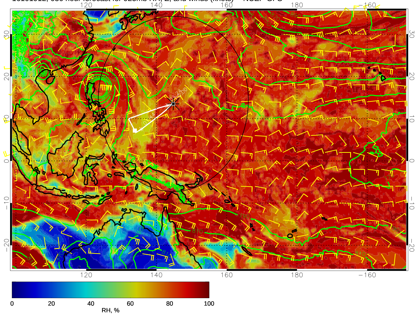
16101912, 036 hour forecast for 925mb RH, Z, and winds (knots) -- NCEP GFS
