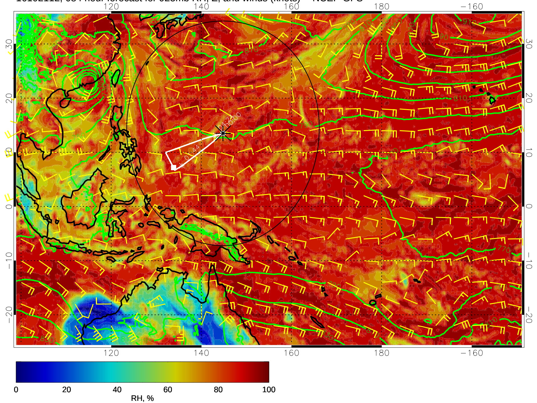
16102112, 084 hour forecast for 925mb RH, Z, and winds (knots) -- NCEP GFS
