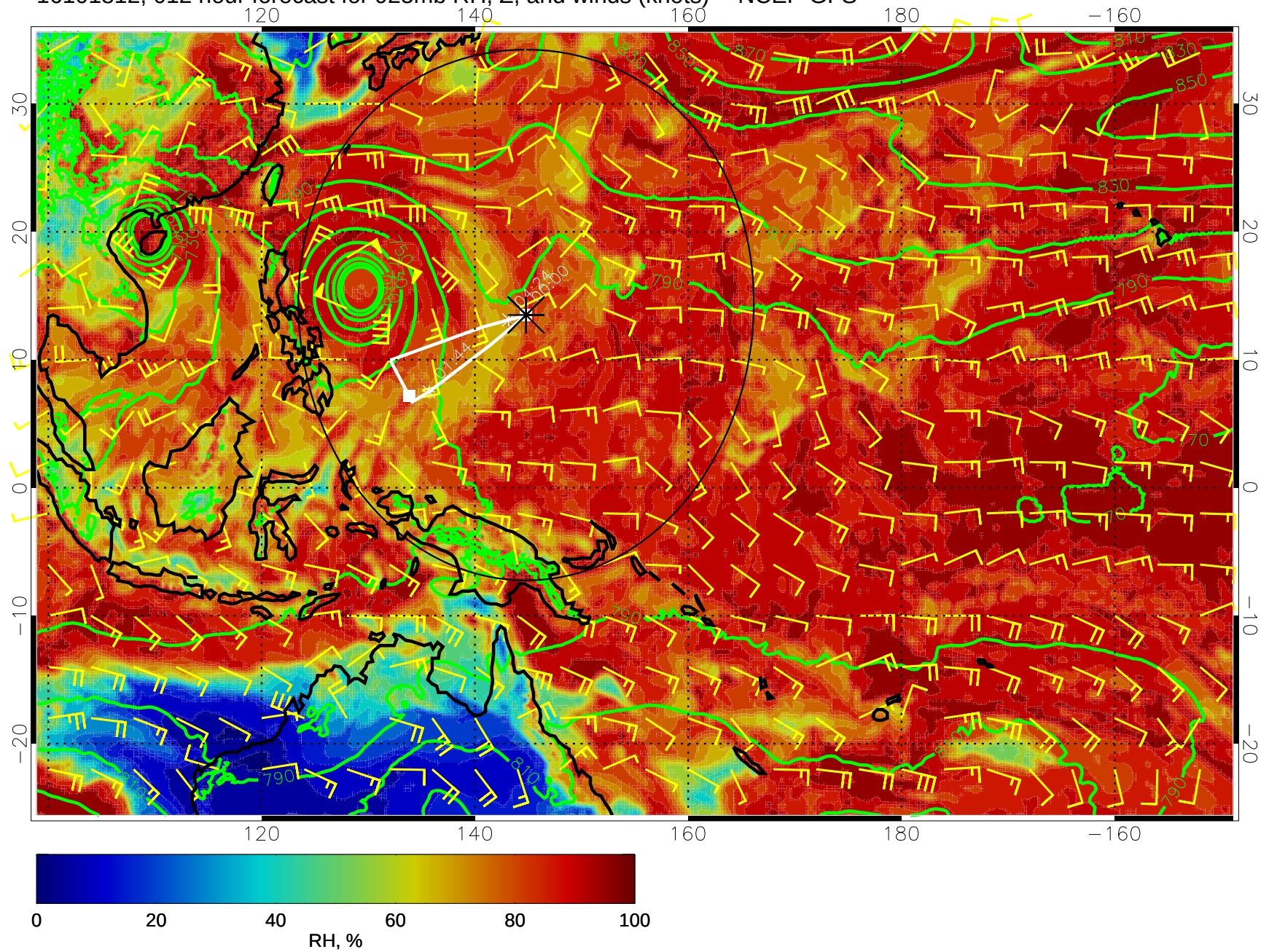
16101812, 012 hour forecast for 925mb RH, Z, and winds (knots) -- NCEP GFS
