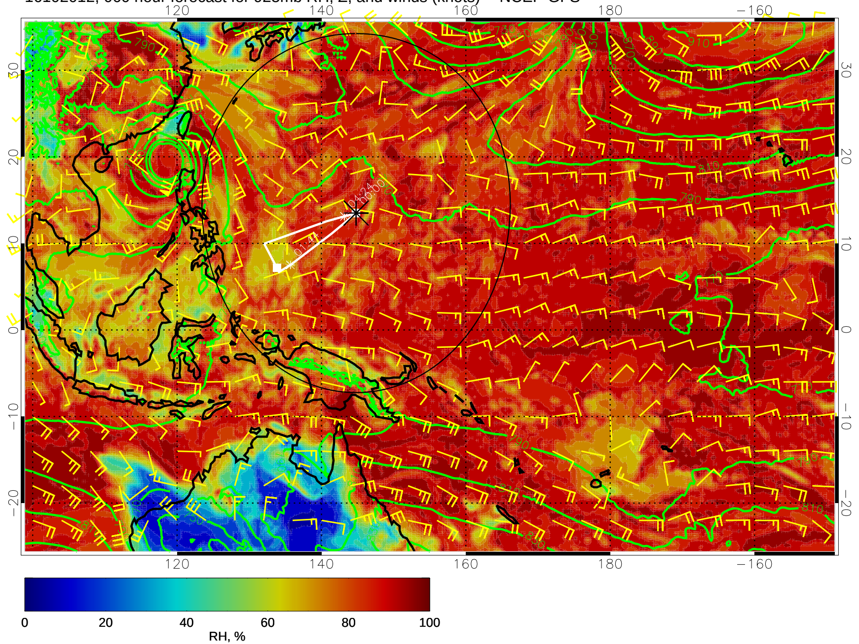
16102012, 060 hour forecast for 925mb RH, Z, and winds (knots) -- NCEP GFS
