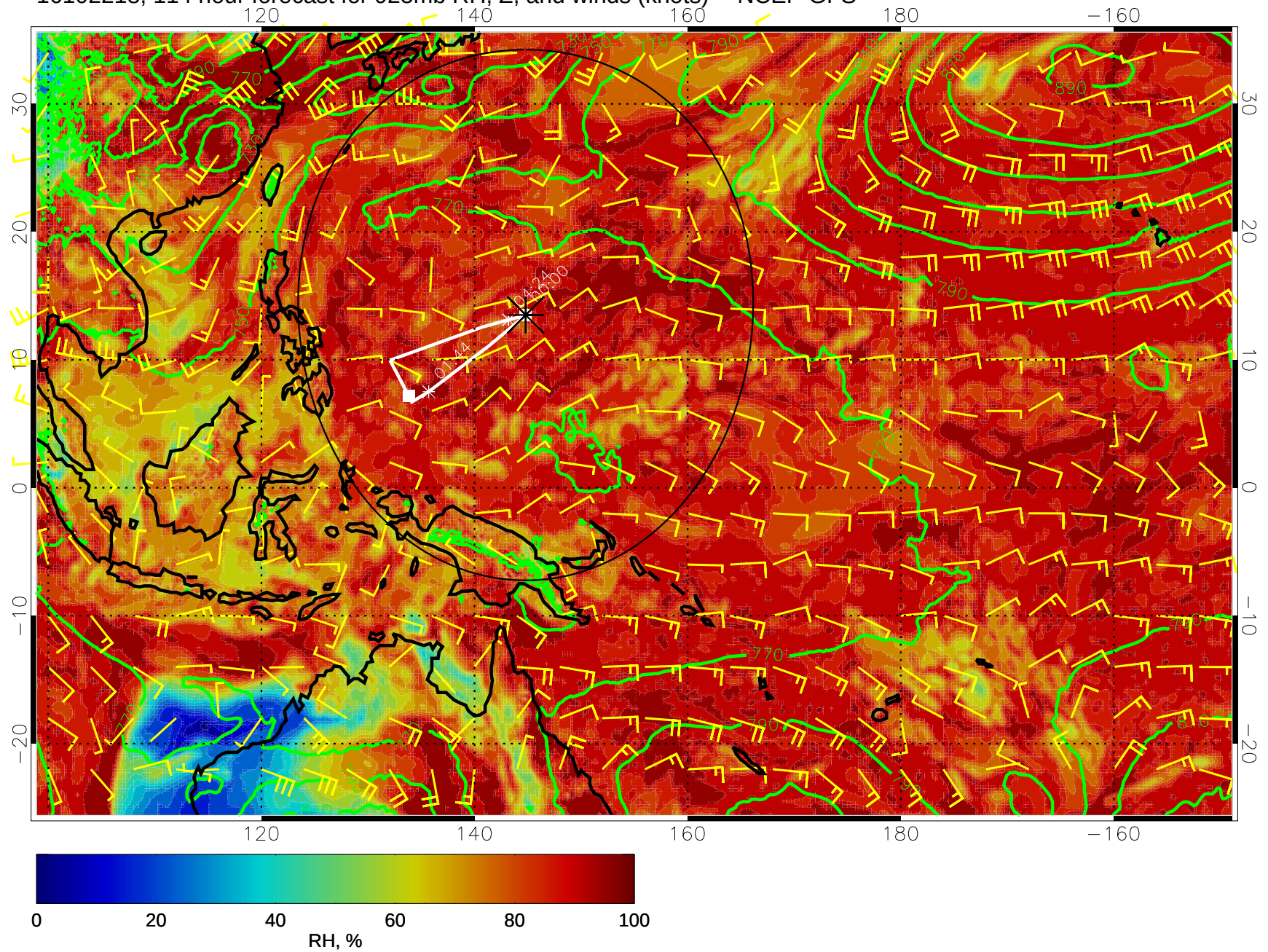
16102218, 114 hour forecast for 925mb RH, Z, and winds (knots) -- NCEP GFS
