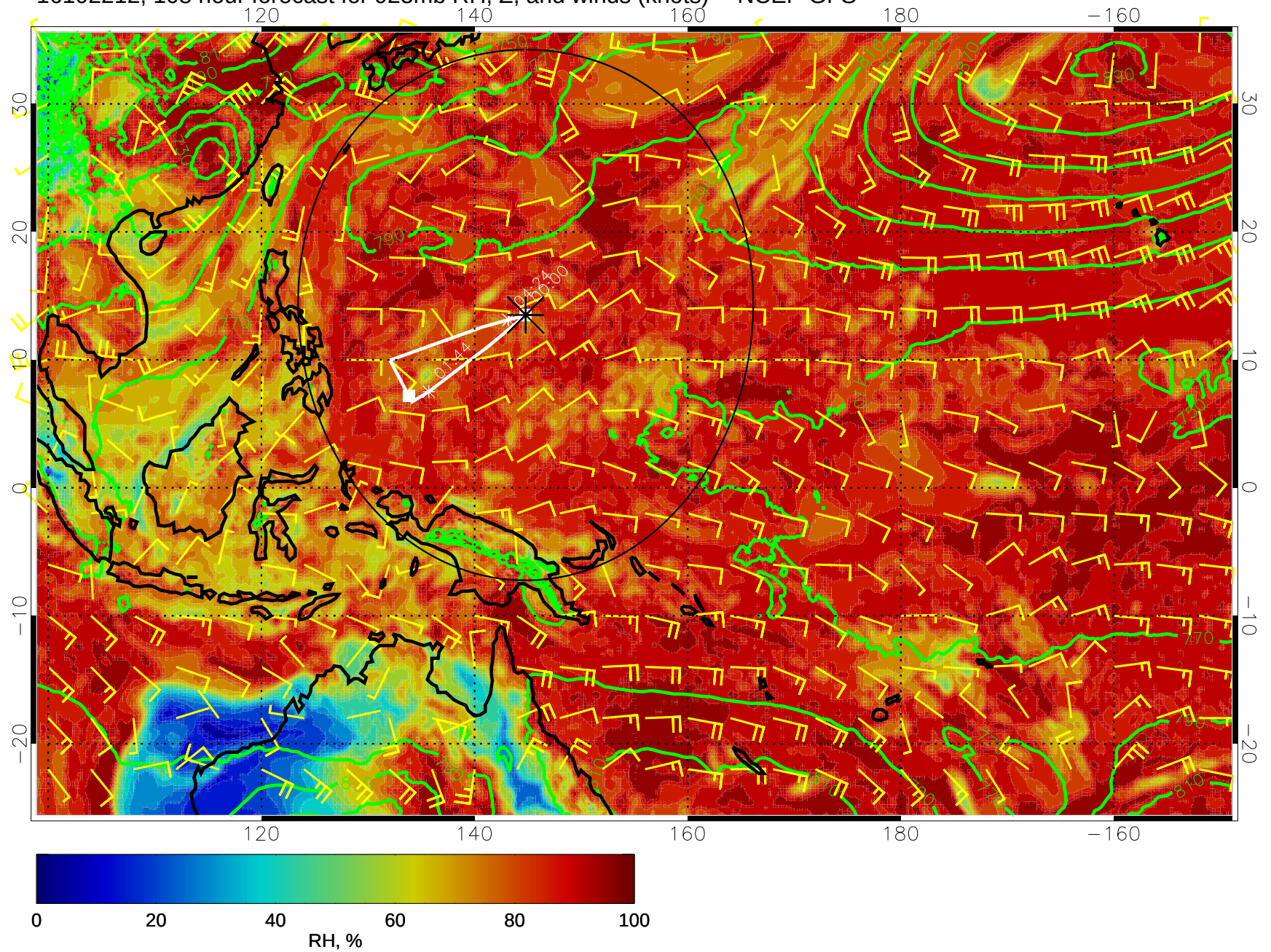
16102212, 108 hour forecast for 925mb RH, Z, and winds (knots) -- NCEP GFS
