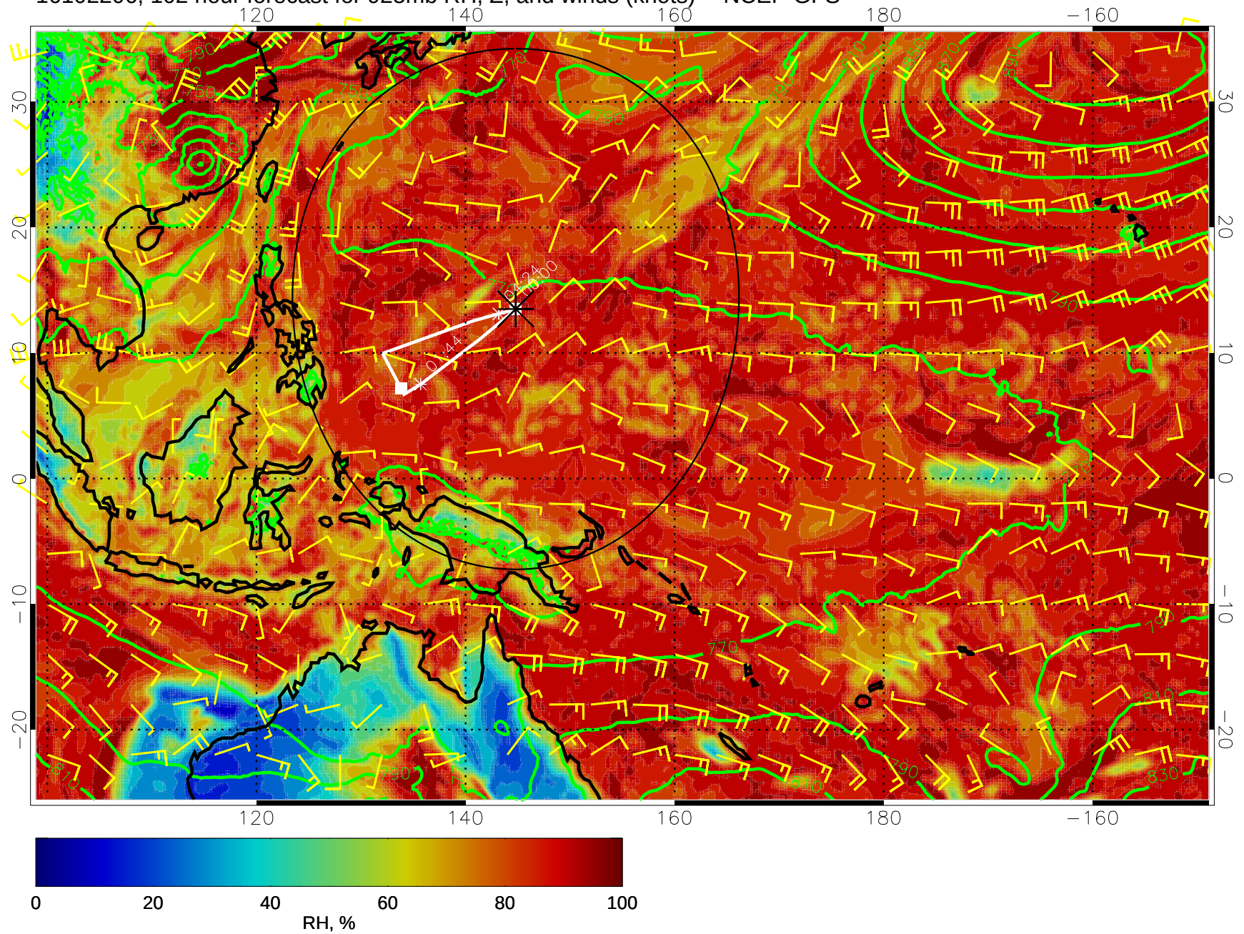
16102206, 102 hour forecast for 925mb RH, Z, and winds (knots) -- NCEP GFS
