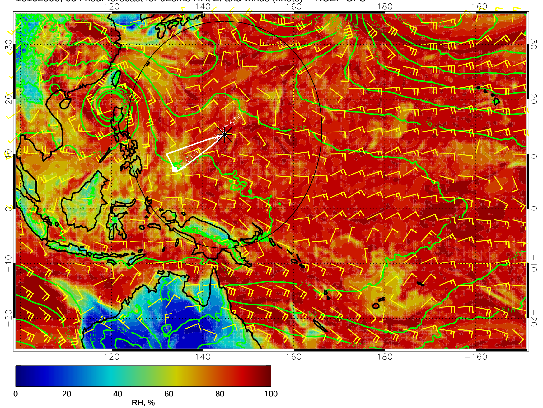
16102006, 054 hour forecast for 925mb RH, Z, and winds (knots) -- NCEP GFS
