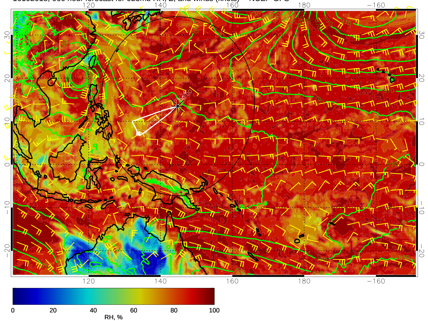
16102018, 066 hour forecast for 925mb RH, Z, and winds (knots) -- NCEP GFS
