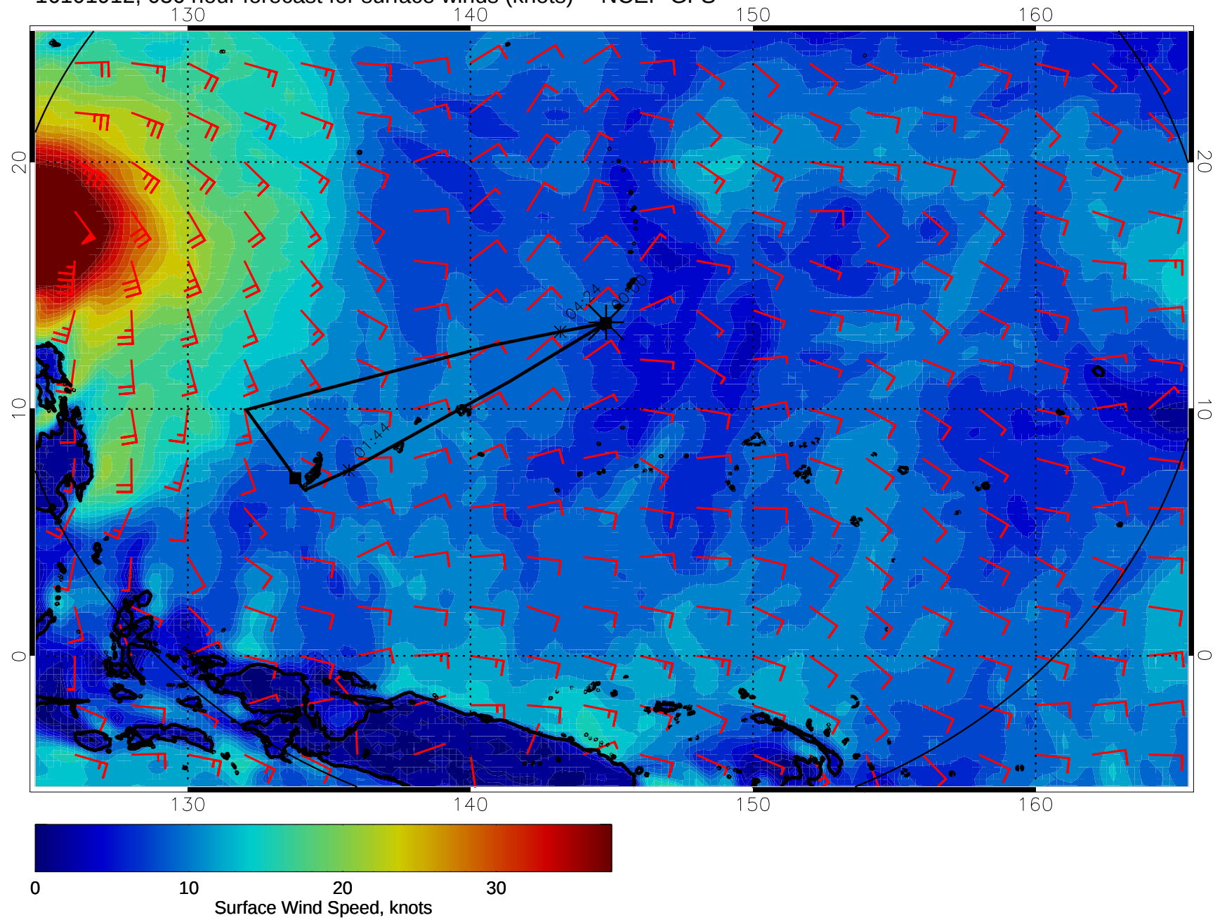
16101912, 036 hour forecast for surface winds (knots) -- NCEP GFS
