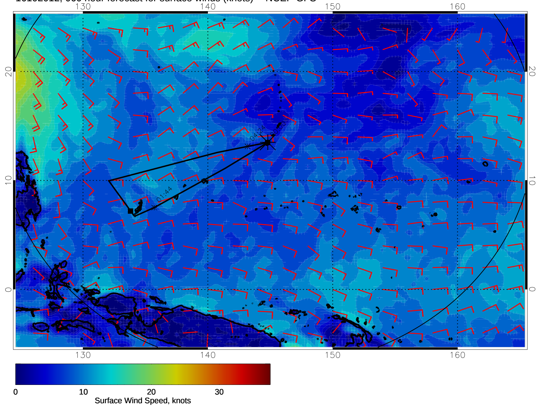
16102012, 060 hour forecast for surface winds (knots) -- NCEP GFS
