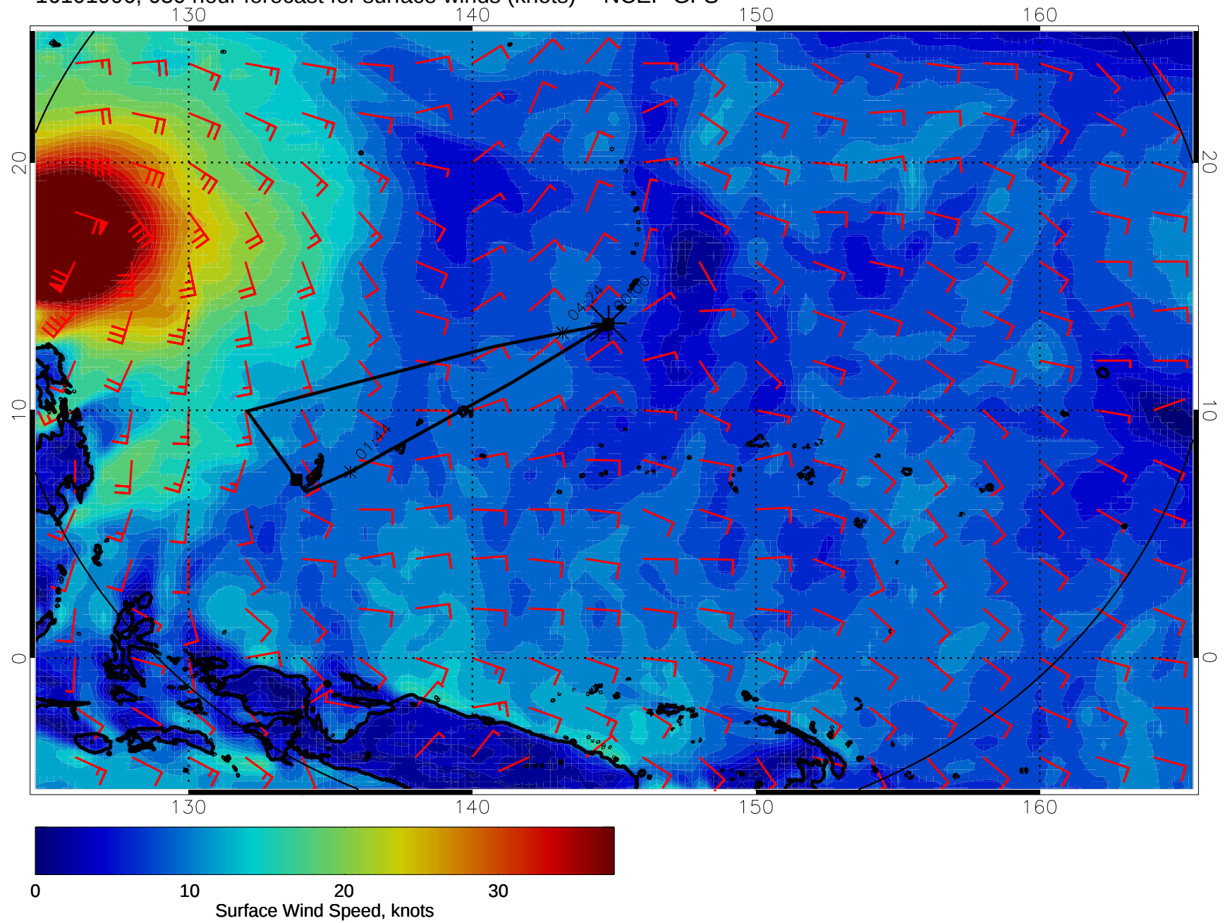
16101906, 030 hour forecast for surface winds (knots) -- NCEP GFS
