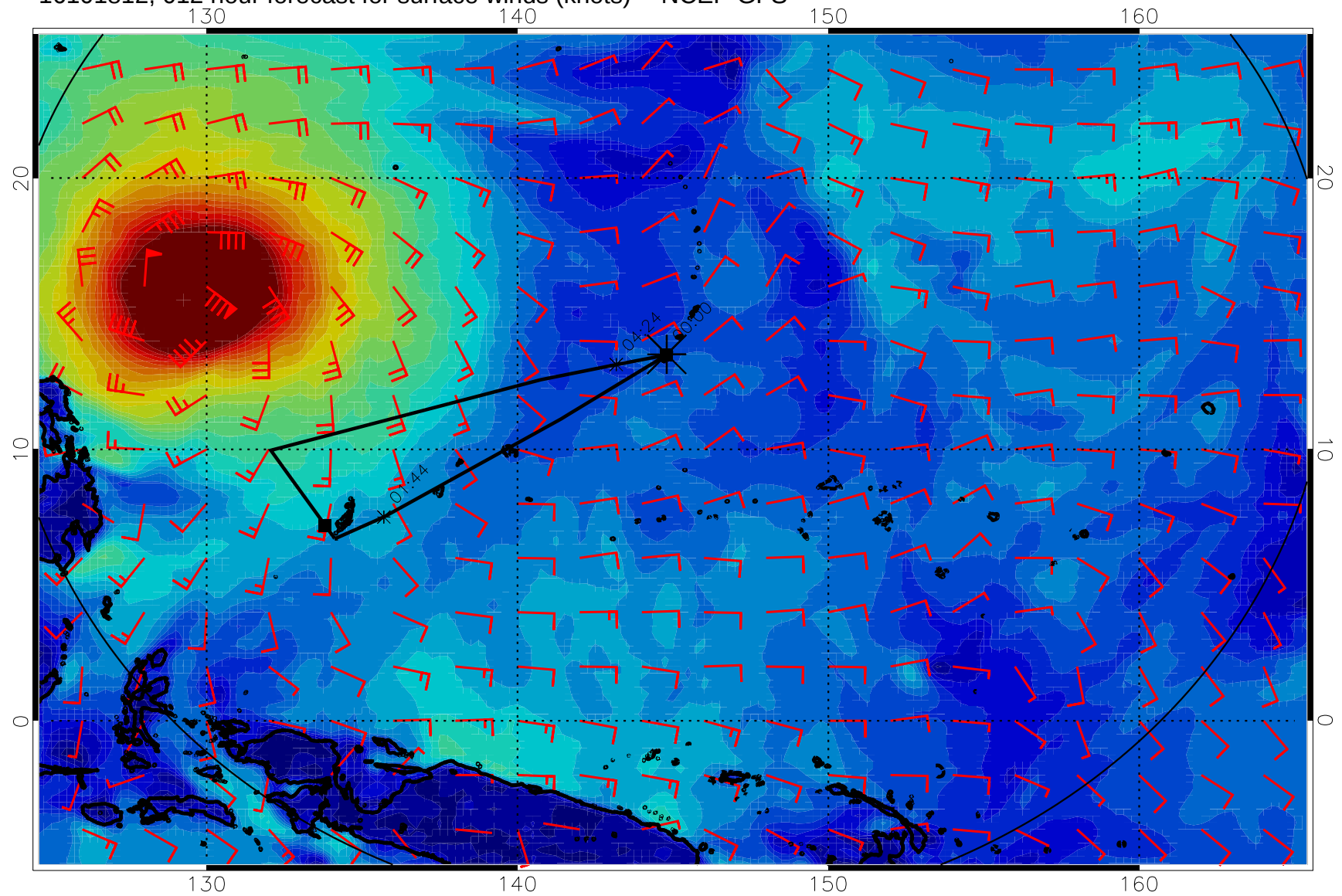
16101812, 012 hour forecast for surface winds (knots) -- NCEP GFS
