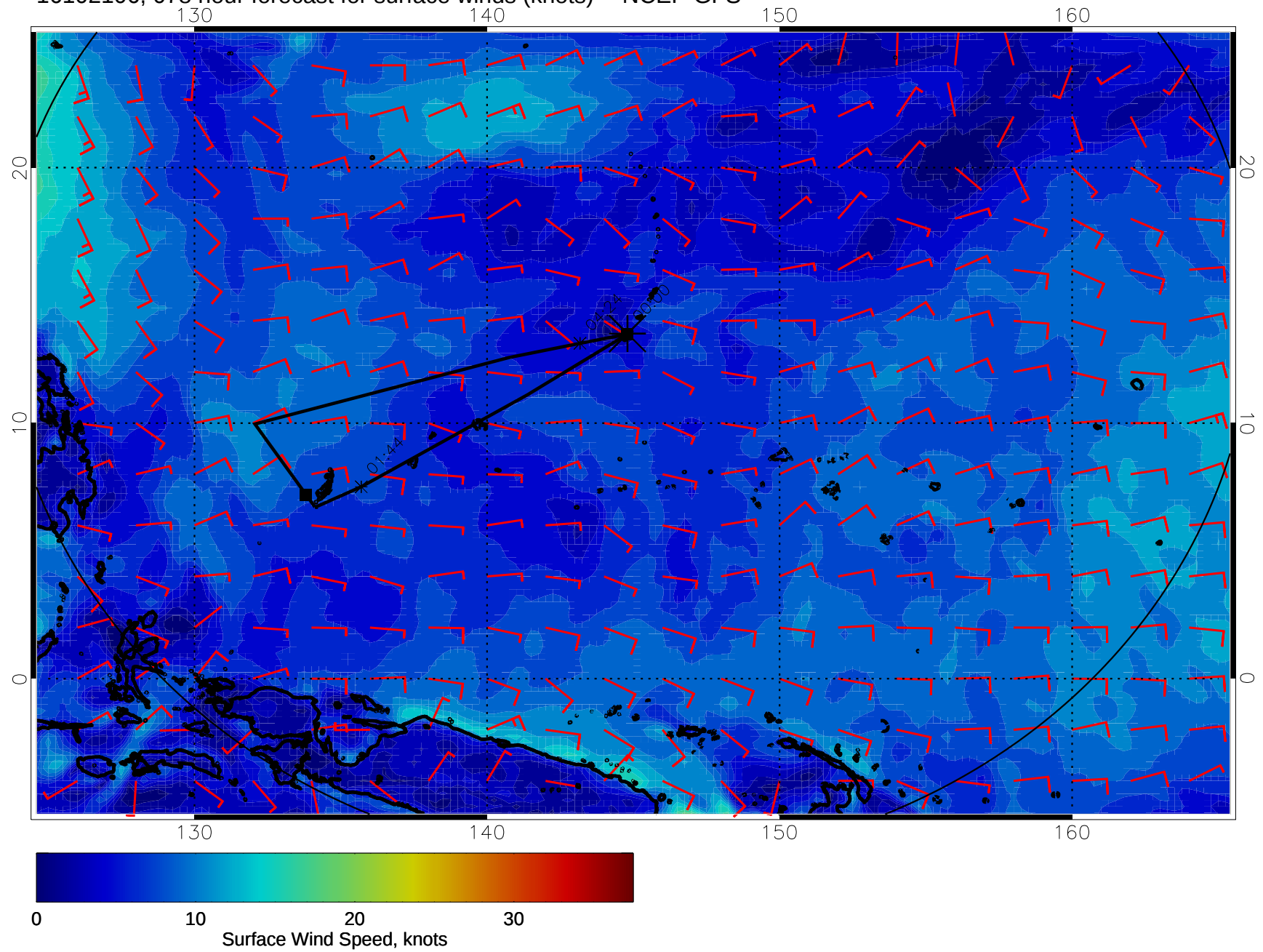
16102106, 078 hour forecast for surface winds (knots) -- NCEP GFS
