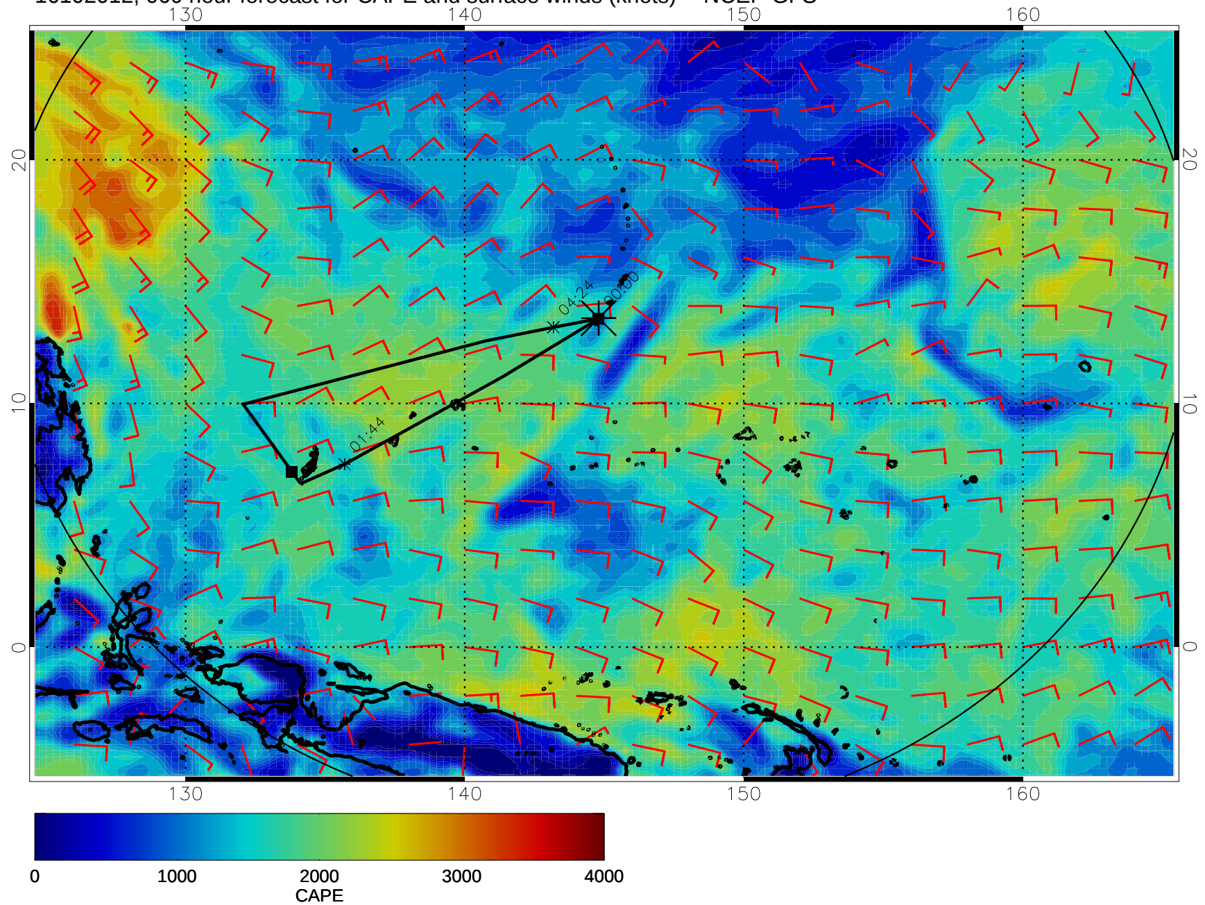
16102012, 060 hour forecast for CAPE and surface winds (knots) -- NCEP GFS
