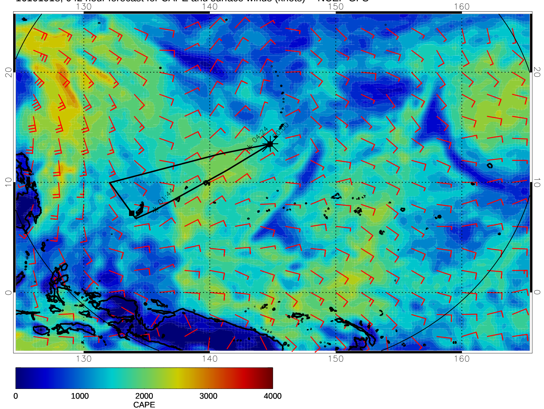
16101918, 042 hour forecast for CAPE and surface winds (knots) -- NCEP GFS
