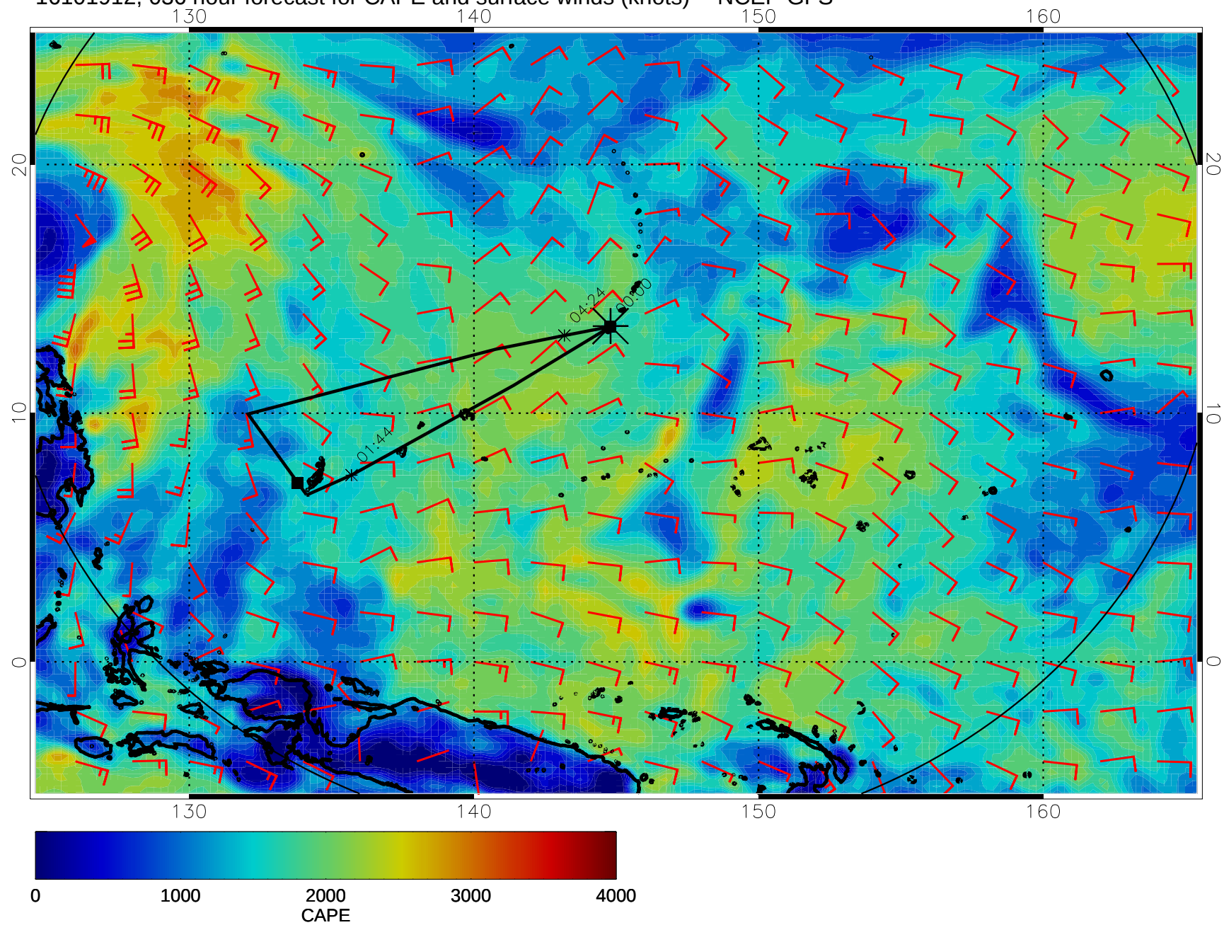
16101912, 036 hour forecast for CAPE and surface winds (knots) -- NCEP GFS
