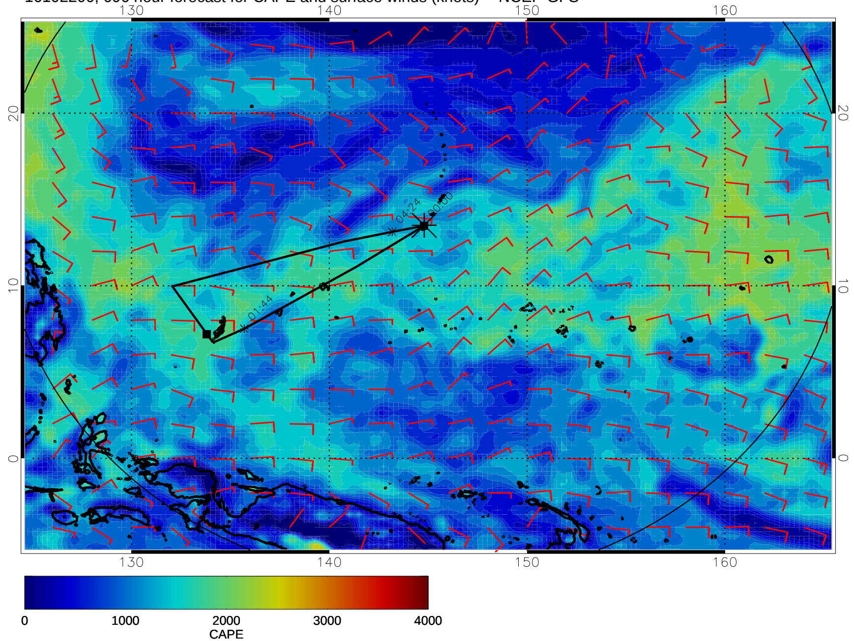
16102200, 096 hour forecast for CAPE and surface winds (knots) -- NCEP GFS
