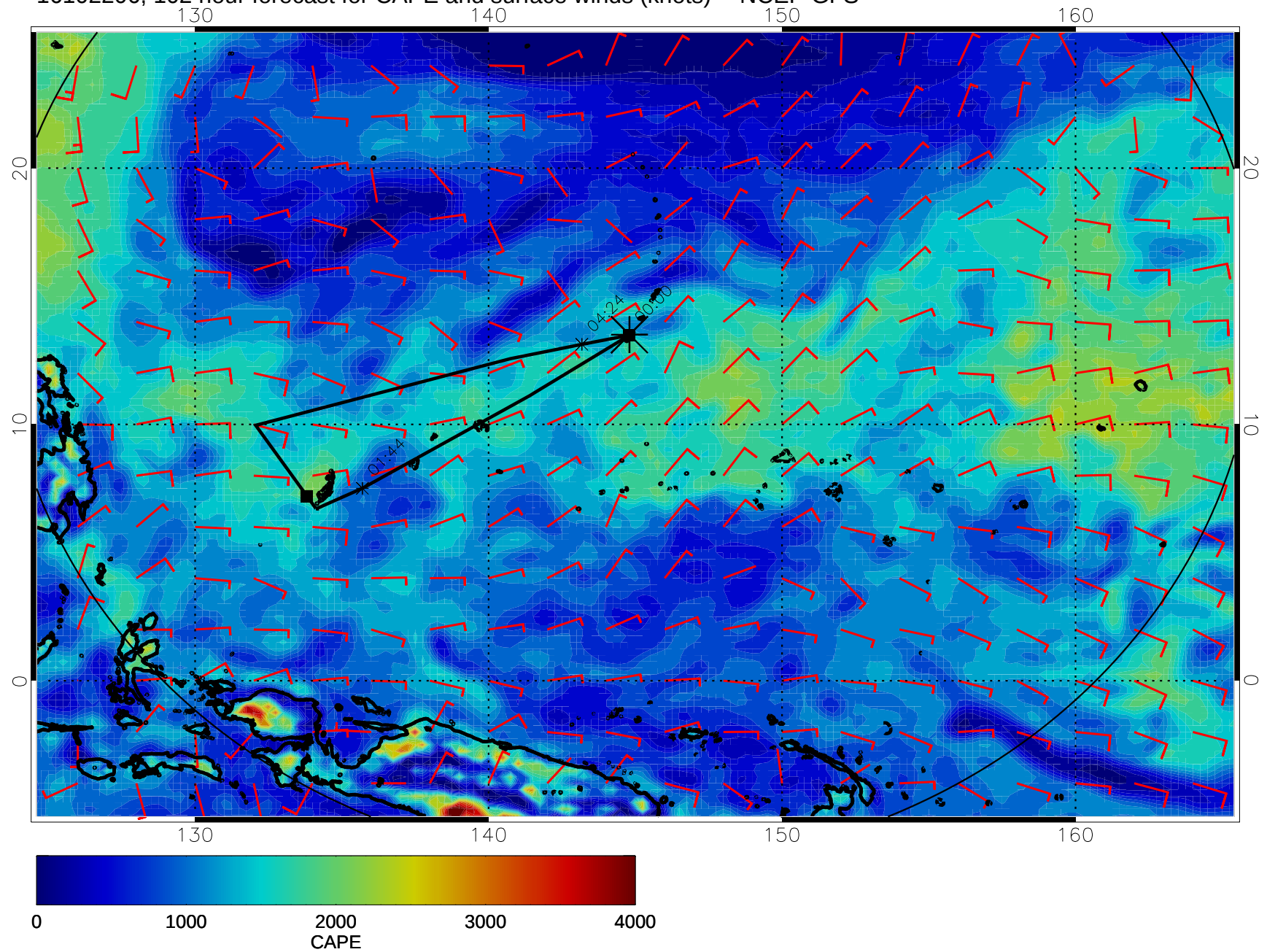
16102206, 102 hour forecast for CAPE and surface winds (knots) -- NCEP GFS
