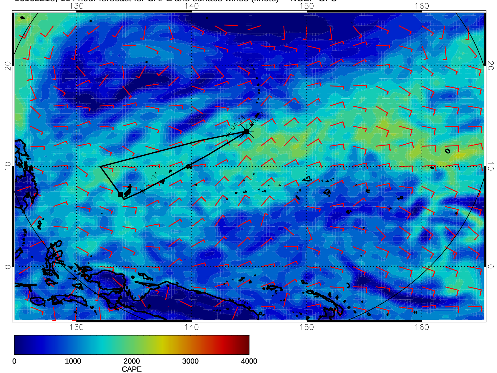
16102218, 114 hour forecast for CAPE and surface winds (knots) -- NCEP GFS
