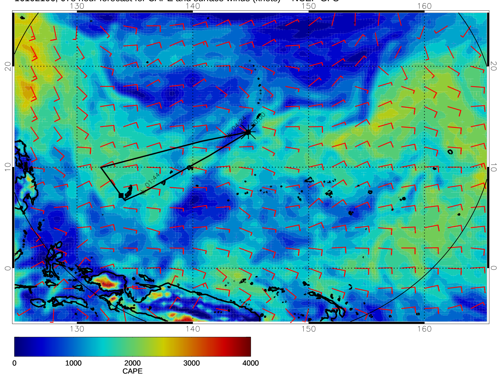
16102106, 078 hour forecast for CAPE and surface winds (knots) -- NCEP GFS
