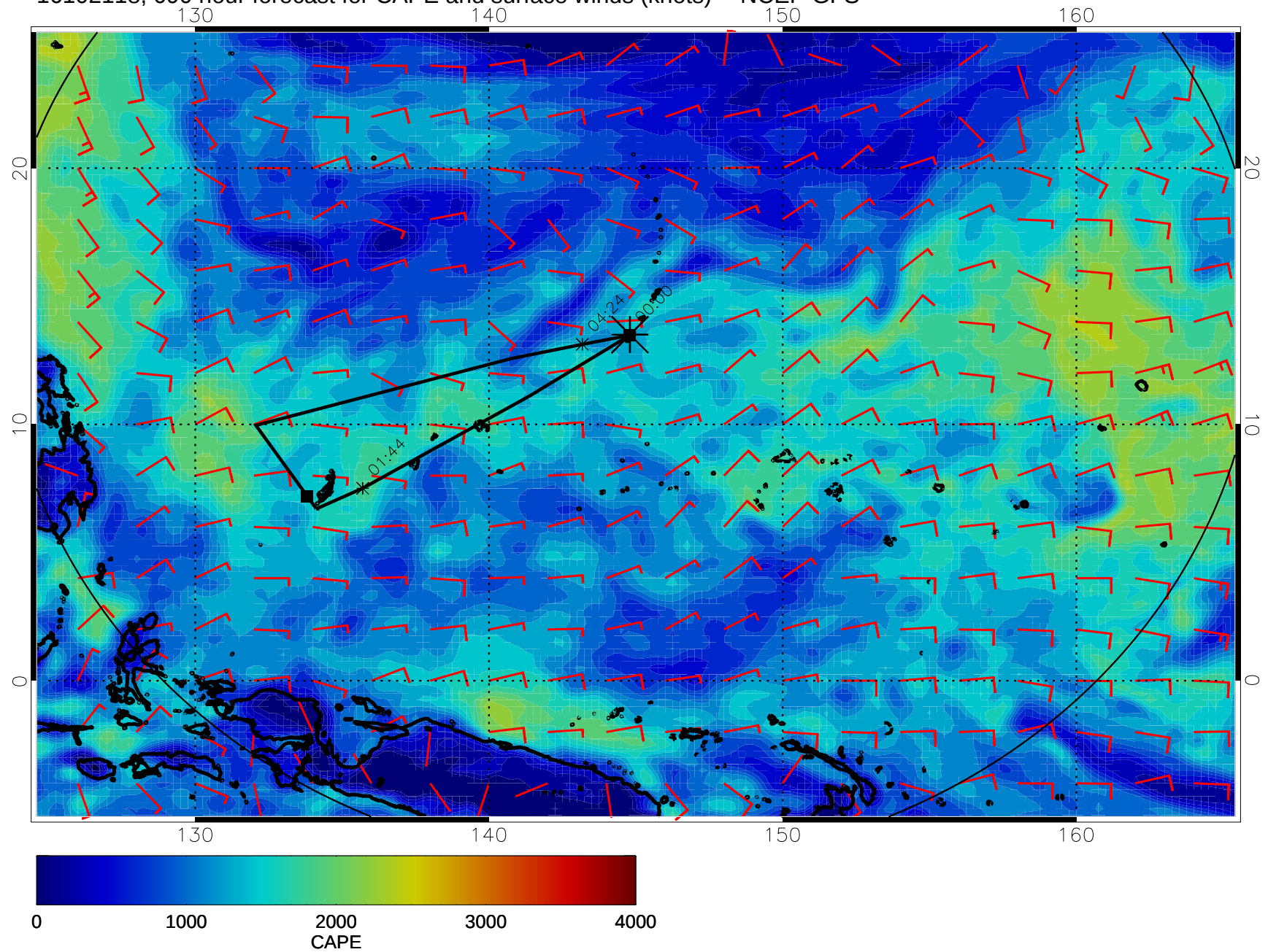
16102118, 090 hour forecast for CAPE and surface winds (knots) -- NCEP GFS
