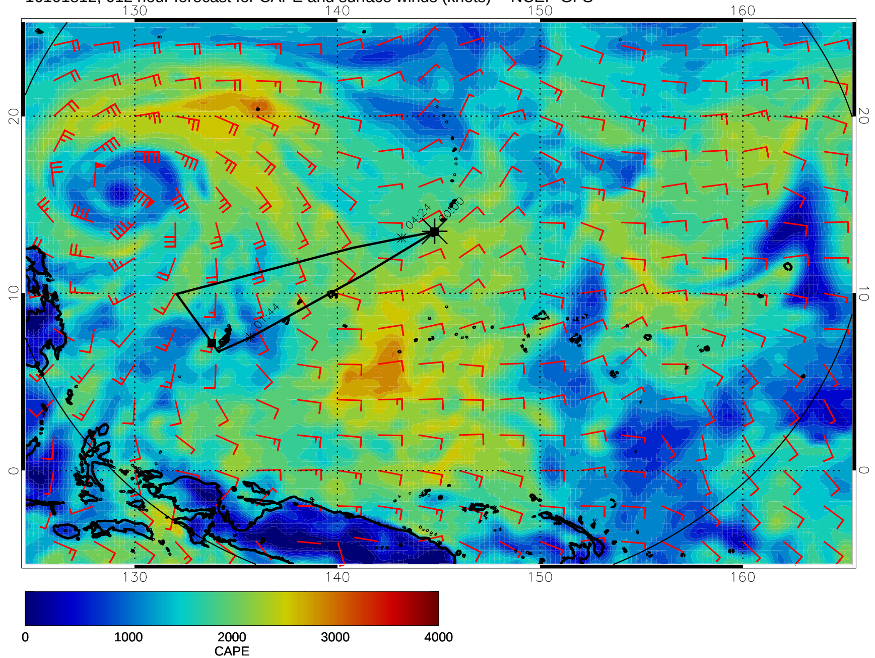
16101812, 012 hour forecast for CAPE and surface winds (knots) -- NCEP GFS
