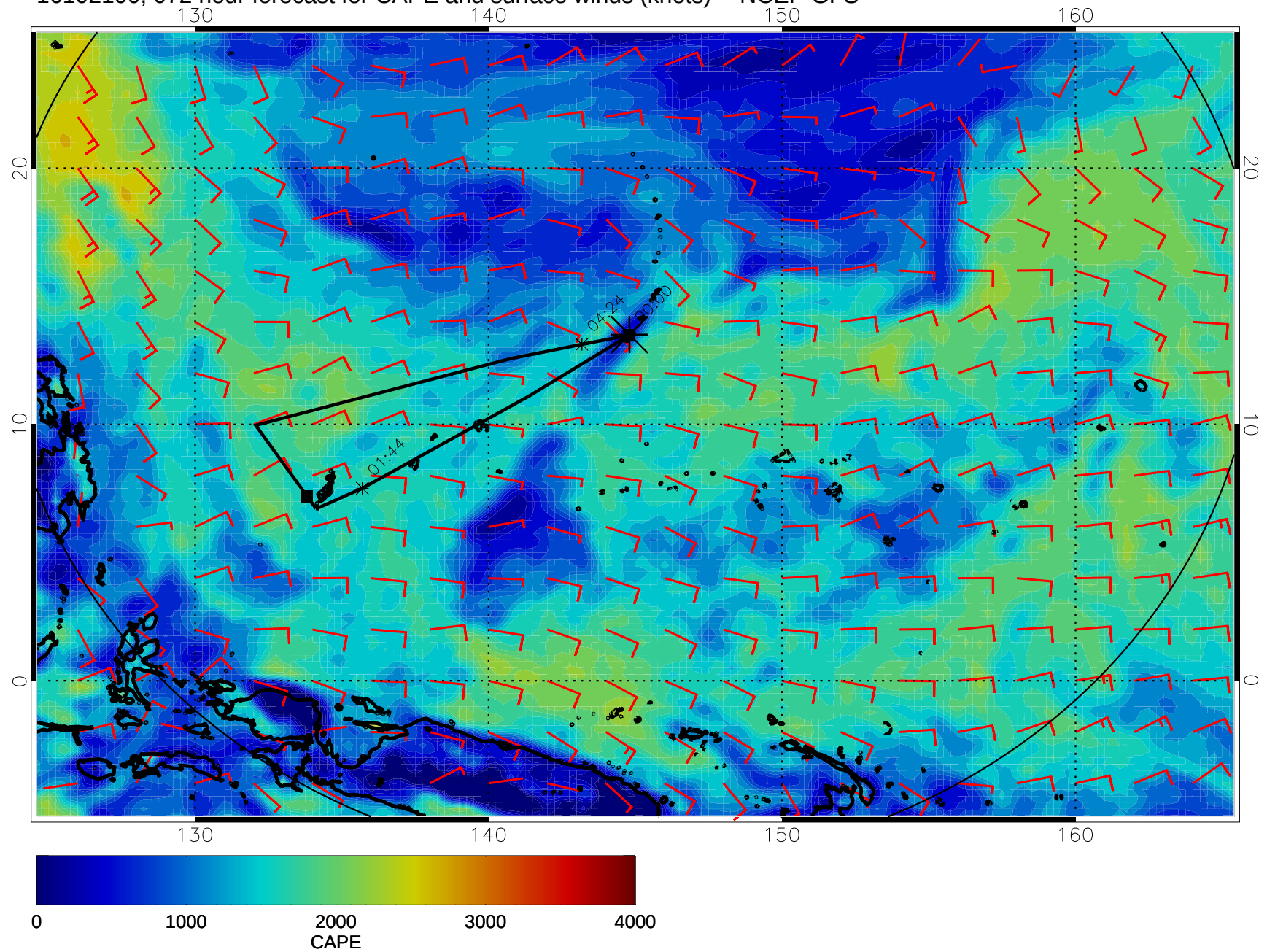
16102100, 072 hour forecast for CAPE and surface winds (knots) -- NCEP GFS
