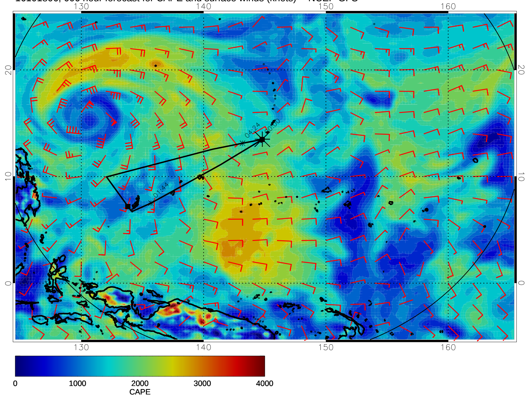
16101806, 006 hour forecast for CAPE and surface winds (knots) -- NCEP GFS
