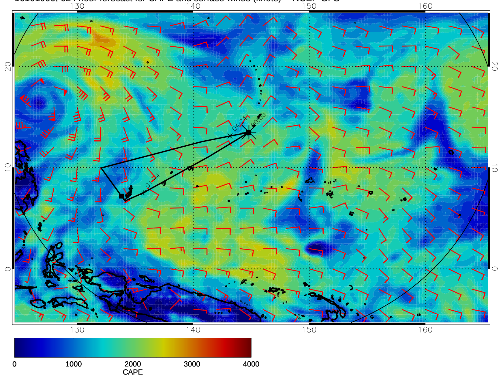
16101900, 024 hour forecast for CAPE and surface winds (knots) -- NCEP GFS
