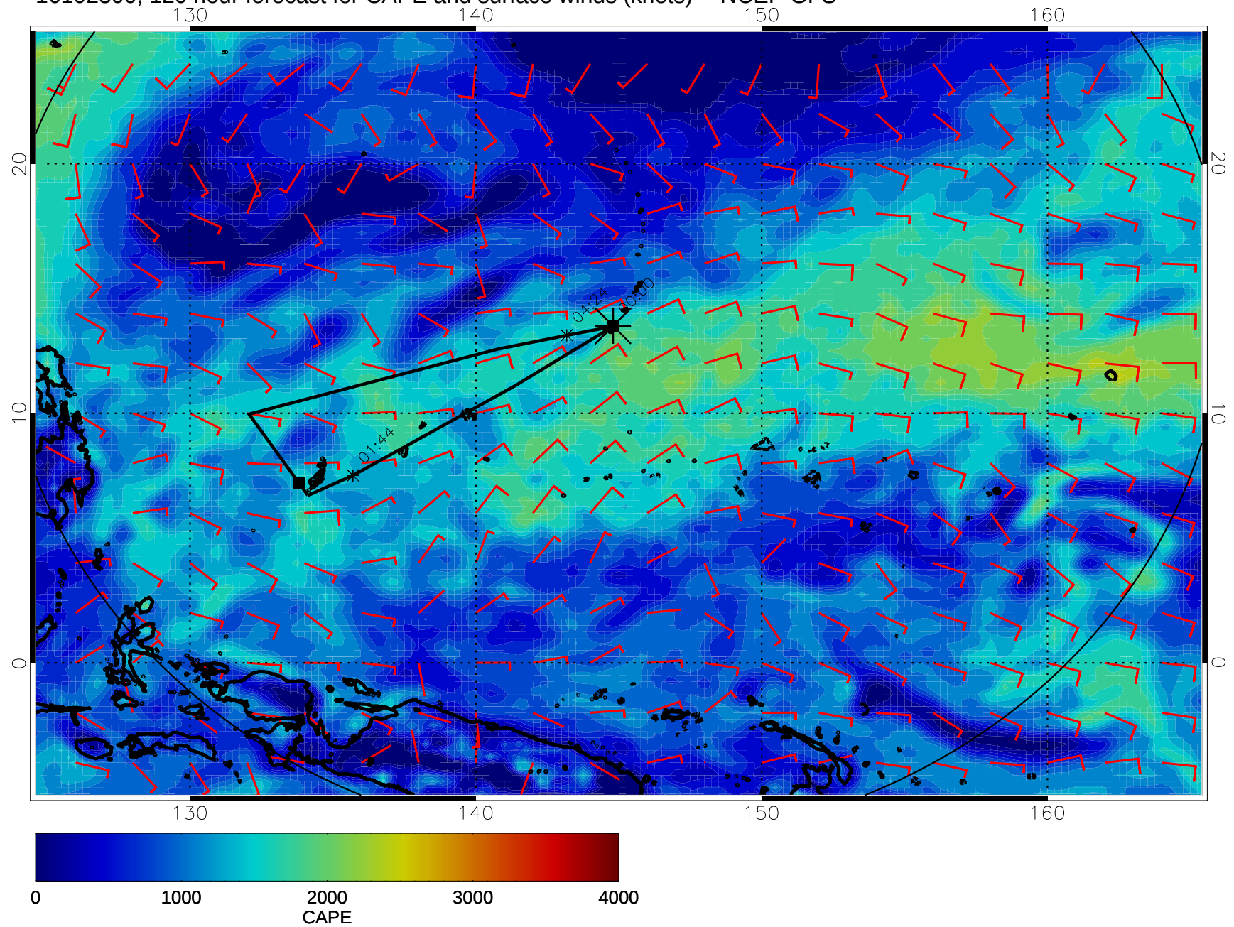
16102300, 120 hour forecast for CAPE and surface winds (knots) -- NCEP GFS
