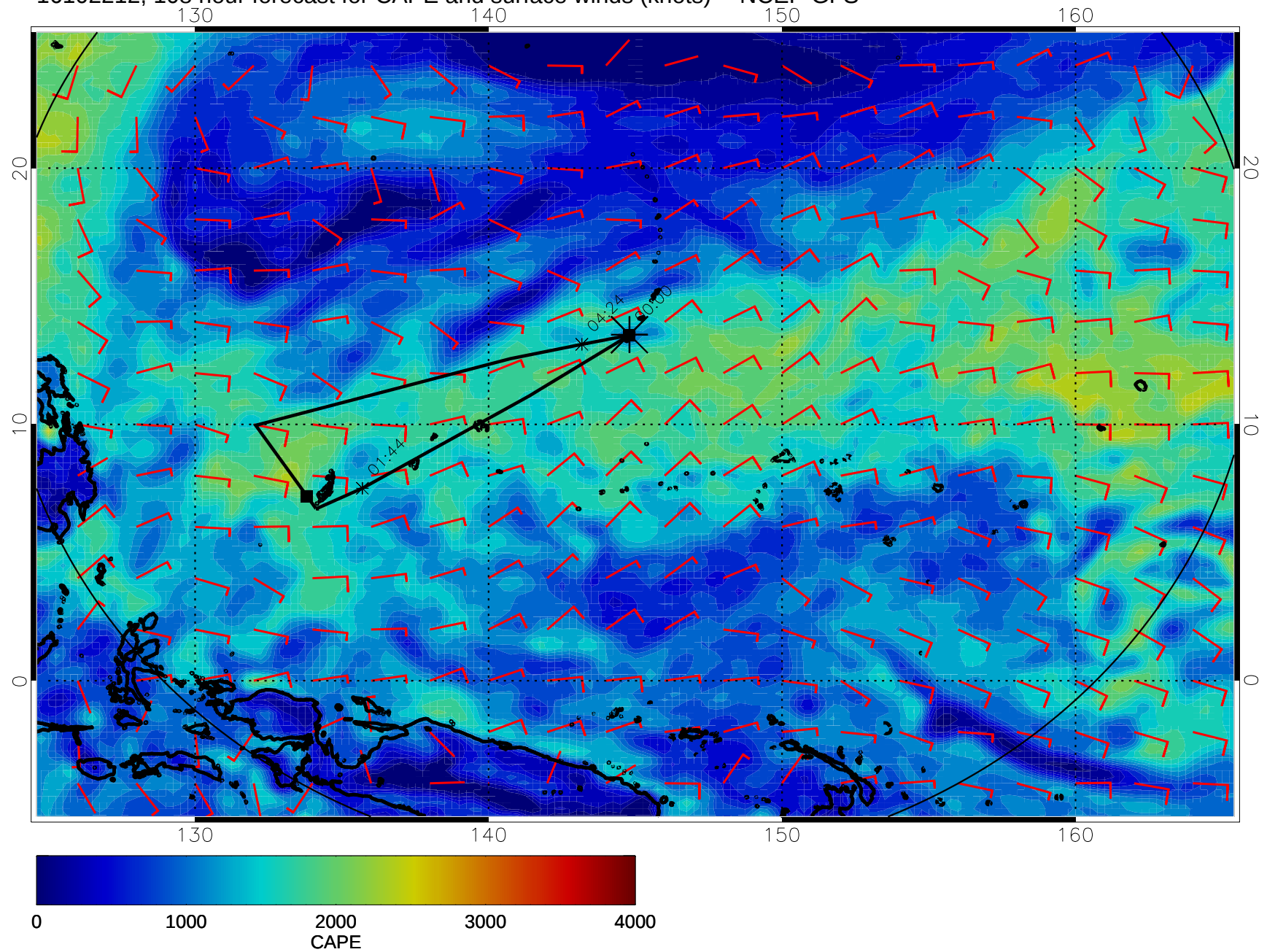
16102212, 108 hour forecast for CAPE and surface winds (knots) -- NCEP GFS
