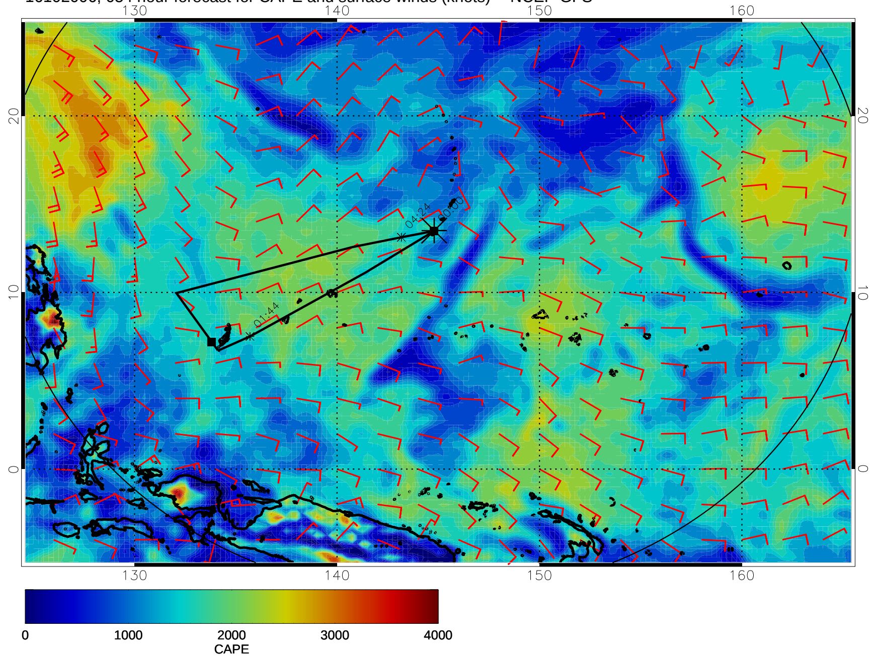
16102006, 054 hour forecast for CAPE and surface winds (knots) -- NCEP GFS
