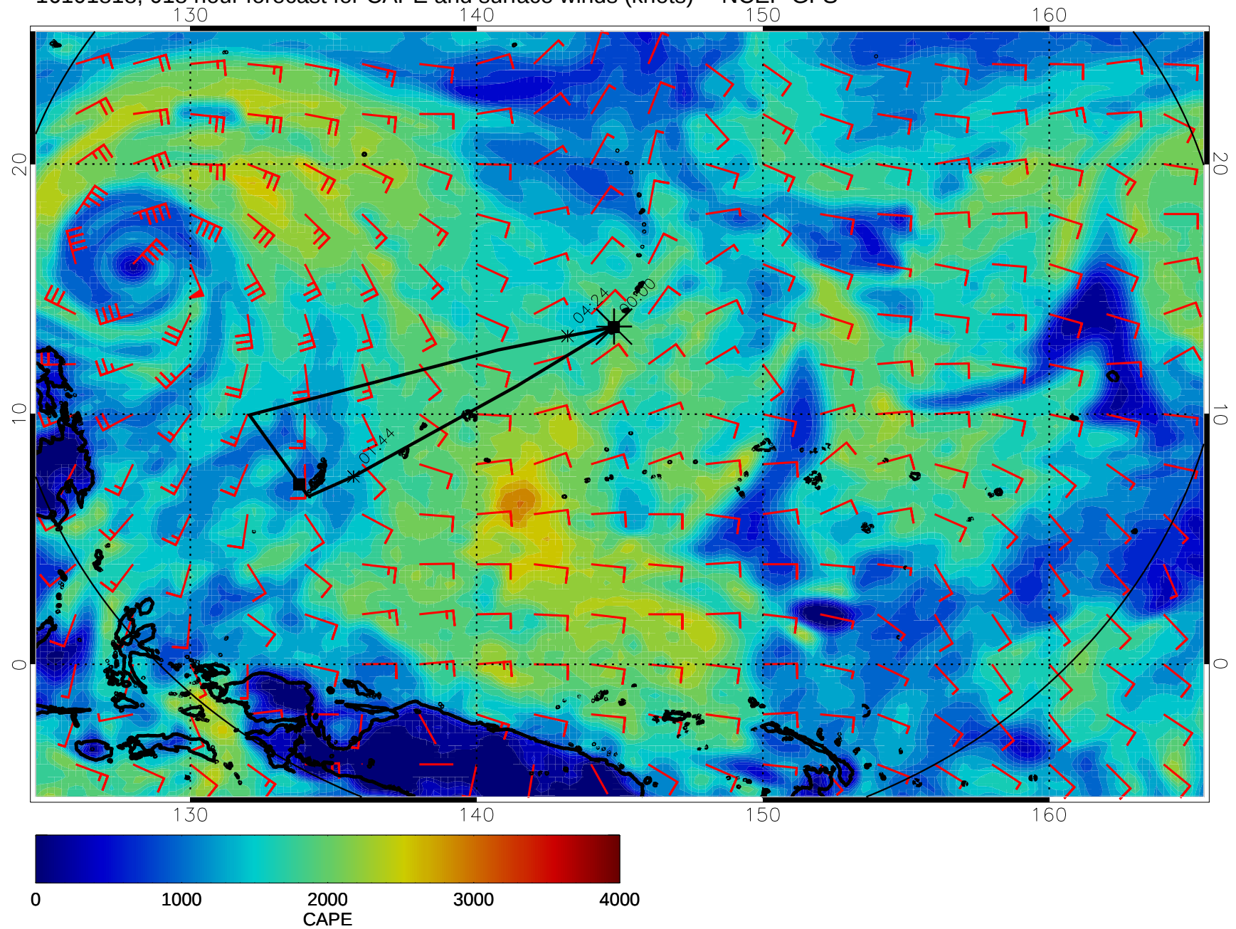
16101818, 018 hour forecast for CAPE and surface winds (knots) -- NCEP GFS
