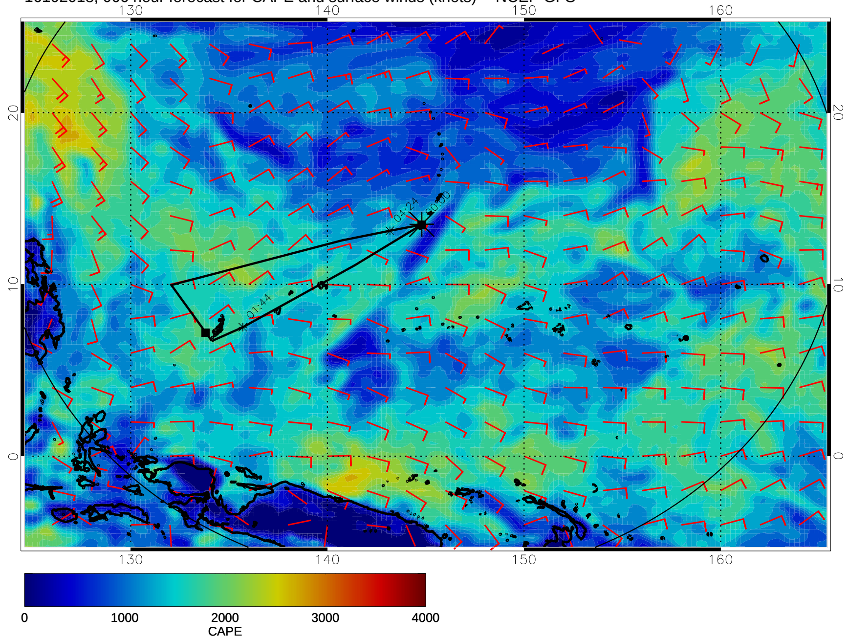
16102018, 066 hour forecast for CAPE and surface winds (knots) -- NCEP GFS
