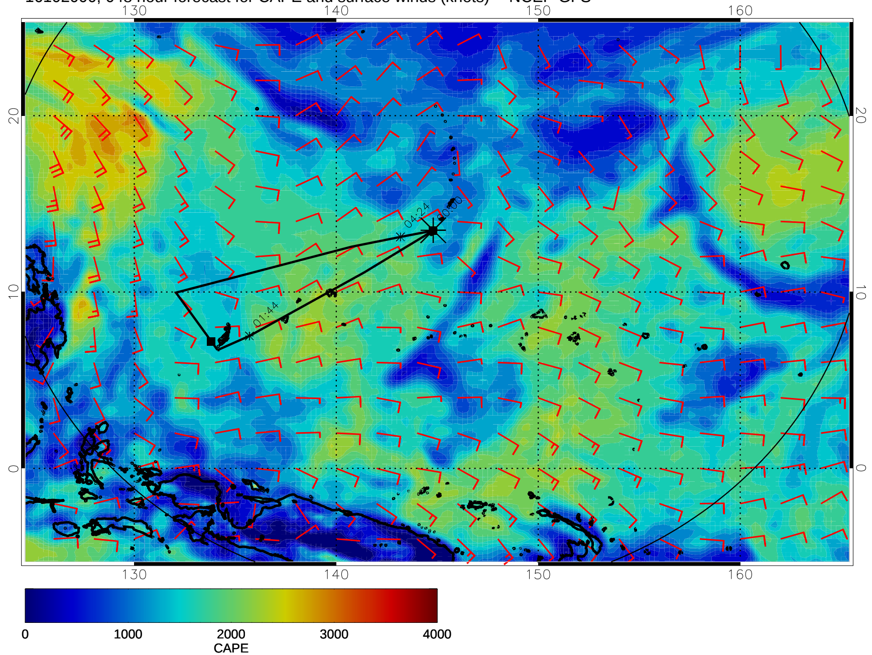
16102000, 048 hour forecast for CAPE and surface winds (knots) -- NCEP GFS
