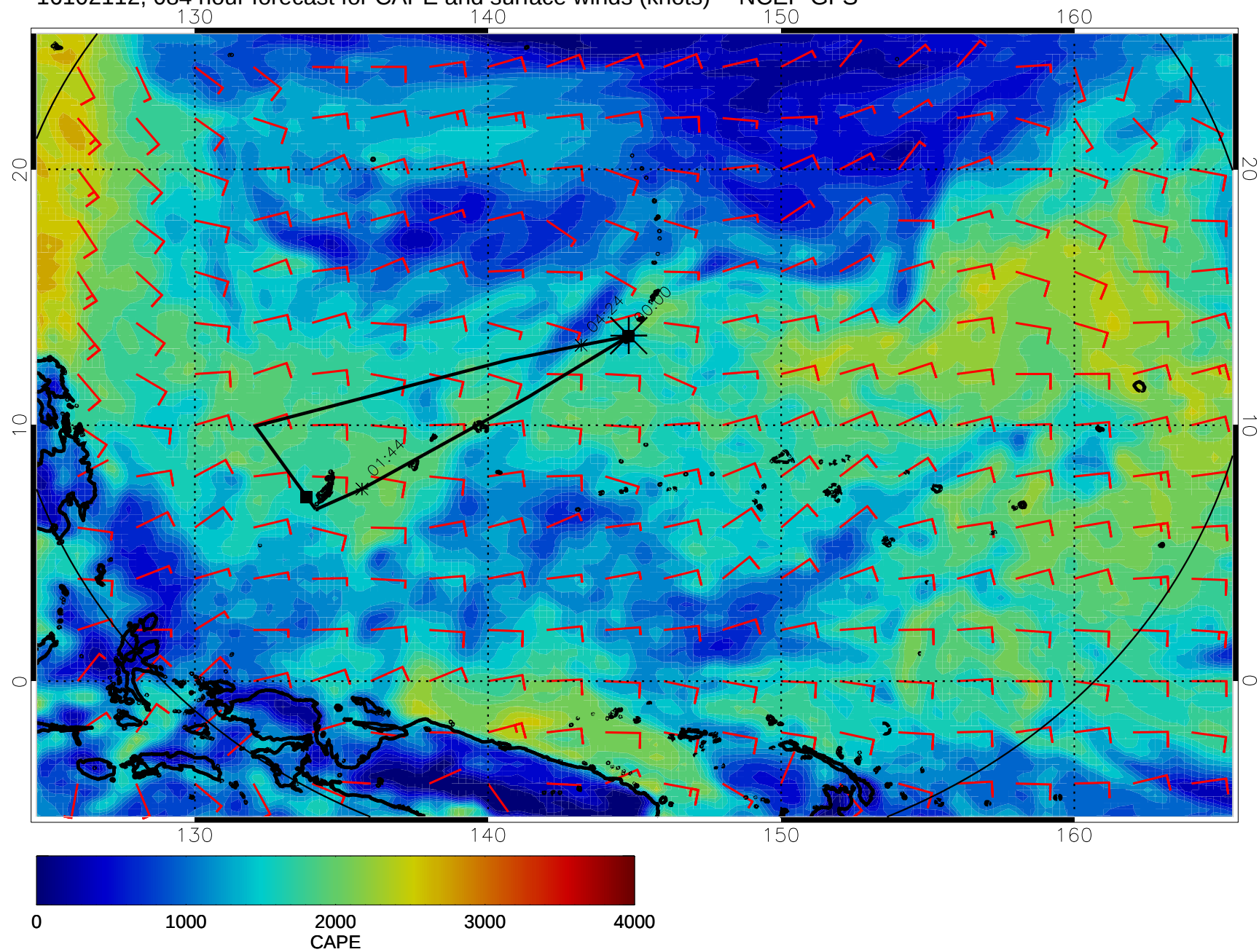
16102112, 084 hour forecast for CAPE and surface winds (knots) -- NCEP GFS
