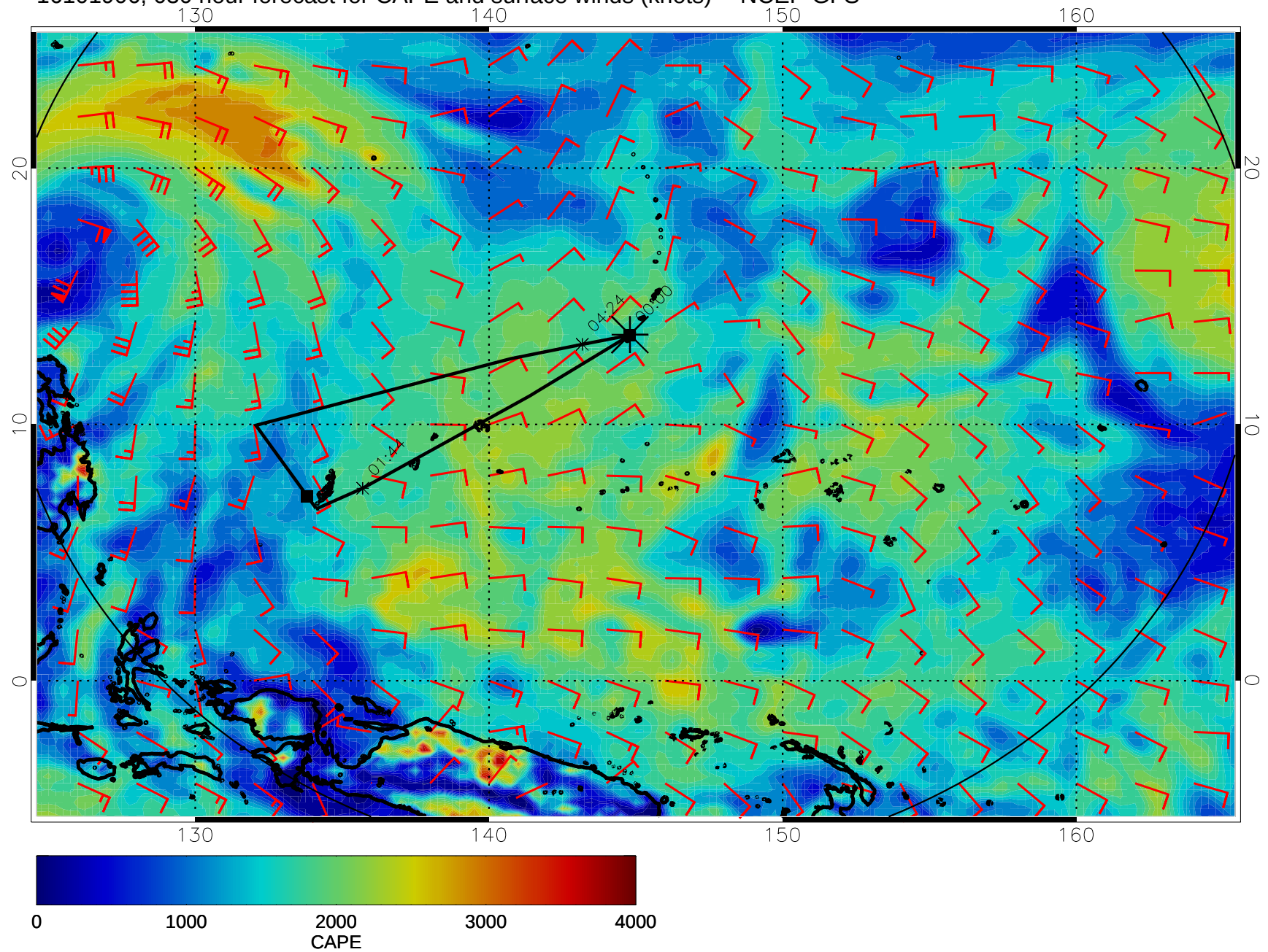
16101906, 030 hour forecast for CAPE and surface winds (knots) -- NCEP GFS
