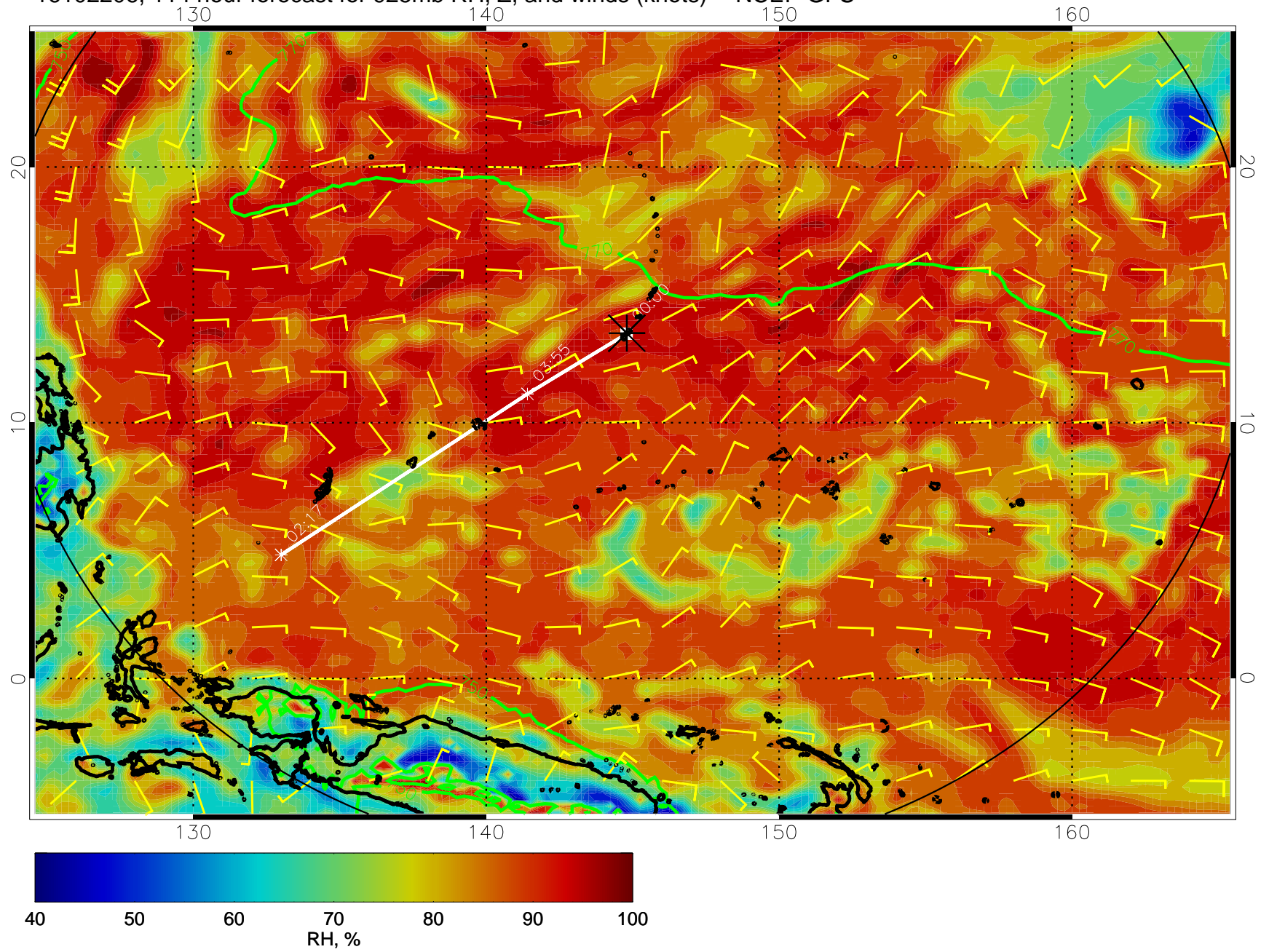
16102206, 114 hour forecast for 925mb RH, Z, and winds (knots) -- NCEP GFS
