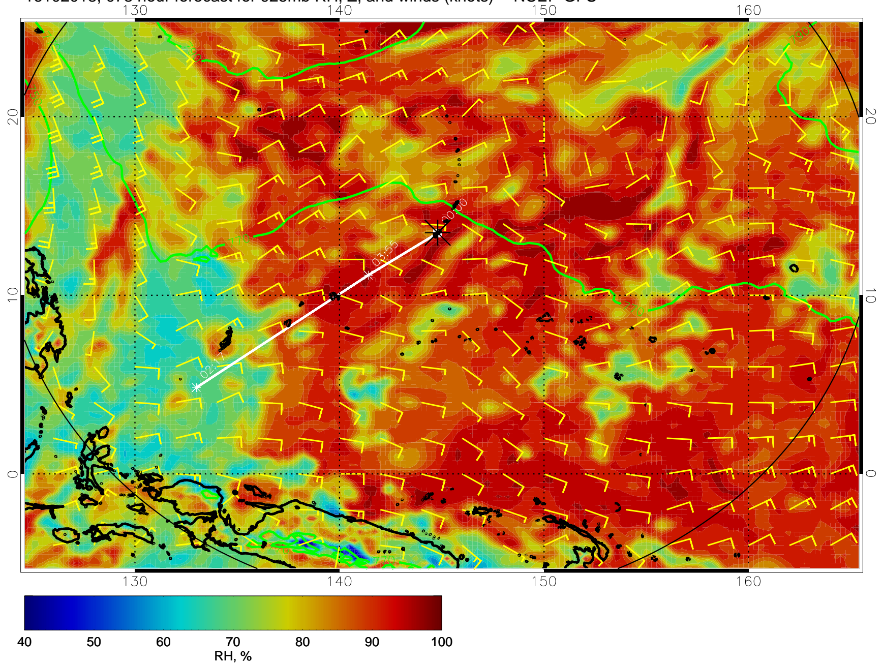
16102018, 078 hour forecast for 925mb RH, Z, and winds (knots) -- NCEP GFS
