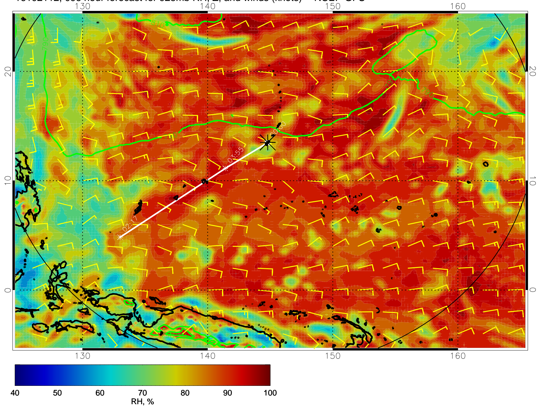
16102112, 096 hour forecast for 925mb RH, Z, and winds (knots) -- NCEP GFS
