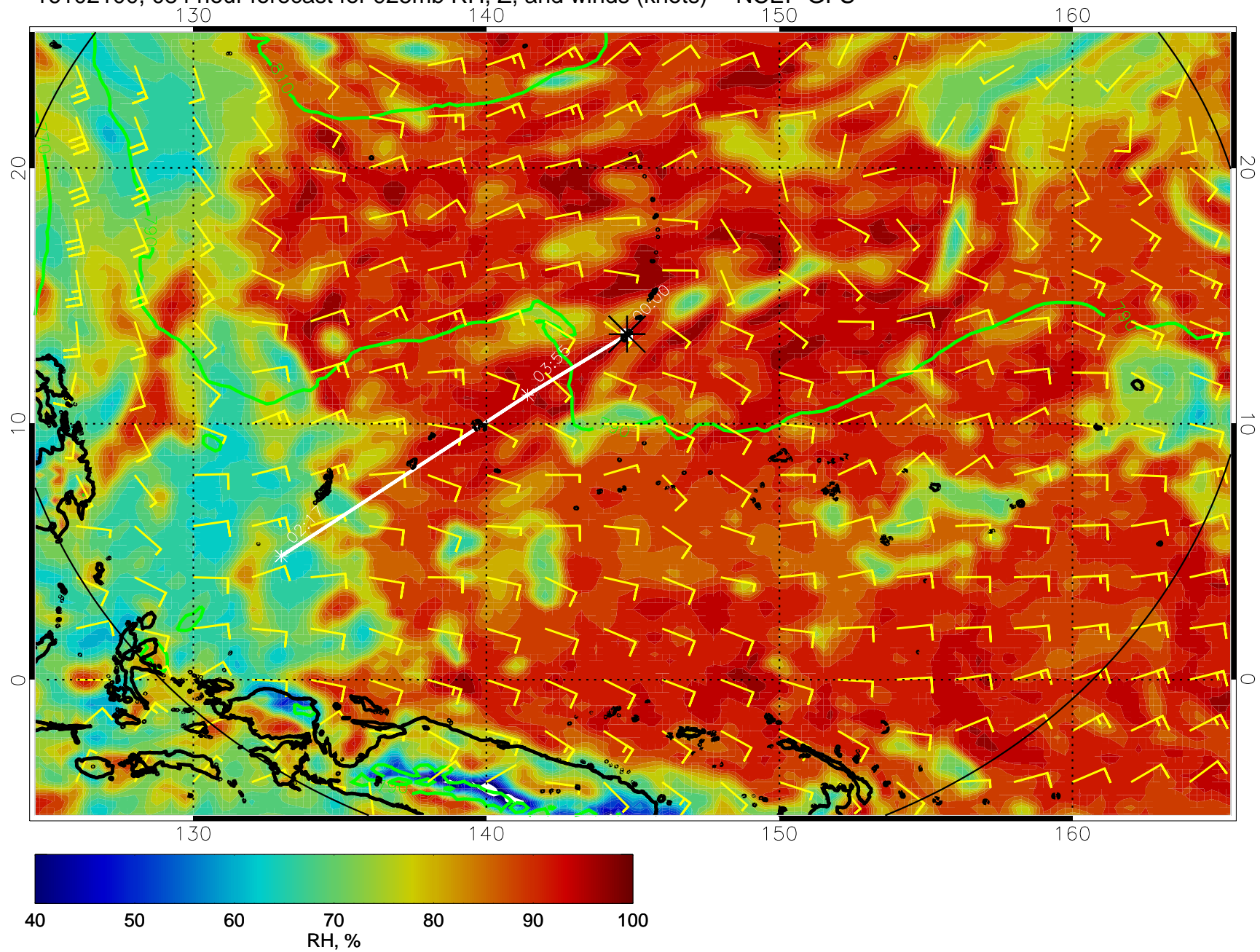
16102100, 084 hour forecast for 925mb RH, Z, and winds (knots) -- NCEP GFS
