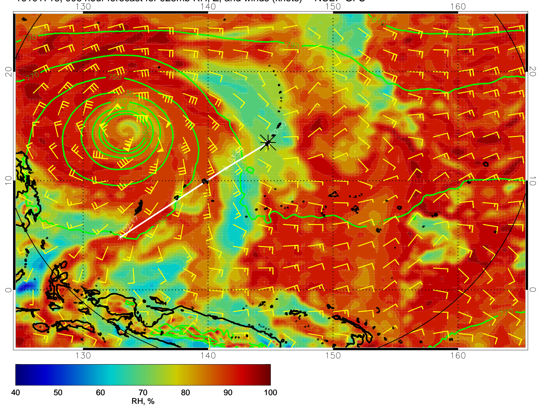
16101718, 006 hour forecast for 925mb RH, Z, and winds (knots) -- NCEP GFS
