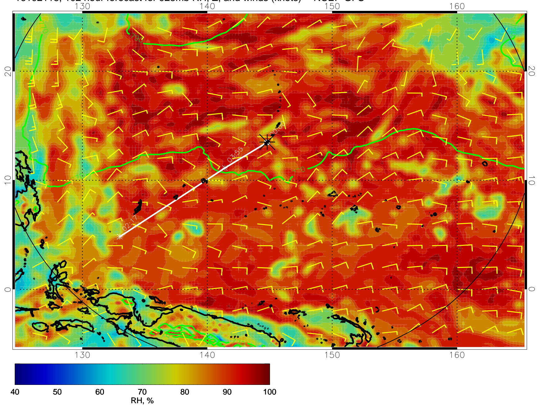
16102118, 102 hour forecast for 925mb RH, Z, and winds (knots) -- NCEP GFS
