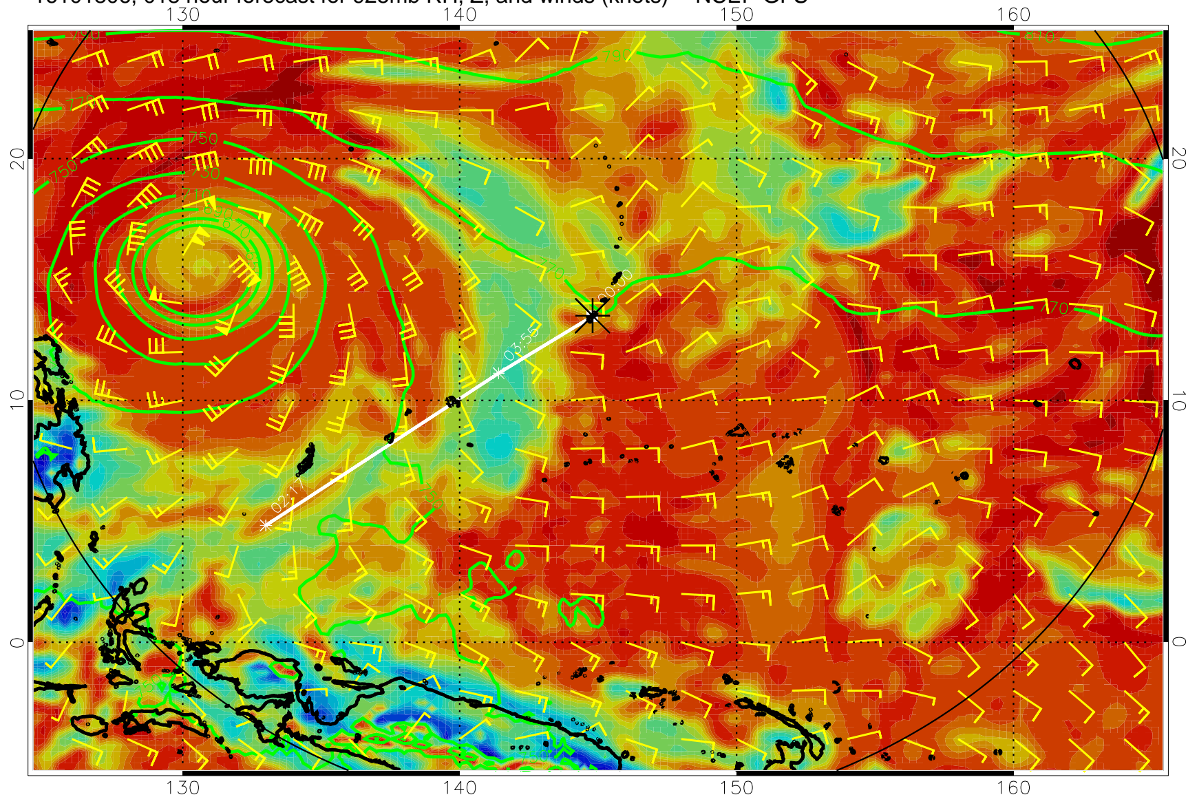
16101806, 018 hour forecast for 925mb RH, Z, and winds (knots) -- NCEP GFS
