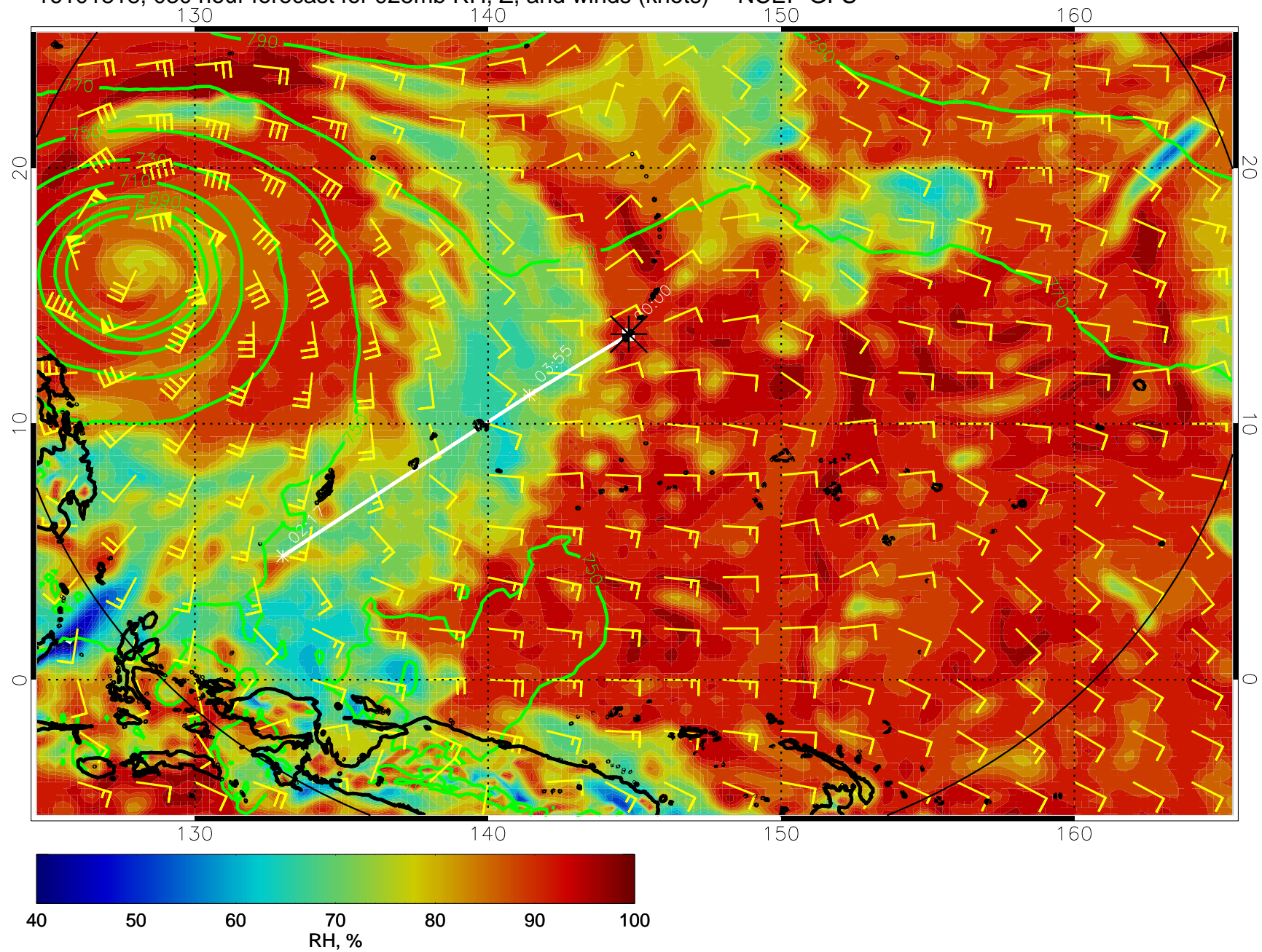
16101818, 030 hour forecast for 925mb RH, Z, and winds (knots) -- NCEP GFS
