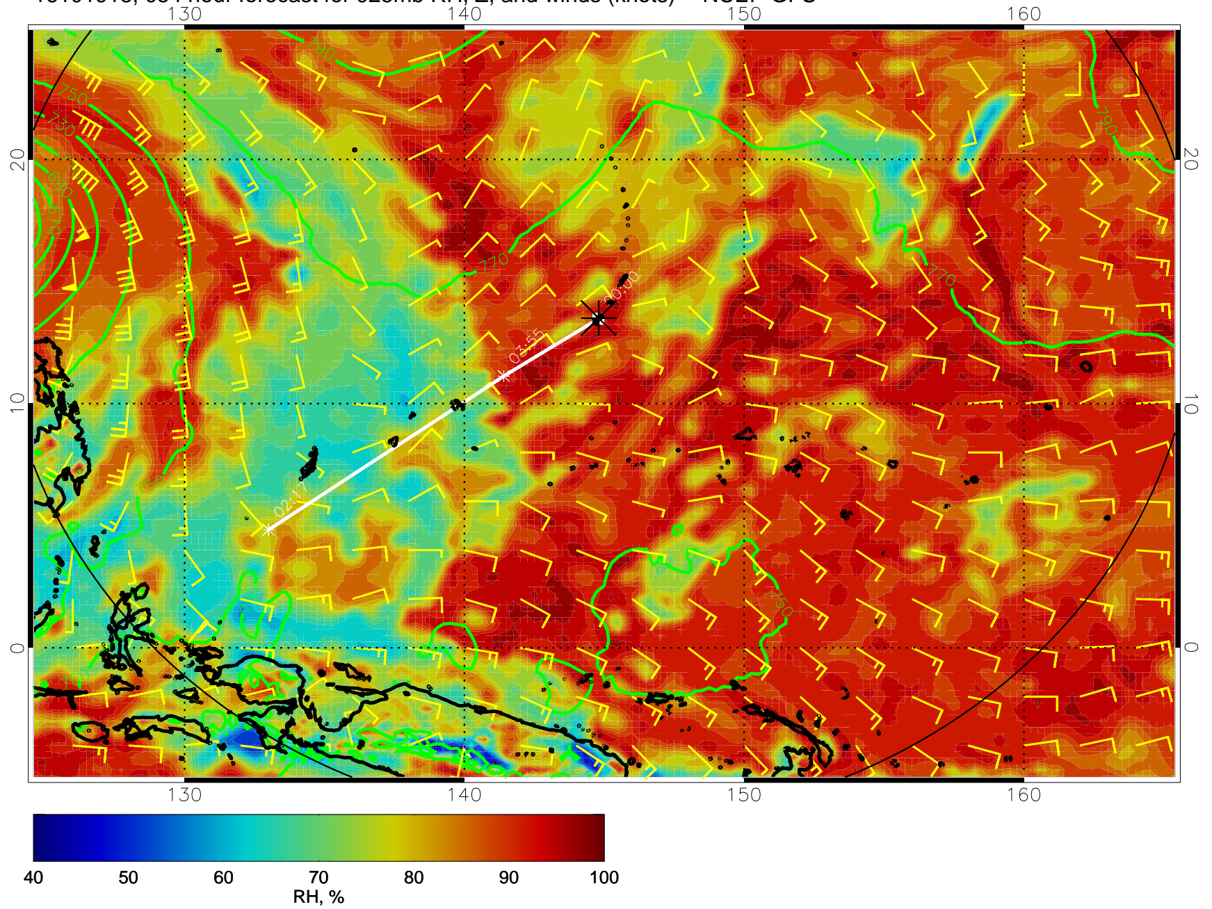
16101918, 054 hour forecast for 925mb RH, Z, and winds (knots) -- NCEP GFS
