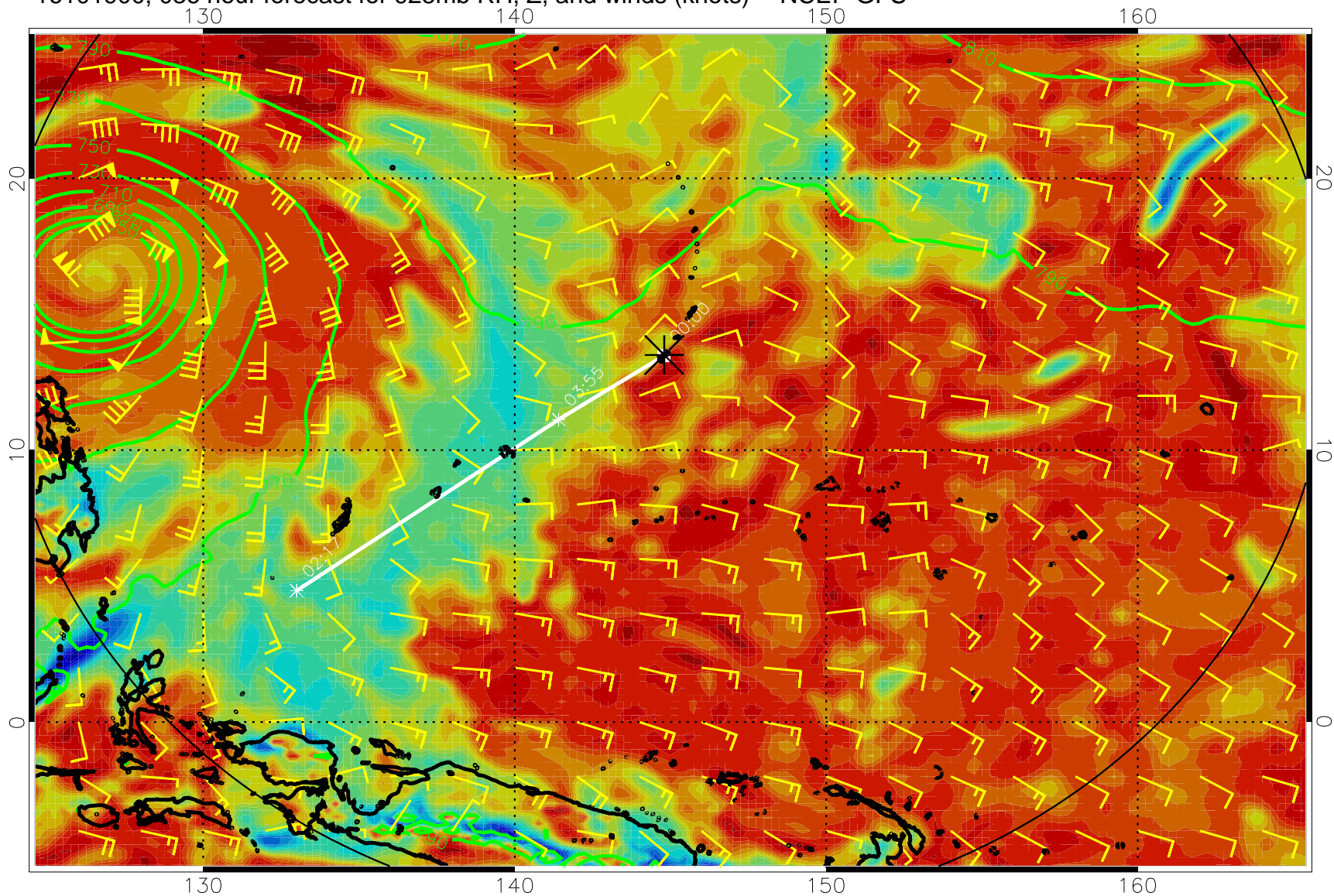
16101900, 036 hour forecast for 925mb RH, Z, and winds (knots) -- NCEP GFS
