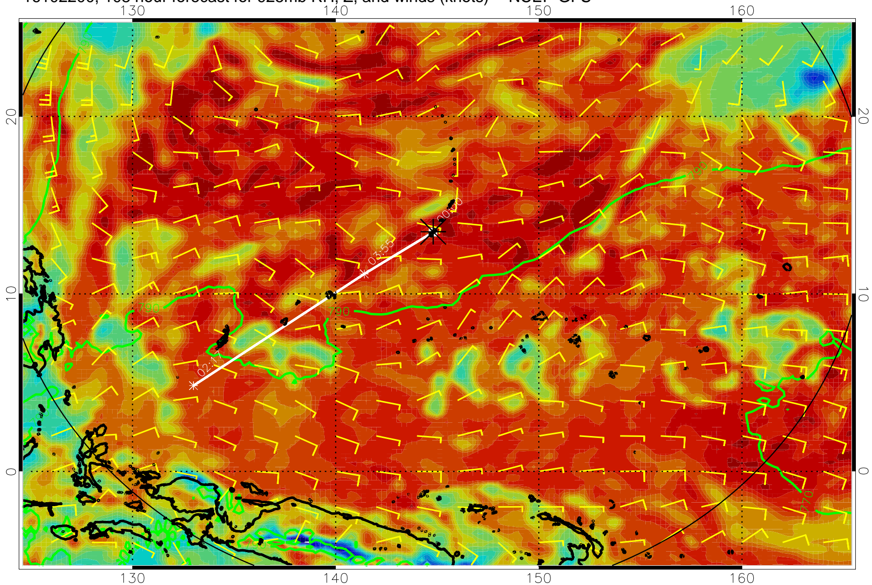
16102200, 108 hour forecast for 925mb RH, Z, and winds (knots) -- NCEP GFS
