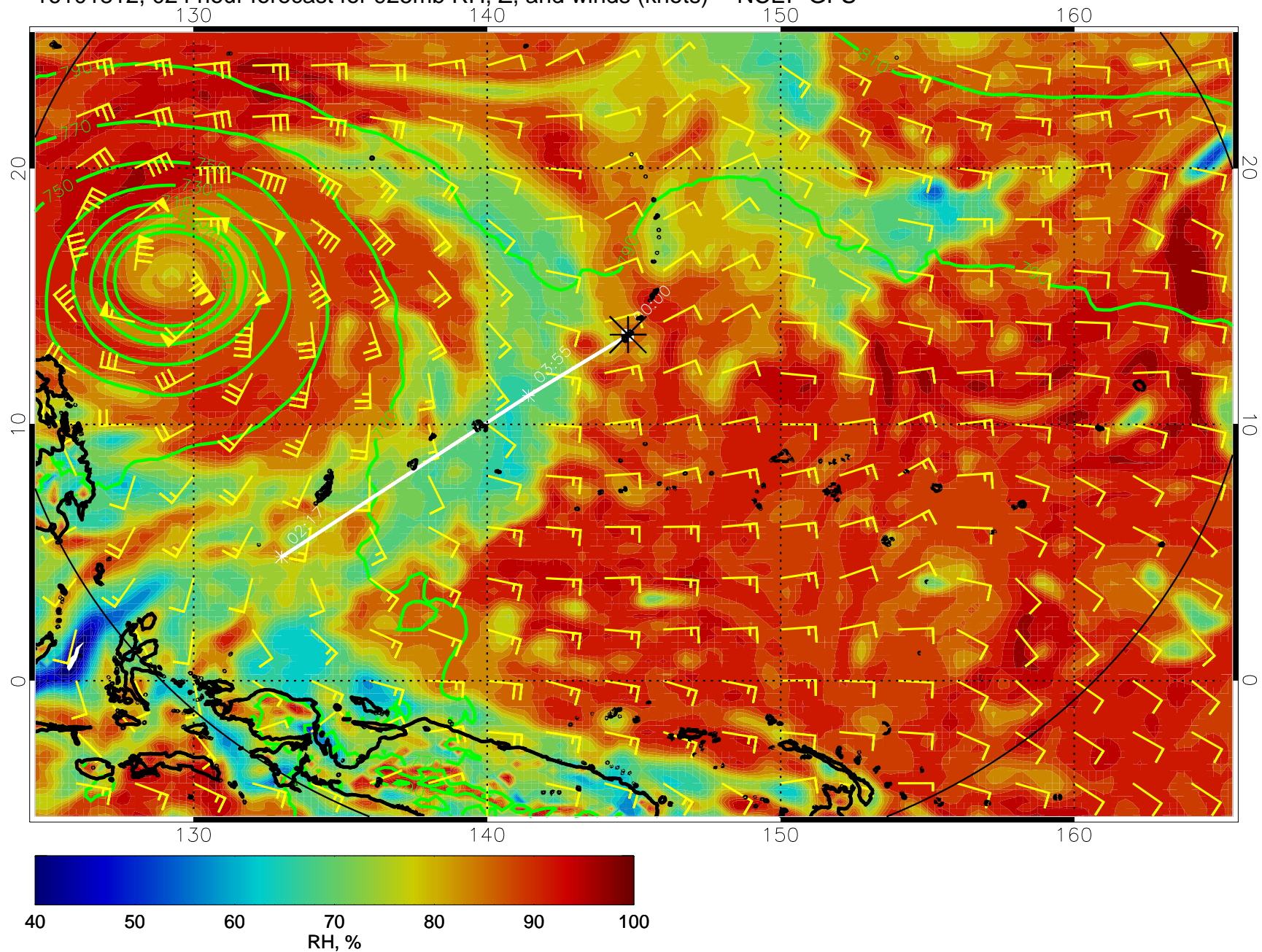
16101812, 024 hour forecast for 925mb RH, Z, and winds (knots) -- NCEP GFS
