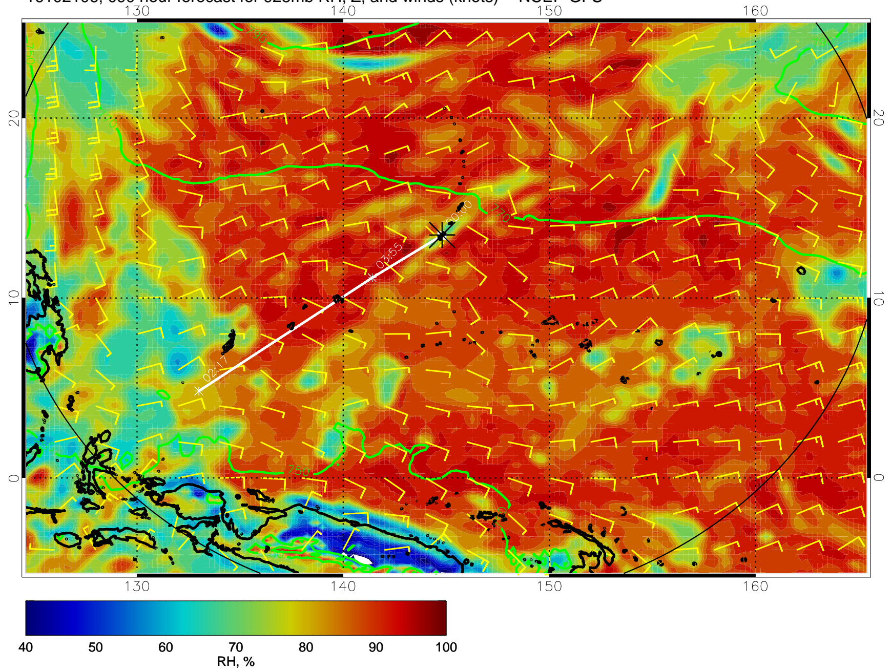
16102106, 090 hour forecast for 925mb RH, Z, and winds (knots) -- NCEP GFS
