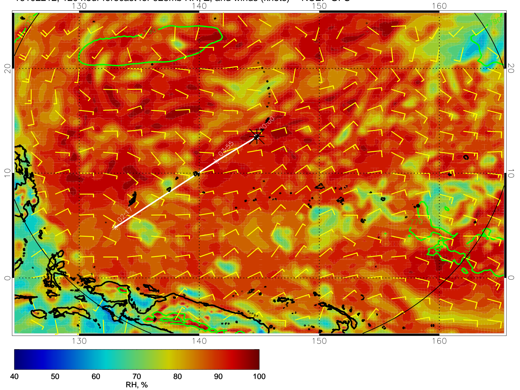
16102212, 120 hour forecast for 925mb RH, Z, and winds (knots) -- NCEP GFS
