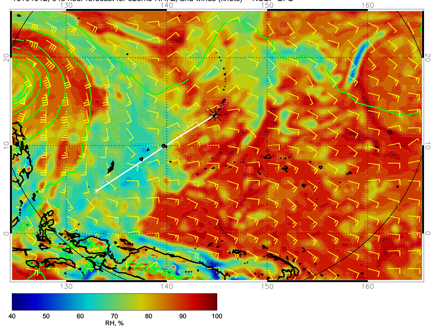
16101912, 048 hour forecast for 925mb RH, Z, and winds (knots) -- NCEP GFS
