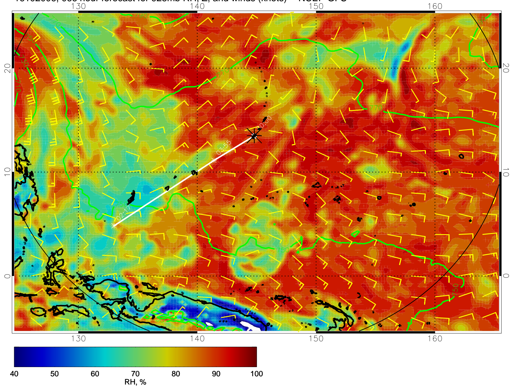
16102006, 066 hour forecast for 925mb RH, Z, and winds (knots) -- NCEP GFS
