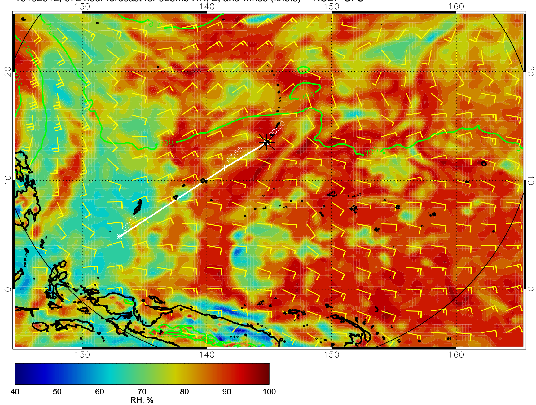
16102012, 072 hour forecast for 925mb RH, Z, and winds (knots) -- NCEP GFS
