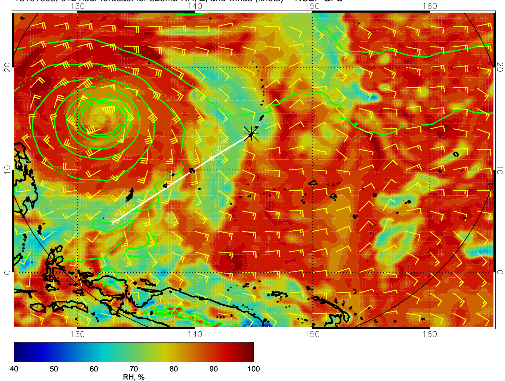
16101800, 012 hour forecast for 925mb RH, Z, and winds (knots) -- NCEP GFS
