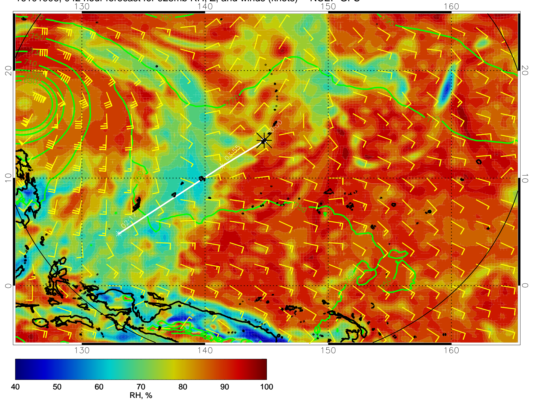
16101906, 042 hour forecast for 925mb RH, Z, and winds (knots) -- NCEP GFS
