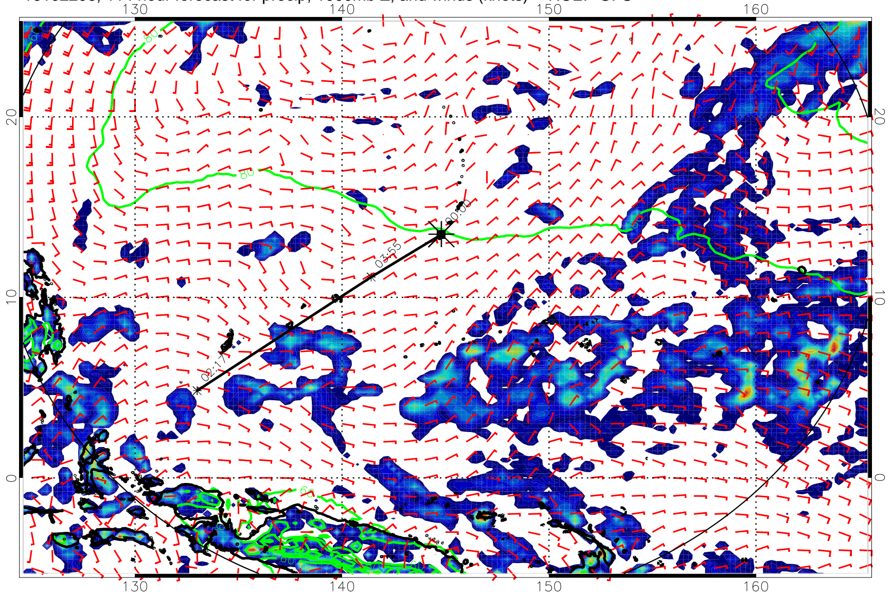
16102206, 114 hour forecast for precip, 1000mb Z, and winds (knots) -- NCEP GFS
