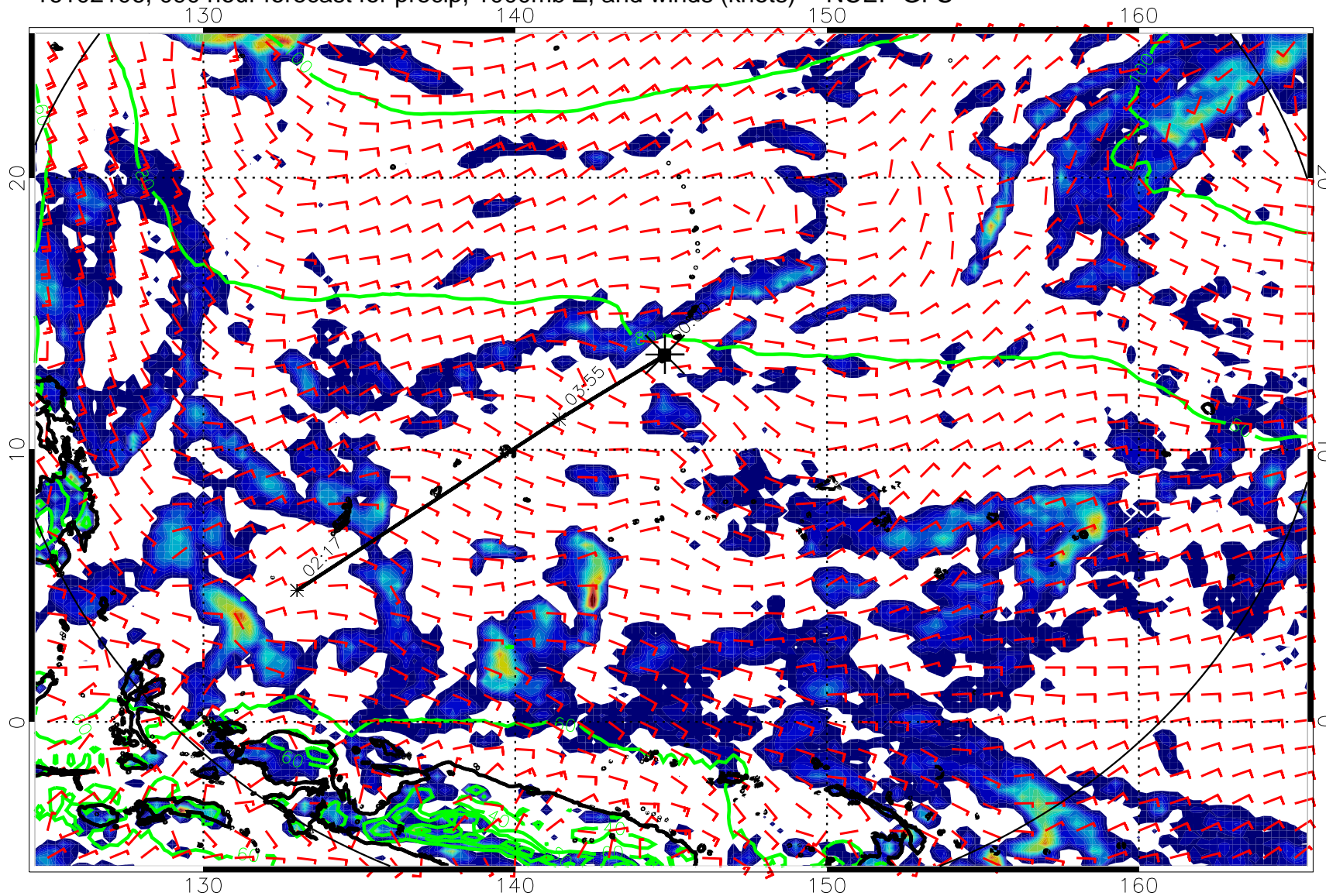
16102106, 090 hour forecast for precip, 1000mb Z, and winds (knots) -- NCEP GFS
