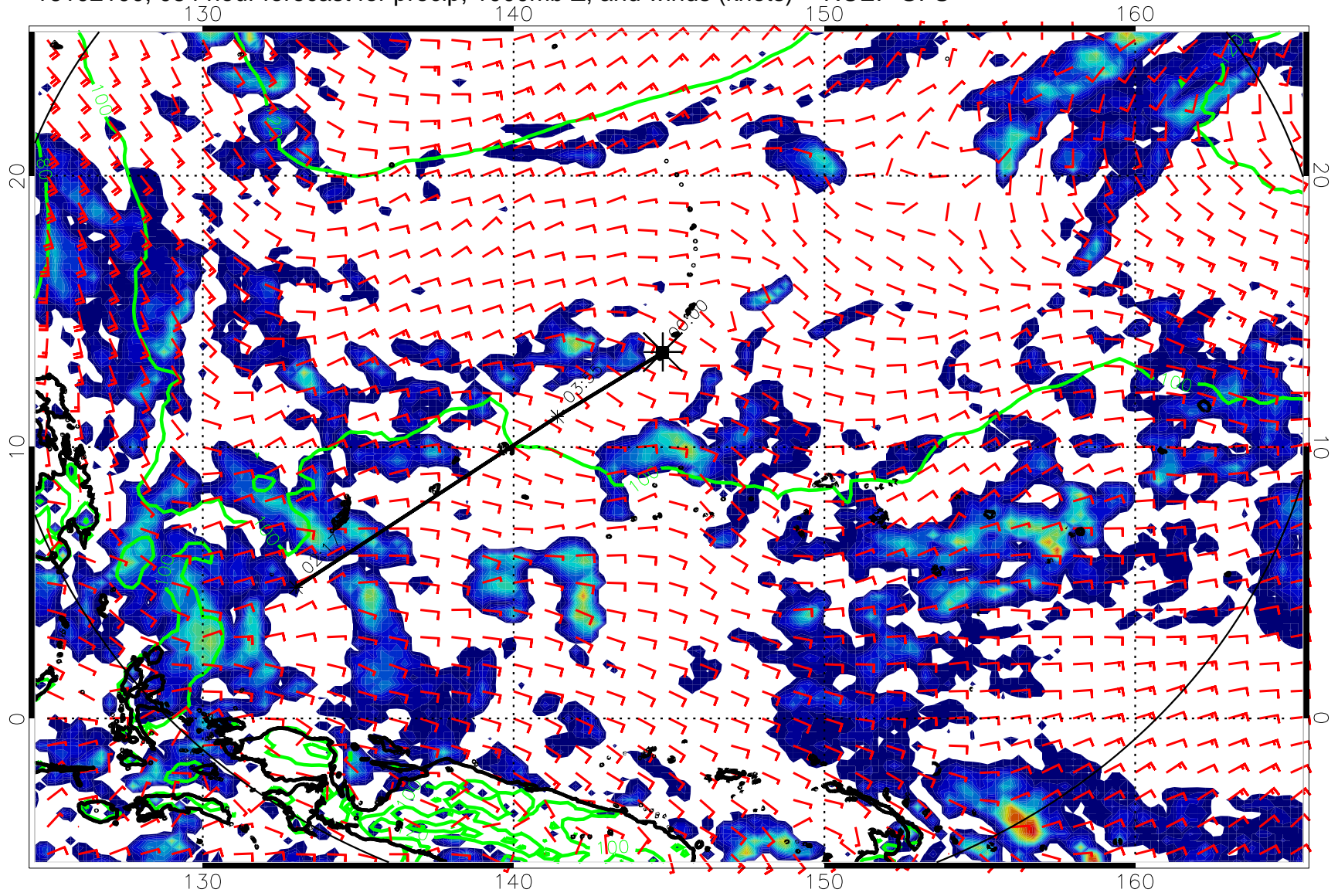
16102100, 084 hour forecast for precip, 1000mb Z, and winds (knots) -- NCEP GFS
