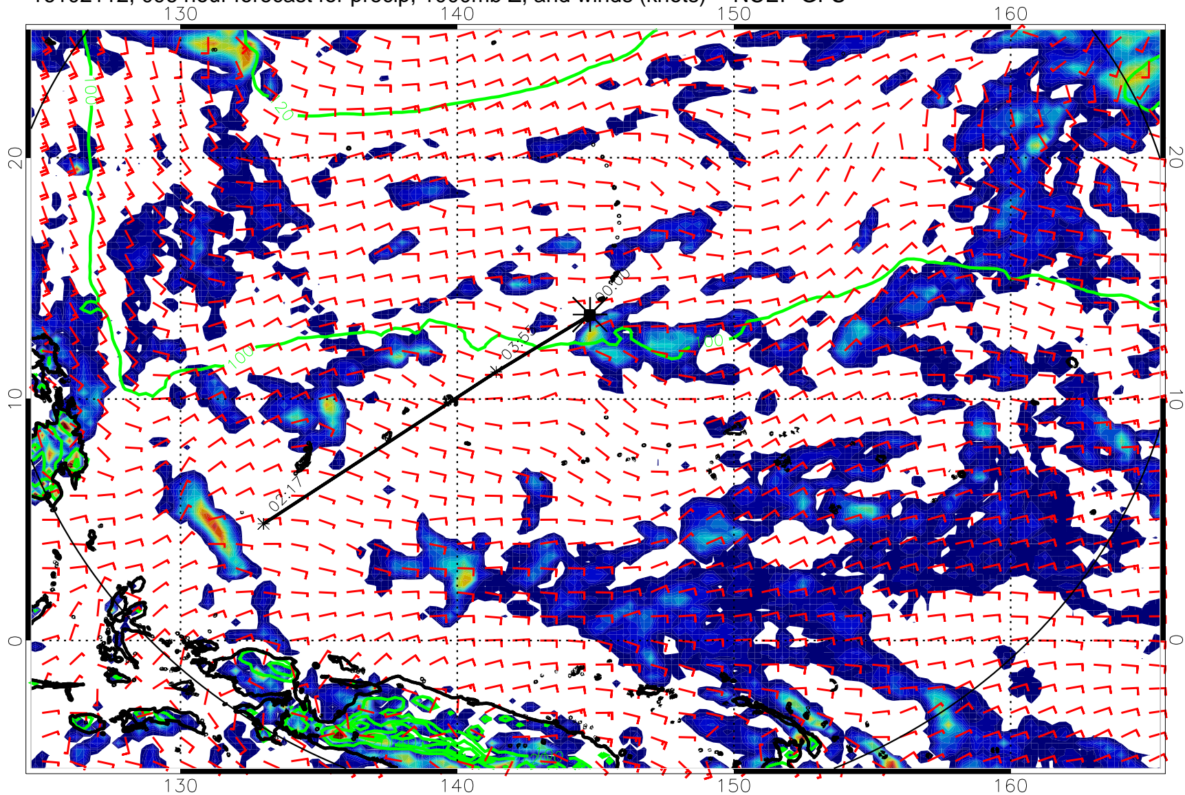
16102112, 096 hour forecast for precip, 1000mb Z, and winds (knots) -- NCEP GFS
