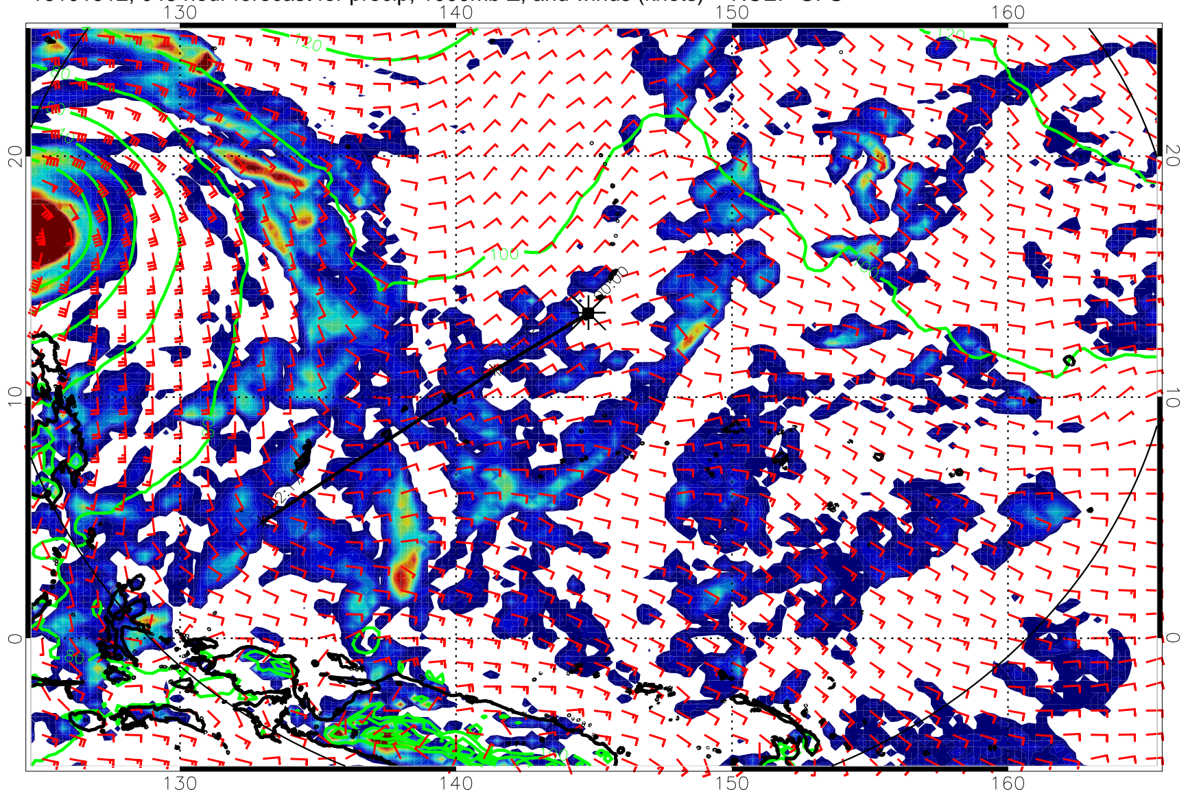
16101912, 048 hour forecast for precip, 1000mb Z, and winds (knots) -- NCEP GFS
