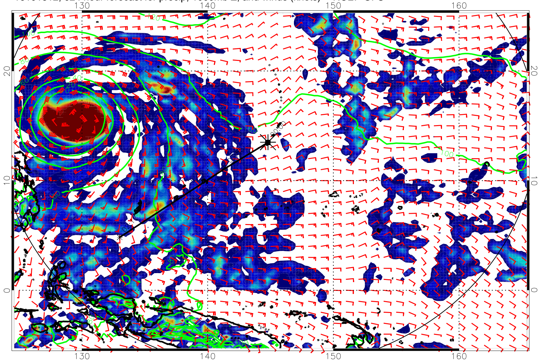
16101812, 024 hour forecast for precip, 1000mb Z, and winds (knots) -- NCEP GFS
