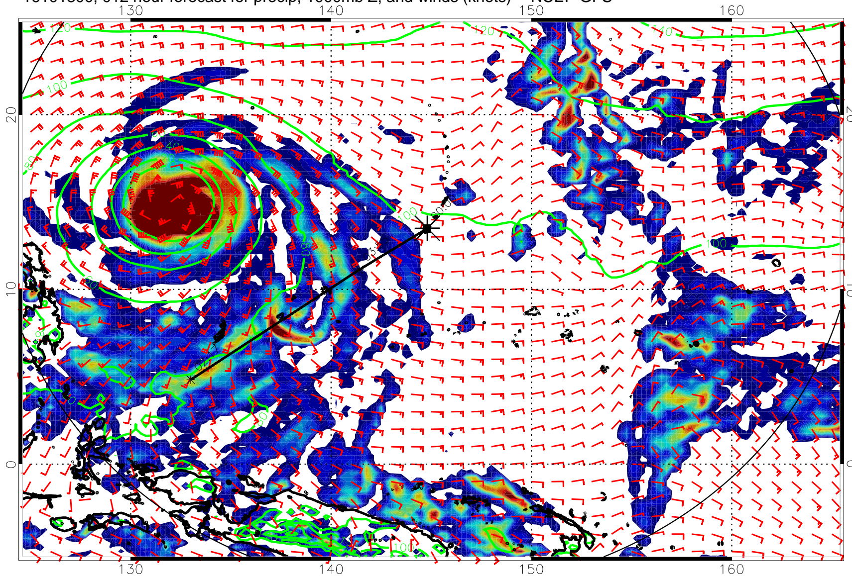
16101800, 012 hour forecast for precip, 1000mb Z, and winds (knots) -- NCEP GFS
