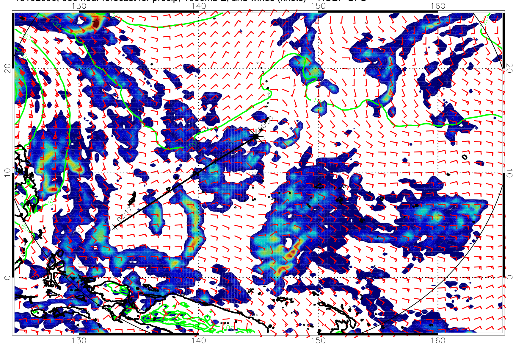
16102000, 060 hour forecast for precip, 1000mb Z, and winds (knots) -- NCEP GFS
