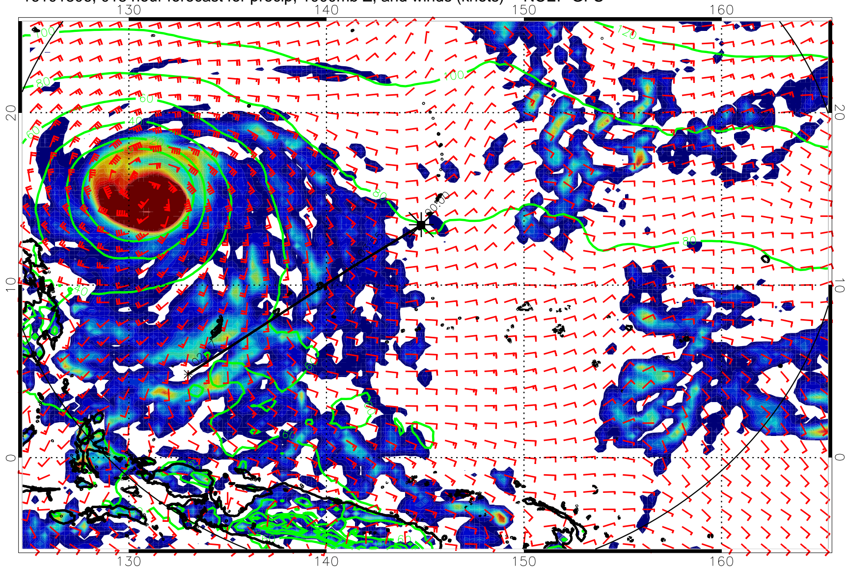
16101806, 018 hour forecast for precip, 1000mb Z, and winds (knots) -- NCEP GFS
