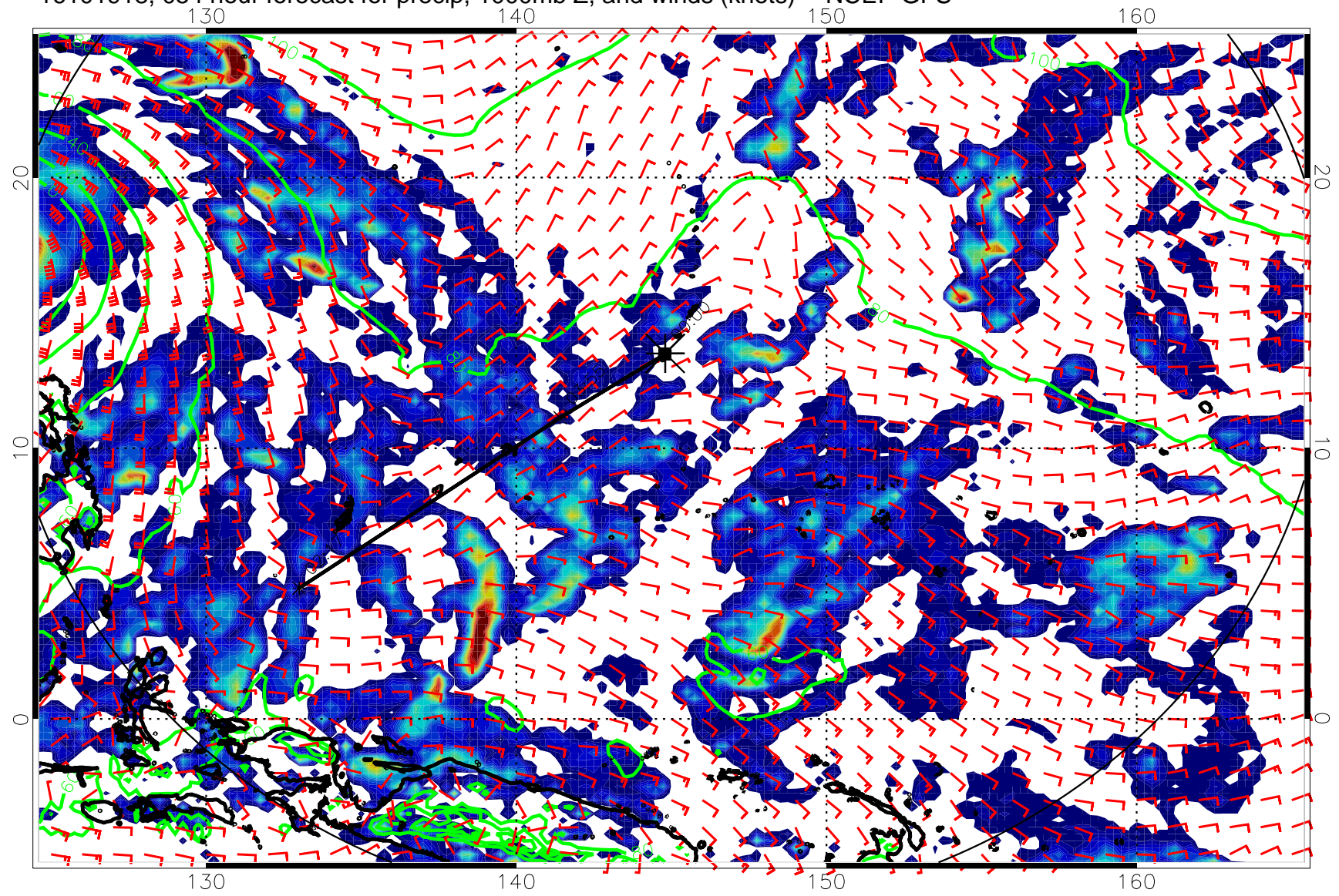
16101918, 054 hour forecast for precip, 1000mb Z, and winds (knots) -- NCEP GFS
