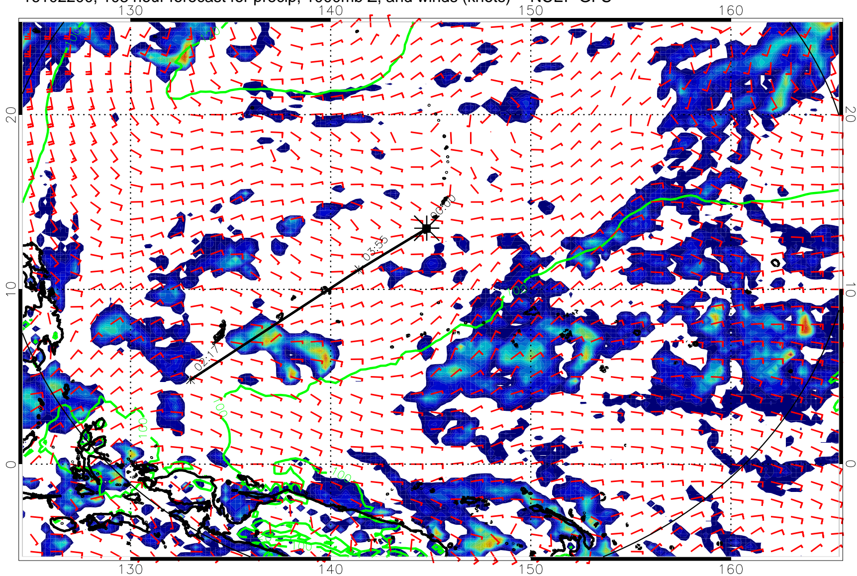
16102200, 108 hour forecast for precip, 1000mb Z, and winds (knots) -- NCEP GFS
