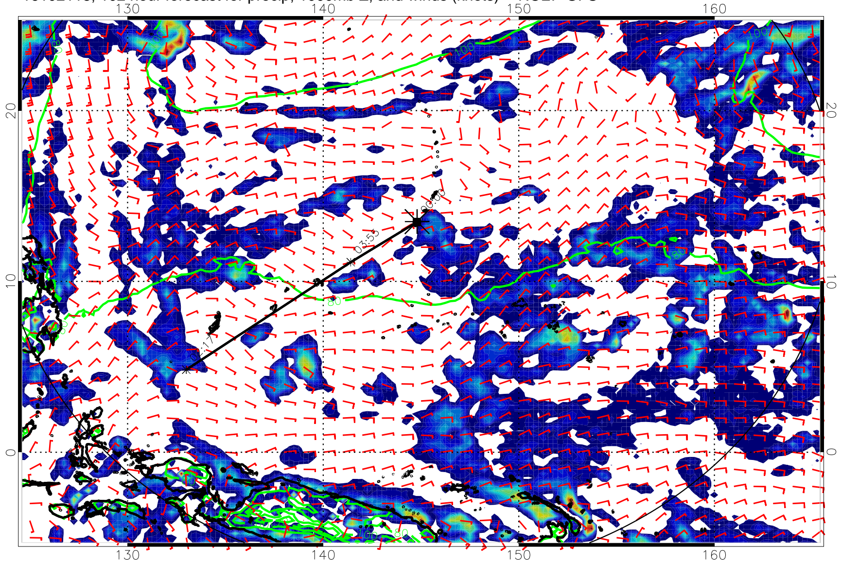
16102118, 102 hour forecast for precip, 1000mb Z, and winds (knots) -- NCEP GFS
