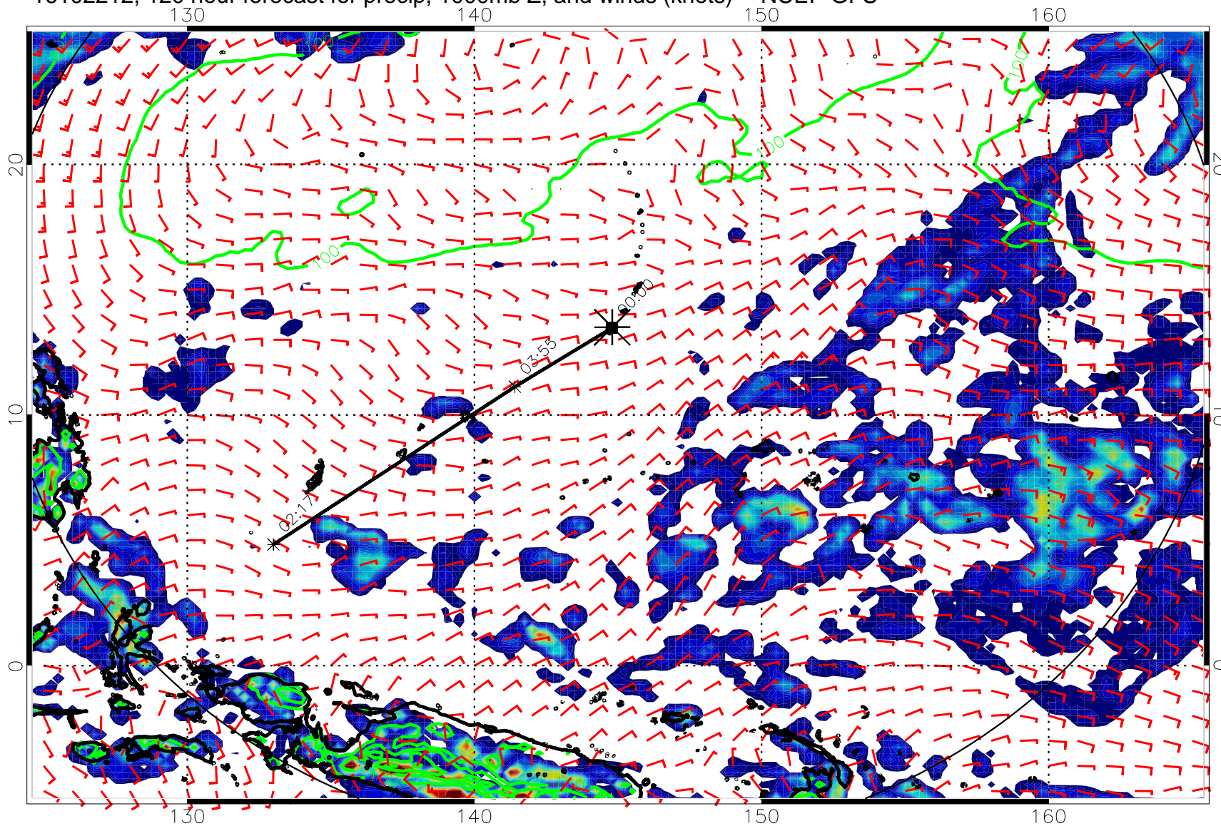
16102212, 120 hour forecast for precip, 1000mb Z, and winds (knots) -- NCEP GFS
