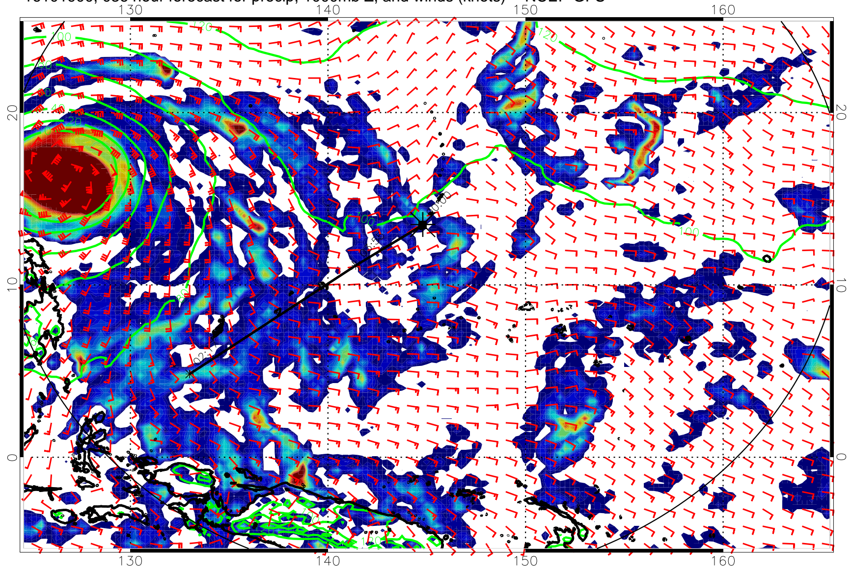
16101900, 036 hour forecast for precip, 1000mb Z, and winds (knots) -- NCEP GFS
