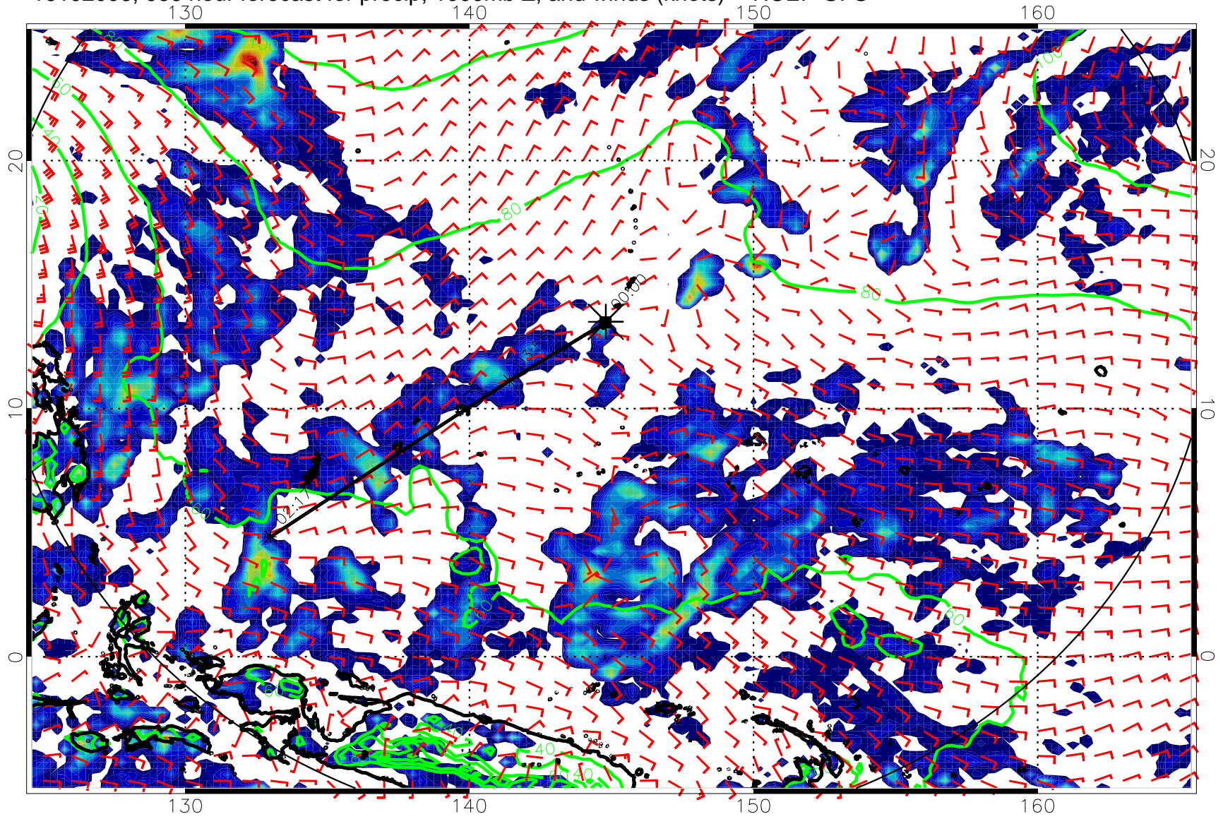
16102006, 066 hour forecast for precip, 1000mb Z, and winds (knots) -- NCEP GFS
