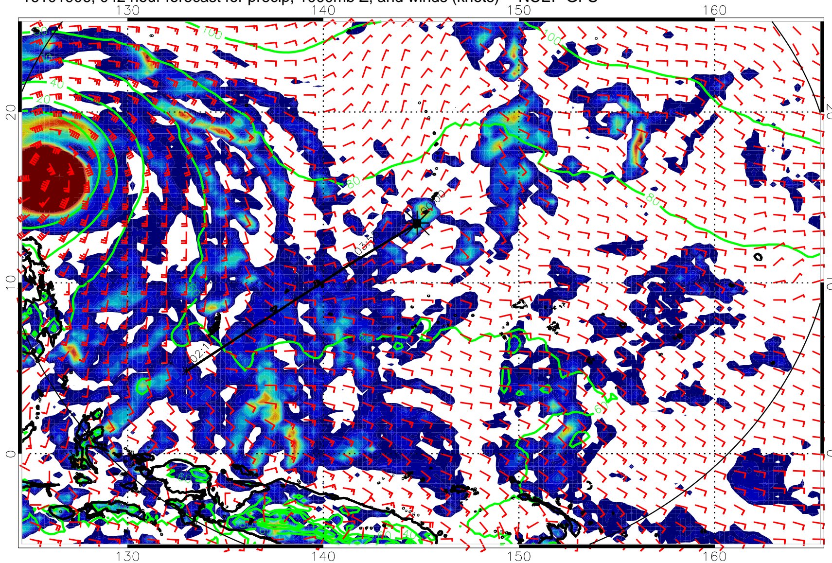
16101906, 042 hour forecast for precip, 1000mb Z, and winds (knots) -- NCEP GFS
