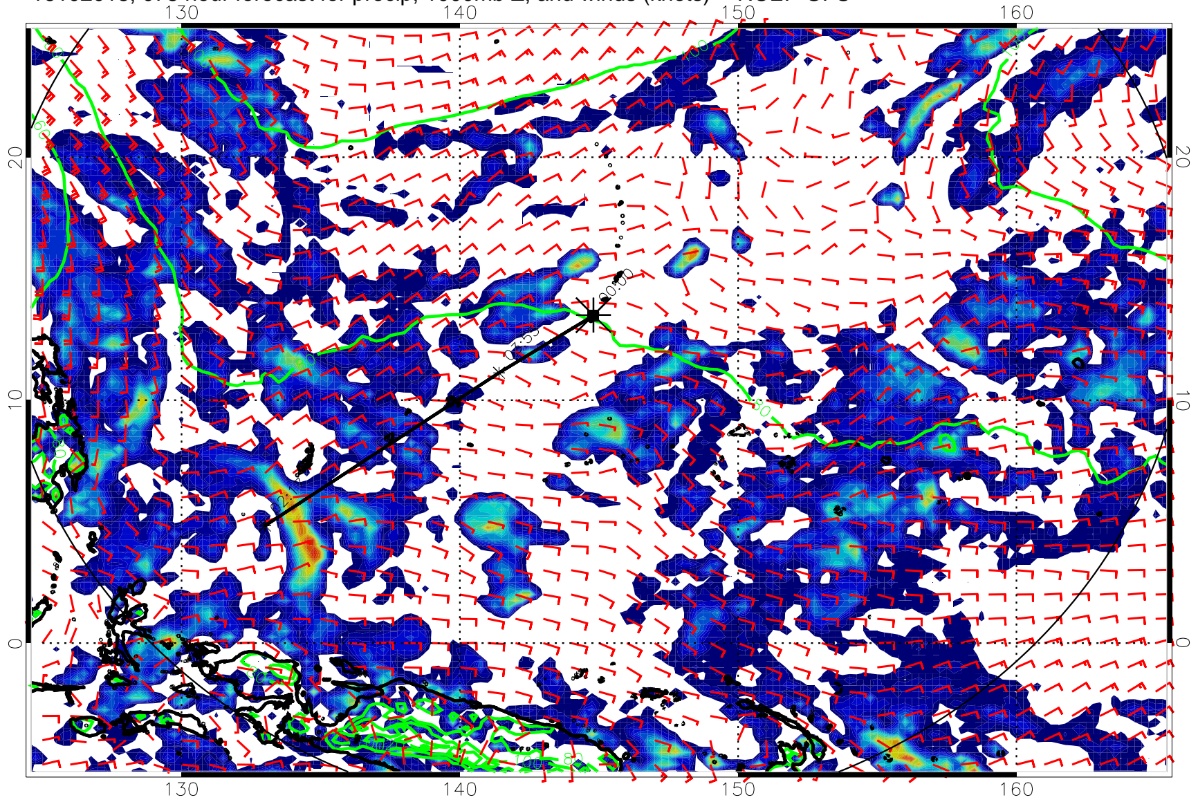
16102018, 078 hour forecast for precip, 1000mb Z, and winds (knots) -- NCEP GFS
