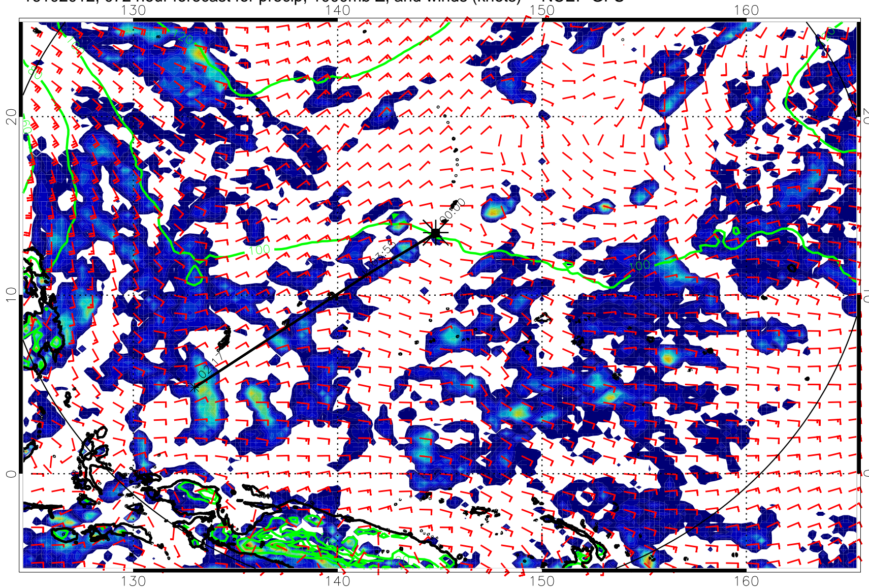
16102012, 072 hour forecast for precip, 1000mb Z, and winds (knots) -- NCEP GFS
