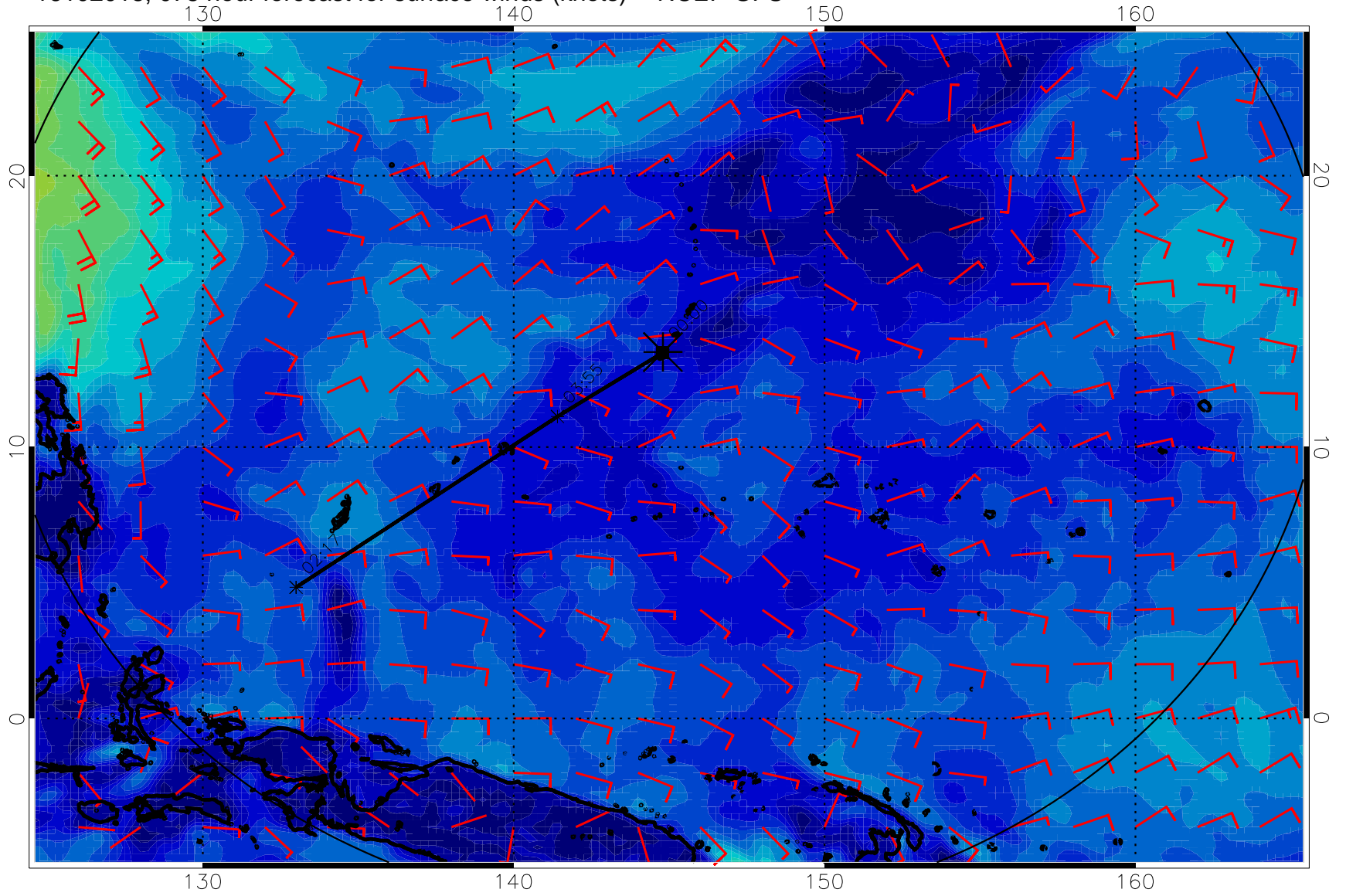
16102018, 078 hour forecast for surface winds (knots) -- NCEP GFS
