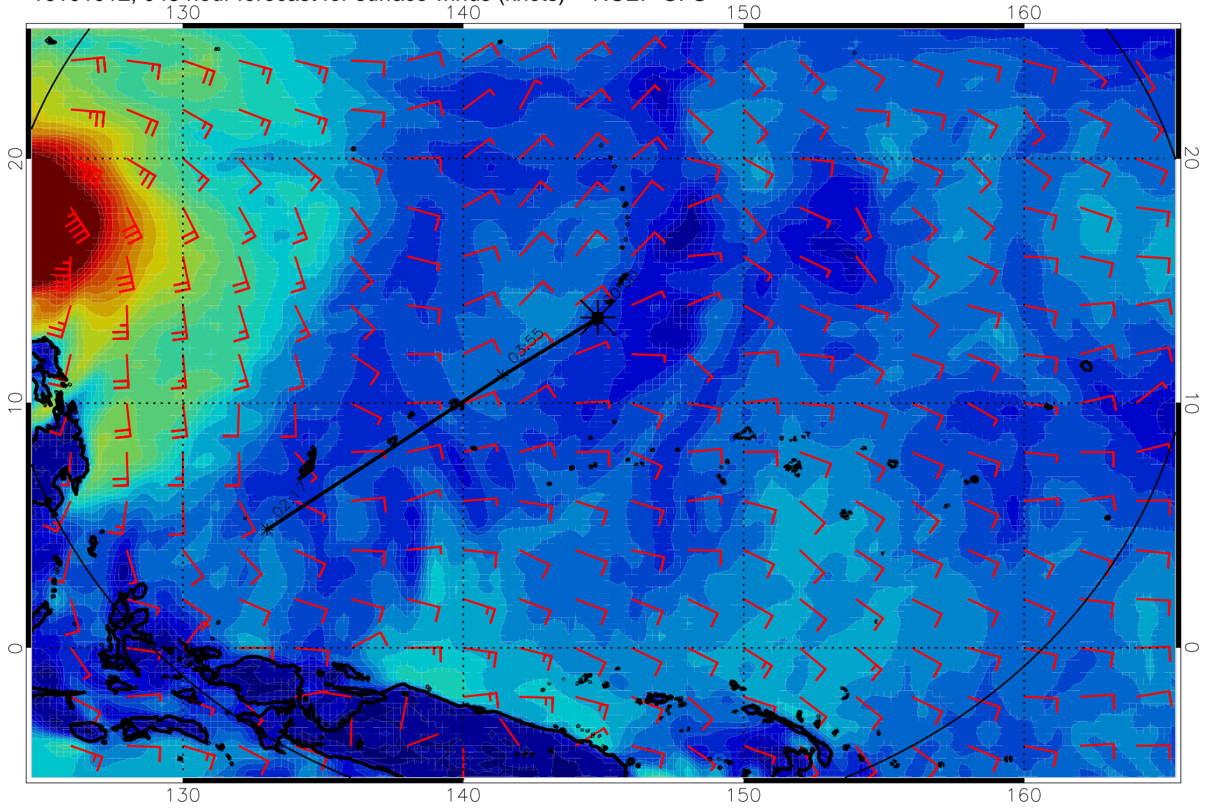
16101912, 048 hour forecast for surface winds (knots) -- NCEP GFS
