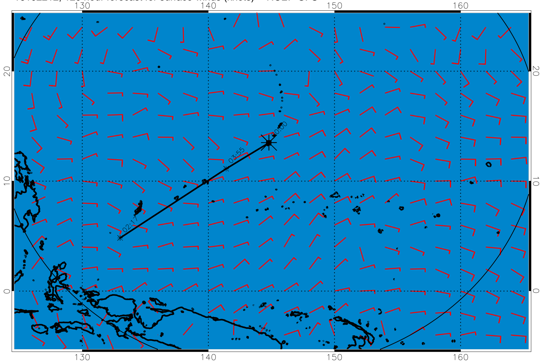
16102212, 120 hour forecast for surface winds (knots) -- NCEP GFS
