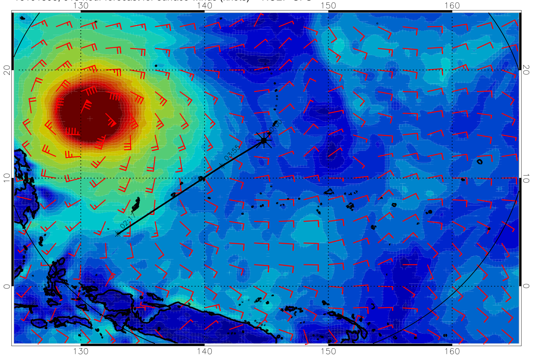
16101806, 018 hour forecast for surface winds (knots) -- NCEP GFS
