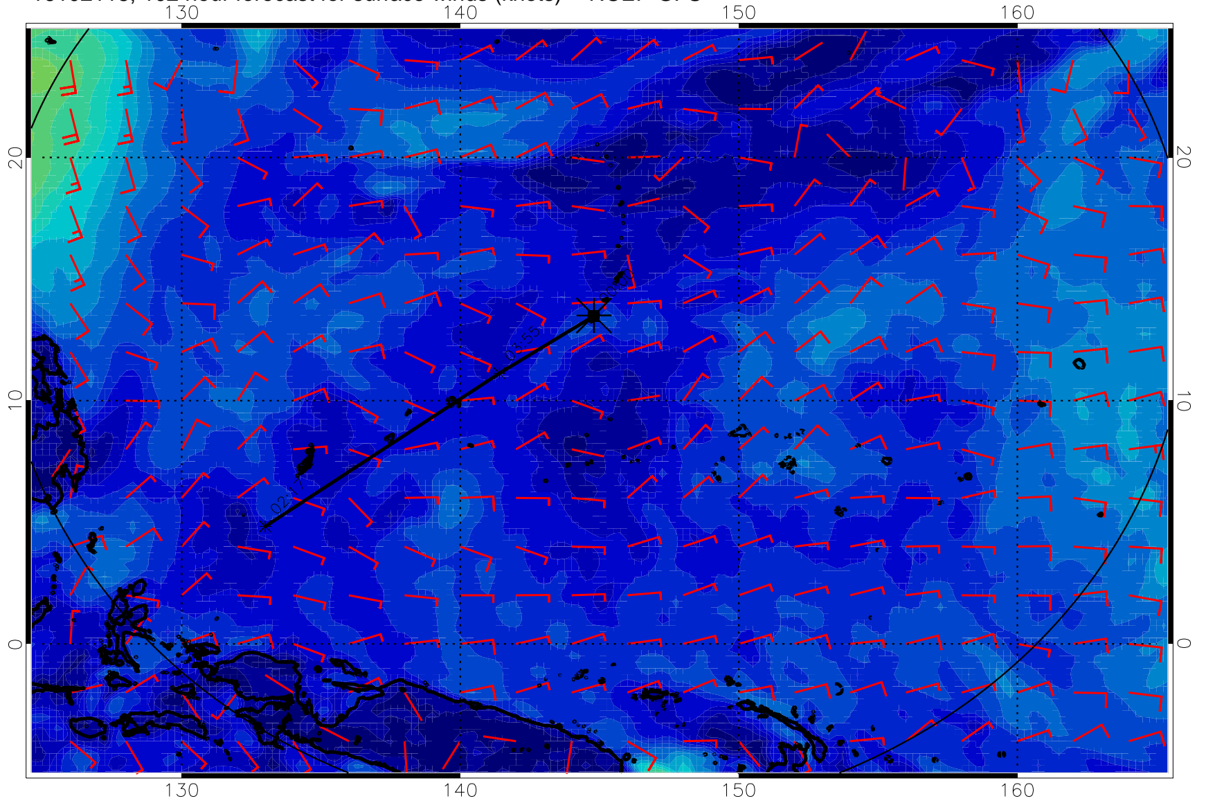
16102118, 102 hour forecast for surface winds (knots) -- NCEP GFS
