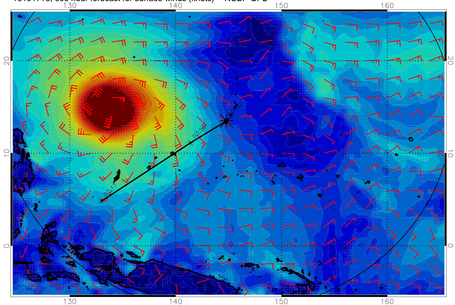
16101718, 006 hour forecast for surface winds (knots) -- NCEP GFS
