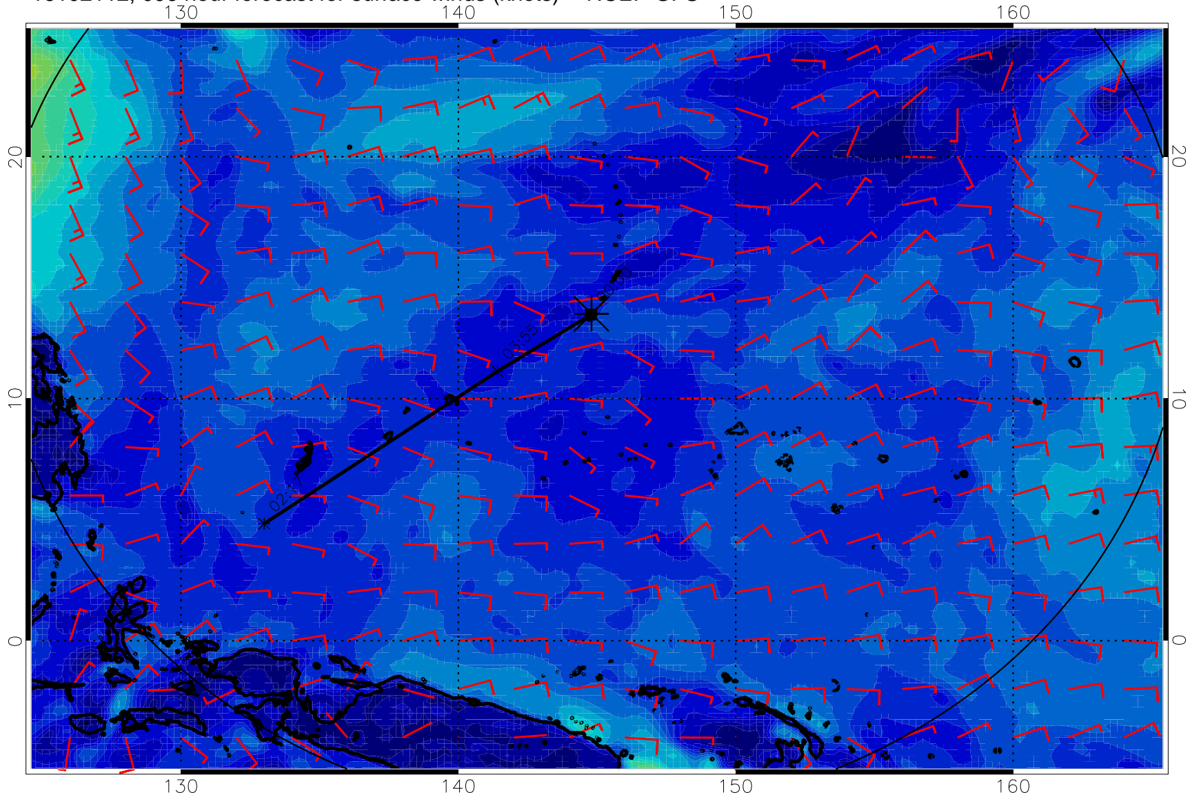
16102112, 096 hour forecast for surface winds (knots) -- NCEP GFS
