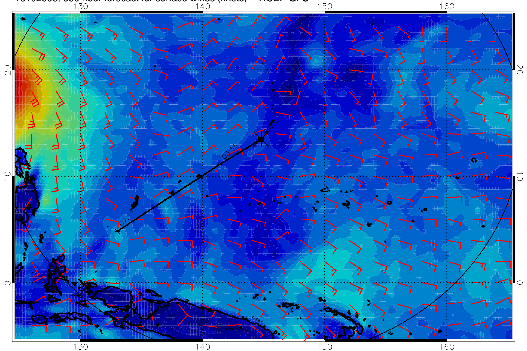
16102000, 060 hour forecast for surface winds (knots) -- NCEP GFS
