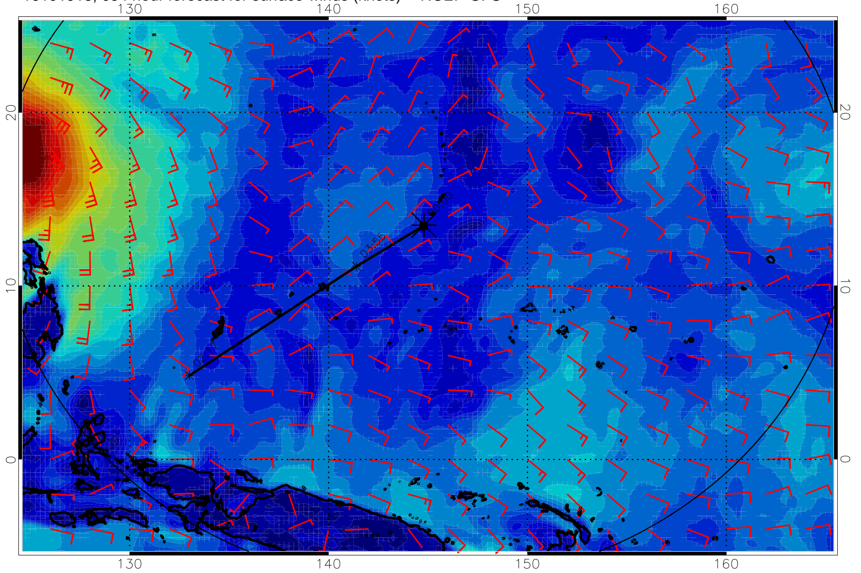
16101918, 054 hour forecast for surface winds (knots) -- NCEP GFS
