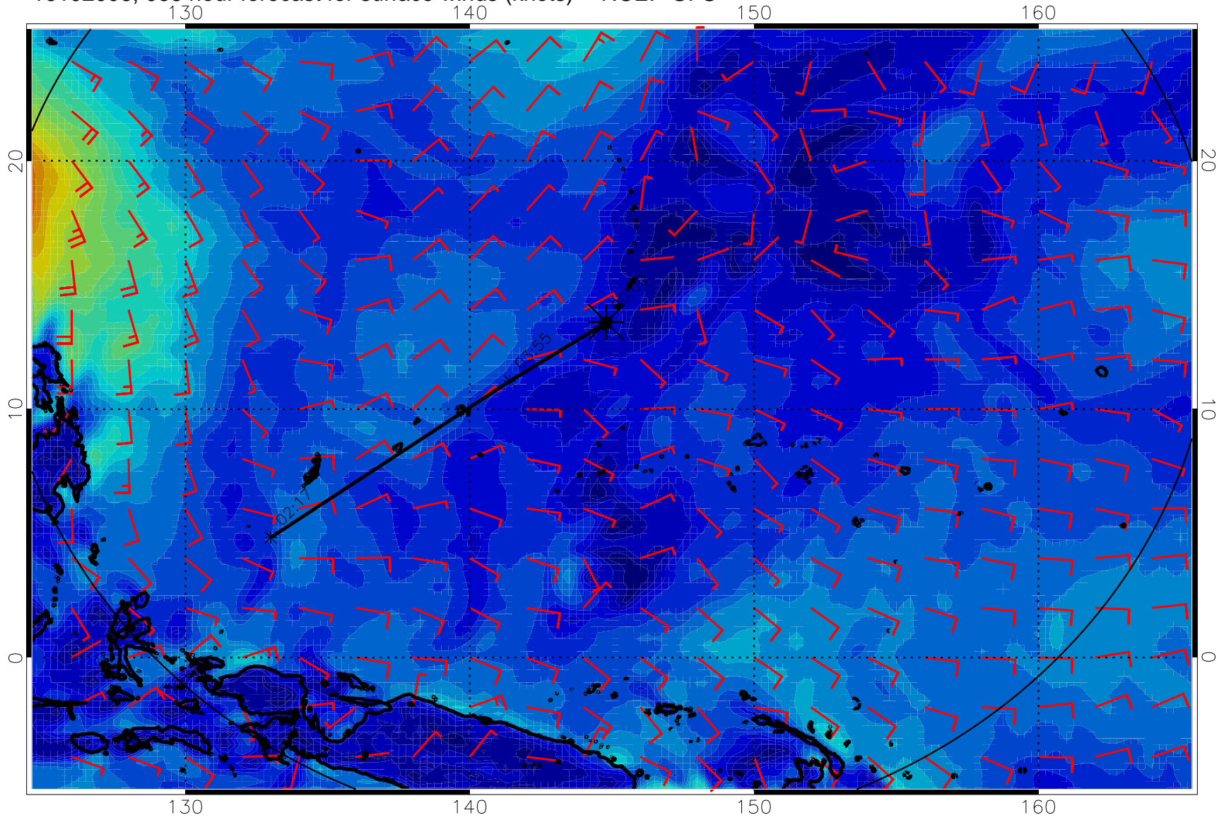
16102006, 066 hour forecast for surface winds (knots) -- NCEP GFS
