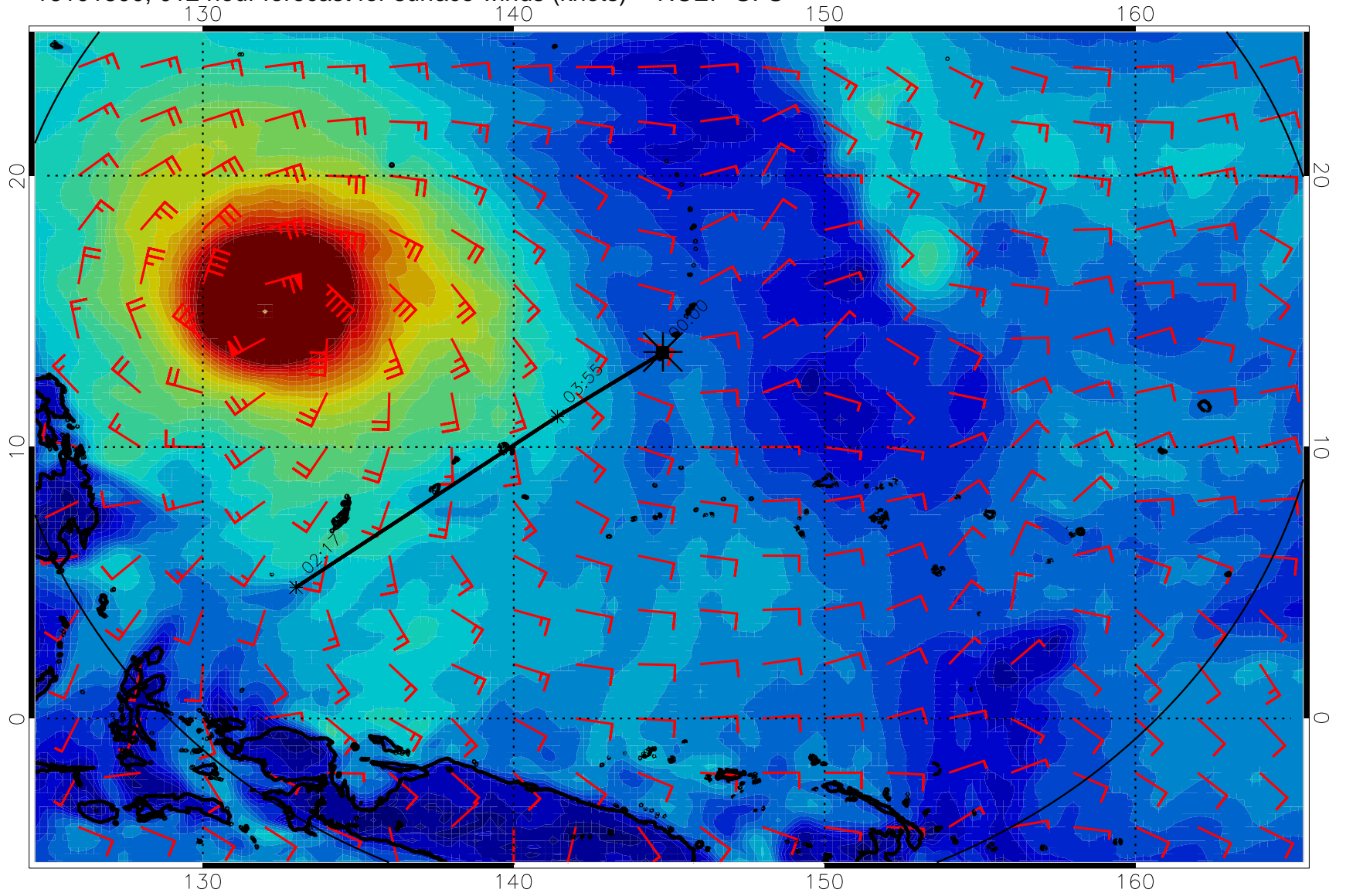
16101800, 012 hour forecast for surface winds (knots) -- NCEP GFS
