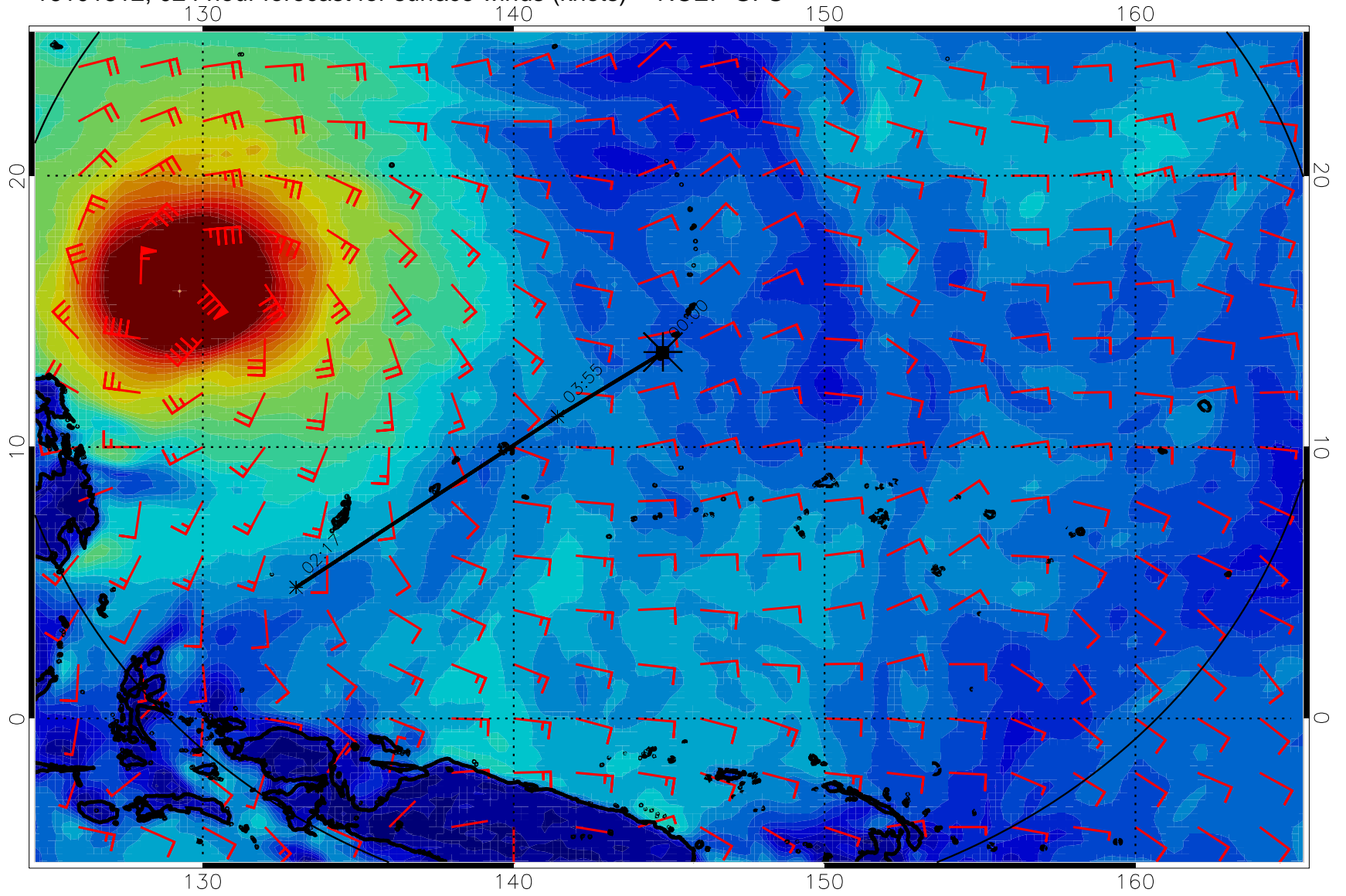
16101812, 024 hour forecast for surface winds (knots) -- NCEP GFS
