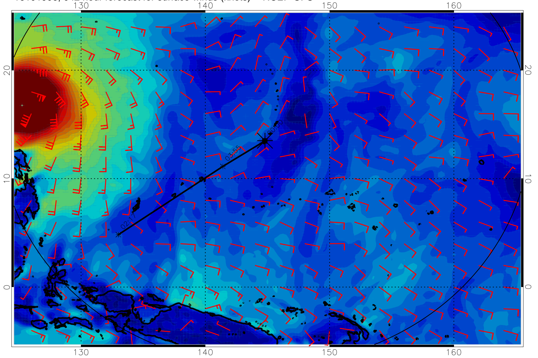
16101906, 042 hour forecast for surface winds (knots) -- NCEP GFS
