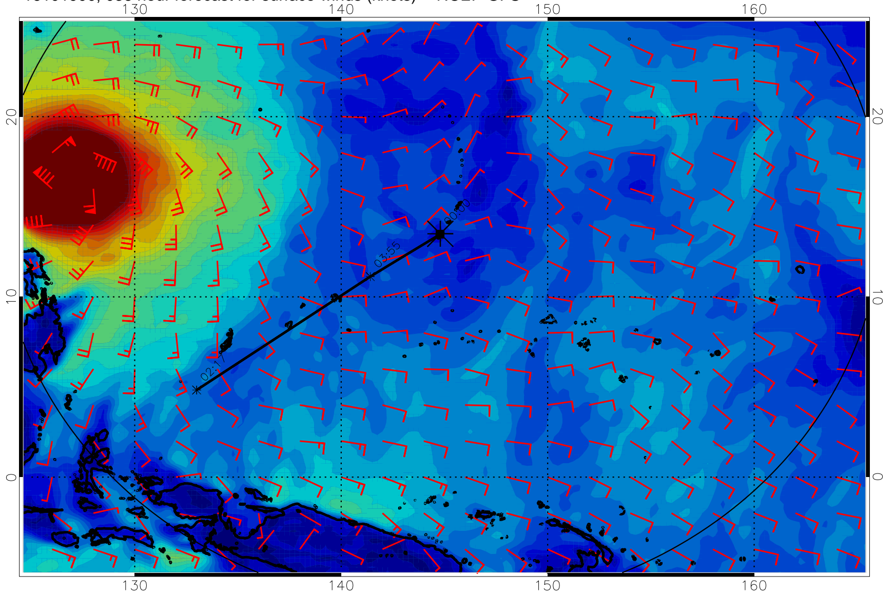
16101900, 036 hour forecast for surface winds (knots) -- NCEP GFS
