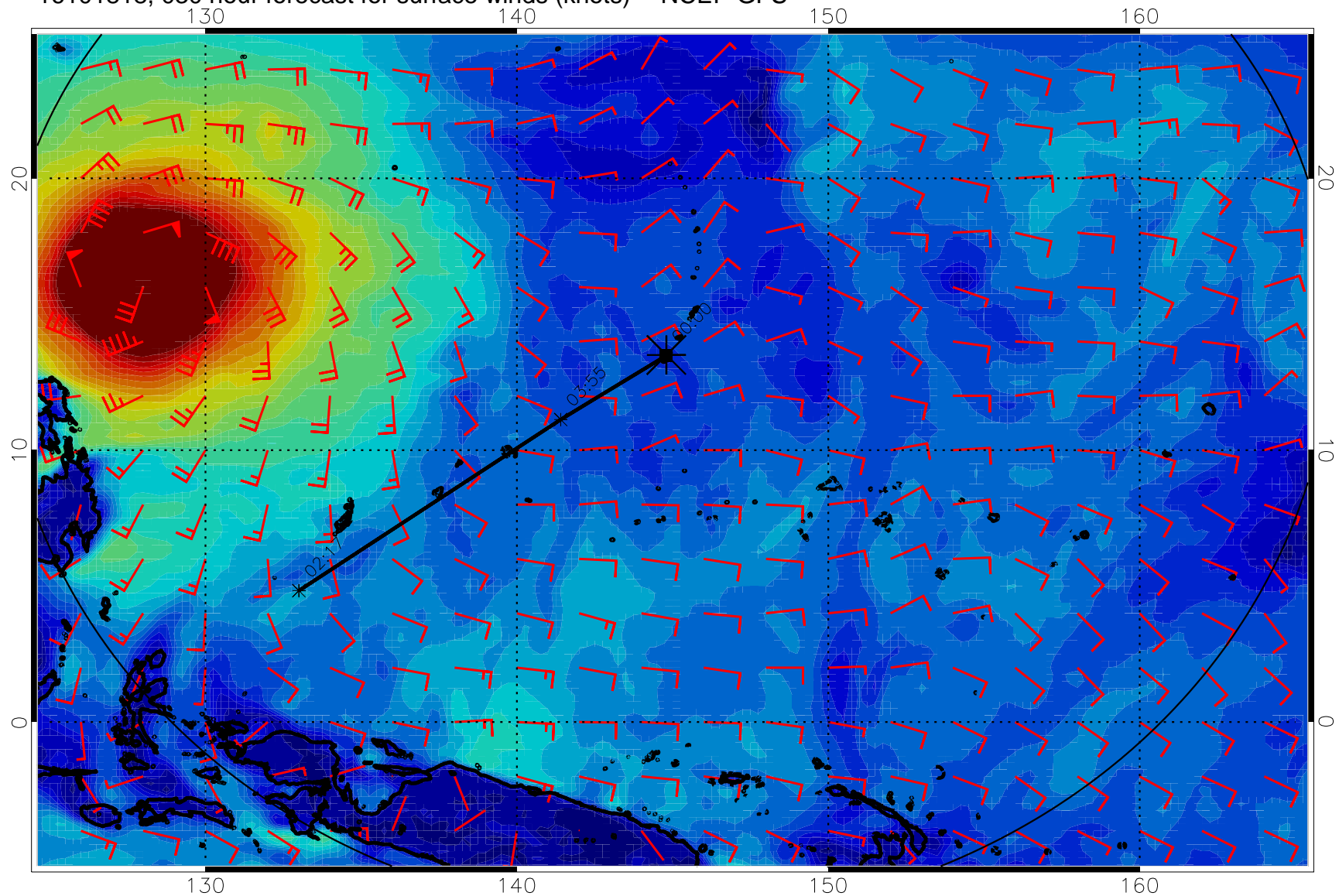
16101818, 030 hour forecast for surface winds (knots) -- NCEP GFS
