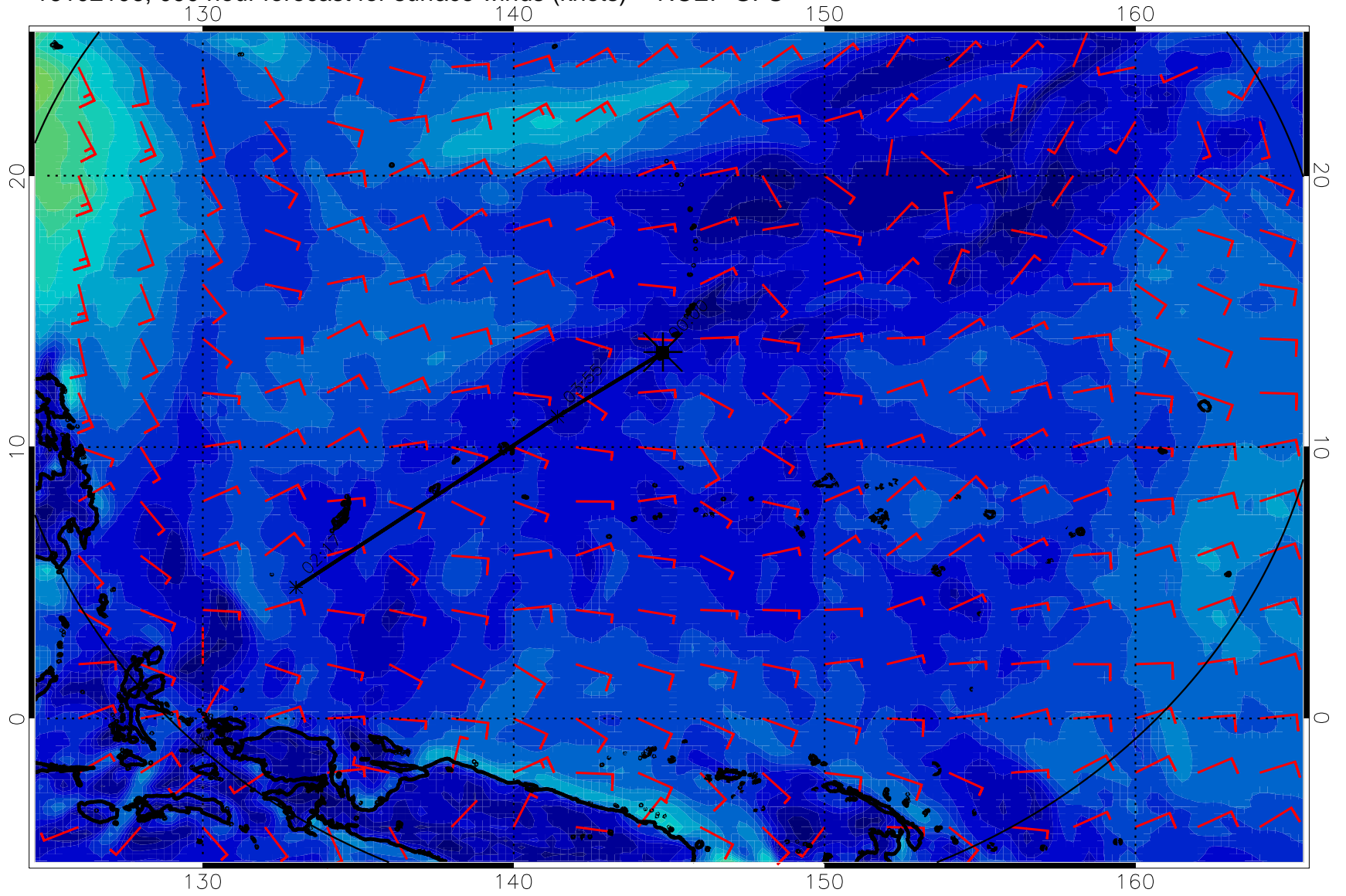
16102106, 090 hour forecast for surface winds (knots) -- NCEP GFS
