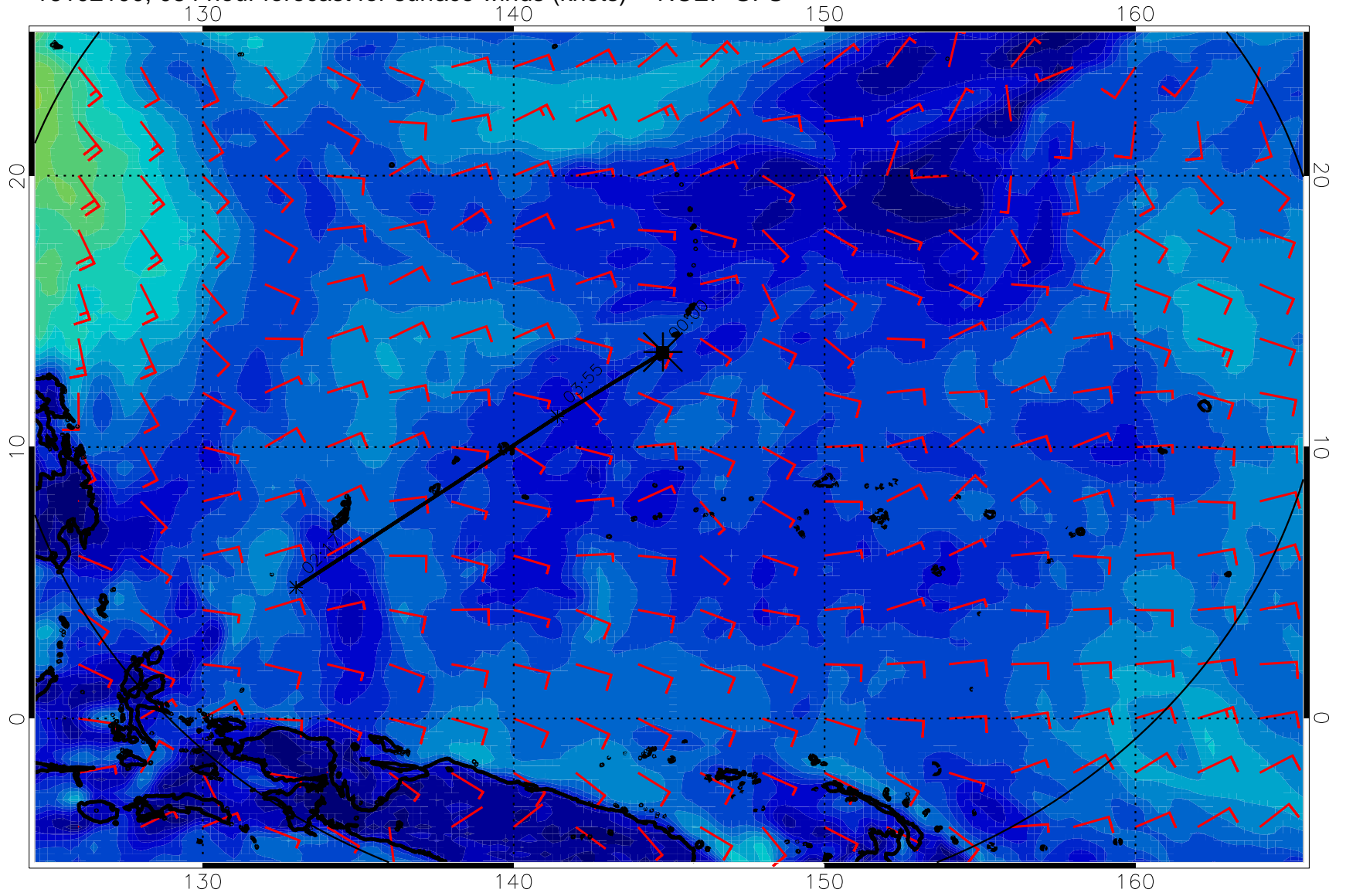
16102100, 084 hour forecast for surface winds (knots) -- NCEP GFS
