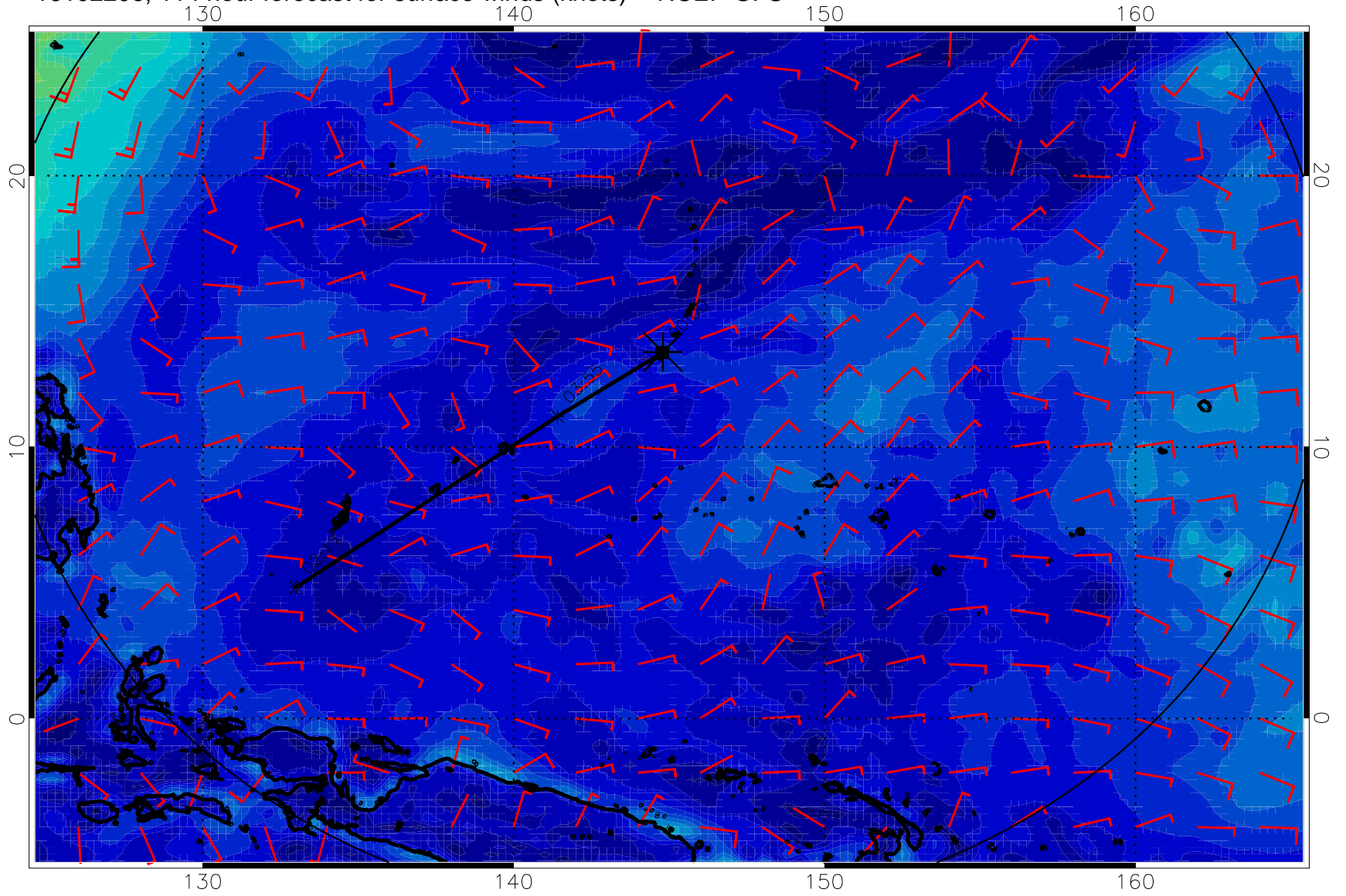
16102206, 114 hour forecast for surface winds (knots) -- NCEP GFS
