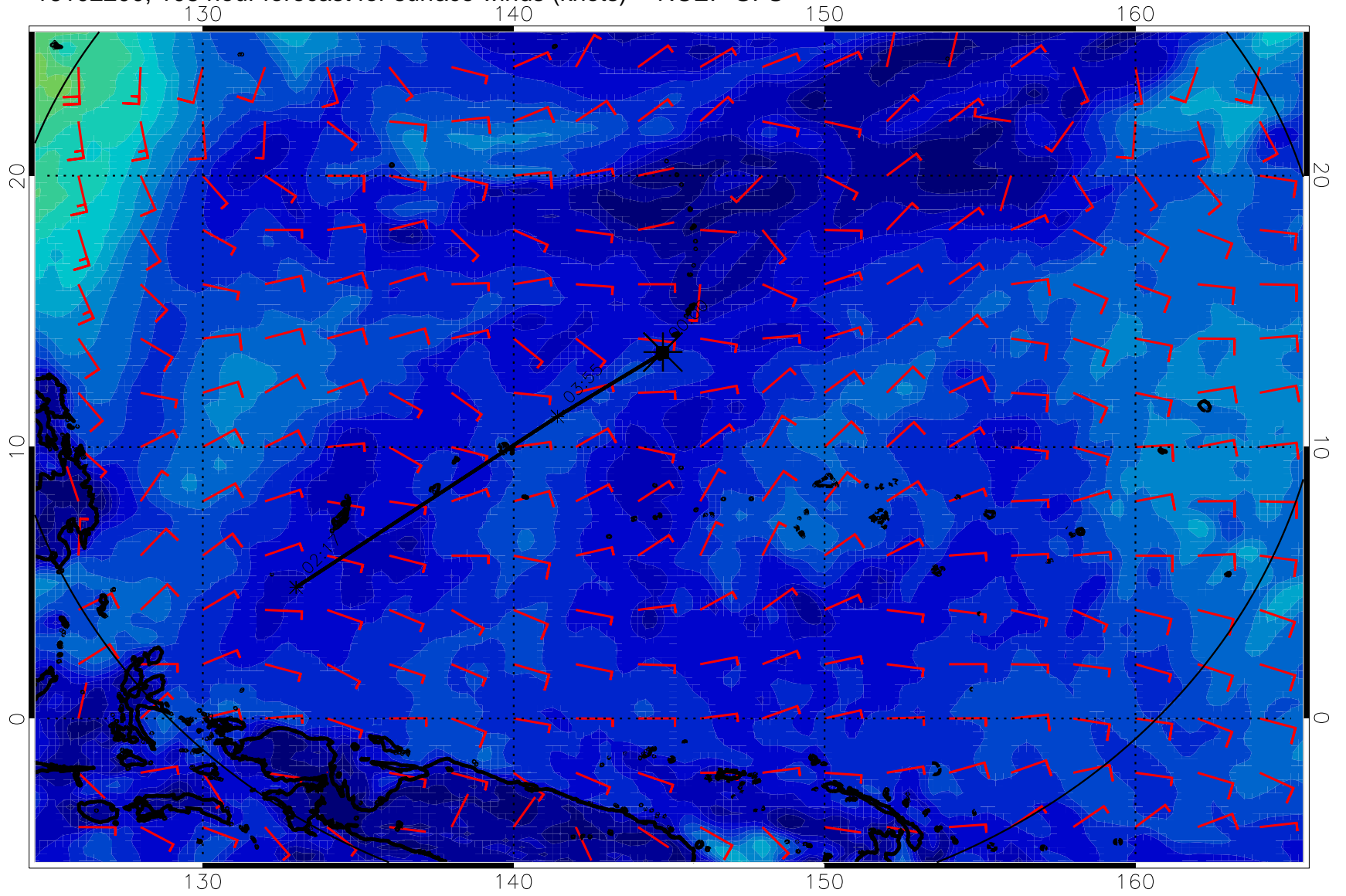
16102200, 108 hour forecast for surface winds (knots) -- NCEP GFS
