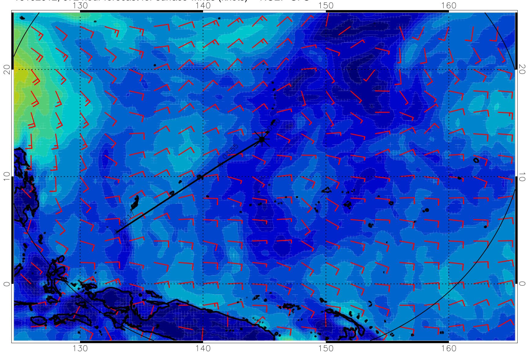
16102012, 072 hour forecast for surface winds (knots) -- NCEP GFS
