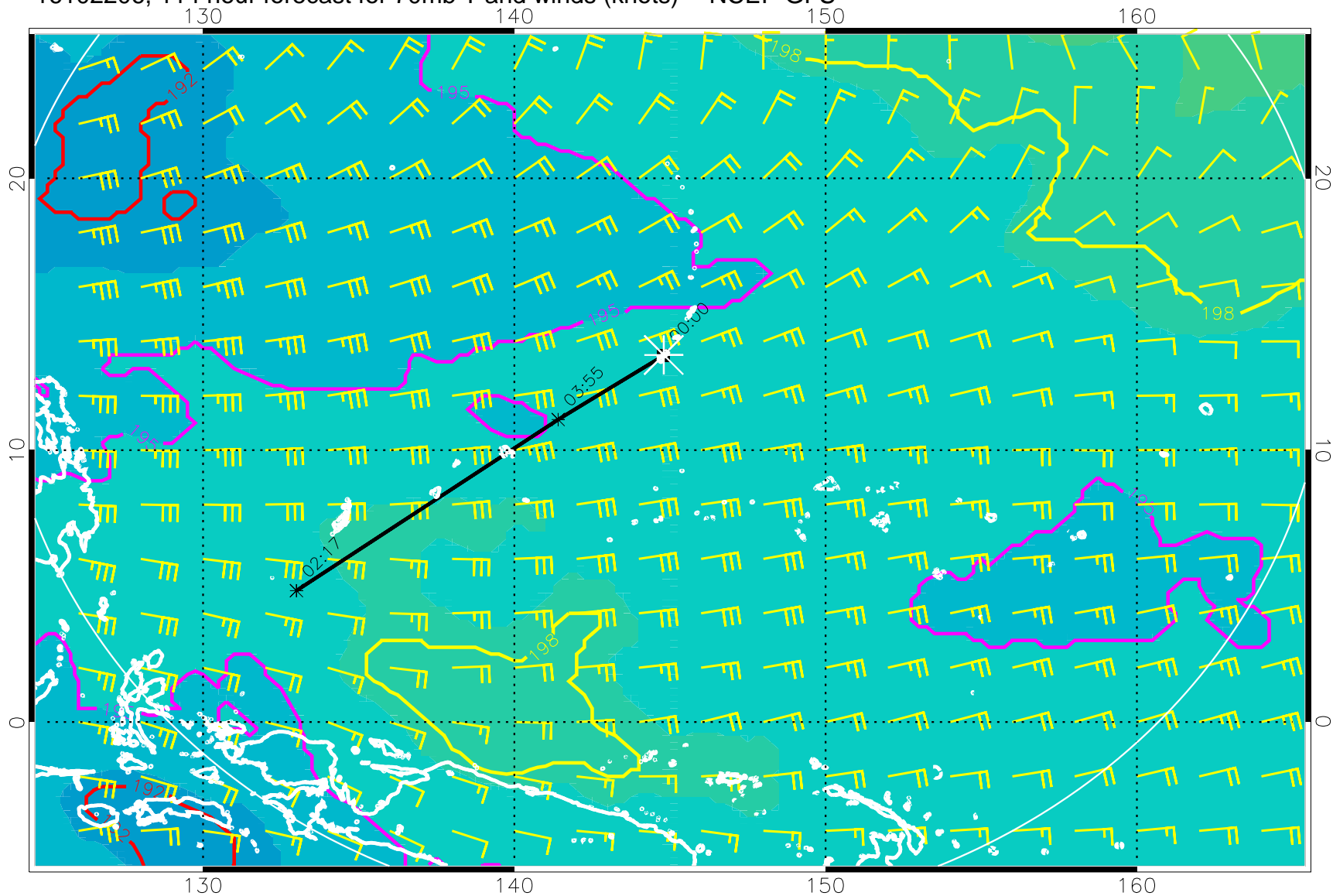
16102206, 114 hour forecast for 70mb T and winds (knots) -- NCEP GFS
