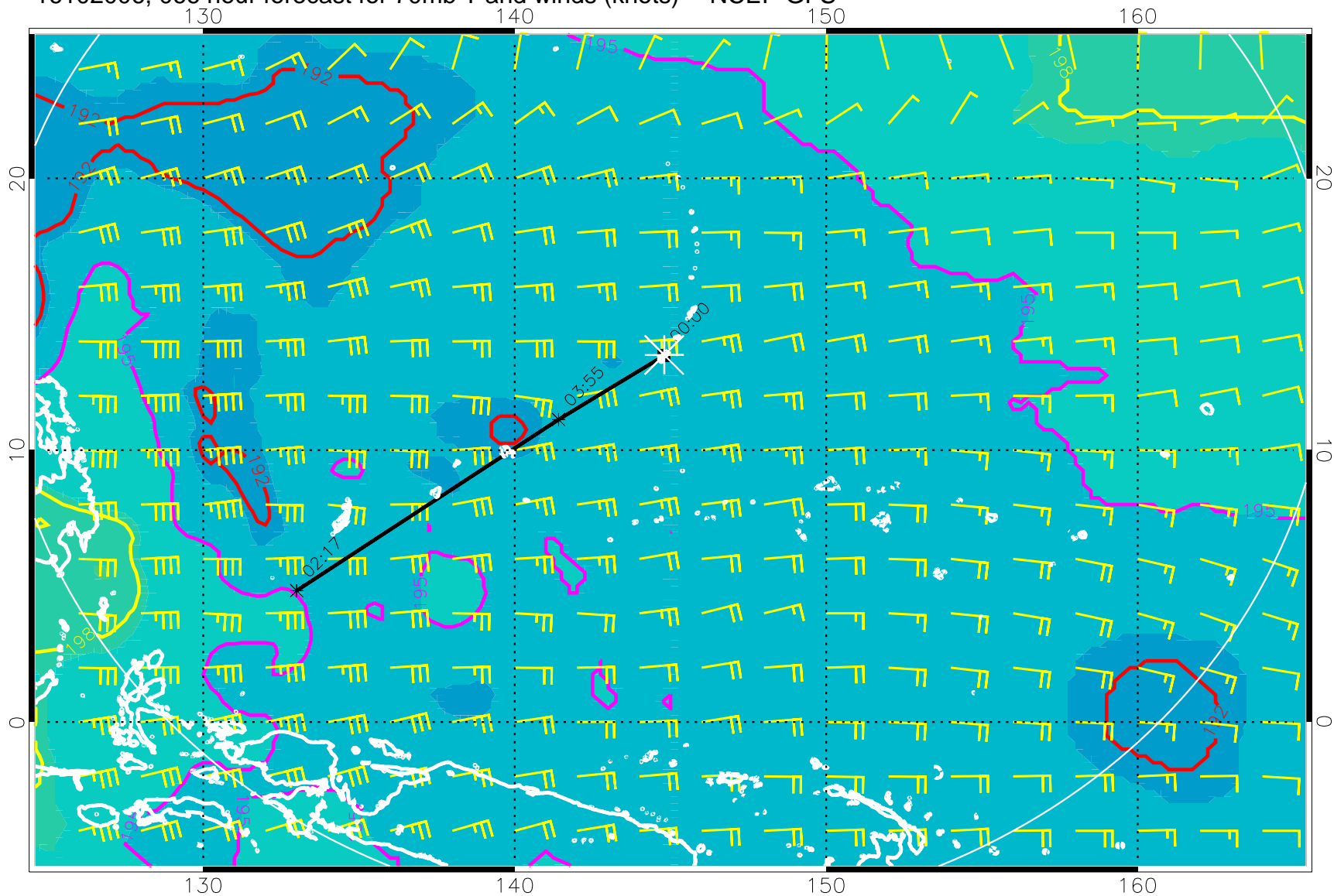
16102006, 066 hour forecast for 70mb T and winds (knots) -- NCEP GFS
