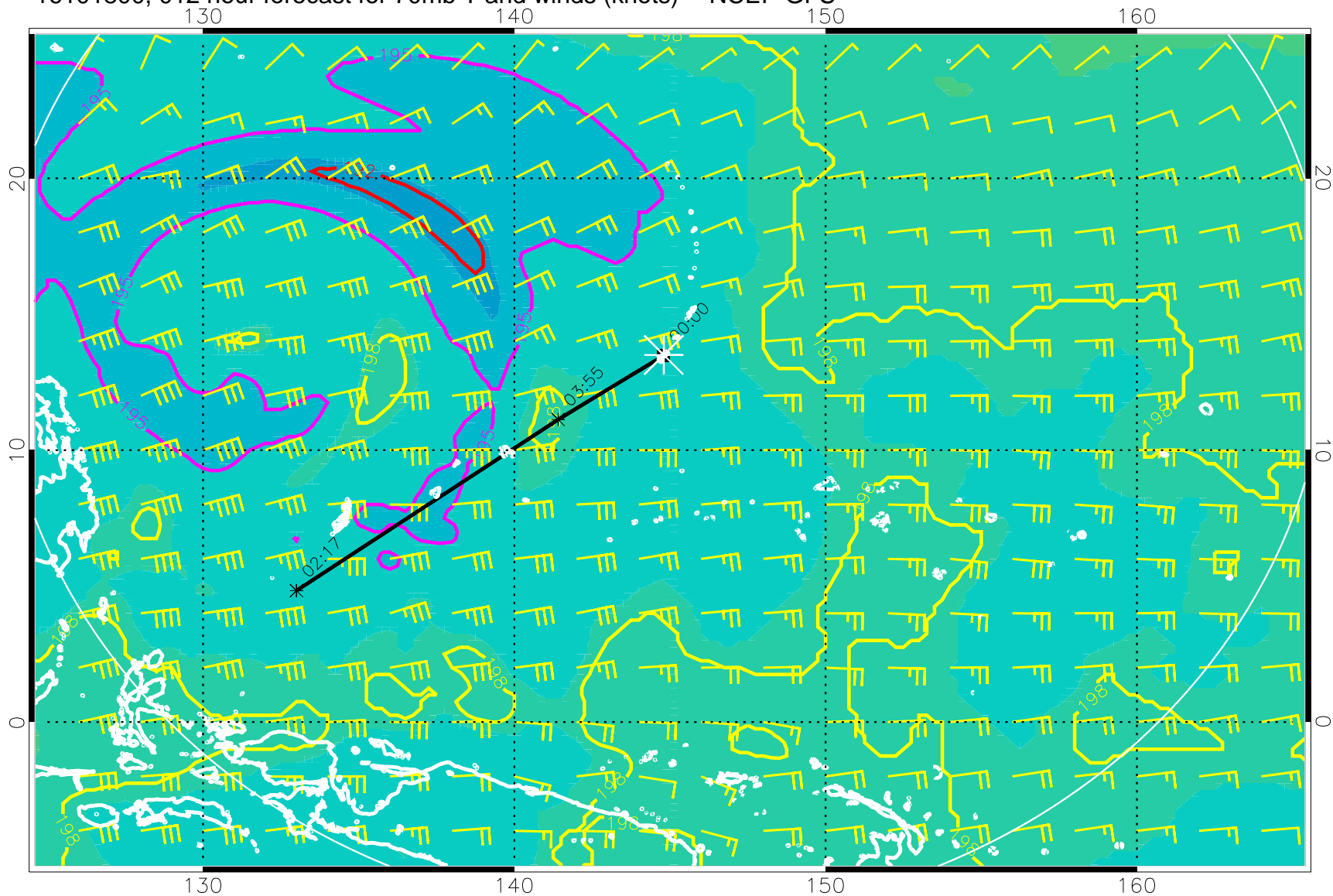
16101800, 012 hour forecast for 70mb T and winds (knots) -- NCEP GFS
