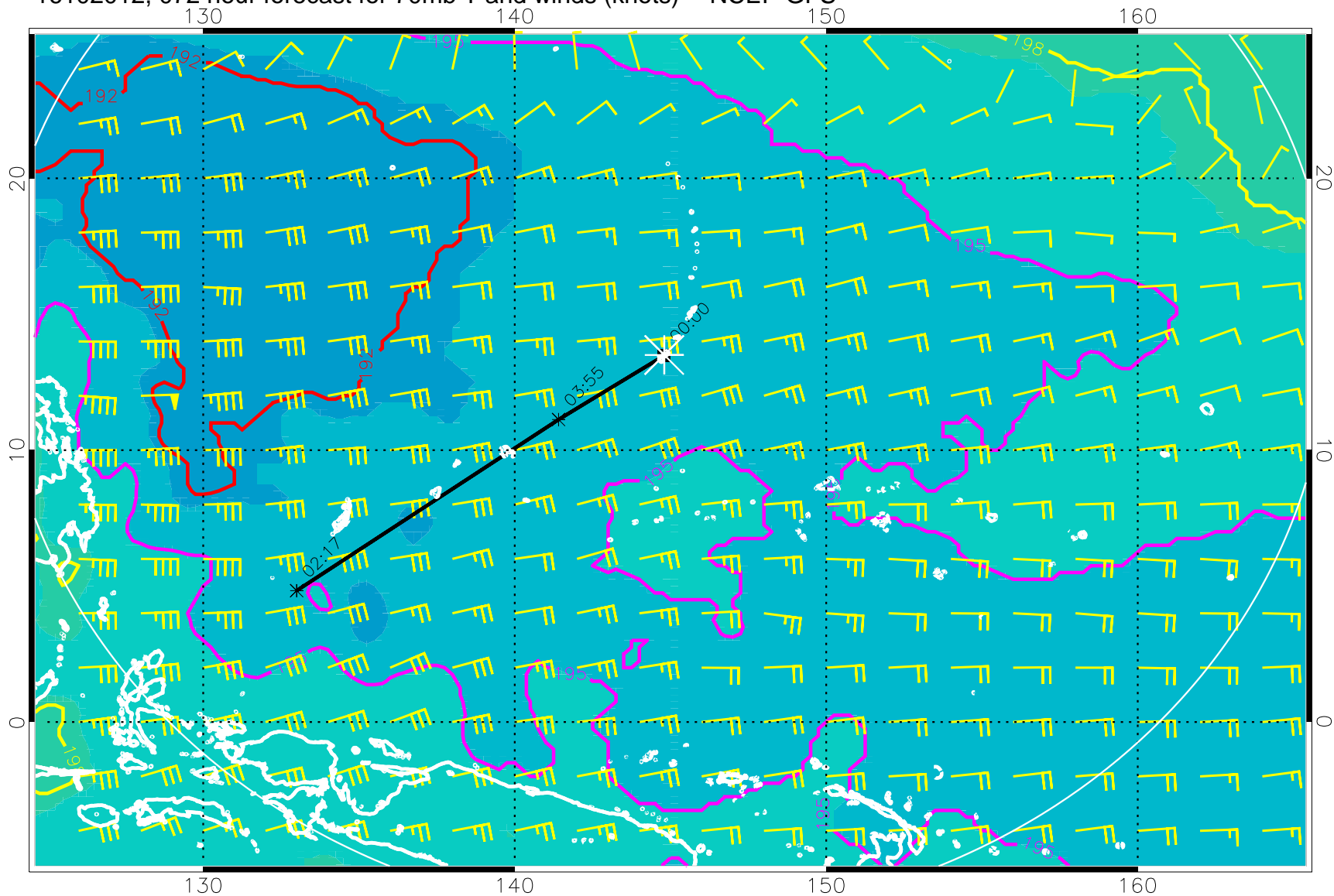
16102012, 072 hour forecast for 70mb T and winds (knots) -- NCEP GFS
