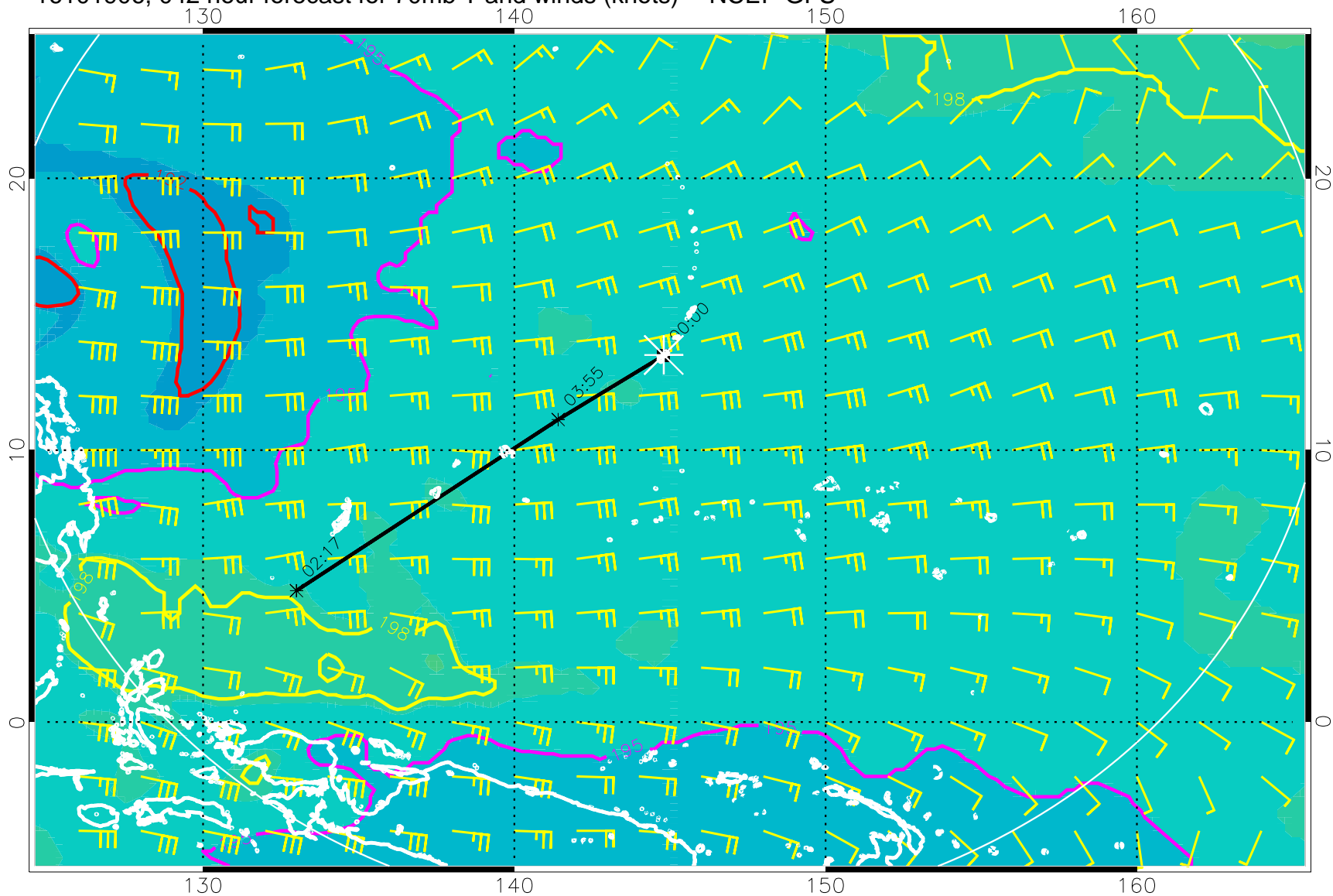
16101906, 042 hour forecast for 70mb T and winds (knots) -- NCEP GFS
