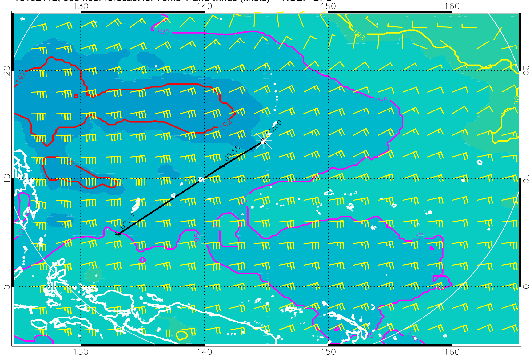
16102112, 096 hour forecast for 70mb T and winds (knots) -- NCEP GFS
