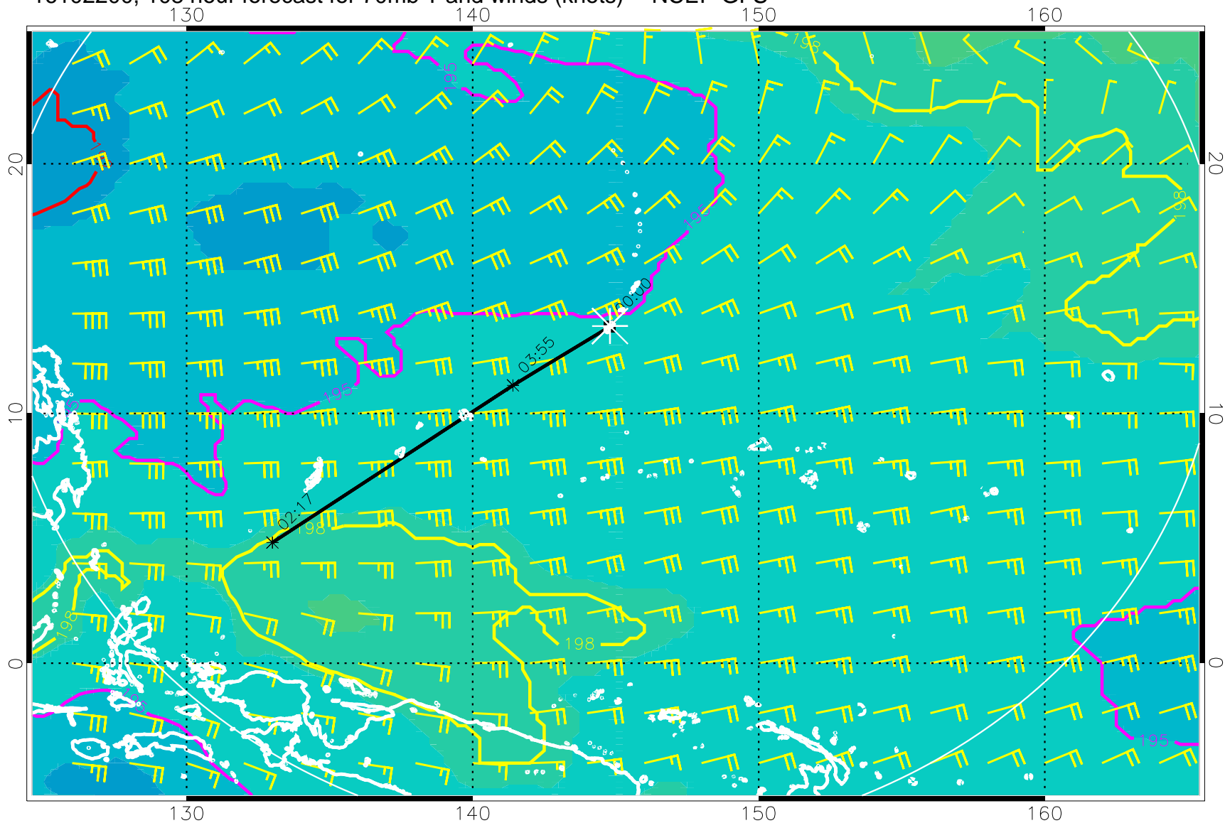
16102200, 108 hour forecast for 70mb T and winds (knots) -- NCEP GFS
