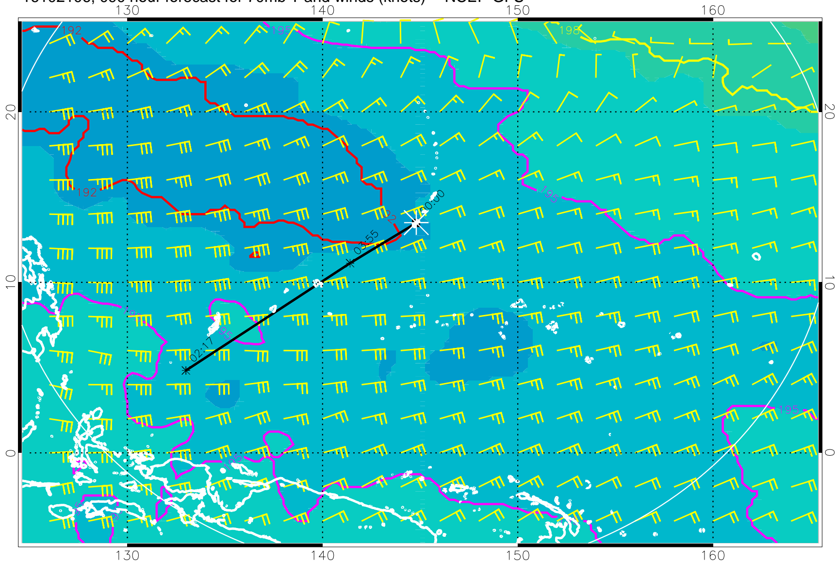
16102106, 090 hour forecast for 70mb T and winds (knots) -- NCEP GFS
