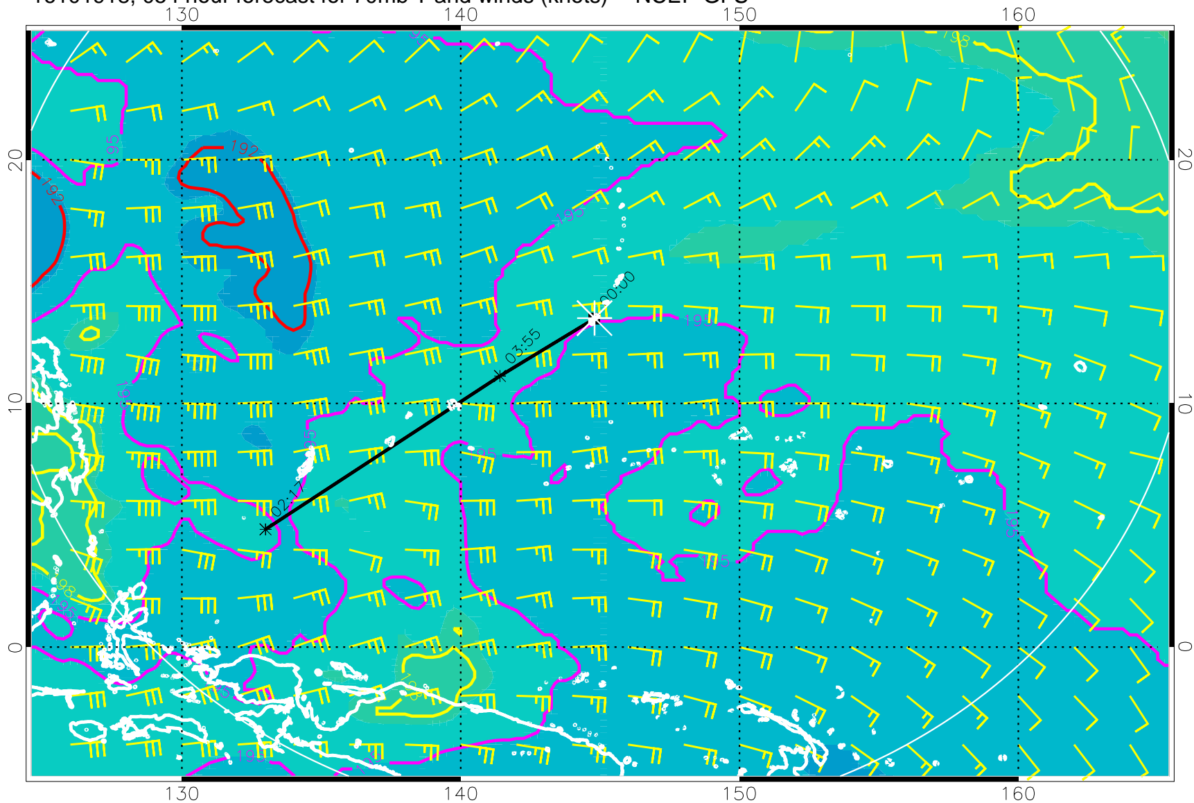
16101918, 054 hour forecast for 70mb T and winds (knots) -- NCEP GFS
