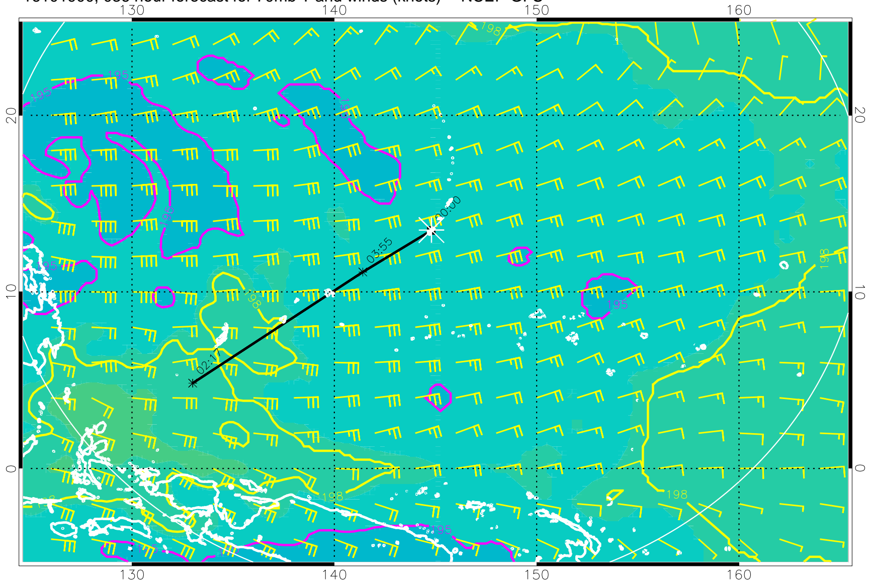
16101900, 036 hour forecast for 70mb T and winds (knots) -- NCEP GFS
