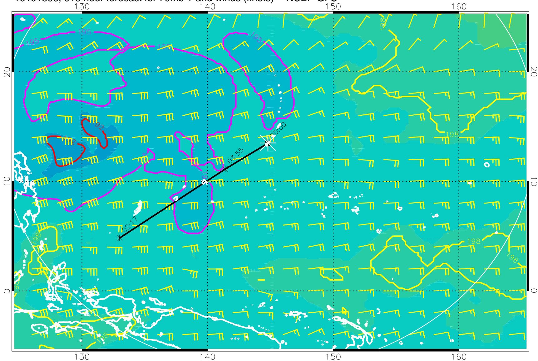
16101806, 018 hour forecast for 70mb T and winds (knots) -- NCEP GFS
