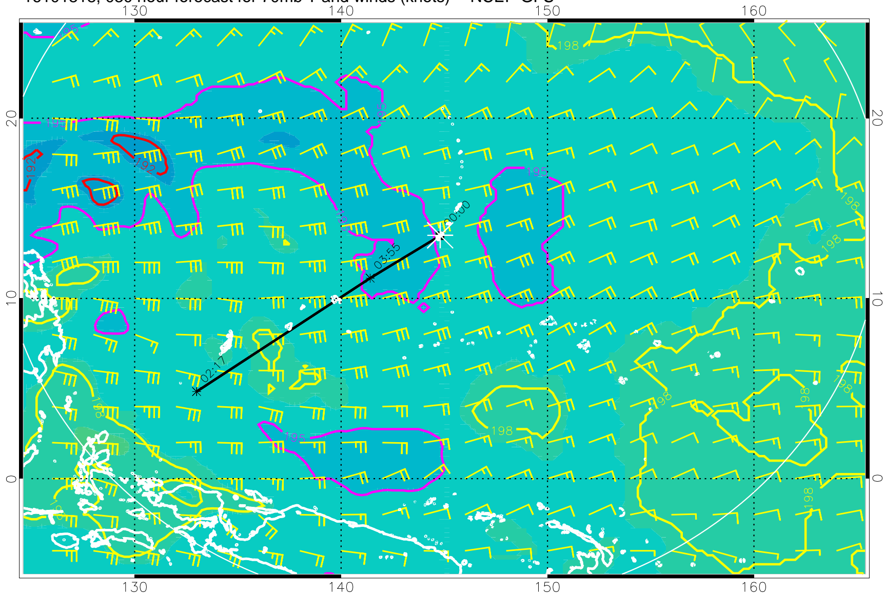
16101818, 030 hour forecast for 70mb T and winds (knots) -- NCEP GFS
