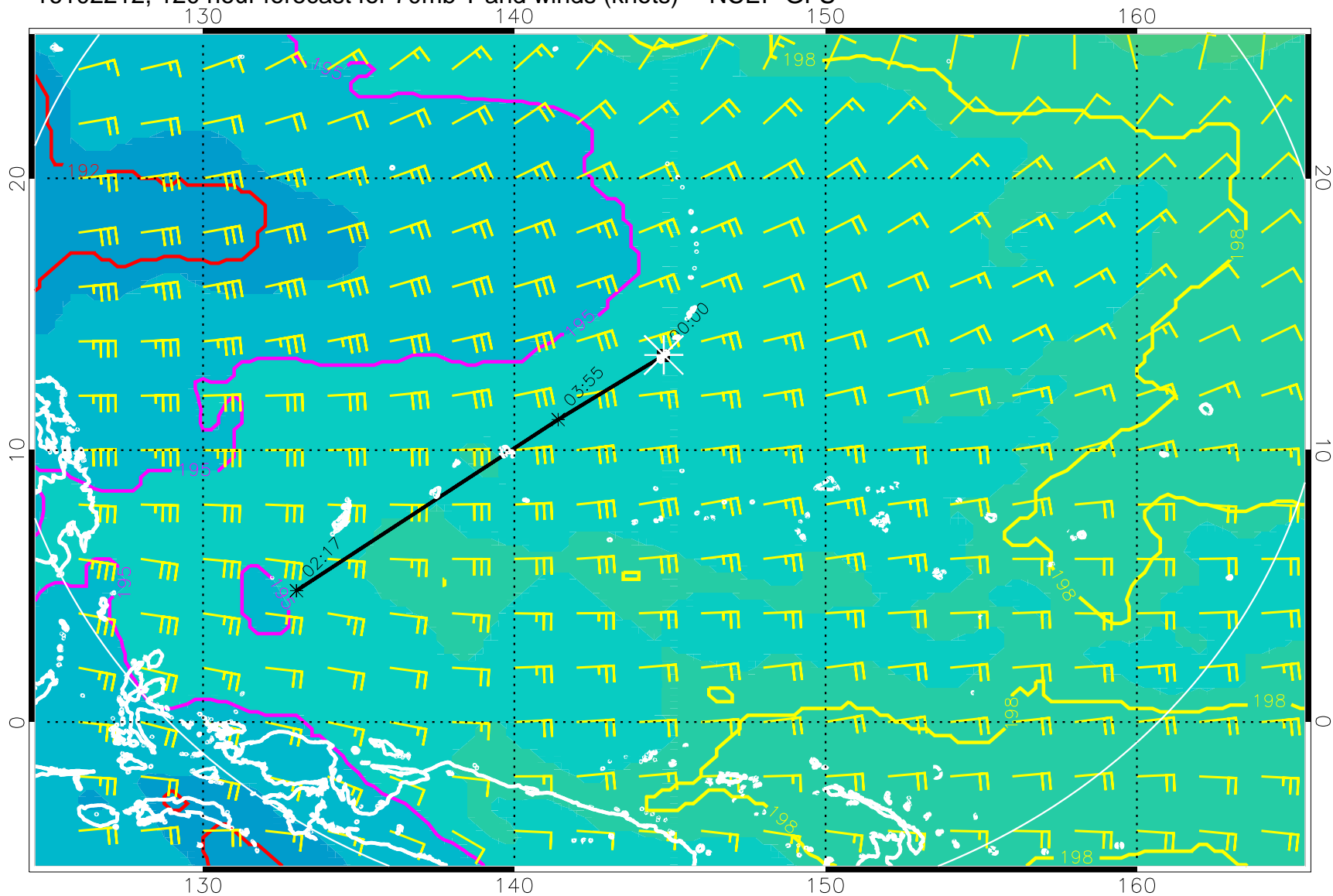
16102212, 120 hour forecast for 70mb T and winds (knots) -- NCEP GFS
