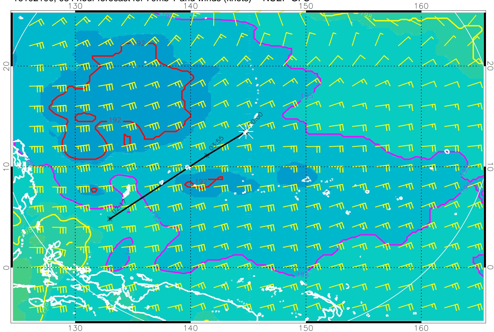
16102100, 084 hour forecast for 70mb T and winds (knots) -- NCEP GFS
