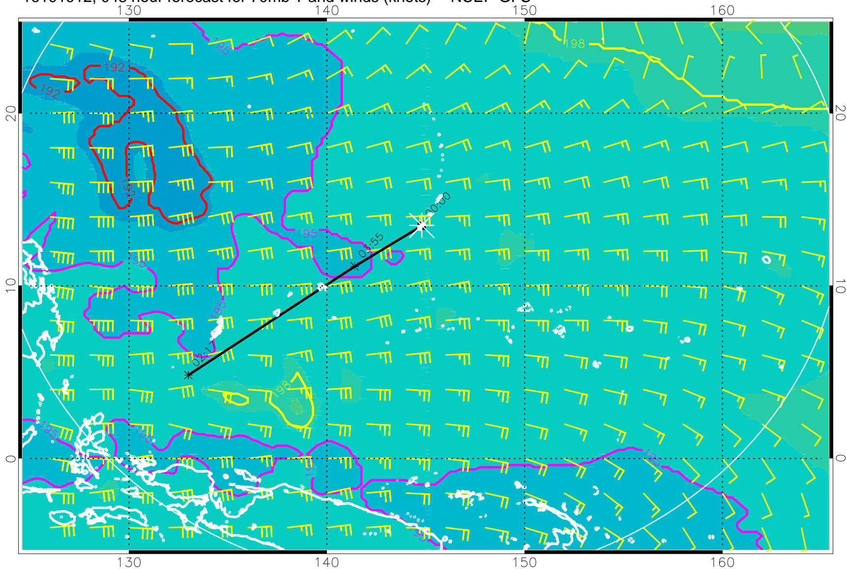
16101912, 048 hour forecast for 70mb T and winds (knots) -- NCEP GFS
