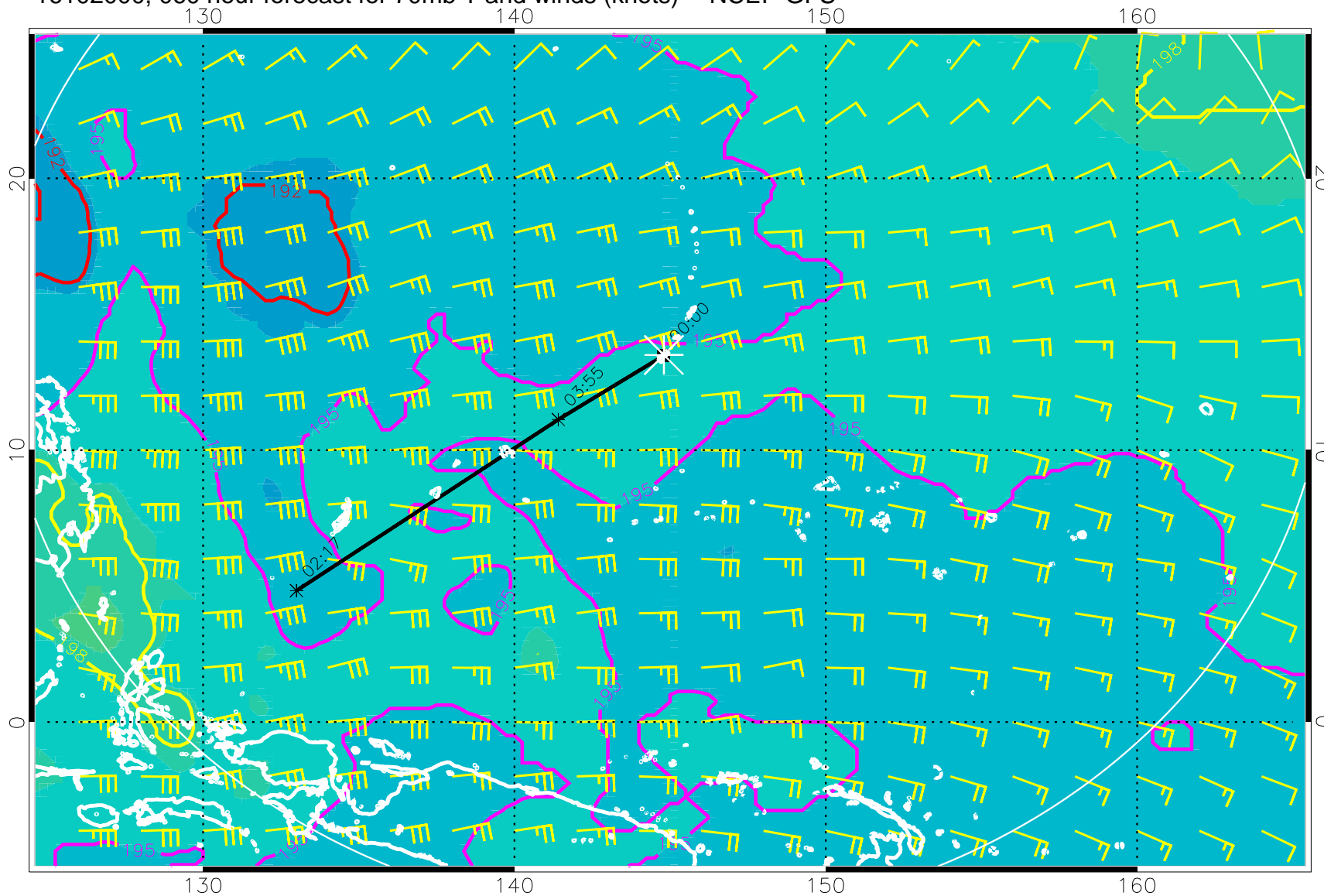
16102000, 060 hour forecast for 70mb T and winds (knots) -- NCEP GFS
