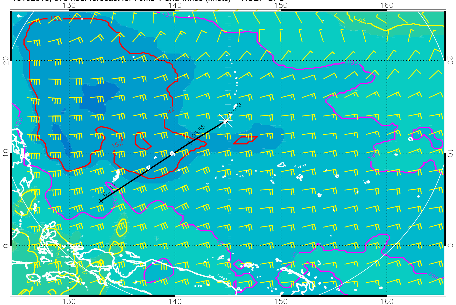
16102018, 078 hour forecast for 70mb T and winds (knots) -- NCEP GFS
