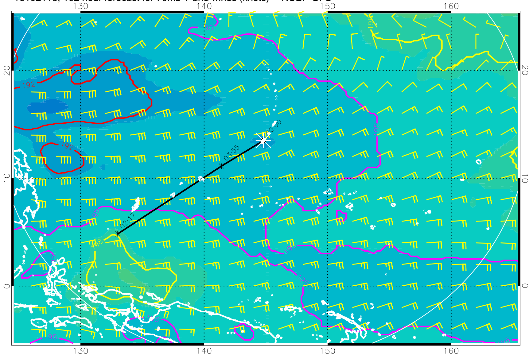
16102118, 102 hour forecast for 70mb T and winds (knots) -- NCEP GFS
