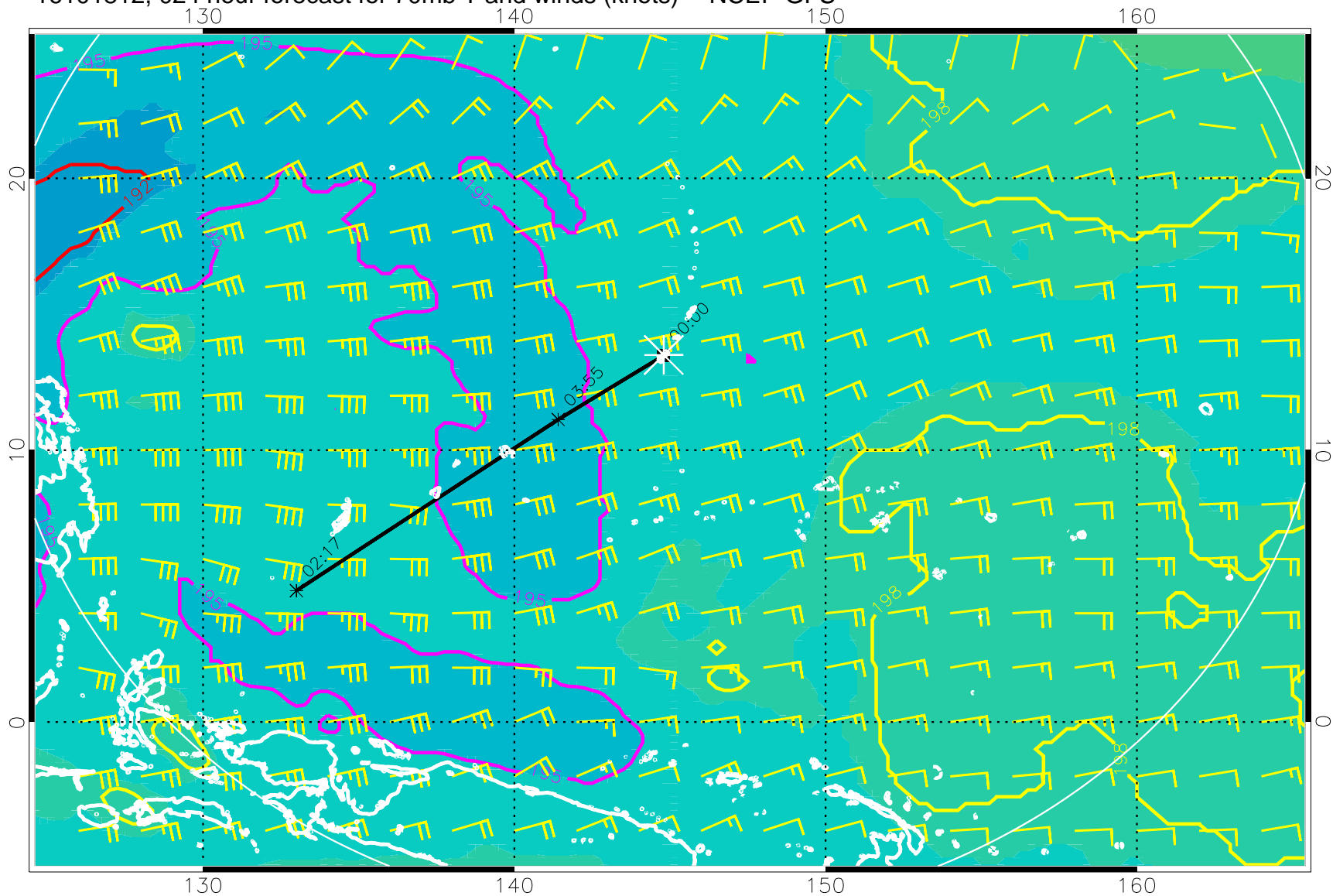
16101812, 024 hour forecast for 70mb T and winds (knots) -- NCEP GFS
