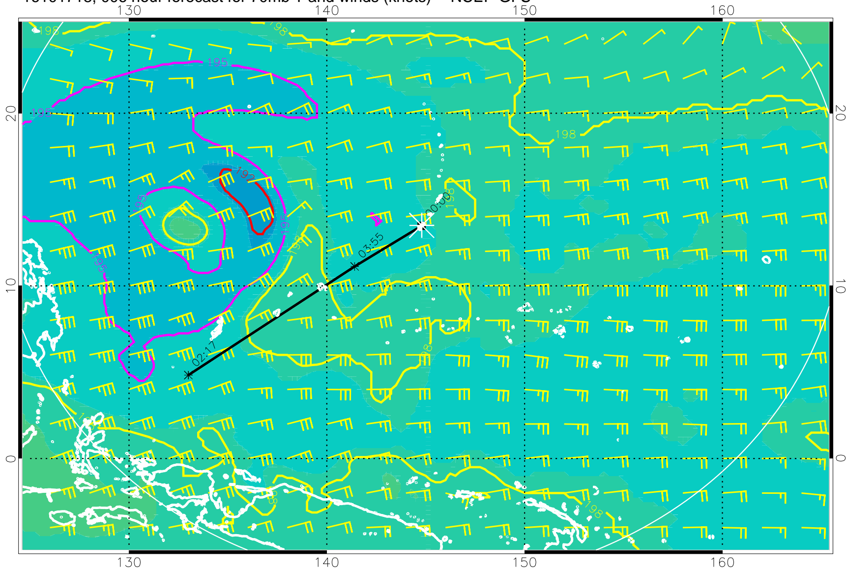
16101718, 006 hour forecast for 70mb T and winds (knots) -- NCEP GFS
