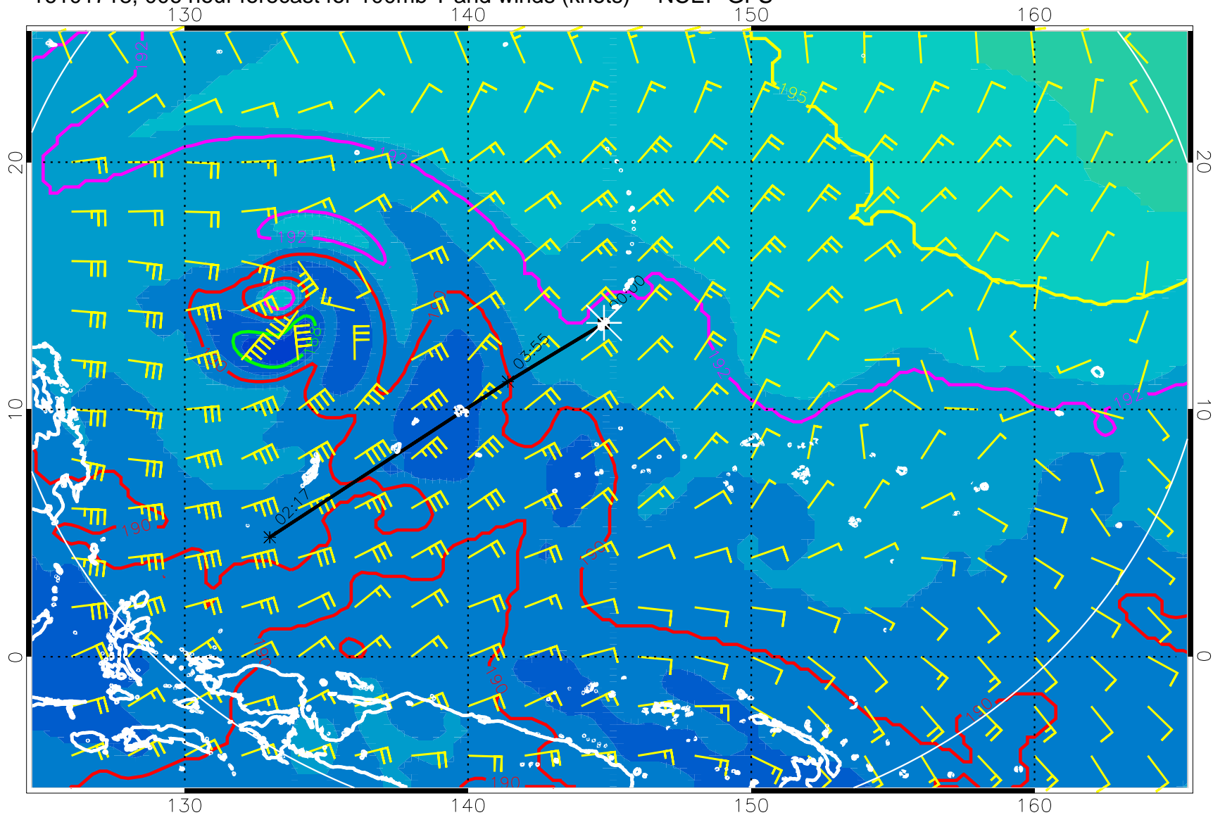
16101718, 006 hour forecast for 100mb T and winds (knots) -- NCEP GFS
