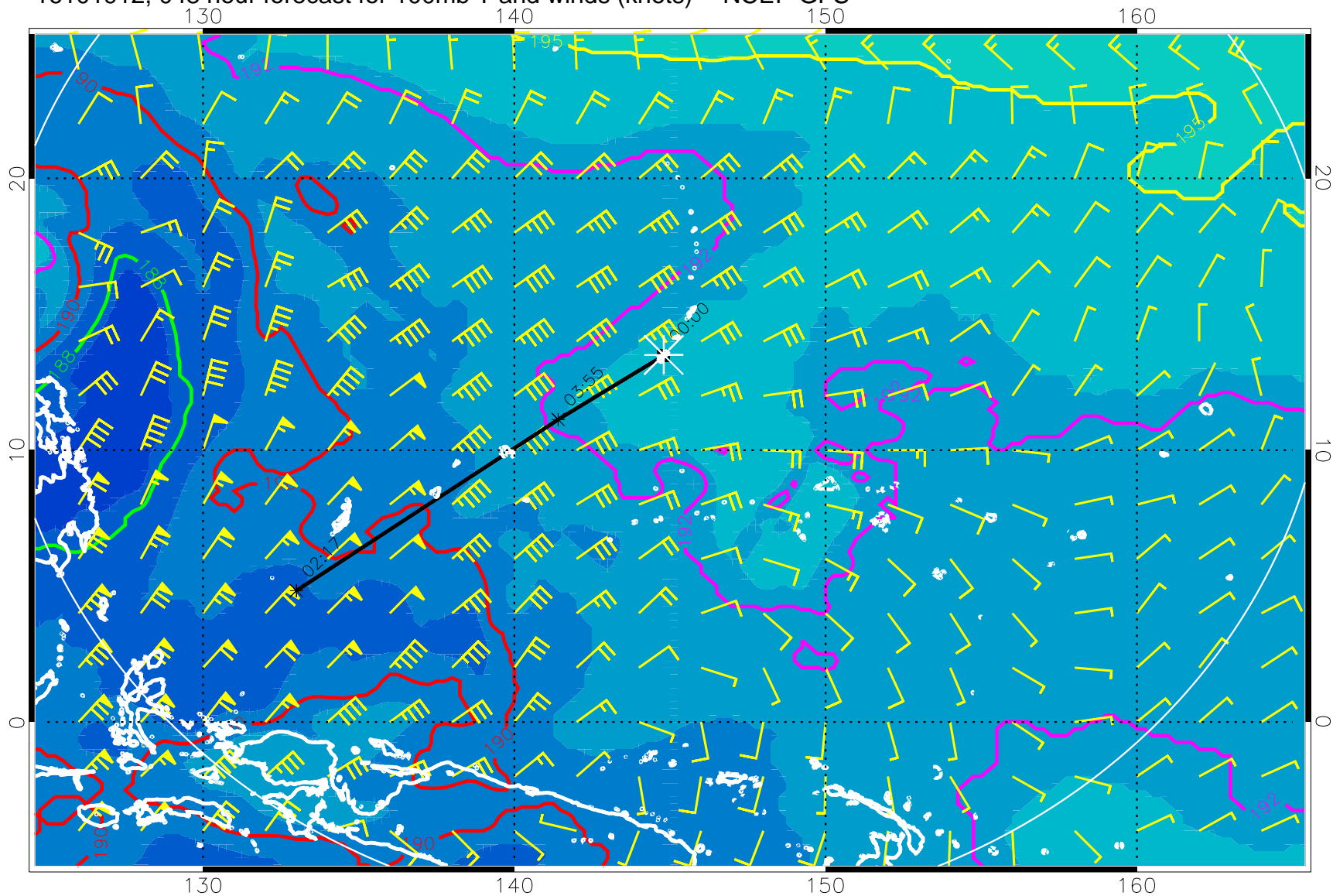
16101912, 048 hour forecast for 100mb T and winds (knots) -- NCEP GFS
