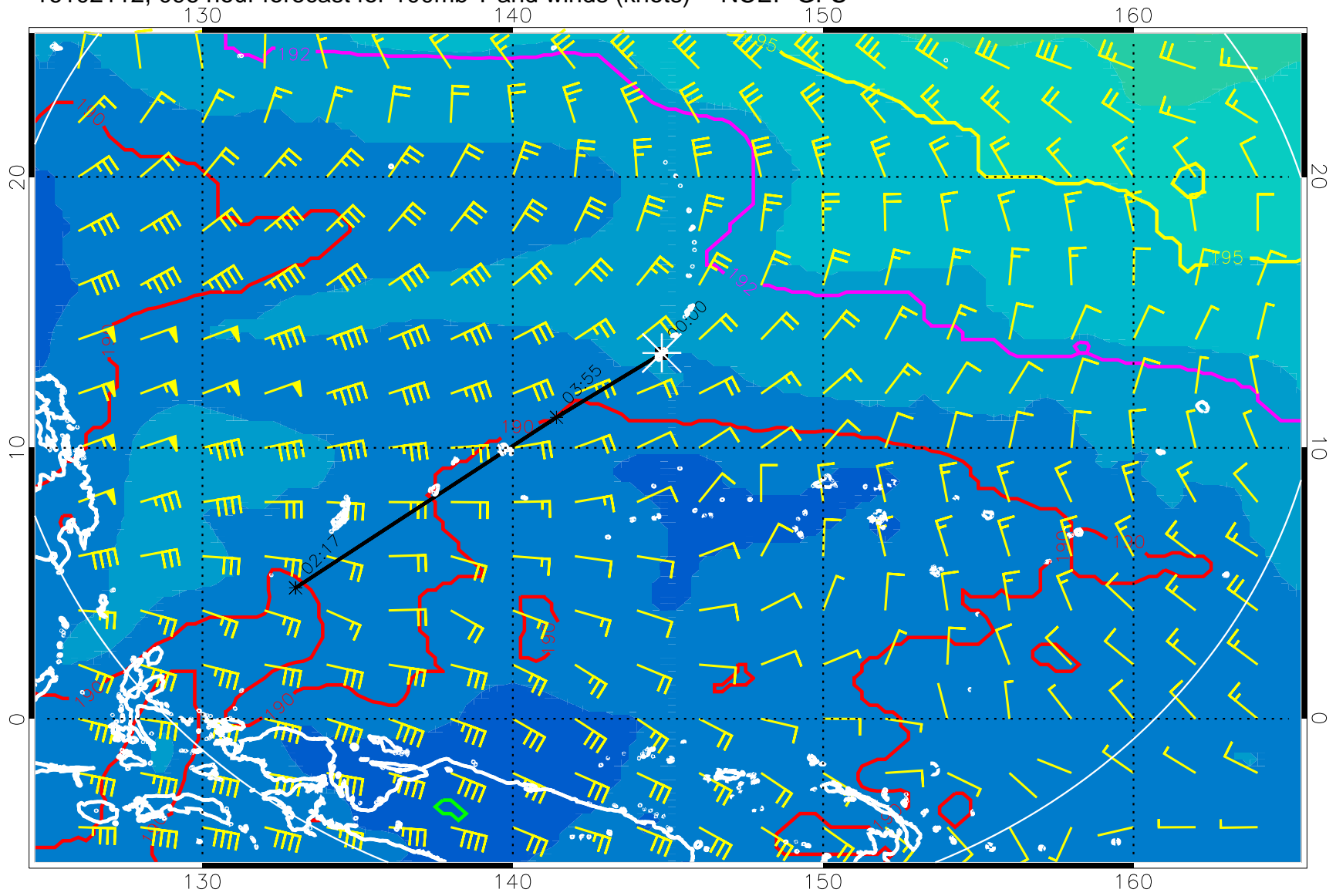
16102112, 096 hour forecast for 100mb T and winds (knots) -- NCEP GFS
