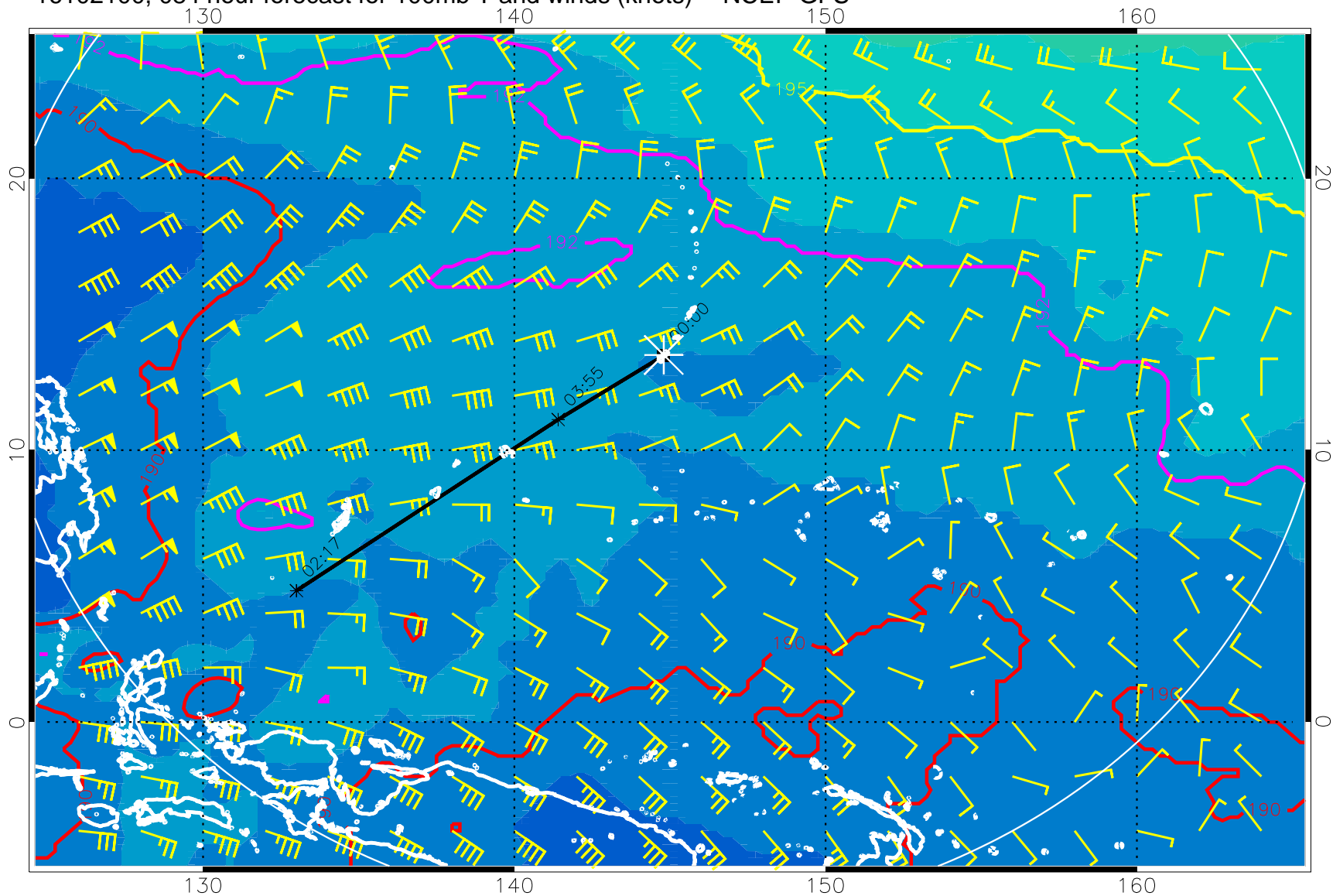
16102100, 084 hour forecast for 100mb T and winds (knots) -- NCEP GFS
