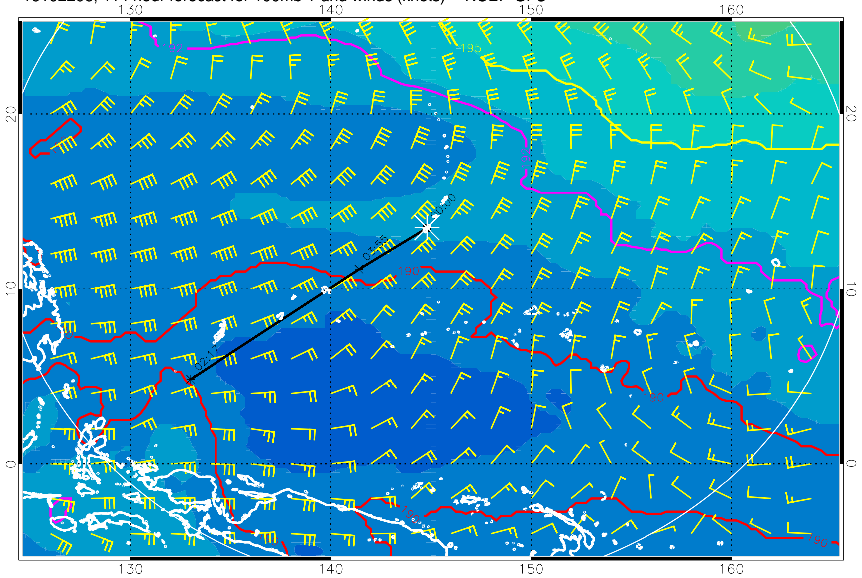
16102206, 114 hour forecast for 100mb T and winds (knots) -- NCEP GFS
