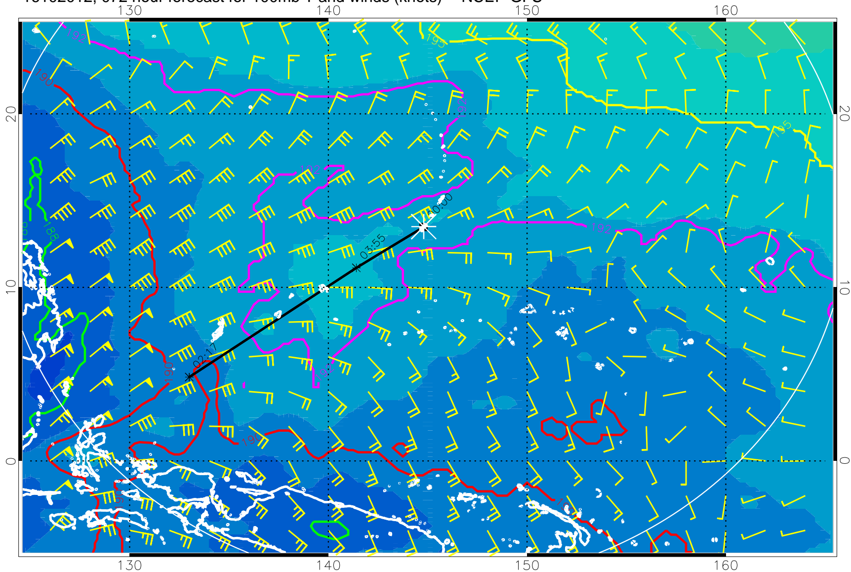
16102012, 072 hour forecast for 100mb T and winds (knots) -- NCEP GFS
