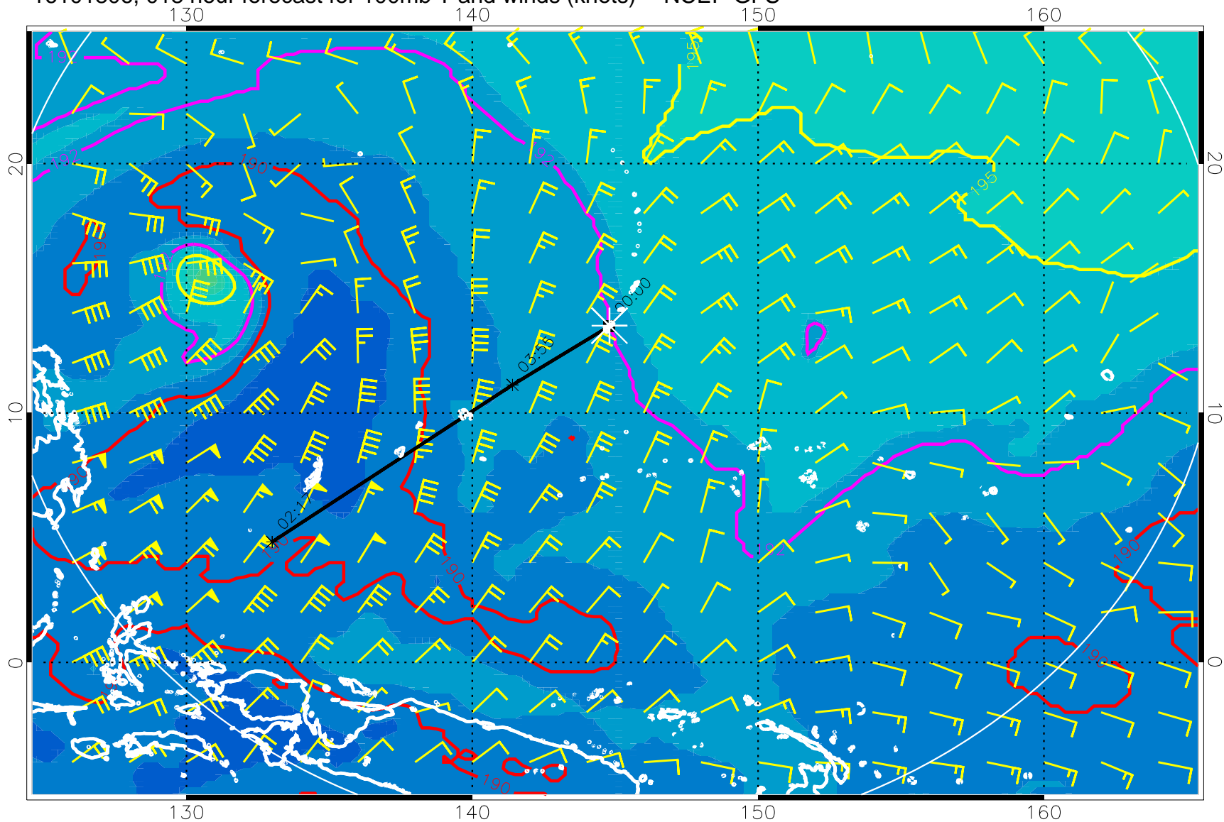
16101806, 018 hour forecast for 100mb T and winds (knots) -- NCEP GFS
