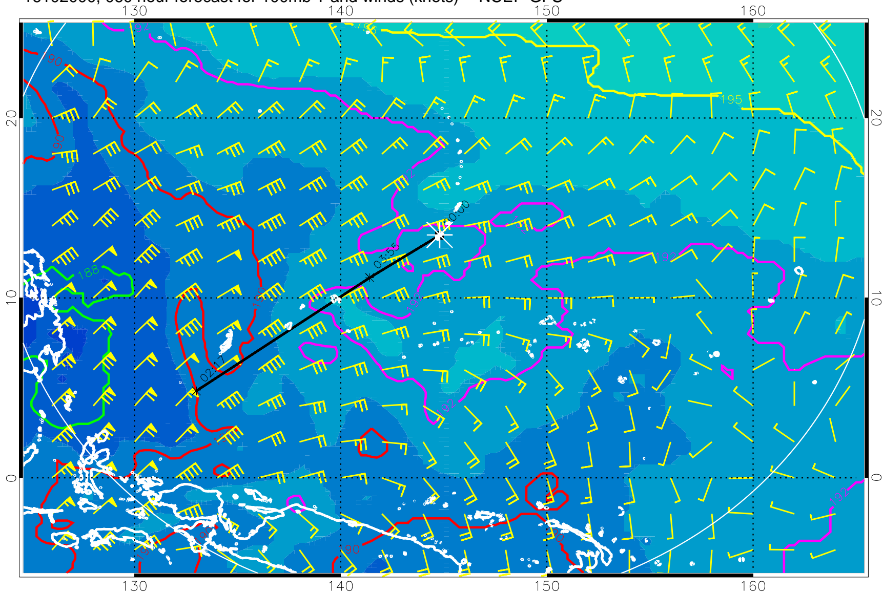
16102000, 060 hour forecast for 100mb T and winds (knots) -- NCEP GFS
