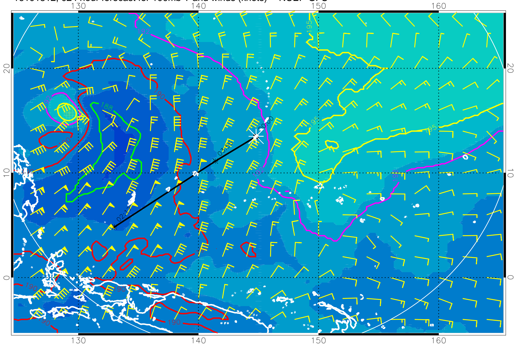
16101812, 024 hour forecast for 100mb T and winds (knots) -- NCEP GFS
