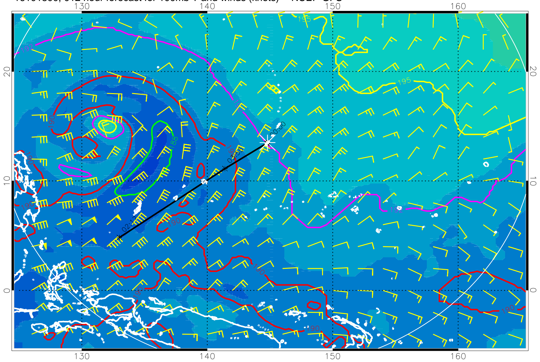
16101800, 012 hour forecast for 100mb T and winds (knots) -- NCEP GFS
