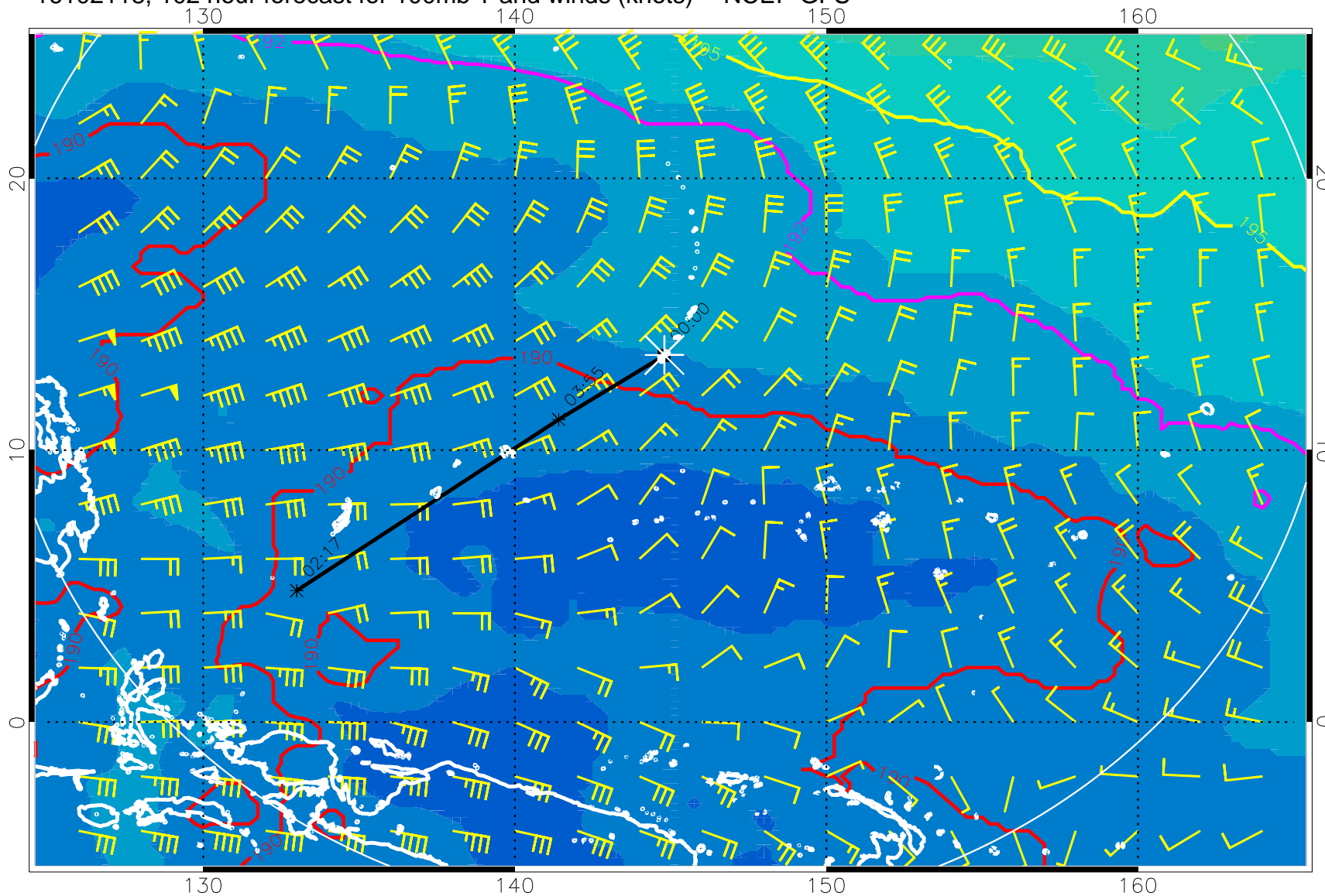
16102118, 102 hour forecast for 100mb T and winds (knots) -- NCEP GFS
