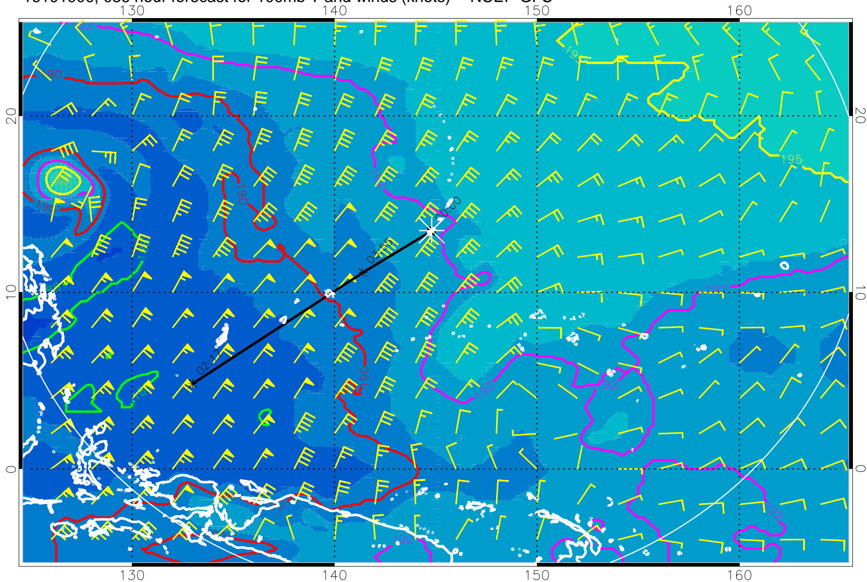
16101900, 036 hour forecast for 100mb T and winds (knots) -- NCEP GFS
