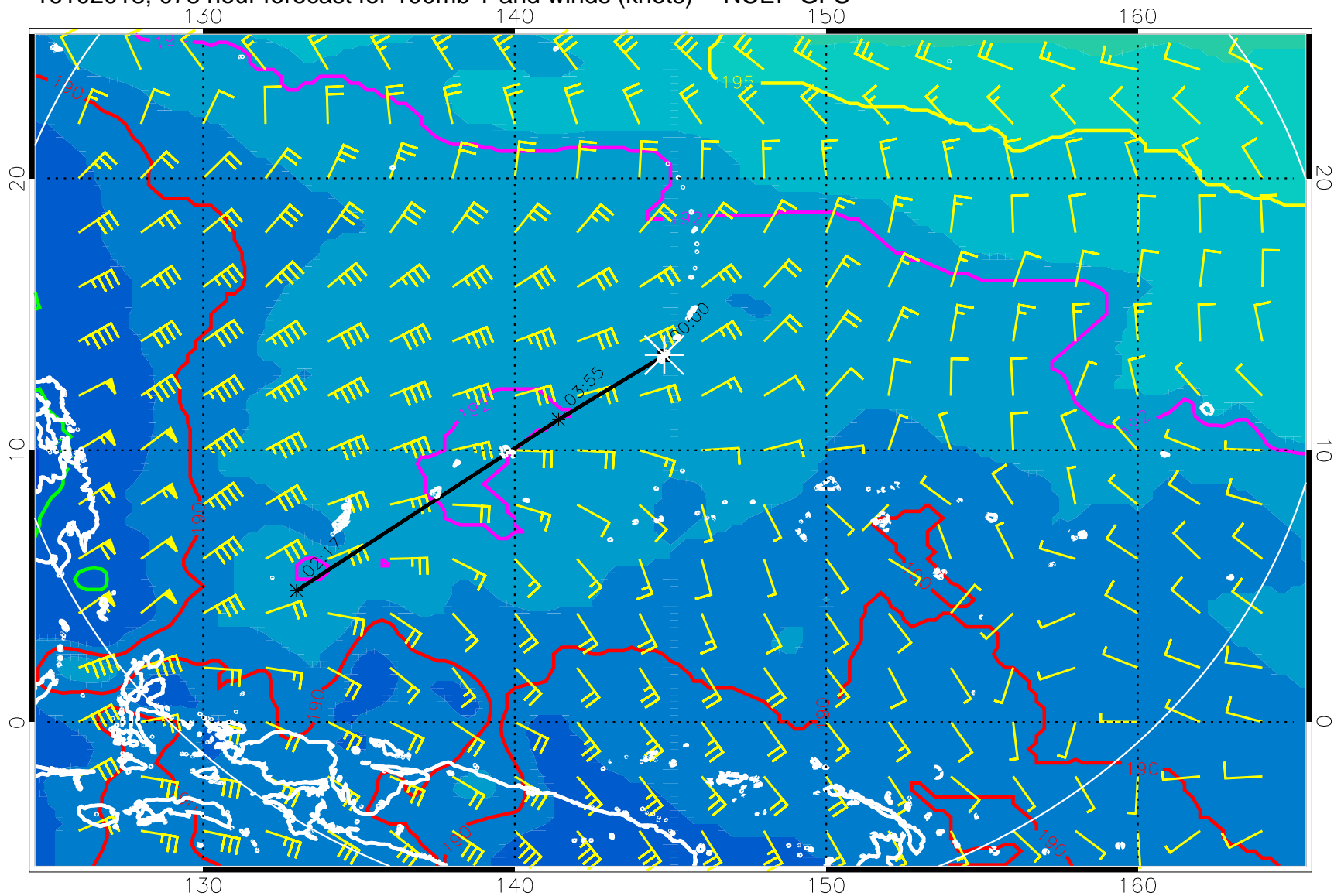
16102018, 078 hour forecast for 100mb T and winds (knots) -- NCEP GFS
