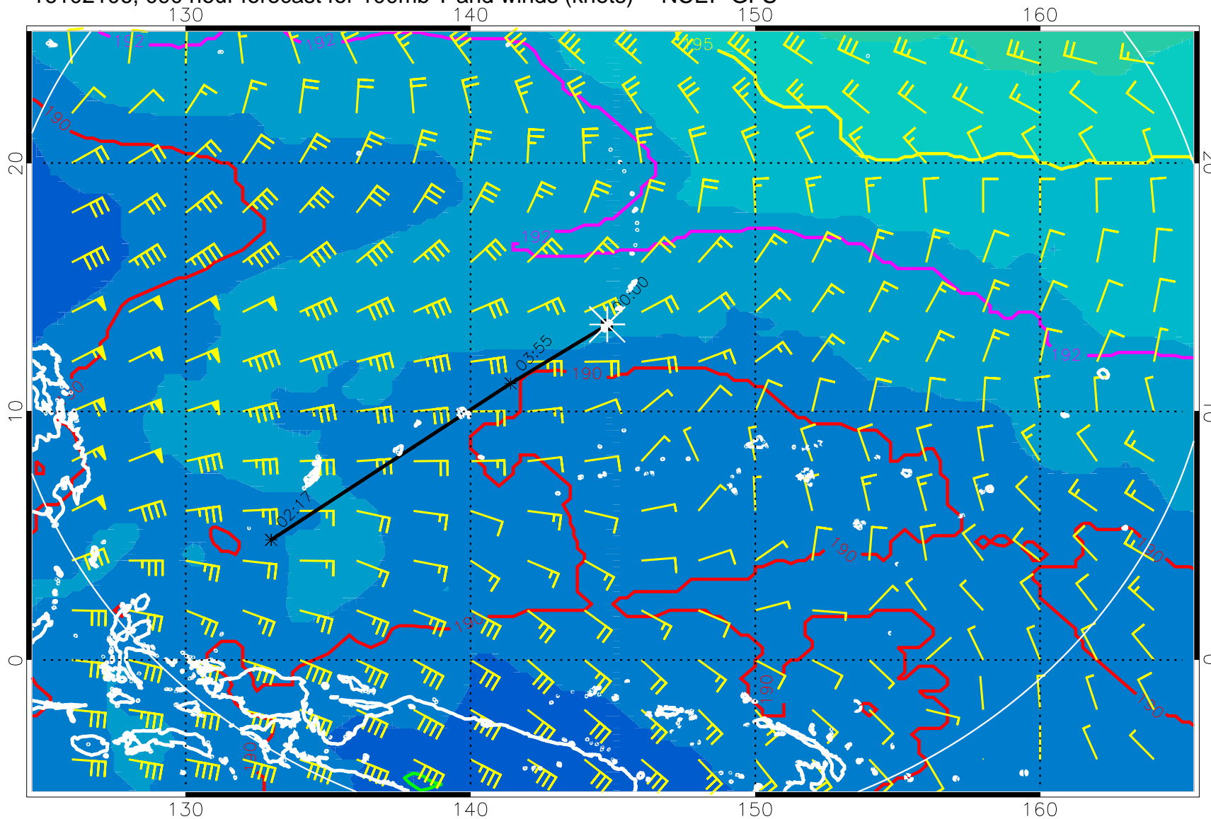
16102106, 090 hour forecast for 100mb T and winds (knots) -- NCEP GFS
