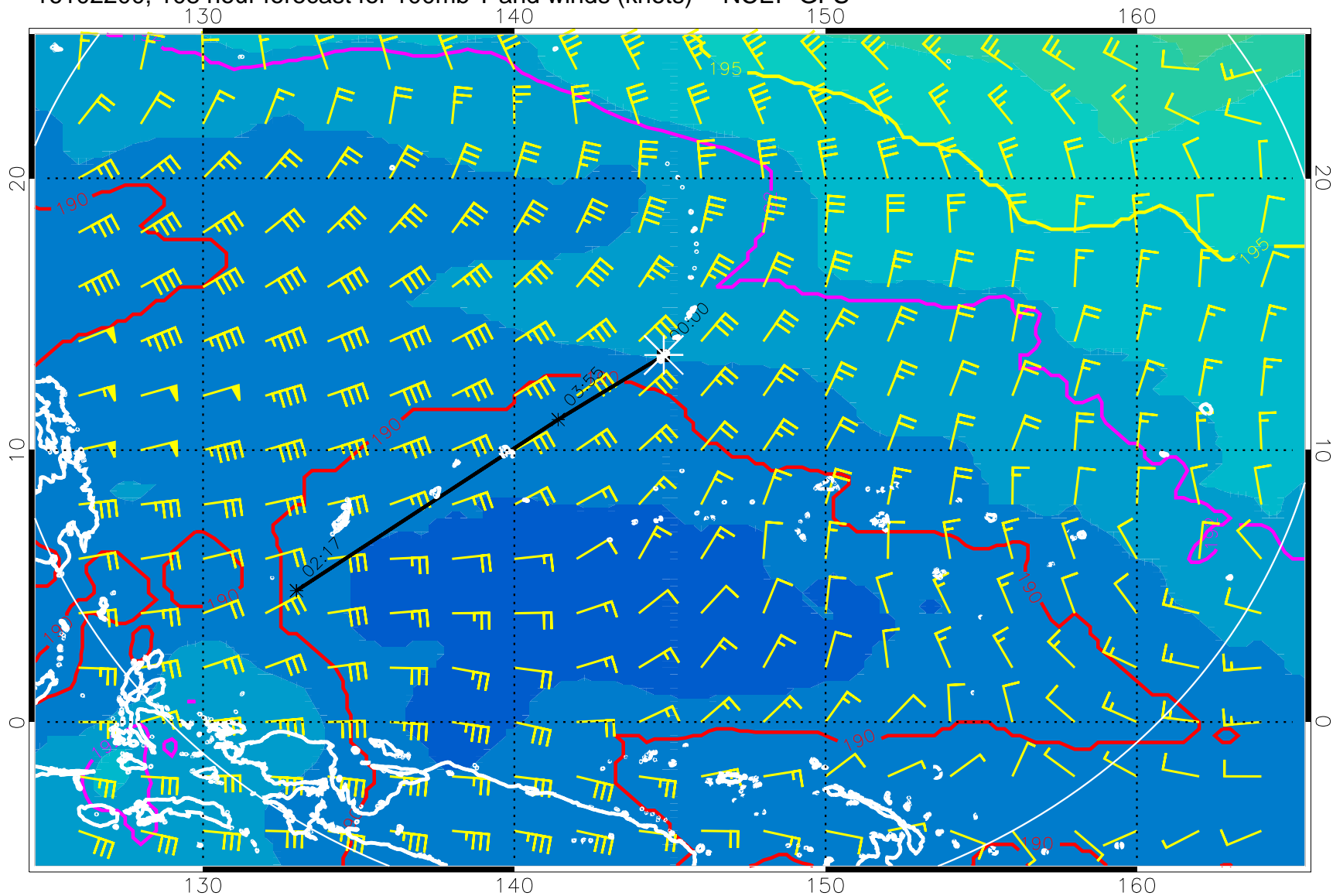
16102200, 108 hour forecast for 100mb T and winds (knots) -- NCEP GFS
