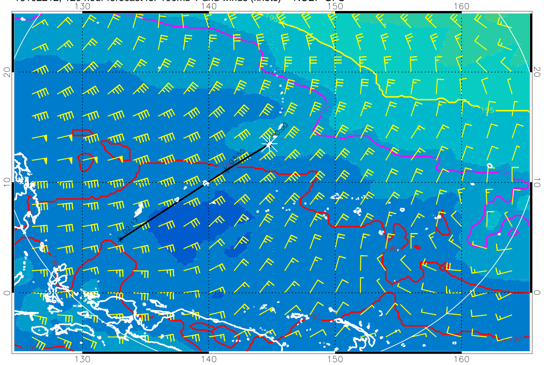
16102212, 120 hour forecast for 100mb T and winds (knots) -- NCEP GFS
