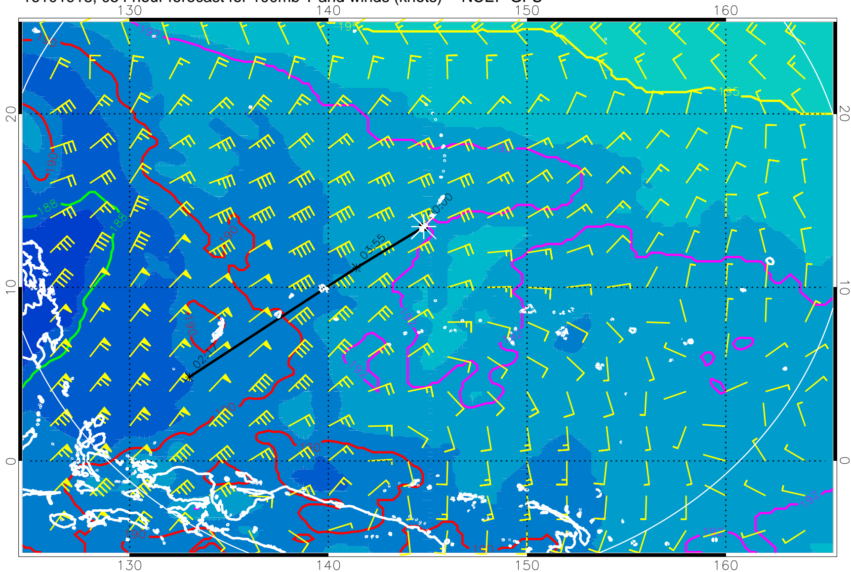
16101918, 054 hour forecast for 100mb T and winds (knots) -- NCEP GFS
