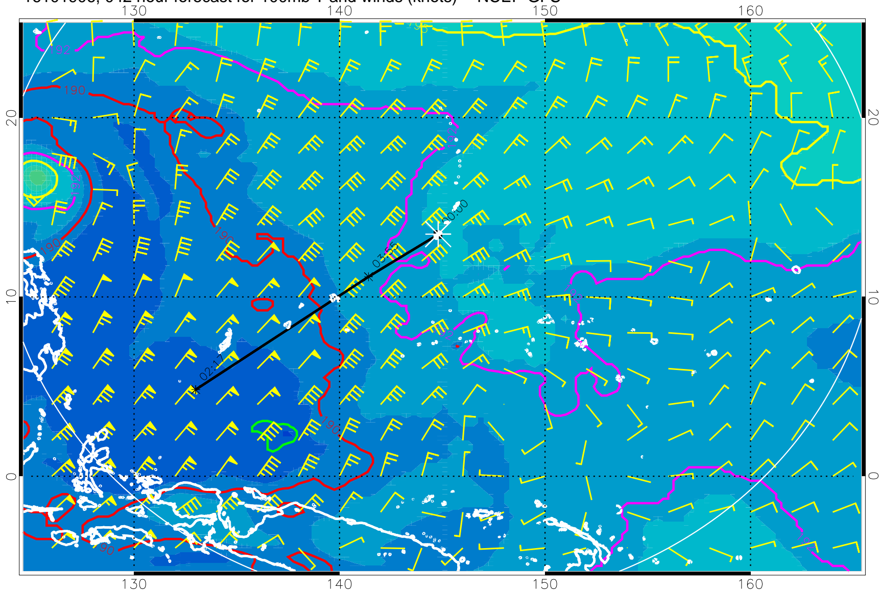
16101906, 042 hour forecast for 100mb T and winds (knots) -- NCEP GFS
