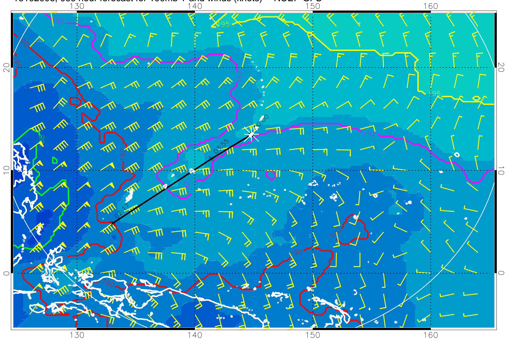
16102006, 066 hour forecast for 100mb T and winds (knots) -- NCEP GFS
