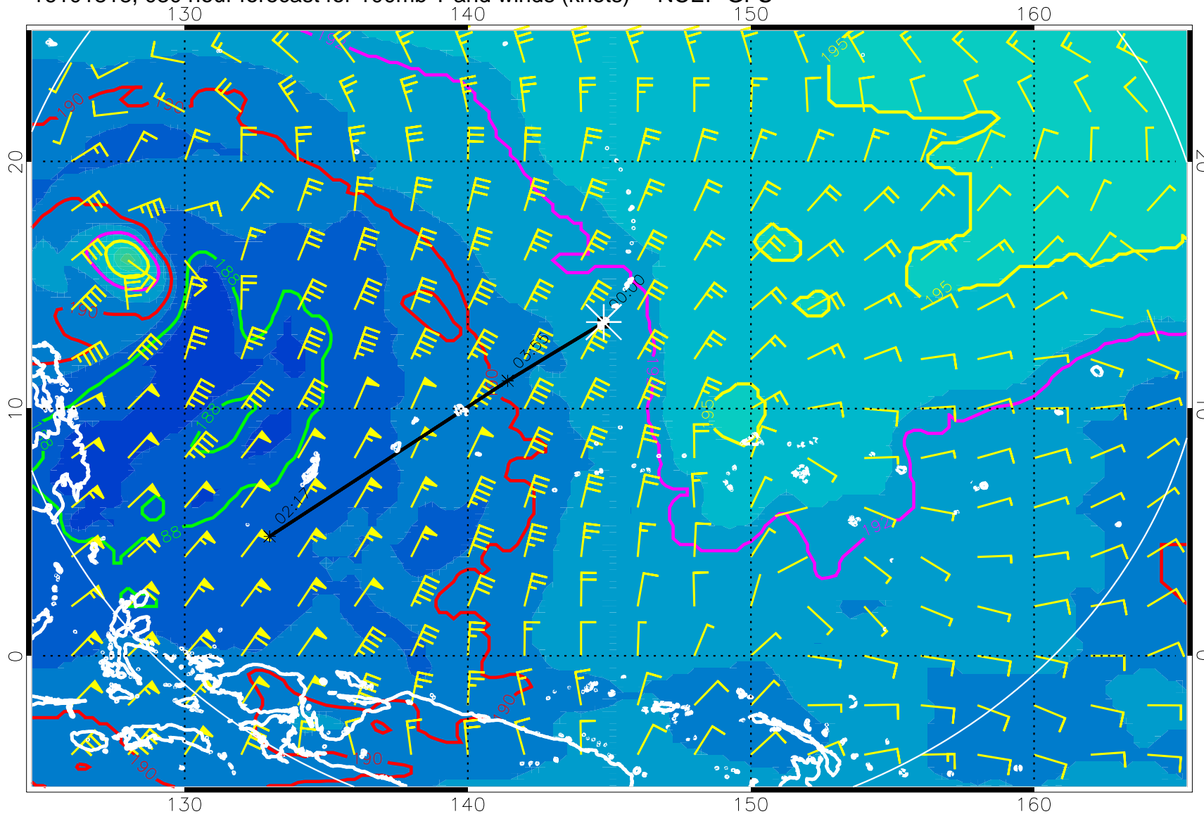
16101818, 030 hour forecast for 100mb T and winds (knots) -- NCEP GFS
