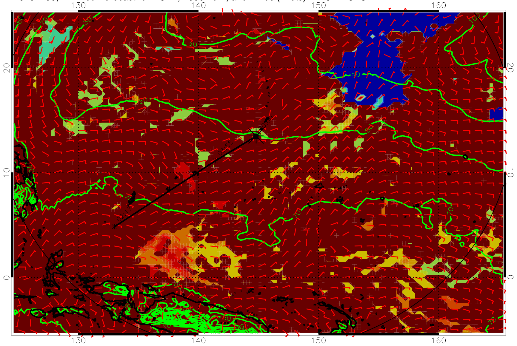
16102206, 114 hour forecast for HCAL, 1000mb Z, and winds (knots) -- NCEP GFS
