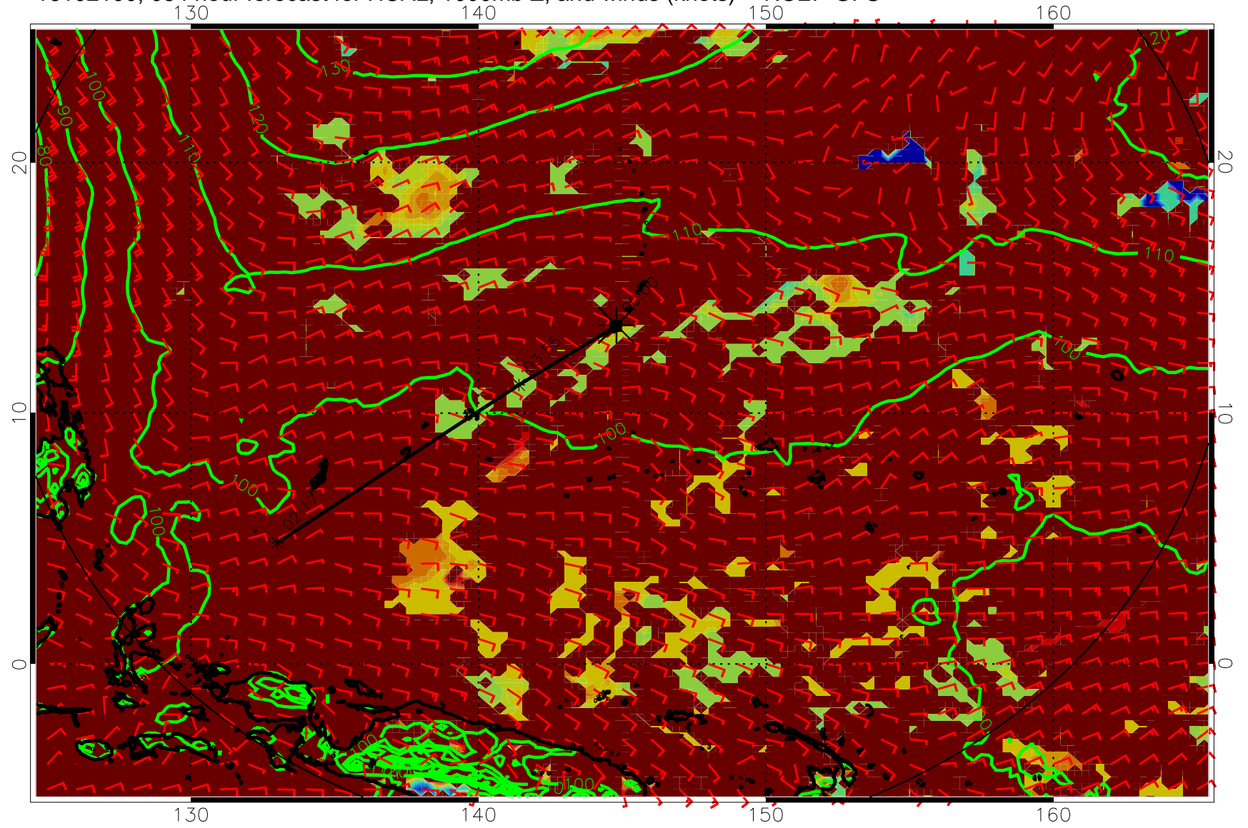
16102100, 084 hour forecast for HCAL, 1000mb Z, and winds (knots) -- NCEP GFS
