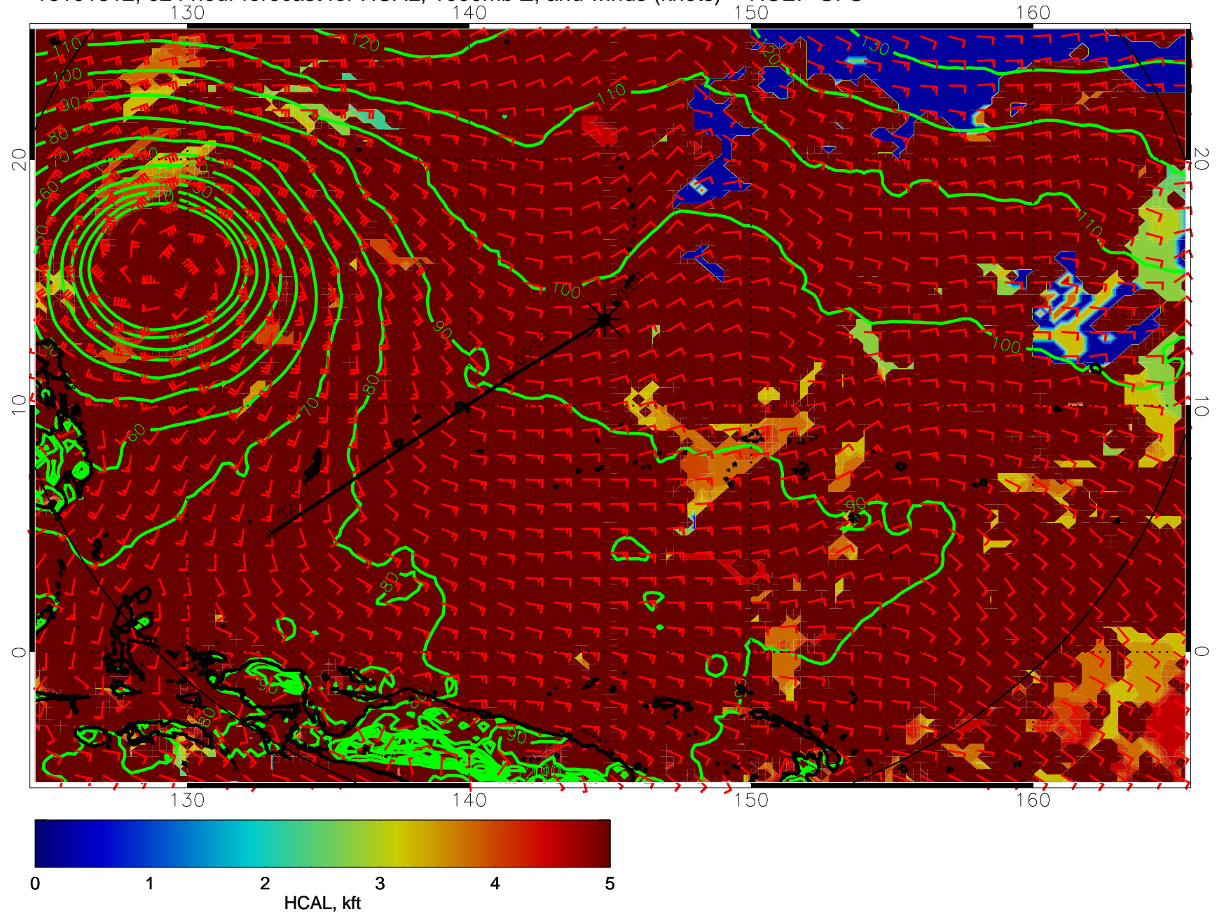
16101812, 024 hour forecast for HCAL, 1000mb Z, and winds (knots) -- NCEP GFS
