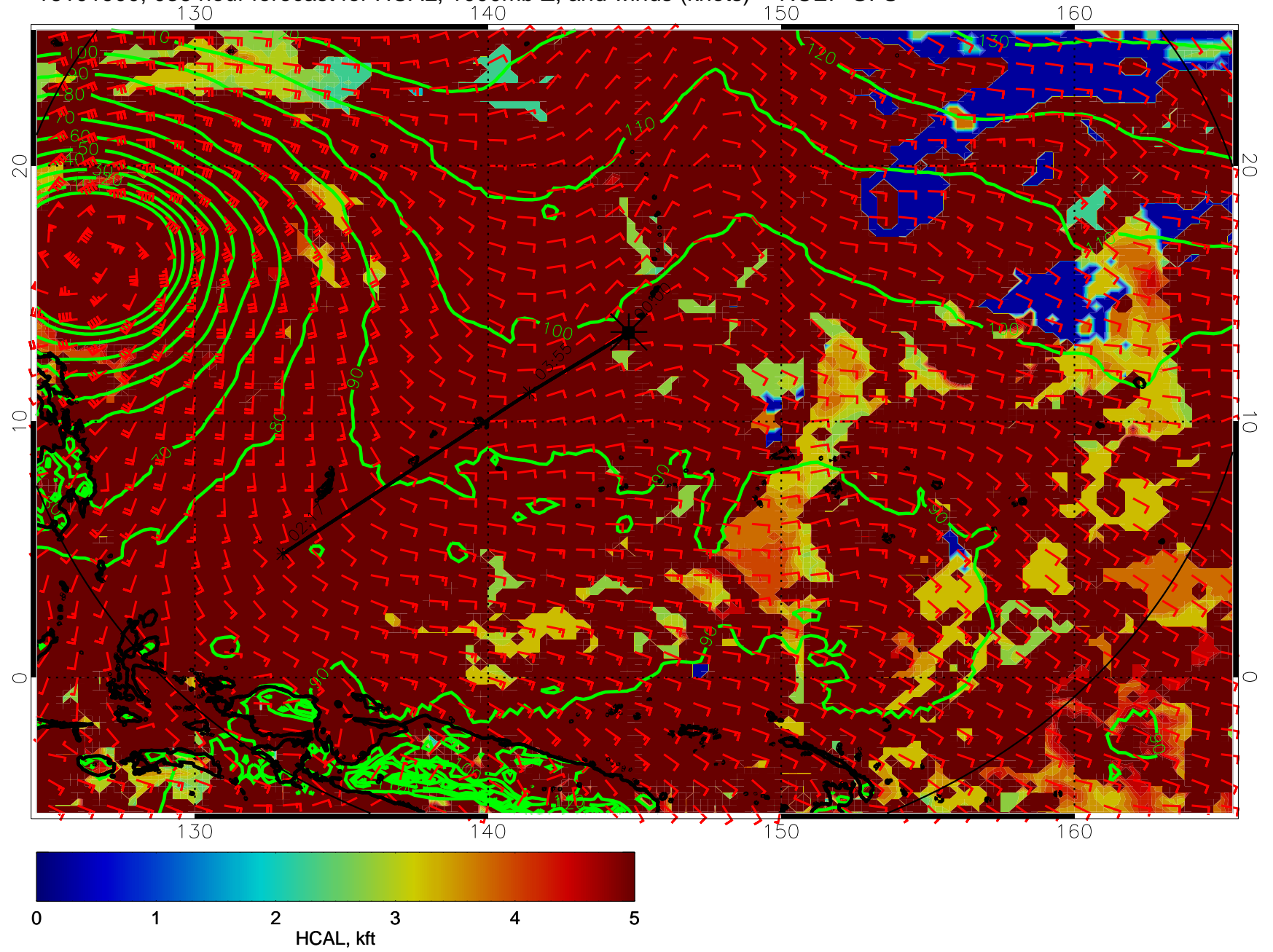
16101900, 036 hour forecast for HCAL, 1000mb Z, and winds (knots) -- NCEP GFS
