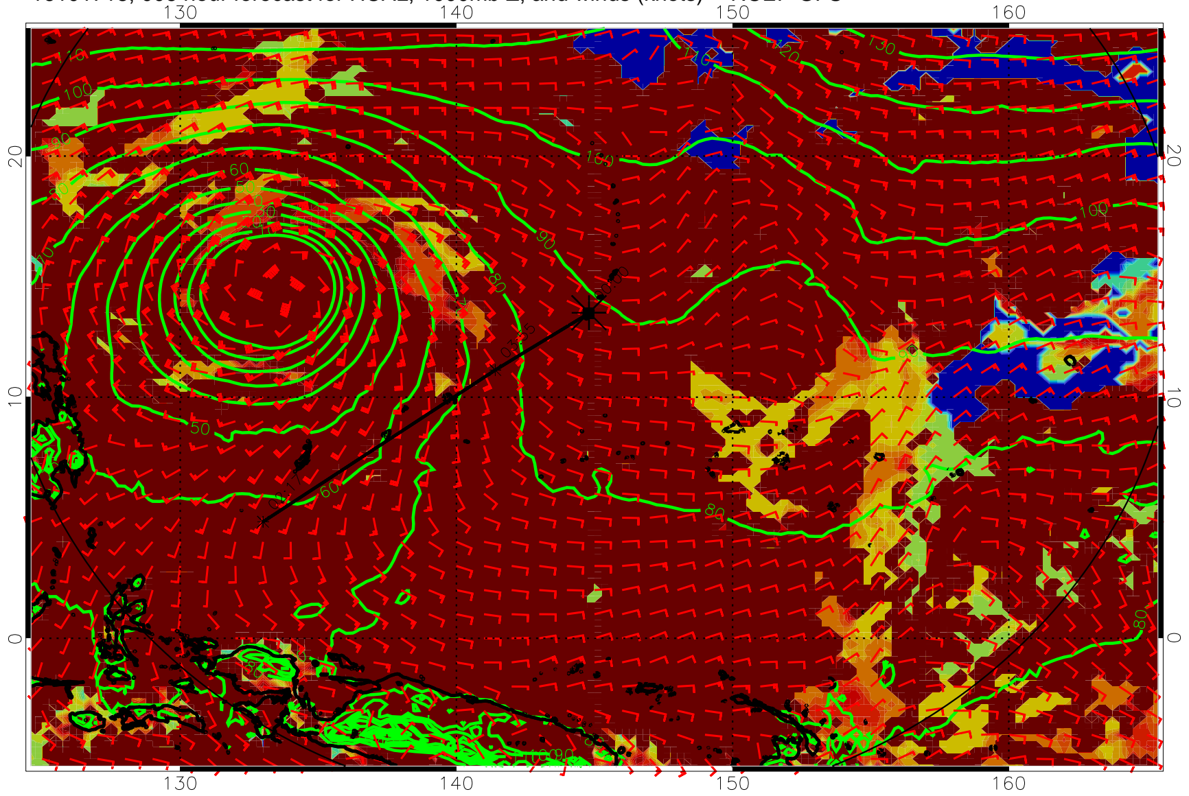
16101718, 006 hour forecast for HCAL, 1000mb Z, and winds (knots) -- NCEP GFS
