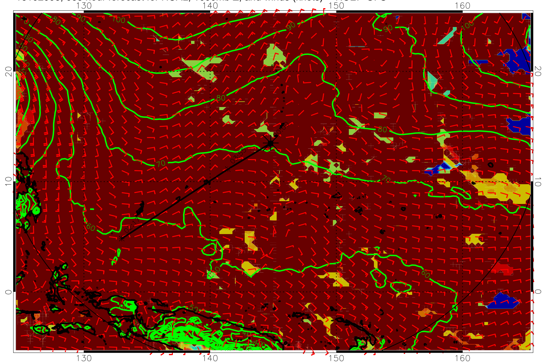
16102006, 066 hour forecast for HCAL, 1000mb Z, and winds (knots) -- NCEP GFS
