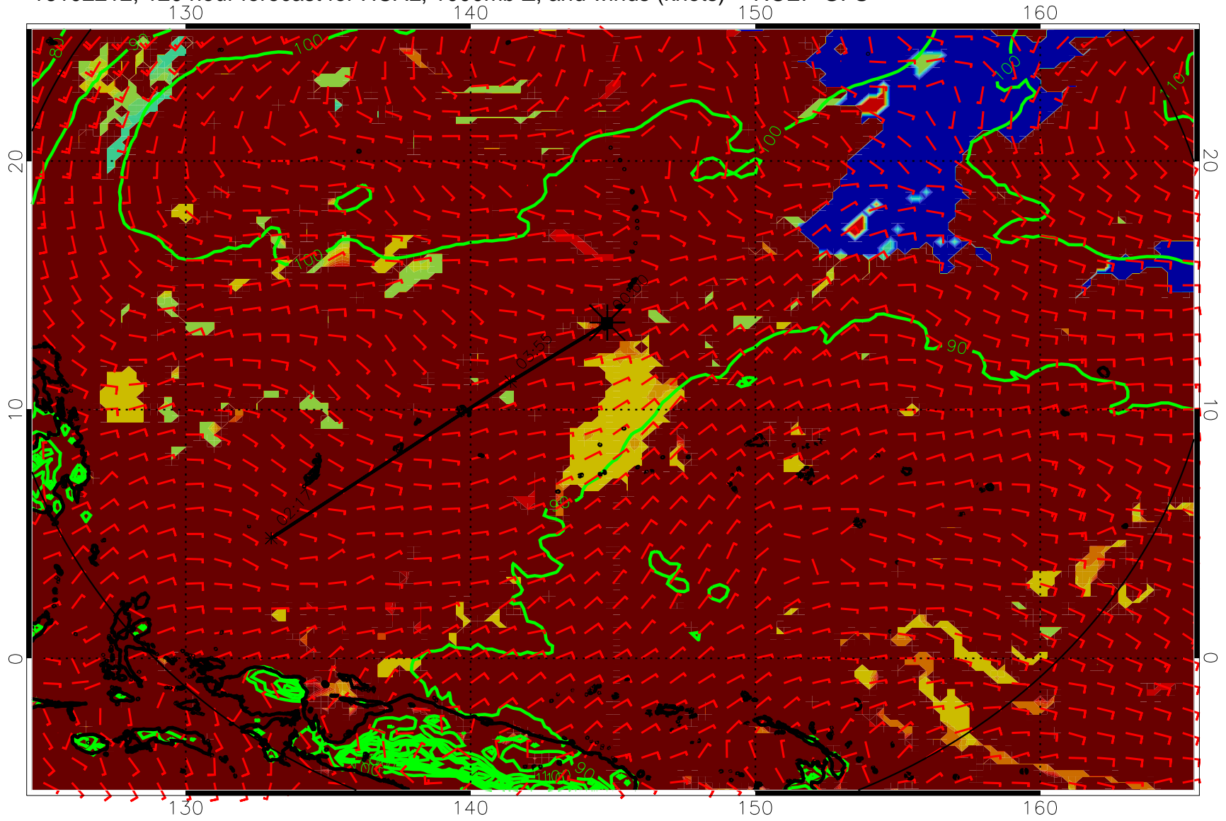
16102212, 120 hour forecast for HCAL, 1000mb Z, and winds (knots) -- NCEP GFS
