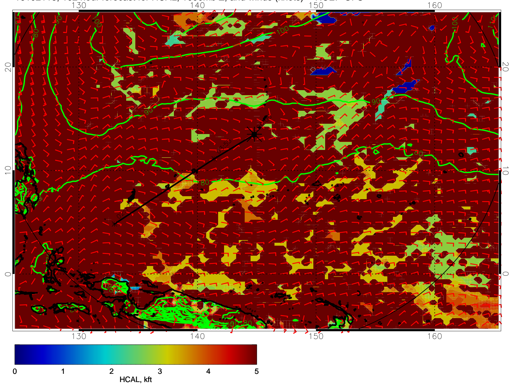
16102118, 102 hour forecast for HCAL, 1000mb Z, and winds (knots) -- NCEP GFS
