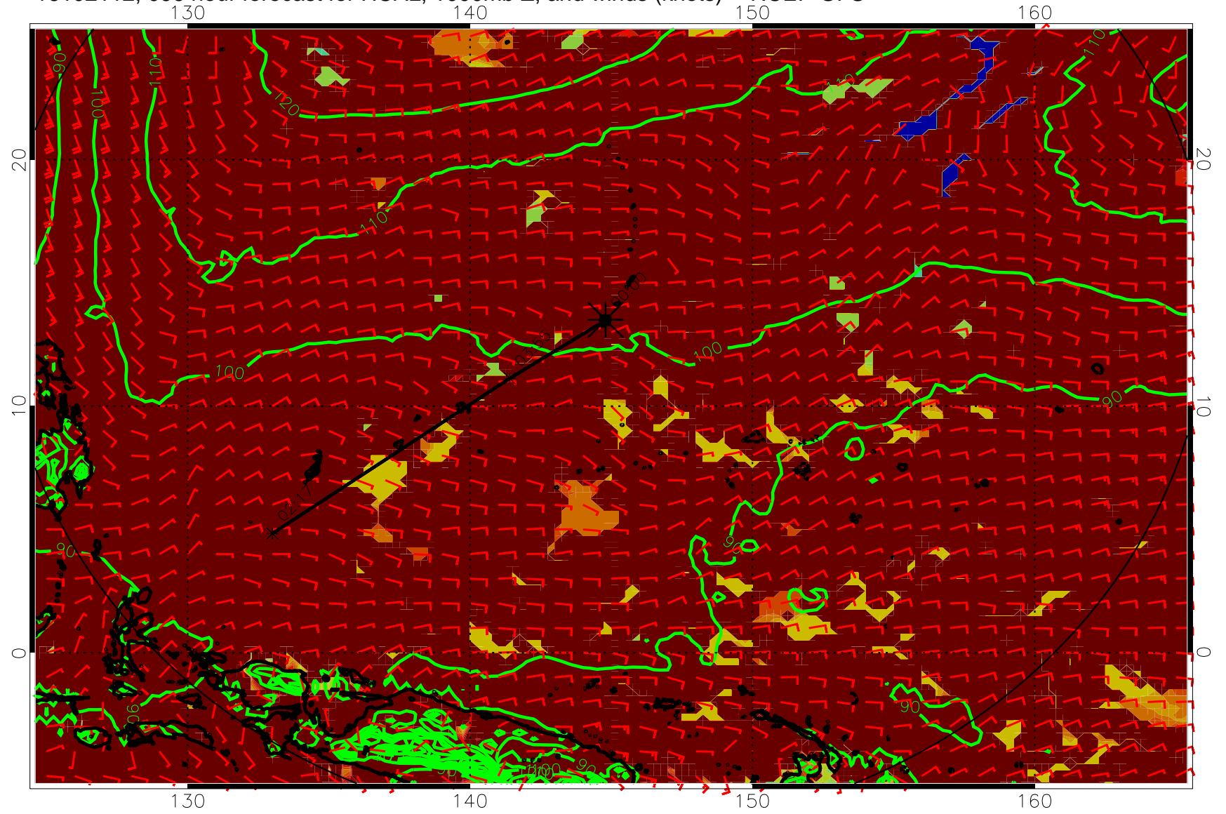
16102112, 096 hour forecast for HCAL, 1000mb Z, and winds (knots) -- NCEP GFS
