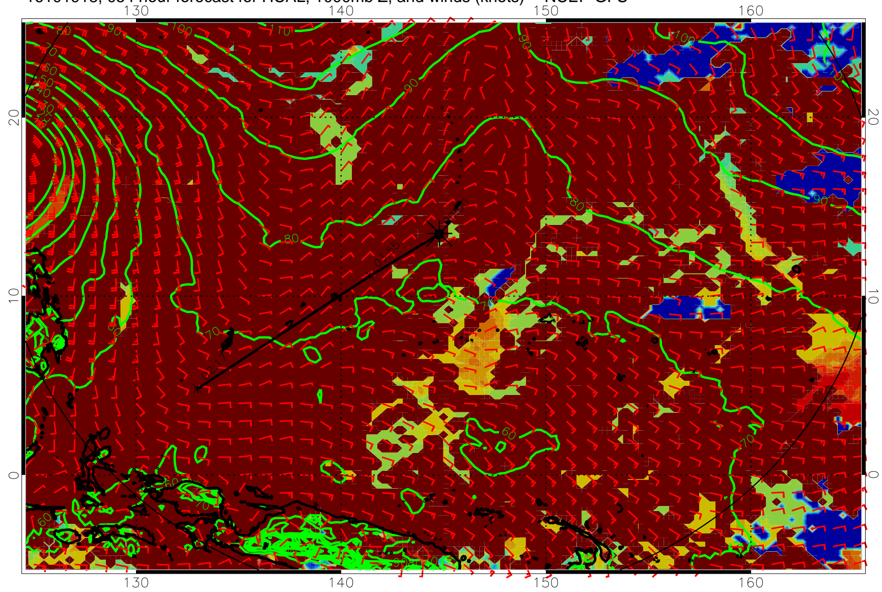
16101918, 054 hour forecast for HCAL, 1000mb Z, and winds (knots) -- NCEP GFS
