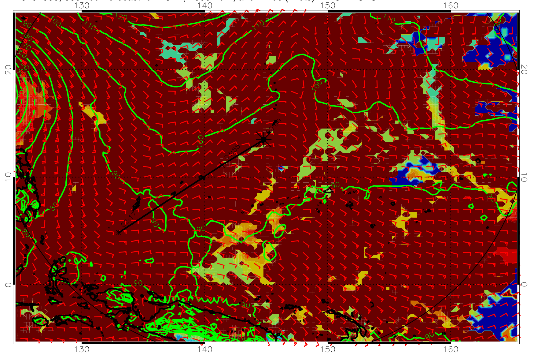
16102000, 060 hour forecast for HCAL, 1000mb Z, and winds (knots) -- NCEP GFS
