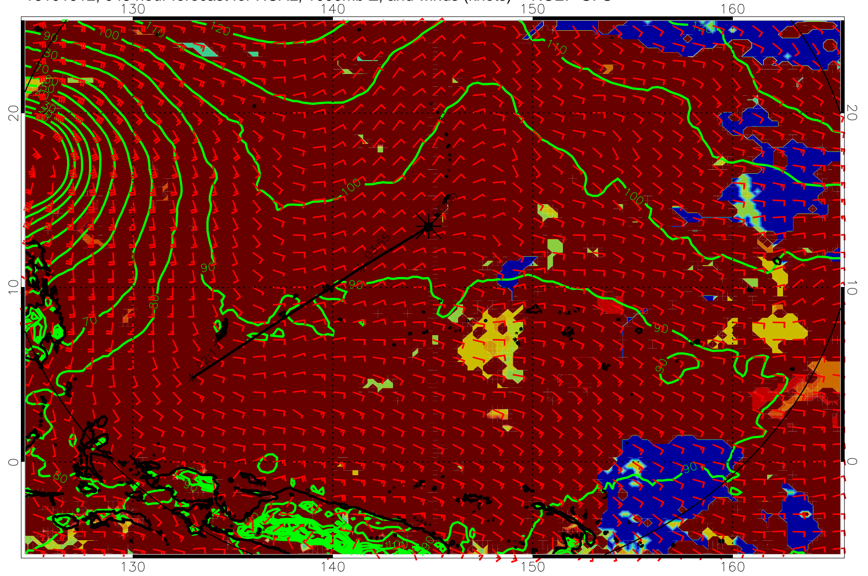
16101912, 048 hour forecast for HCAL, 1000mb Z, and winds (knots) -- NCEP GFS
