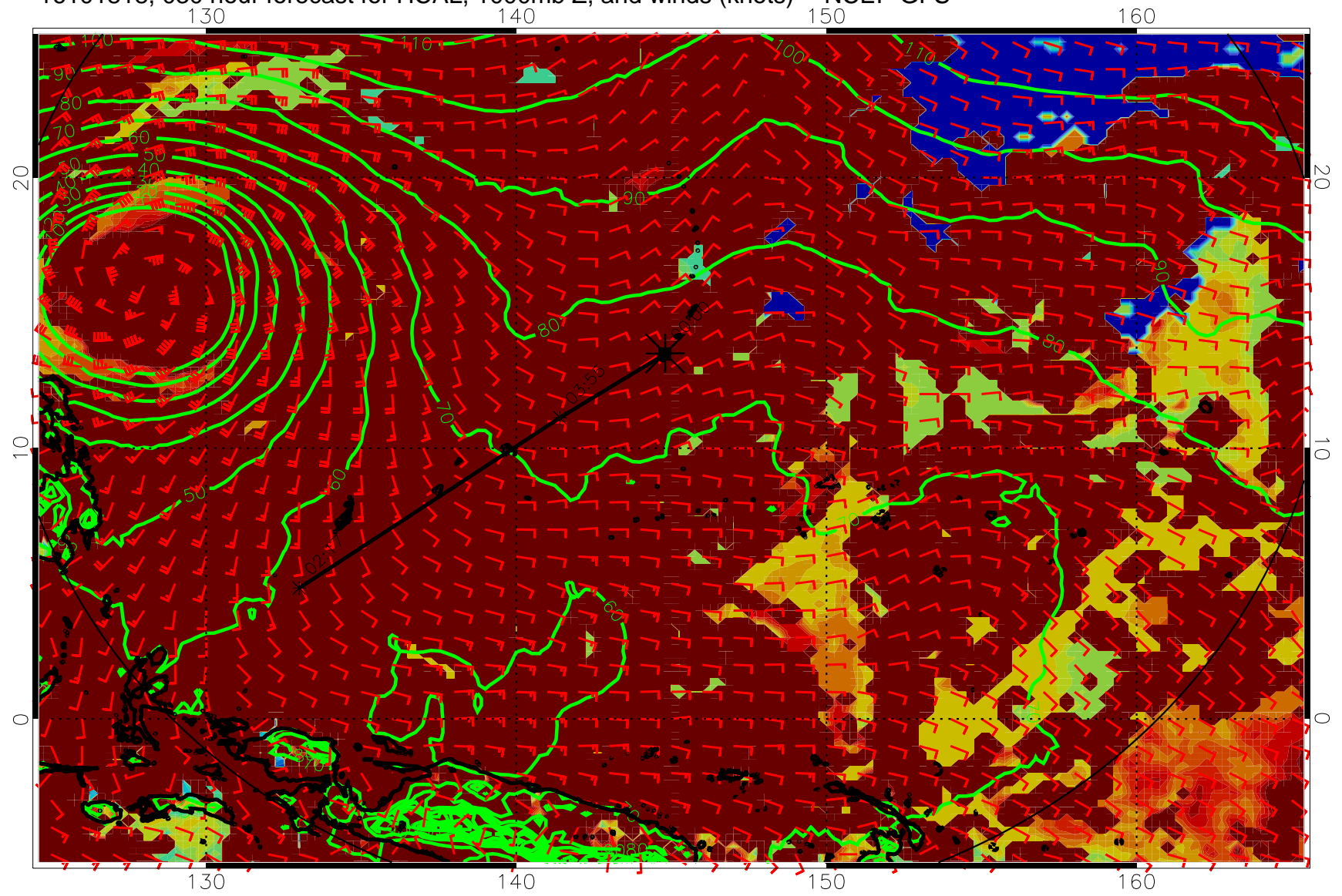
16101818, 030 hour forecast for HCAL, 1000mb Z, and winds (knots) -- NCEP GFS
