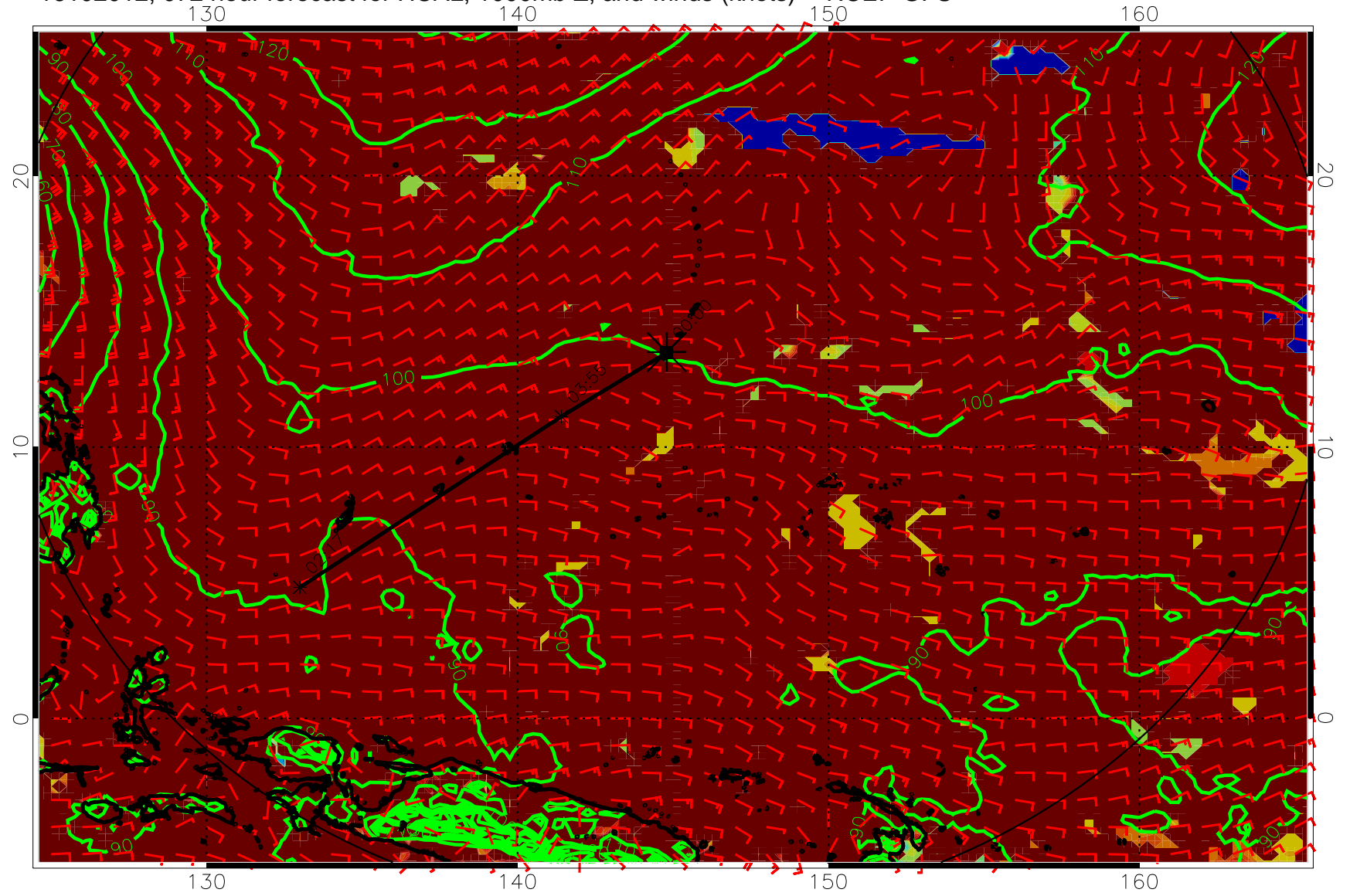
16102012, 07Z hour forecast for HCAL, 1000mb Z, and winds (knots) -- NCEP GFS
