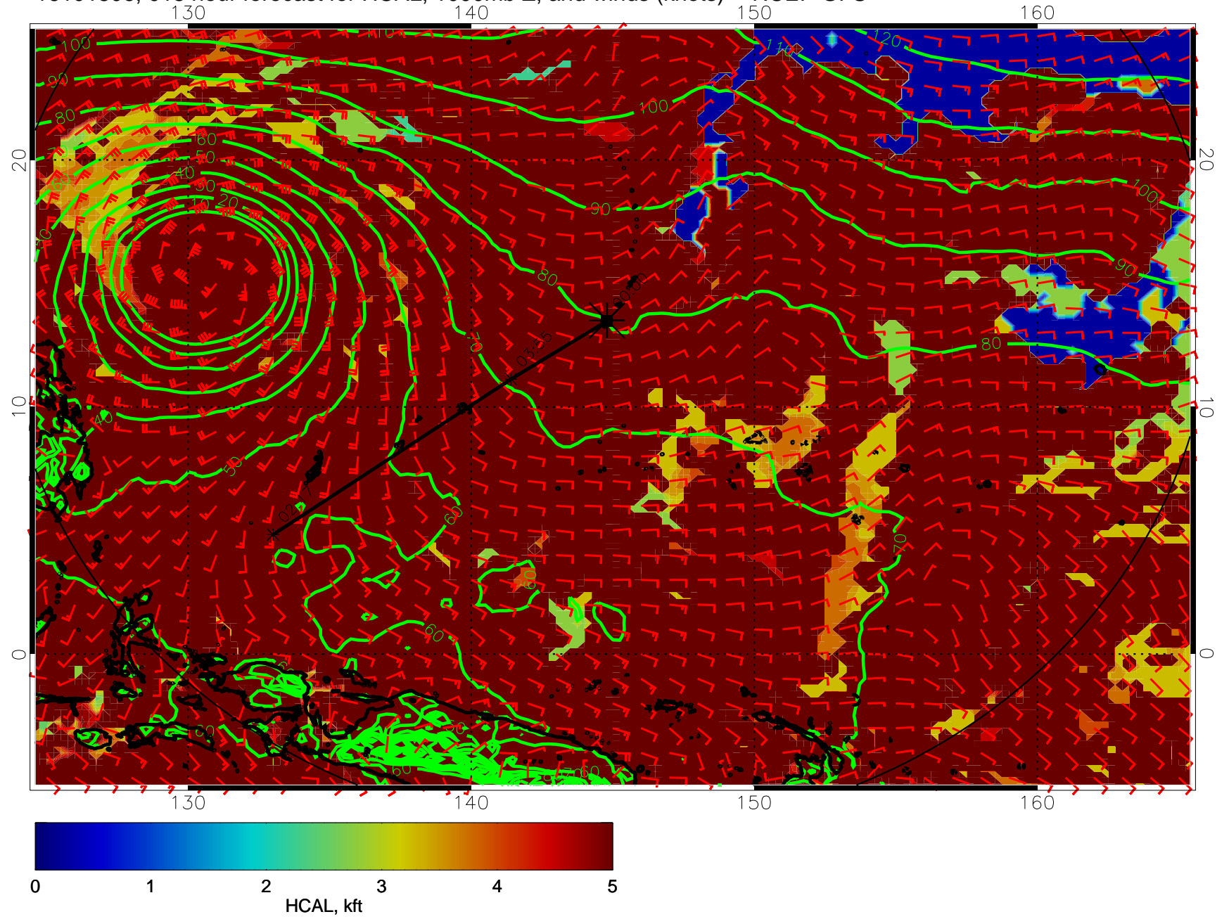
16101806, 018 hour forecast for HCAL, 1000mb Z, and winds (knots) -- NCEP GFS
