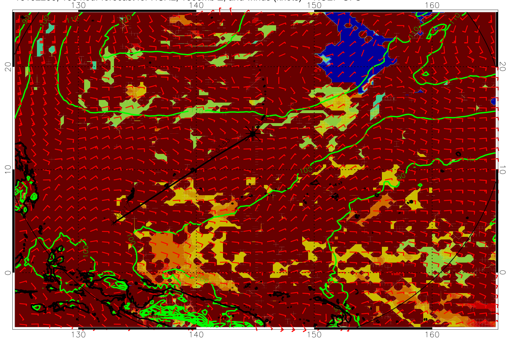
16102200, 108 hour forecast for HCAL, 1000mb Z, and winds (knots) -- NCEP GFS
