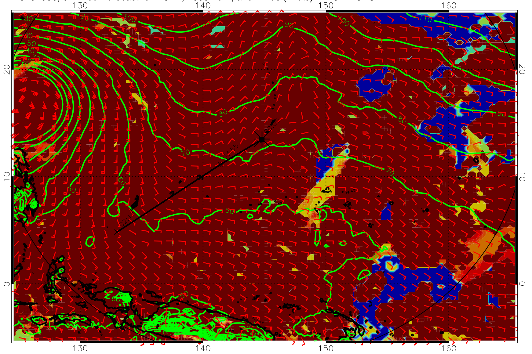
16101906, 042 hour forecast for HCAL, 1000mb Z, and winds (knots) -- NCEP GFS
