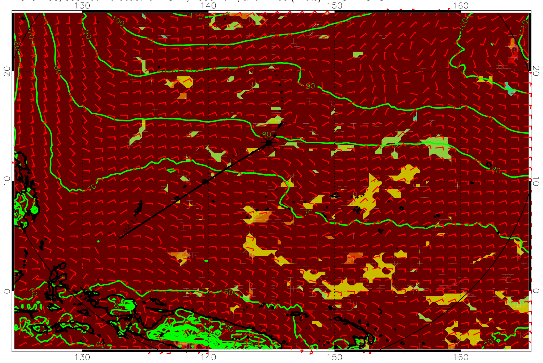
16102106, 090 hour forecast for HCAL, 1000mb Z, and winds (knots) -- NCEP GFS
