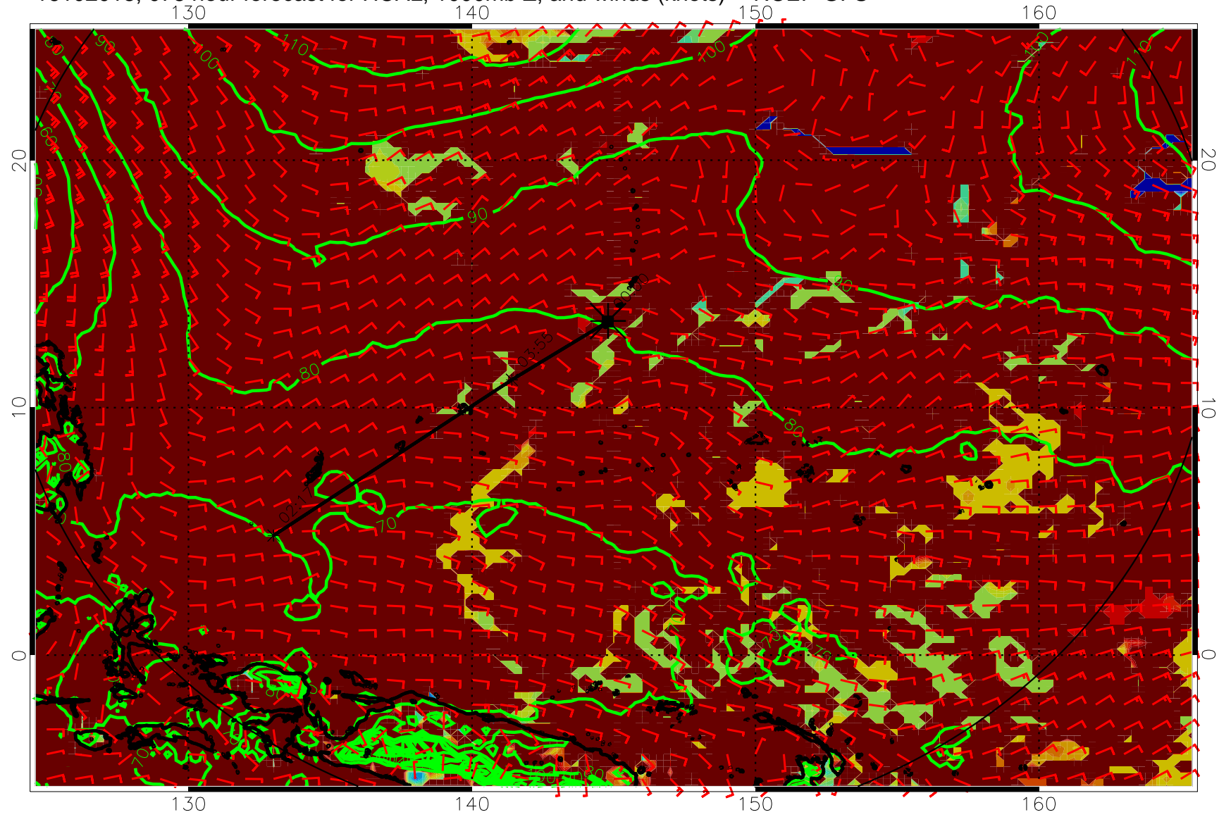
16102018, 078 hour forecast for HCAL, 1000mb Z, and winds (knots) -- NCEP GFS
