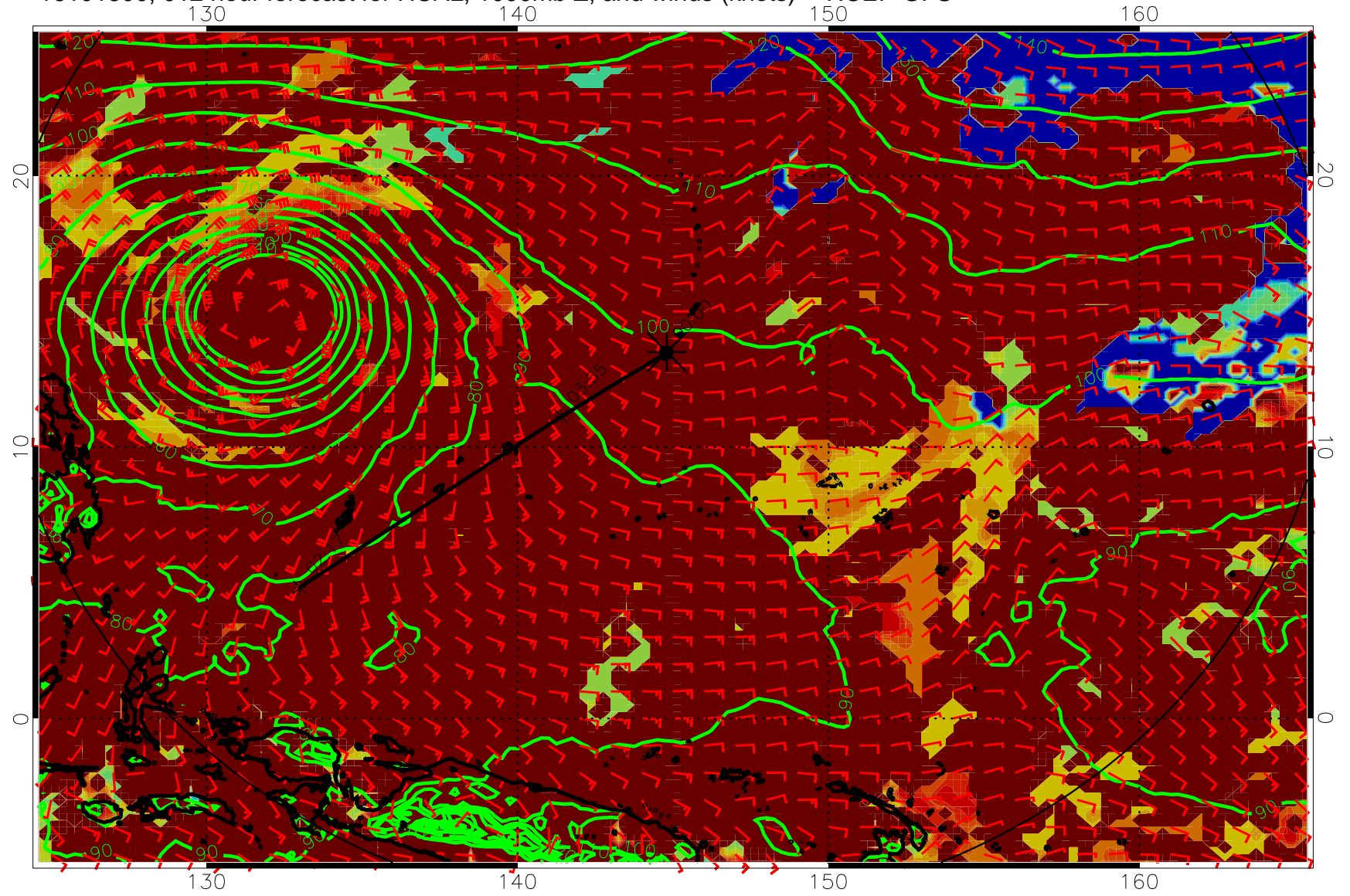
16101800, 012 hour forecast for HCAL, 1000mb Z, and winds (knots) -- NCEP GFS
