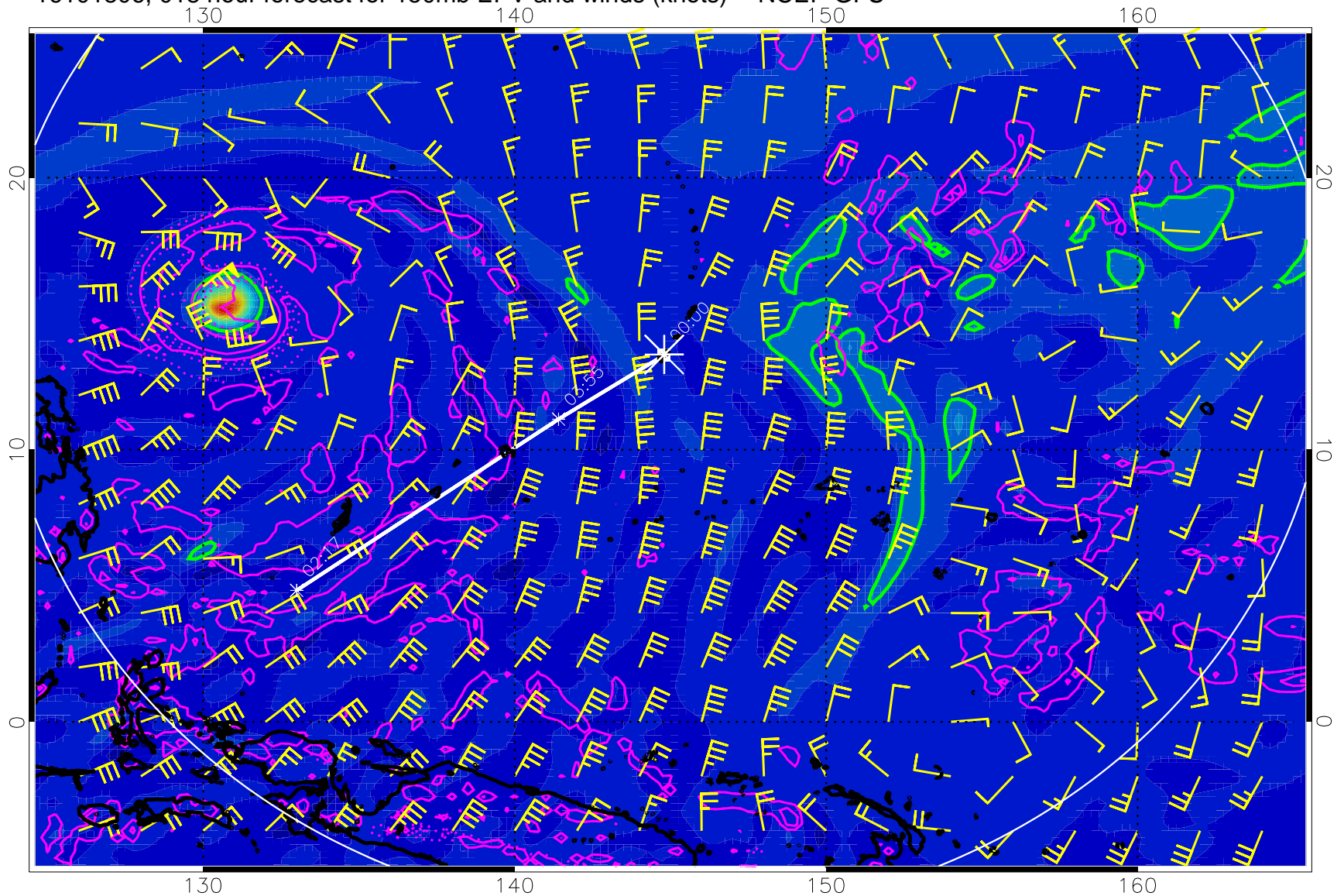
16101806, 018 hour forecast for 150mb EPV and winds (knots) -- NCEP GFS
