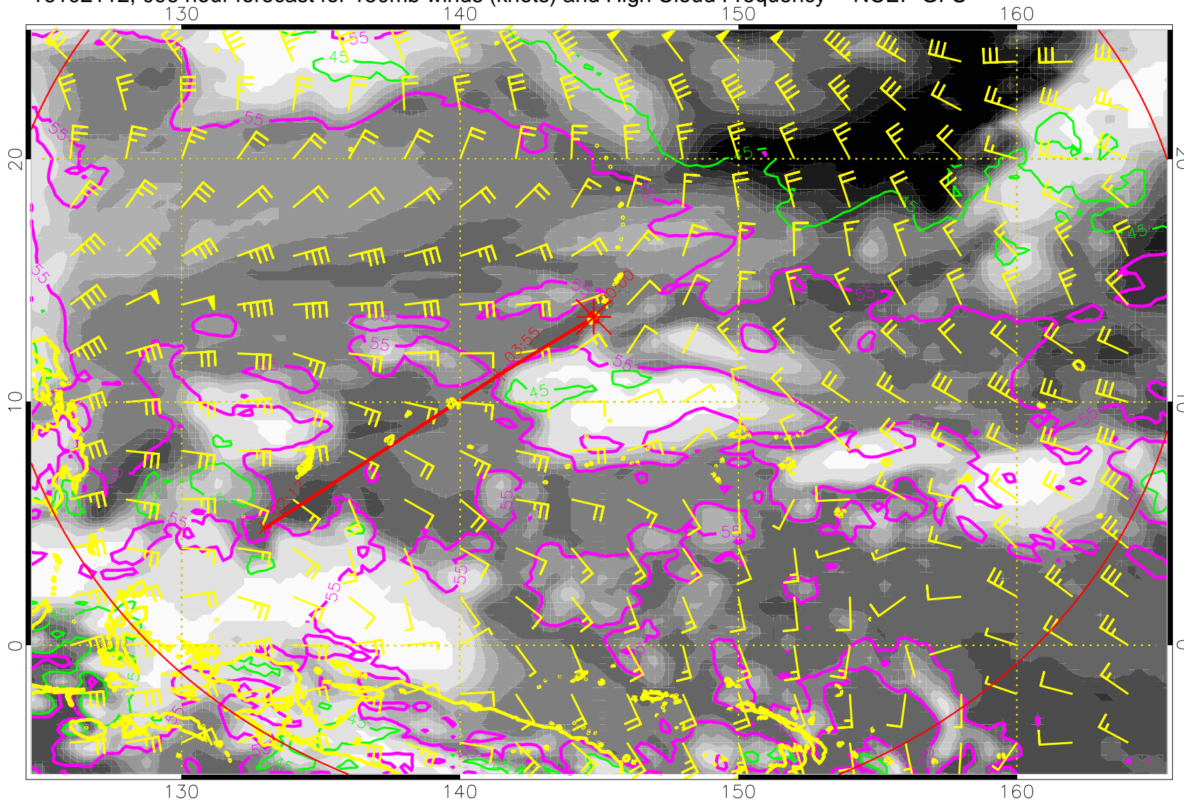
16102112, 096 hour forecast for 150mb winds (knots) and High Cloud Frequency -- NCEP GFS
