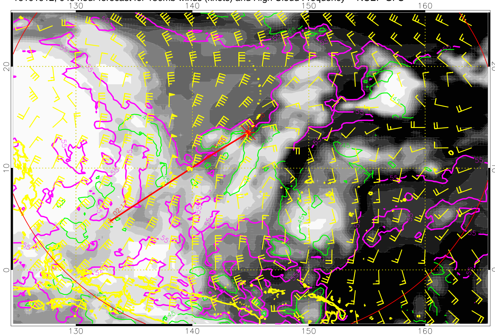
16101912, 048 hour forecast for 150mb winds (knots) and High Cloud Frequency -- NCEP GFS
