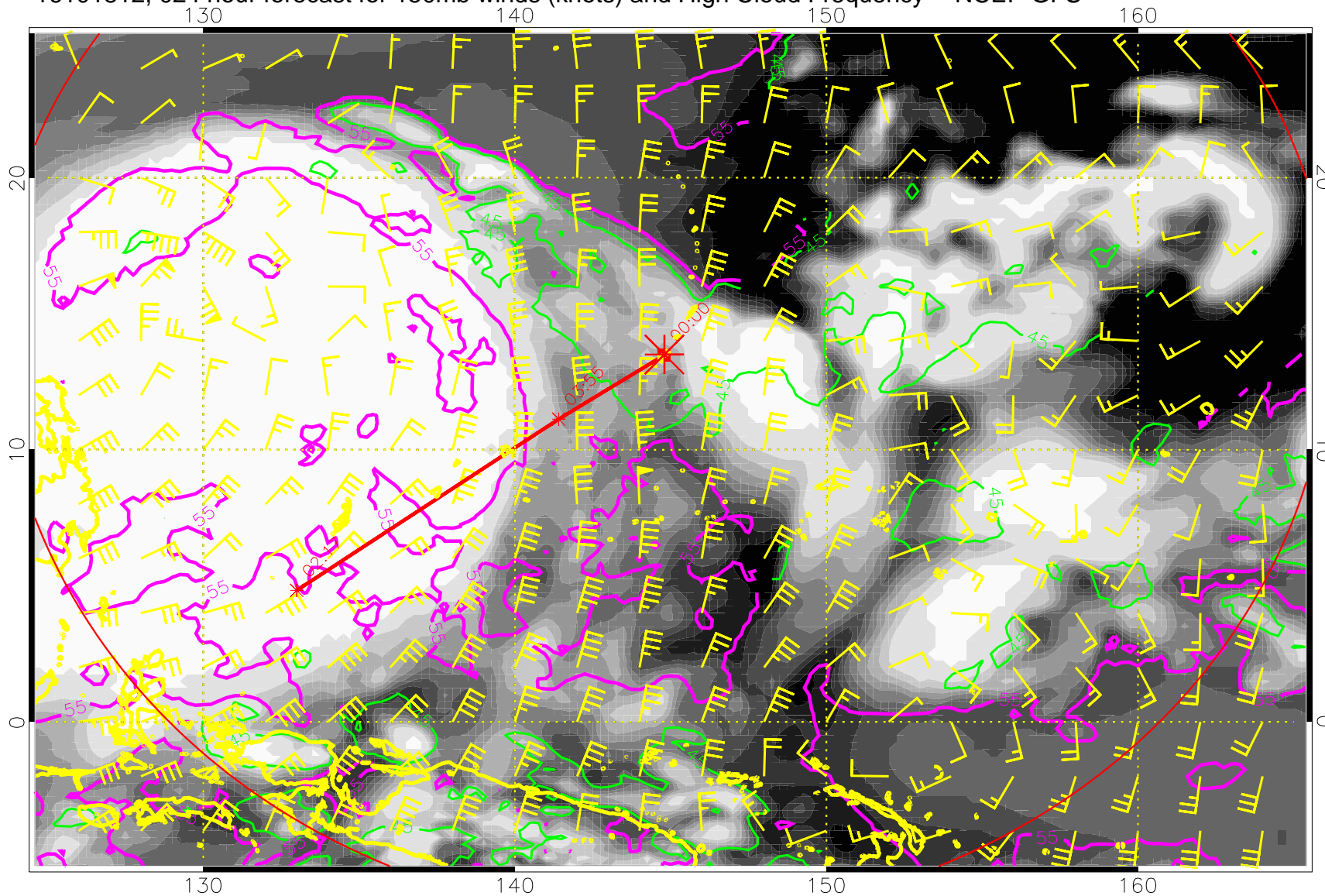
16101812, 024 hour forecast for 150mb winds (knots) and High Cloud Frequency -- NCEP GFS
