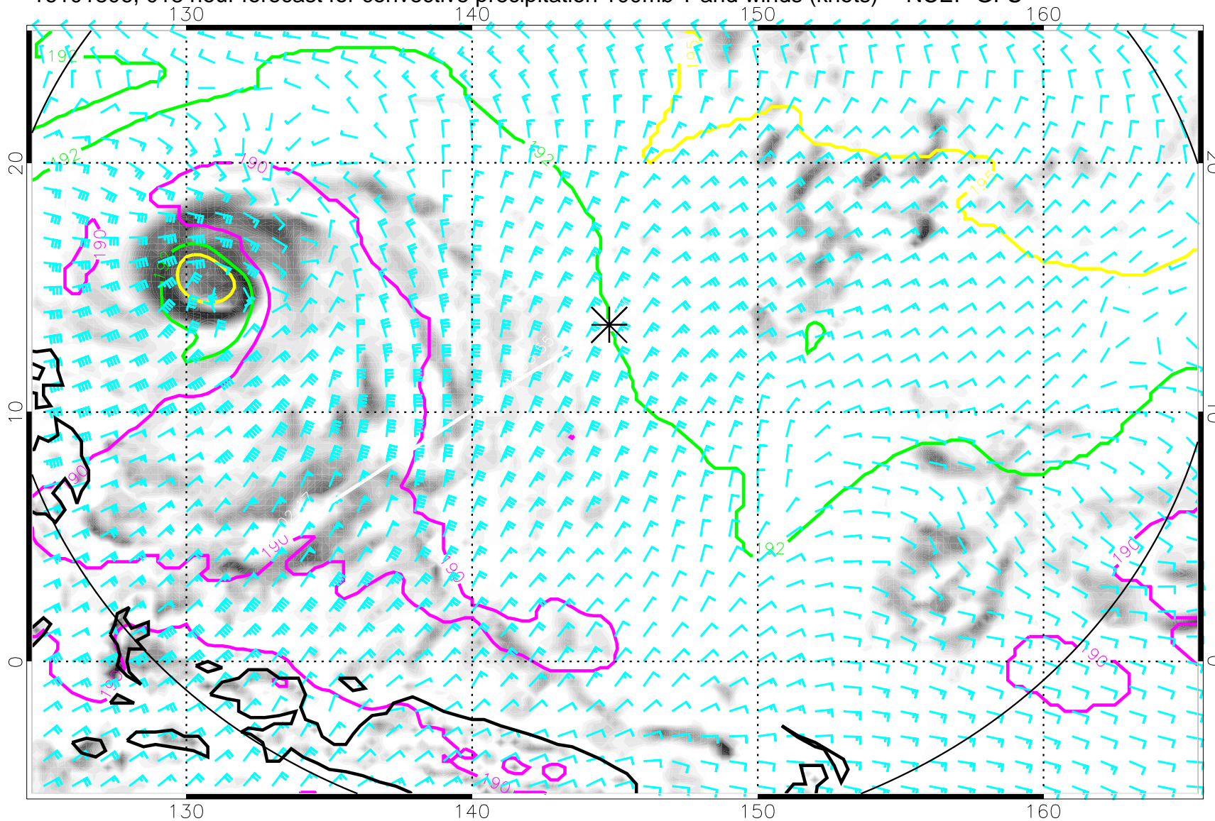
16101806, 018 hour forecast for convective precipitation 100mb T and winds (knots) -- NCEP GFS
