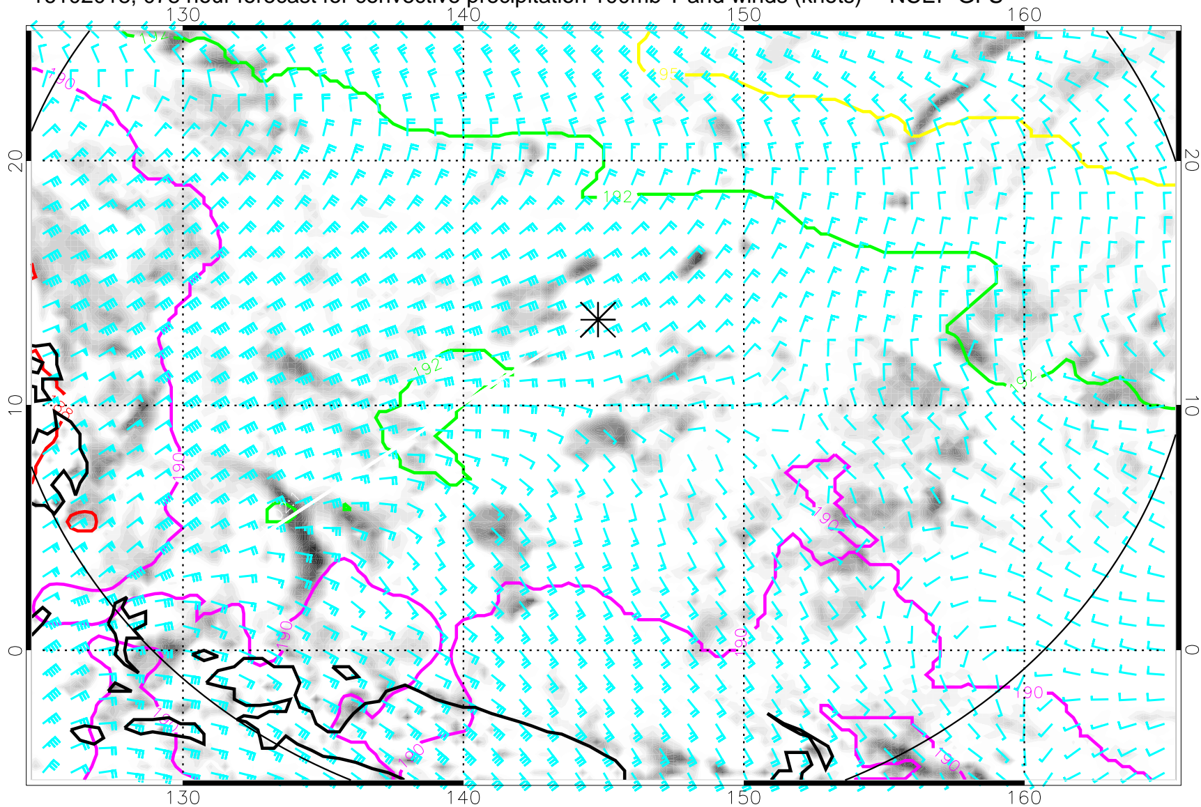
16102018, 078 hour forecast for convective precipitation 100mb T and winds (knots) -- NCEP GFS
