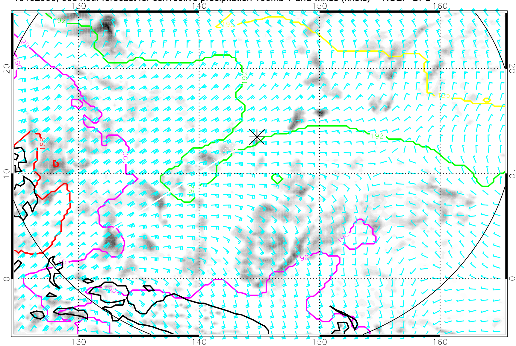
16102006, 066 hour forecast for convective precipitation 100mb T and winds (knots) -- NCEP GFS
