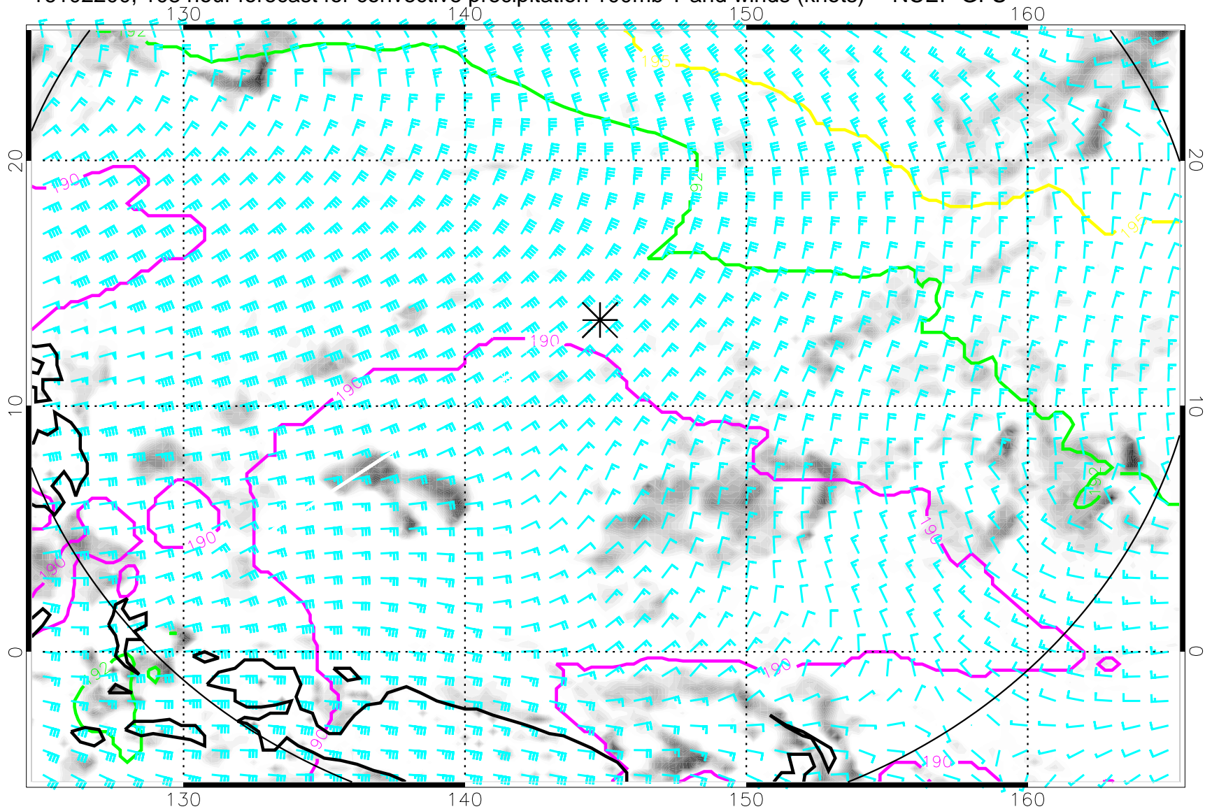
16102200, 108 hour forecast for convective precipitation 100mb T and winds (knots) -- NCEP GFS
