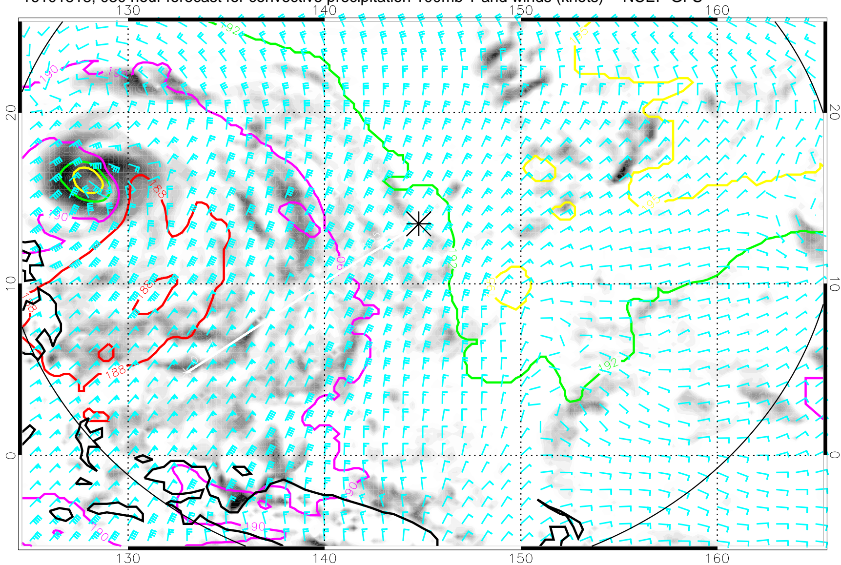
16101818, 030 hour forecast for convective precipitation 100mb T and winds (knots) -- NCEP GFS
