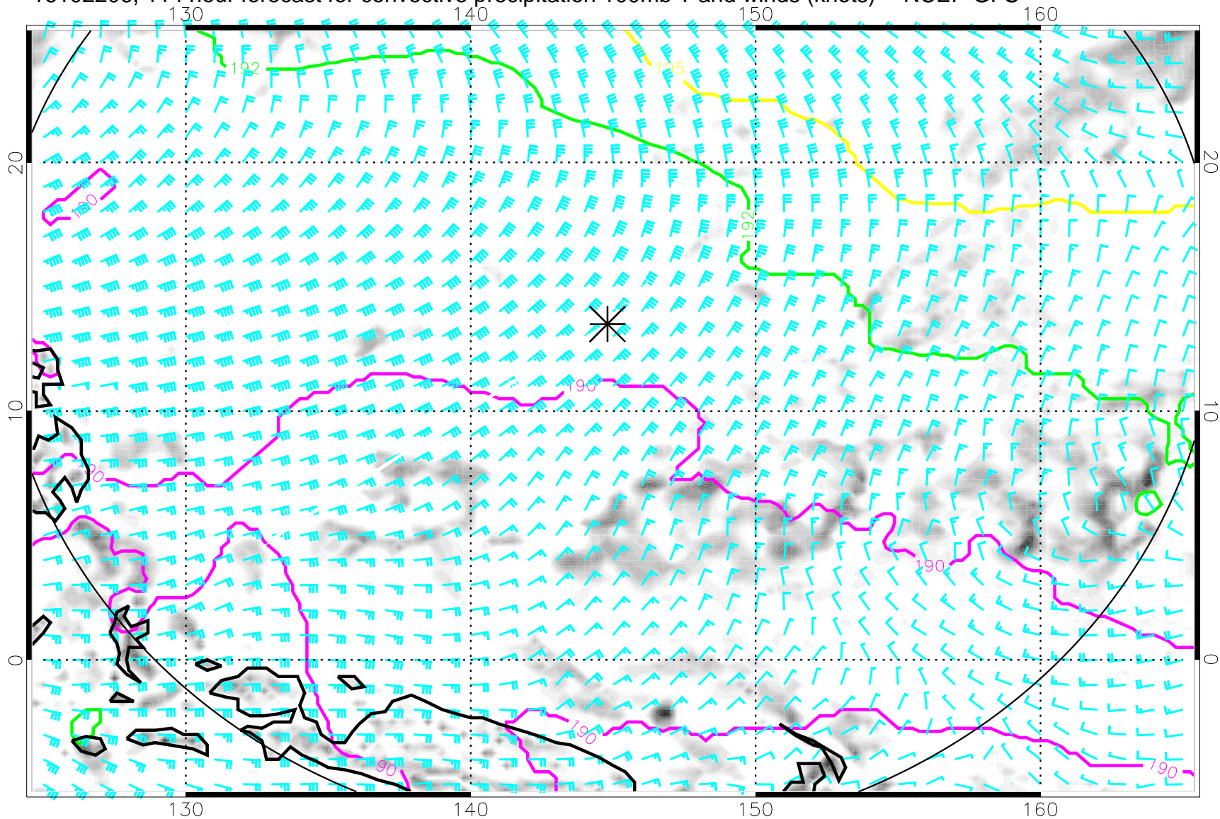
16102206, 114 hour forecast for convective precipitation 100mb T and winds (knots) -- NCEP GFS
