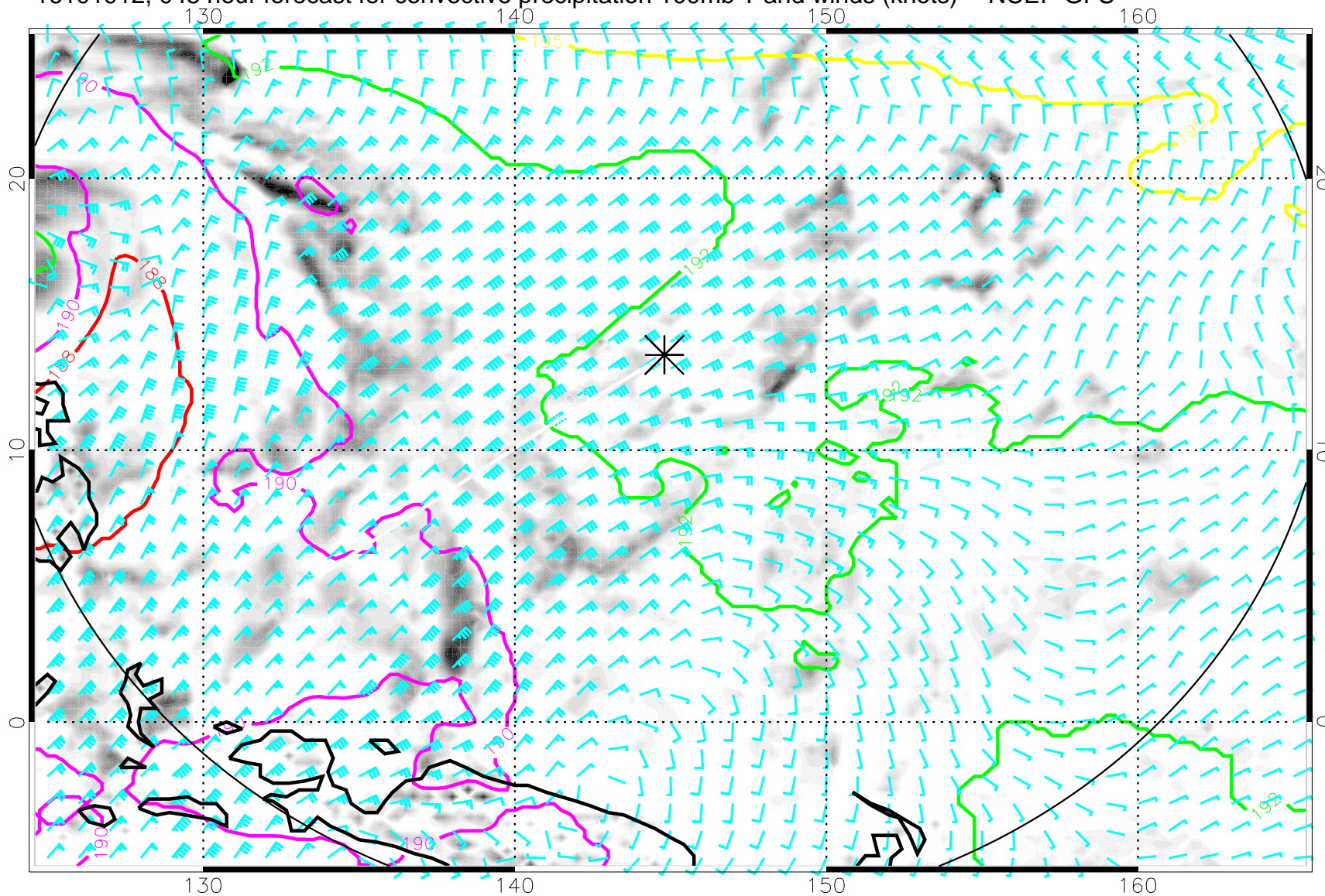
16101912, 048 hour forecast for convective precipitation 100mb T and winds (knots) -- NCEP GFS
