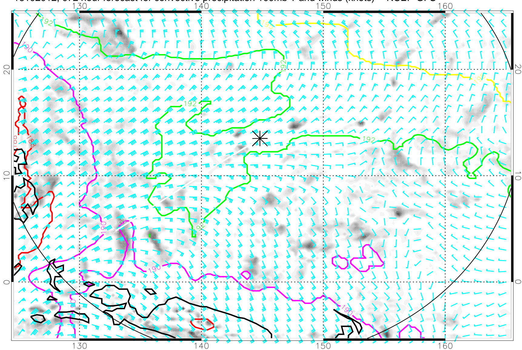
16102012, 07Z hour forecast for convective precipitation 100mb T and winds (knots) -- NCEP GFS
