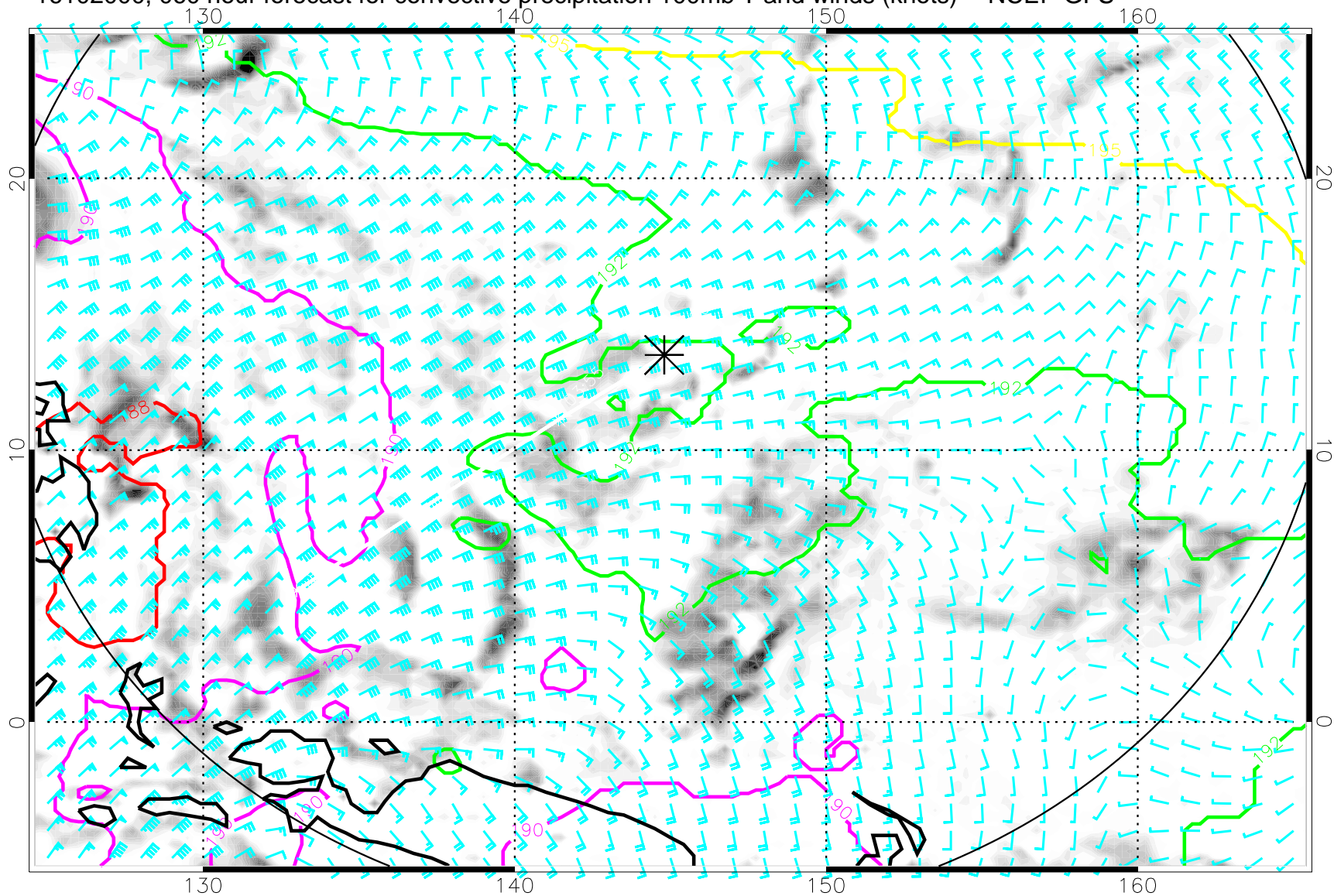
16102000, 060 hour forecast for convective precipitation 100mb T and winds (knots) -- NCEP GFS
