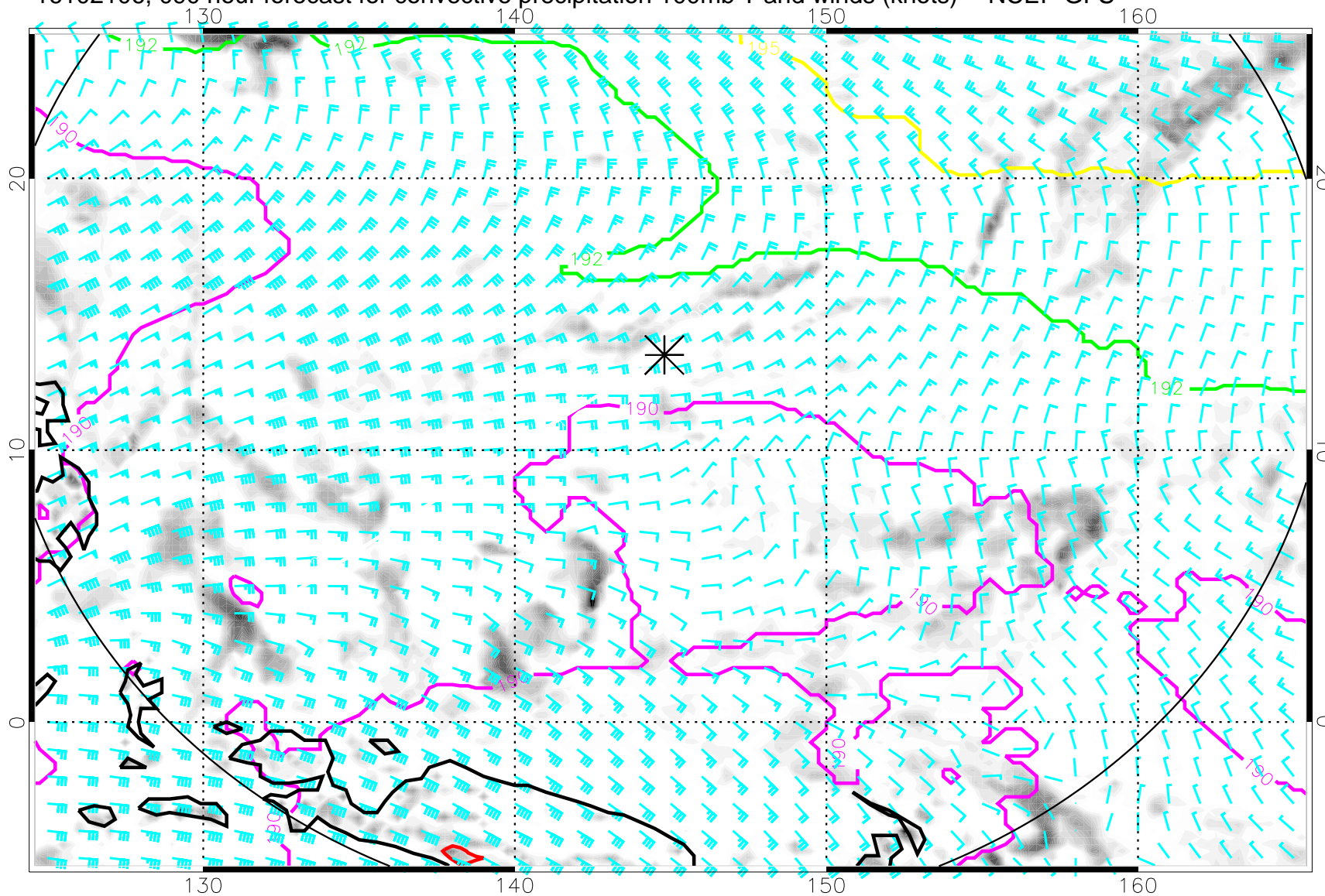
16102106, 090 hour forecast for convective precipitation 100mb T and winds (knots) -- NCEP GFS
