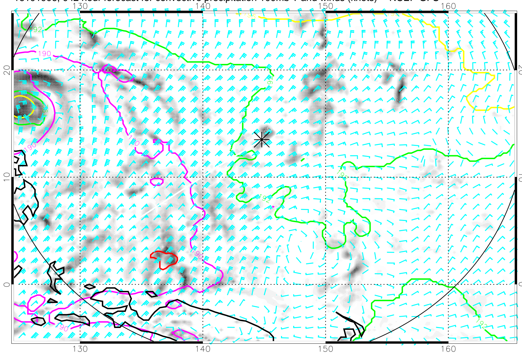
16101906, 042 hour forecast for convective precipitation 100mb T and winds (knots) -- NCEP GFS
