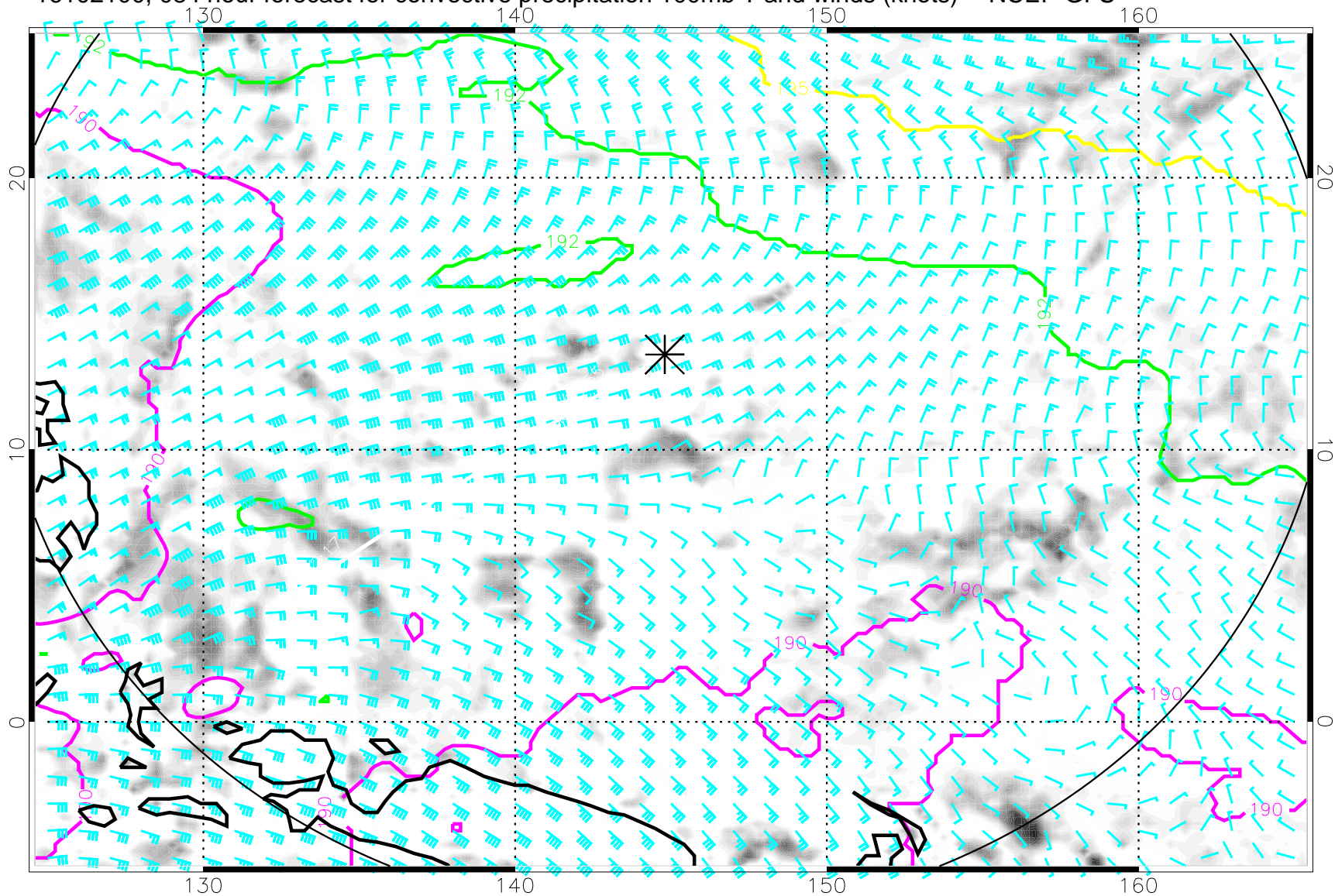
16102100, 084 hour forecast for convective precipitation 100mb T and winds (knots) -- NCEP GFS
