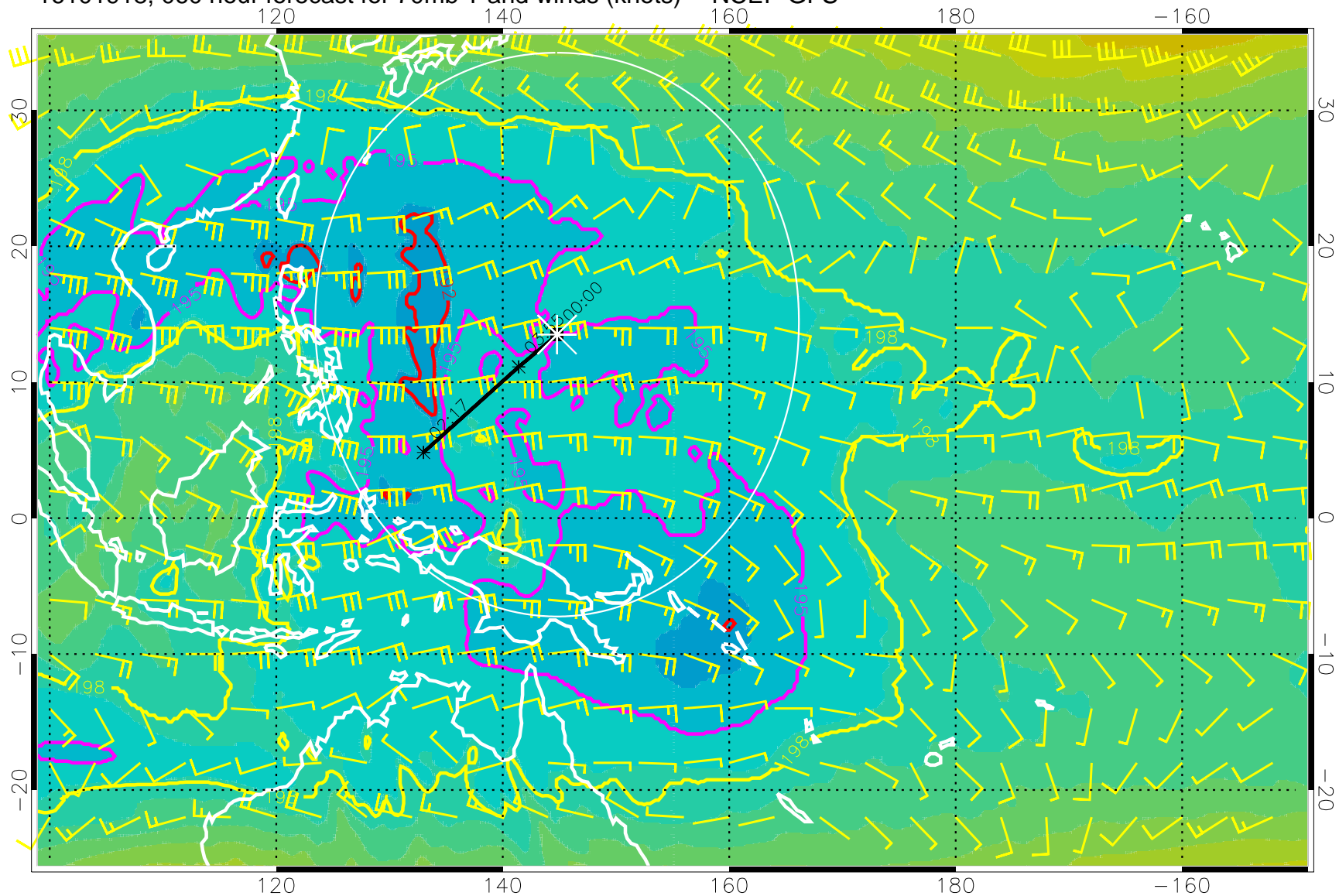
16101918, 060 hour forecast for 70mb T and winds (knots) -- NCEP GFS
