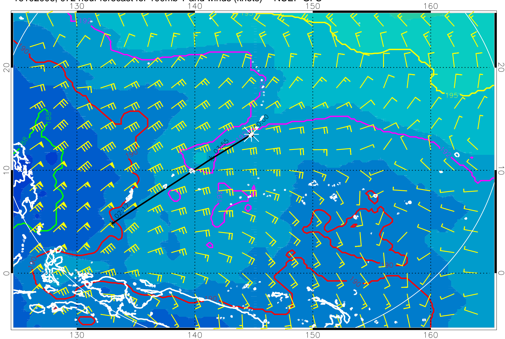
16102006, 072 hour forecast for 100mb T and winds (knots) -- NCEP GFS
