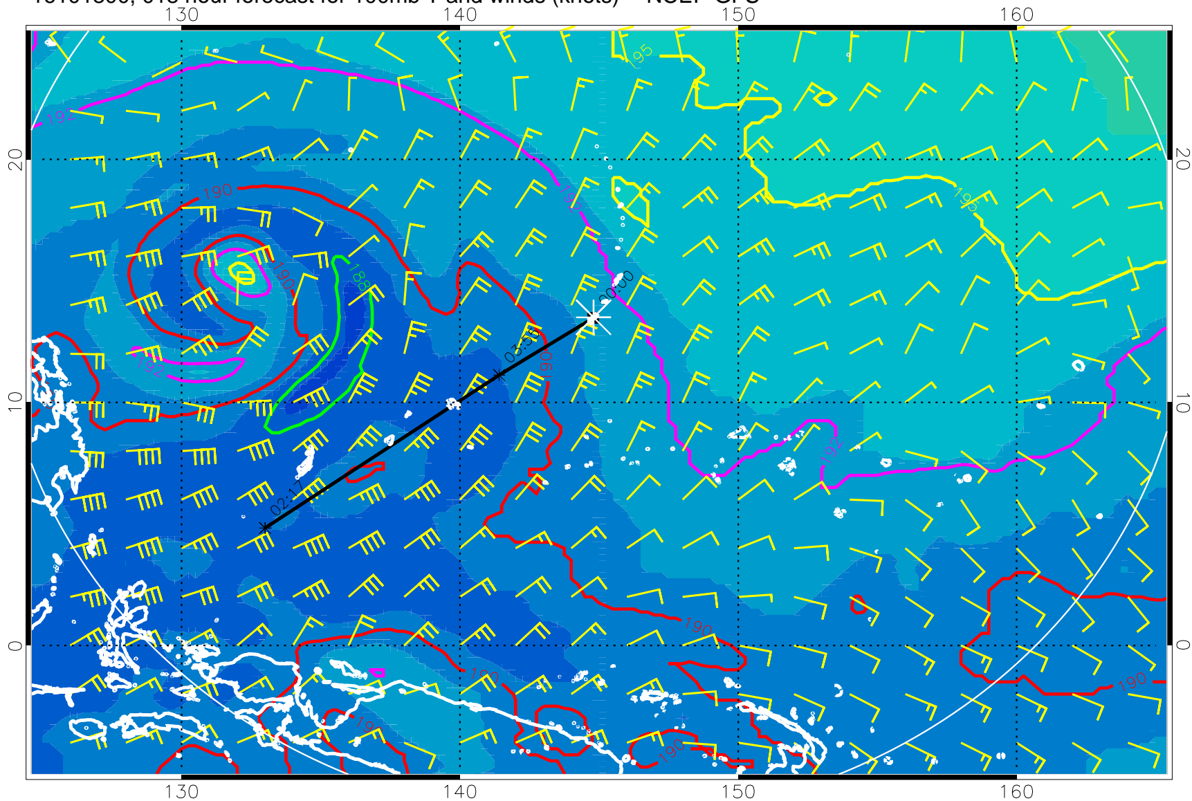
16101800, 018 hour forecast for 100mb T and winds (knots) -- NCEP GFS
