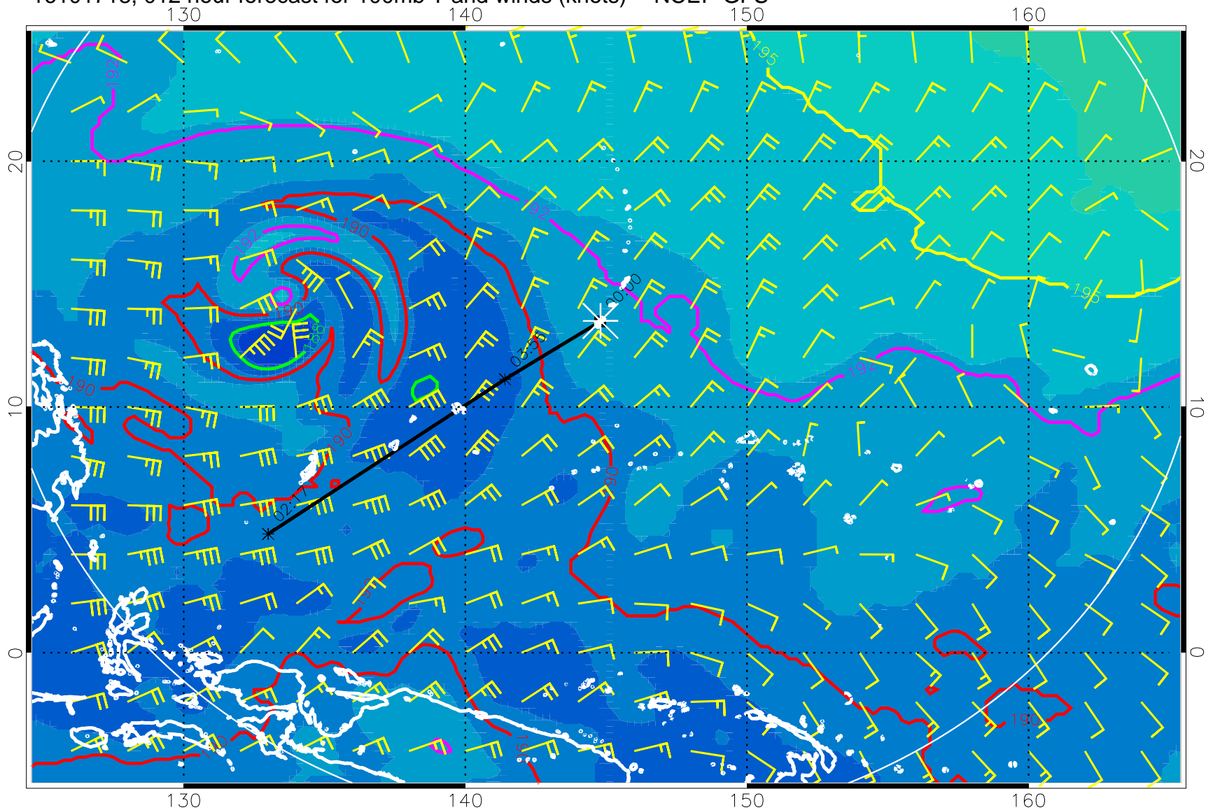
16101718, 012 hour forecast for 100mb T and winds (knots) -- NCEP GFS
