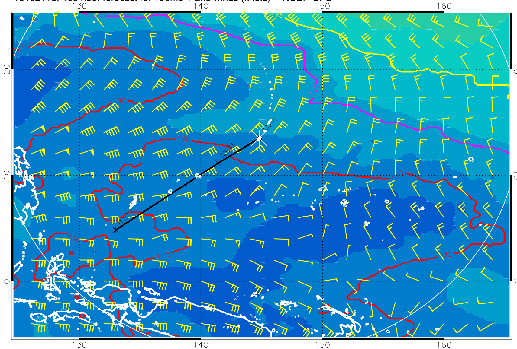
16102118, 108 hour forecast for 100mb T and winds (knots) -- NCEP GFS
