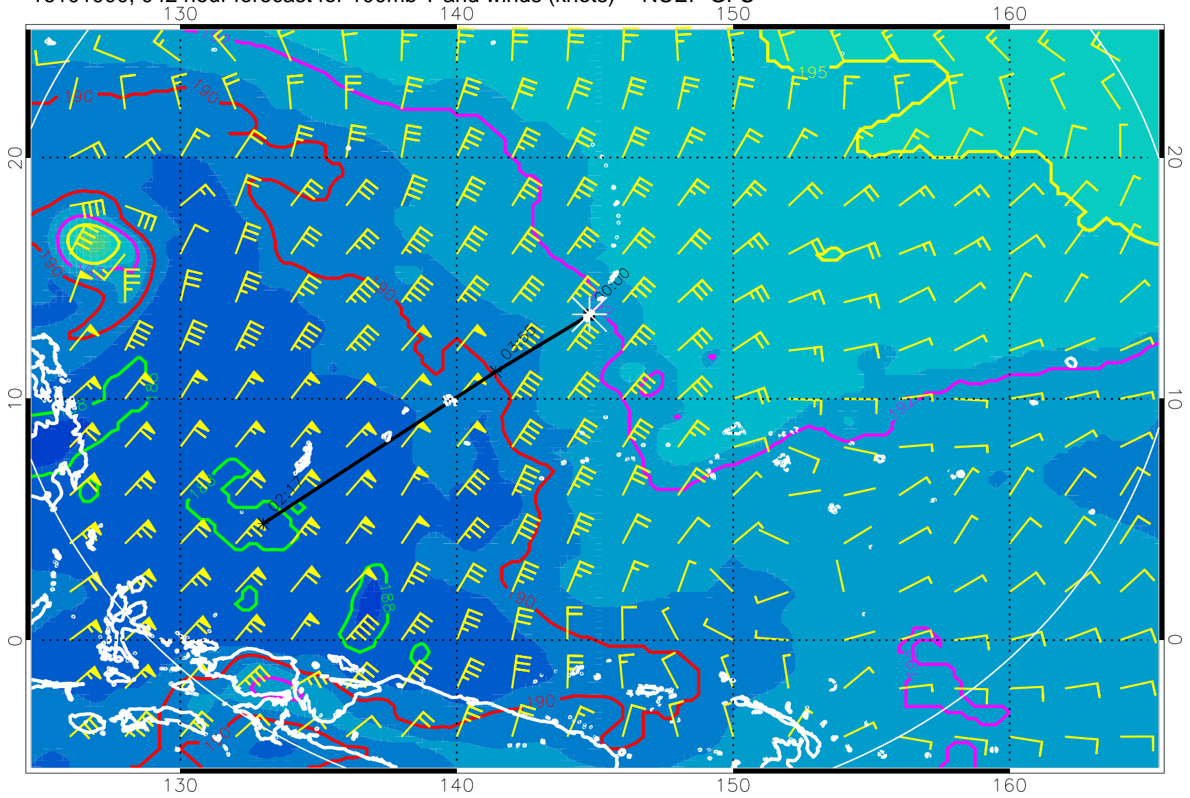
16101900, 042 hour forecast for 100mb T and winds (knots) -- NCEP GFS
