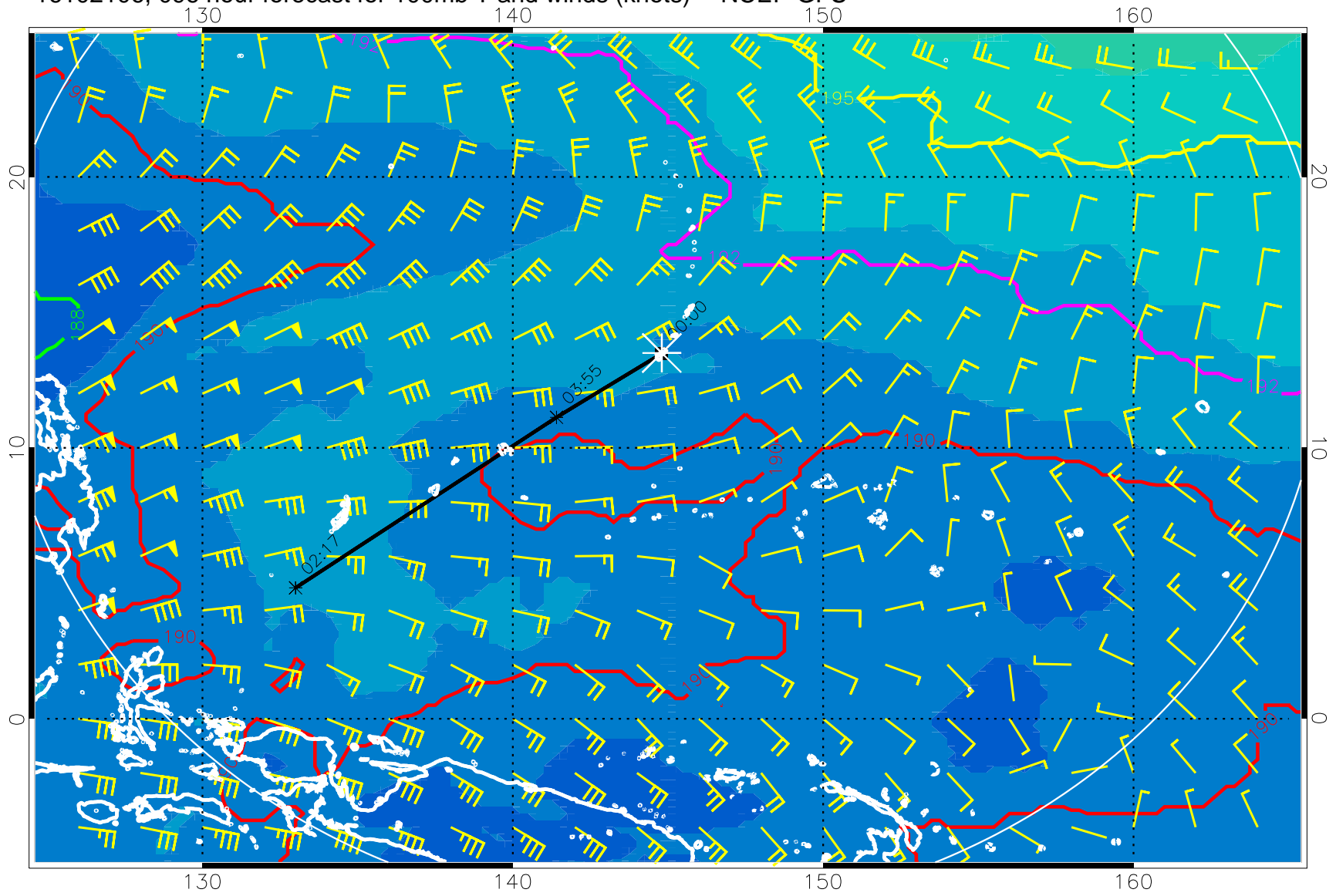
16102106, 096 hour forecast for 100mb T and winds (knots) -- NCEP GFS
