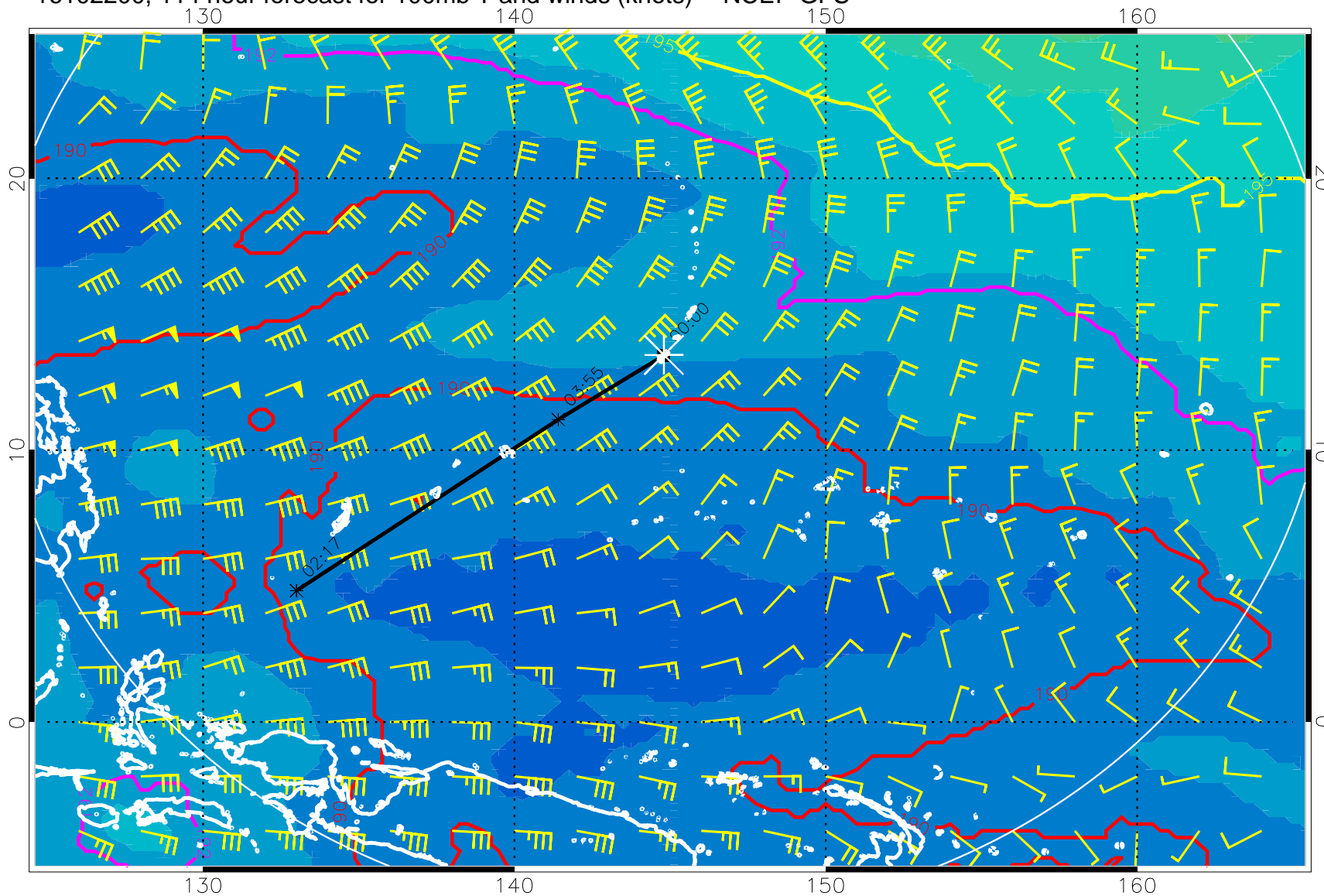
16102200, 114 hour forecast for 100mb T and winds (knots) -- NCEP GFS
