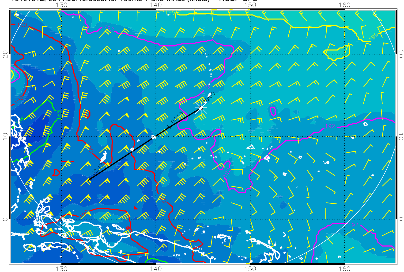
16101912, 054 hour forecast for 100mb T and winds (knots) -- NCEP GFS
