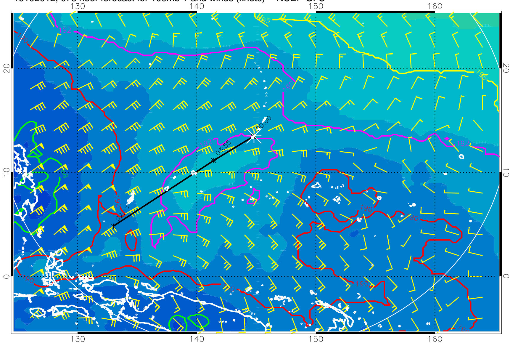
16102012, 078 hour forecast for 100mb T and winds (knots) -- NCEP GFS
