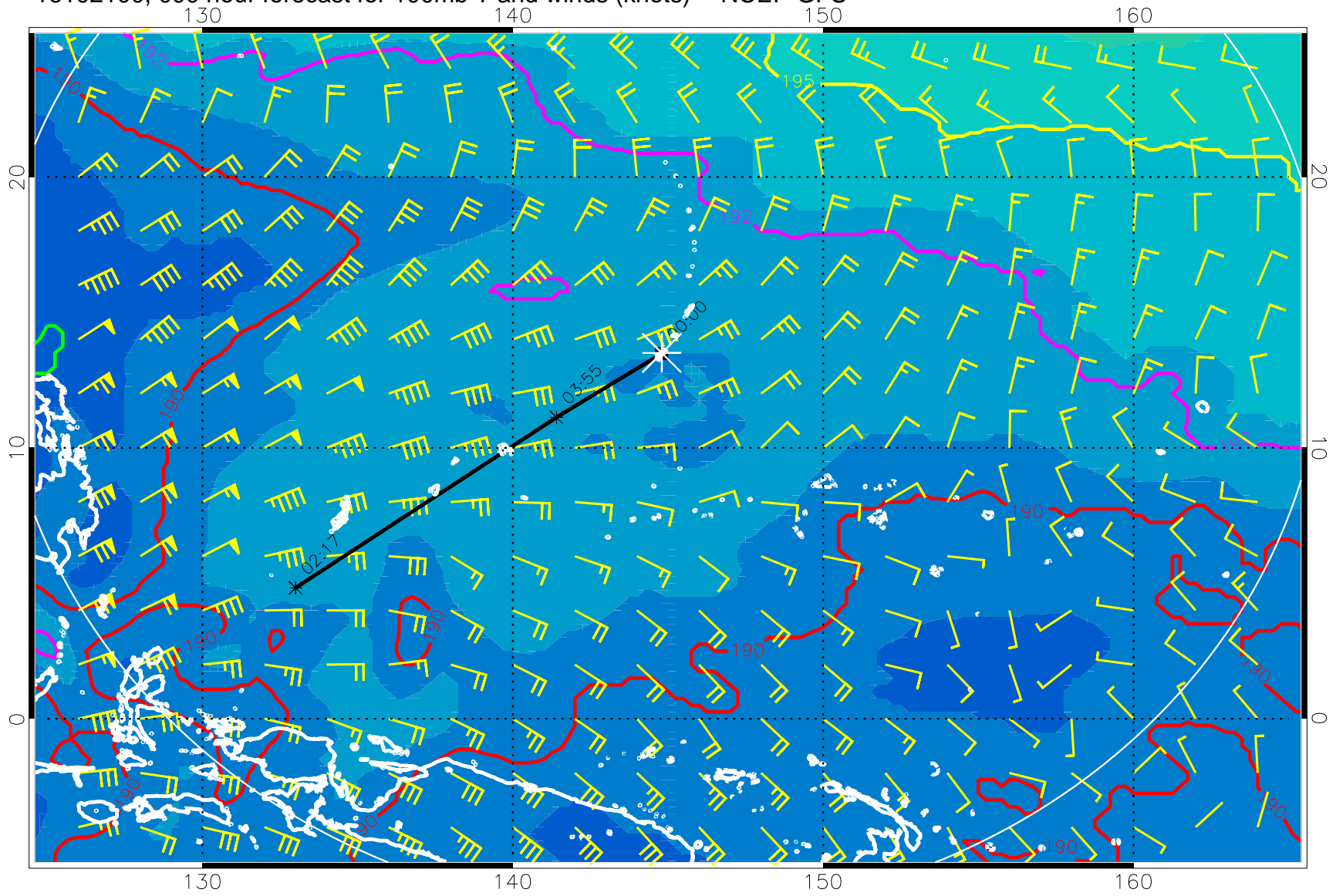
16102100, 090 hour forecast for 100mb T and winds (knots) -- NCEP GFS
