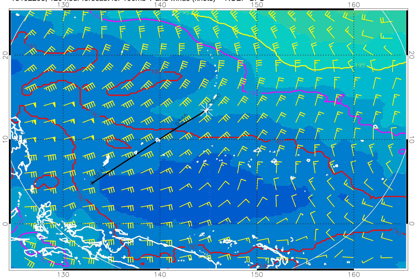
16102206, 120 hour forecast for 100mb T and winds (knots) -- NCEP GFS
