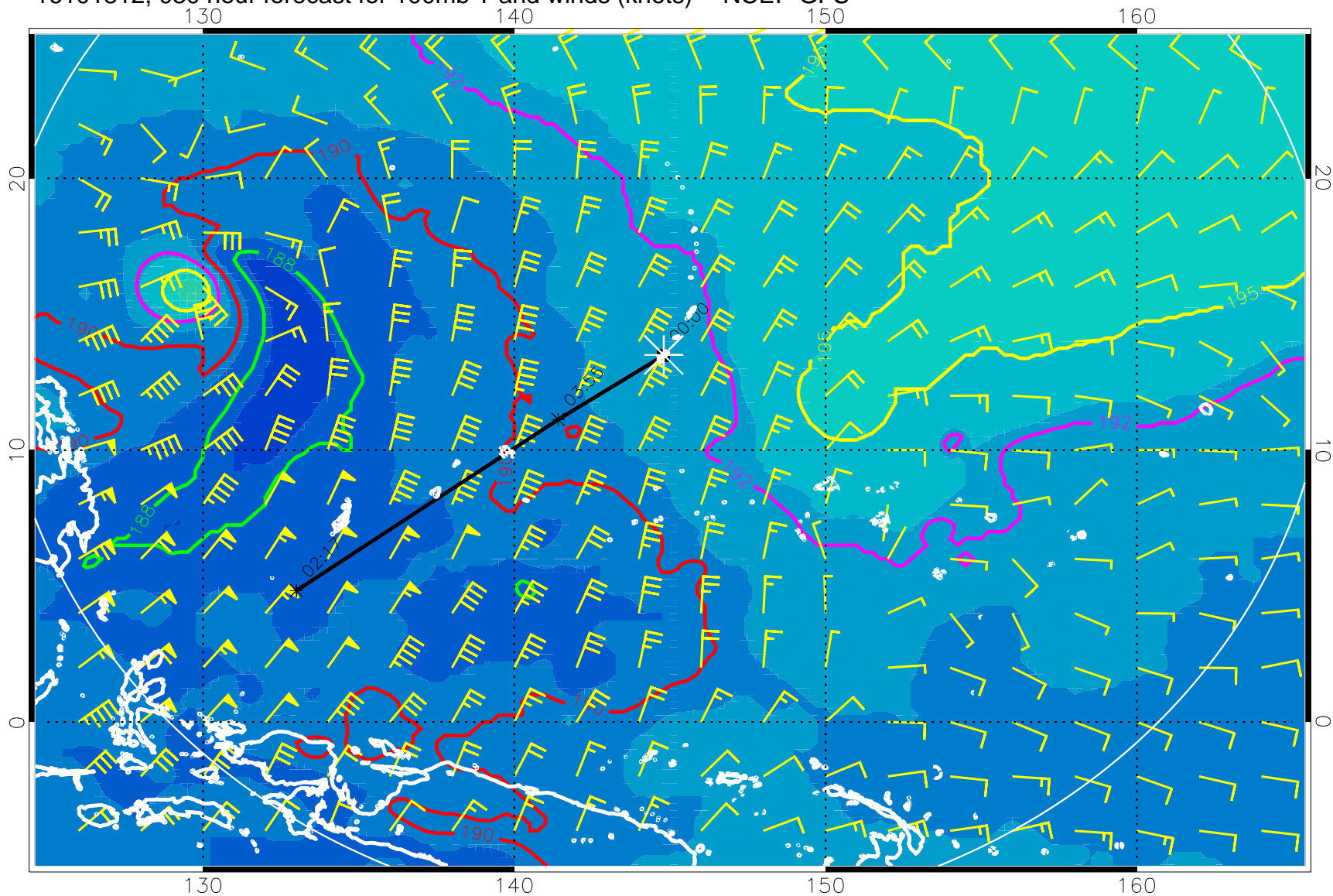
16101812, 030 hour forecast for 100mb T and winds (knots) -- NCEP GFS
