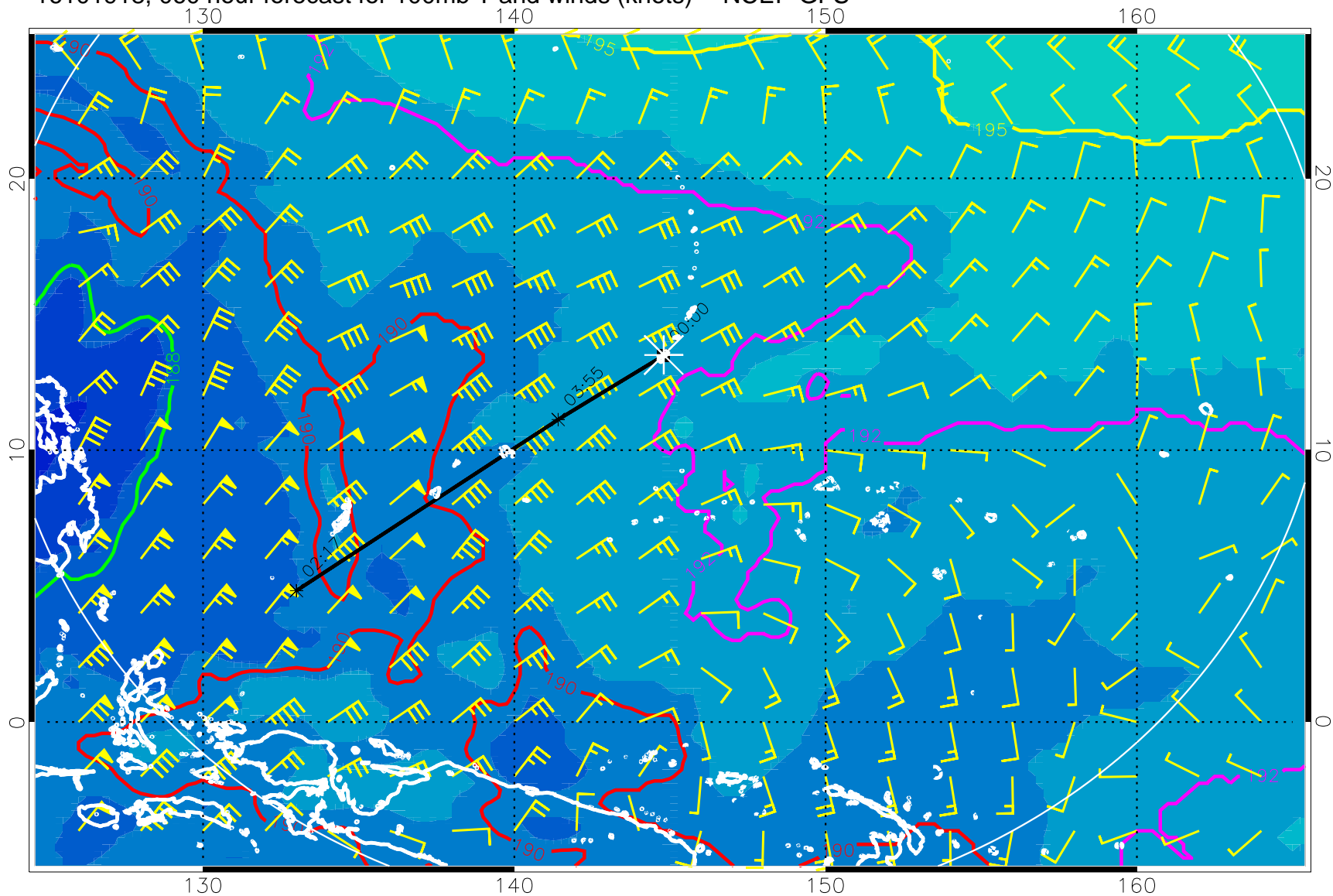
16101918, 060 hour forecast for 100mb T and winds (knots) -- NCEP GFS
