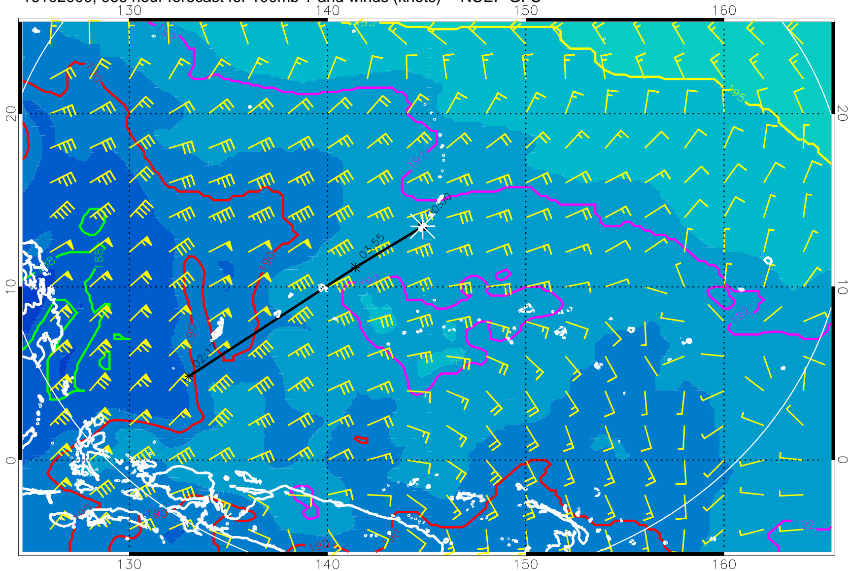
16102000, 066 hour forecast for 100mb T and winds (knots) -- NCEP GFS
