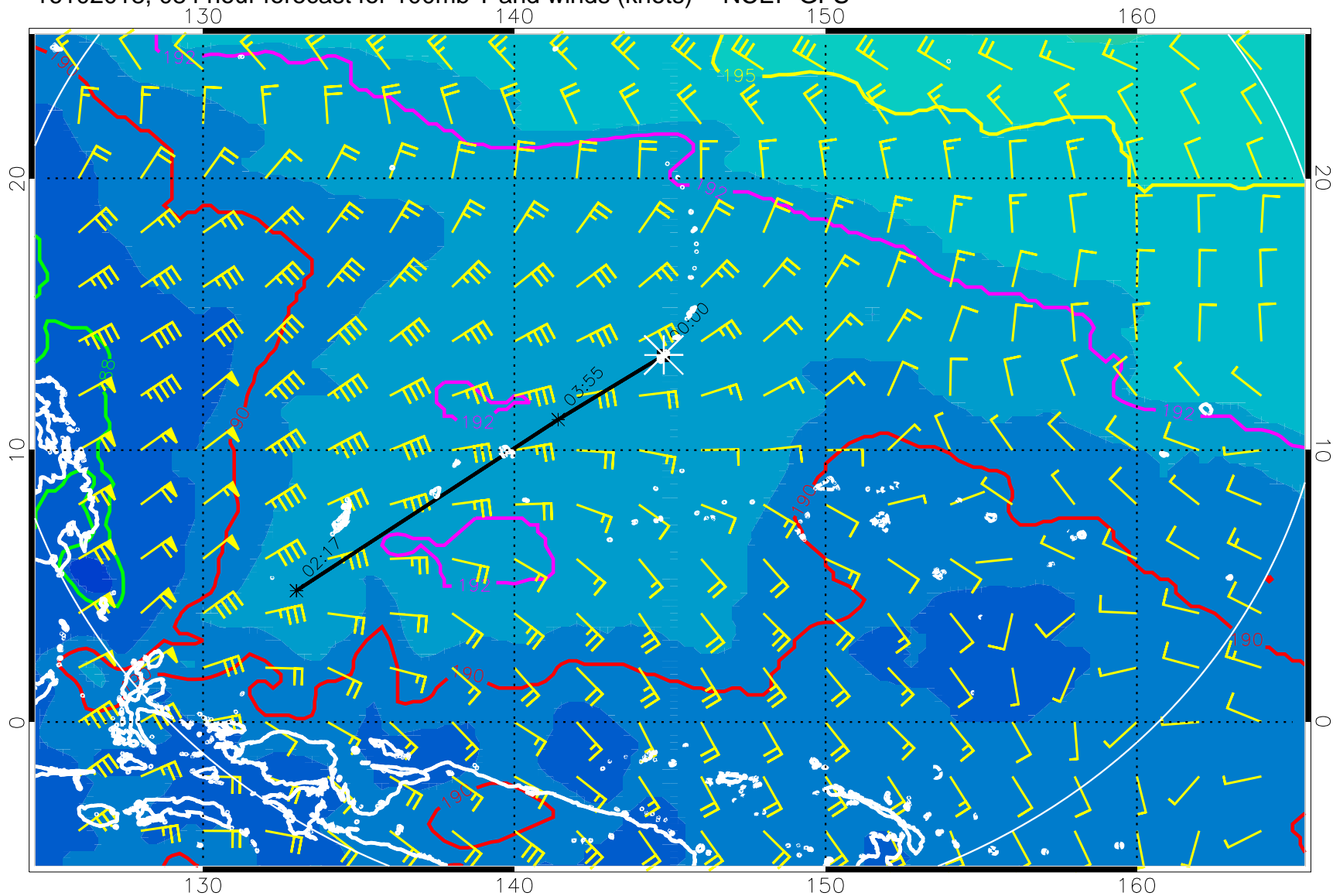
16102018, 084 hour forecast for 100mb T and winds (knots) -- NCEP GFS
