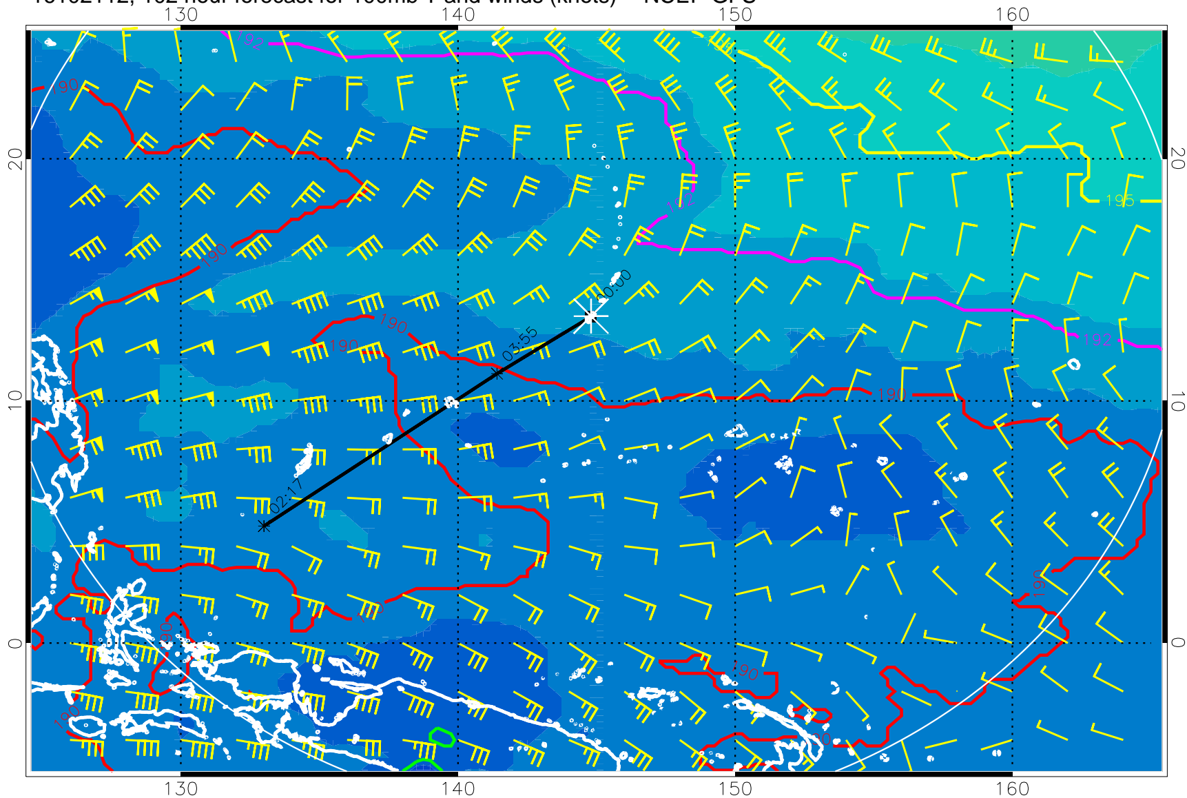
16102112, 102 hour forecast for 100mb T and winds (knots) -- NCEP GFS
