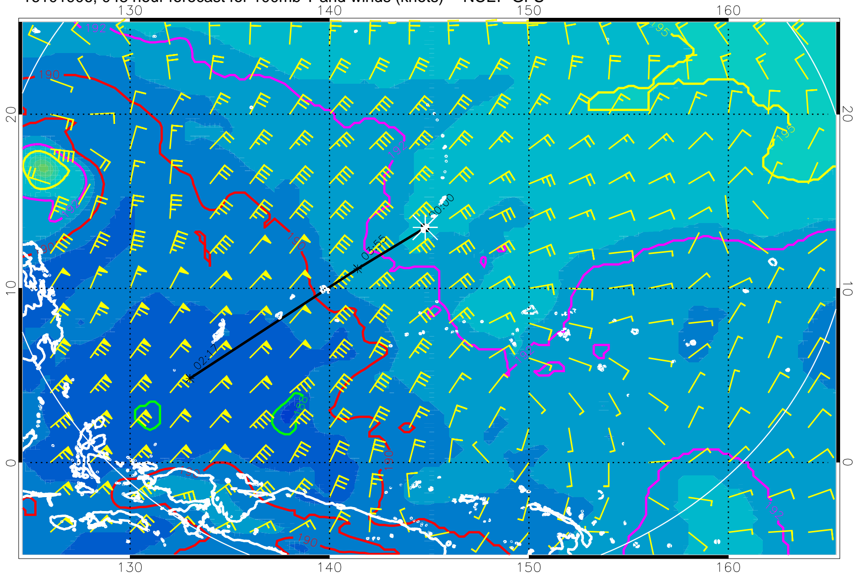
16101906, 048 hour forecast for 100mb T and winds (knots) -- NCEP GFS
