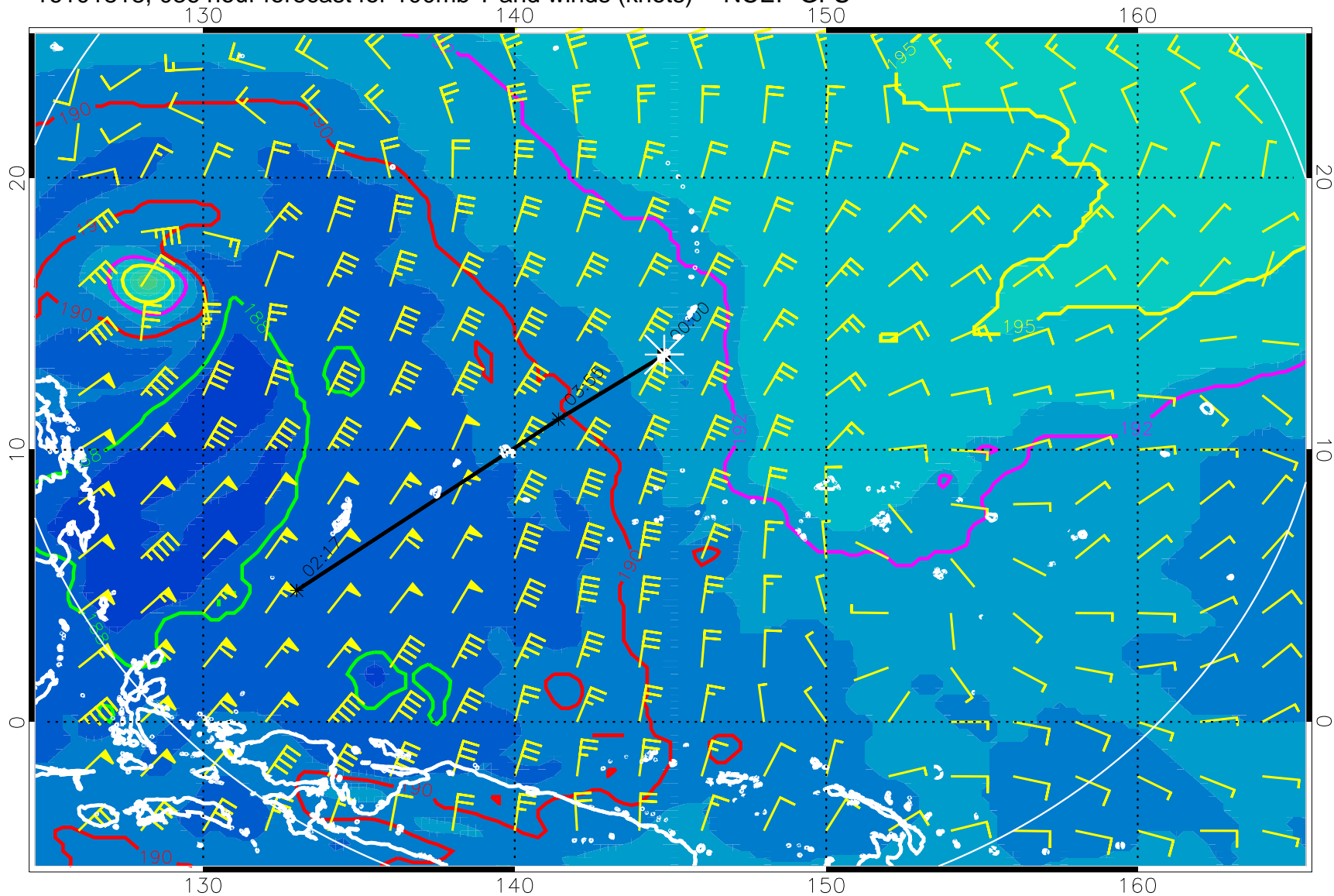
16101818, 036 hour forecast for 100mb T and winds (knots) -- NCEP GFS
