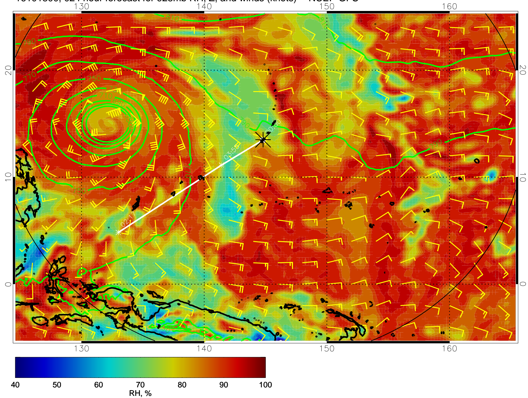
16101800, 024 hour forecast for 925mb RH, Z, and winds (knots) -- NCEP GFS
