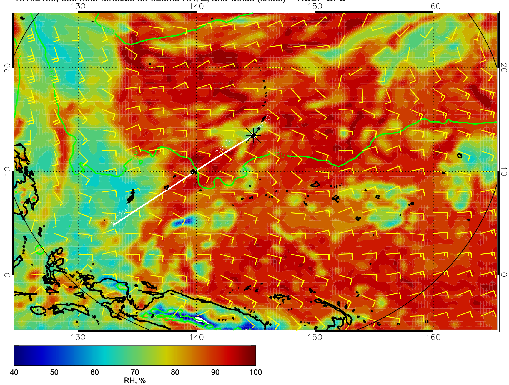
16102100, 096 hour forecast for 925mb RH, Z, and winds (knots) -- NCEP GFS
