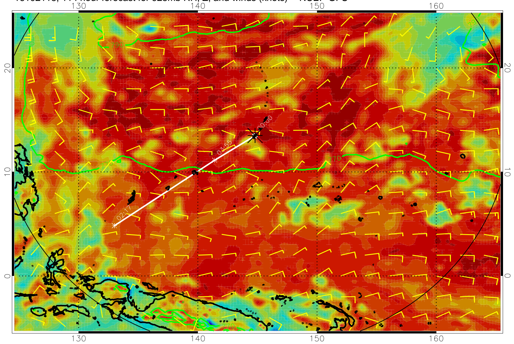
16102118, 114 hour forecast for 925mb RH, Z, and winds (knots) -- NCEP GFS
