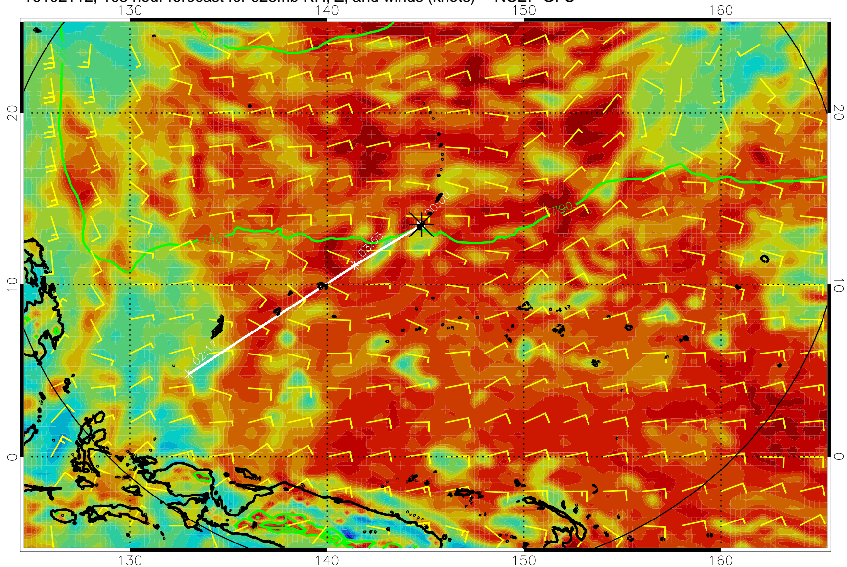
16102112, 108 hour forecast for 925mb RH, Z, and winds (knots) -- NCEP GFS
