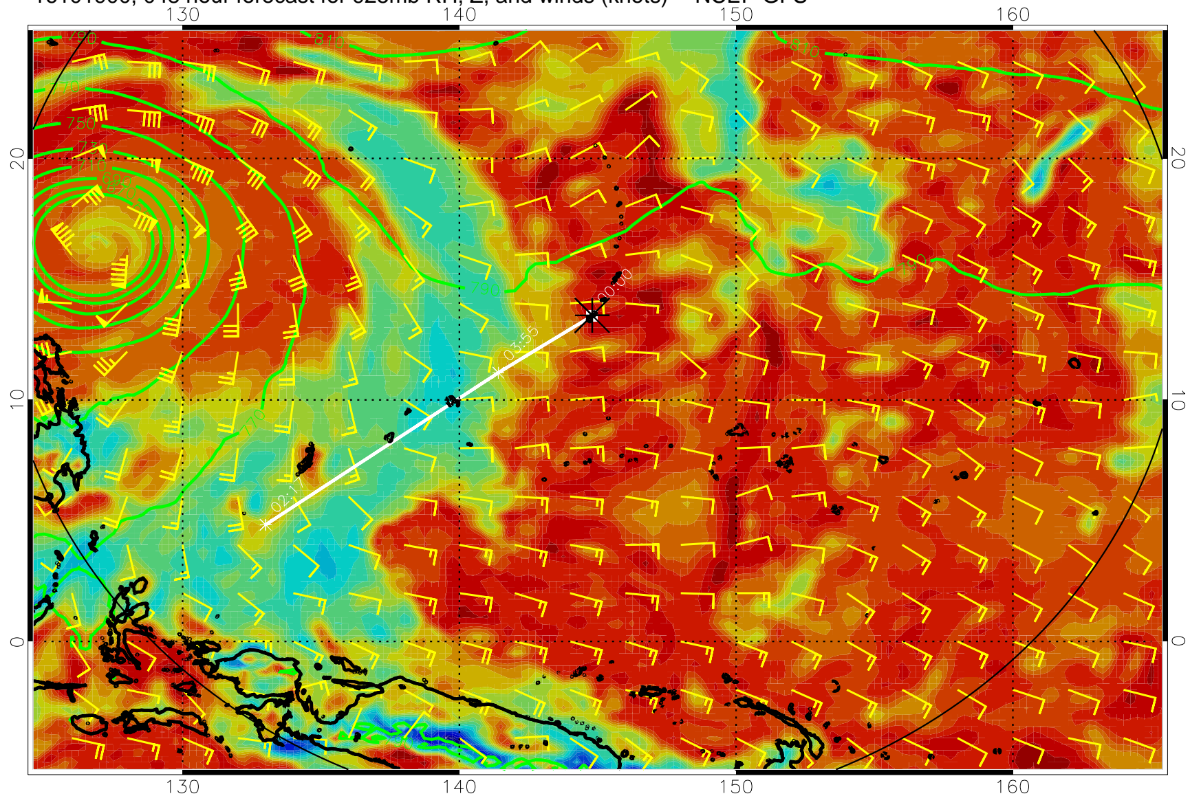
16101900, 048 hour forecast for 925mb RH, Z, and winds (knots) -- NCEP GFS
