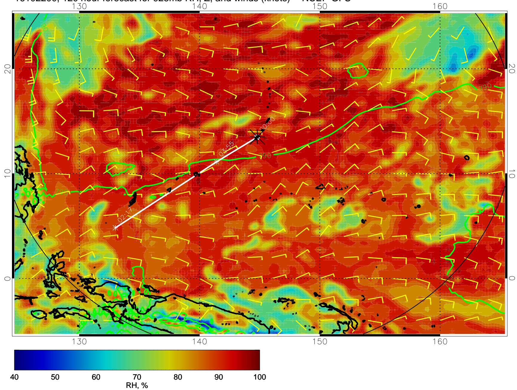
16102200, 120 hour forecast for 925mb RH, Z, and winds (knots) -- NCEP GFS
