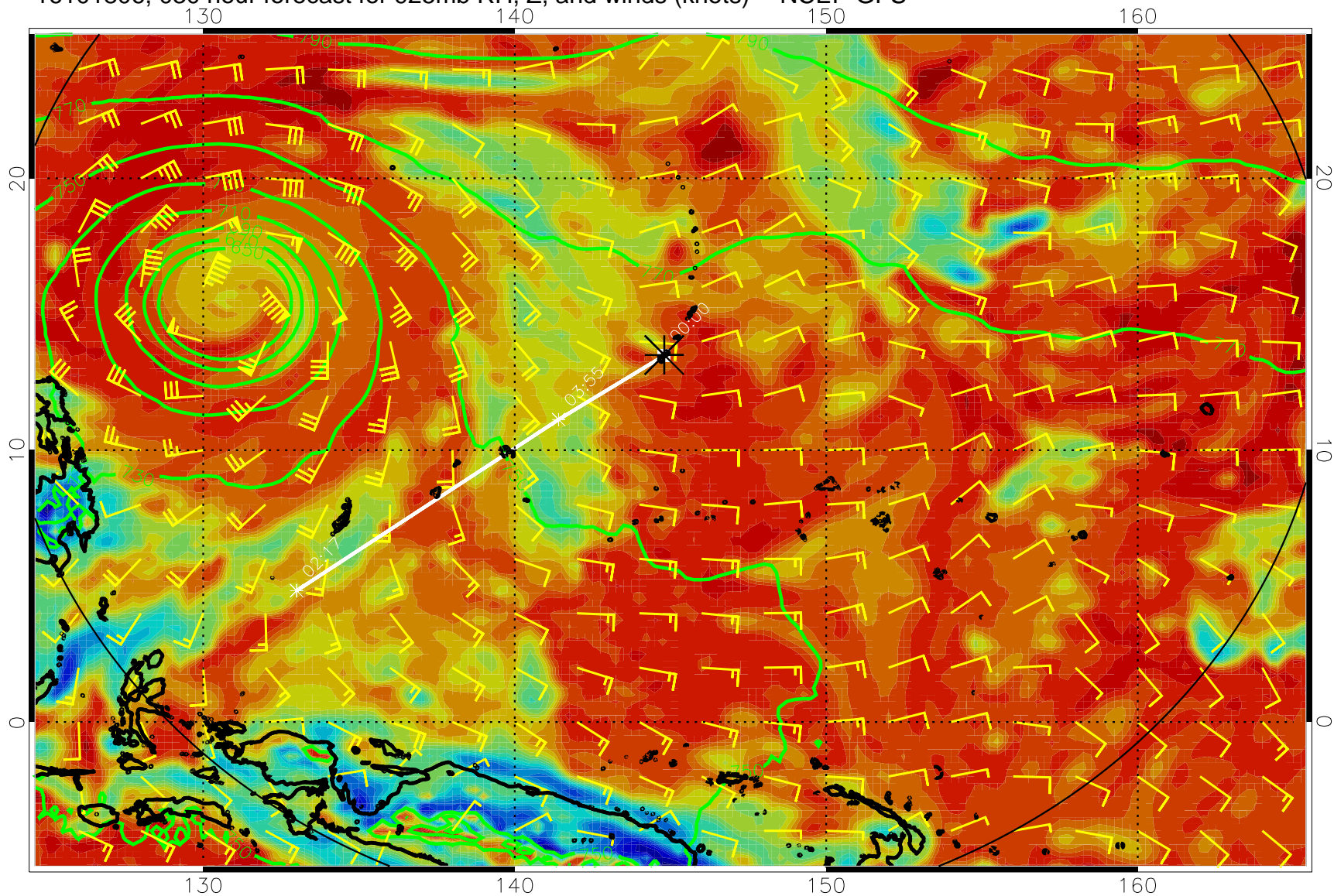
16101806, 030 hour forecast for 925mb RH, Z, and winds (knots) -- NCEP GFS
