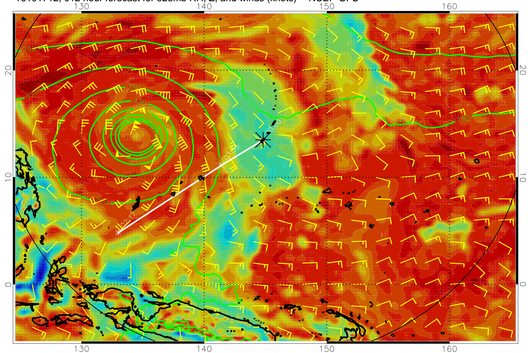
16101712, 012 hour forecast for 925mb RH, Z, and winds (knots) -- NCEP GFS
