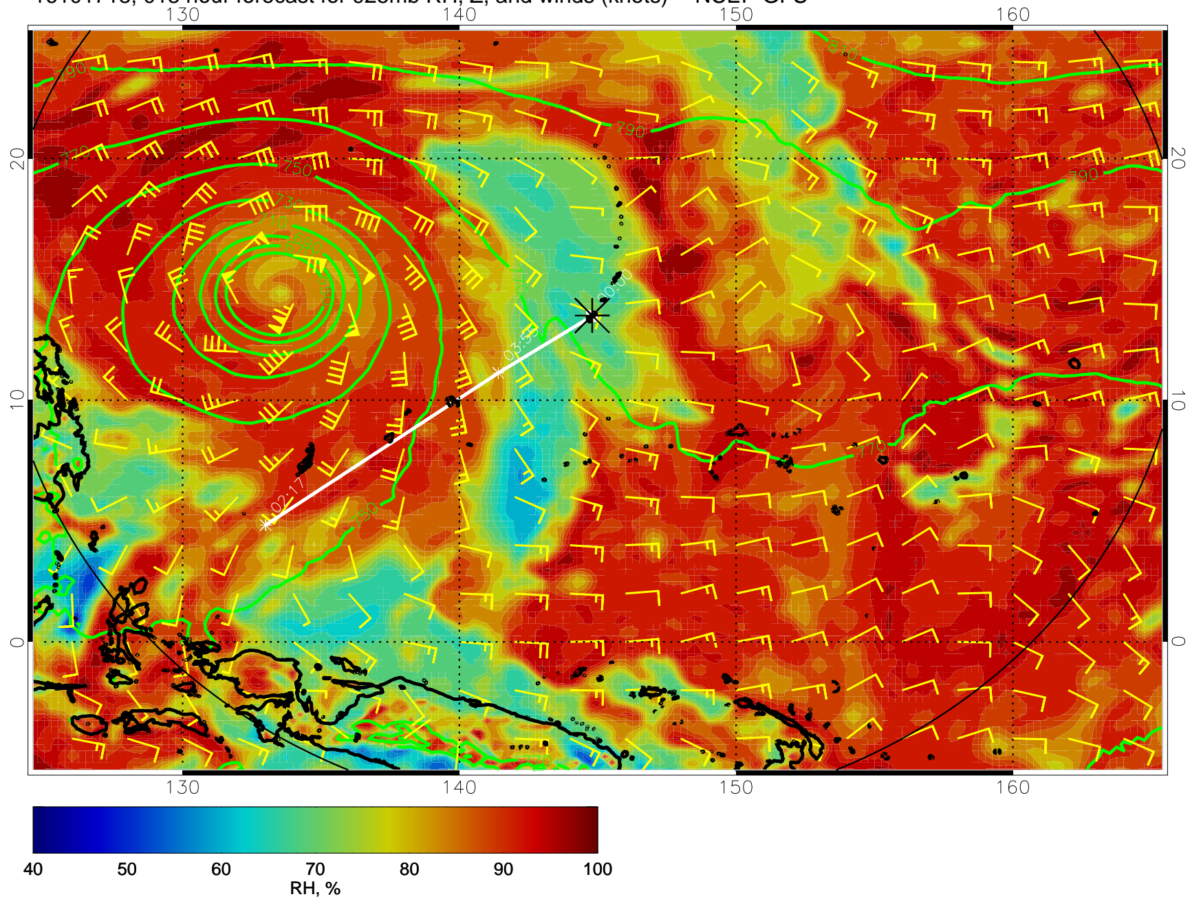
16101718, 018 hour forecast for 925mb RH, Z, and winds (knots) -- NCEP GFS
