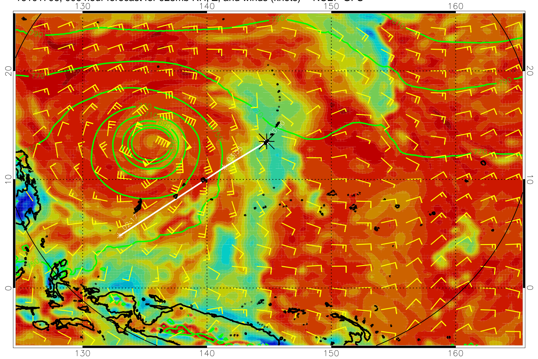
16101706, 006 hour forecast for 925mb RH, Z, and winds (knots) -- NCEP GFS
