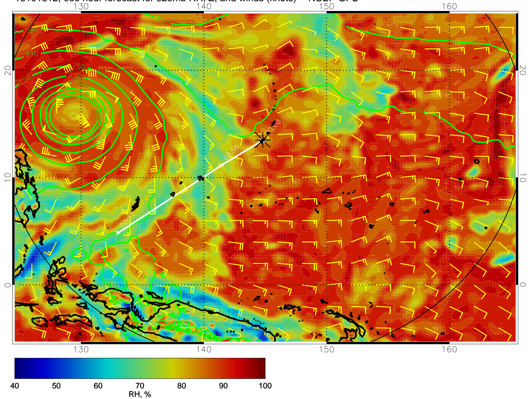
16101812, 036 hour forecast for 925mb RH, Z, and winds (knots) -- NCEP GFS
