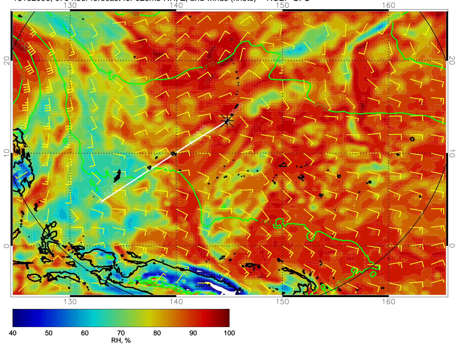
16102006, 078 hour forecast for 925mb RH, Z, and winds (knots) -- NCEP GFS
