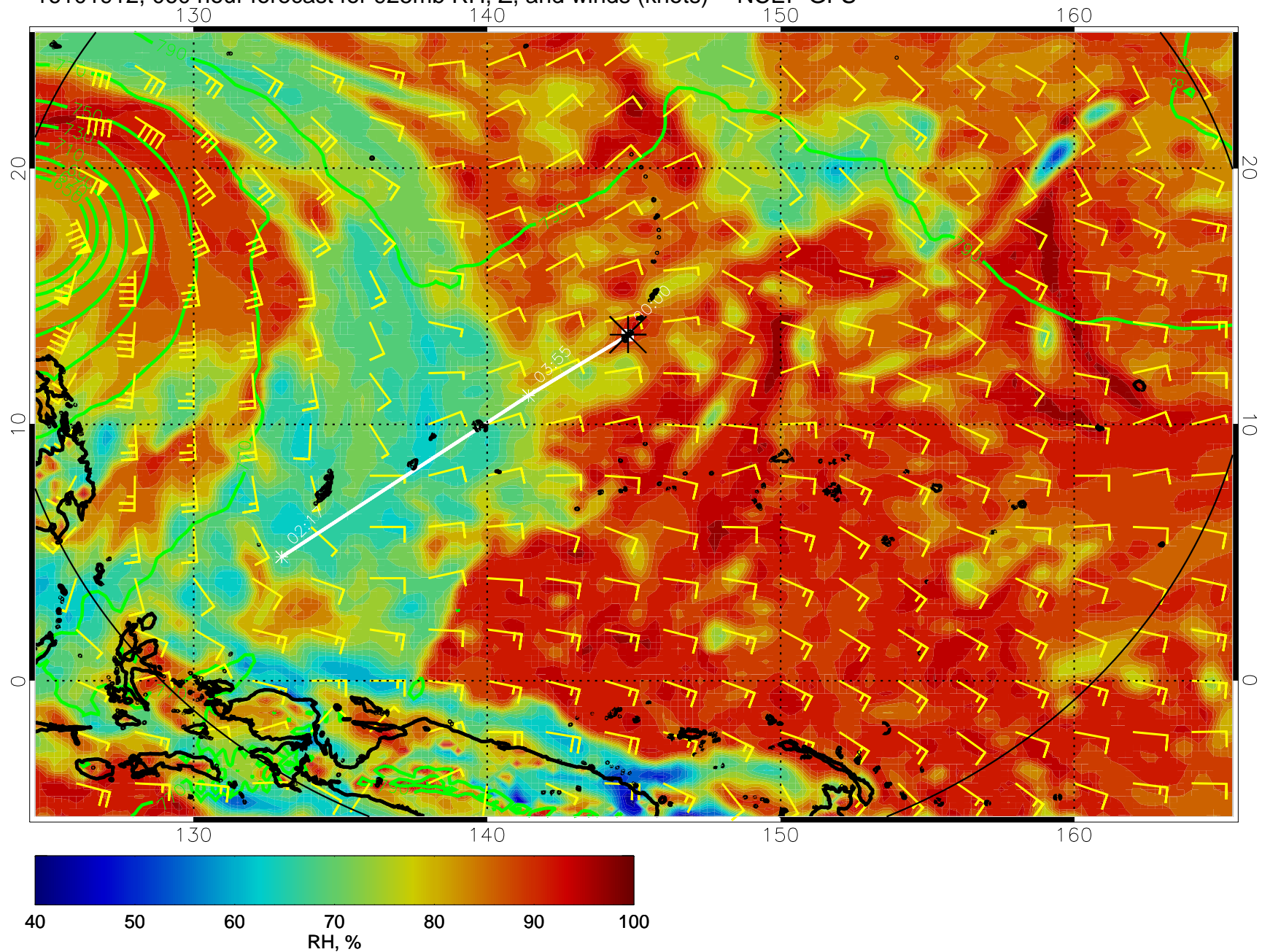
16101912, 060 hour forecast for 925mb RH, Z, and winds (knots) -- NCEP GFS
