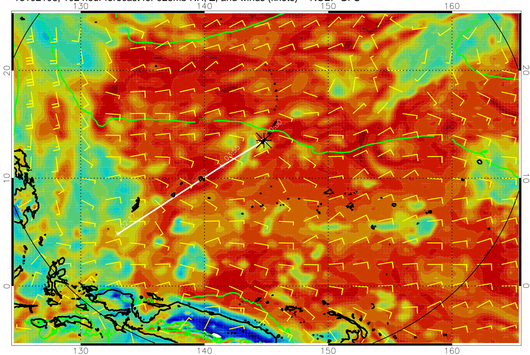
16102106, 102 hour forecast for 925mb RH, Z, and winds (knots) -- NCEP GFS
