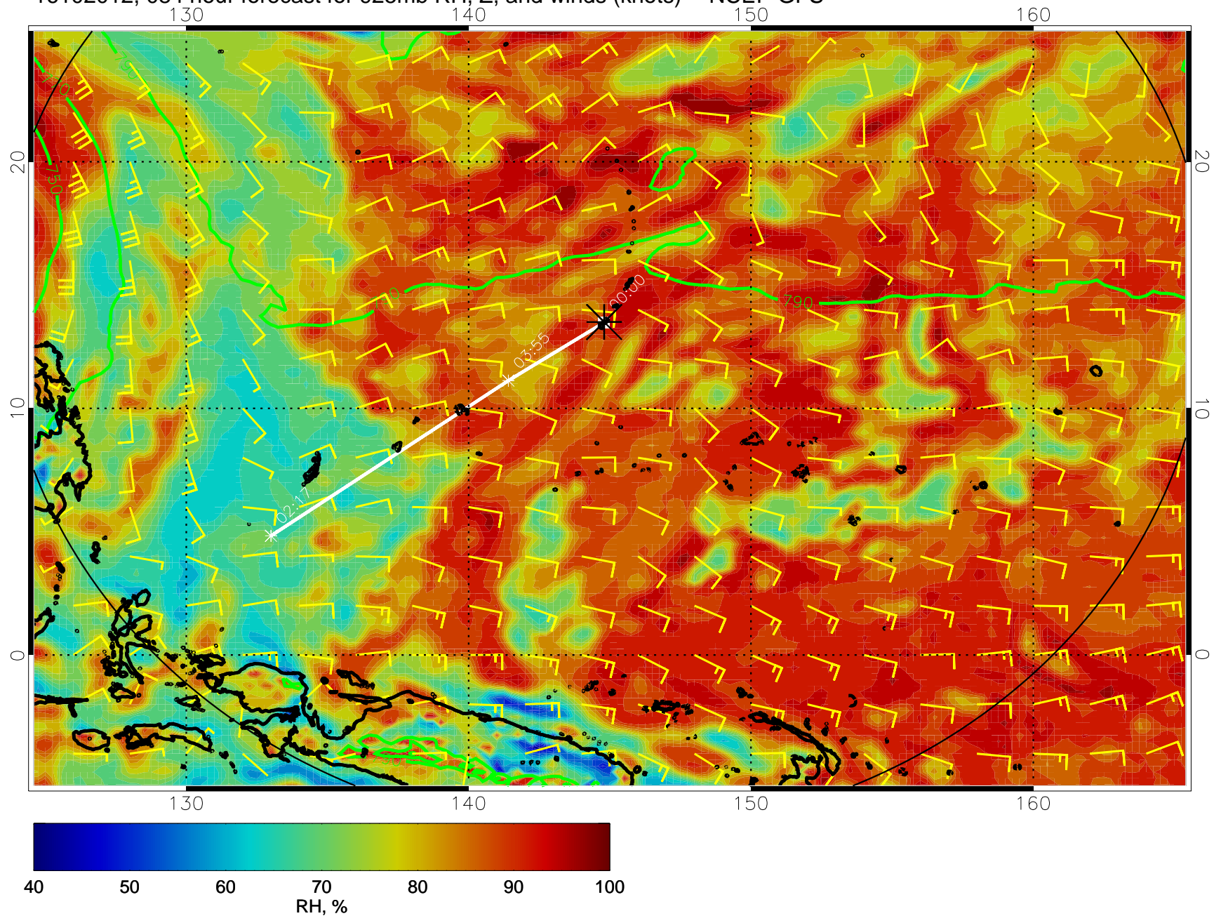
16102012, 084 hour forecast for 925mb RH, Z, and winds (knots) -- NCEP GFS
