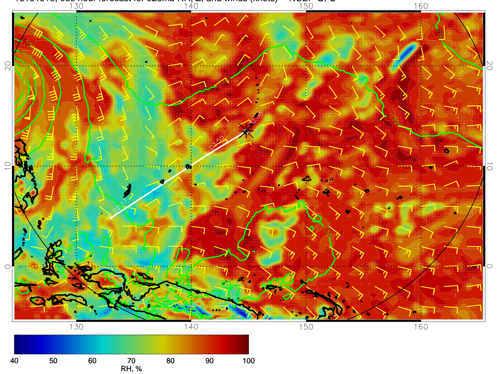
16101918, 066 hour forecast for 925mb RH, Z, and winds (knots) -- NCEP GFS
