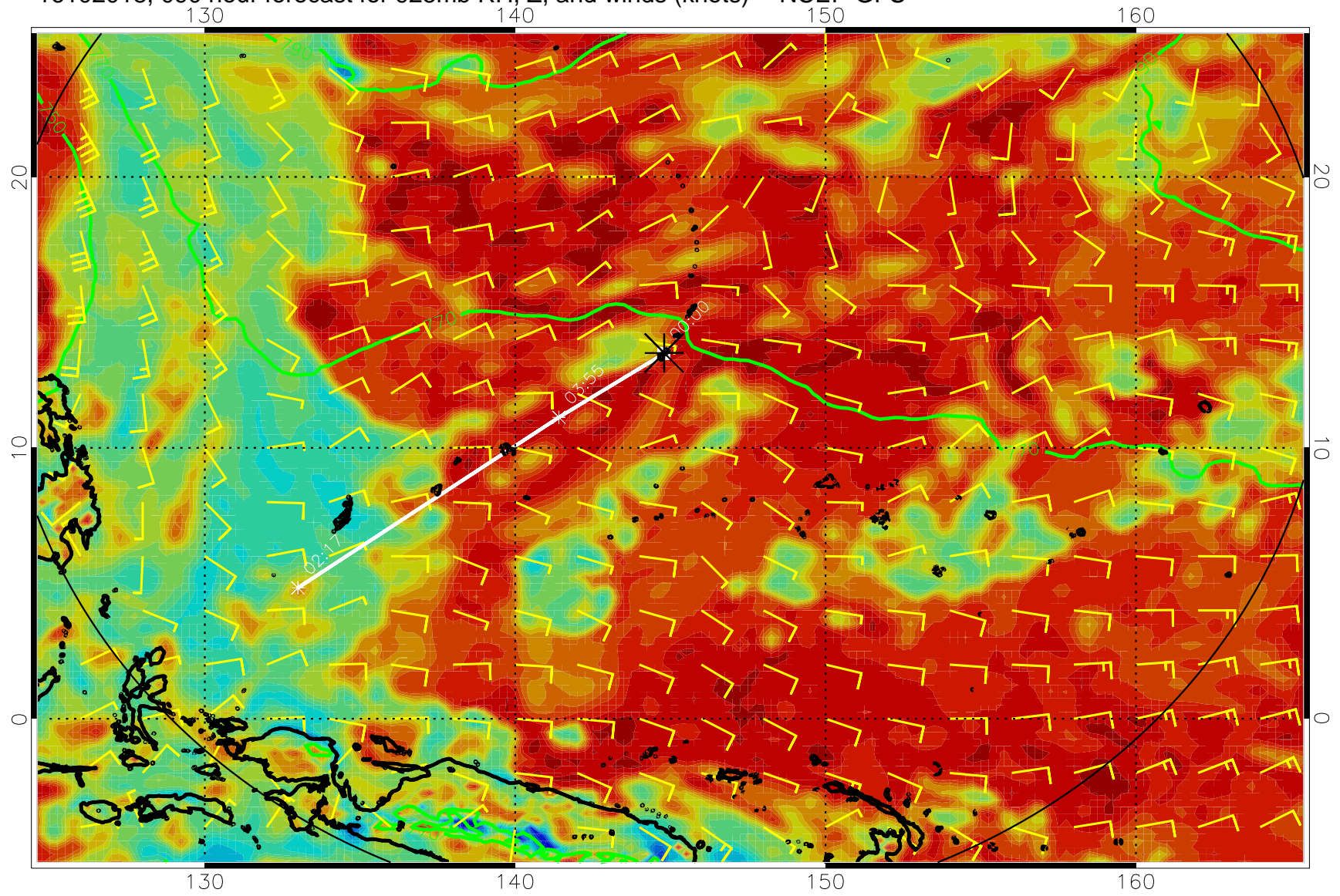
16102018, 090 hour forecast for 925mb RH, Z, and winds (knots) -- NCEP GFS
