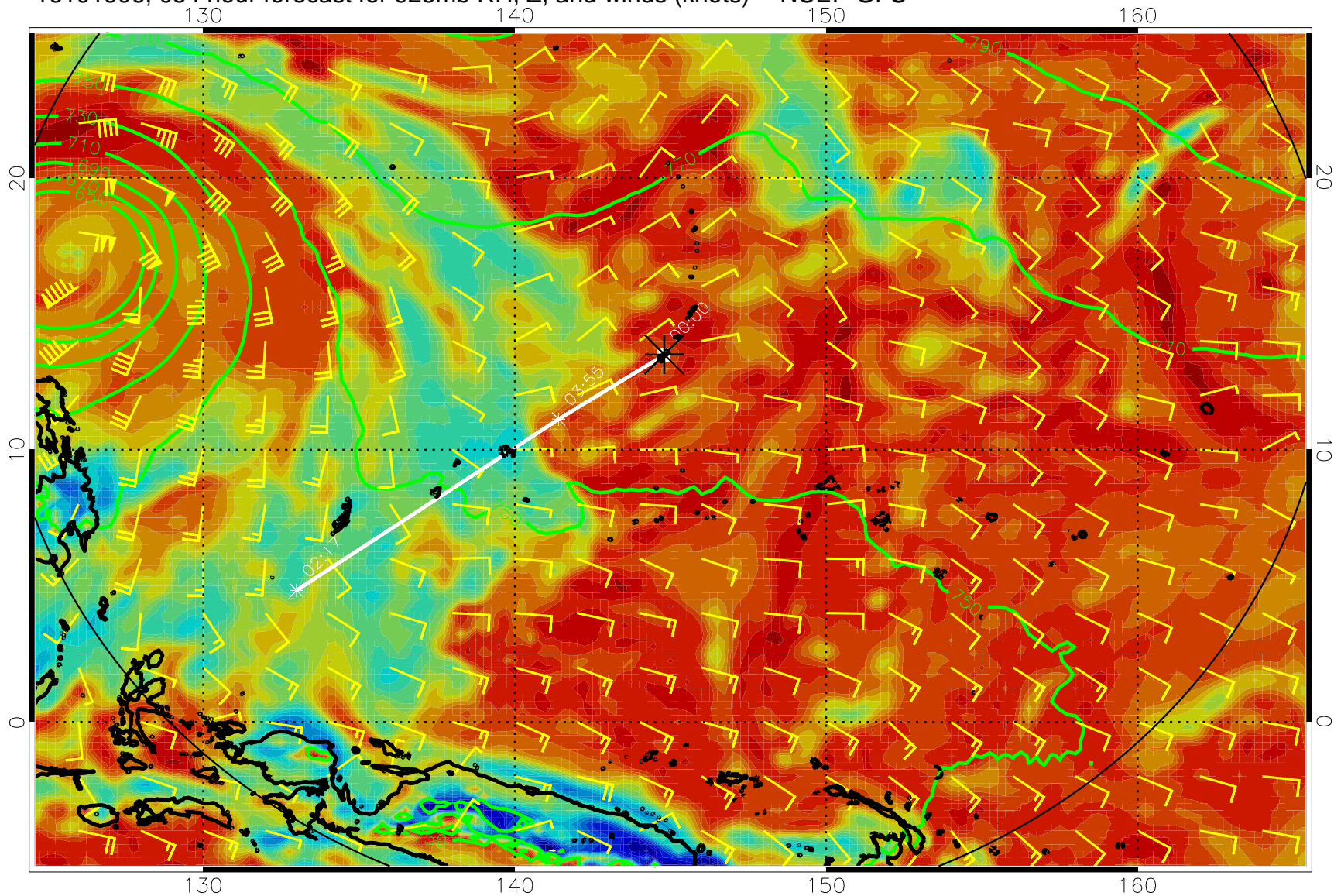
16101906, 054 hour forecast for 925mb RH, Z, and winds (knots) -- NCEP GFS
