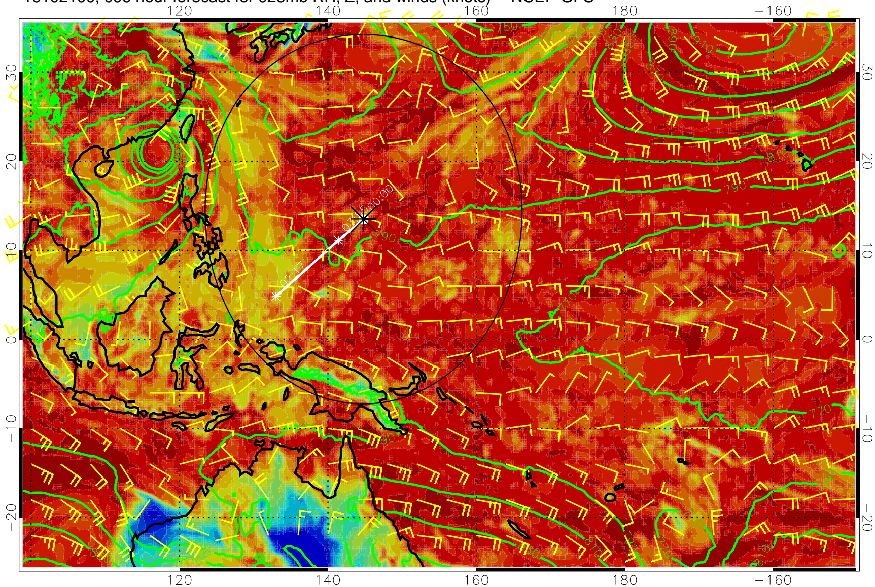
16102100, 096 hour forecast for 925mb RH, Z, and winds (knots) -- NCEP GFS
