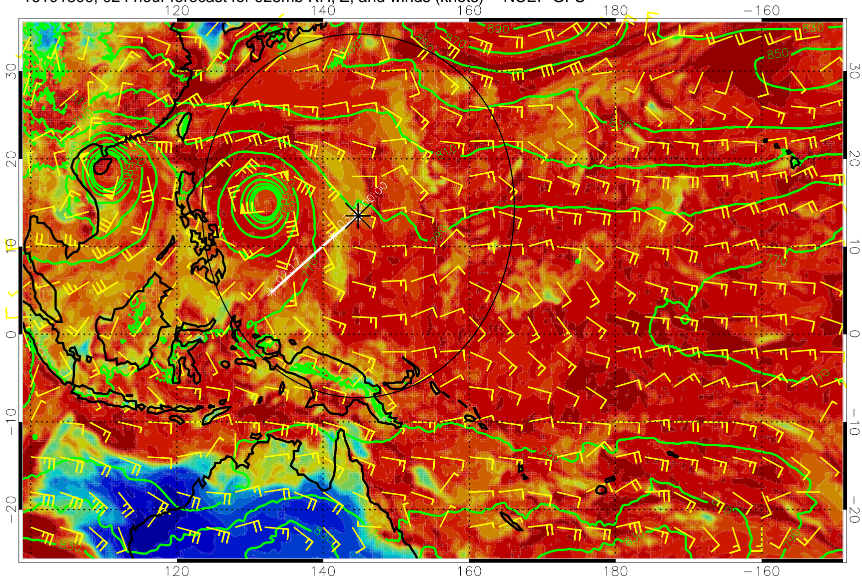
16101800, 024 hour forecast for 925mb RH, Z, and winds (knots) -- NCEP GFS
