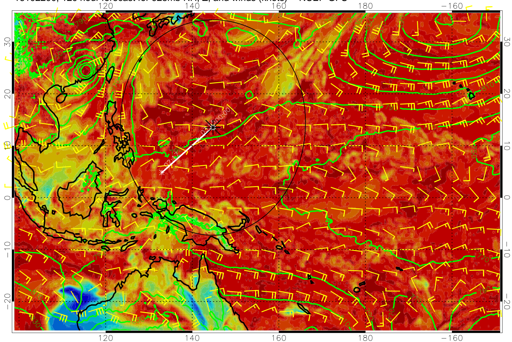
16102200, 120 hour forecast for 925mb RH, Z, and winds (knots) -- NCEP GFS
