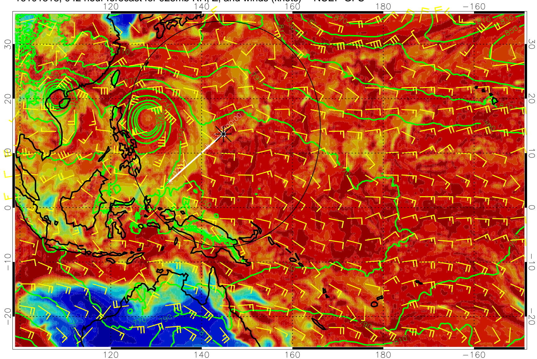
16101818, 042 hour forecast for 925mb RH, Z, and winds (knots) -- NCEP GFS
