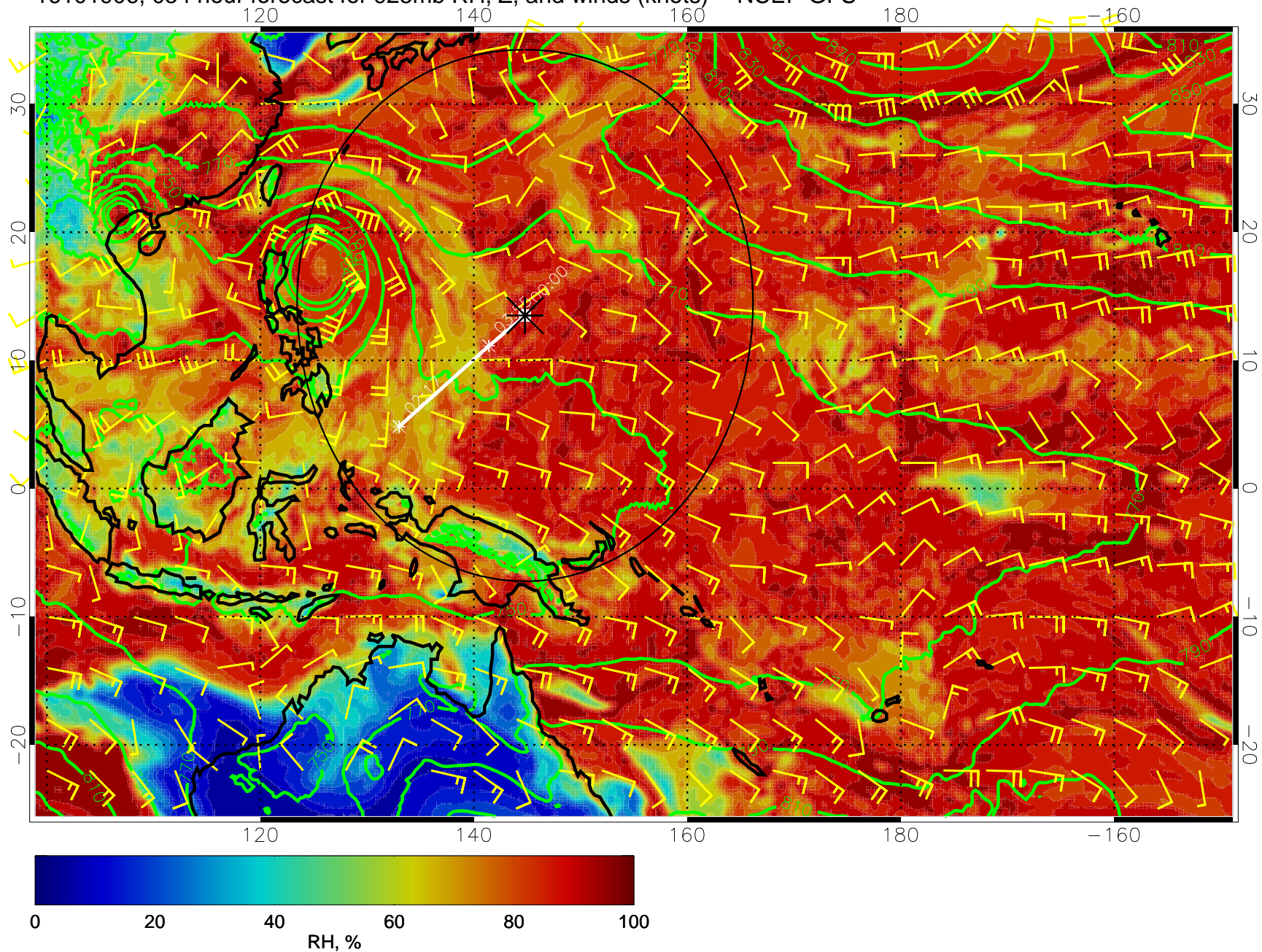
16101906, 054 hour forecast for 925mb RH, Z, and winds (knots) -- NCEP GFS
