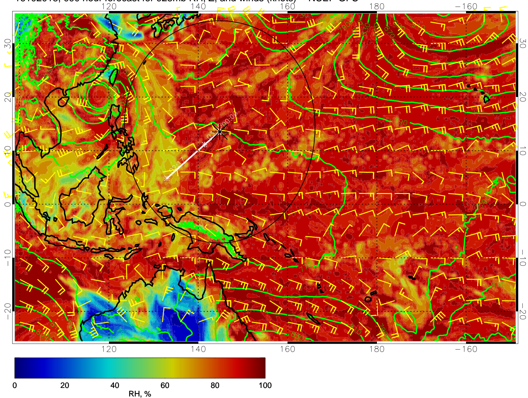
16102018, 090 hour forecast for 925mb RH, Z, and winds (knots) -- NCEP GFS
