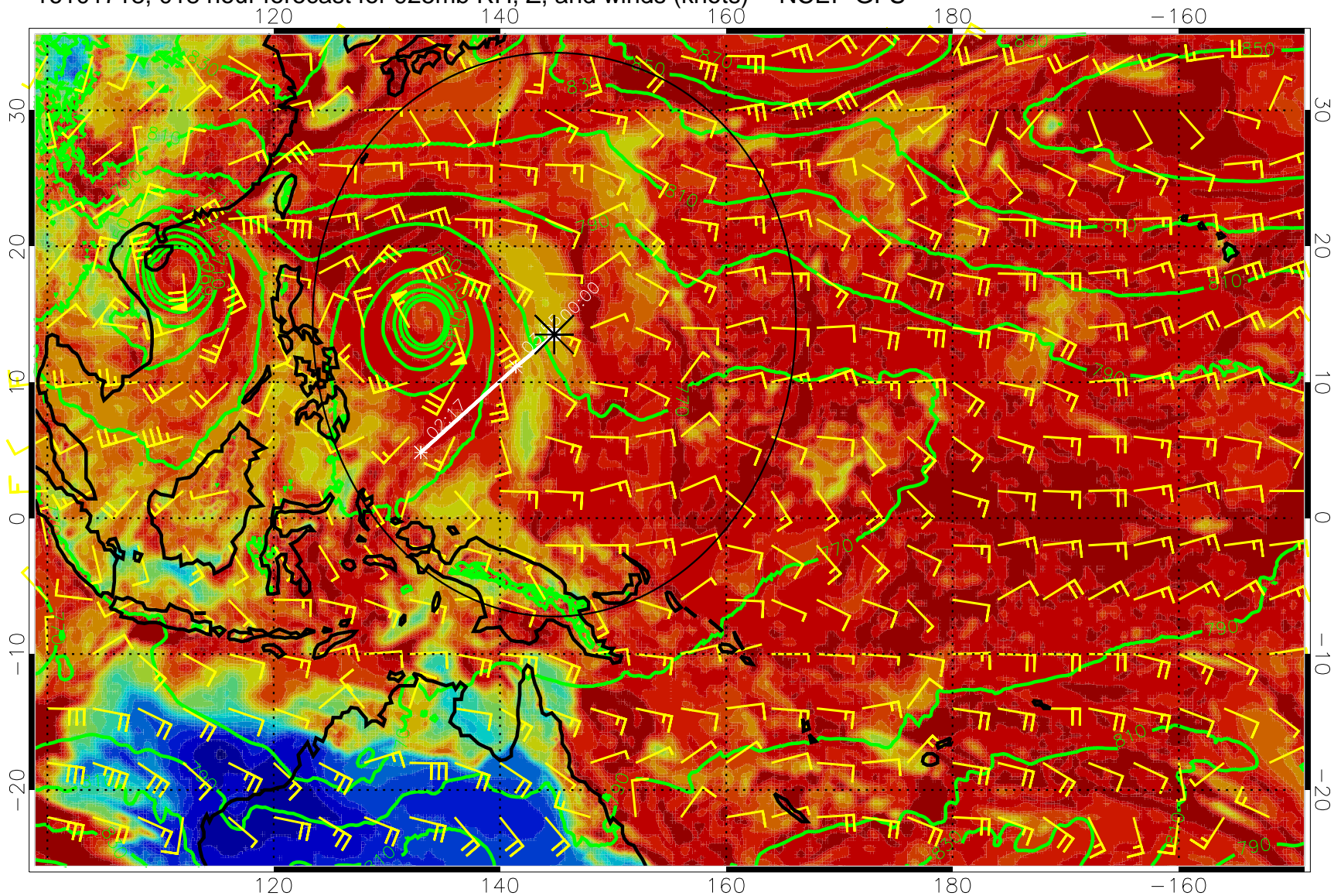
16101718, 018 hour forecast for 925mb RH, Z, and winds (knots) -- NCEP GFS
