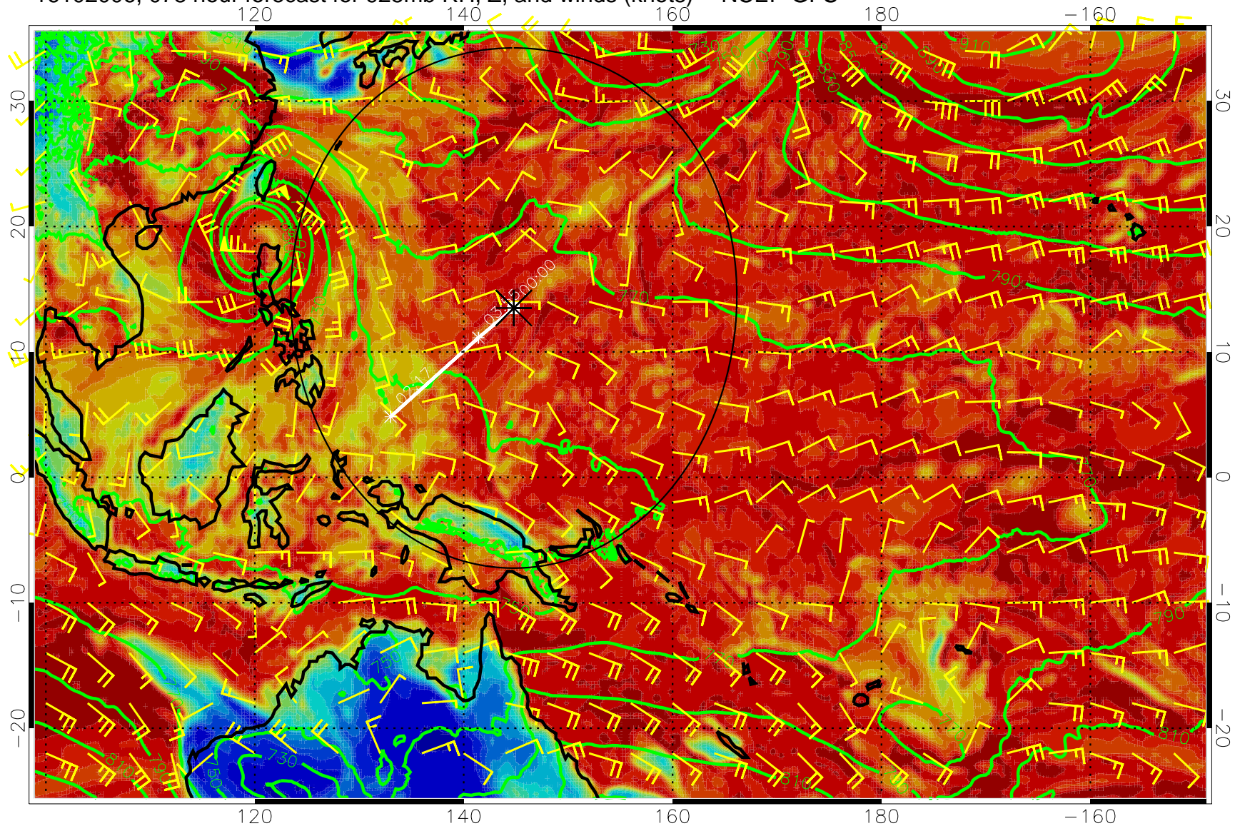
16102006, 078 hour forecast for 925mb RH, Z, and winds (knots) -- NCEP GFS
